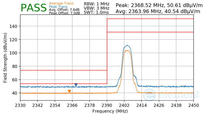
Plot 7-297. Radiated Restricted Lower Band Edge Measurement TxBF
