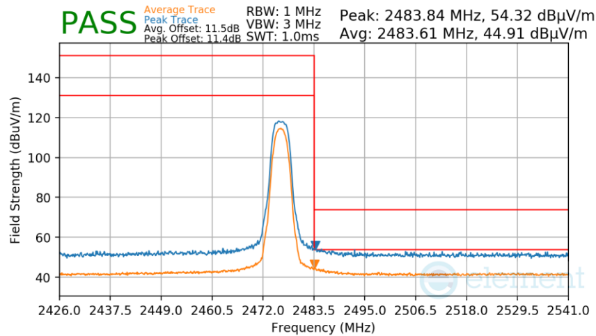
Plot 7-277. Radiated Restricted Upper Band Edge Measurement Antenna 4a
