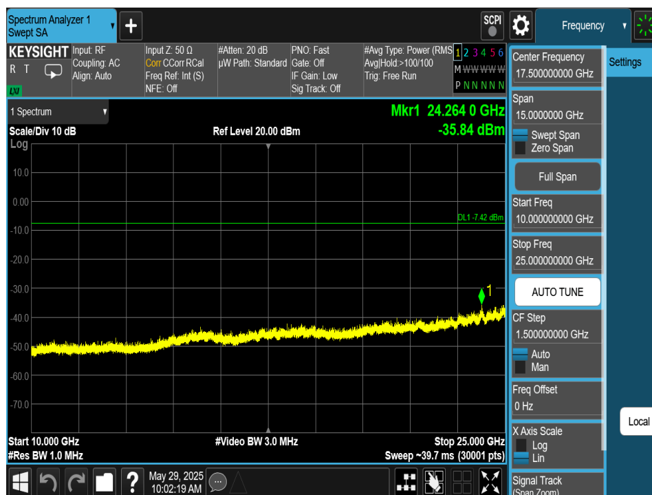
Plot 7-264. Conducted Spurious Plot Antenna 2a (Bluetooth (HDT2), 2Mbps, ePA – Ch. 73)
