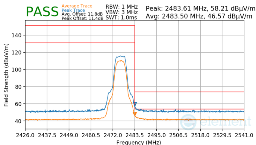
Plot 7-302. Radiated Restricted Upper Band Edge Measurement TxBF
