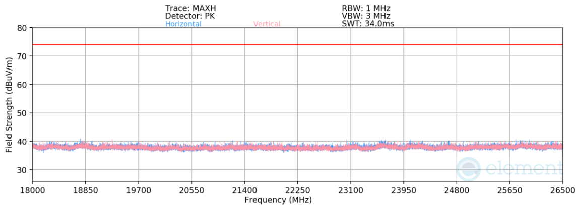
Plot 7-267. Radiated Spurious Emissions above 18GHz TxBF (4Mbps, HDR4, ePA – Ch. 38)
