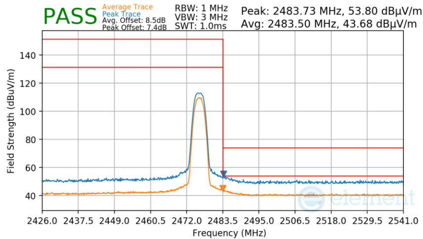
Plot 7-275. Radiated Restricted Upper Band Edge Measurement Antenna 4a
