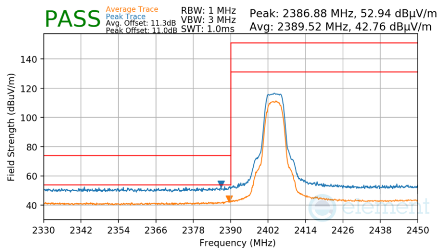
Plot 7-272. Radiated Restricted Lower Band Edge Measurement Antenna 4a
