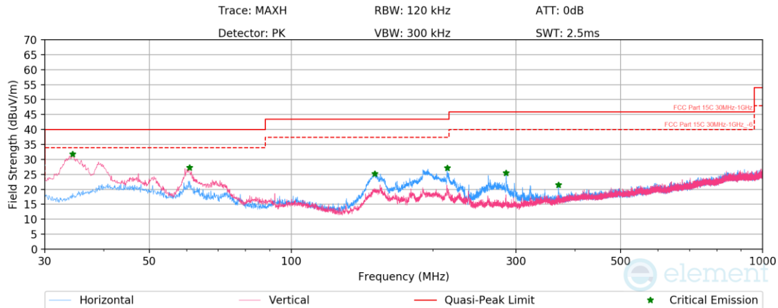
Plot 7-305. Radiated Spurious Emissions Below 1GHz TxBF (HDR4, 4Mbps, ePA – Ch.38 with AC/DC Adapter)
