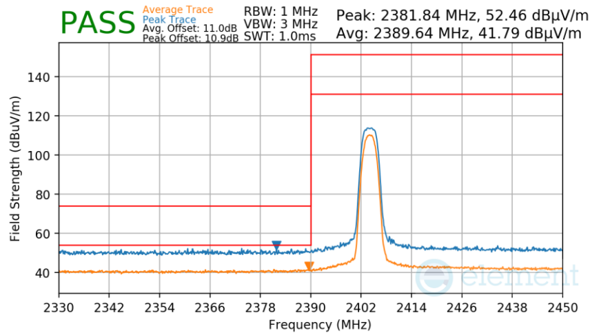
Plot 7-283. Radiated Restricted Lower Band Edge Measurement Antenna 2a
