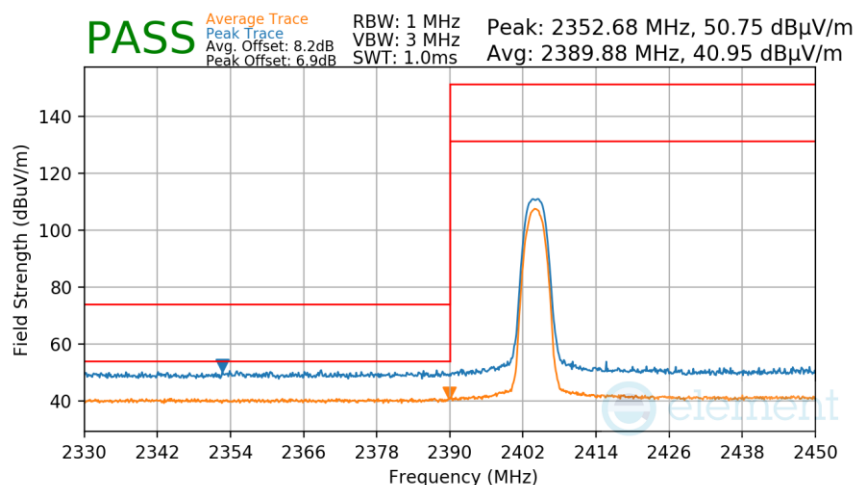
Plot 7-293. Radiated Restricted Lower Band Edge Measurement TxBF
