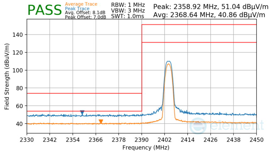
Plot 7-281. Radiated Restricted Lower Band Edge Measurement Antenna 2a
