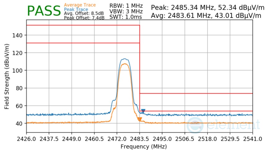
Plot 7-276. Radiated Restricted Upper Band Edge Measurement Antenna 4a
