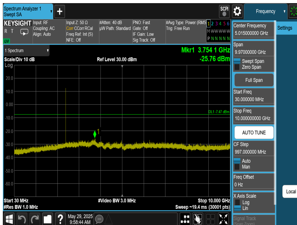
Plot 7-259. Conducted Spurious Plot Antenna 2a (Bluetooth (HDT2), 2Mbps, ePA – Ch. 1)
