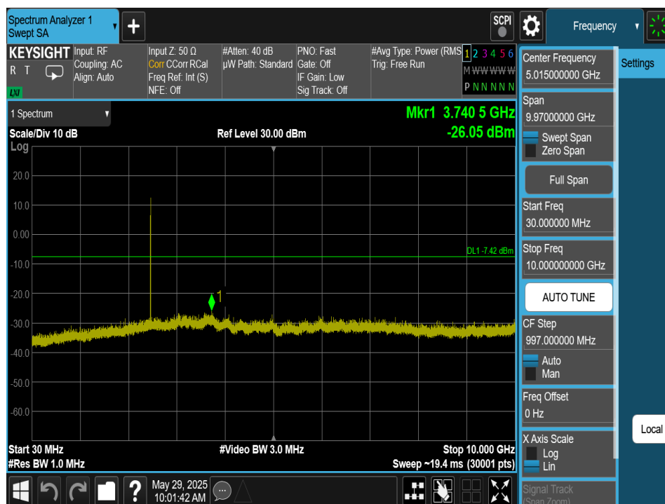
Plot 7-263. Conducted Spurious Plot Antenna 2a (Bluetooth (HDT2), 2Mbps, ePA – Ch. 73)
