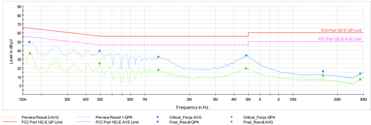
Plot 7-306. AC Line Conducted Plot with Bluetooth HDR TxBF (L1, HDR4, 4Mbps ePA - Ch.38 with AC/DC Adapter)
