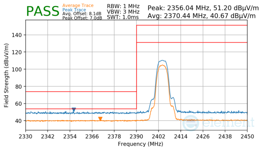
Plot 7-294. Radiated Restricted Lower Band Edge Measurement TxBF
