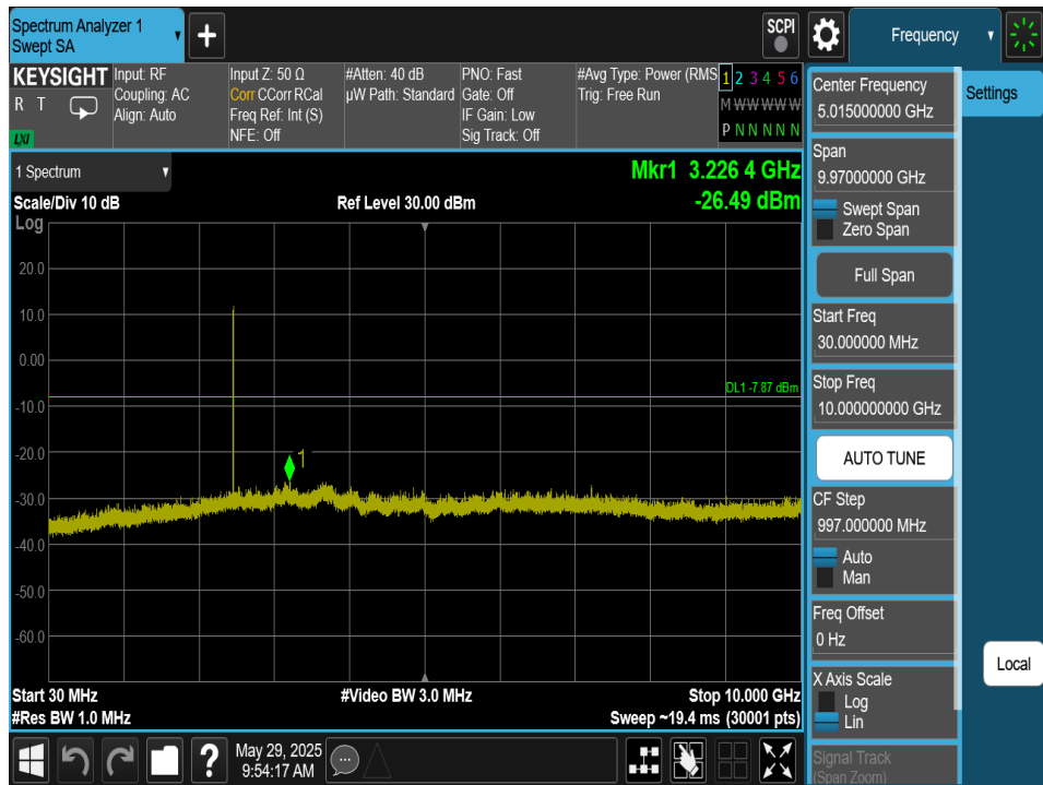
Plot 7-251. Conducted Spurious Plot Antenna 2a (Bluetooth (XHDRPM6), 6Mbps, ePA – Ch. 73)
