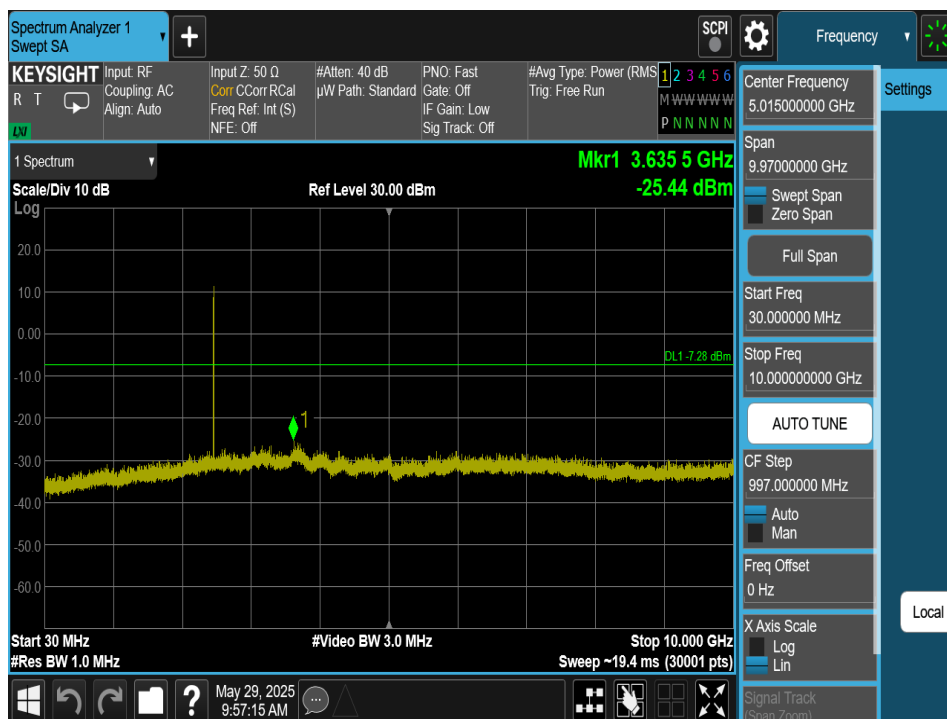
Plot 7-257. Conducted Spurious Plot Antenna 2a (Bluetooth (HDRPM16), 16Mbps, ePA – Ch. 73)
