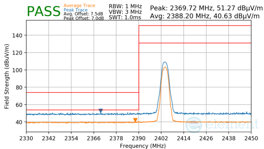
Plot 7-274. Radiated Restricted Lower Band Edge Measurement Antenna 4a
