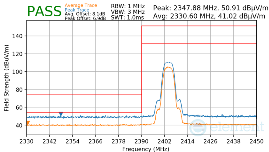
Plot 7-270. Radiated Restricted Lower Band Edge Measurement Antenna 4a
