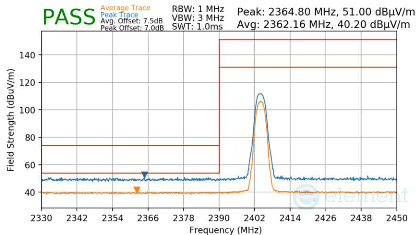
Plot 7-298. Radiated Restricted Lower Band Edge Measurement TxBF
