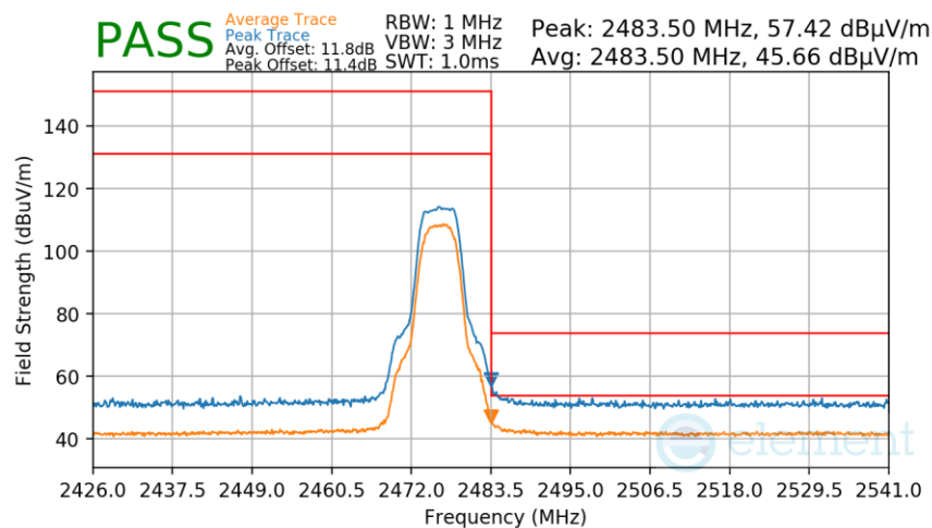
Plot 7-290. Radiated Restricted Upper Band Edge Measurement Antenna 2a
