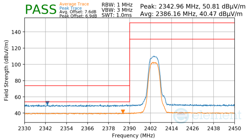
Plot 7-285. Radiated Restricted Lower Band Edge Measurement Antenna 2a
