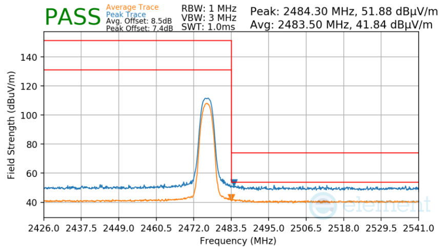
Plot 7-299. Radiated Restricted Upper Band Edge Measurement TxBF
