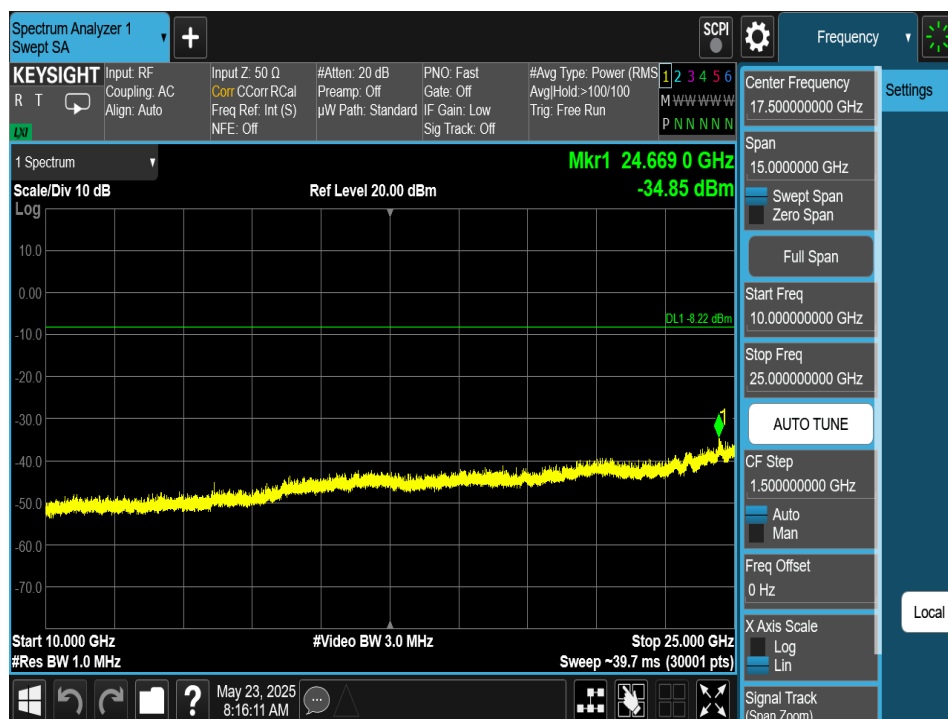
Plot 7-250. Conducted Spurious Plot Antenna 2a (Bluetooth (XHDRPM6), 6Mbps, ePA – Ch. 38)
