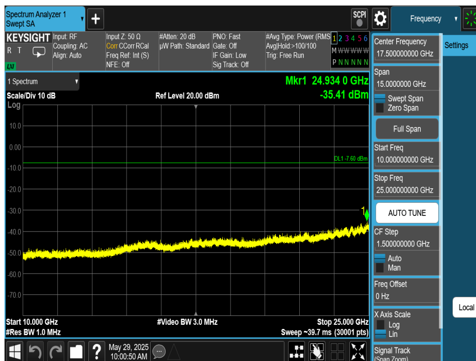
Plot 7-262. Conducted Spurious Plot Antenna 2a (Bluetooth (HDT2), 2Mbps, ePA – Ch. 37)
