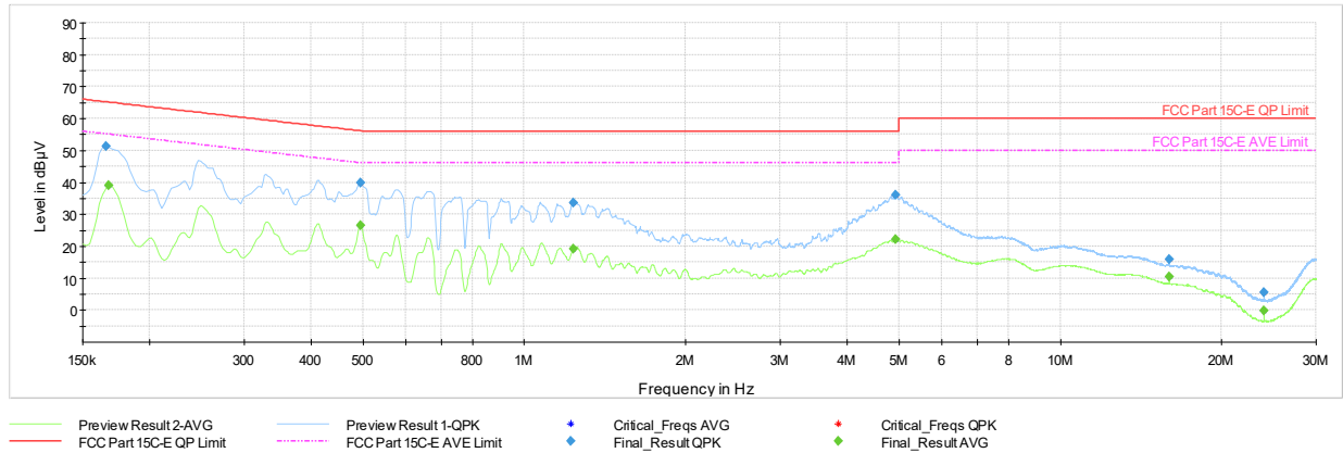
Plot 7-307. AC Line Conducted Plot with Bluetooth HDR (N, HDR4, 4Mbps ePA - Ch.38 with AC/DC Adapter)
