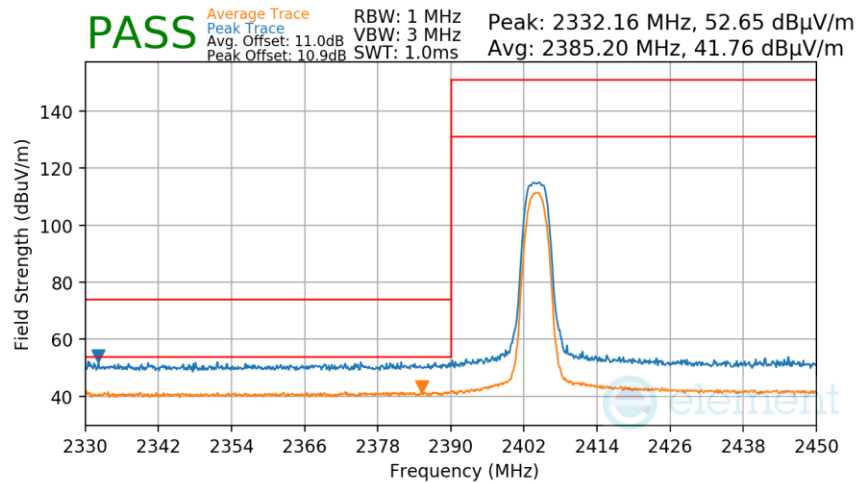
Plot 7-295. Radiated Restricted Lower Band Edge Measurement TxBF
