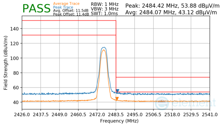
Plot 7-289. Radiated Restricted Upper Band Edge Measurement Antenna 2a
