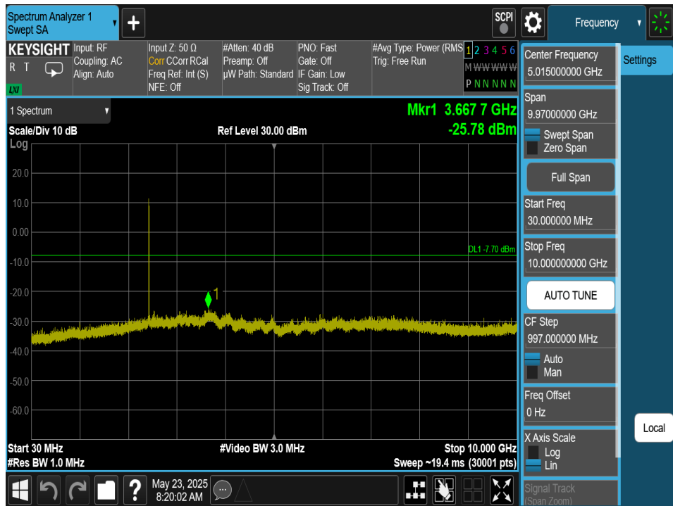
Plot 7-255. Conducted Spurious Plot Antenna 2a (Bluetooth (HDRPM16), 16Mbps, ePA – Ch. 38)
