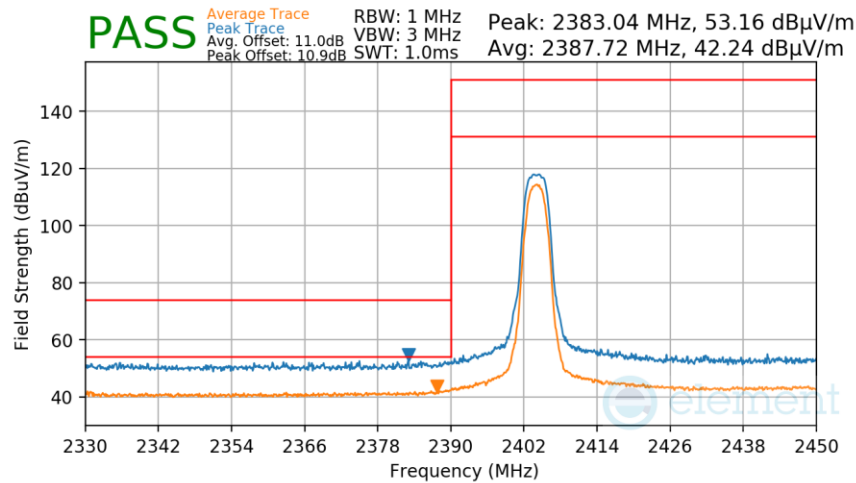
Plot 7-271. Radiated Restricted Lower Band Edge Measurement Antenna 4a
