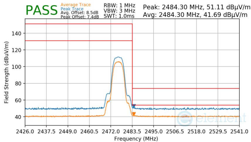
Plot 7-300. Radiated Restricted Upper Band Edge Measurement TxBF
