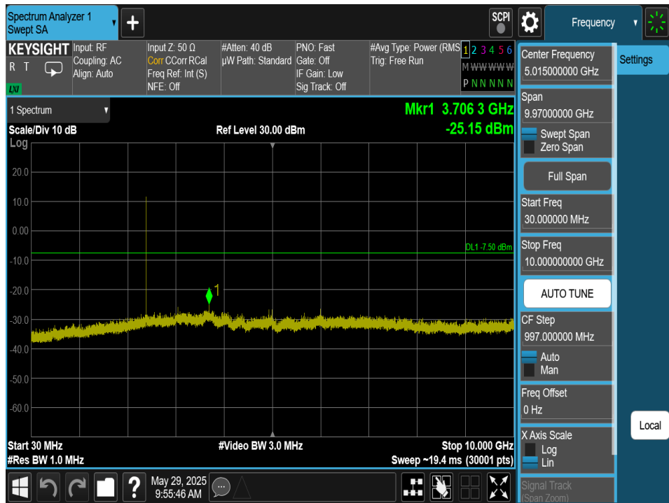
Plot 7-253. Conducted Spurious Plot Antenna 2a (Bluetooth (HDRPM16), 16Mbps, ePA – Ch. 1)
