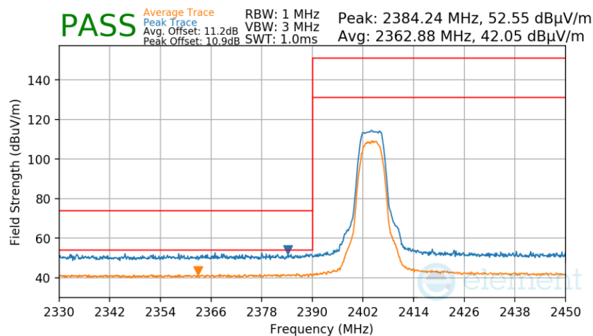
Plot 7-296. Radiated Restricted Lower Band Edge Measurement TxBF
