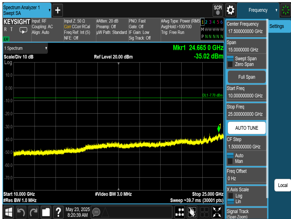
Plot 7-256. Conducted Spurious Plot Antenna 2a (Bluetooth (HDRPM16), 16Mbps, ePA – Ch. 38)
