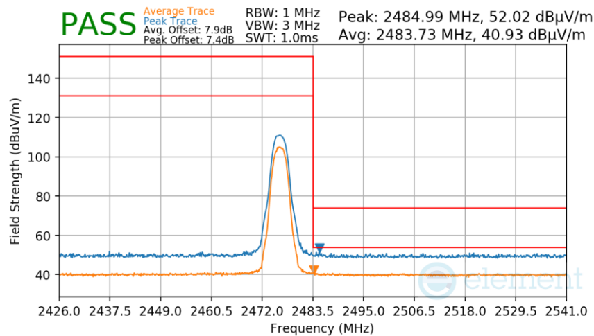
Plot 7-292. Radiated Restricted Upper Band Edge Measurement Antenna 2a
