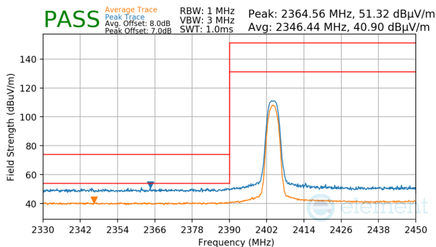
Plot 7-269. Radiated Restricted Lower Band Edge Measurement Antenna 4a
