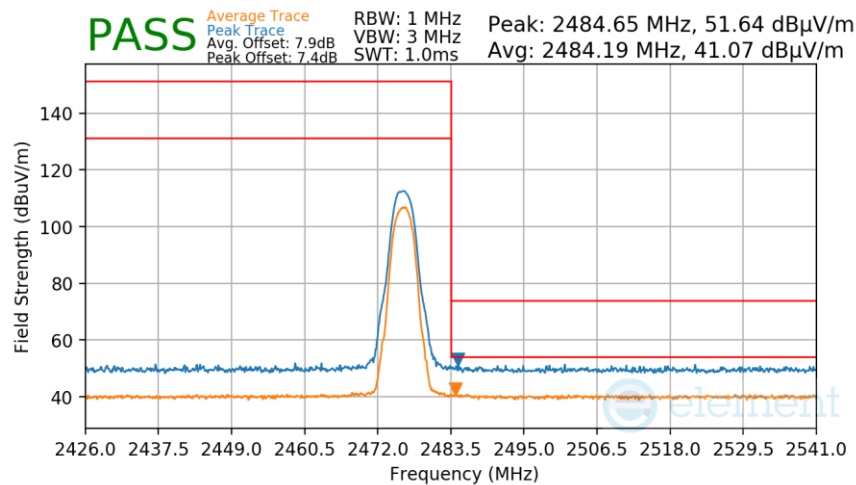
Plot 7-304. Radiated Restricted Upper Band Edge Measurement TxBF
