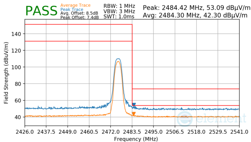
Plot 7-287. Radiated Restricted Upper Band Edge Measurement Antenna 2a
