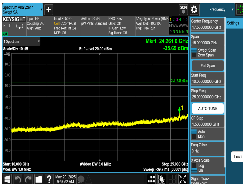
Plot 7-258. Conducted Spurious Plot Antenna 2a (Bluetooth (HDRPM16), 16Mbps, ePA – Ch. 73)
