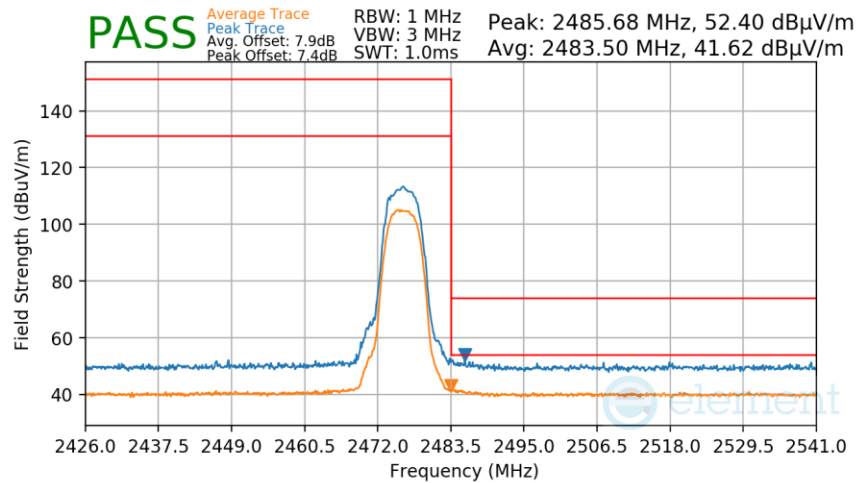
Plot 7-279. Radiated Restricted Upper Band Edge Measurement Antenna 4a
