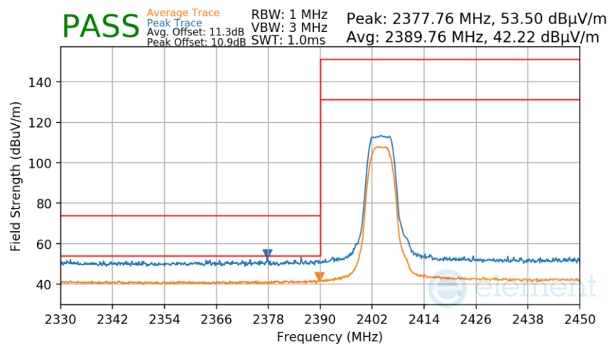
Plot 7-284. Radiated Restricted Lower Band Edge Measurement Antenna 2a
