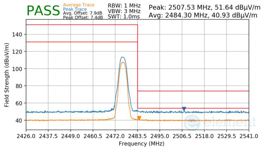
Plot 7-280. Radiated Restricted Upper Band Edge Measurement Antenna 4a
