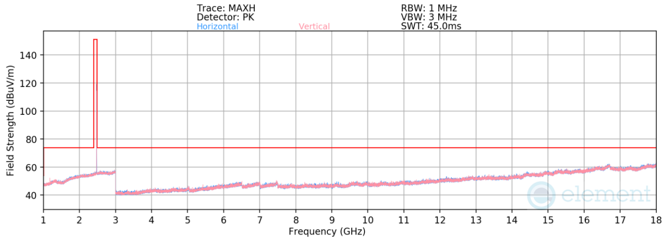
Plot 7-268. Radiated Spurious Emissions above 1GHz TxBF (4Mbps, HDR4, ePA – Ch. 73)
