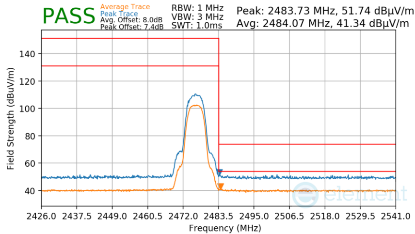
Plot 7-291. Radiated Restricted Upper Band Edge Measurement Antenna 2a
