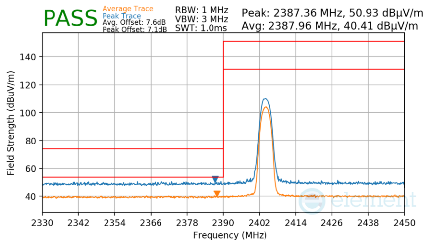
Plot 7-286. Radiated Restricted Lower Band Edge Measurement Antenna 2a
