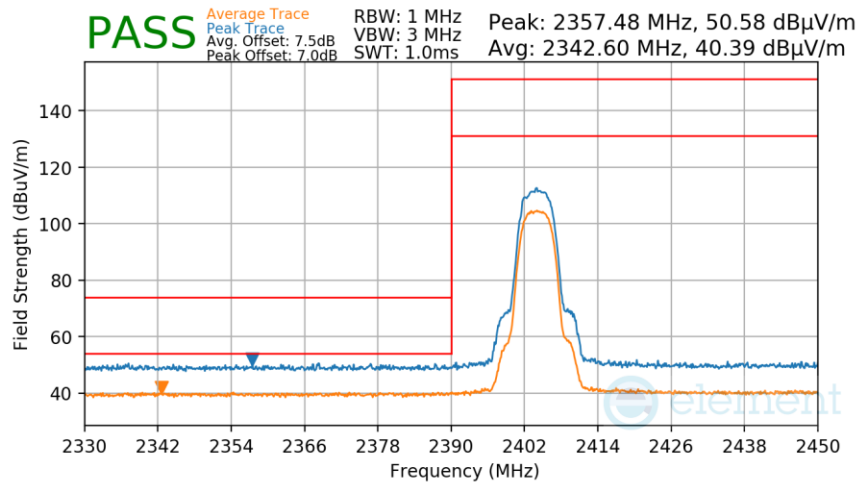
Plot 7-273. Radiated Restricted Lower Band Edge Measurement Antenna 4a
