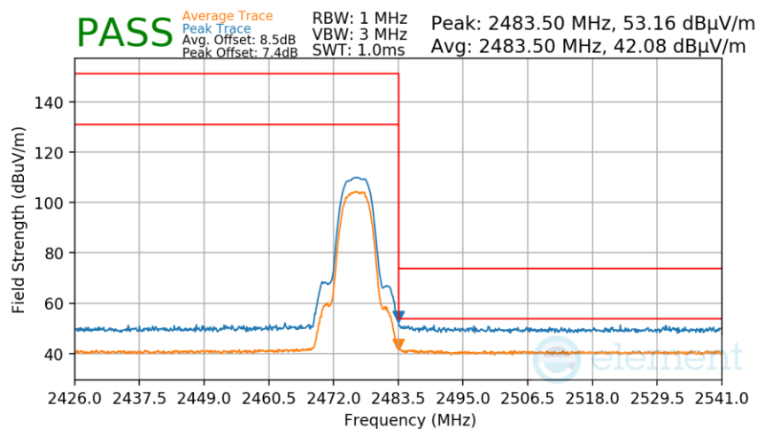
Plot 7-288. Radiated Restricted Upper Band Edge Measurement Antenna 2a
