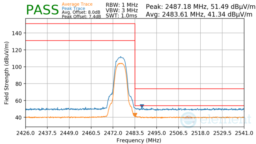
Plot 7-303. Radiated Restricted Upper Band Edge Measurement TxBF
