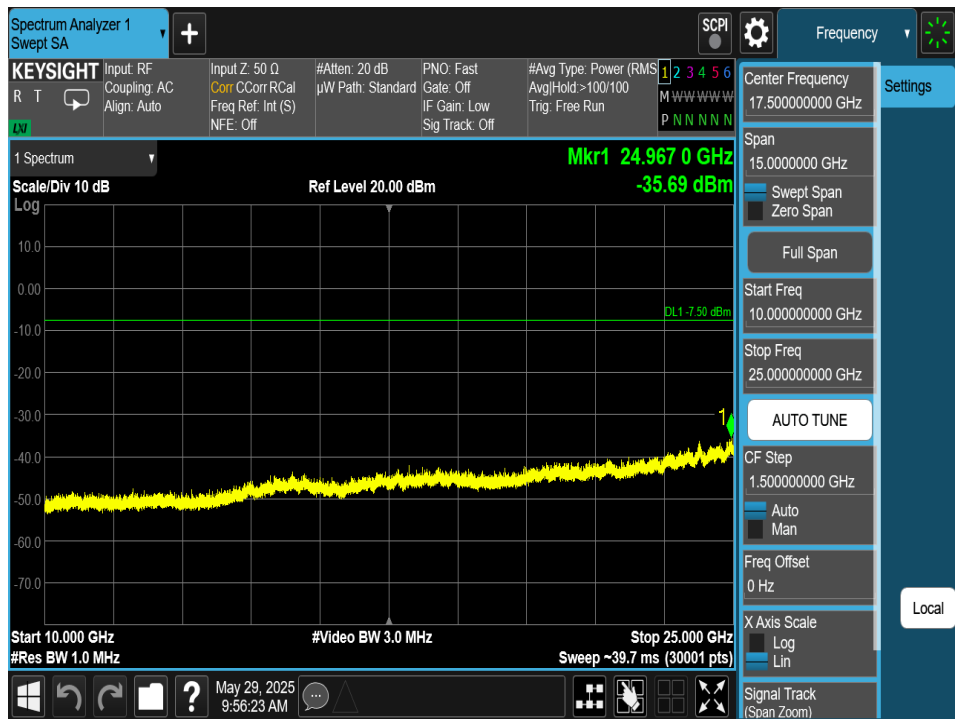
Plot 7-254. Conducted Spurious Plot Antenna 2a (Bluetooth (HDRPM16), 16Mbps, ePA – Ch. 1)
