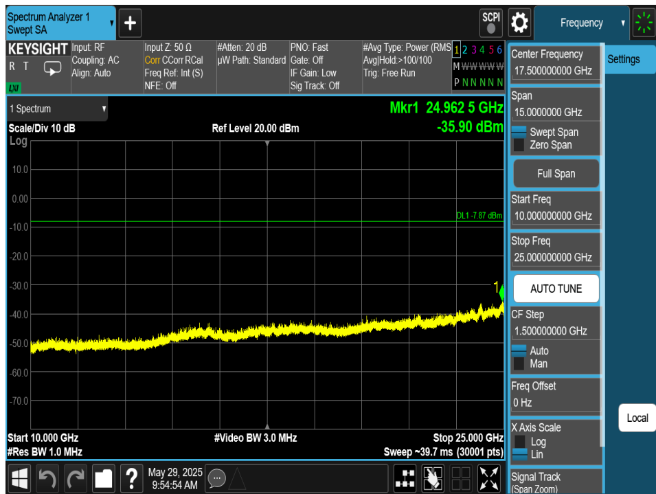
Plot 7-252. Conducted Spurious Plot Antenna 2a (Bluetooth (XHDRPM6), 6Mbps, ePA – Ch. 73)
