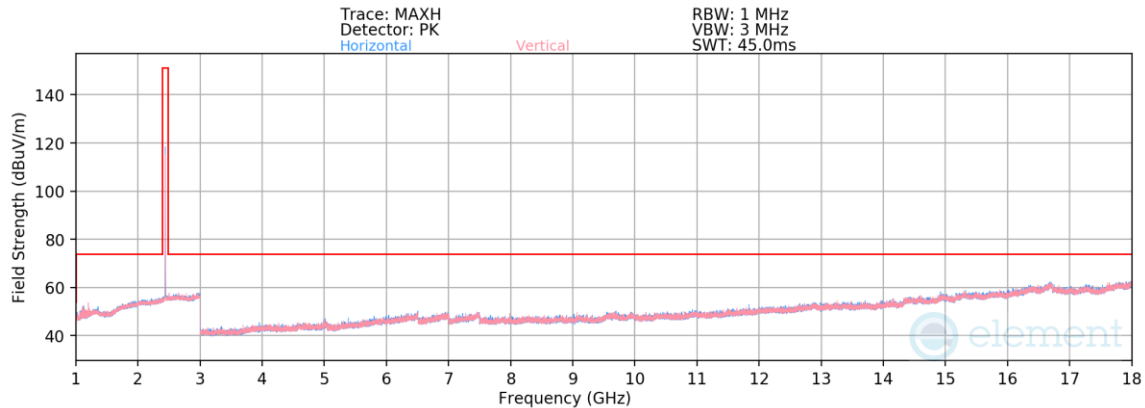
Plot 7-266. Radiated Spurious Emissions above 1GHz TxBF (4Mbps, HDR4, ePA – Ch. 38)
