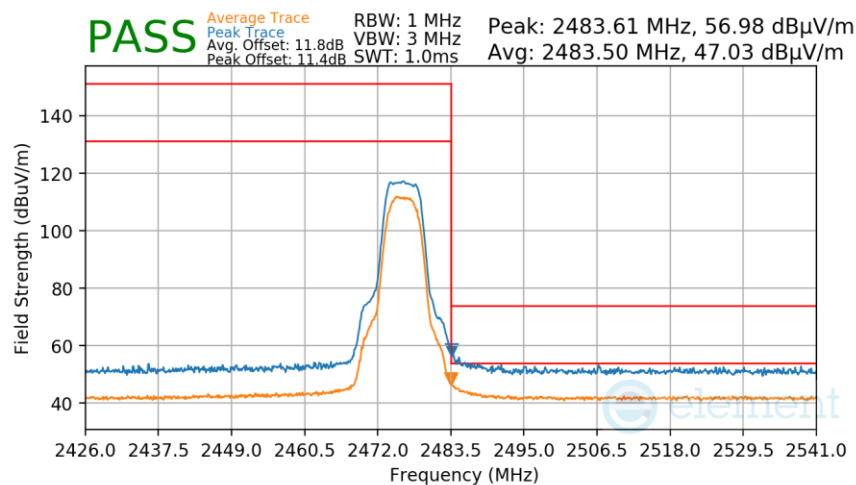
Plot 7-278. Radiated Restricted Upper Band Edge Measurement Antenna 4a
