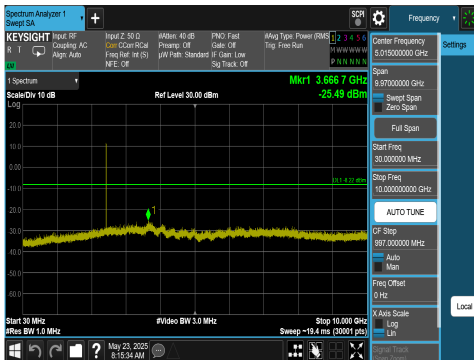
Plot 7-249. Conducted Spurious Plot Antenna 2a (Bluetooth (XHDRPM6), 6Mbps, ePA – Ch. 38)
