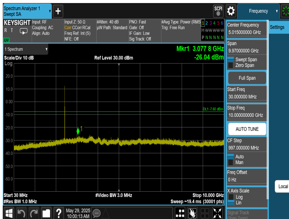
Plot 7-261. Conducted Spurious Plot Antenna 2a (Bluetooth (HDT2), 2Mbps, ePA – Ch. 37)
