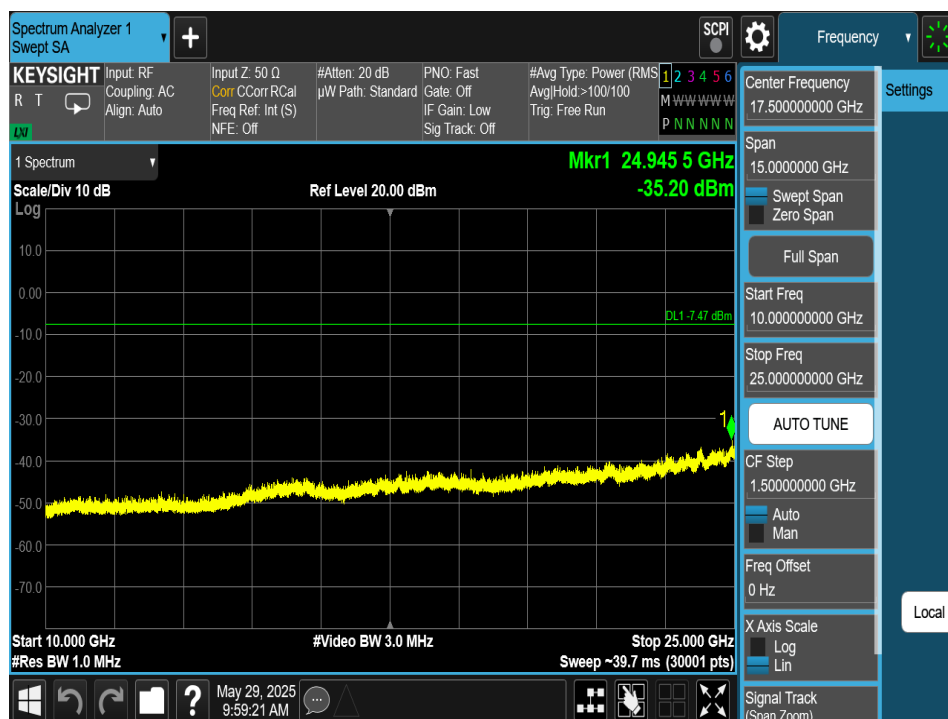
Plot 7-260. Conducted Spurious Plot Antenna 2a (Bluetooth (HDT2), 2Mbps, ePA – Ch. 1)
