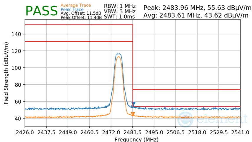
Plot 7-301. Radiated Restricted Upper Band Edge Measurement TxBF
