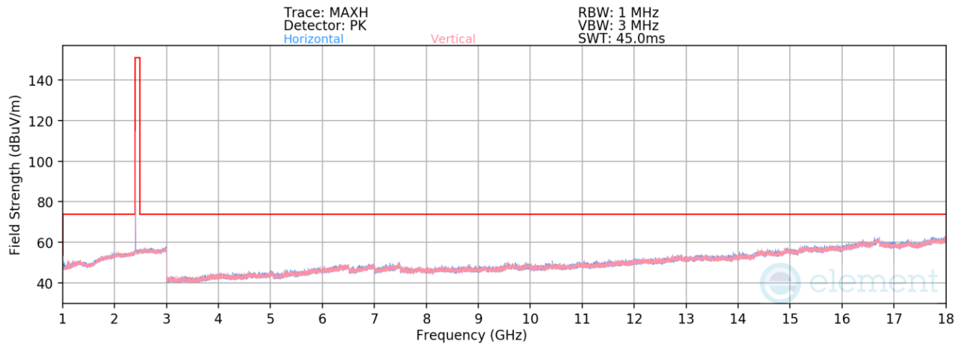
Plot 7-265. Radiated Spurious Emissions above 1GHz TxBF (4Mbps, HDR4, ePA – Ch. 1)
