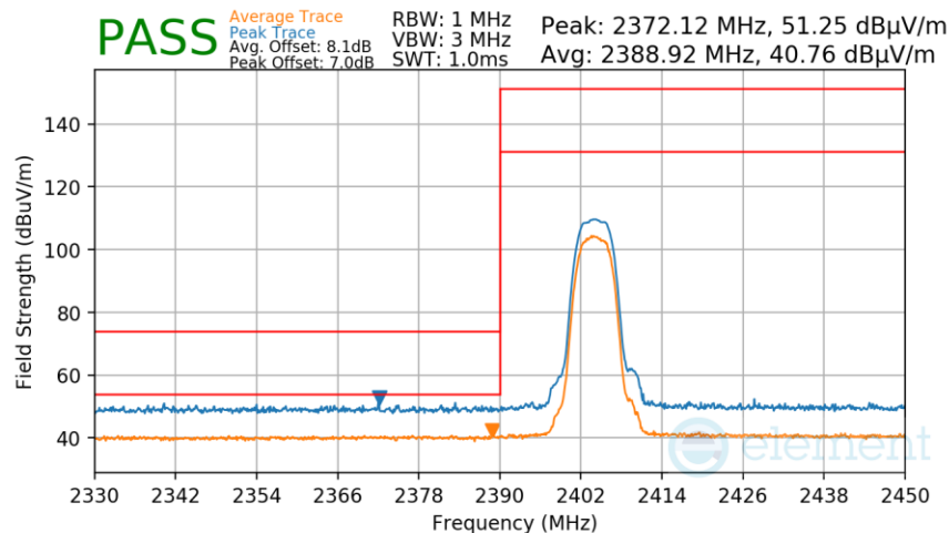
Plot 7-282. Radiated Restricted Lower Band Edge Measurement Antenna 2a
