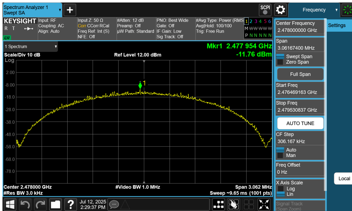
Plot 7-72. Power Spectral Density Plot Antenna 2a (Bluetooth (LE), 2Mbps, iPA – Ch. 38)
