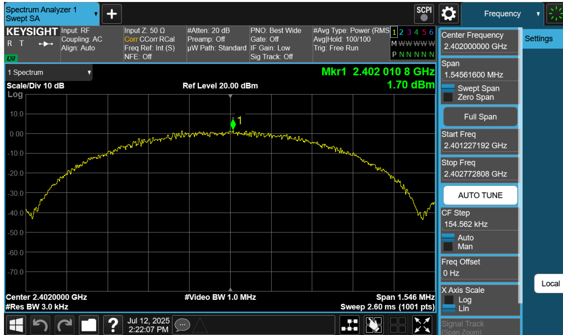
Plot 7-61. Power Spectral Density Plot Antenna 2a (Bluetooth (LE), 1Mbps, ePA – Ch. 0)
