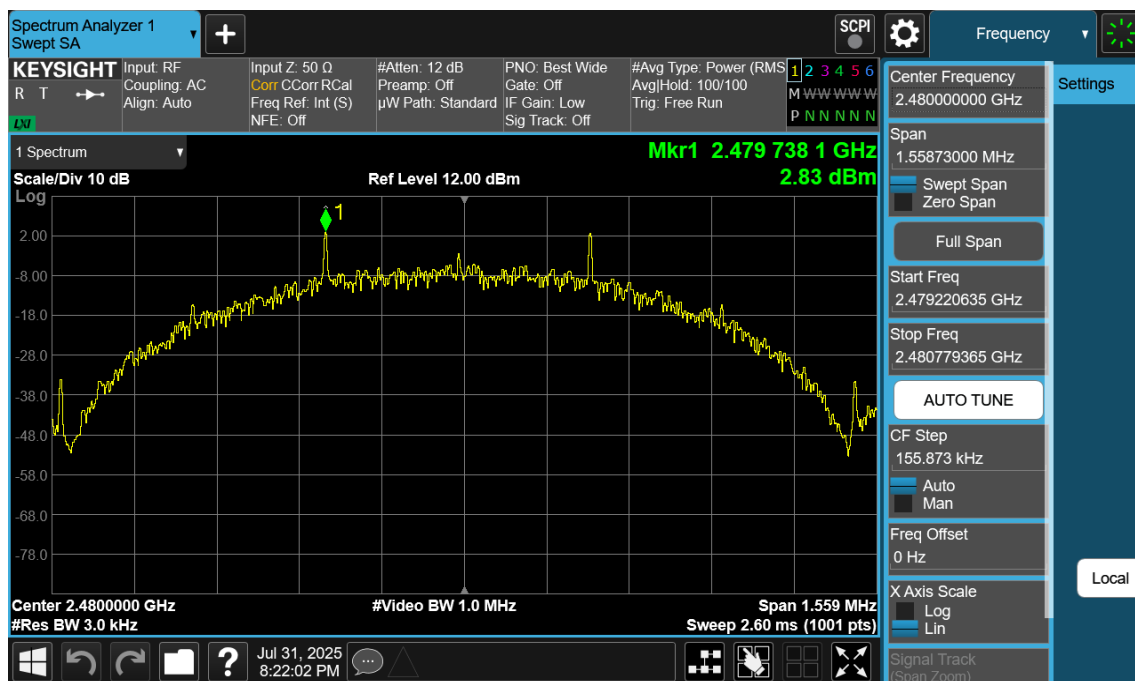
Plot 7-90. Power Spectral Density Plot Antenna 2a (Bluetooth (LE), 500kbps, ePA – Ch. 39)
