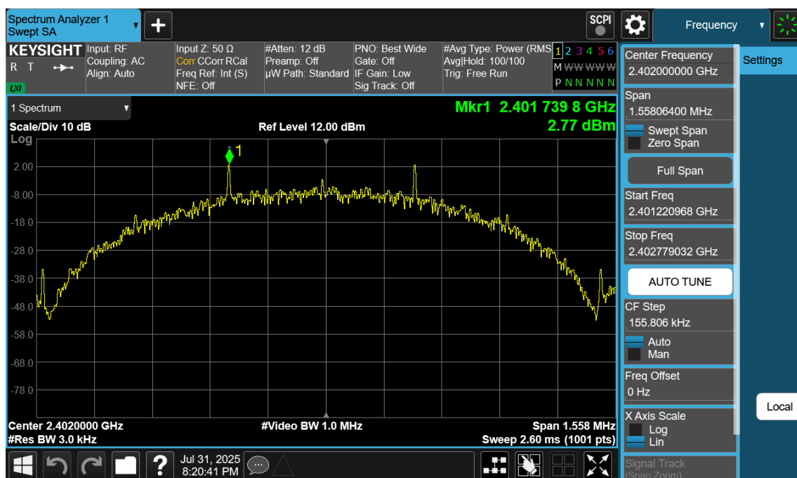
Plot 7-86. Power Spectral Density Plot Antenna 2a (Bluetooth (LE), 500kbps, ePA – Ch. 0)
