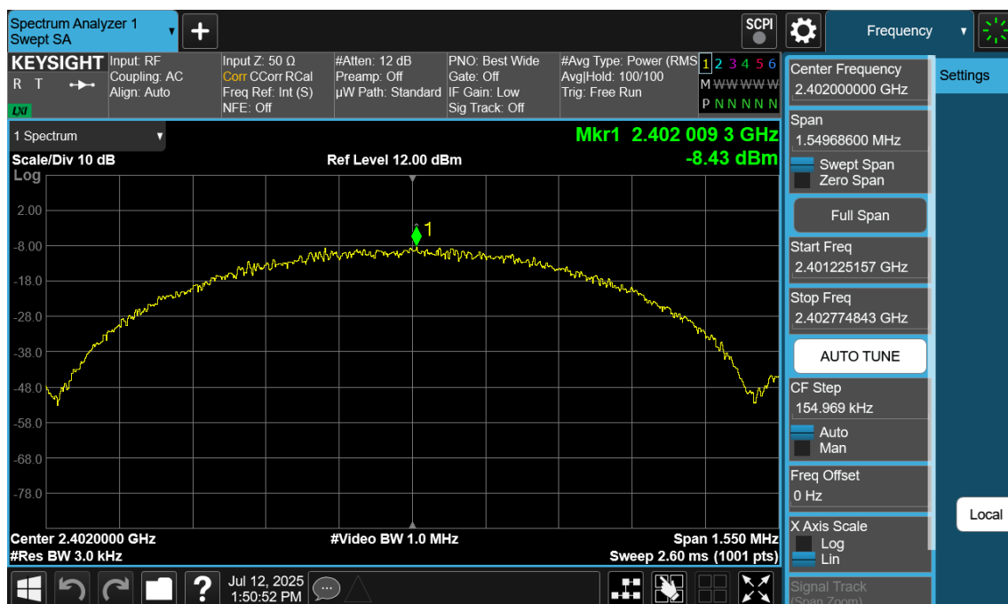
Plot 7-103. Power Spectral Density Plot Antenna 4a (Bluetooth (LE), 1Mbps, iPA – Ch. 0)
