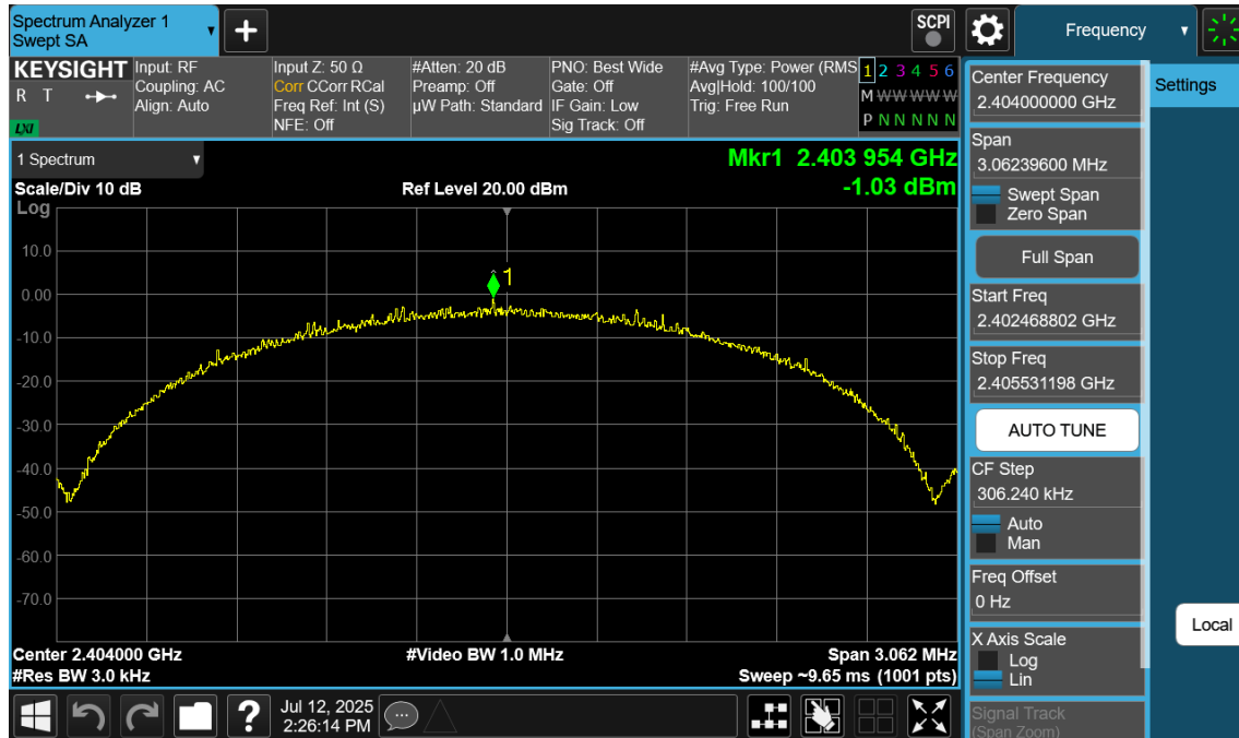
Plot 7-67. Power Spectral Density Plot Antenna 2a (Bluetooth (LE), 2Mbps, ePA – Ch. 1)
