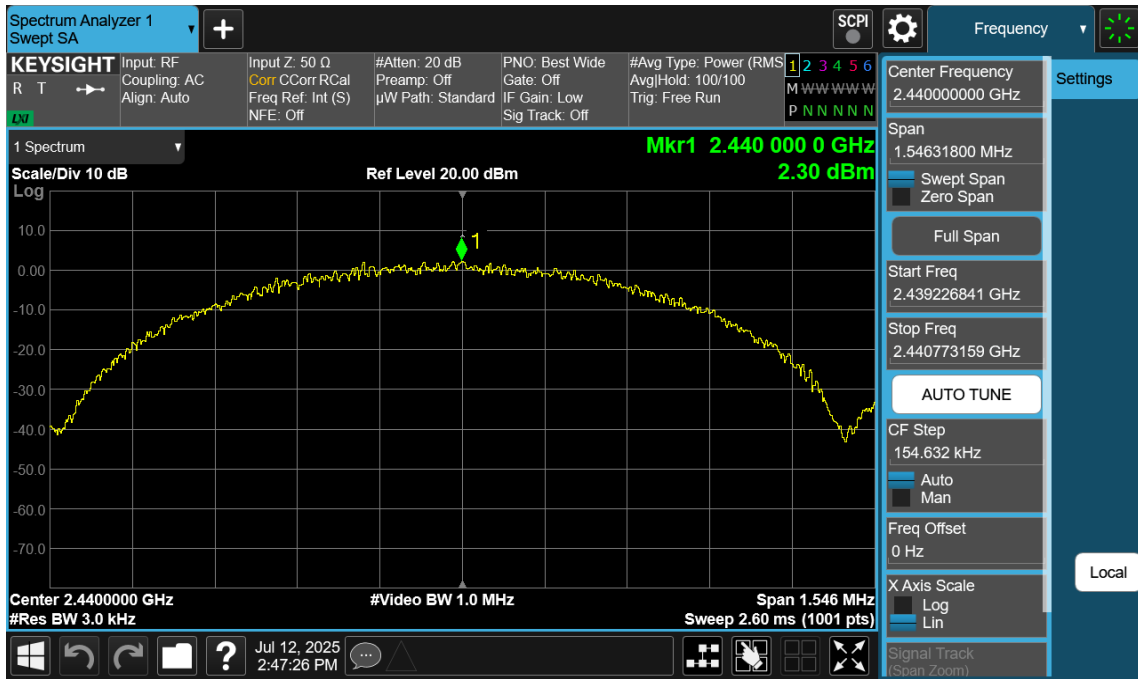
Plot 7-100. Power Spectral Density Plot Antenna 2a (Bluetooth (LE), 1Mbps, ePA – Ch. 19)
