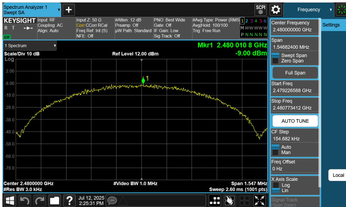
Plot 7-66. Power Spectral Density Plot Antenna 2a (Bluetooth (LE), 1Mbps, iPA – Ch. 39)
