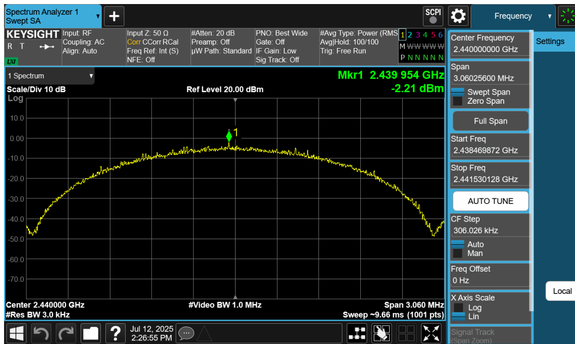
Plot 7-68. Power Spectral Density Plot Antenna 2a (Bluetooth (LE), 2Mbps, ePA – Ch. 19)
