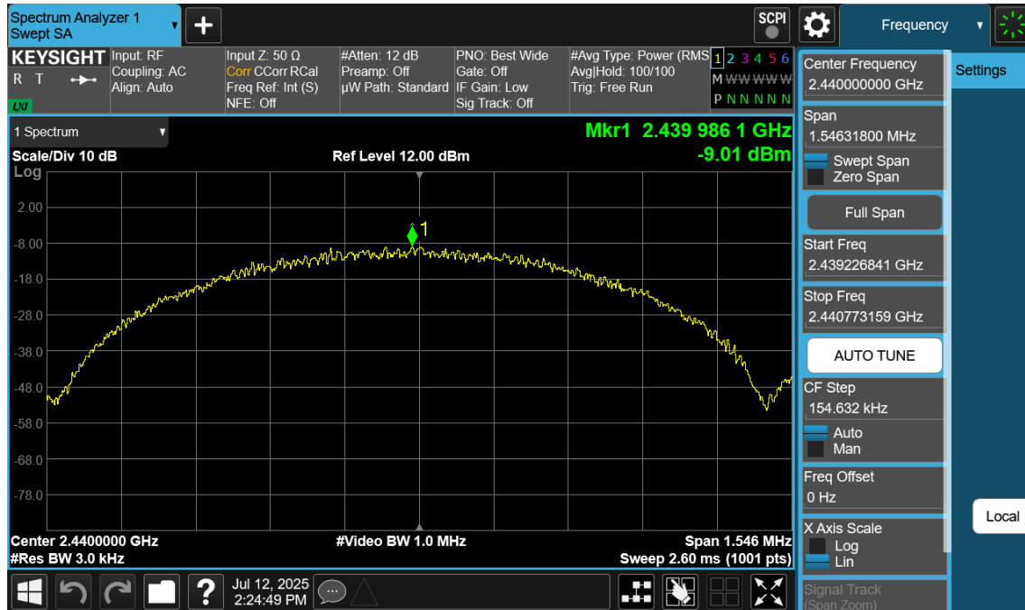
Plot 7-65. Power Spectral Density Plot Antenna 2a (Bluetooth (LE), 1Mbps, iPA – Ch. 19)
