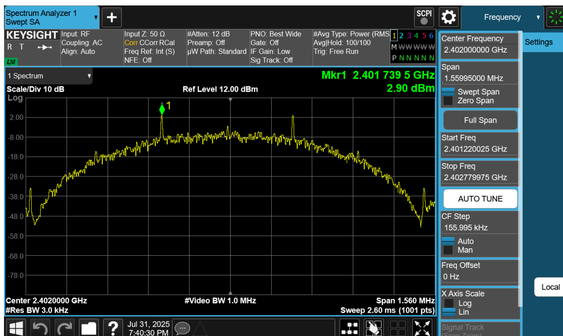
Plot 7-85. Power Spectral Density Plot Antenna 4a (Bluetooth (LE), 500kbps, ePA – Ch. 0)
