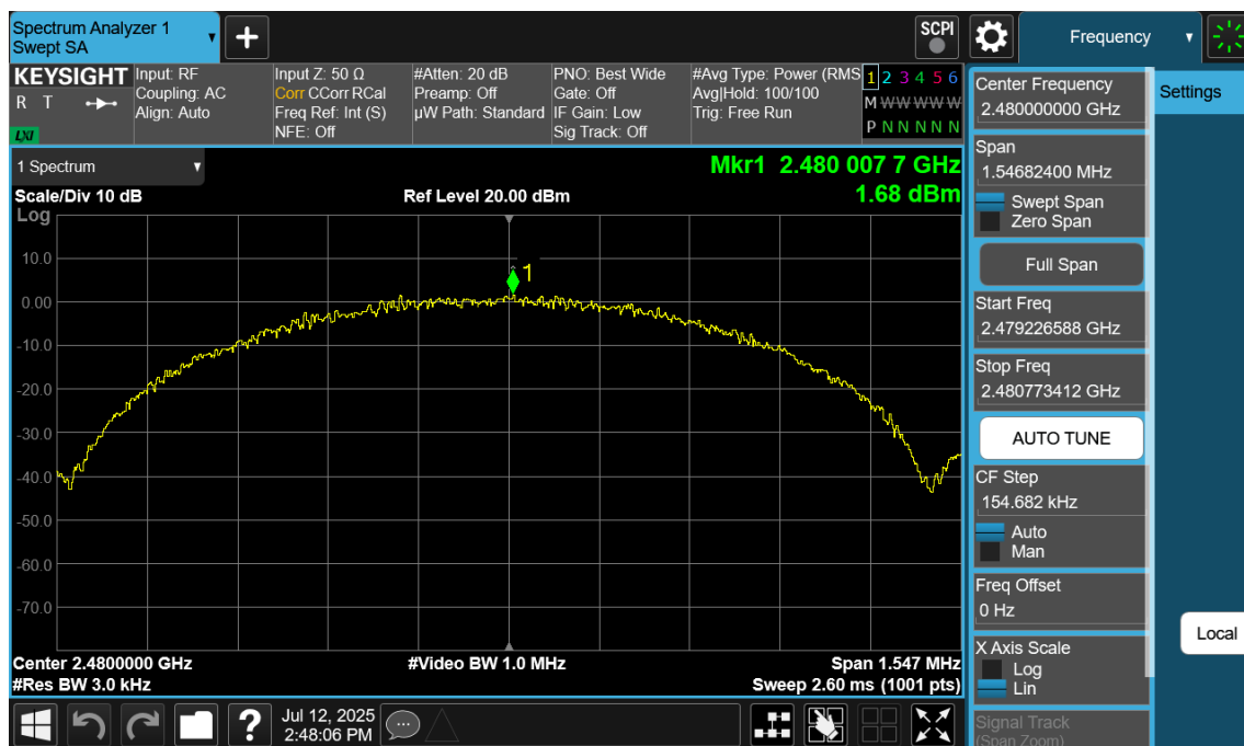
Plot 7-102. Power Spectral Density Plot Antenna 2a (Bluetooth (LE), 1Mbps, ePA – Ch. 39)
