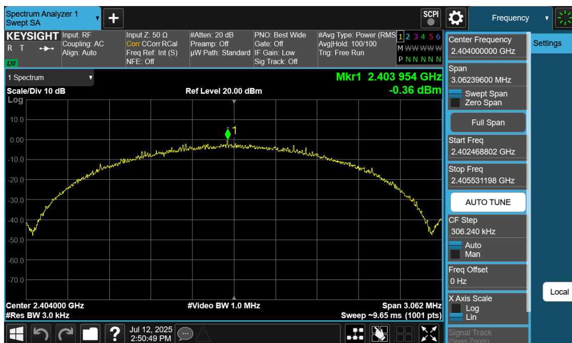
Plot 7-110. Power Spectral Density Plot Antenna 2a (Bluetooth (LE), 2Mbps, ePA – Ch. 1)
