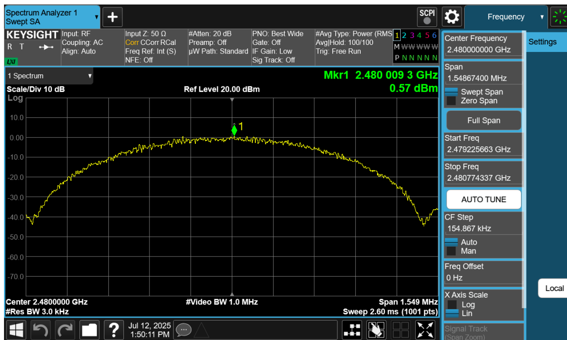
Plot 7-101. Power Spectral Density Plot Antenna 4a (Bluetooth (LE), 1Mbps, ePA – Ch. 39)
