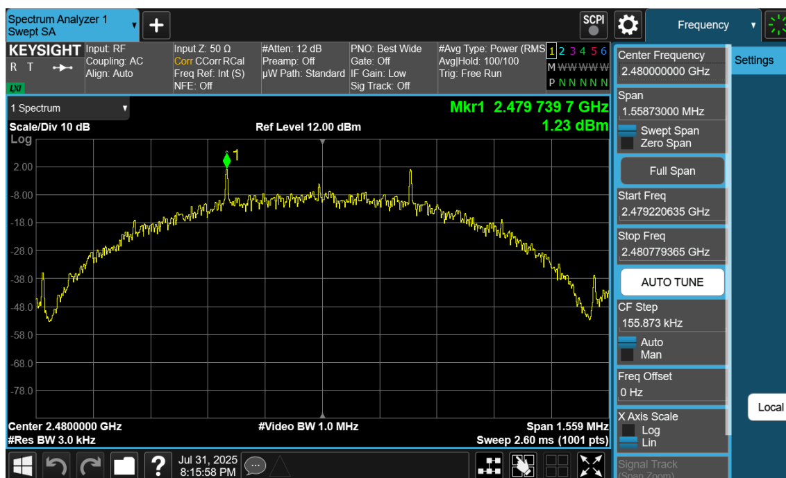
Plot 7-60. Power Spectral Density Plot Antenna 2a (Bluetooth (LE), 500kbps, iPA – Ch. 39)
