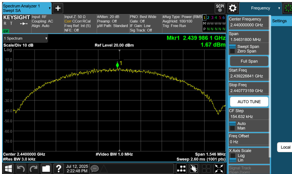
Plot 7-62. Power Spectral Density Plot Antenna 2a (Bluetooth (LE), 1Mbps, ePA – Ch. 19)
