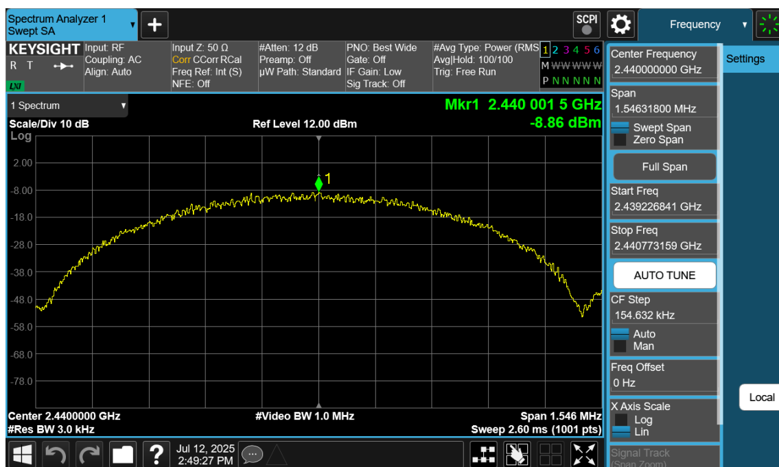
Plot 7-106. Power Spectral Density Plot Antenna 2a (Bluetooth (LE), 1Mbps, iPA – Ch. 19)
