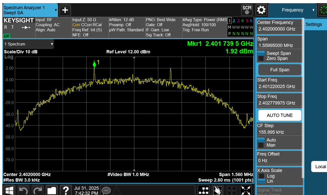
Plot 7-91. Power Spectral Density Plot Antenna 4a (Bluetooth (LE), 500kbps, iPA – Ch. 0)
