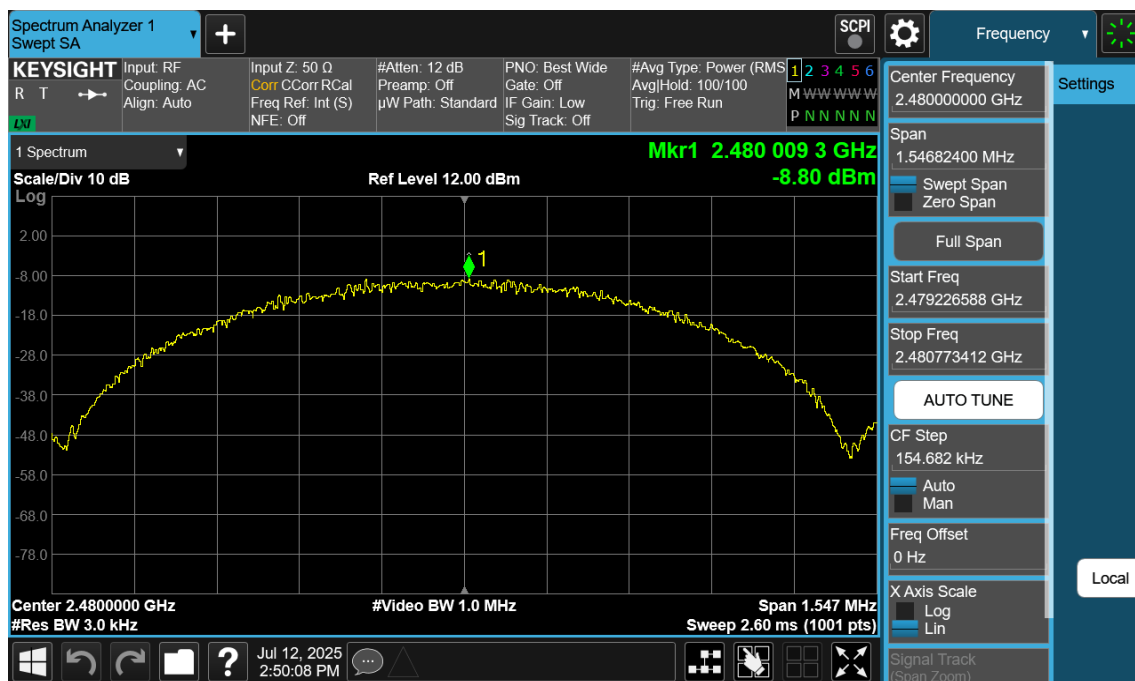
Plot 7-108. Power Spectral Density Plot Antenna 2a (Bluetooth (LE), 1Mbps, iPA – Ch. 39)
