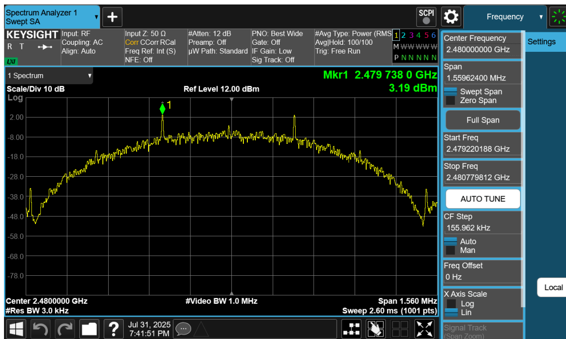
Plot 7-89. Power Spectral Density Plot Antenna 4a (Bluetooth (LE), 500kbps, ePA – Ch. 39)
