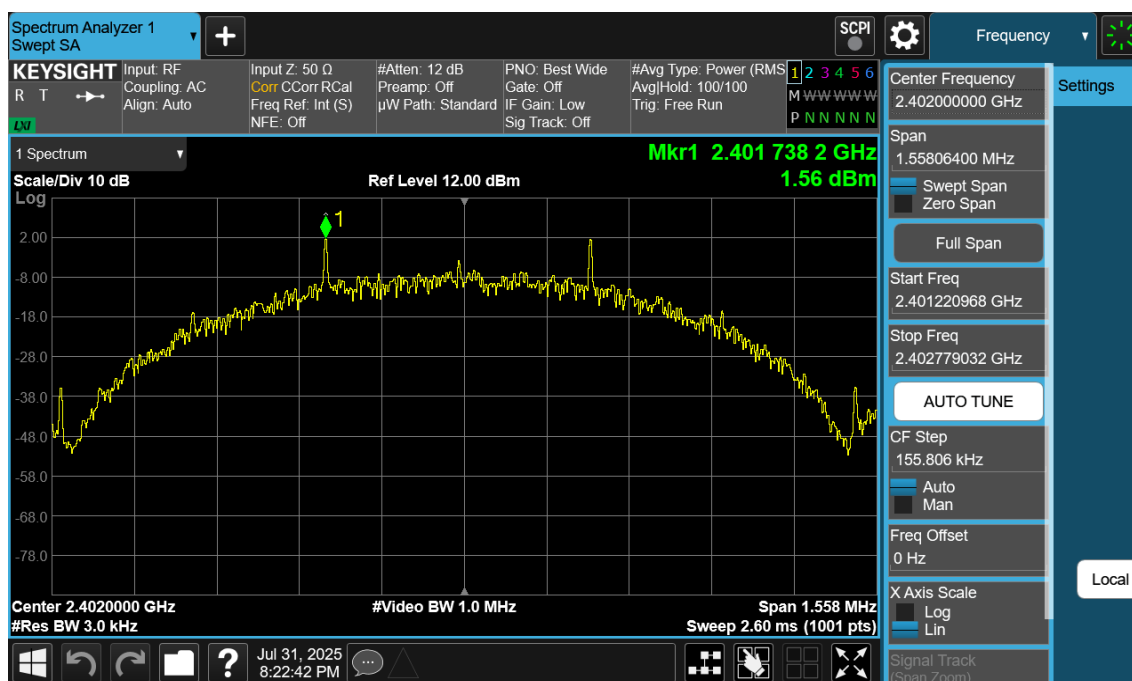
Plot 7-92. Power Spectral Density Plot Antenna 2a (Bluetooth (LE), 500kbps, iPA – Ch. 0)
