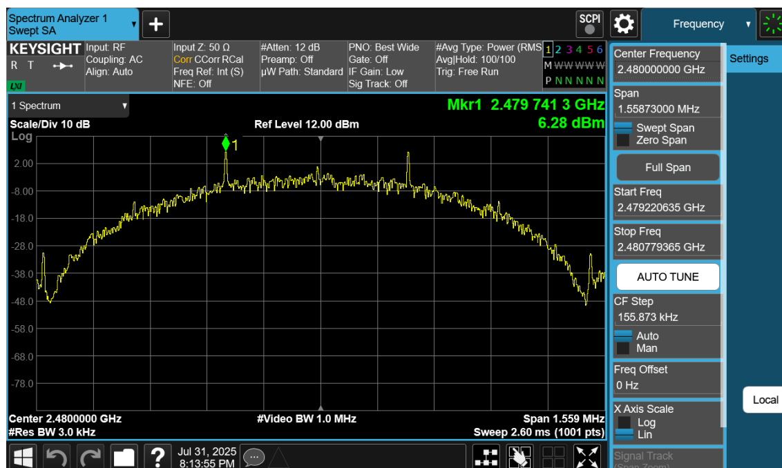
Plot 7-57. Power Spectral Density Plot Antenna 2a (Bluetooth (LE), 500kbps, ePA – Ch. 39)
