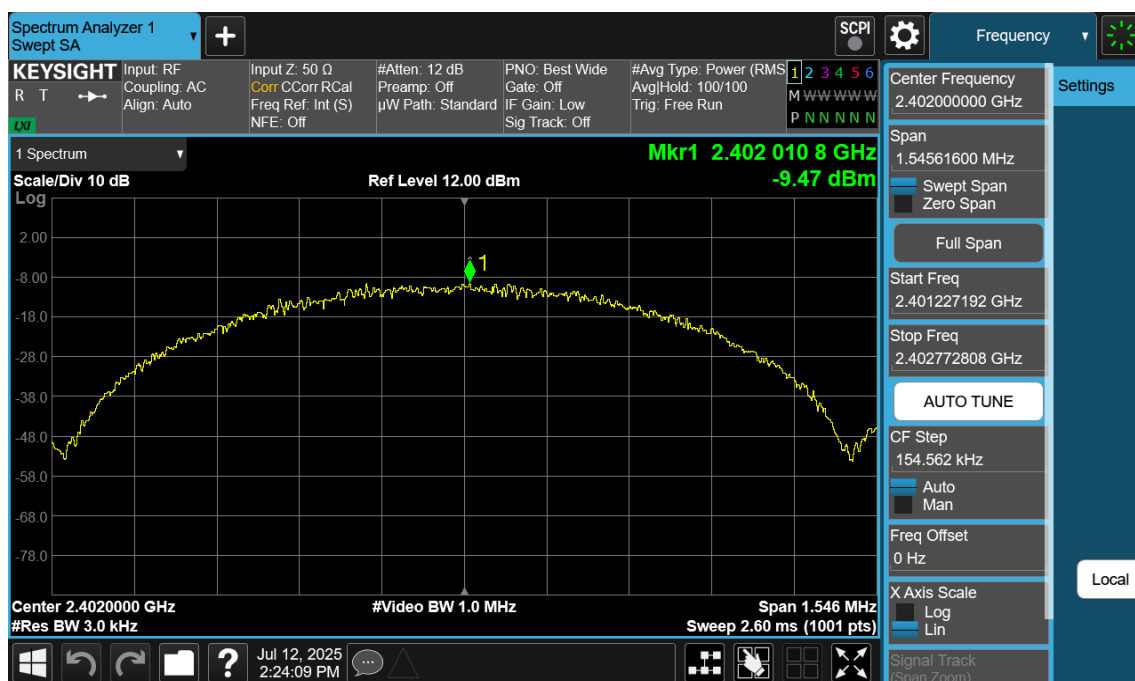
Plot 7-64. Power Spectral Density Plot Antenna 2a (Bluetooth (LE), 1Mbps, iPA – Ch. 0)
