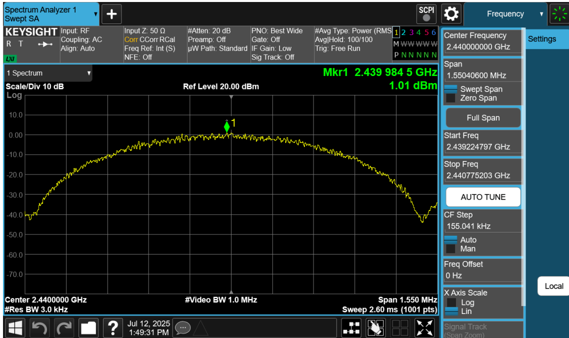
Plot 7-99. Power Spectral Density Plot Antenna 4a (Bluetooth (LE), 1Mbps, ePA – Ch. 19)
