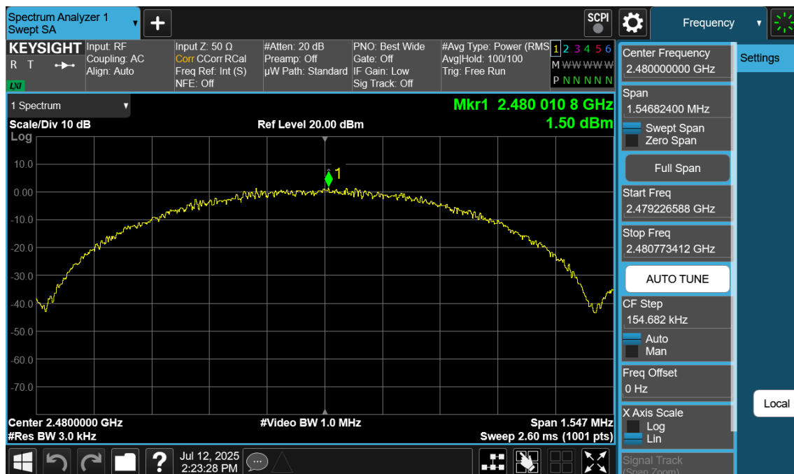
Plot 7-63. Power Spectral Density Plot Antenna 2a (Bluetooth (LE), 1Mbps, ePA – Ch. 39)
