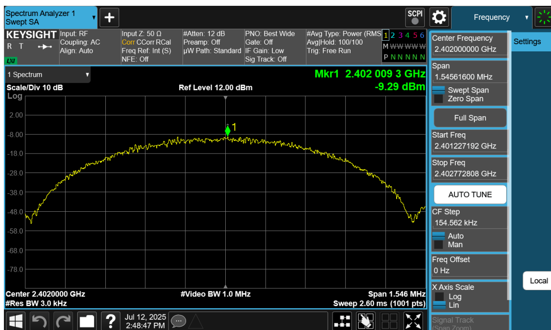
Plot 7-104. Power Spectral Density Plot Antenna 2a (Bluetooth (LE), 1Mbps, iPA – Ch. 0)
