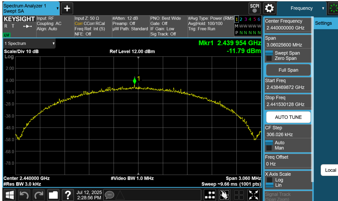
Plot 7-71. Power Spectral Density Plot Antenna 2a (Bluetooth (LE), 2Mbps, iPA – Ch. 19)
