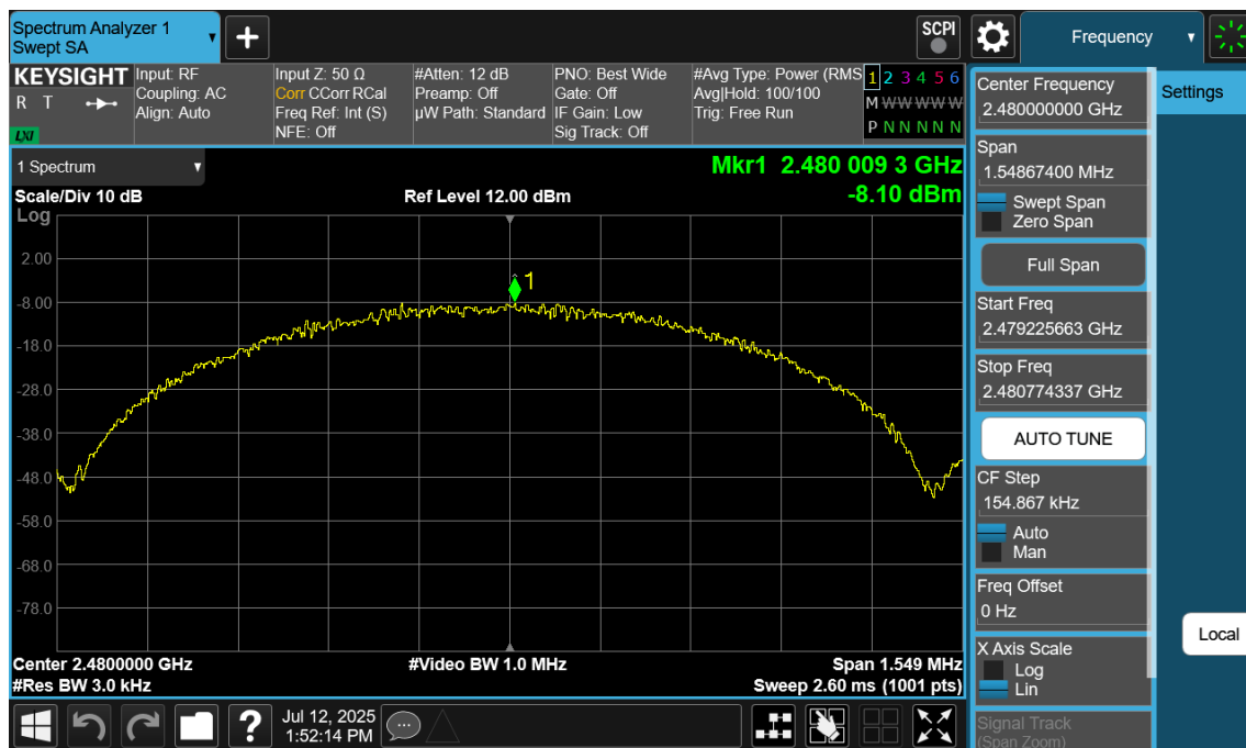
Plot 7-107. Power Spectral Density Plot Antenna 4a (Bluetooth (LE), 1Mbps, iPA – Ch. 39)
