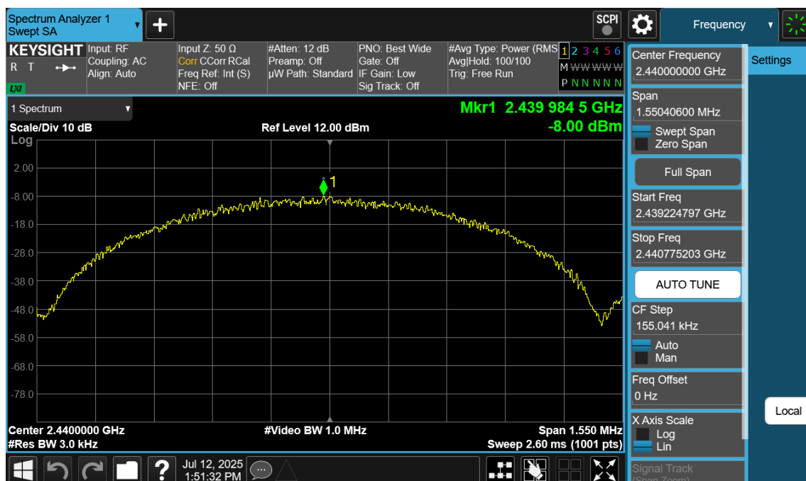
Plot 7-105. Power Spectral Density Plot Antenna 4a (Bluetooth (LE), 1Mbps, iPA – Ch. 19)
