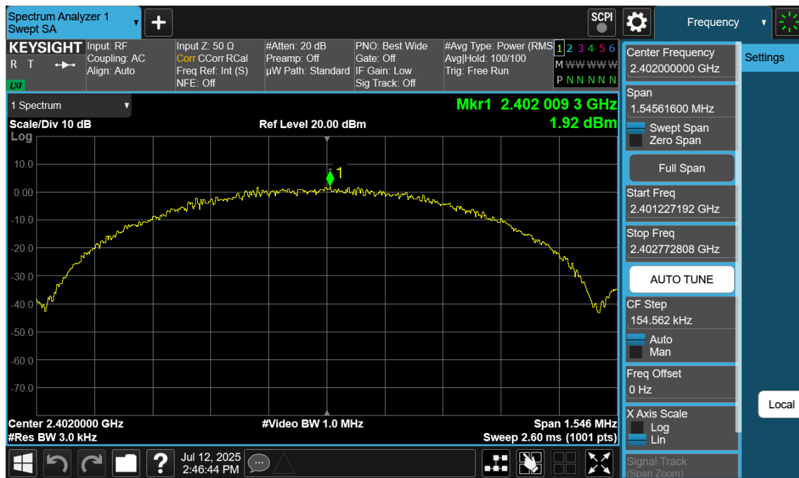
Plot 7-98. Power Spectral Density Plot Antenna 2a (Bluetooth (LE), 1Mbps, ePA – Ch. 0)
