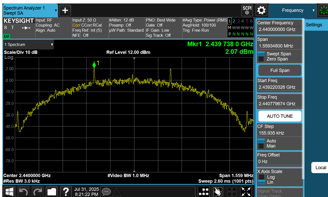
Plot 7-88. Power Spectral Density Plot Antenna 2a (Bluetooth (LE), 500kbps, ePA – Ch. 19)
