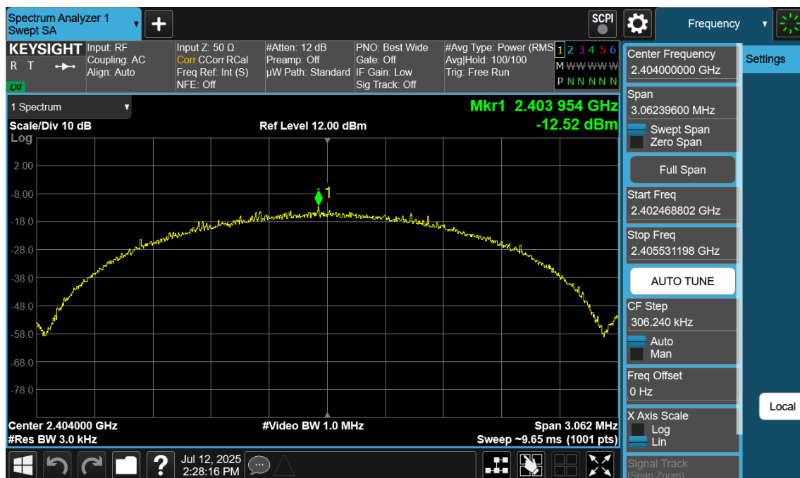
Plot 7-70. Power Spectral Density Plot Antenna 2a (Bluetooth (LE), 2Mbps, iPA – Ch. 1)
