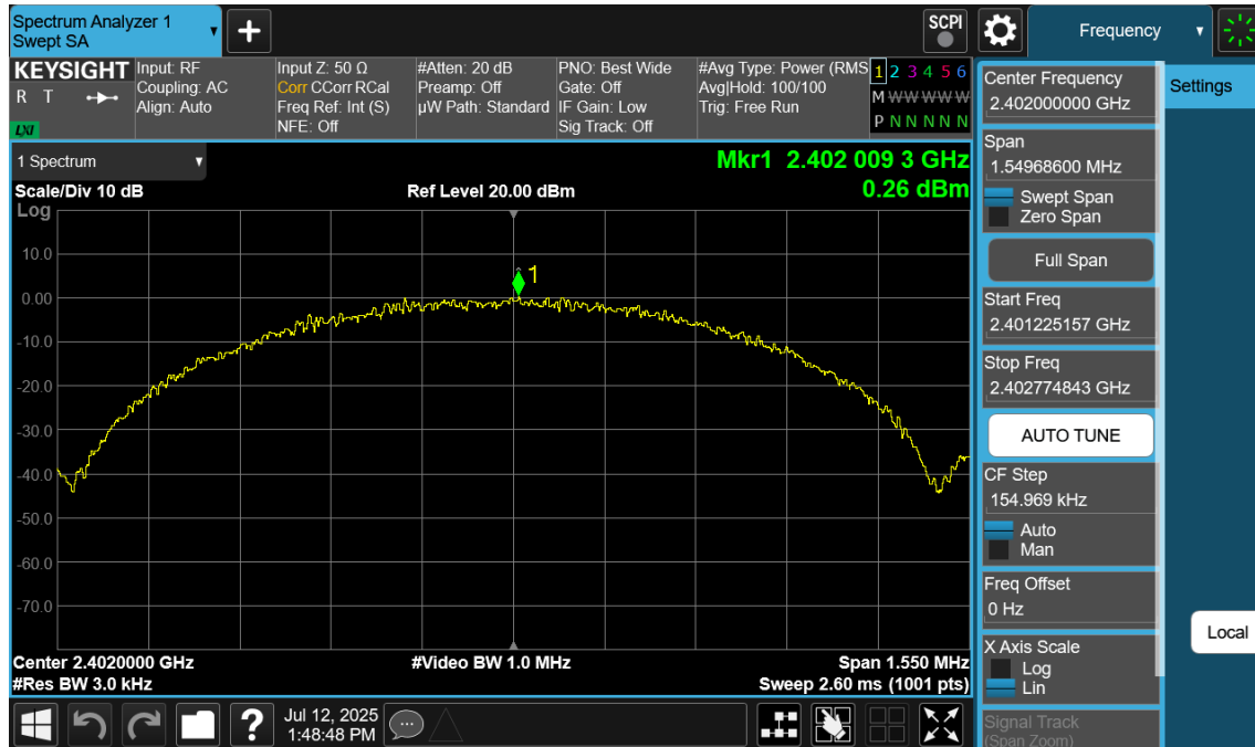
Plot 7-97. Power Spectral Density Plot Antenna 4a (Bluetooth (LE), 1Mbps, ePA – Ch. 0)
