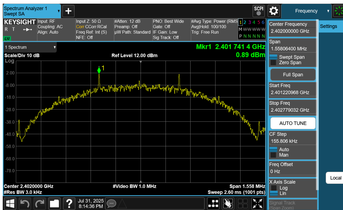
Plot 7-58. Power Spectral Density Plot Antenna 2a (Bluetooth (LE), 500kbps, iPA – Ch. 0)
