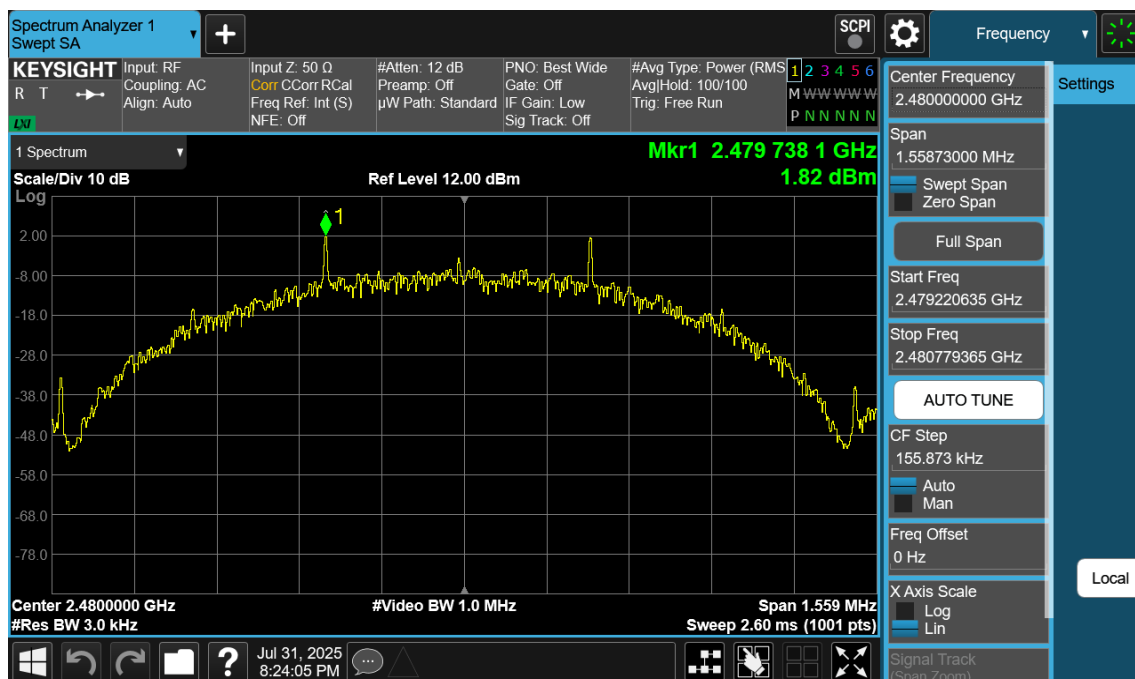
Plot 7-96. Power Spectral Density Plot Antenna 2a (Bluetooth (LE), 500kbps, iPA – Ch. 39)
