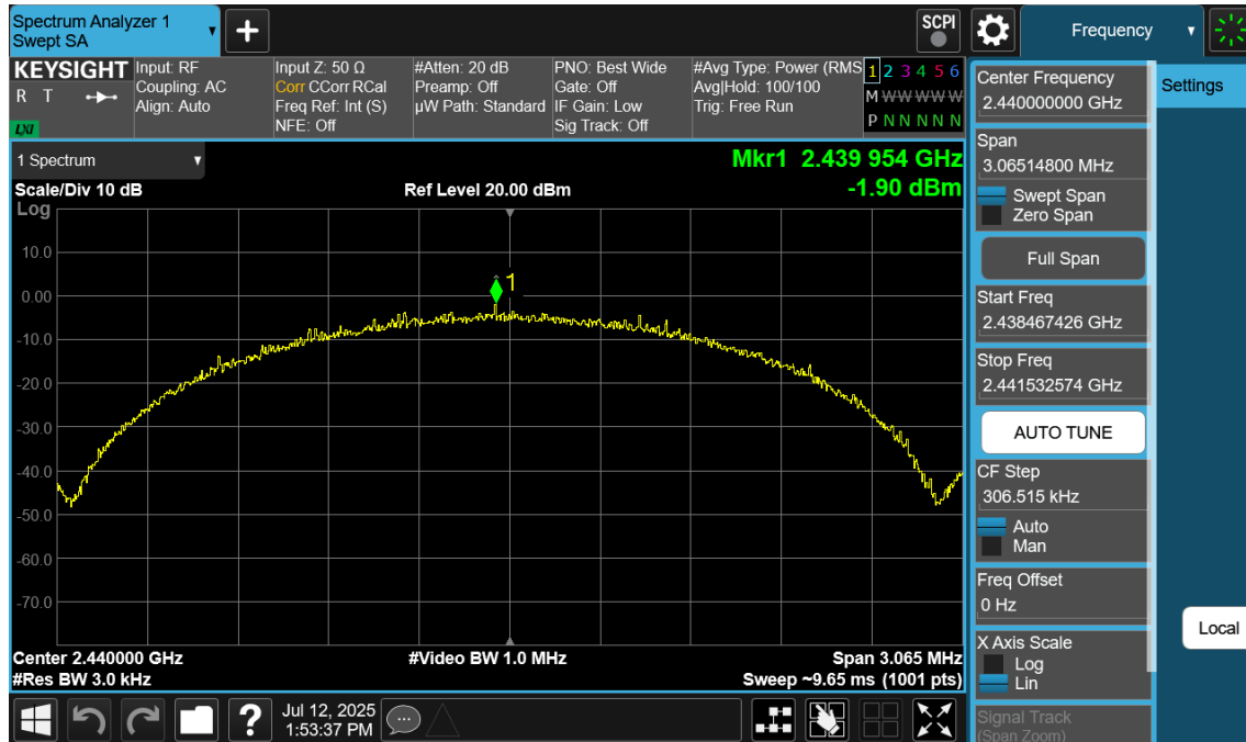
Plot 7-111. Power Spectral Density Plot Antenna 4a (Bluetooth (LE), 2Mbps, ePA – Ch. 19)
