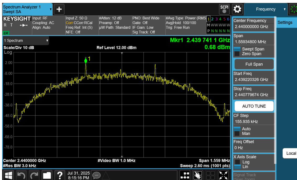
Plot 7-59. Power Spectral Density Plot Antenna 2a (Bluetooth (LE), 500kbps, iPA – Ch. 19)
