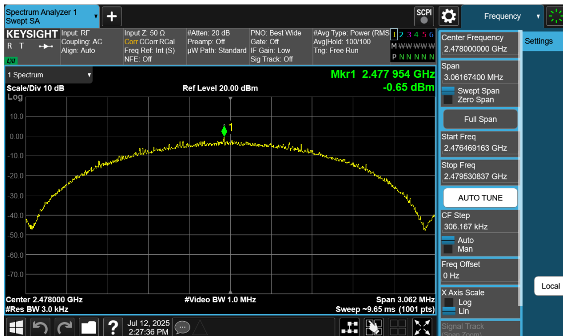
Plot 7-69. Power Spectral Density Plot Antenna 2a (Bluetooth (LE), 2Mbps, ePA – Ch. 38)
