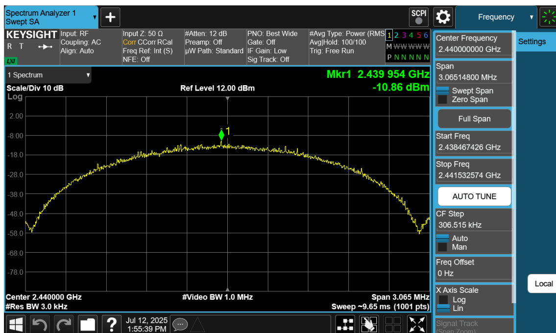
Plot 7-117. Power Spectral Density Plot Antenna 4a (Bluetooth (LE), 2Mbps, iPA – Ch. 19)
