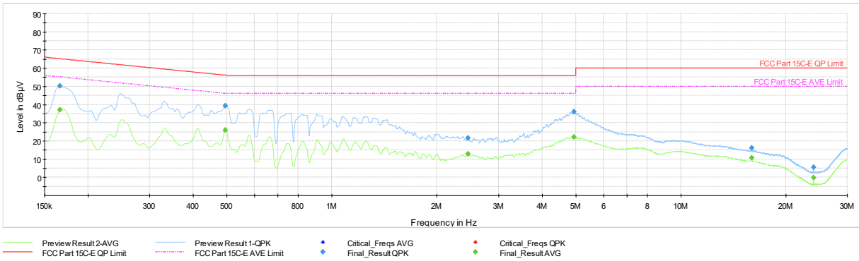
Plot 7-167. AC Line Conducted Plot with Bluetooth LE Tx BF (N, 1Mbps ePA – Ch.19, with AC/DC Adapter)
