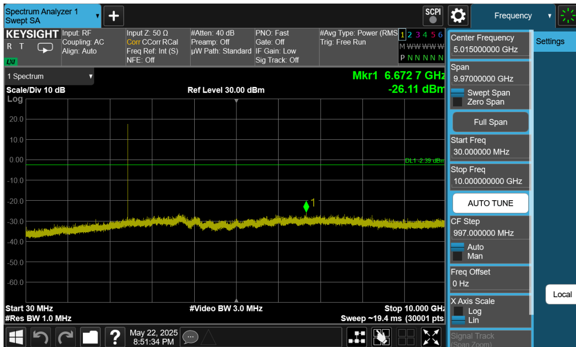
Plot 7-139. Conducted Spurious Plot Antenna 4a (Bluetooth (LE), 1Mbps, ePA – Ch. 19)
