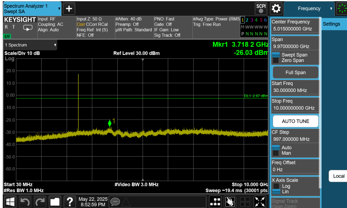
Plot 7-141. Conducted Spurious Plot Antenna 4a (Bluetooth (LE), 1Mbps, ePA – Ch. 39)
