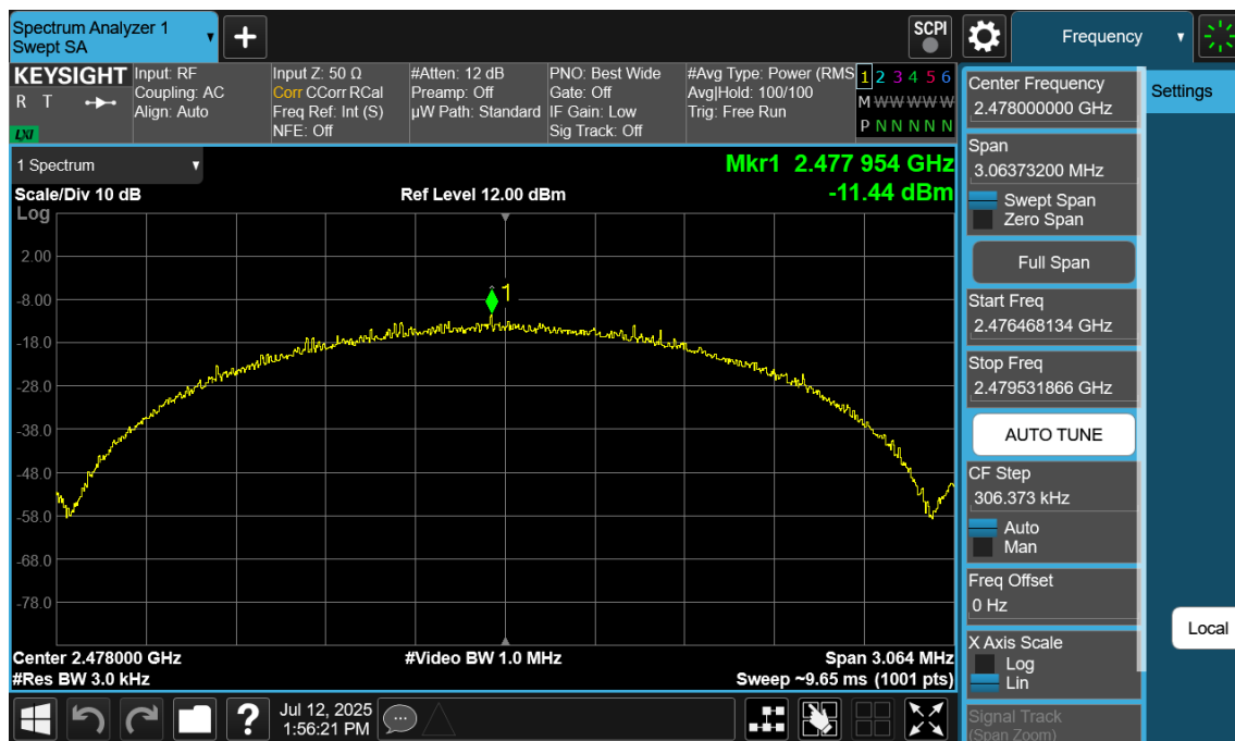
Plot 7-119. Power Spectral Density Plot Antenna 4a (Bluetooth (LE), 2Mbps, iPA – Ch. 38)
