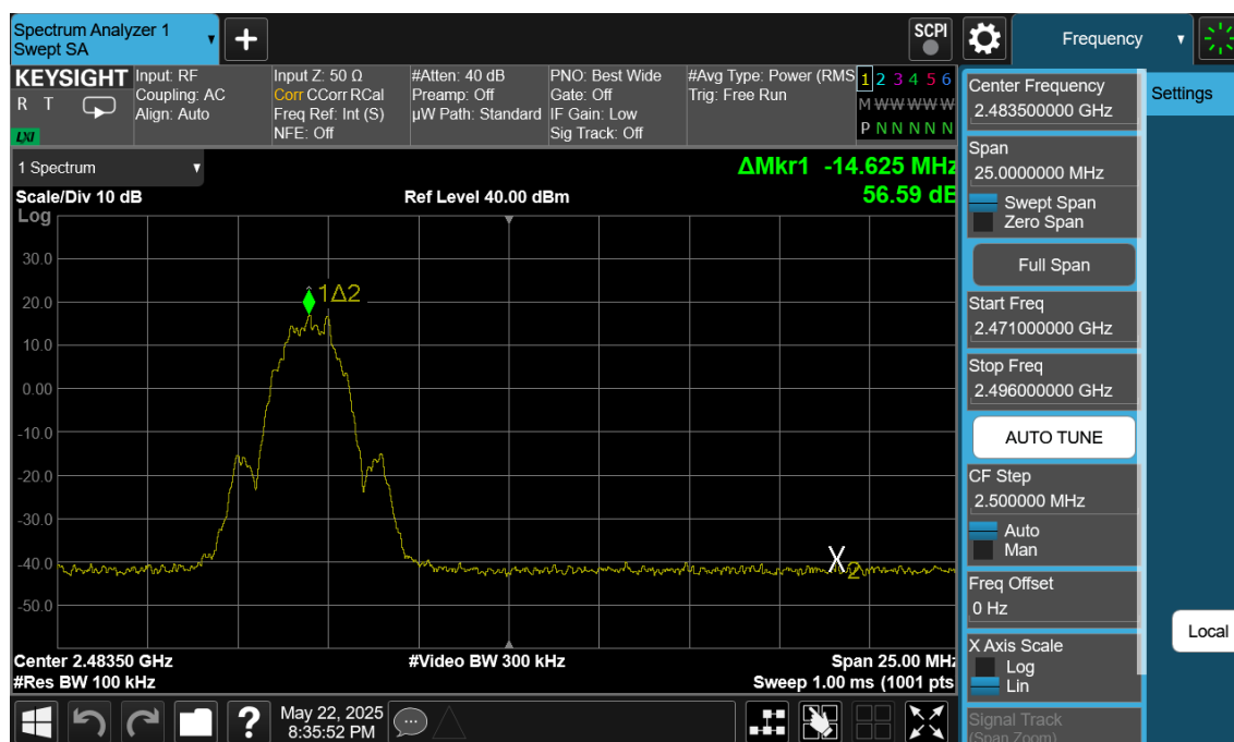
Plot 7-128. Band Edge Plot Antenna 4a (Bluetooth (LE), 2Mbps, ePA – Ch. 38)
