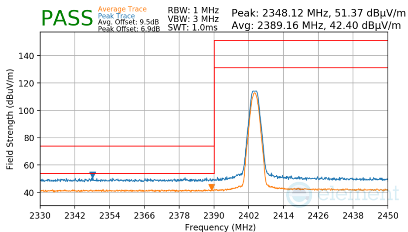
Plot 7-159. Radiated Restricted Lower Band Edge Measurement Antenna 2a (Average & Peak)
