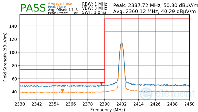
Plot 7-157. Radiated Restricted Lower Band Edge Measurement Antenna 2a (Average & Peak)
