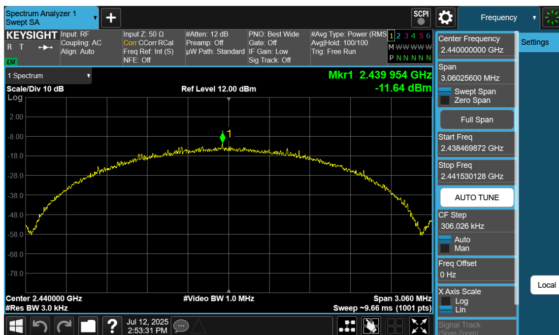
Plot 7-118. Power Spectral Density Plot Antenna 2a (Bluetooth (LE), 2Mbps, iPA – Ch. 19)
