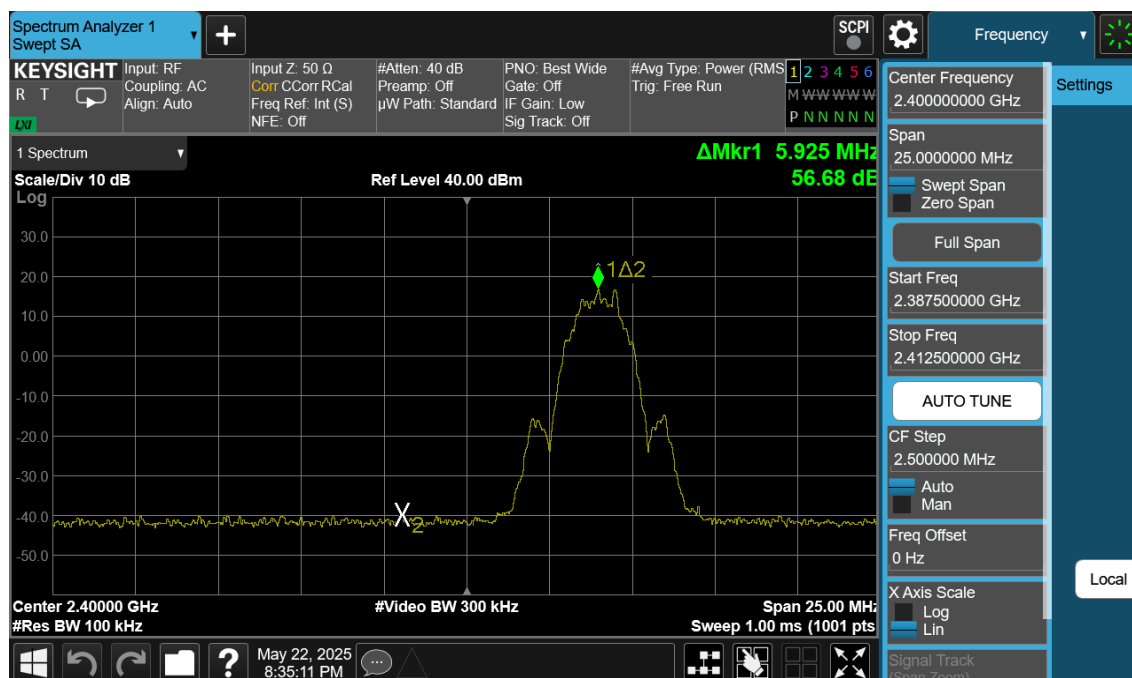
Plot 7-127. Band Edge Plot Antenna 4a (Bluetooth (LE), 2Mbps, ePA – Ch. 1)
