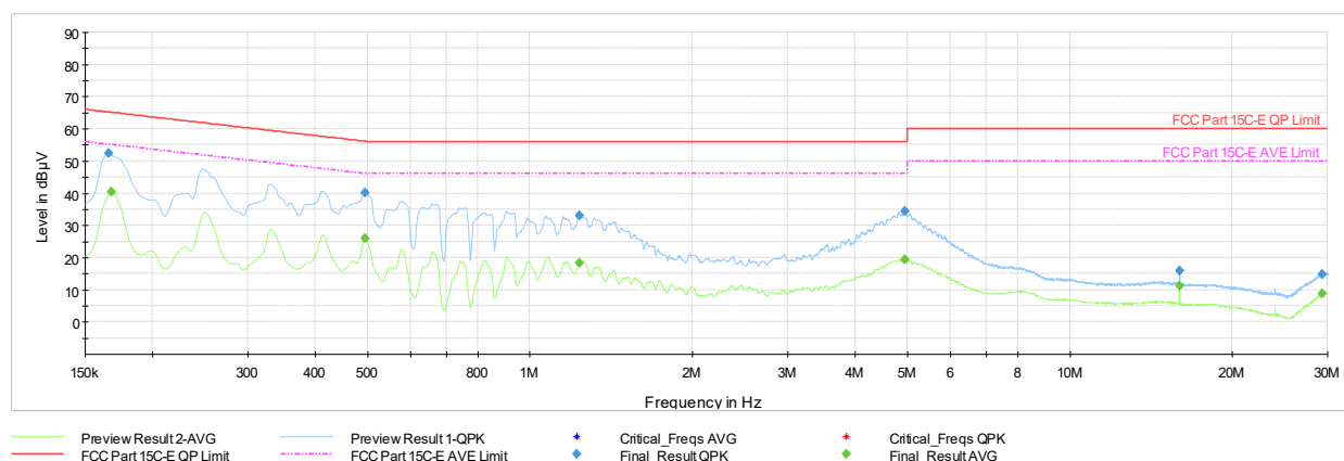
Plot 7-166. AC Line Conducted Plot with Bluetooth LE Tx BF (L1, 1Mbps ePA – Ch.19 with AC/DC Adapter)
