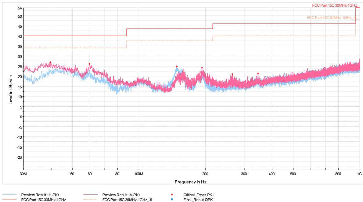
Plot 7-165. Radiated Spurious Emissions Below 1GHz TxBF (1Mbps, ePA – Ch.19, Pol. H & V, with AC/DC Adapter)
