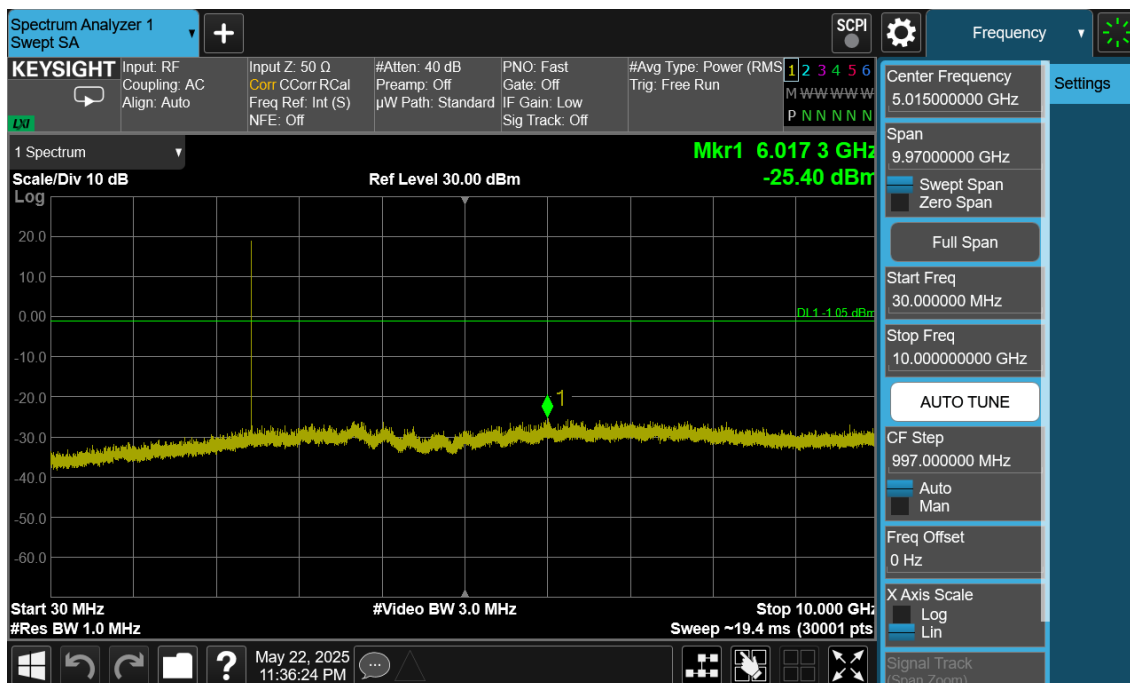
Plot 7-145. Conducted Spurious Plot Antenna 2a (Bluetooth (LE), 1Mbps, ePA – Ch. 19)
