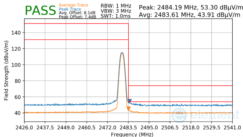
Plot 7-158. Radiated Restricted Upper Band Edge Measurement Antenna 2a (Average & Peak)
