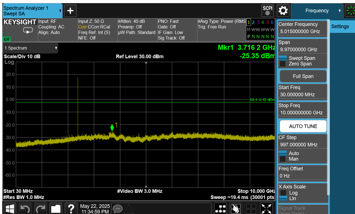
Plot 7-143. Conducted Spurious Plot Antenna 2a (Bluetooth (LE), 1Mbps, ePA – Ch. 0)
