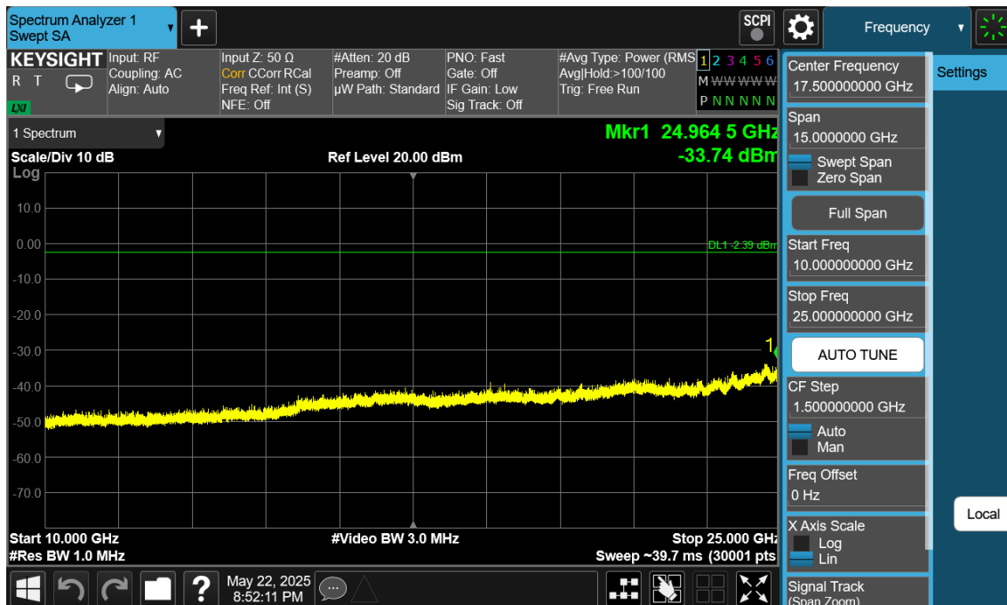
Plot 7-140. Conducted Spurious Plot Antenna 4a (Bluetooth (LE), 1Mbps, ePA – Ch. 19)
