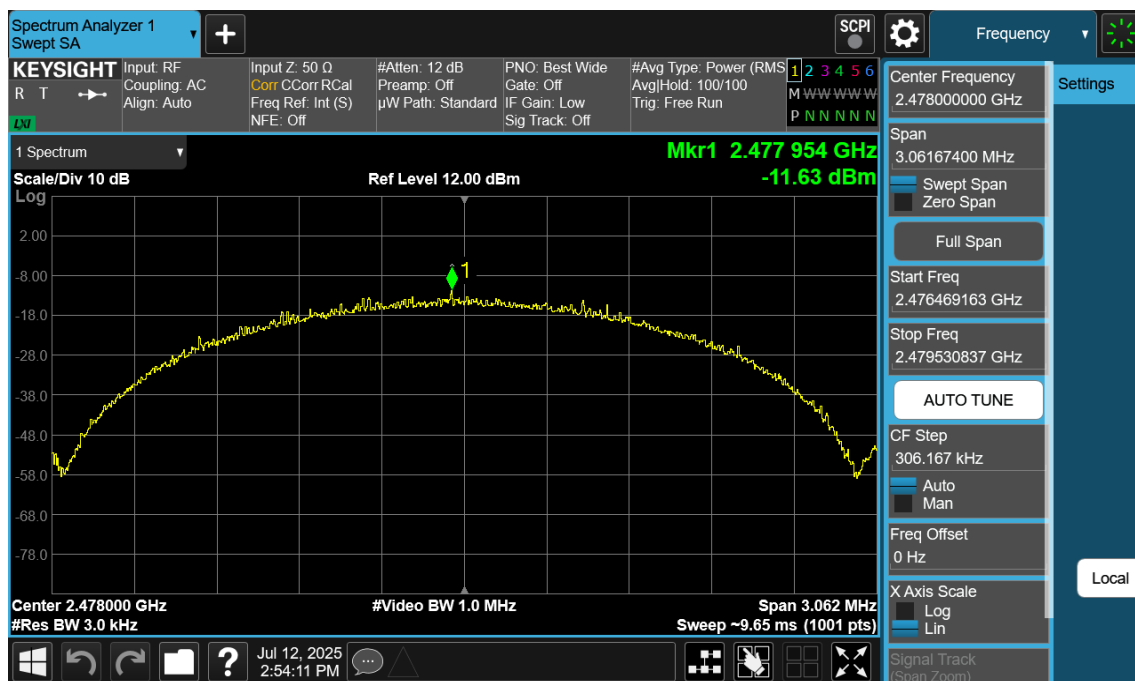
Plot 7-120. Power Spectral Density Plot Antenna 2a (Bluetooth (LE), 2Mbps, iPA – Ch. 38)
