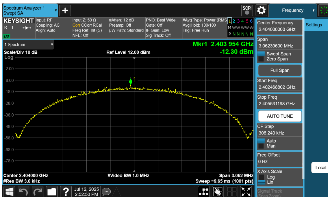
Plot 7-116. Power Spectral Density Plot Antenna 2a (Bluetooth (LE), 2Mbps, iPA – Ch. 1)
