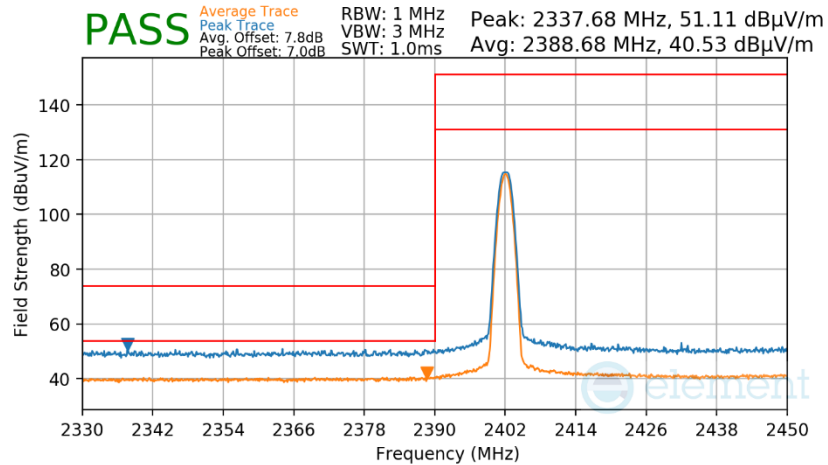
Plot 7-161. Radiated Restricted Lower Band Edge Measurement TxBF (Average & Peak)
