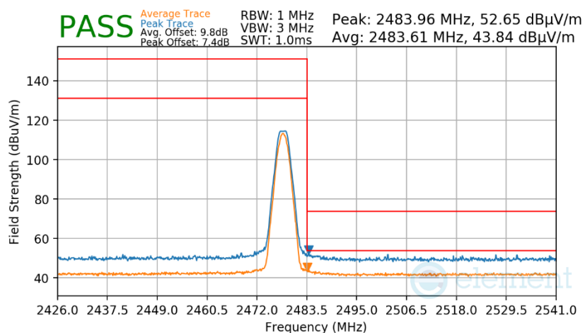
Plot 7-160. Radiated Restricted Upper Band Edge Measurement Antenna 2a (Average & Peak)
