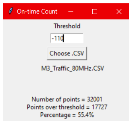
Figure 9-8. 5530MHz - Channel Loading Calculation - Mode 3 (80MHz)
