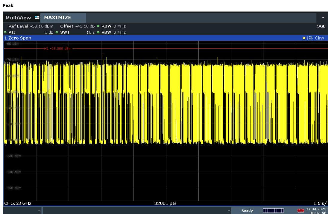
Figure 9-9. 5530 MHz - Channel Loading - Mode 4 (80MHz)
