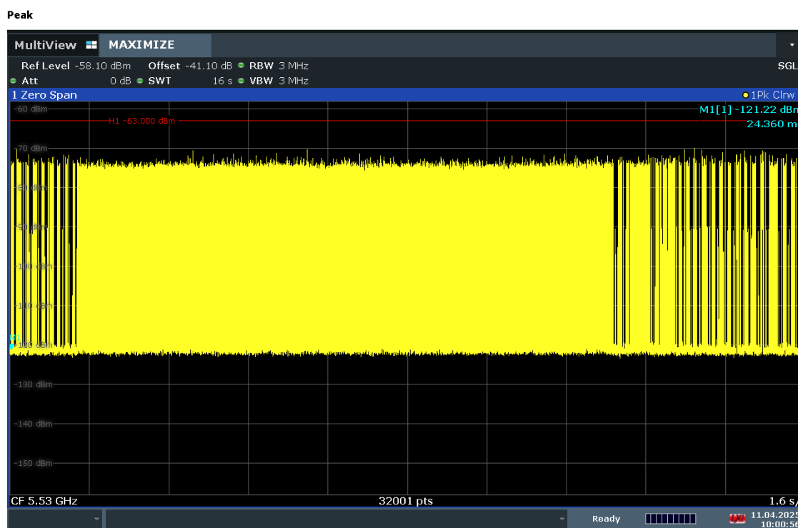
Figure 9-1. 5530MHz - Channel Loading - Mode 1 (80MHz)
