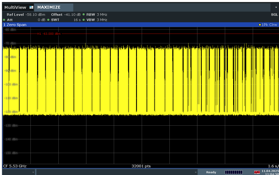
Figure 9-5. 5530MHz - Channel Loading - Mode 2 (80MHz)
