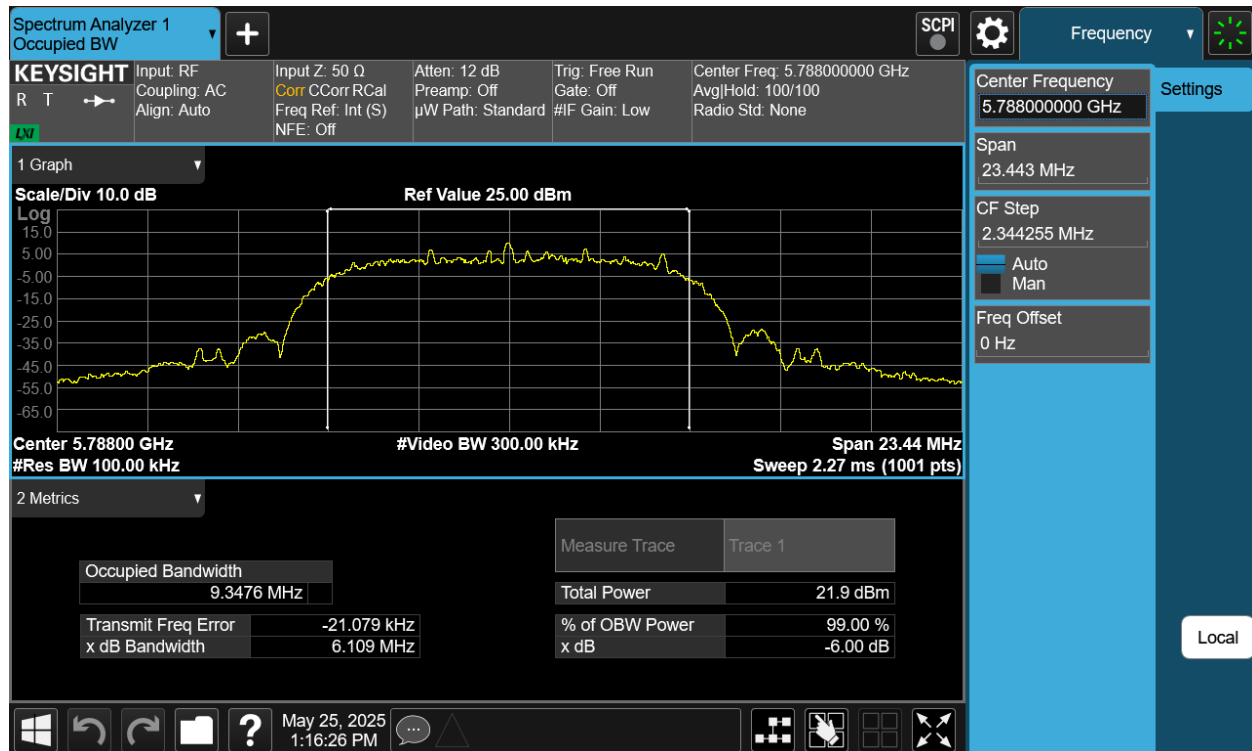
Plot 7-48. 6dB BW & 99% OBW Antenna WF5B (NB UNII HDRPL12, ePA – 5788MHz)
