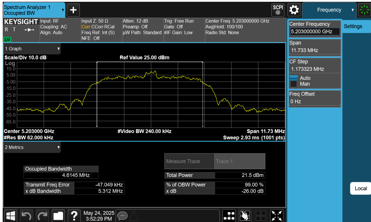
Plot 7-5. 26dB BW & 99% OBW Antenna WF5B (NB UNII HDR8, ePA- 5203MHz)
