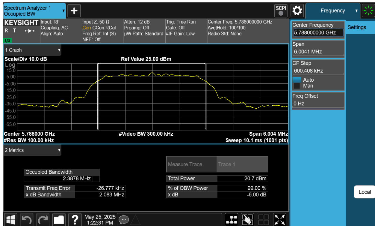
Plot 7-50. 6dB BW & 99% OBW Antenna WF5B (NB UNII HDT2, ePA- 5788MHz)
