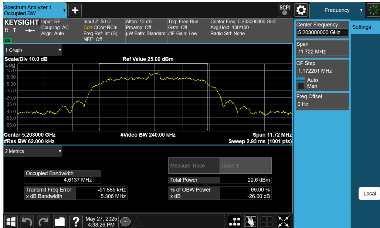
Plot 7-18. 26dB BW & 99% OBW Antenna 4a (NB UNII HDR8, ePA- 5203MHz)
