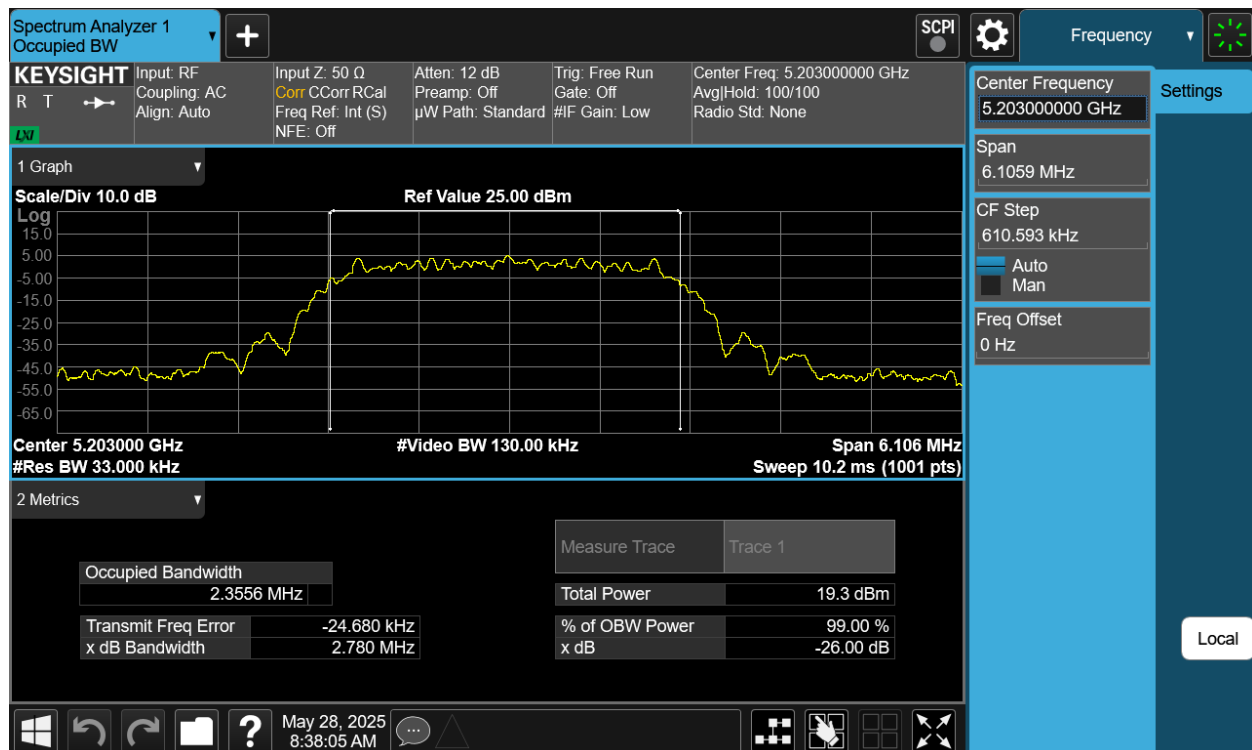
Plot 7-38. 26dB BW & 99% OBW Antenna 2a (NB UNII HDT4, ePA- 5203MHz)
