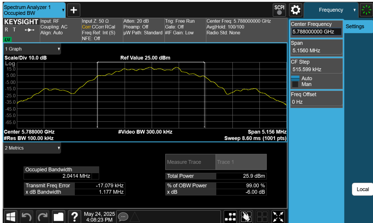
Plot 7-42. 6dB BW & 99% OBW Antenna WF5B (NB UNII LE2M, ePA- 5788MHz)
