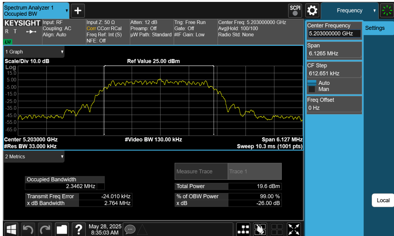
Plot 7-37. 26dB BW & 99% OBW Antenna 2a (NB UNII HDT2, ePA- 5203MHz)
