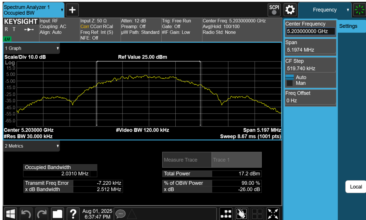
Plot 7-16. 26dB BW & 99% OBW Antenna 4a (NB UNII LE2M, ePA- 5203MHz)
