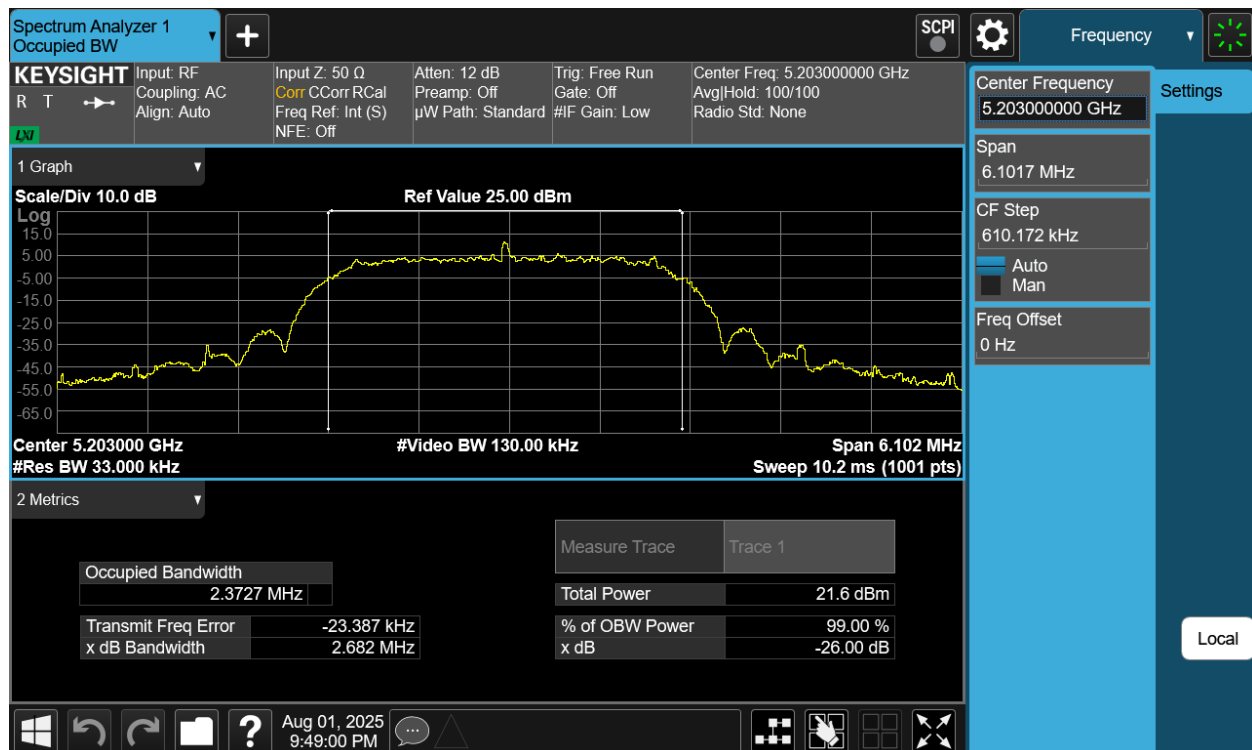
Plot 7-19. 26dB BW & 99% OBW Antenna 4a (NB UNII HDRPS2, ePA- 5203MHz)
