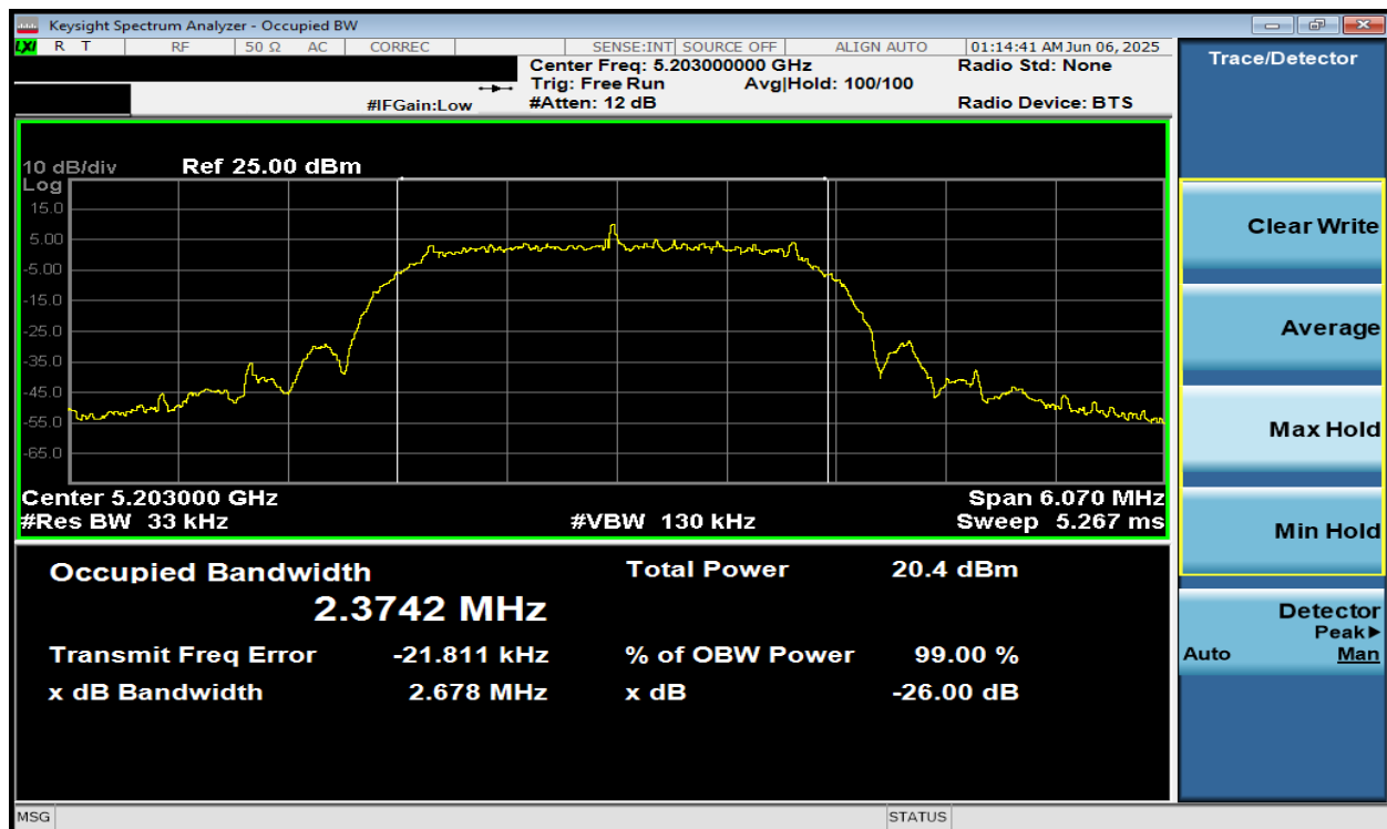
Plot 7-32. 26dB BW & 99% OBW Antenna 2a (NB UNII HDRPS2, ePA- 5203MHz)
