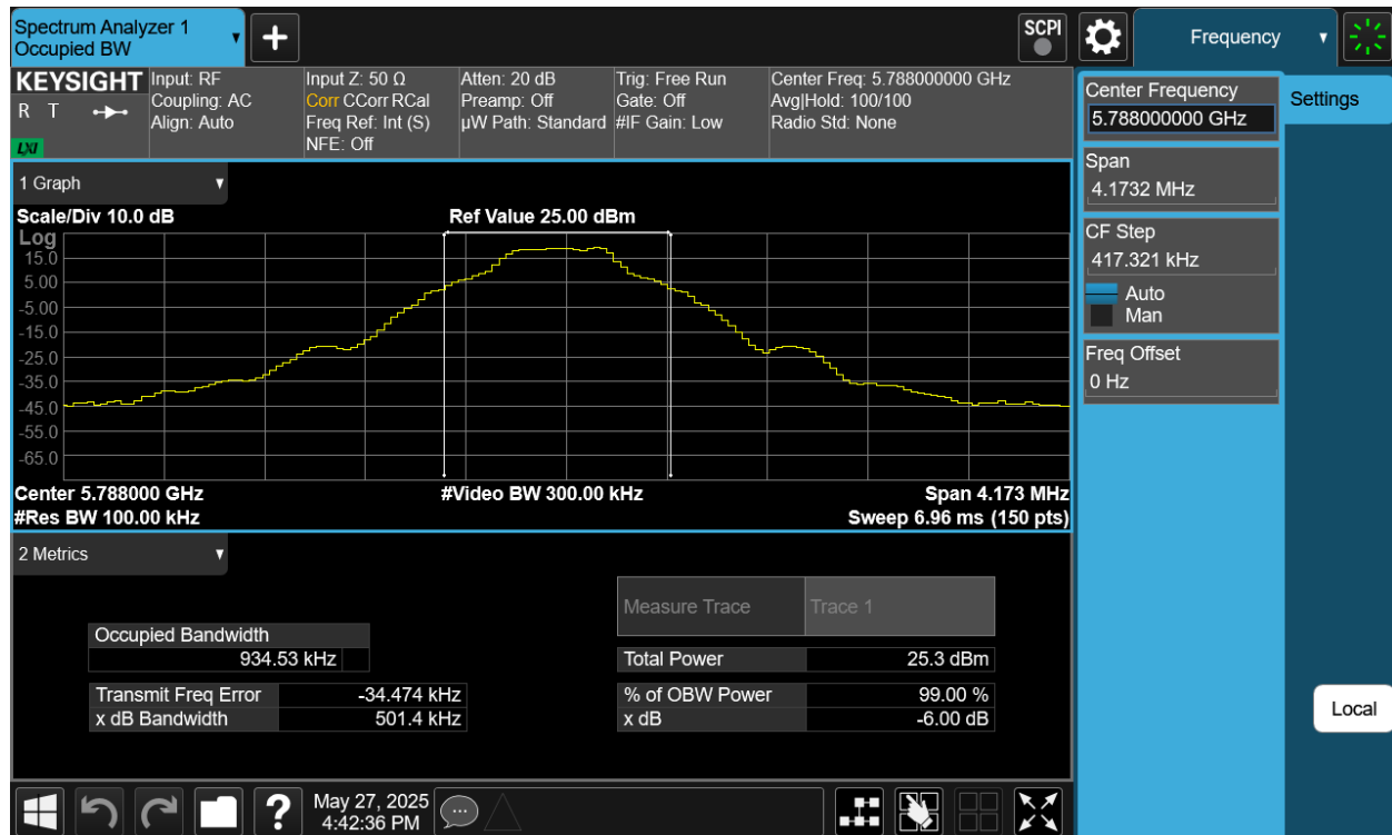
Plot 7-53. 6dB BW & 99% OBW Antenna 4a (NB UNII BDR, ePA – 5788MHz)
