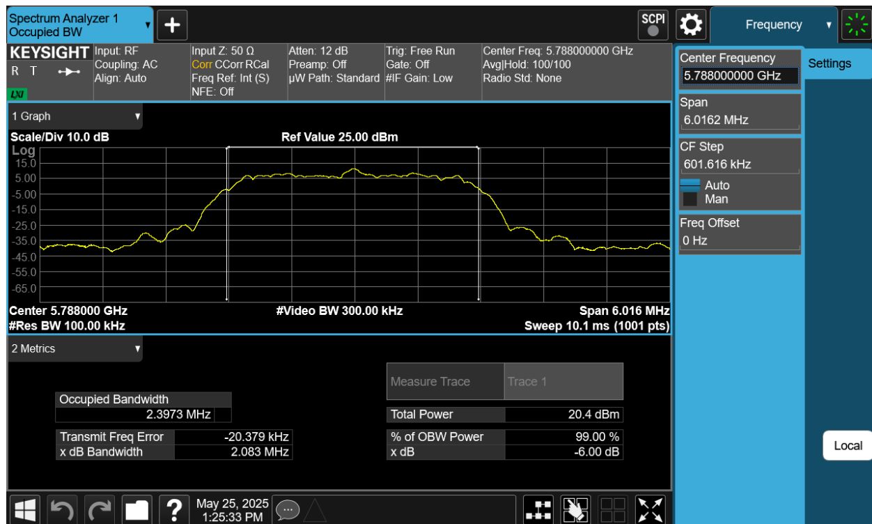
Plot 7-51. 6dB BW & 99% OBW Antenna WF5B (NB UNII HDT4, ePA- 5788MHz)
