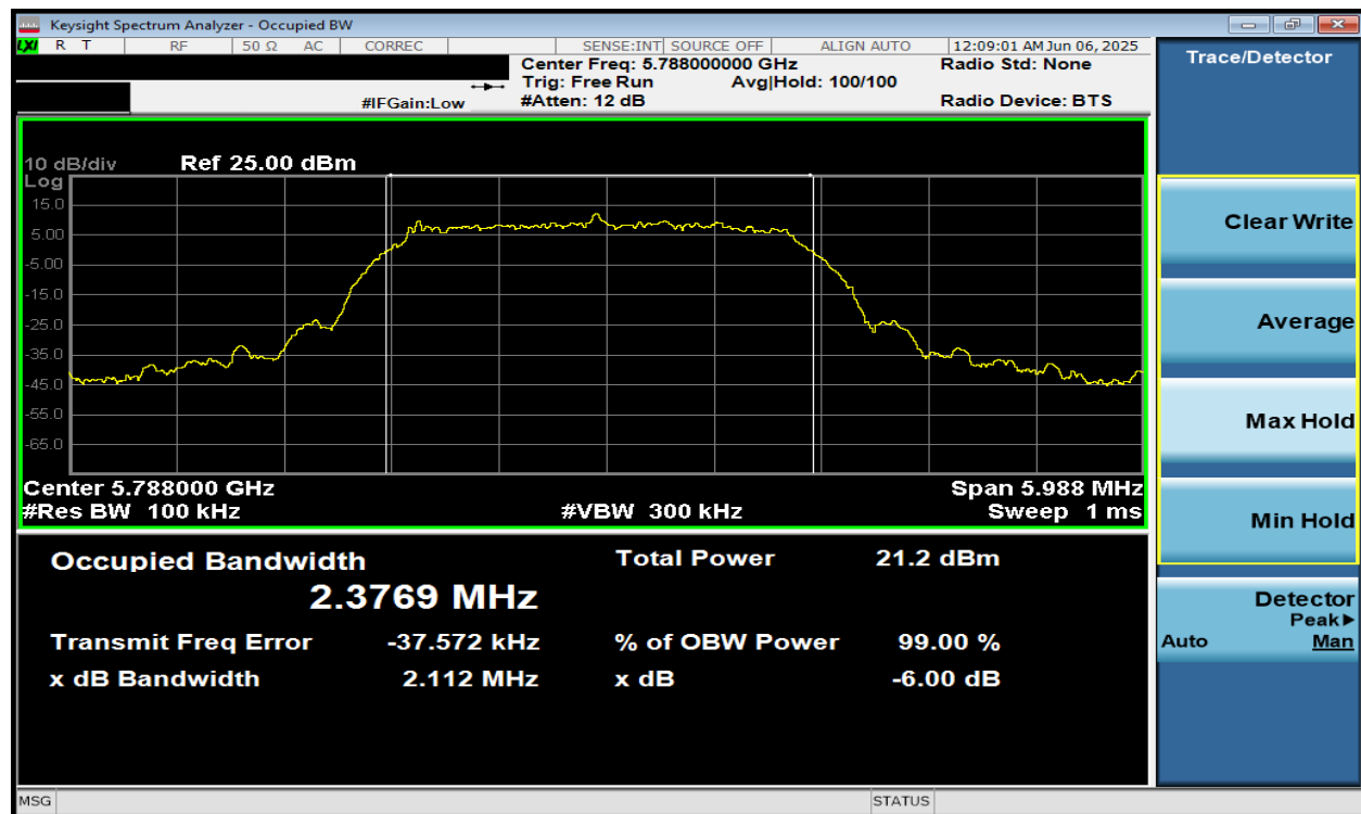
Plot 7-45. 6dB BW & 99% OBW Antenna WF5B (NB UNII HDRPS2, ePA – 5788MHz)
