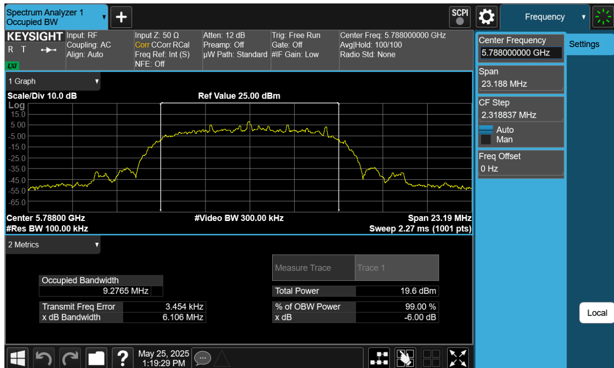
Plot 7-49. 6dB BW & 99% OBW Antenna WF5B (NB UNII HDRPL32, ePA – 5788MHz)
