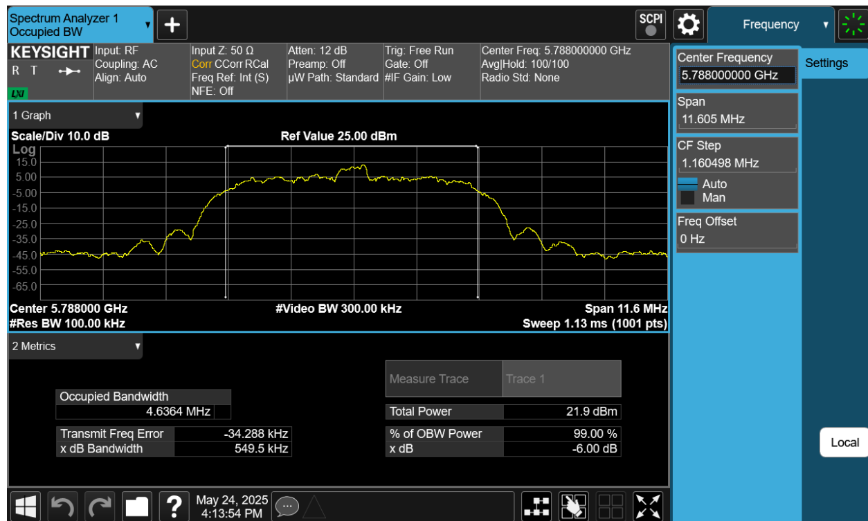
Plot 7-44. 6dB BW & 99% OBW Antenna WF5B (NB UNII HDR8, ePA – 5788MHz)
