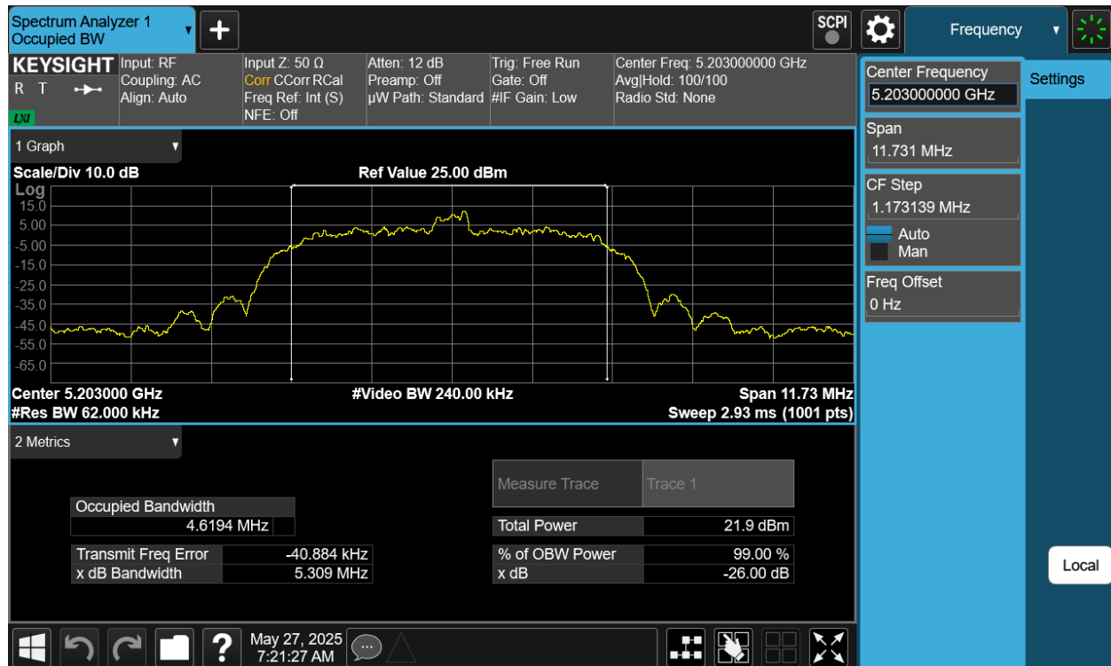
Plot 7-31. 26dB BW & 99% OBW Antenna 2a (NB UNII HDR8, ePA- 5203MHz)
