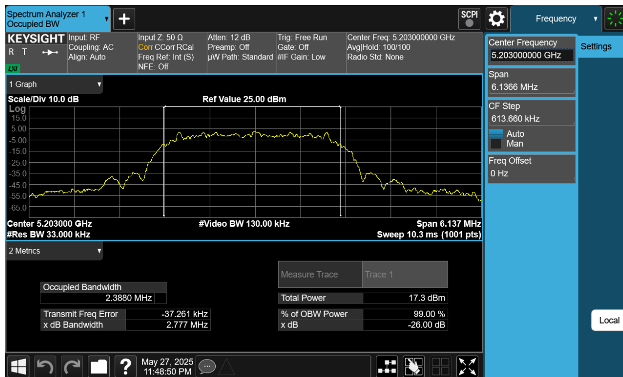
Plot 7-26. 26dB BW & 99% OBW Antenna 4a (NB UNII HDT6, ePA– 5203MHz)
