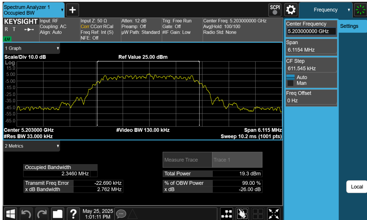
Plot 7-11. 26dB BW & 99% OBW Antenna WF5B (NB UNII HDT2, ePA- 5203MHz)
