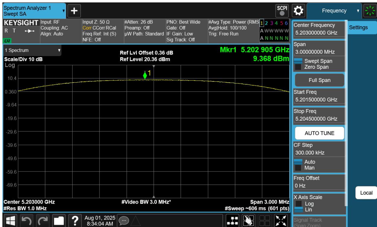
Plot 7-89. PSD Antenna WF5B (NB UNII HDRPS2, ePA – 5203MHz)
