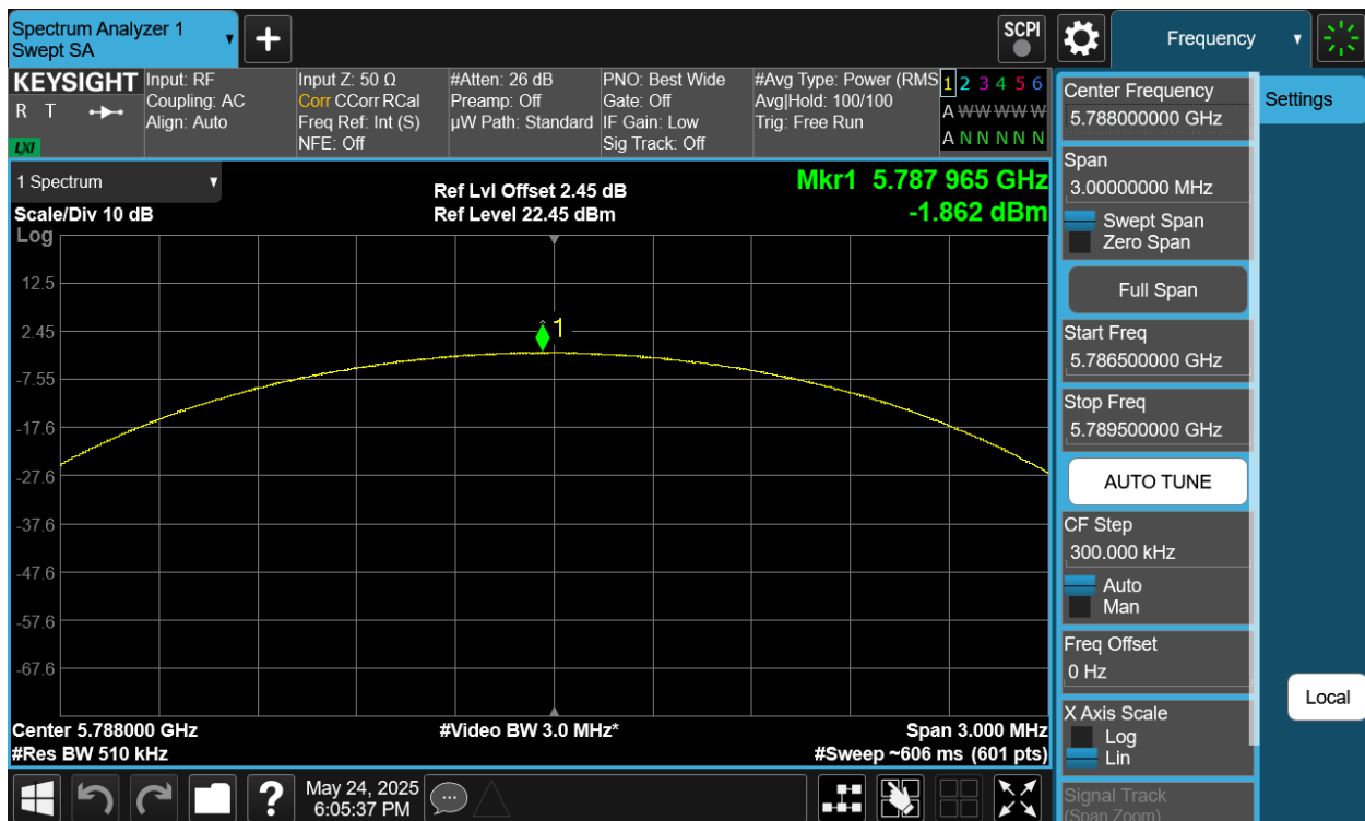
Plot 7-110. PSD Antenna WF5B (NB UNII LE2M, iPA – 5788MHz)
