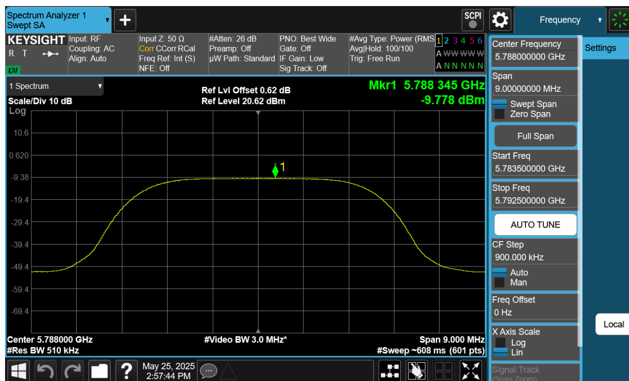
Plot 7-118. PSD Antenna WF5B (NB UNII XHDRPM6, iPA – 5788MHz)
