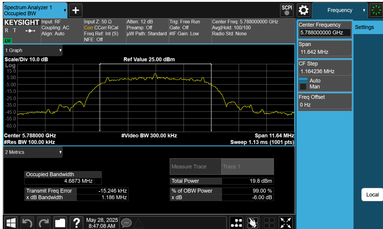
Plot 7-73. 6dB BW & 99% OBW Antenna 2a (NB UNII HDRPM16, ePA – 5788MHz)
