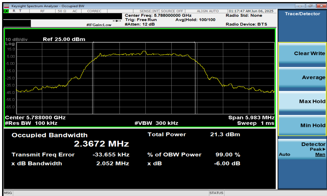
Plot 7-71. 6dB BW & 99% OBW Antenna 2a (NB UNII HDRPS2, ePA – 5788MHz)
