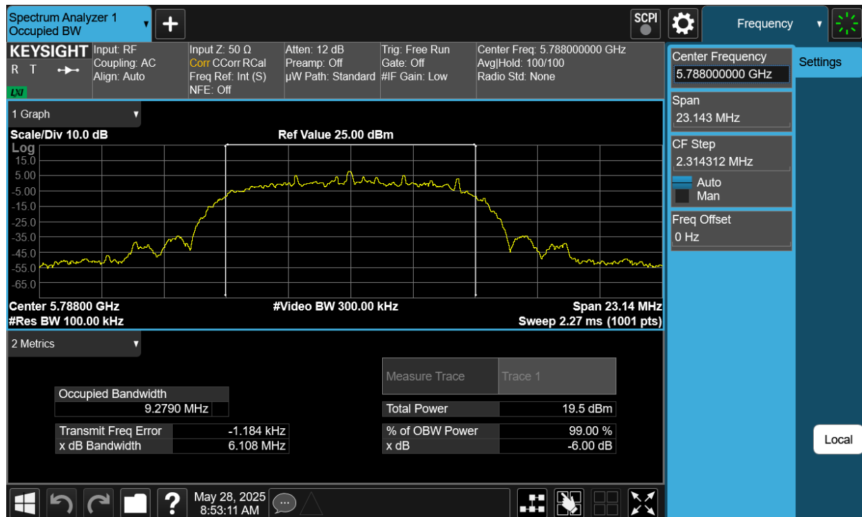
Plot 7-75. 6dB BW & 99% OBW Antenna 2a (NB UNII HDRPL32, ePA – 5788MHz)
