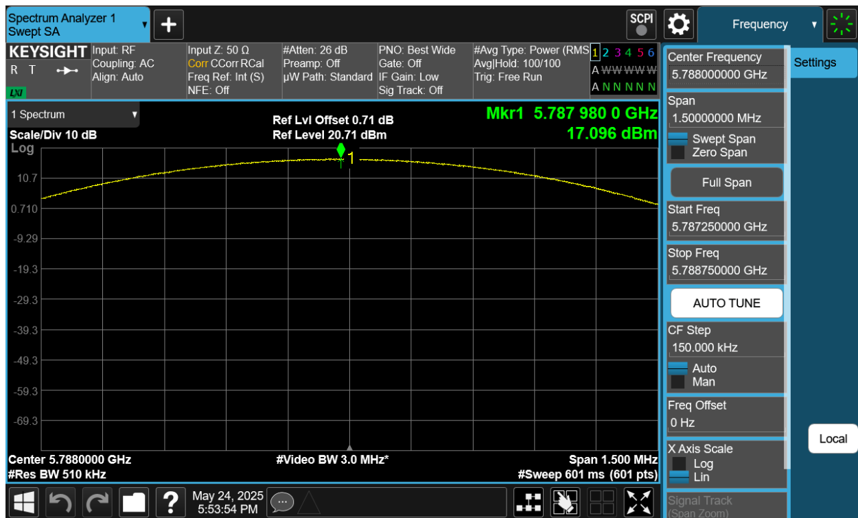
Plot 7-107. PSD Antenna WF5B (NB UNII LE1M, ePA – 5788MHz)
