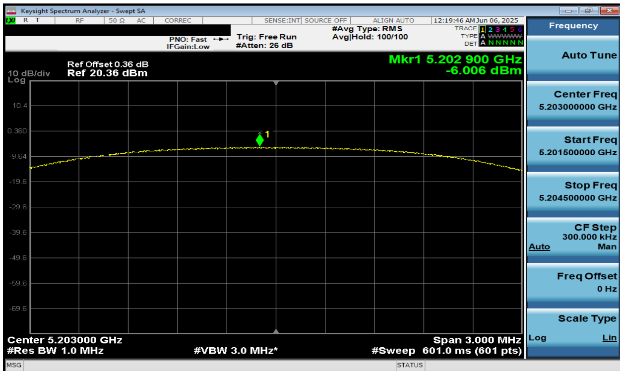
Plot 7-90. PSD Antenna WF5B (NB UNII HDRPS2, iPA – 5203MHz)
