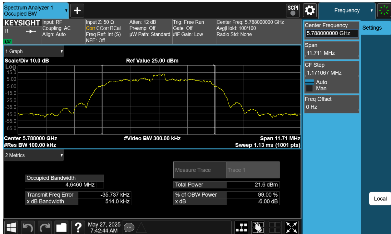
Plot 7-70. 6dB BW & 99% OBW Antenna 2a (NB UNII HDR8, ePA – 5788MHz)
