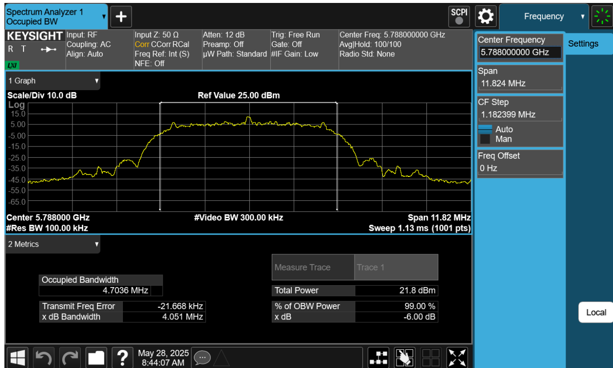
Plot 7-72. 6dB BW & 99% OBW Antenna 2a (NB UNII XHDRPM6, ePA – 5788MHz)
