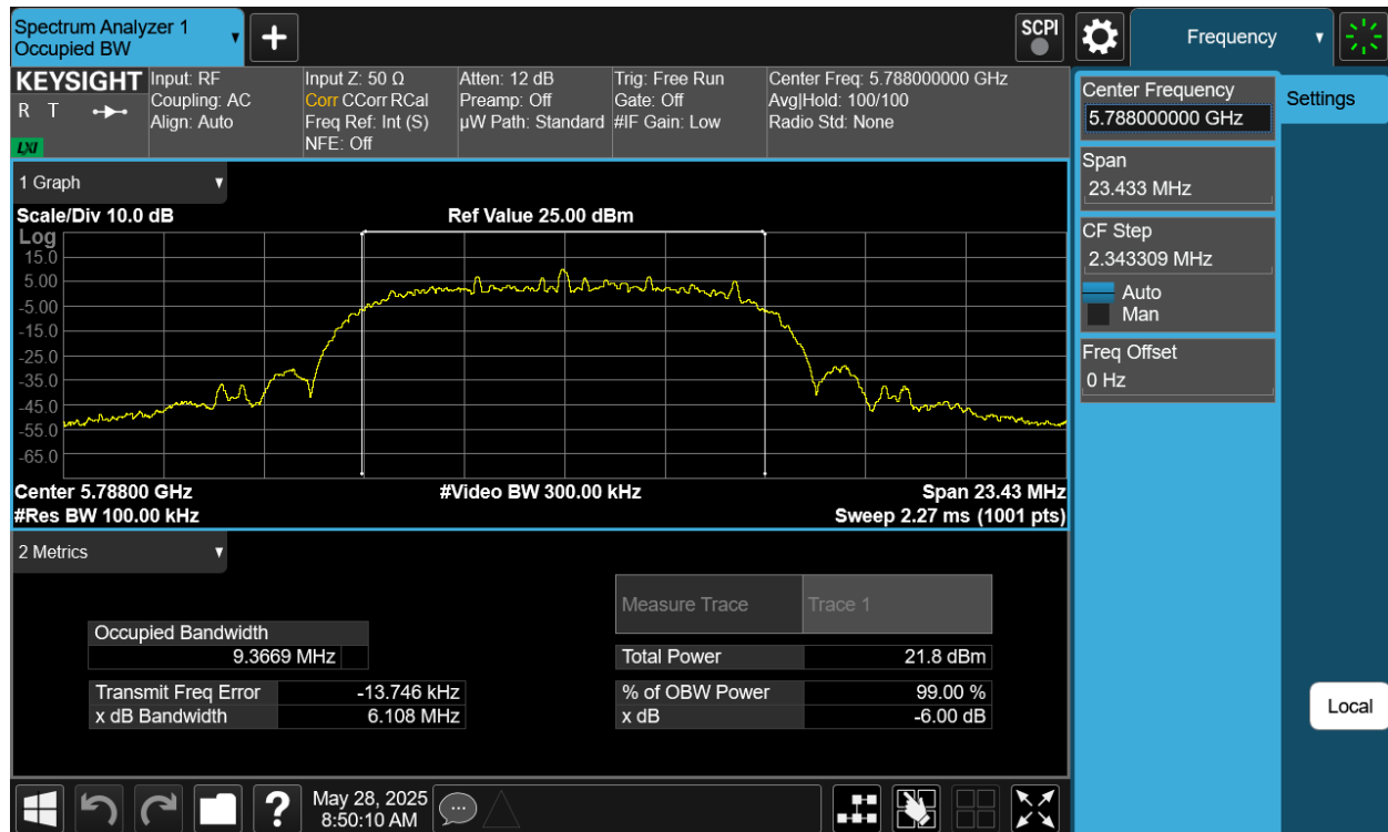
Plot 7-74. 6dB BW & 99% OBW Antenna 2a (NB UNII HDRPL12, ePA – 5788MHz)
