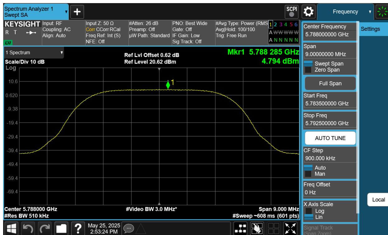
Plot 7-117. PSD Antenna WF5B (NB UNII XHDRPM6, ePA – 5788MHz)
