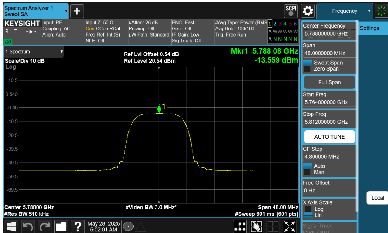
Plot 7-429. PSD TxBF Diversity Antenna 4a (NB UNII HDRPL32, iPA – 5788MHz)
