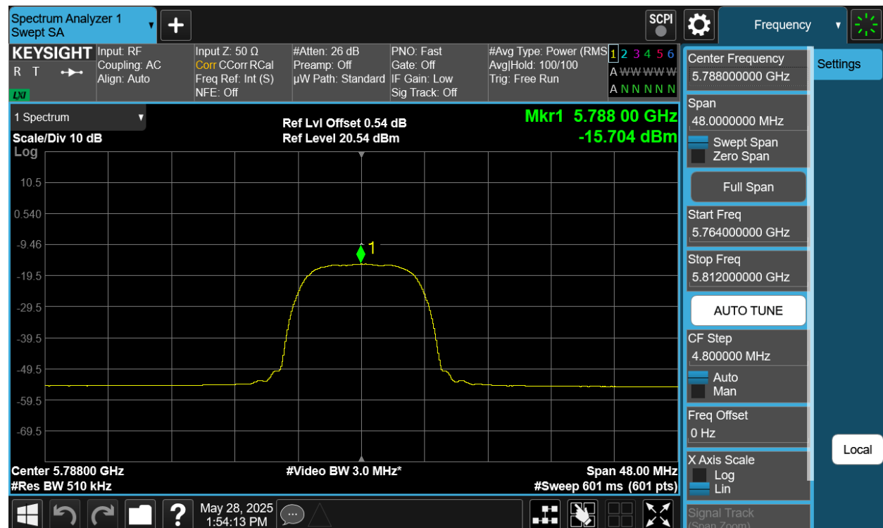
Plot 7-430. PSD TxBF Diversity Antenna 2a (NB UNII HDRPL32, iPA – 5788MHz)
