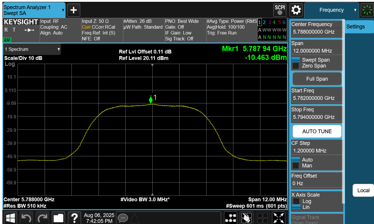
Plot 7-410. PSD TxBF Diversity Antenna 2a (NB UNII HDR8, iPA – 5788MHz)
