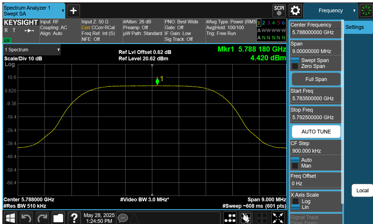
Plot 7-416. PSD Tx BF Diversity Antenna 2a (NB UNII XHDRPM6, ePA – 5788MHz)
