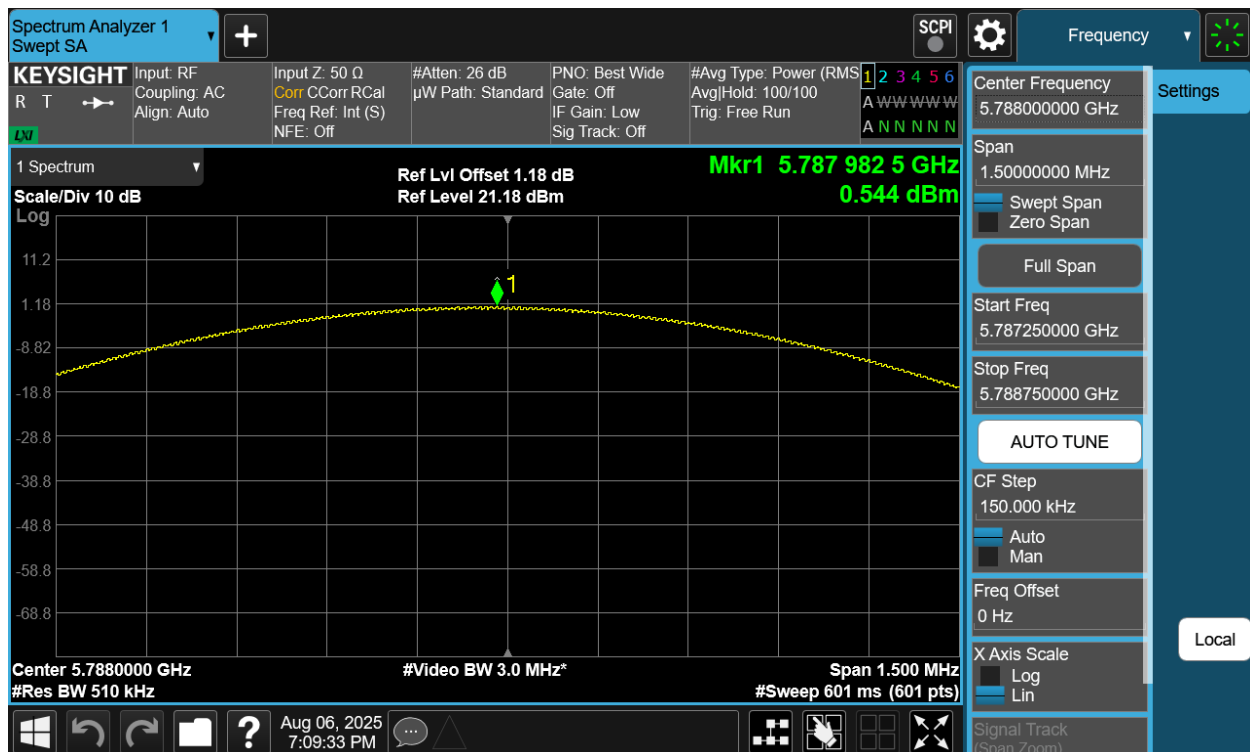
Plot 7-394. PSD Tx BF Diversity Antenna 2a (NB UNII BDR, iPA – 5788MHz)
