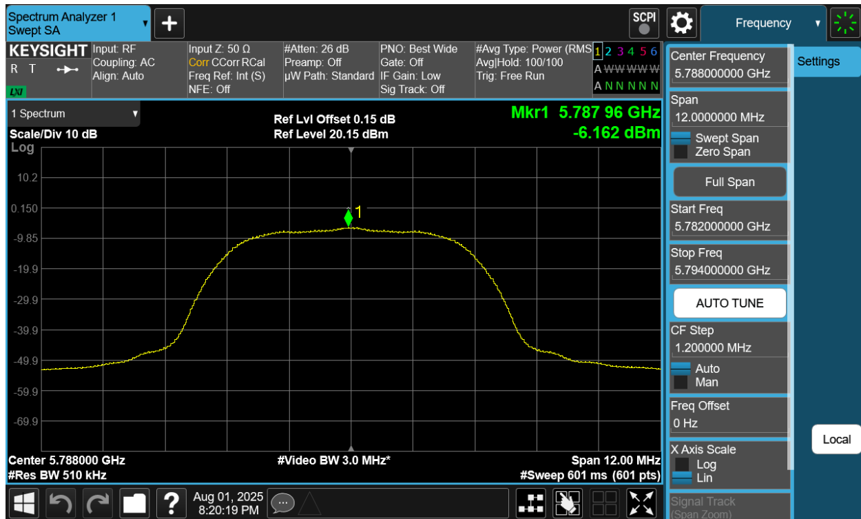
Plot 7-409. PSD TxBF Diversity Antenna 4a (NB UNII HDR8, iPA – 5788MHz)
