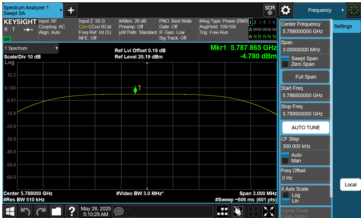
Plot 7-433. PSD TxBF Diversity Antenna 4a (NB UNII HDT2, iPA – 5788MHz)
