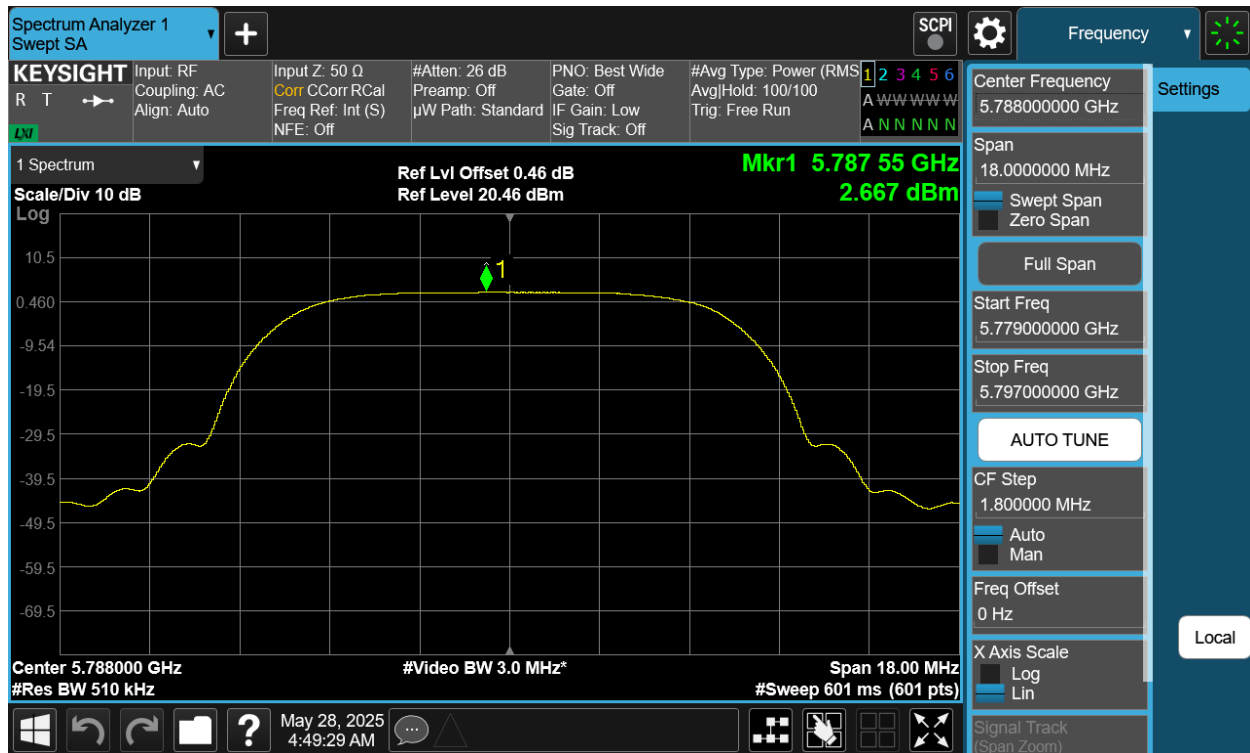
Plot 7-423. PSD TxBF Diversity Antenna 4a (NB UNII HDRPL12, ePA – 5788MHz)
