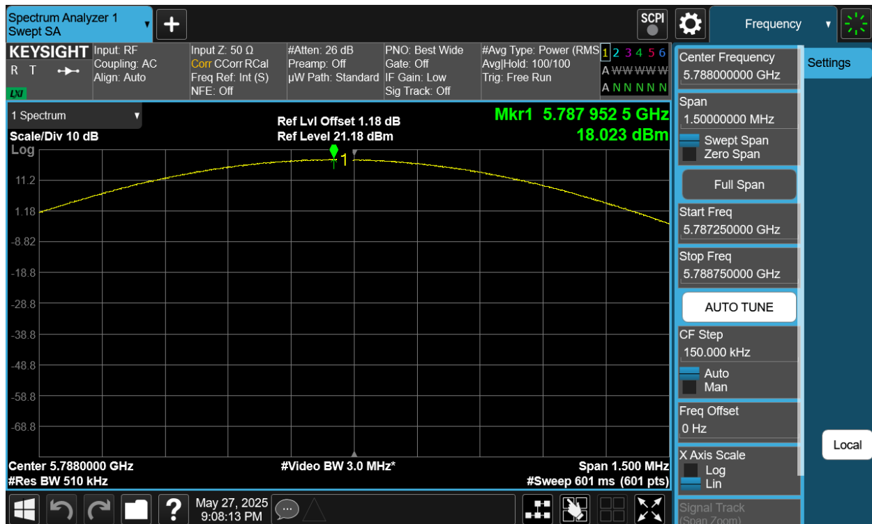
Plot 7-391. PSD Tx B F Diversity Antenna 4a (NB UNII BDR, ePA – 5788MHz)
