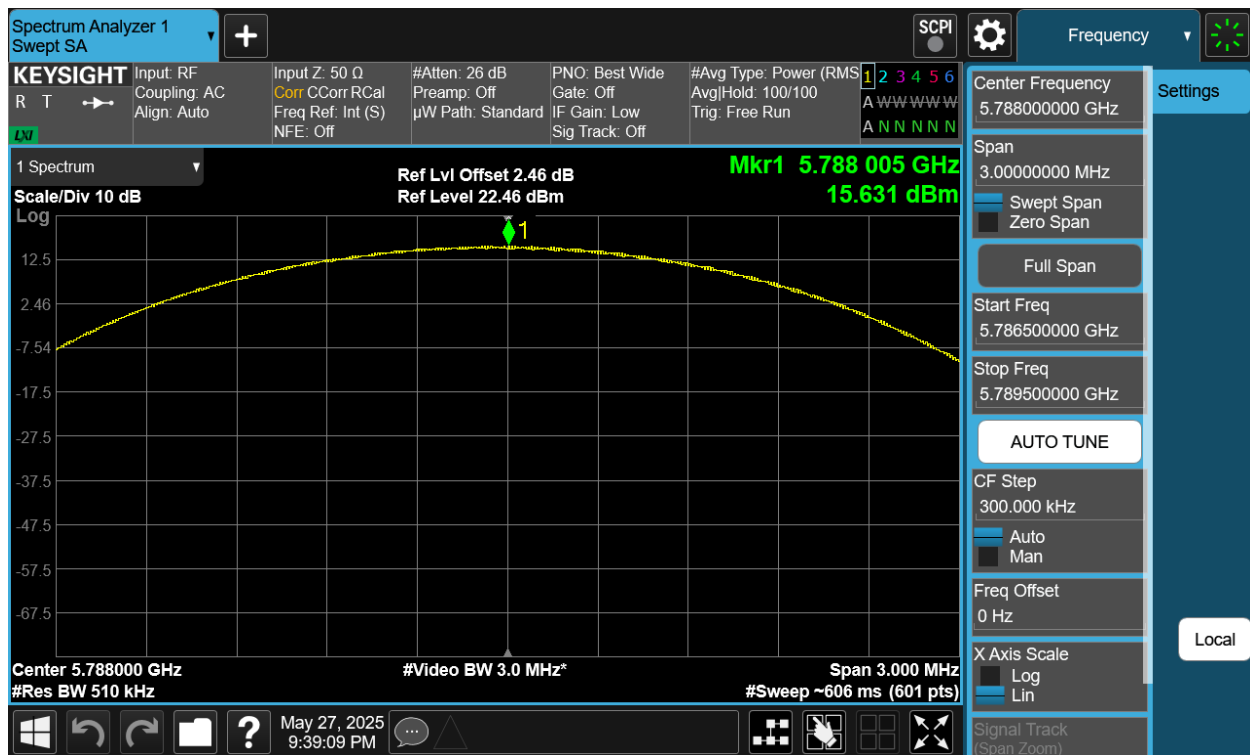
Plot 7-399. PSD TxBF Diversity Antenna 4a (NB UNII LE2M, ePA – 5788MHz)
