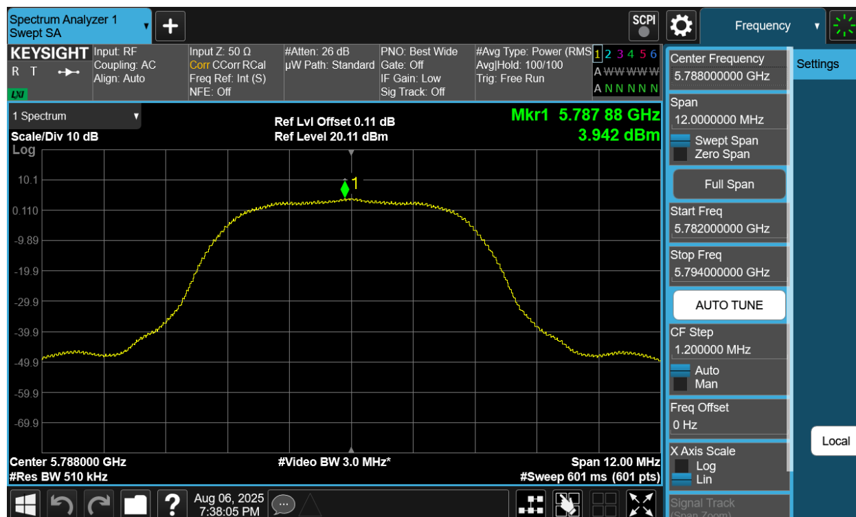
Plot 7-408. PSD TxBF Diversity Antenna 2a (NB UNII HDR8, ePA – 5788MHz)
