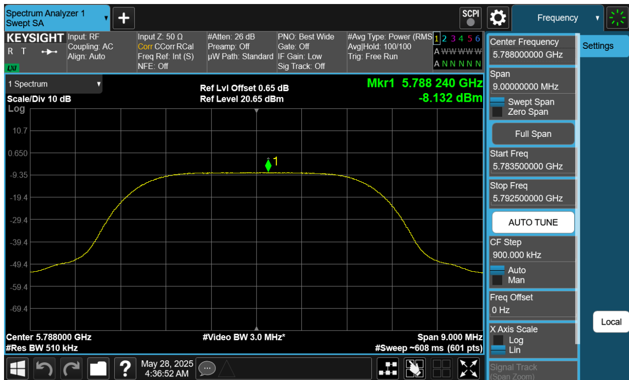
Plot 7-417. PSD TxBF Diversity Antenna 4a (NB UNII XHDRPM6, iPA – 5788MHz)
