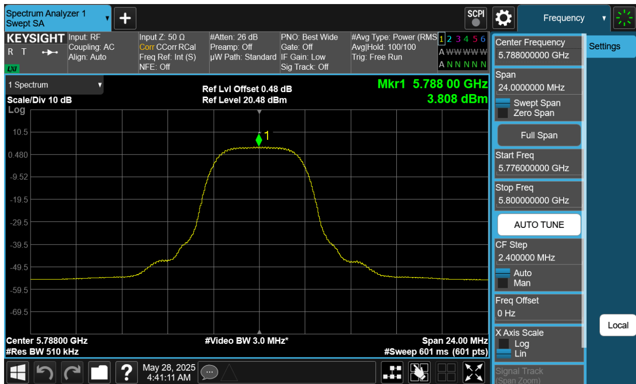
Plot 7-419. PSD TxBF Diversity Antenna 4a (NB UNII HDRPM16, ePA – 5788MHz)
