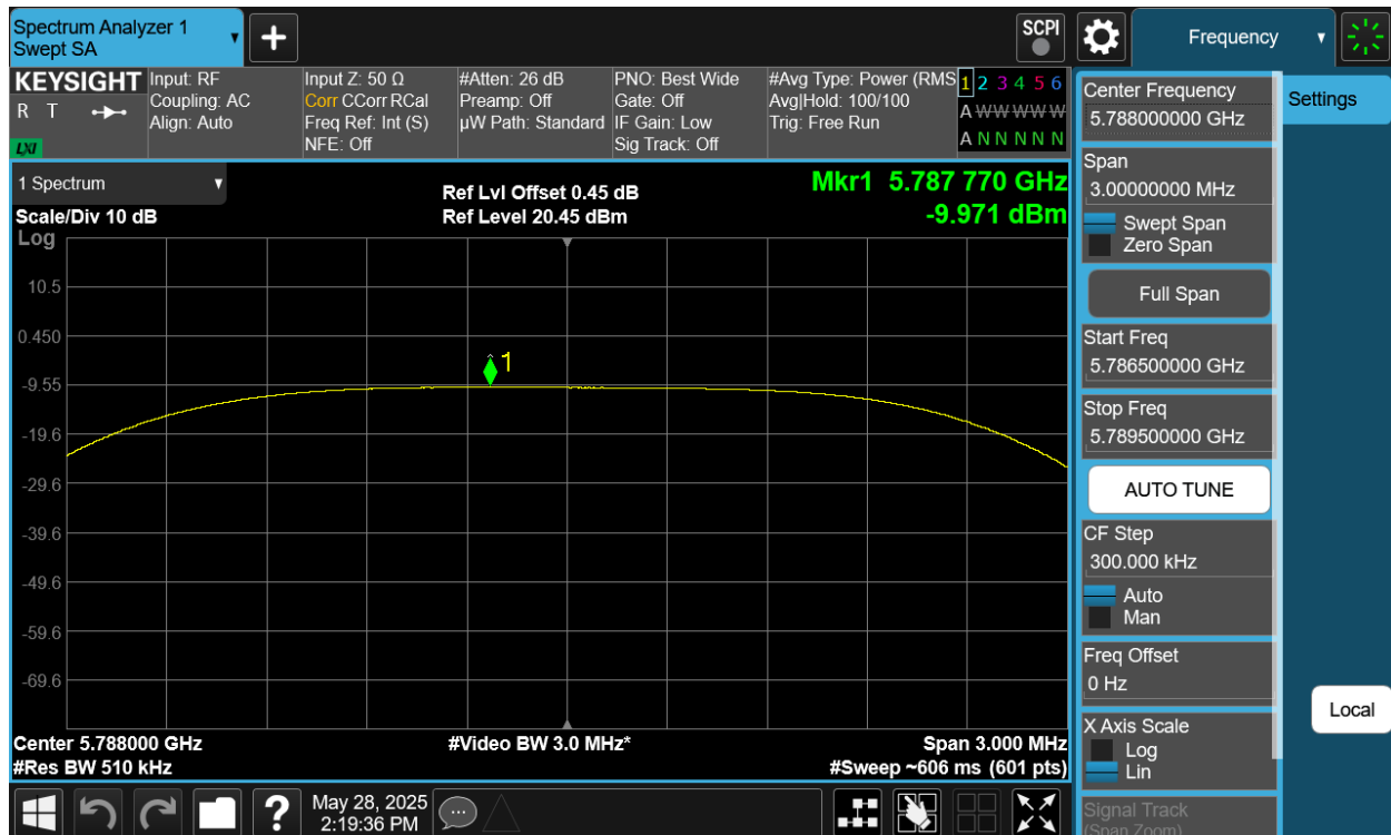
Plot 7-442. PSD Tx BF Diversity Antenna 2a (NB UNII HDT6, iPA – 5788MHz)
