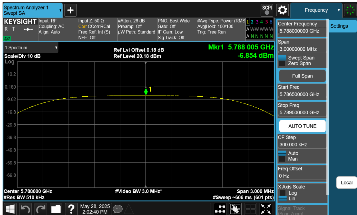
Plot 7-434. PSD TxBF Diversity Antenna 2a (NB UNII HDT2, iPA – 5788MHz)
