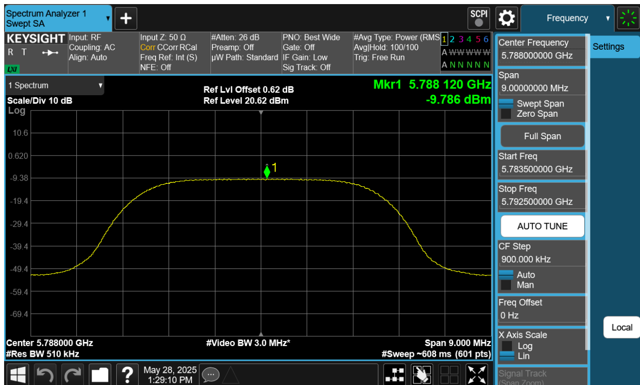
Plot 7-418. PSD TxBF Diversity Antenna 2a (NB UNII XHDRPM6, iPA – 5788MHz)
