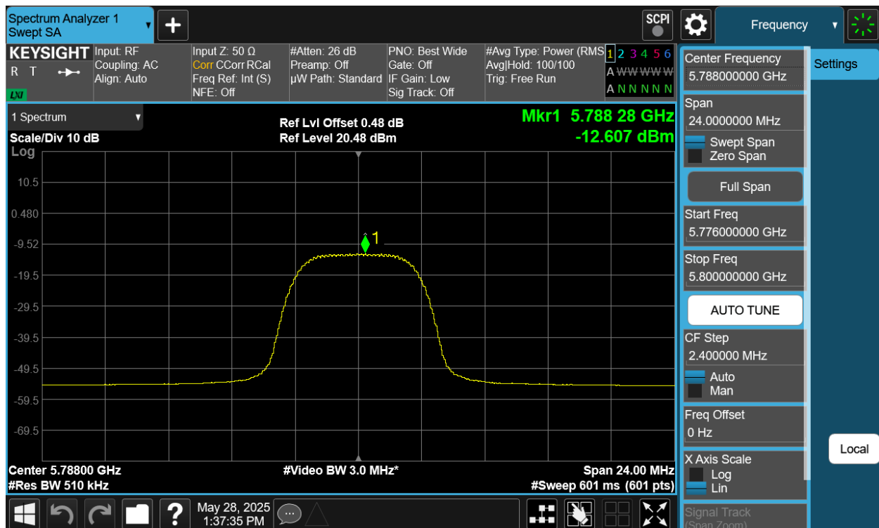
Plot 7-422. PSD TxBF Diversity Antenna 2a (NB UNII HDRPM16, iPA – 5788MHz)
