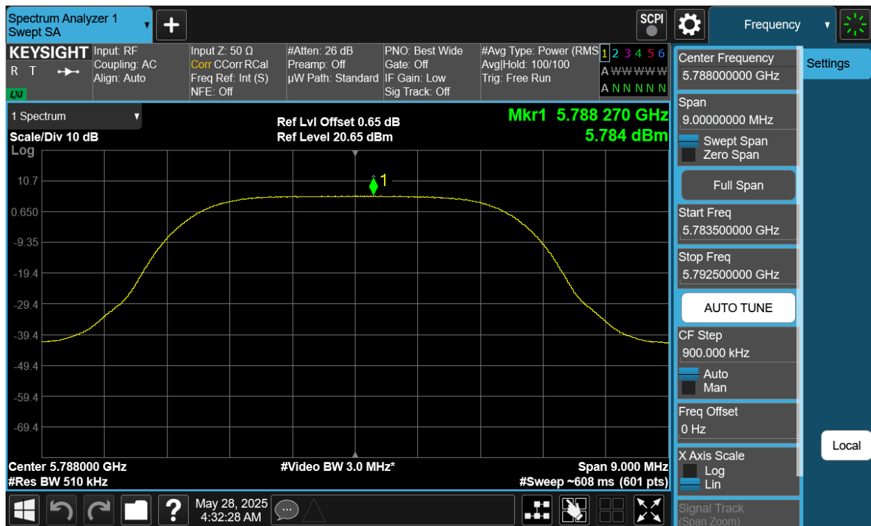
Plot 7-415. PSD Tx BF Diversity Antenna 4a (NB UNII XHDRPM6, ePA – 5788MHz)
