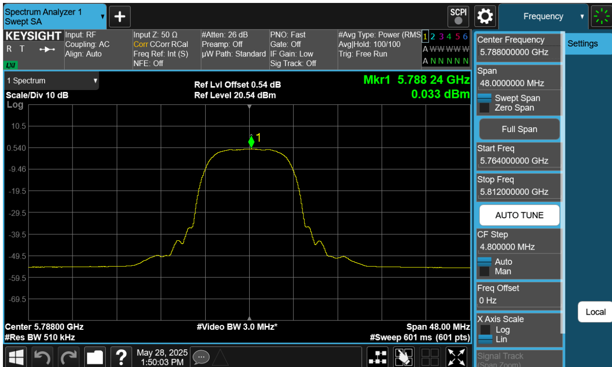
Plot 7-428. PSD TxBF Diversity Antenna 2a (NB UNII HDRPL32, ePA – 5788MHz)
