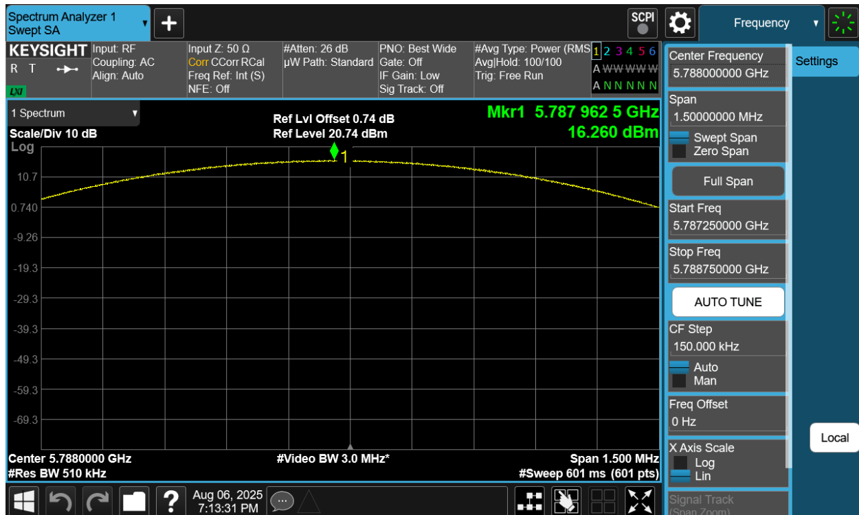
Plot 7-396. PSD Tx BF Diversity Antenna 2a (NB UNII LE1M, ePA – 5788MHz)
