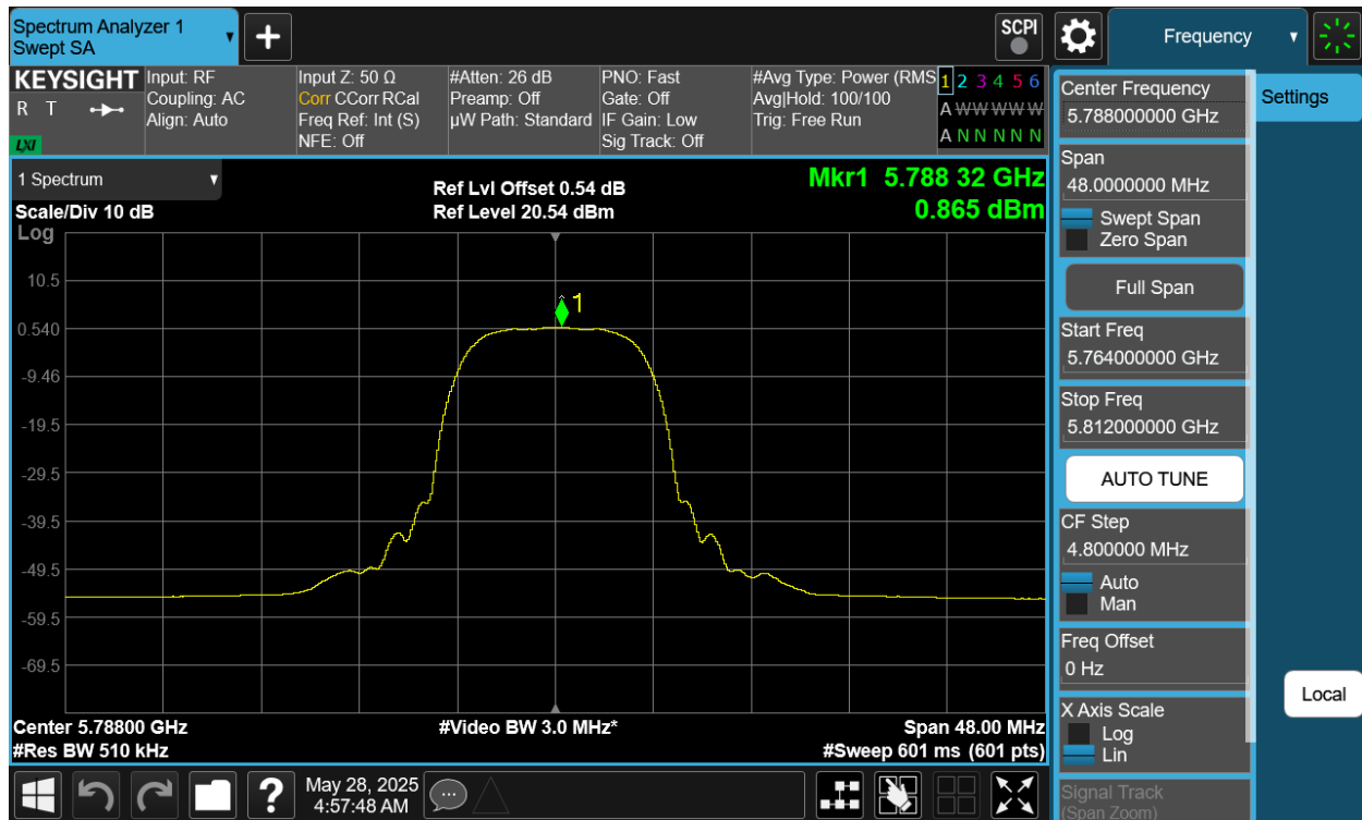
Plot 7-427. PSD TxBF Diversity Antenna 4a (NB UNII HDRPL32, ePA – 5788MHz)
