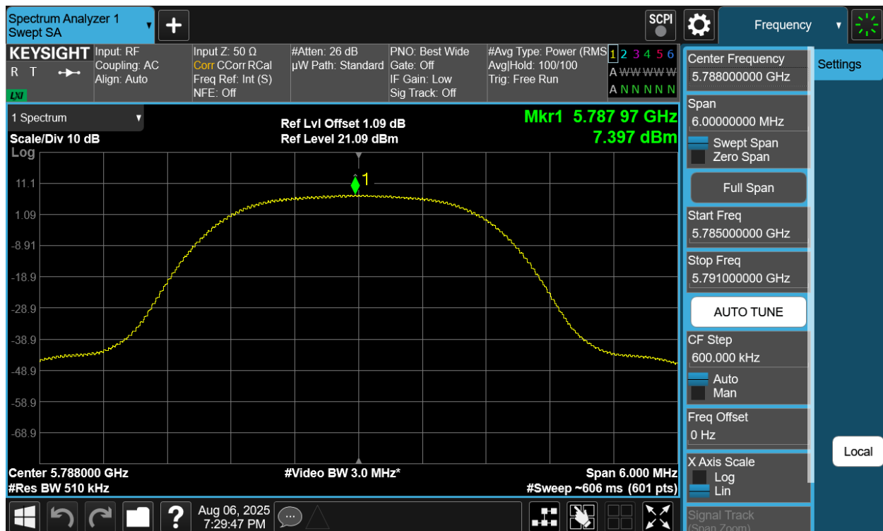
Plot 7-404. PSD TxBF Diversity Antenna 2a (NB UNII HDR4, ePA – 5788MHz)
