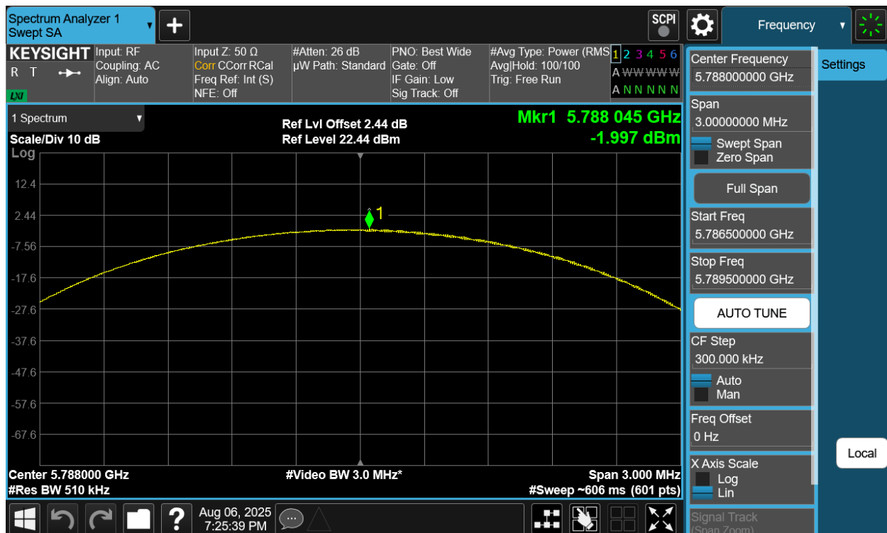
Plot 7-402. PSD Tx BF Diversity Antenna 2a (NB UNII LE2M, iPA – 5788MHz)
