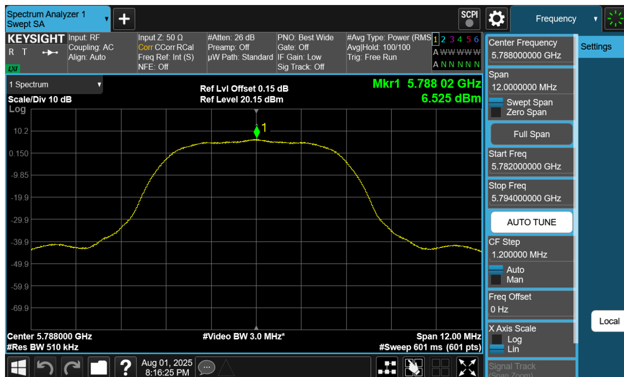
Plot 7-407. PSD TxBF Diversity Antenna 4a (NB UNII HDR8, ePA – 5788MHz)
