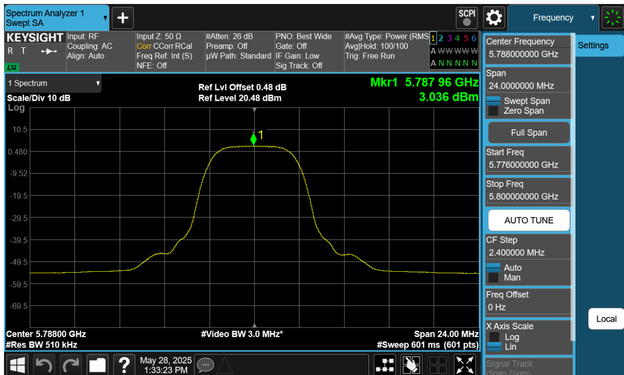
Plot 7-420. PSD TxBF Diversity Antenna 2a (NB UNII HDRPM16, ePA – 5788MHz)
