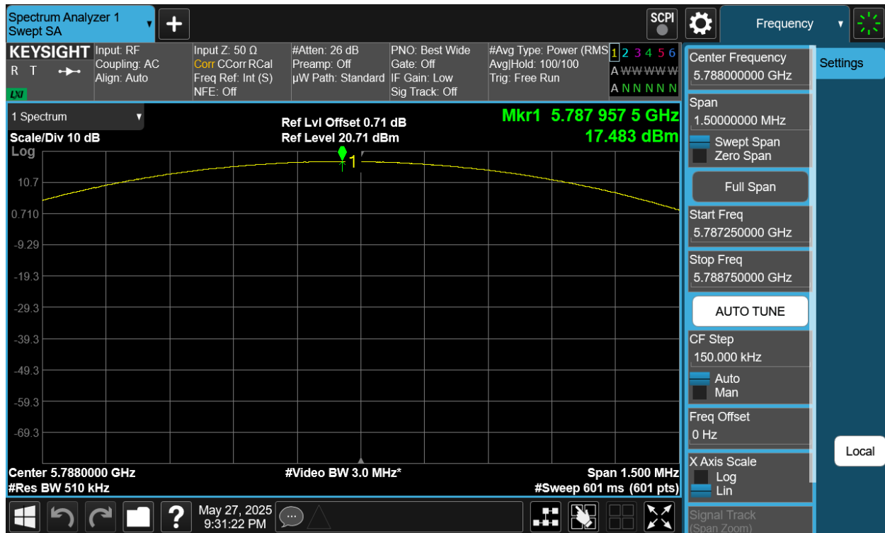
Plot 7-395. PSD Tx BF Diversity Antenna 4a (NB UNII LE1M, ePA – 5788MHz)
