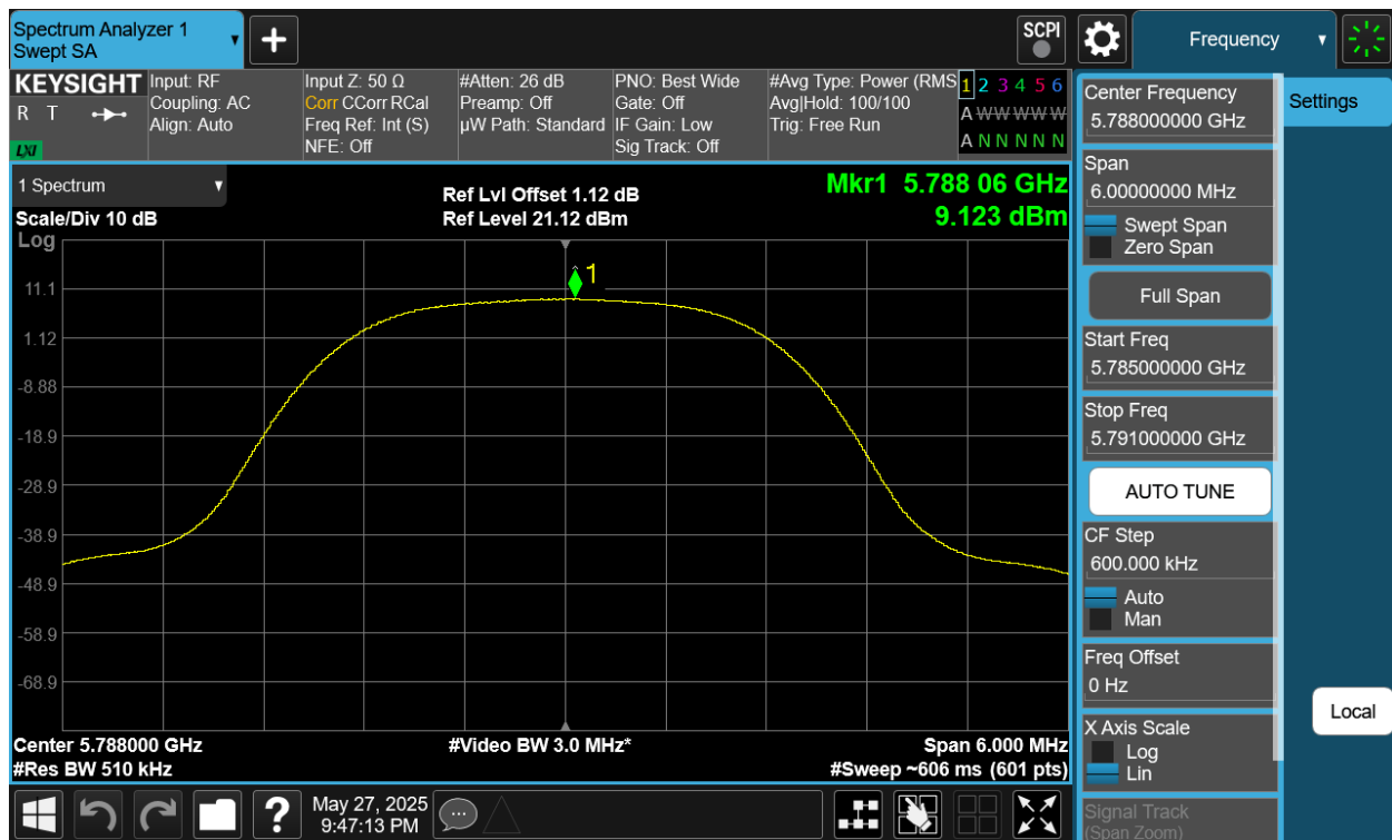
Plot 7-403. PSD TxBF Diversity Antenna 4a (NB UNII HDR4, ePA – 5788MHz)
