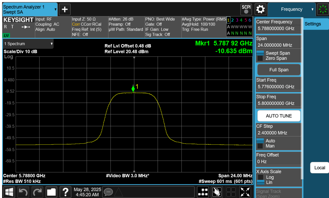
Plot 7-421. PSD TxBF Diversity Antenna 4a (NB UNII HDRPM16, iPA – 5788MHz)
