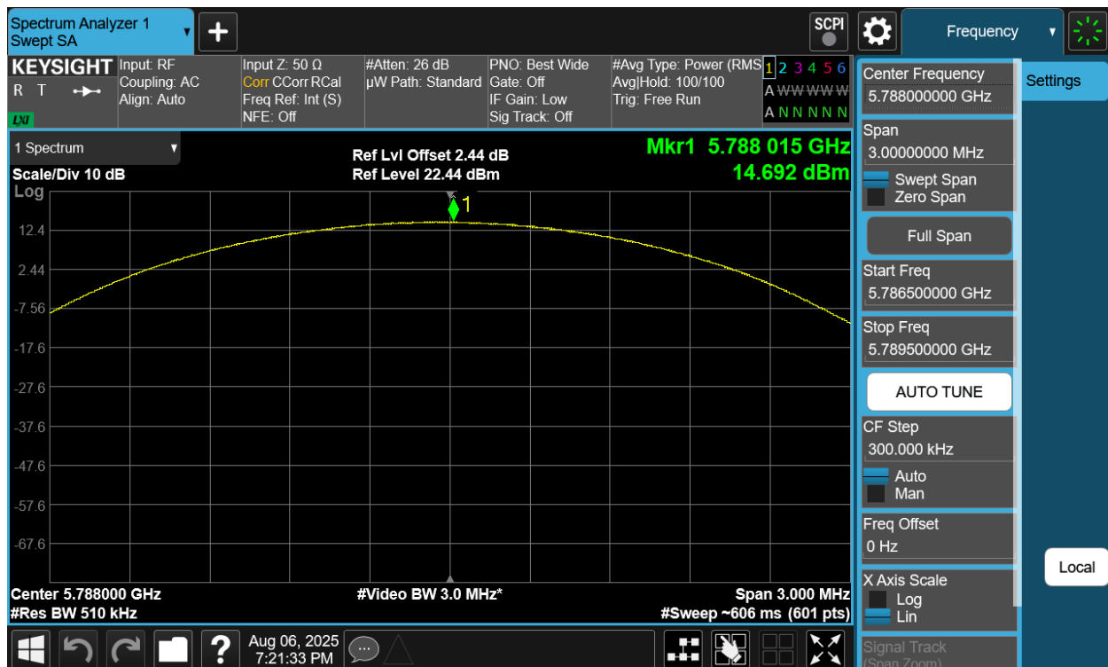
Plot 7-400. PSD TxBF Diversity Antenna 2a (NB UNII LE2M, ePA – 5788MHz)
