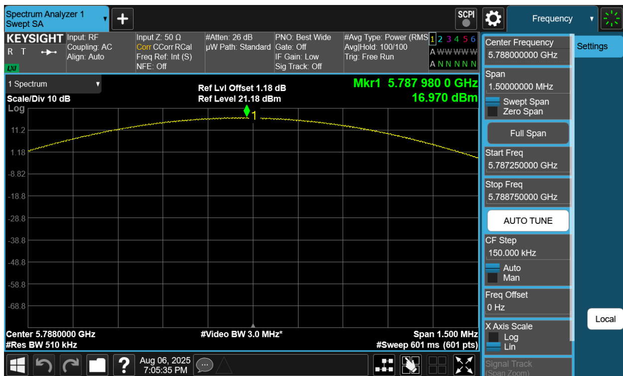
Plot 7-392. PSD Tx B F Diversity Antenna 2a (NB UNII BDR, ePA – 5788MHz)
