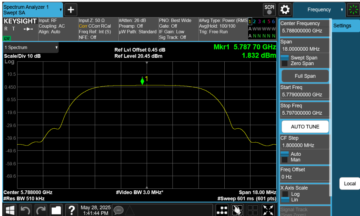
Plot 7-424. PSD TxBF Diversity Antenna 2a (NB UNII HDRPL12, ePA – 5788MHz)
