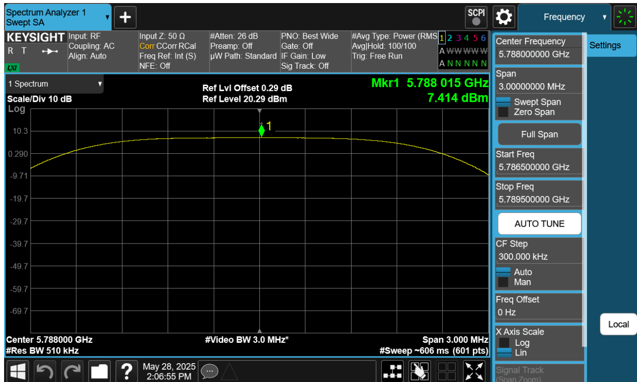
Plot 7-436. PSD Tx BF Diversity Antenna 2a (NB UNII HDT4, ePA – 5788MHz)
