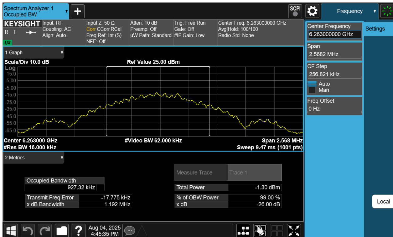
Plot 7-27. 26dB BW & 99% OBW Antenna 2a (NB UNII BDR, ePA- 6263MHz)
