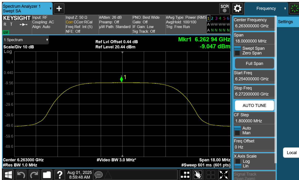
Plot 7-56. PSD Antenna WF5B (NB UNII HDRPL12, ePA – 6263MHz)
