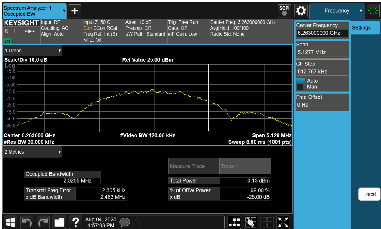
Plot 7-29. 26dB BW & 99% OBW Antenna 2a (NB UNII LE2M, ePA- 6263MHz)
