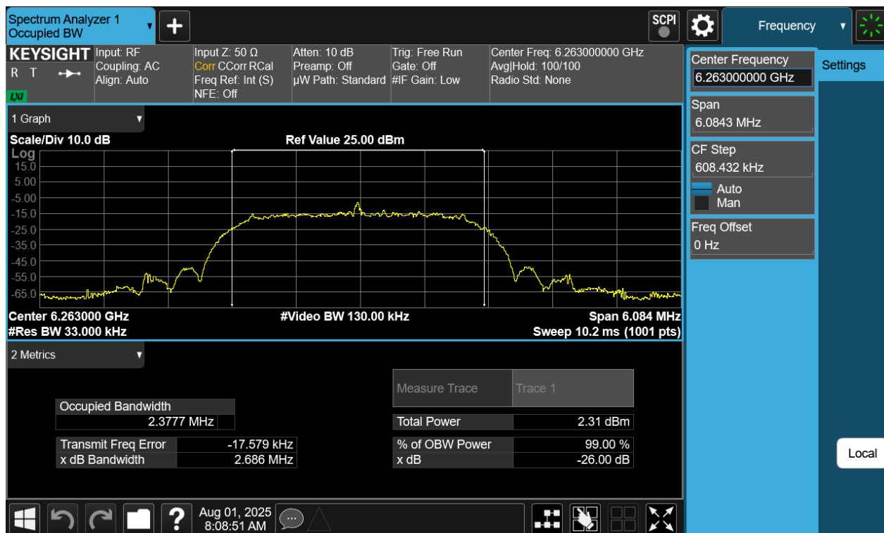
Plot 7-6. 26dB BW & 99% OBW Antenna WF5B (NB UNII HDRPS2, ePA- 6263MHz)
