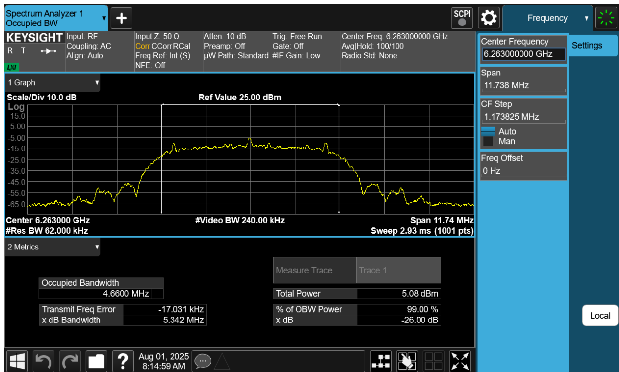
Plot 7-8. 26dB BW & 99% OBW Antenna WF5B (NB UNII HDRPM16, ePA- 6263MHz)
