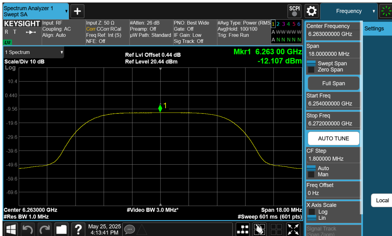
Plot 7-57. PSD Antenna WF5B (NB UNII HDRPL12, iPA – 6263MHz)
