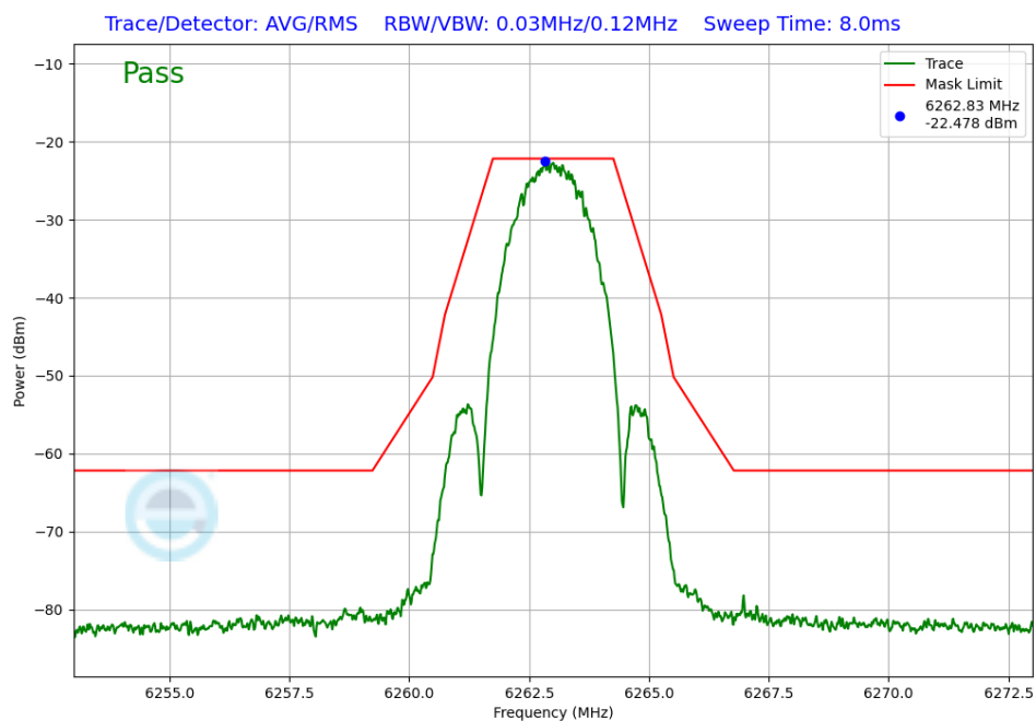
Plot 7-252. In-Band Emission Antenna 4a (NB UNII LE2M, ePA – 6263MHz)
