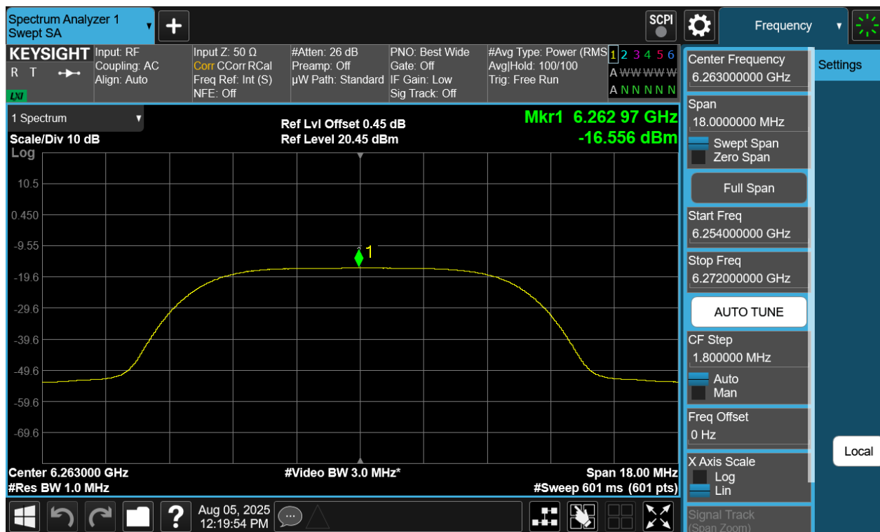
Plot 7-205. PSD TxBF Diversity Antenna 2a (NB UNII HDRPL12, iPA – 6263MHz)
