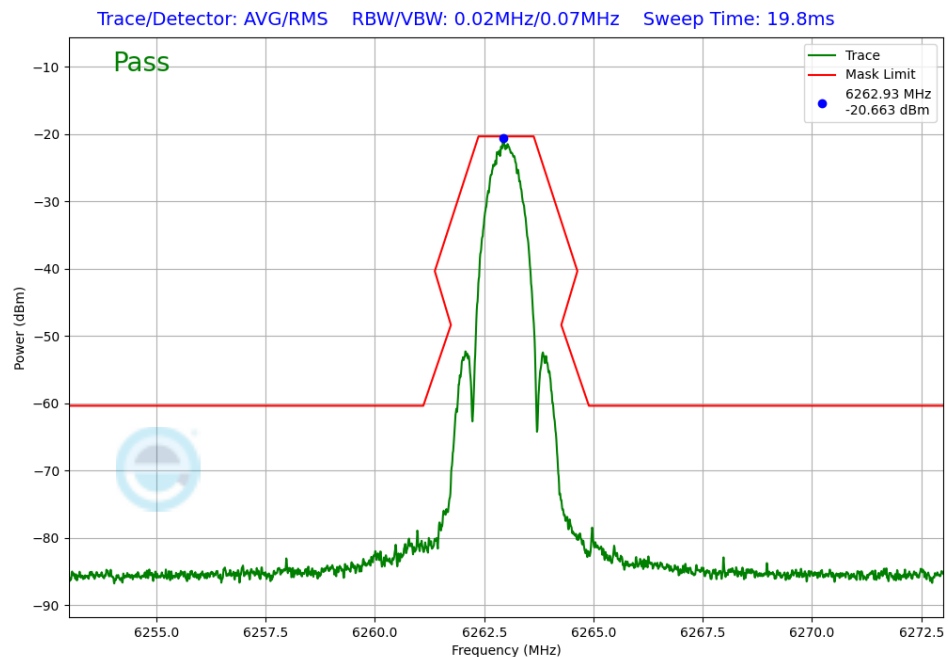
Plot 7-251. In-Band Emission Antenna 4a (NB UNII LE1M, iPA – 6263MHz)
