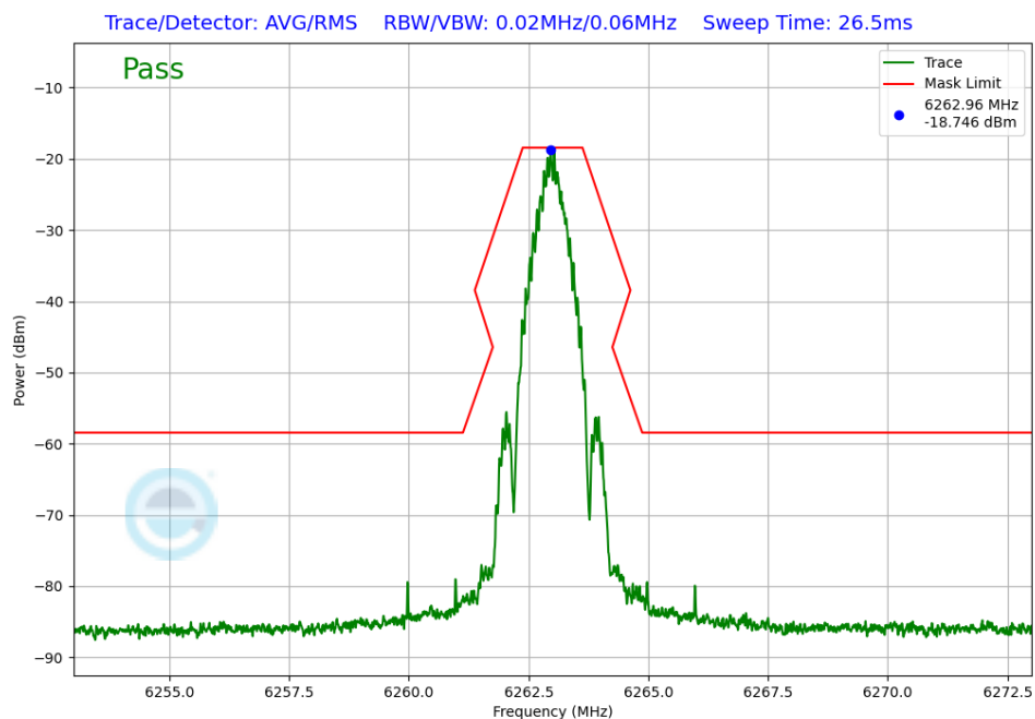
Plot 7-249. In-Band Emission Antenna 4a (NB UNII BDR, iPA – 6263MHz)
