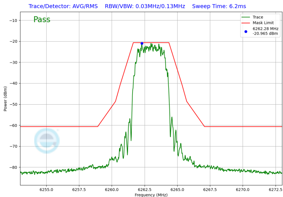
Plot 7-255. In-Band Emission Antenna 4a (NB UNII HDR4, iPA – 6263MHz)
