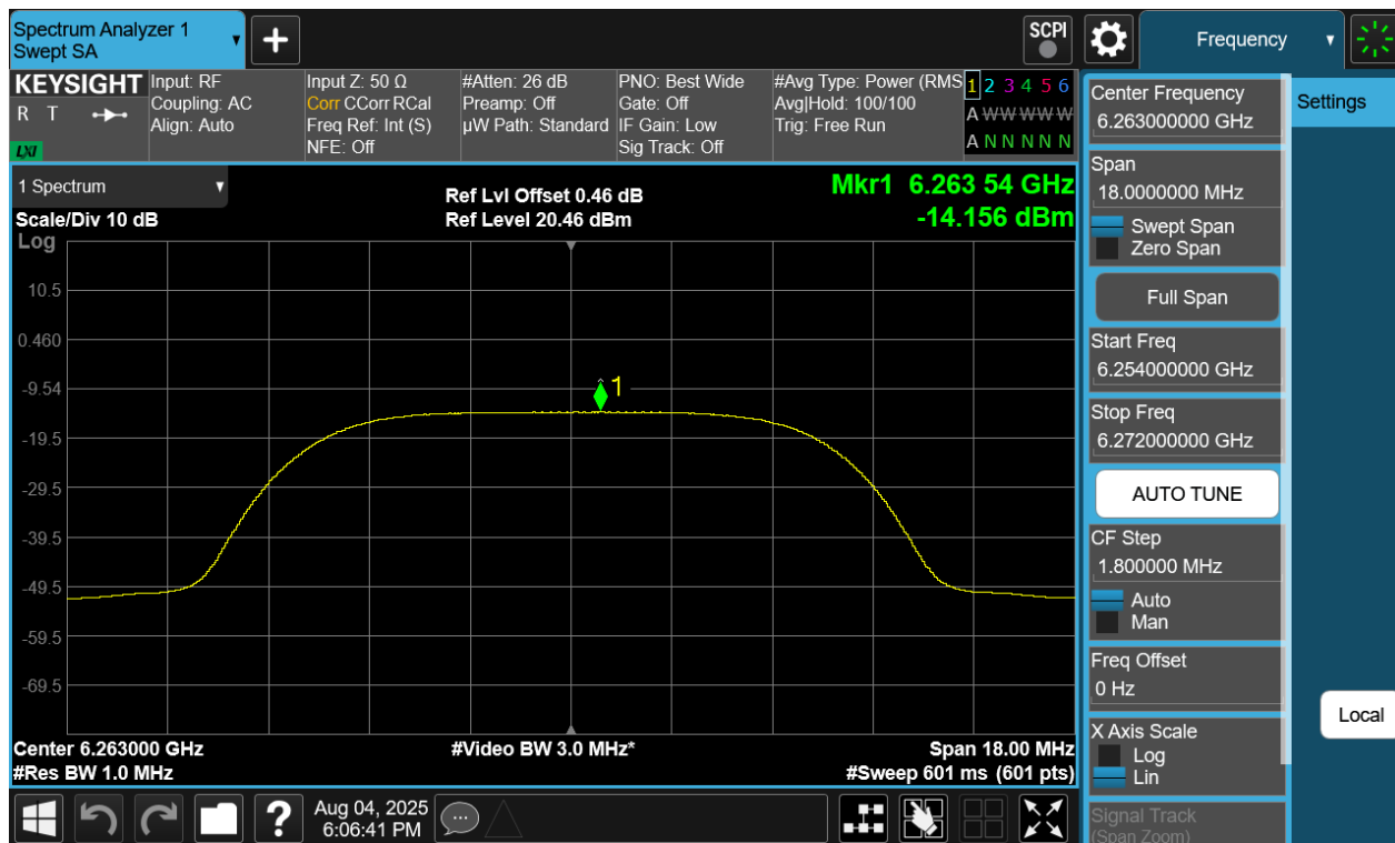
Plot 7-204. PSD TxBF Diversity Antenna 4a (NB UNII HDRPL12, iPA – 6263MHz)
