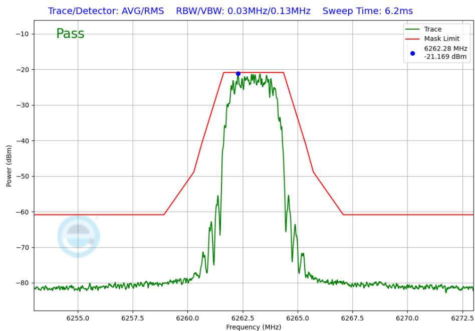
Plot 7-254. In-Band Emission Antenna 4a (NB UNII HDR4, ePA – 6263MHz)
