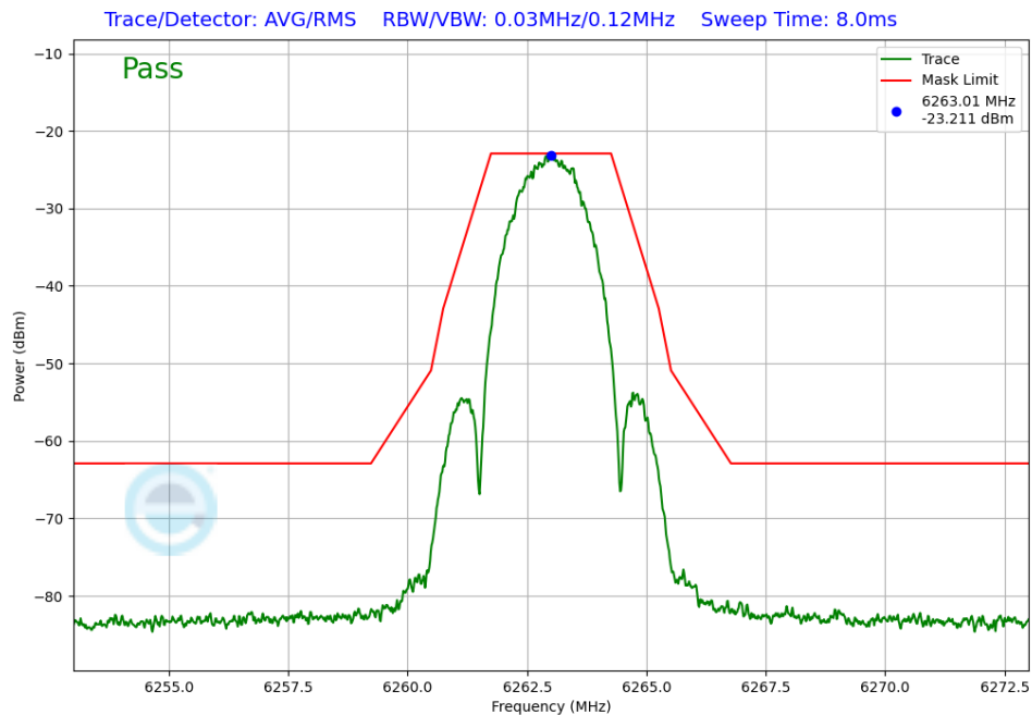
Plot 7-253. In-Band Emission Antenna 4a (NB UNII LE2M, iPA – 6263MHz)
