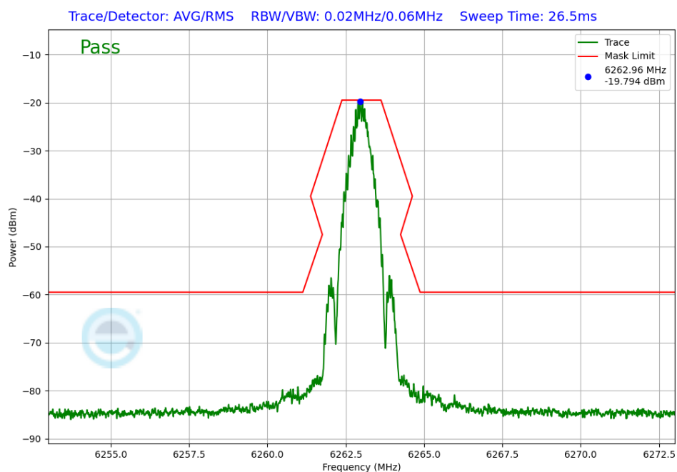
Plot 7-248. In-Band Emission Antenna 4a (NB UNII BDR, ePA – 6263MHz)
