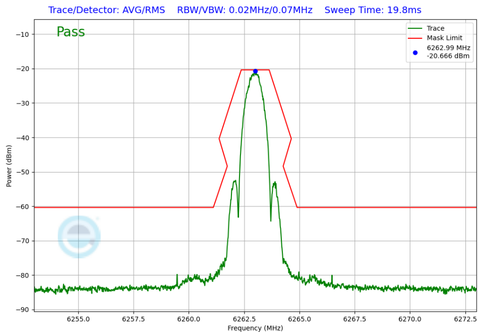
Plot 7-250. In-Band Emission Antenna 4a (NB UNII LE1M, ePA – 6263MHz)
