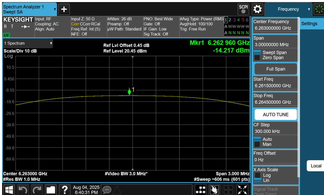
Plot 7-220. PSD TxBF Diversity Antenna 4a (NB UNII HDT6, iPA – 6263MHz)
