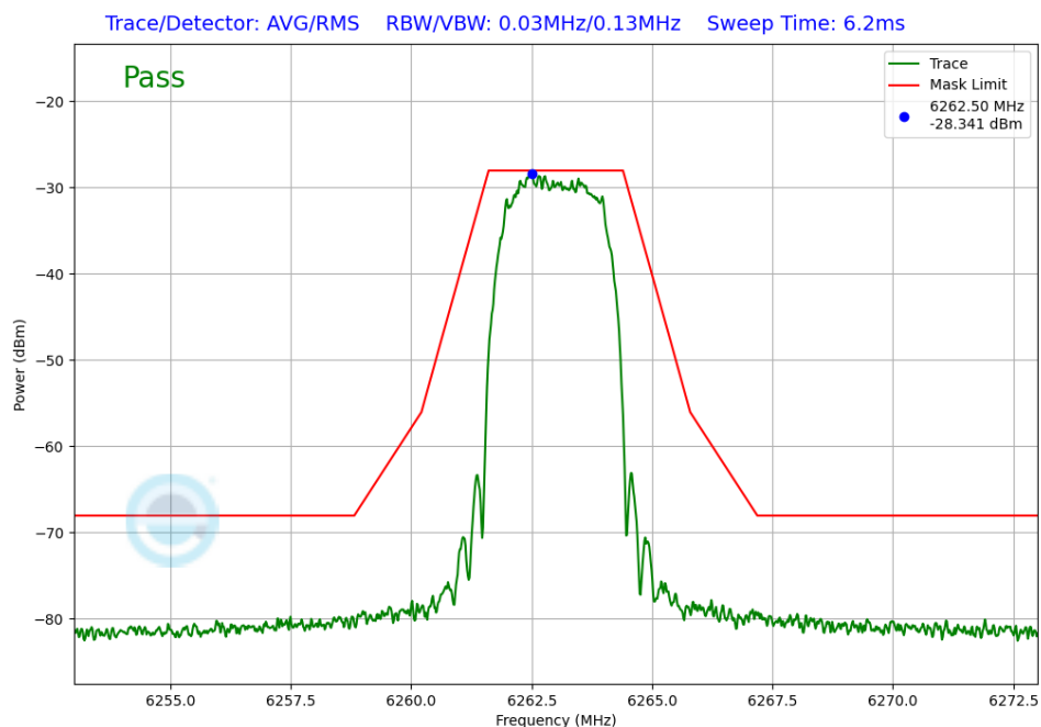
Plot 7-400. In-Band Emission TxBF Diversity Antenna 4a (NB UNII HDT6, ePA – 6263MHz)
