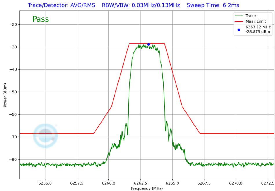
Plot 7-403. In-Band Emission TxBF Diversity Antenna 2a (NB UNII HDT6, iPA – 6263MHz)
