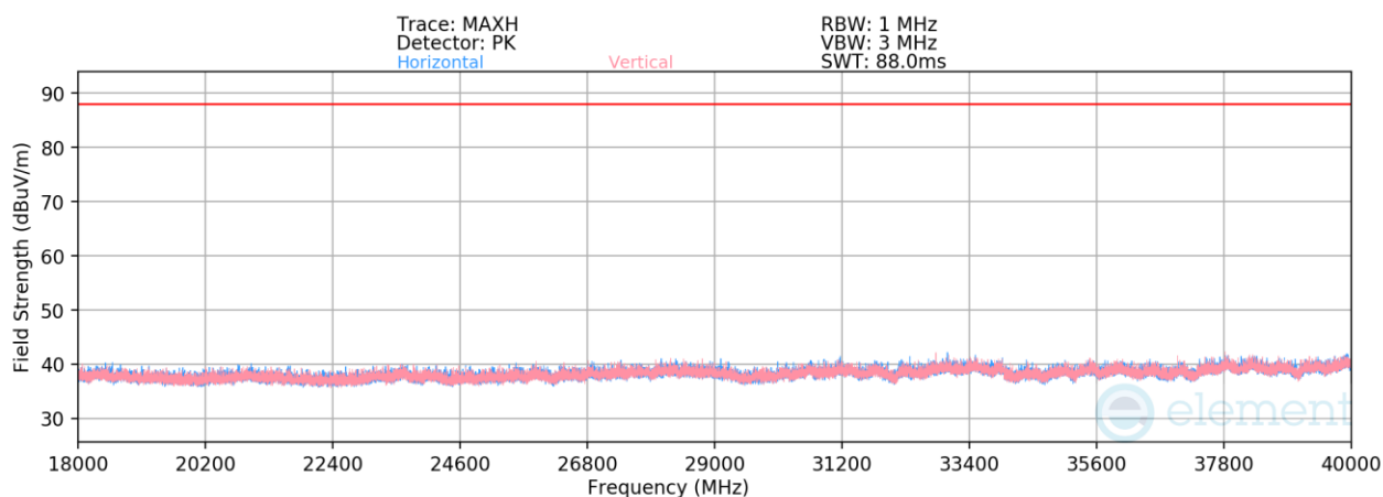
Plot 7-433. Radiated Spurious Emissions Above 18GHz (LE1M GFSK ePA – 6263MHz)
