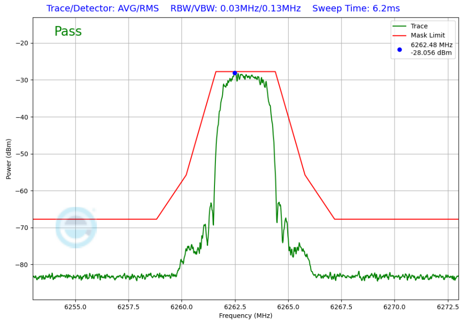
Plot 7-402. In-Band Emission TxBF Diversity Antenna 4a (NB UNII HDT6, iPA – 6263MHz)
