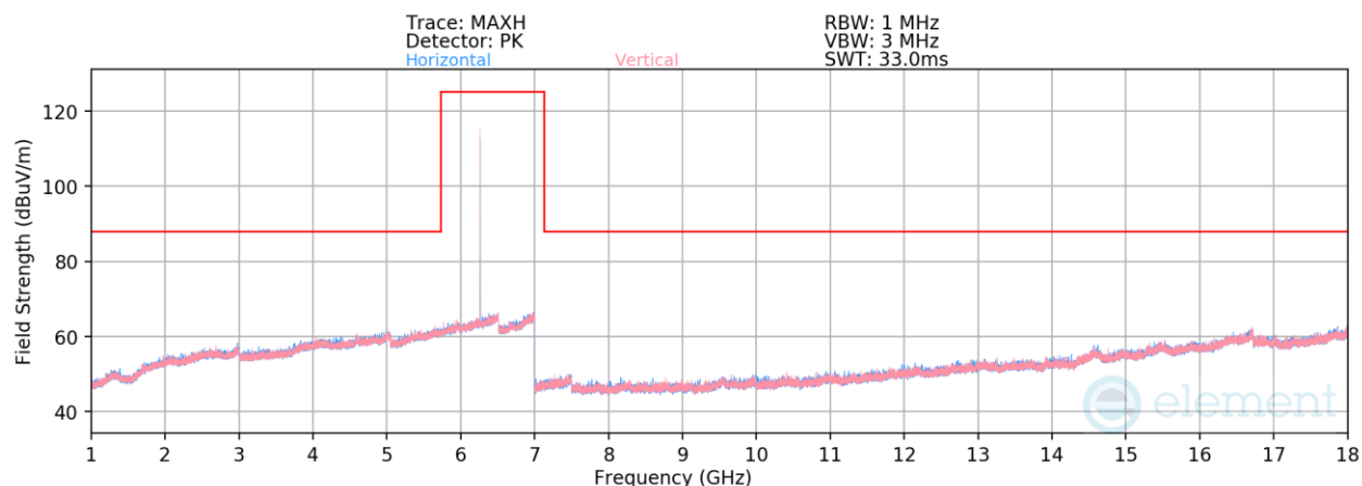
Plot 7-432. Radiated Spurious Emissions 1-18GHz TxBF Diversity (LE1M GFSK ePA – 6263MHz)
