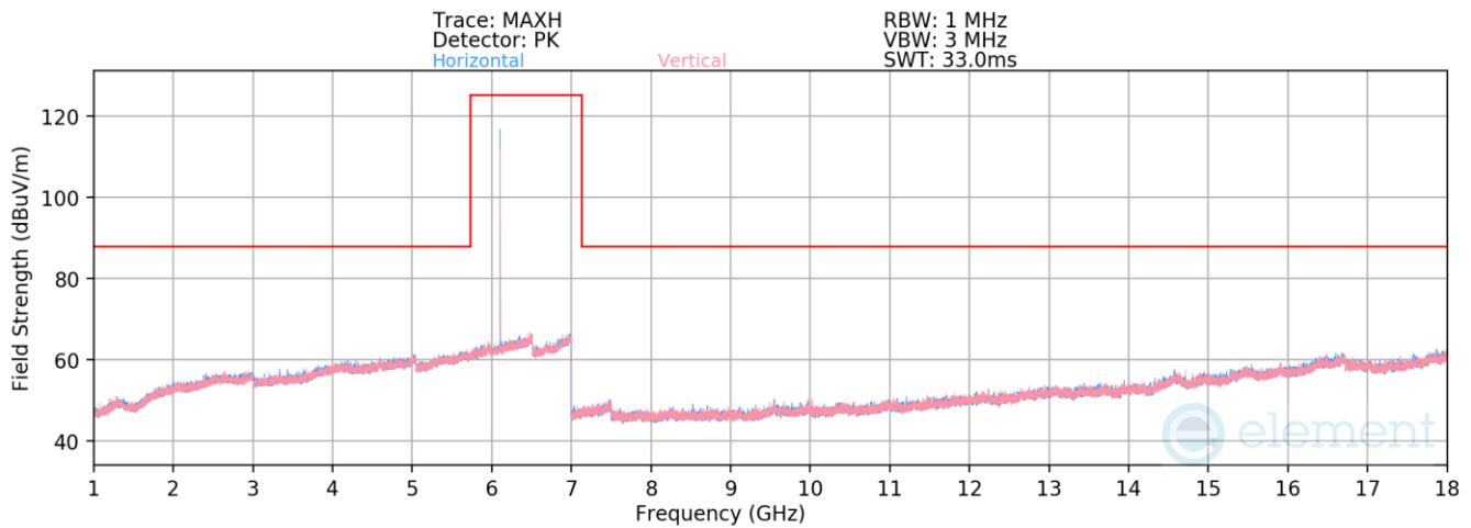
Plot 7-419. Radiated Spurious Emissions 1-18GHz TxBF Primary (LE1M GFSK ePA – 6106MHz)
