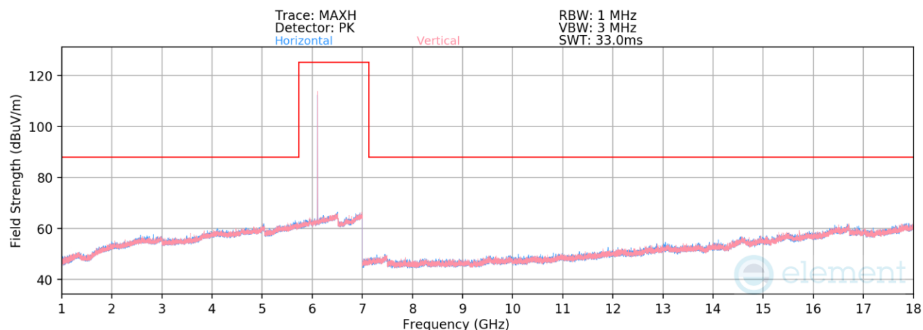
Plot 7-427. Radiated Spurious Emissions 1-18GHz TxBF Diversity (HDR4 GFSK ePA – 6106MHz)
