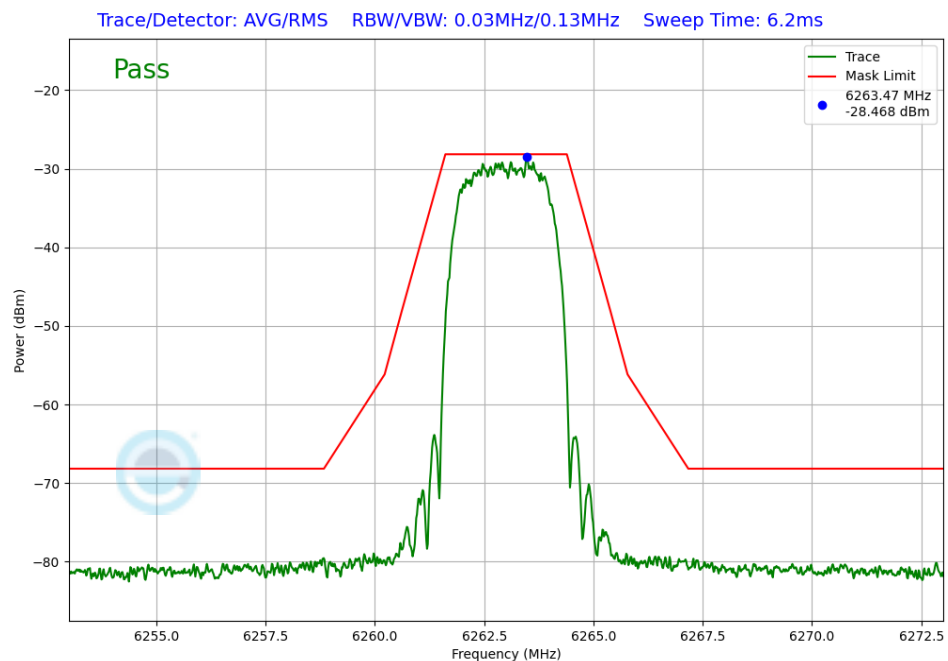
Plot 7-401. In-Band Emission TxBF Diversity Antenna 2a (NB UNII HDT6, ePA – 6263MHz)
