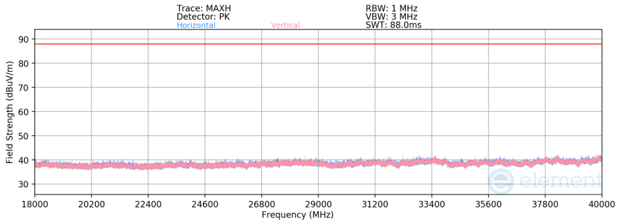
Plot 7-429. Radiated Spurious Emissions Above 18GHz (HDR4 GFSK ePA – 6263MHz)
