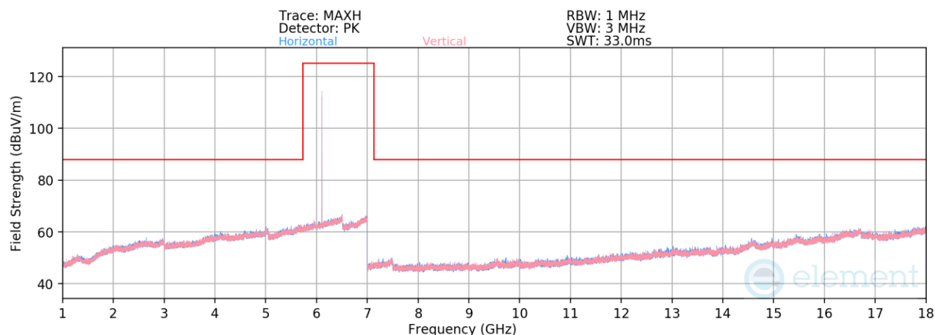
Plot 7-431. Radiated Spurious Emissions 1-18GHz TxBF Diversity (LE1M GFSK ePA – 6106MHz)
