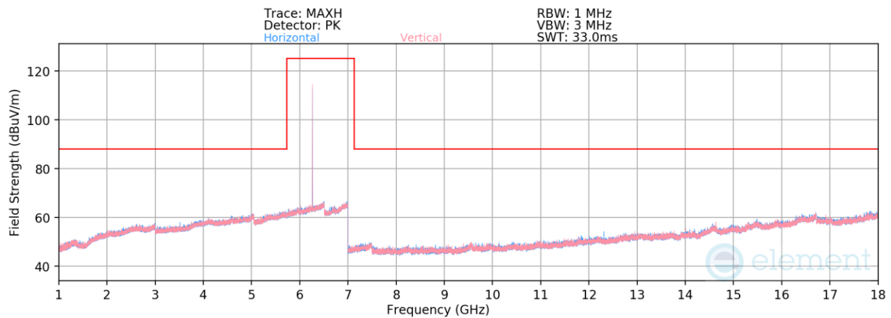
Plot 7-428. Radiated Spurious Emissions 1-18GHz TxBF Diversity (HDR4 GFSK ePA – 6263MHz)
