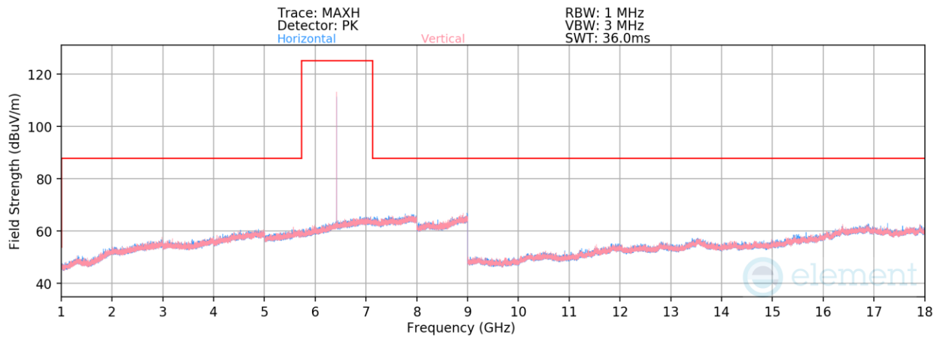
Plot 7-422. Radiated Spurious Emissions 1-18GHz TxBF Primary (LE1M GFSK ePA – 6420MHz)
