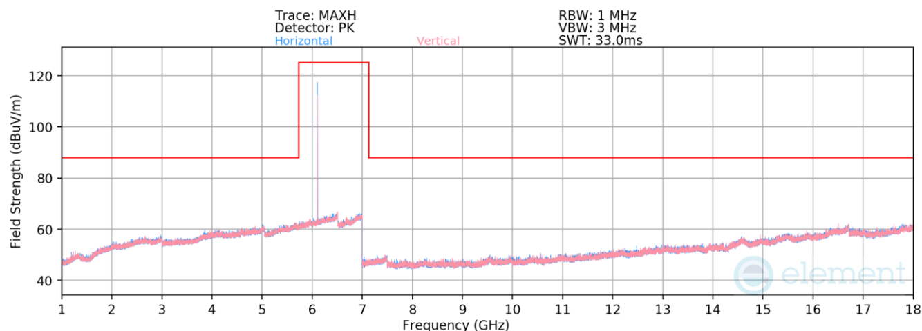
Plot 7-415. Radiated Spurious Emissions 1-18GHz TxBF Primary (HDR4 GFSK ePA – 6106MHz)
