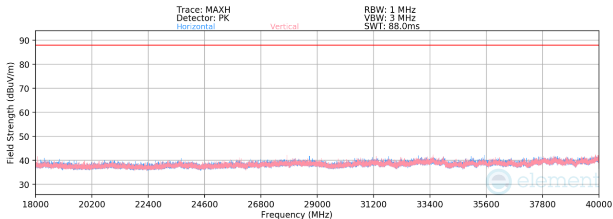
Plot 7-421. Radiated Spurious Emissions Above 18GHz (LE1M GFSK ePA – 6263MHz)
