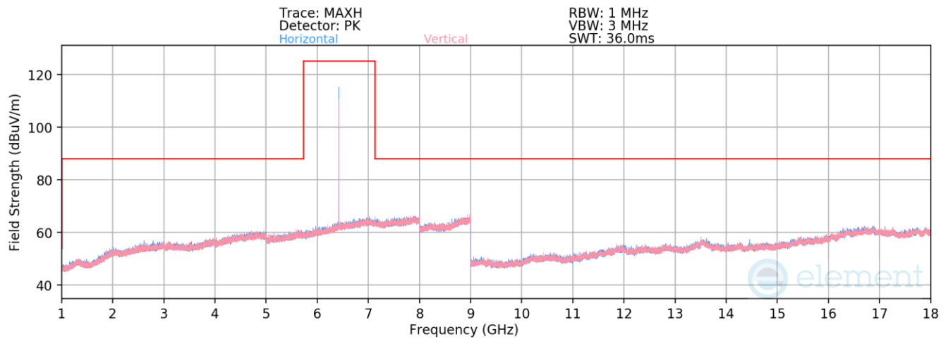
Plot 7-434. Radiated Spurious Emissions 1-18GHz TxBF Diversity (LE1M GFSK ePA - 6420MHz)
