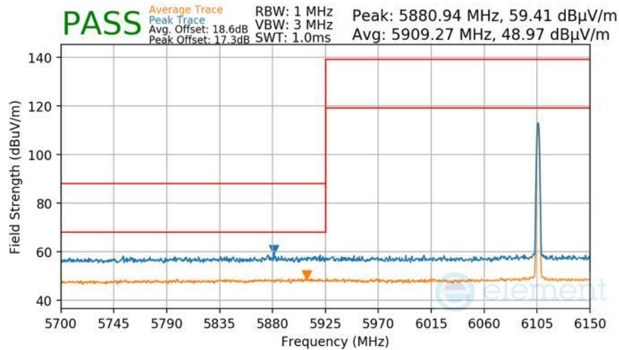
Plot 7-457 Radiated Lower Band Edge Measurement Antenna 2a
