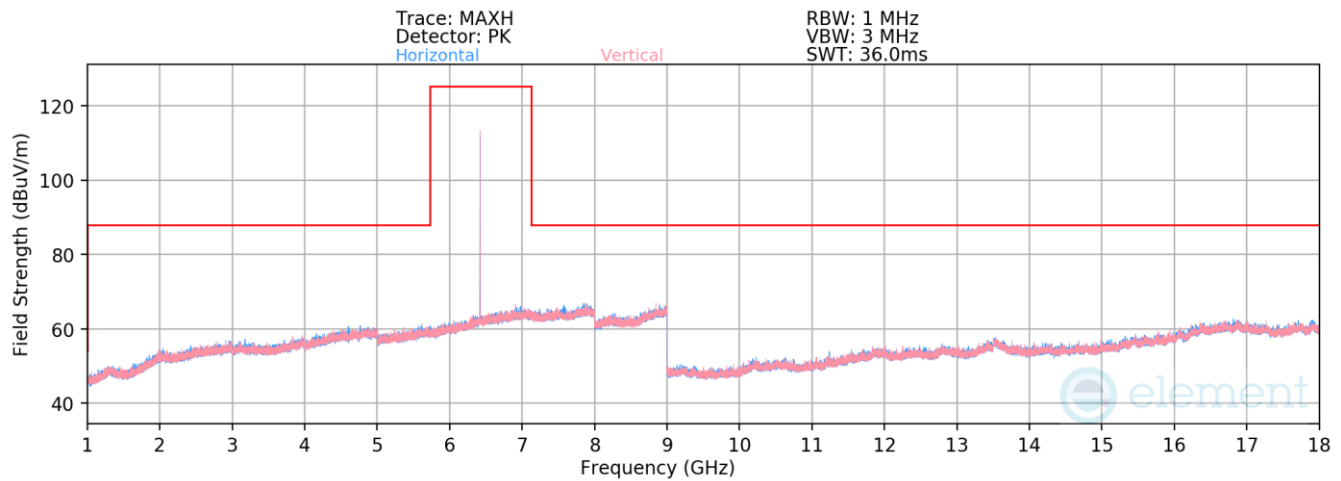
Plot 7-430. Radiated Spurious Emissions 1-18GHz TxBF Diversity (HDR4 GFSK ePA - 6420MHz)
