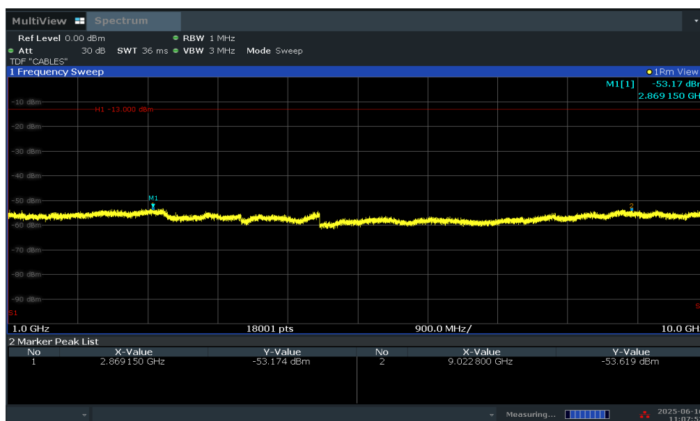
Plot 7-47. Conducted Spurious Plot (LTE Band 26/5 - 10MHz QPSK - RB Size 1, RB Offset 0 - Mid Channel)
