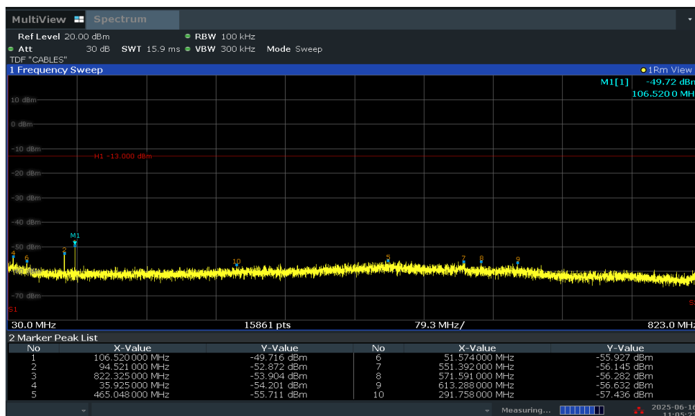
Plot 7-42. Conducted Spurious Plot (LTE Band 26/5 - 10MHz QPSK - RB Size 1, RB Offset 0 - Low Channel)
