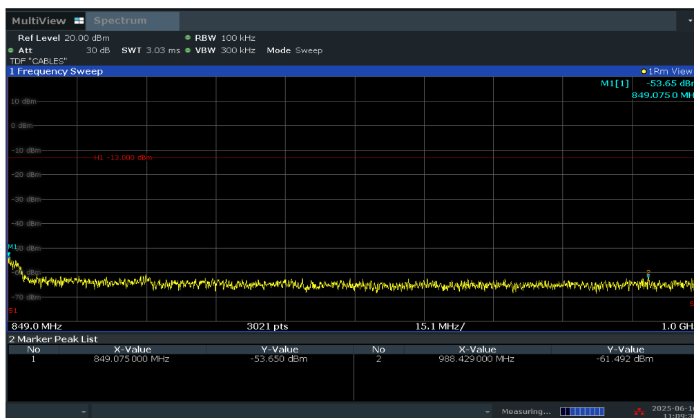
Plot 7-49. Conducted Spurious Plot (LTE Band 26/5 - 10MHz QPSK - RB Size 1, RB Offset 0 - High Channel)
