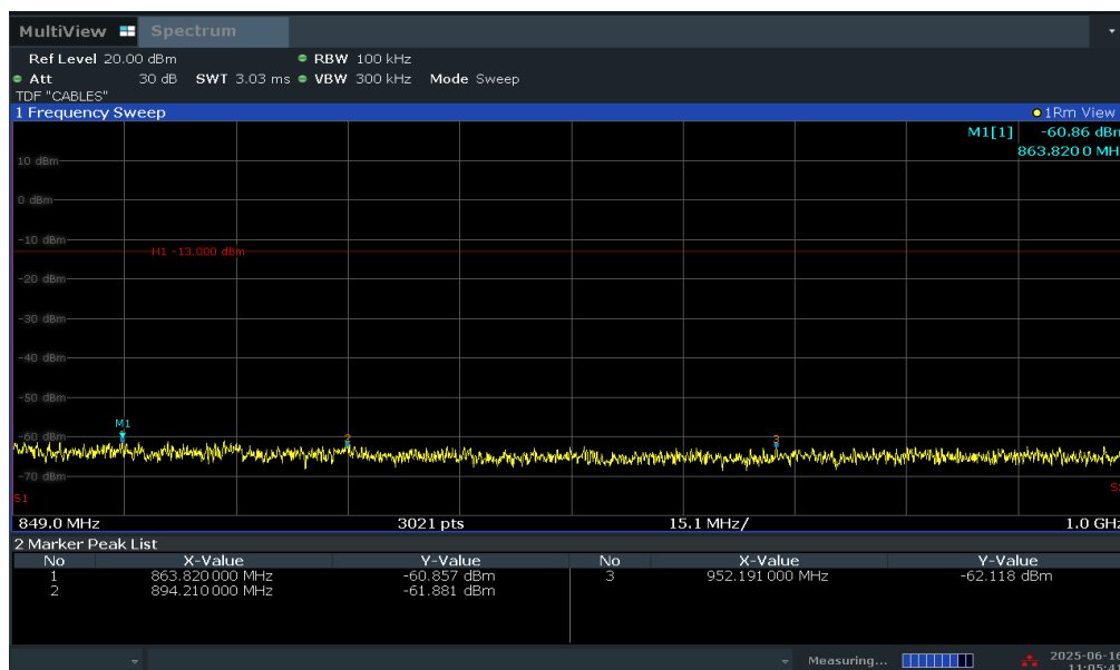
Plot 7-43. Conducted Spurious Plot (LTE Band 26/5 - 10MHz QPSK - RB Size 1, RB Offset 0 - Low Channel)
