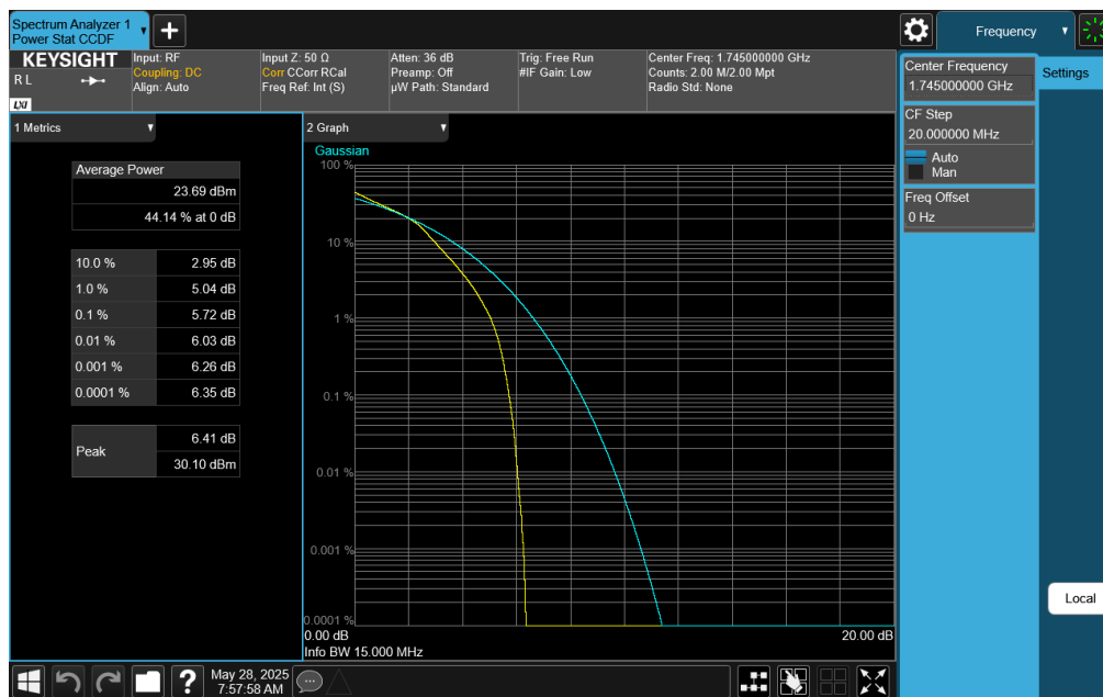
Plot 7-400. PAR Plot (LTE Band 66 - 15MHz 16-QAM - Full RB)
