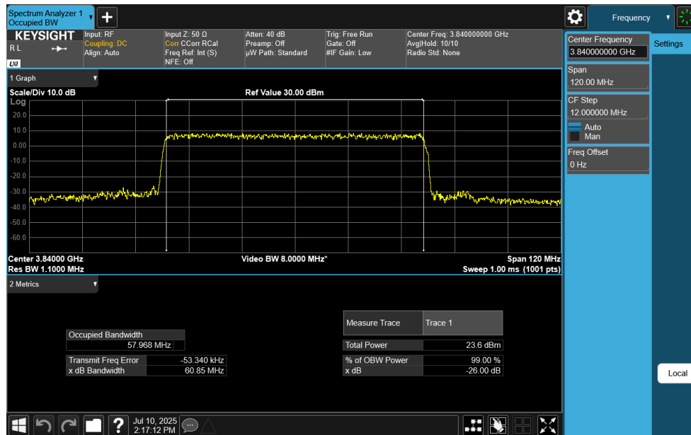
Plot 7-97. Occupied Bandwidth Plot (NR Band n77 C-Band - 60MHz CP-OFDM QPSK - Full RB)
