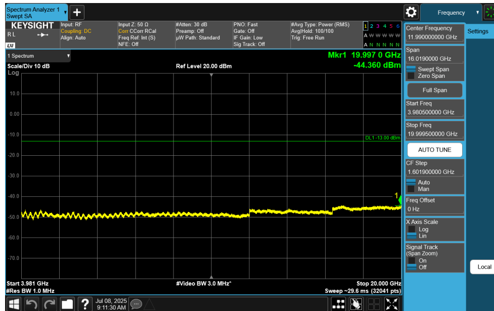
Plot 7-134. Conducted Spurious Plot (NR Band n77 C-Band - 100MHz DFT-s-OFDM QPSK – RB Size 1, RB Offset 0 – Mid Channel)
