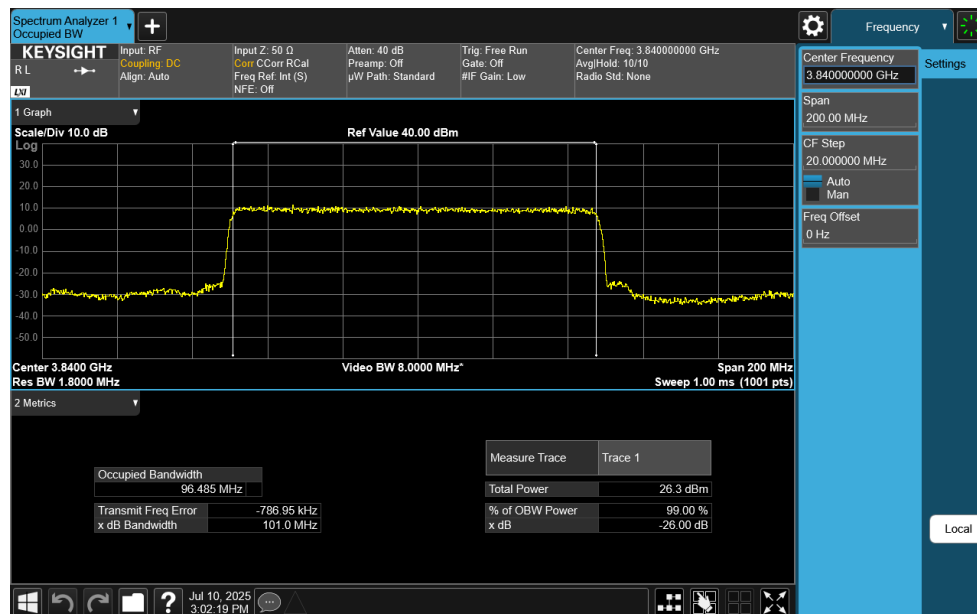
Plot 7-116. Occupied Bandwidth Plot (NR Band n77 C-Band - 100MHz DFT-s-OFDM \pi/2 BPSK - Full RB)
