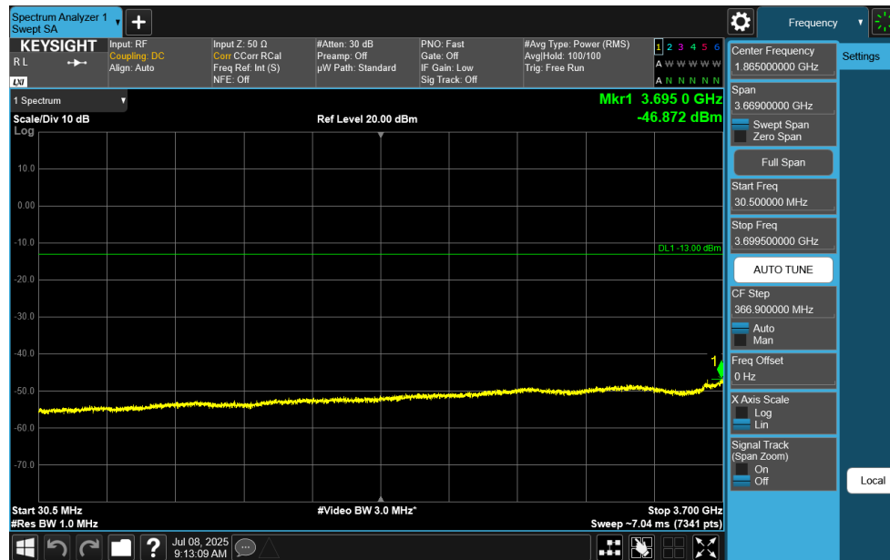
Plot 7-136. Conducted Spurious Plot (NR Band n77 C-Band - 100MHz DFT-s-OFDM QPSK – RB Size 1, RB Offset 0 – High Channel)
