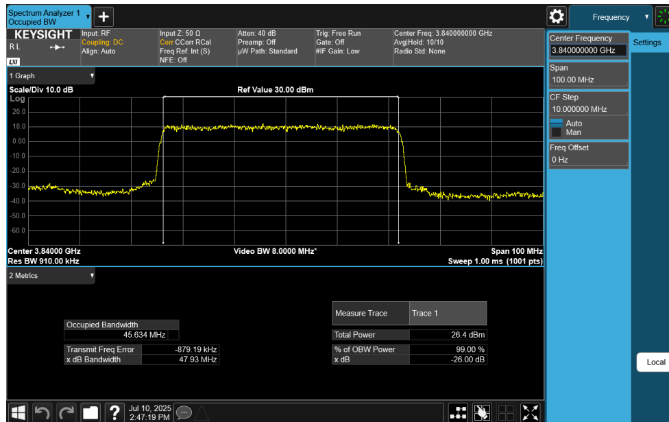
Plot 7-91. Occupied Bandwidth Plot (NR Band n77 C-Band - 50MHz DFT-s-OFDM \pi/2 BPSK - Full RB)
