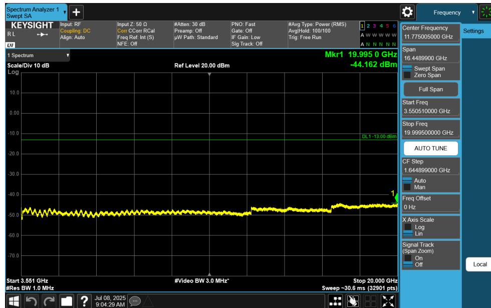
Plot 7-125. Conducted Spurious Plot (NR Band n77 DoD Band - 100MHz DFT-s-OFDM QPSK – RB Size 1, RB Offset 0 – Mid Channel)
