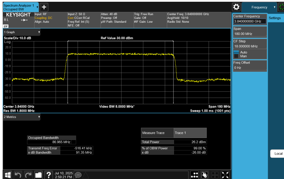
Plot 7-111. Occupied Bandwidth Plot (NR Band n77 C-Band - 90MHz DFT-s-OFDM \pi/2 BPSK - Full RB)
