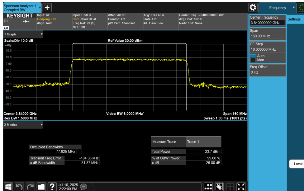
Plot 7-107. Occupied Bandwidth Plot (NR Band n77 C-Band - 80MHz CP-OFDM QPSK - Full RB)
