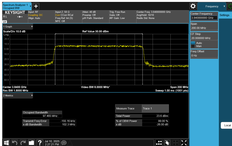
Plot 7-118. Occupied Bandwidth Plot (NR Band n77 C-Band - 100MHz CP-OFDM 16-QAM - Full RB)
