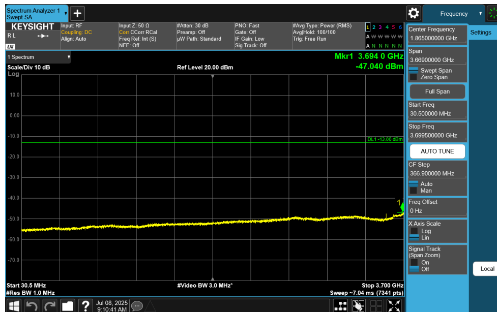
Plot 7-133. Conducted Spurious Plot (NR Band n77 C-Band - 100MHz DFT-s-OFDM QPSK – RB Size 1, RB Offset 0 – Mid Channel)
