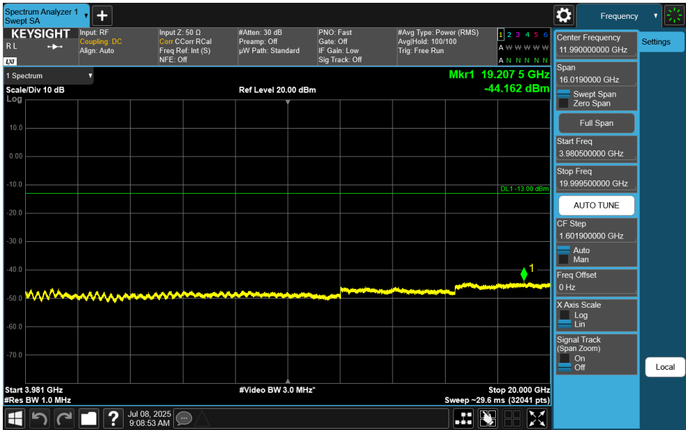
Plot 7-131. Conducted Spurious Plot (NR Band n77 C-Band - 100MHz DFT-s-OFDM QPSK – RB Size 1, RB Offset 0 – Low Channel)
