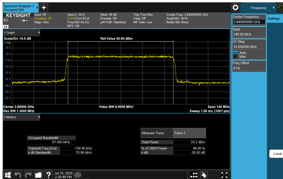
Plot 7-104. Occupied Bandwidth Plot (NR Band n77 C-Band - 70MHz CP-OFDM 64-QAM - Full RB)
