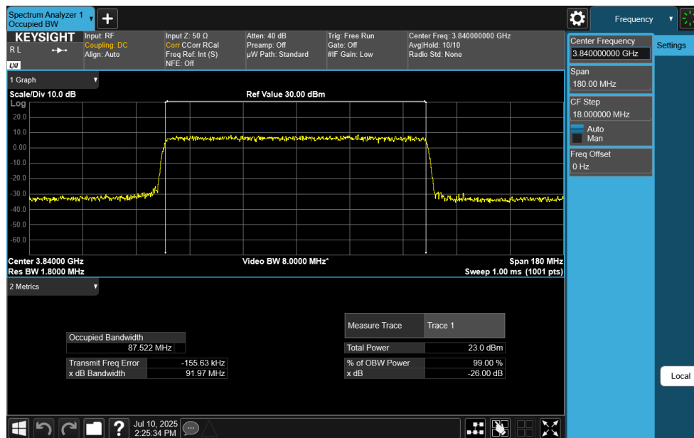
Plot 7-114. Occupied Bandwidth Plot (NR Band n77 C-Band - 90MHz CP-OFDM 64-QAM - Full RB)
