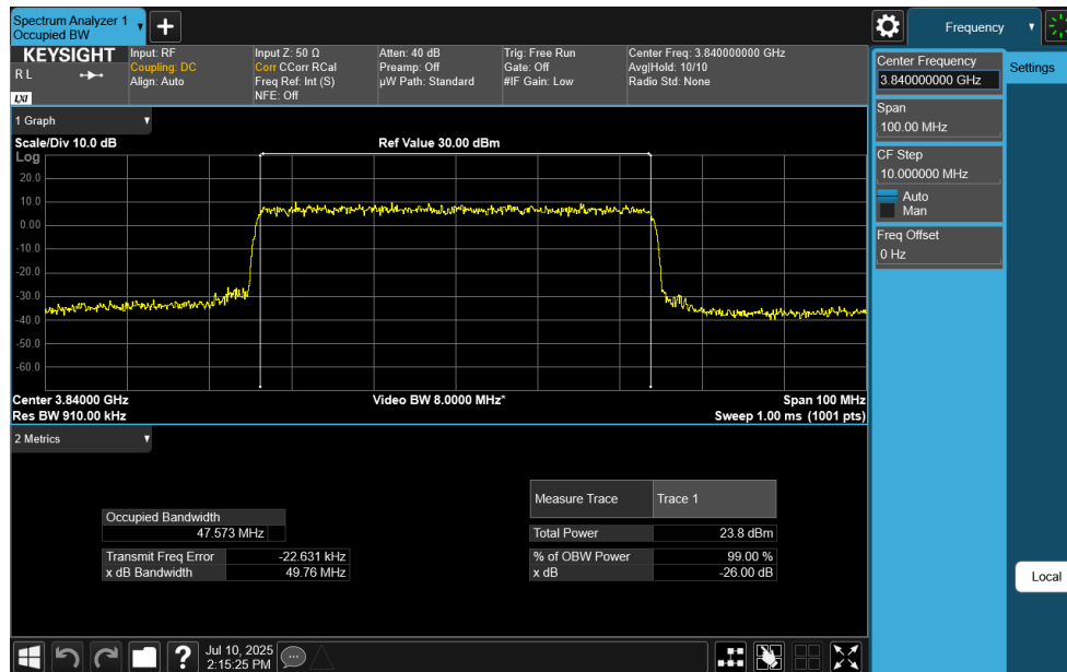
Plot 7-93. Occupied Bandwidth Plot (NR Band n77 C-Band - 50MHz CP-OFDM 16-QAM - Full RB)
