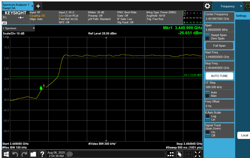
Plot 7-141. Lower Band Edge Plot (NR Band n77 DoD-Band - 10MHz DFT-s-OFDM QPSK – Full RB)
