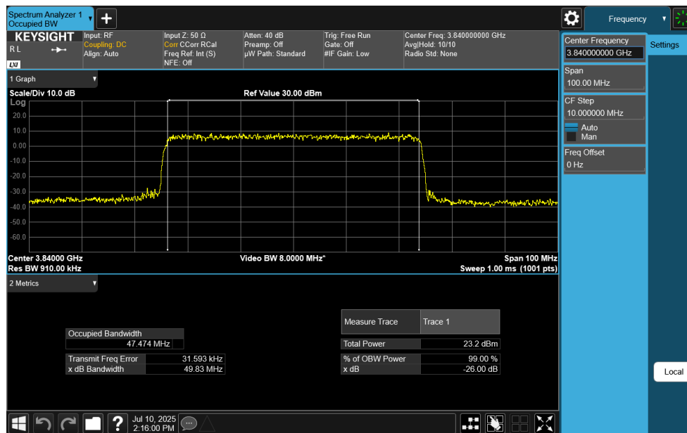
Plot 7-94. Occupied Bandwidth Plot (NR Band n77 C-Band - 50MHz CP-OFDM 64-QAM - Full RB)
