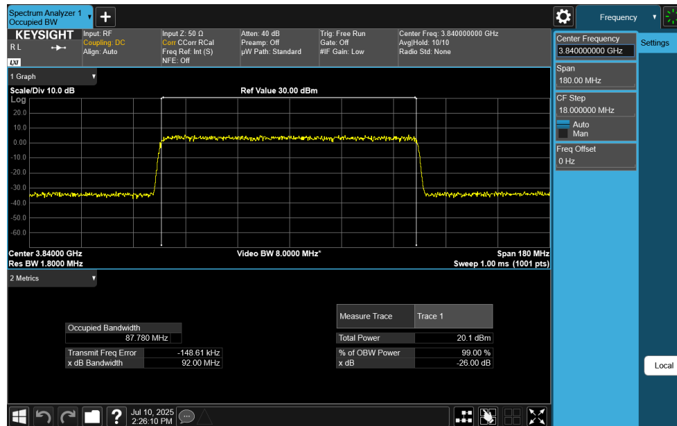
Plot 7-115. Occupied Bandwidth Plot (NR Band n77 C-Band - 90MHz CP-OFDM 256-QAM - Full RB)
