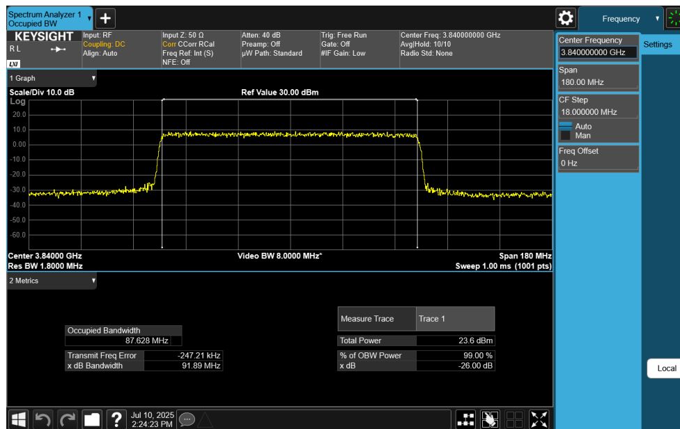
Plot 7-112. Occupied Bandwidth Plot (NR Band n77 C-Band - 90MHz CP-OFDM QPSK - Full RB)
