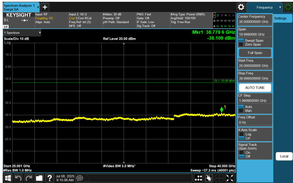
Plot 7-138. Conducted Spurious Plot (NR Band n77 C-Band - 100MHz DFT-s-OFDM QPSK – RB Size 1, RB Offset 0 – High Channel)
