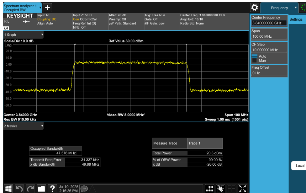
Plot 7-95. Occupied Bandwidth Plot (NR Band n77 C-Band - 50MHz CP-OFDM 256-QAM - Full RB)
