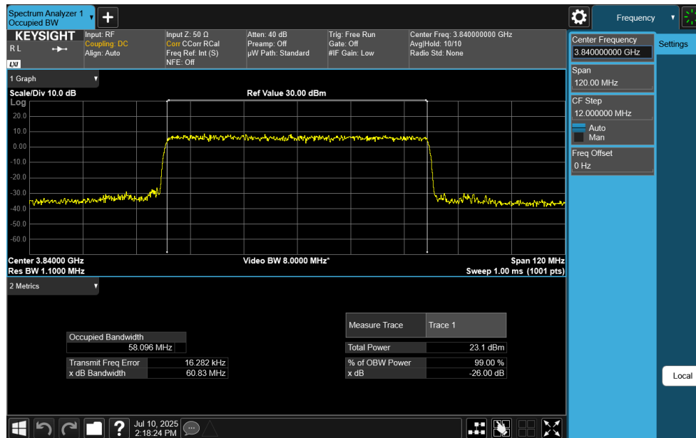
Plot 7-99. Occupied Bandwidth Plot (NR Band n77 C-Band - 60MHz CP-OFDM 64-QAM - Full RB)
