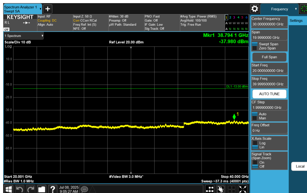
Plot 7-126. Conducted Spurious Plot (NR Band n77 DoD Band - 100MHz DFT-s-OFDM QPSK – RB Size 1, RB Offset 0 – Mid Channel)
