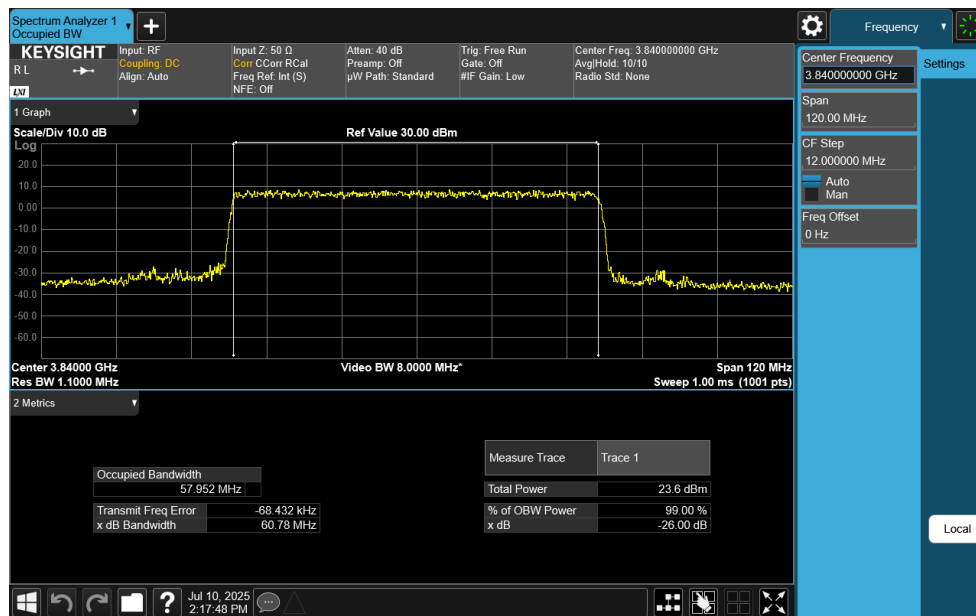
Plot 7-98. Occupied Bandwidth Plot (NR Band n77 C-Band - 60MHz CP-OFDM 16-QAM - Full RB)
