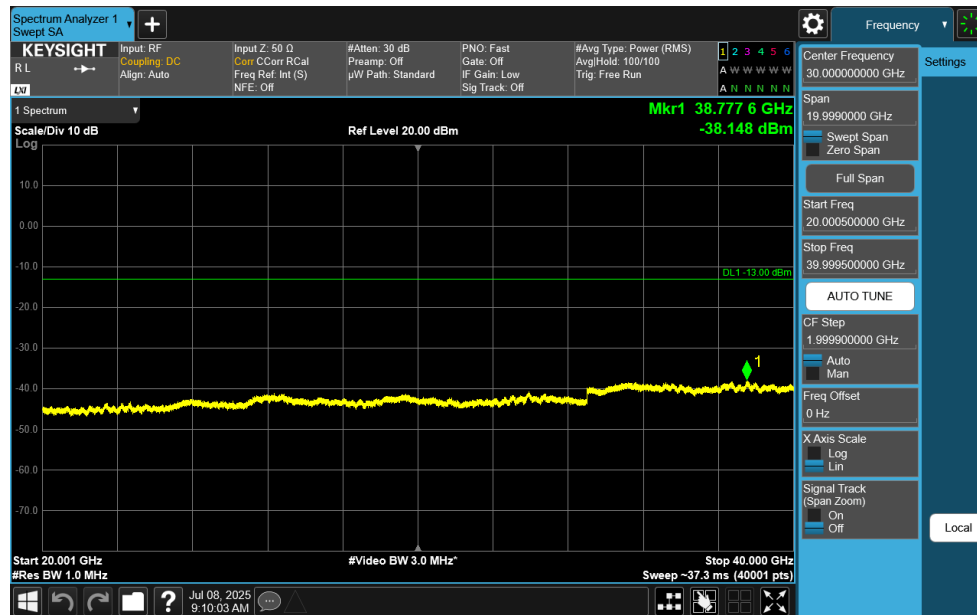
Plot 7-132. Conducted Spurious Plot (NR Band n77 C-Band - 100MHz DFT-s-OFDM QPSK – RB Size 1, RB Offset 0 – Low Channel)
