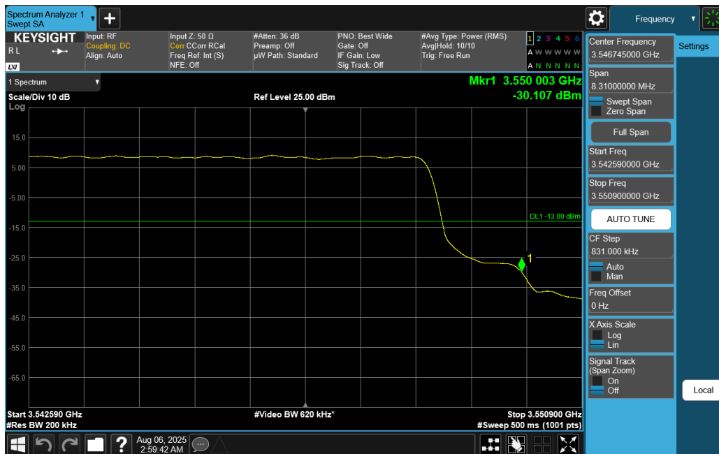
Plot 7-148. Upper Band Edge Plot (NR Band n77 DoD-Band - 15MHz DFT-s-OFDM QPSK – Full RB)
