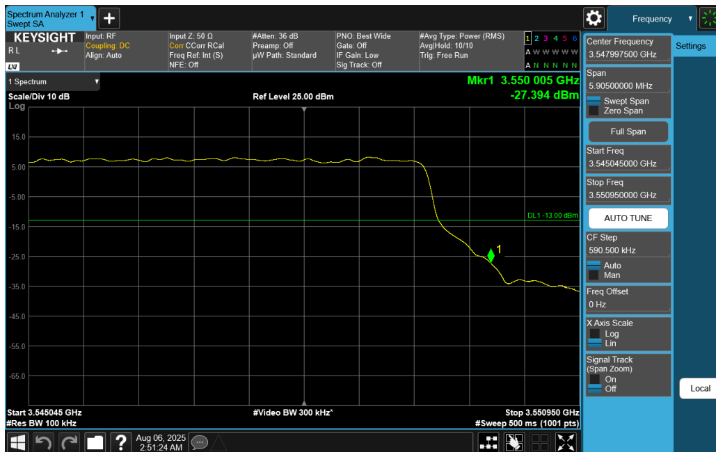
Plot 7-142. Upper Band Edge Plot (NR Band n77 DoD-Band - 10MHz DFT-s-OFDM QPSK – Full RB)
