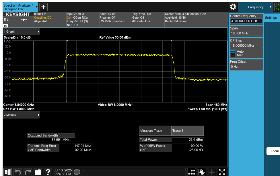
Plot 7-113. Occupied Bandwidth Plot (NR Band n77 C-Band - 90MHz CP-OFDM 16-QAM - Full RB)
