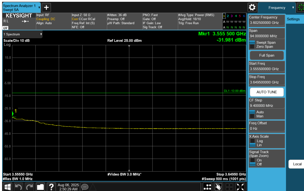
Plot 7-144. Extended Upper Band Edge Plot (NR Band n77 DoD-Band - 10MHz DFT-s-OFDM QPSK – Full RB)
