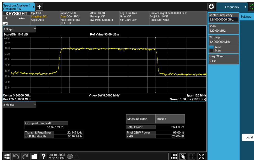
Plot 7-96. Occupied Bandwidth Plot (NR Band n77 C-Band - 60MHz DFT-s-OFDM \pi/2 BPSK - Full RB)
