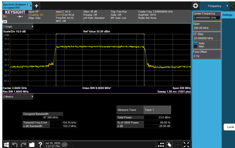
Plot 7-119. Occupied Bandwidth Plot (NR Band n77 C-Band - 100MHz CP-OFDM 64-QAM - Full RB)
