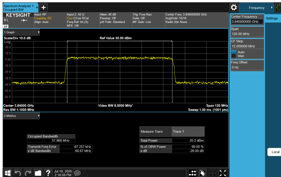
Plot 7-100. Occupied Bandwidth Plot (NR Band n77 C-Band - 60MHz CP-OFDM 256-QAM - Full RB)
