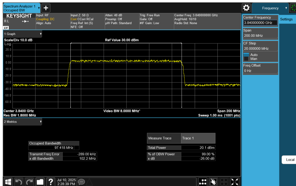
Plot 7-120. Occupied Bandwidth Plot (NR Band n77 C-Band - 100MHz CP-OFDM 256-QAM - Full RB)
