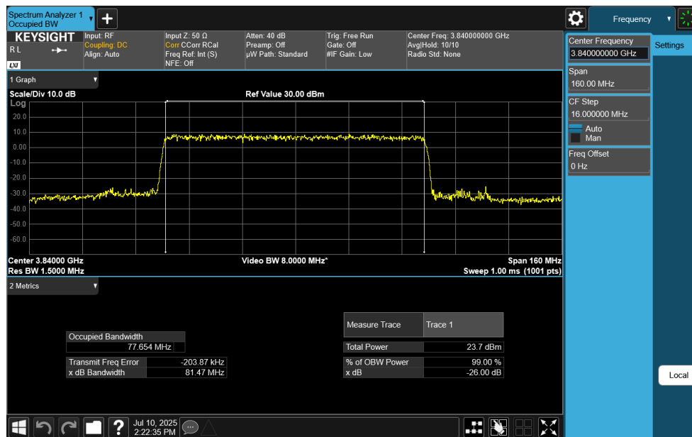
Plot 7-108. Occupied Bandwidth Plot (NR Band n77 C-Band - 80MHz CP-OFDM 16-QAM - Full RB)
