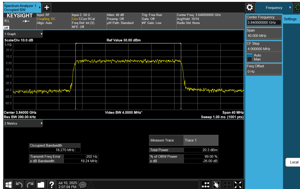
Plot 7-75. Occupied Bandwidth Plot (NR Band n77 C-Band - 20MHz CP-OFDM 256-QAM - Full RB)
