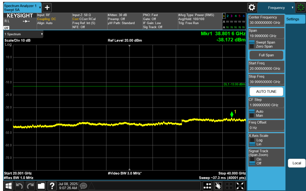
Plot 7-129. Conducted Spurious Plot (NR Band n77 DoD Band - 90MHz DFT-s-OFDM QPSK – RB Size 1, RB Offset 0 – High Channel)
