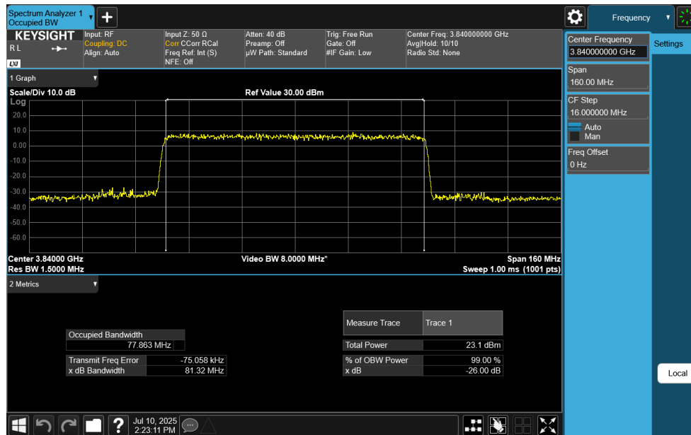
Plot 7-109. Occupied Bandwidth Plot (NR Band n77 C-Band - 80MHz CP-OFDM 64-QAM - Full RB)
