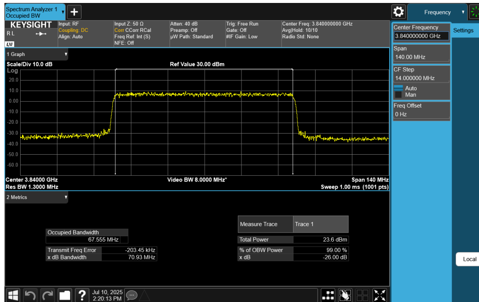
Plot 7-103. Occupied Bandwidth Plot (NR Band n77 C-Band - 70MHz CP-OFDM 16-QAM - Full RB)
