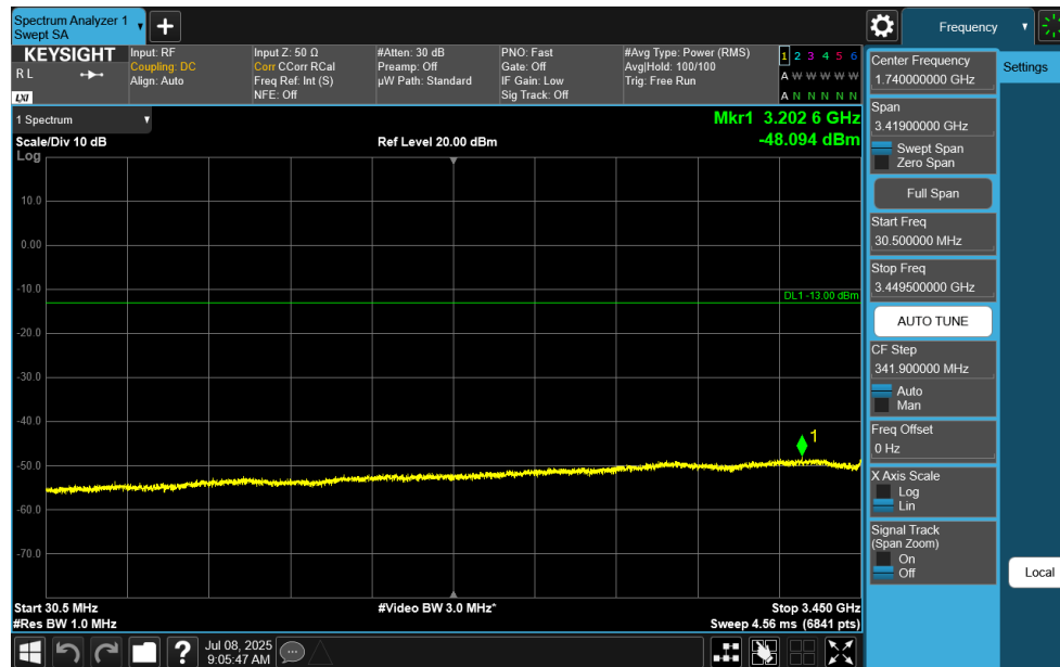
Plot 7-127. Conducted Spurious Plot (NR Band n77 DoD Band - 90MHz DFT-s-OFDM QPSK – RB Size 1, RB Offset 0 – High Channel)
