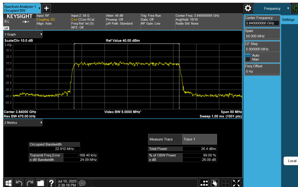
Plot 7-76. Occupied Bandwidth Plot (NR Band n77 C-Band - 25MHz DFT-s-OFDM \pi/2 BPSK - Full RB)
