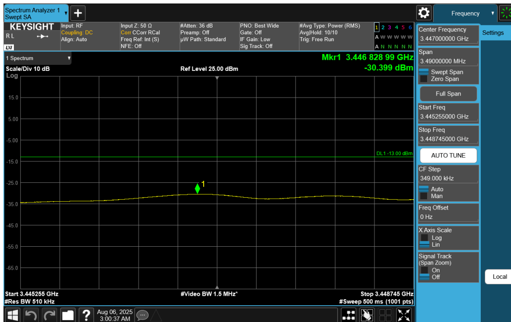
Plot 7-146. Extended Lower Band Edge Plot (NR Band n77 DoD-Band - 15MHz DFT-s-OFDM QPSK – Full RB)
