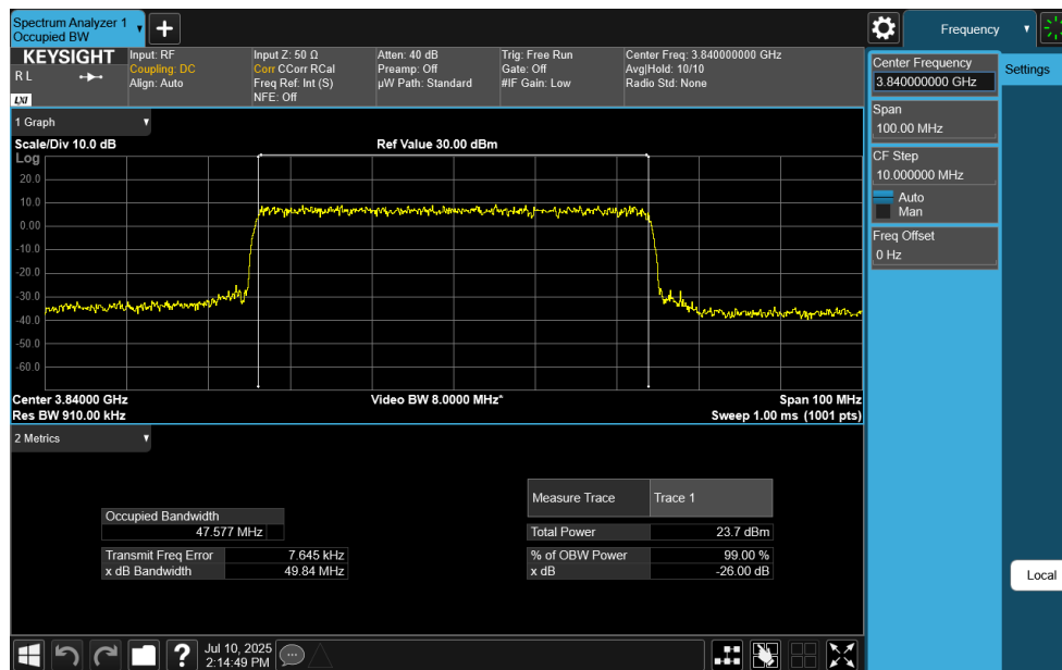
Plot 7-92. Occupied Bandwidth Plot (NR Band n77 C-Band - 50MHz CP-OFDM QPSK - Full RB)
