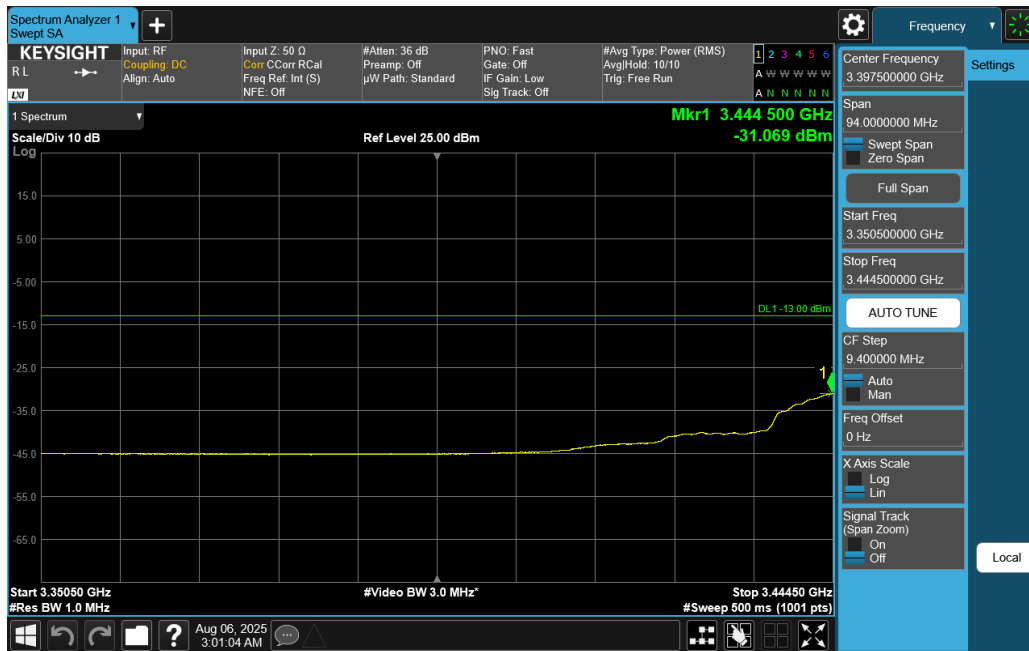
Plot 7-145. Extended Lower Band Edge Plot (NR Band n77 DoD-Band - 15MHz DFT-s-OFDM QPSK – Full RB)
