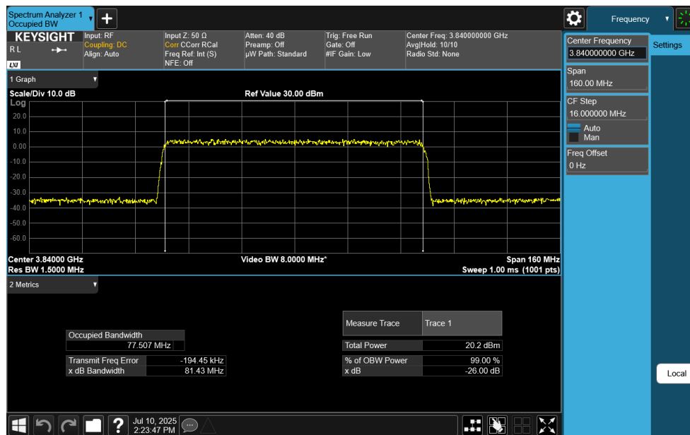
Plot 7-110. Occupied Bandwidth Plot (NR Band n77 C-Band - 80MHz CP-OFDM 256-QAM - Full RB)
