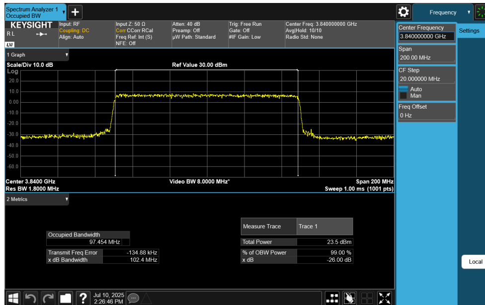
Plot 7-117. Occupied Bandwidth Plot (NR Band n77 C-Band - 100MHz CP-OFDM QPSK - Full RB)
