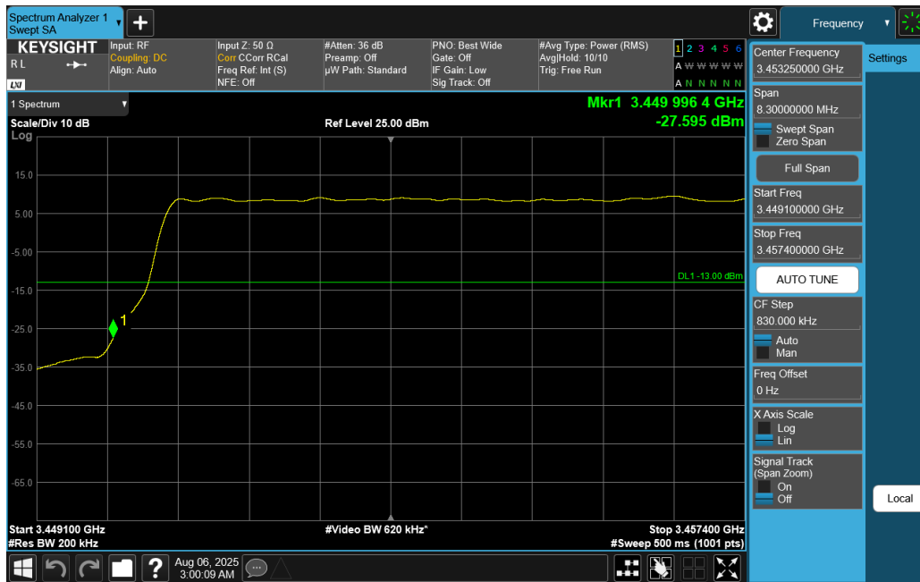
Plot 7-147. Lower Band Edge Plot (NR Band n77 DoD-Band - 15MHz DFT-s-OFDM QPSK – Full RB)
