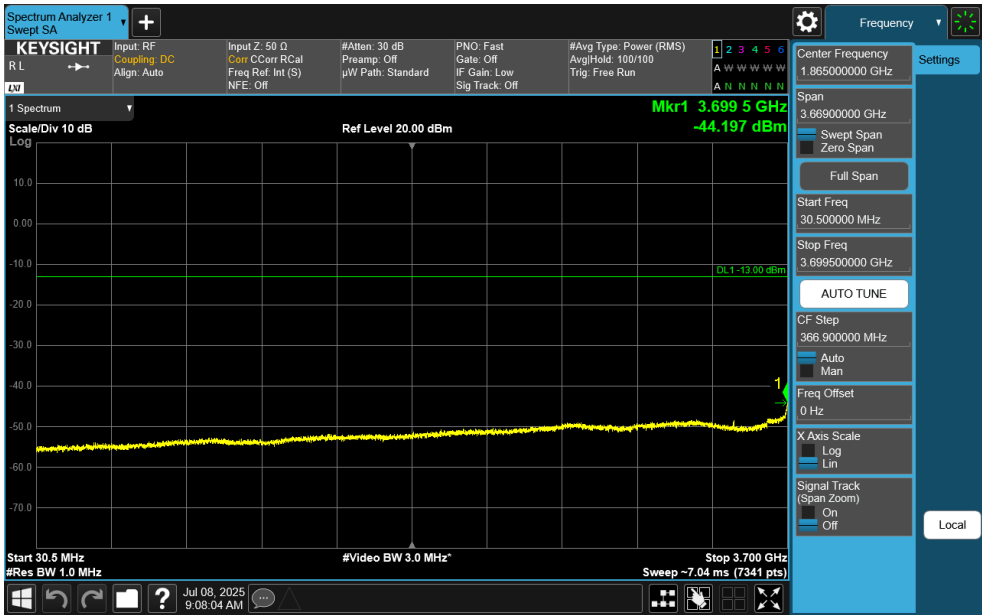
Plot 7-130. Conducted Spurious Plot (NR Band n77 C-Band - 100MHz DFT-s-OFDM QPSK – RB Size 1, RB Offset 0 – Low Channel)
