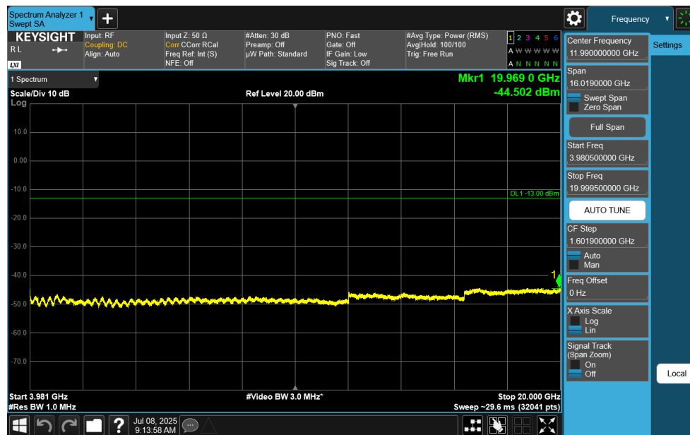
Plot 7-137. Conducted Spurious Plot (NR Band n77 C-Band - 100MHz DFT-s-OFDM QPSK – RB Size 1, RB Offset 0 – High Channel)
