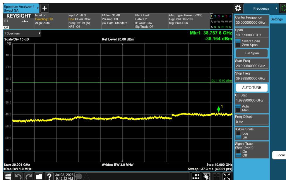
Plot 7-135. Conducted Spurious Plot (NR Band n77 C-Band - 100MHz DFT-s-OFDM QPSK – RB Size 1, RB Offset 0 – Mid Channel)
