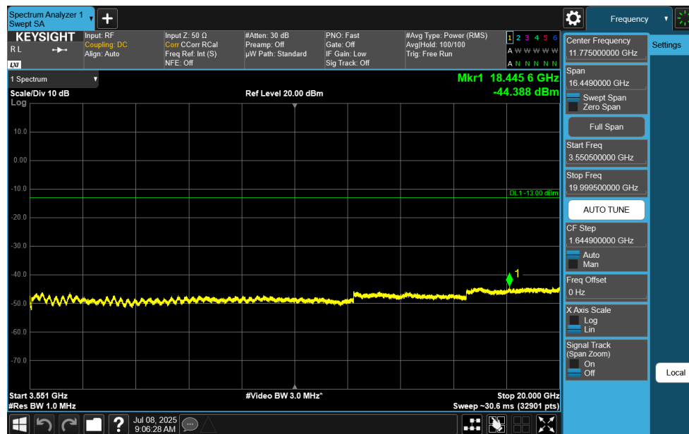
Plot 7-128. Conducted Spurious Plot (NR Band n77 DoD Band - 90MHz DFT-s-OFDM QPSK – RB Size 1, RB Offset 0 – High Channel)
