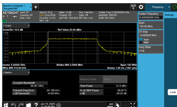
Plot 7-42 26dB BW & 99% OBW Antenna 4a (40MHz BW 802.11be(SU) - Ch.91)
