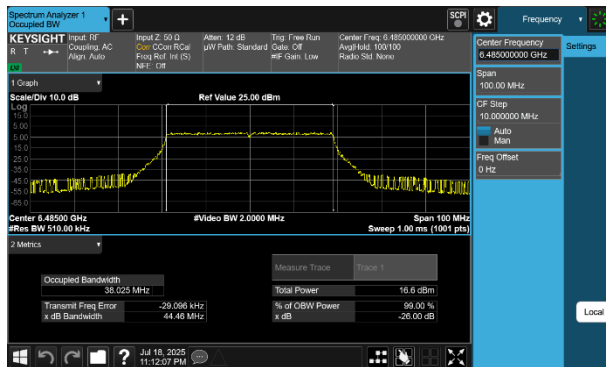
Plot 7-18 26dB BW & 99% OBW Antenna WF5B (40MHz BW 802.11be(SU) - Ch.107)
