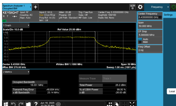
Plot 7-33 26dB BW & 99% OBW Antenna 4a (20MHz BW 802.11a - Ch.97)
