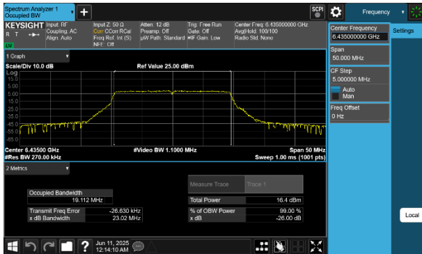
Plot 7-45 26dB BW & 99% OBW Antenna 4a (20MHz BW 802.11be(SU) - Ch.97)
