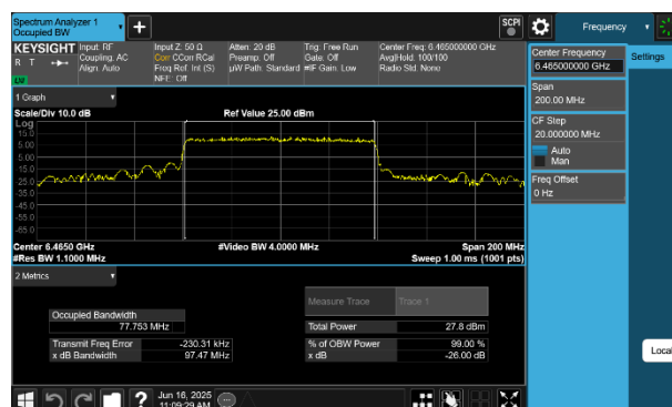
Plot 7-35 26dB BW & 99% OBW Antenna 4a (80MHz BW 802.11be(SU) - Ch.103)
