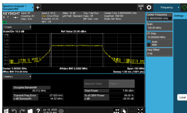
Plot 7-70 26dB BW & 99% OBW Antenna 2a (40MHz BW 802.11be(SU) - Ch.3)
