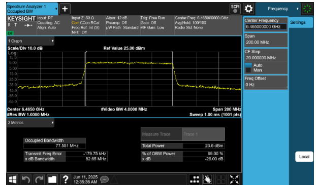
Plot 7-47 26dB BW & 99% OBW Antenna 4a (80MHz BW 802.11be(SU) - Ch.103)
