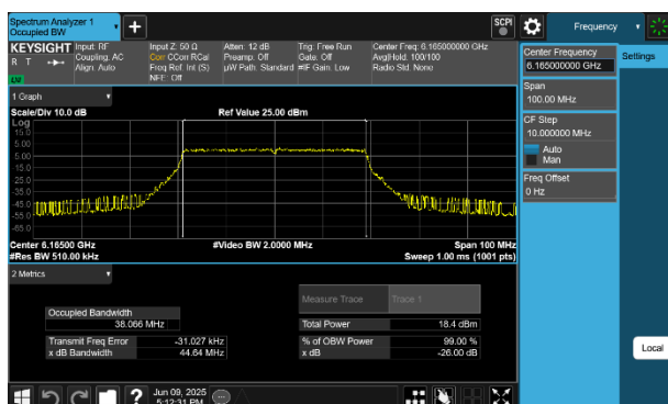
Plot 7-14 26dB BW & 99% OBW Antenna WF5B (40MHz BW 802.11be(SU) - Ch.43)
