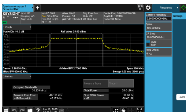
Plot 7-30 26dB BW & 99% OBW Antenna 4a (40MHz BW 802.11be(SU) - Ch.3)
