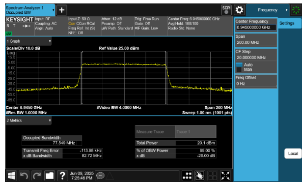
Plot 7-27 26dB BW & 99% OBW Antenna WF5B (80MHz BW 802.11be(SU) - Ch.199)
