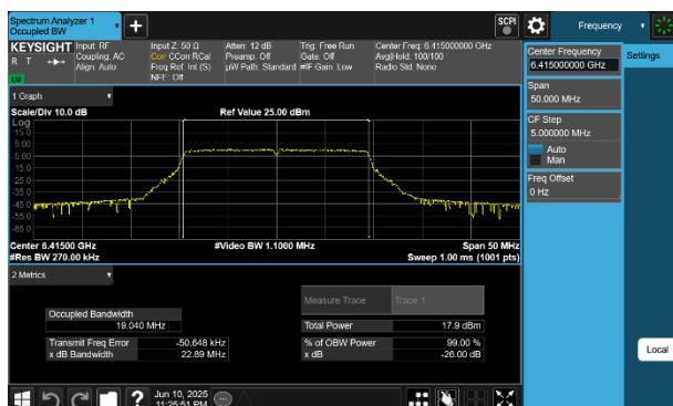
Plot 7-41 26dB BW & 99% OBW Antenna 4a (20MHz BW 802.11be(SU) - Ch.93)
