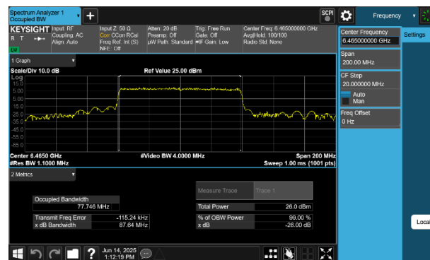
Plot 7-63 26dB BW & 99% OBW Antenna 2a (80MHz BW 802.11be(SU) - Ch.103)
