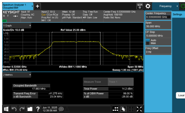
Plot 7-49 26dB BW & 99% OBW Antenna 4a (20MHz BW 802.11a - Ch.117)
