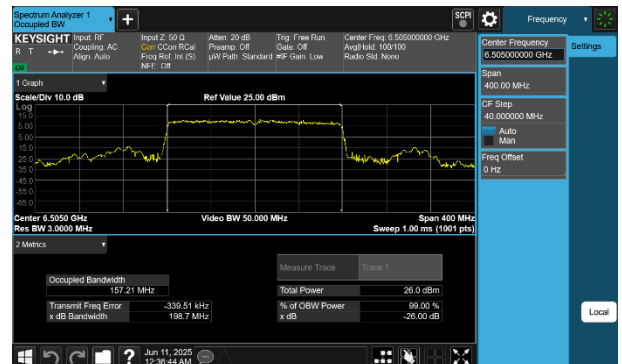
Plot 7-48 26dB BW & 99% OBW Antenna 4a (160MHz BW 802.11be(SU) - Ch.111)
