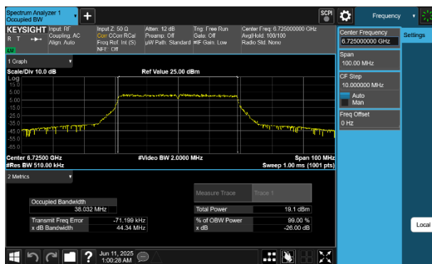
Plot 7-50 26dB BW & 99% OBW Antenna 4a (40MHz BW 802.11be(SU) - Ch.155)
