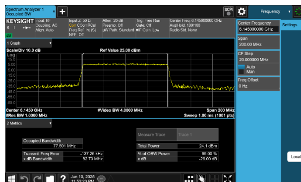
Plot 7-43 26dB BW & 99% OBW Antenna 4a (80MHz BW 802.11be(SU) - Ch.39)
