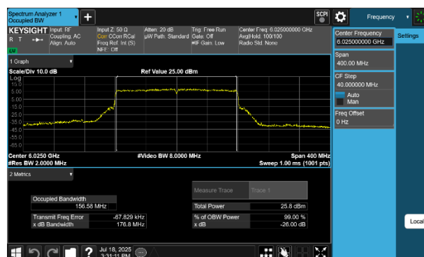
Plot 7-44 26dB BW & 99% OBW Antenna 4a (160MHz BW 802.11be(SU) - Ch.15)
