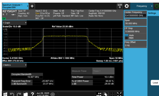
Plot 7-13 26dB BW & 99% OBW Antenna WF5B (20MHz BW 802.11be(SU) - Ch.93)
