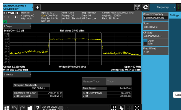
Plot 7-16 26dB BW & 99% OBW Antenna WF5B (160MHz BW 802.11be(SU) - Ch.15)
