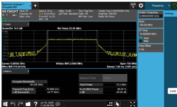
Plot 7-26 26dB BW & 99% OBW Antenna WF5B (40MHz BW 802.11be(SU) - Ch.187)
