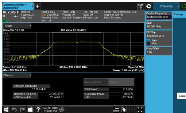
Plot 7-17 26dB BW & 99% OBW Antenna WF5B (20MHz BW 802.11a - Ch.113)
