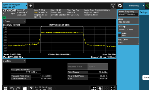
Plot 7-15 26dB BW & 99% OBW Antenna WF5B (80MHz BW 802.11be(SU) - Ch.7)
