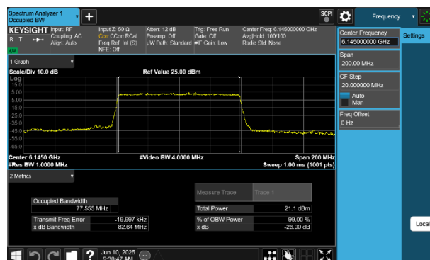
Plot 7-71 26dB BW & 99% OBW Antenna 2a (80MHz BW 802.11be(SU) - Ch.39)
