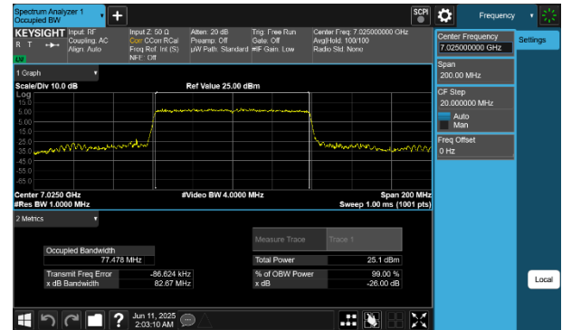
Plot 7-55 26dB BW & 99% OBW Antenna 4a (80MHz BW 802.11be(SU) - Ch.215)
