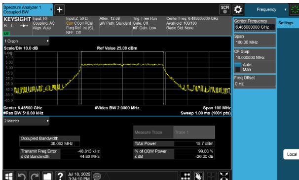
Plot 7-46 26dB BW & 99% OBW Antenna 4a (40MHz BW 802.11be(SU) - Ch.107)
