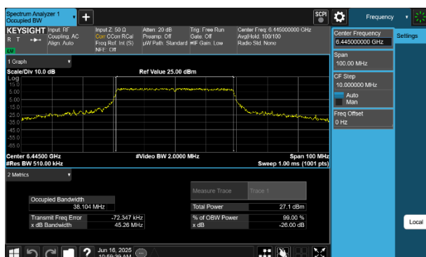
Plot 7-34 26dB BW & 99% OBW Antenna 4a (40MHz BW 802.11be(SU) - Ch.99)
