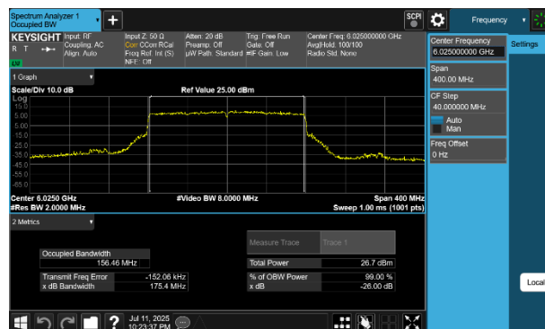
Plot 7-32 26dB BW & 99% OBW Antenna 4a (160MHz BW 802.11be(SU) - Ch.15)
