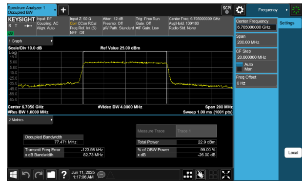
Plot 7-51 26dB BW & 99% OBW Antenna 4a (80MHz BW 802.11be(SU) - Ch.151)
