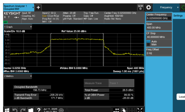
Plot 7-4 26dB BW & 99% OBW Antenna WF5B (160MHz BW 802.11be(SU) - Ch.15)
