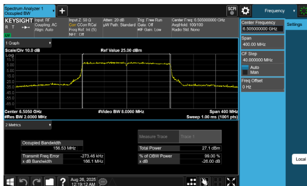
Plot 7-36 26dB BW & 99% OBW Antenna 4a (160MHz BW 802.11be(SU) - Ch.111)
