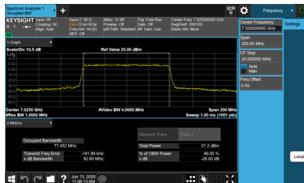
Plot 7-31 26dB BW & 99% OBW Antenna 4a (80MHz BW 802.11be(SU) - Ch.215)
