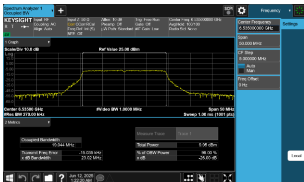
Plot 7-9 26dB BW & 99% OBW Antenna WF5B (20MHz BW 802.11be(SU) - Ch.117)
