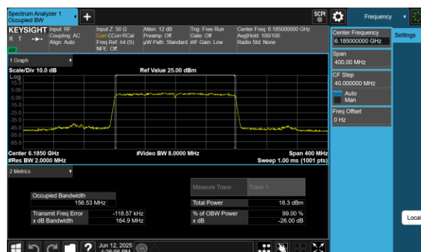
Plot 7-36 26dB BW & 99% OBW Antenna 2a (160MHz BW 802.11be(SU) - Ch.47)
