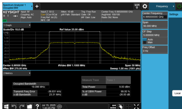
Plot 7-13 26dB BW & 99% OBW Antenna WF5B (20MHz BW 802.11be(SU) - Ch.209)
