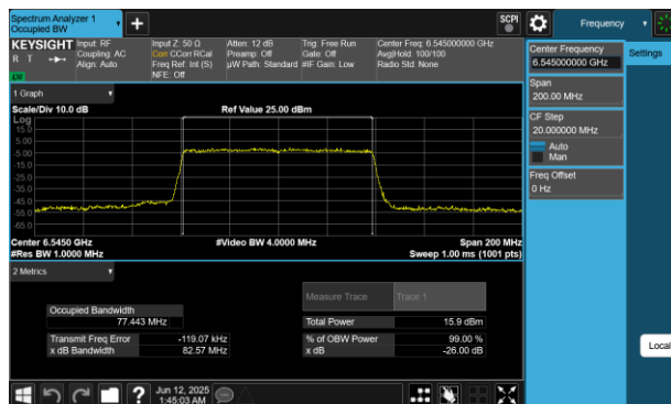
Plot 7-11 26dB BW & 99% OBW Antenna WF5B (80MHz BW 802.11be(SU) - Ch.119)
