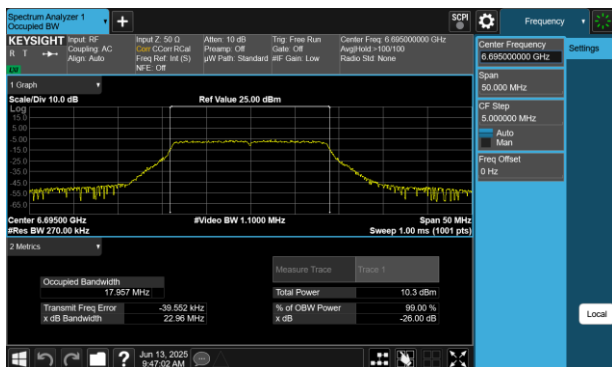
Plot 7-25 26dB BW & 99% OBW Antenna 4a (20MHz BW 802.11a - Ch.149)
