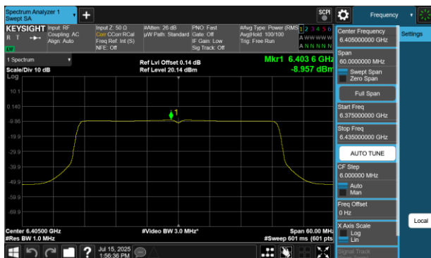
Plot 7-50 PSD Antenna WF5B (40MHz BW 802.11be(SU) - Ch.91)
