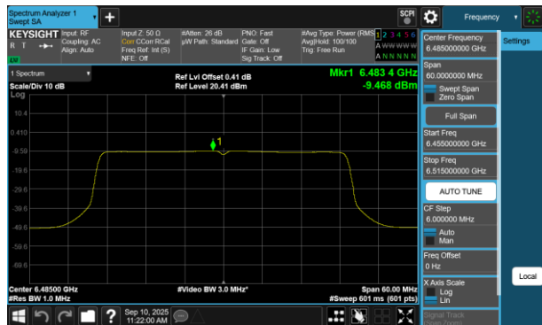
Plot 7-54 PSD Antenna WF5B (40MHz BW 802.11be(SU) - Ch.107)
