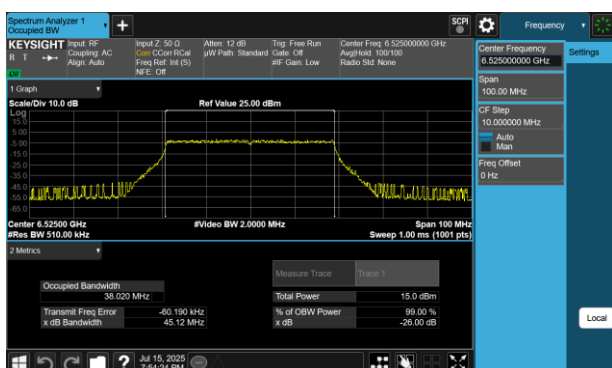
Plot 7-22 26dB BW & 99% OBW Antenna 4a (40MHz BW 802.11be(SU) - Ch.115)
