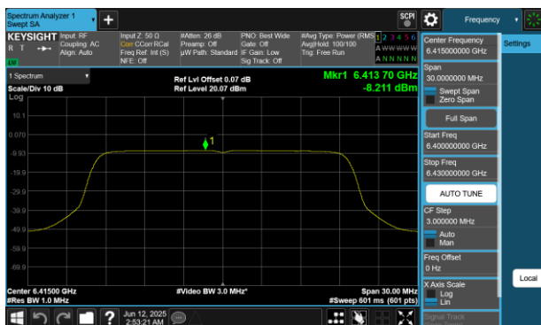
Plot 7-49 PSD Antenna WF5B (20MHz BW 802.11be(SU) - Ch.93)
