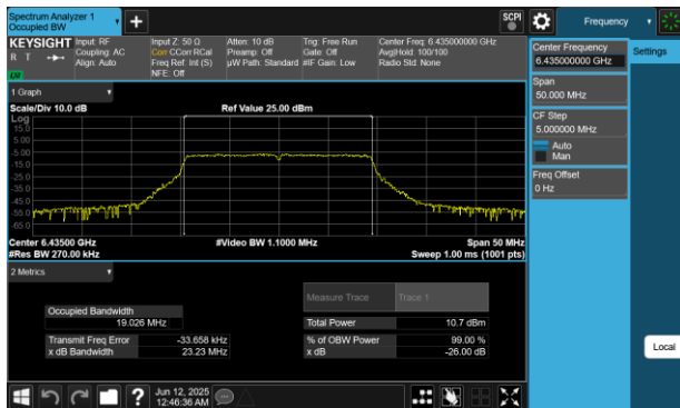
Plot 7-5 26dB BW & 99% OBW Antenna WF5B (20MHz BW 802.11be(SU) - Ch.97)
