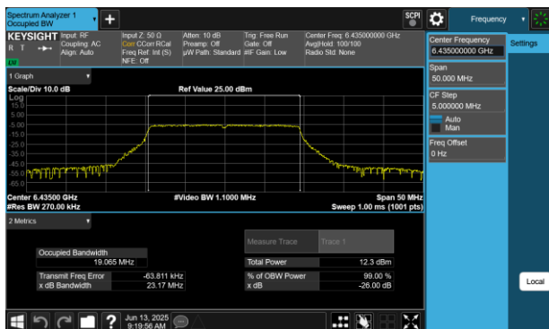
Plot 7-21 26dB BW & 99% OBW Antenna 4a (20MHz BW 802.11be(SU) - Ch.97)
