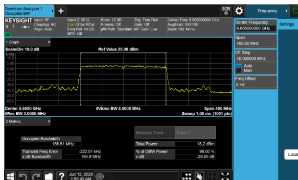
Plot 7-12 26dB BW & 99% OBW Antenna WF5B (160MHz BW 802.11be(SU) - Ch.143)
