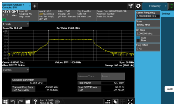
Plot 7-29 26dB BW & 99% OBW Antenna 4a (20MHz BW 802.11a - Ch.189)
