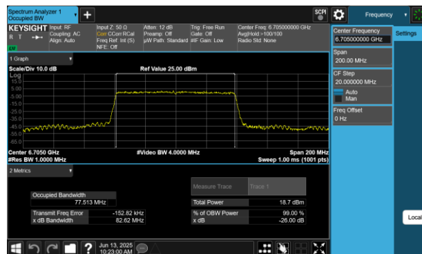
Plot 7-27 26dB BW & 99% OBW Antenna 4a (80MHz BW 802.11be(SU) - Ch.151)
