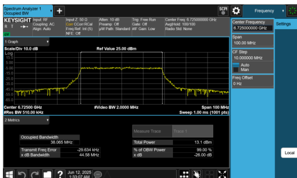
Plot 7-10 26dB BW & 99% OBW Antenna WF5B (40MHz BW 802.11be(SU) - Ch.155)
