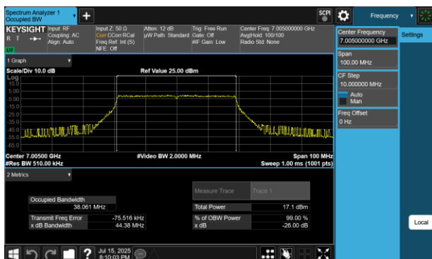
Plot 7-30 26dB BW & 99% OBW Antenna 4a (40MHz BW 802.11be(SU) - Ch.211)
