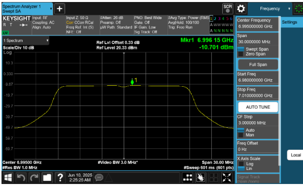
Plot 7-217 PSD CDD Primary Antenna WF5B (20MHz BW 802.11a - Ch.209)
