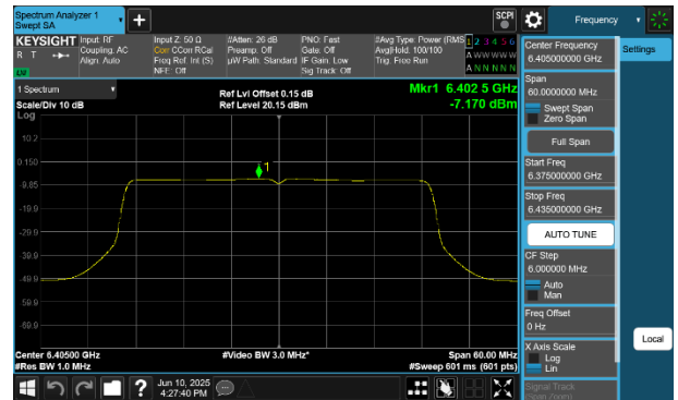
Plot 7-254 PSD SDM Diversity Antenna 2a (40MHz BW 802.11be(SU) - Ch.91)
