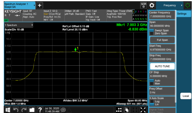
Plot 7-222 PSD SDM Primary Antenna 4a (40MHz BW 802.11be(SU) - Ch.211)
