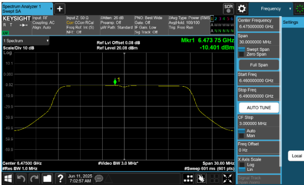
Plot 7-257 PSD CDD Diversity Antenna 4a (20MHz BW 802.11a - Ch.105)
