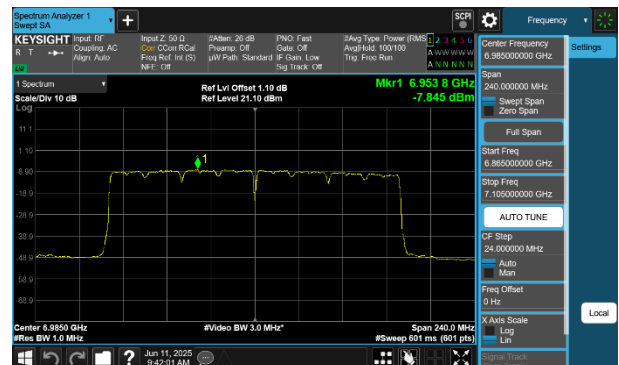
Plot 7-224 PSD SDM Primary Antenna 4a (160MHz BW 802.11be(SU) - Ch.207)
