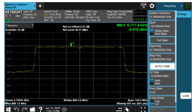
Plot 7-247 PSD CDD Diversity Antenna 2a (80MHz BW 802.11be(SU) - Ch.167)
