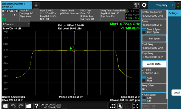
Plot 7-266 PSD SDM Diversity Antenna 4a (40MHz BW 802.11be(SU) - Ch.155)
