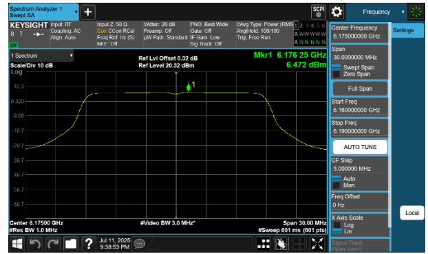
Plot 7-229 PSD CDD Diversity Antenna 2a (20MHz BW 802.11a - Ch.45)
