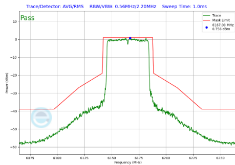
Plot 7-282 In-Band Emission Plot Antenna WF5B (40MHz BW 802.11be(SU) (UNII Band 5) - Ch.43)
