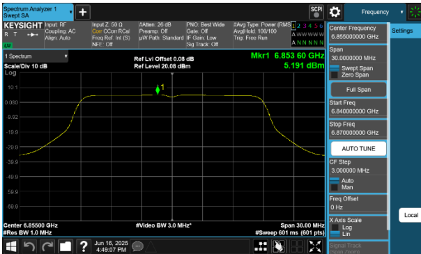
Plot 7-241 PSD CDD Diversity Antenna 4a (20MHz BW 802.11a - Ch.181)
