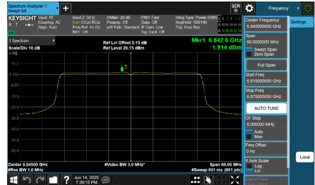
Plot 7-246 PSD CDD Diversity Antenna 2a (40MHz BW 802.11be(SU) - Ch.179)
