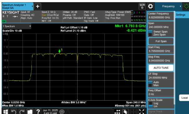
Plot 7-268 PSD SDM Diversity Antenna 4a (160MHz BW 802.11be(SU) - Ch.175)
