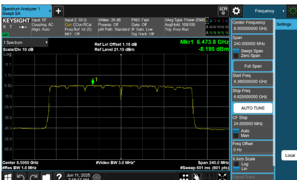
Plot 7-260 PSD SDM Diversity Antenna 4a (160MHz BW 802.11be(SU) - Ch.111)
