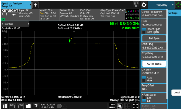
Plot 7-242 PSD CDD Diversity Antenna 4a (40MHz BW 802.11be(SU) - Ch.179)
