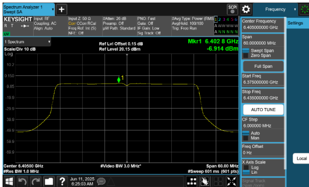
Plot 7-250 PSD SDM Diversity Antenna 4a (40MHz BW 802.11be(SU) - Ch.91)
