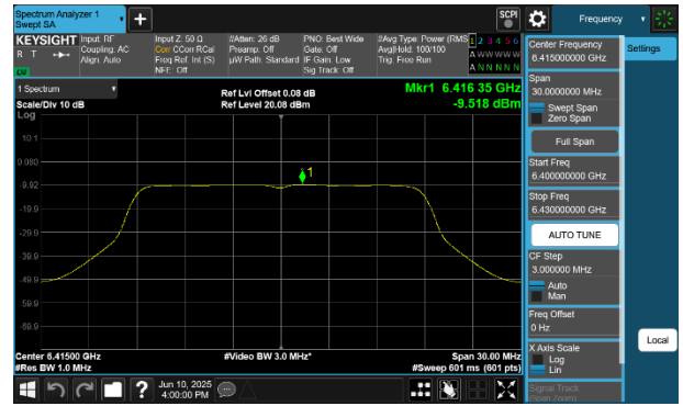
Plot 7-253 PSD CDD Diversity Antenna 2a (20MHz BW 802.11a - Ch.93)
