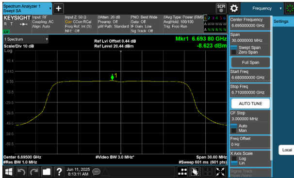
Plot 7-265 PSD SDM Diversity Antenna 4a (20MHz BW 802.11be(SU) - Ch.149)
