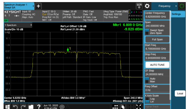
Plot 7-272 PSD SDM Diversity Antenna 2a (160MHz BW 802.11be(SU) - Ch.175)
