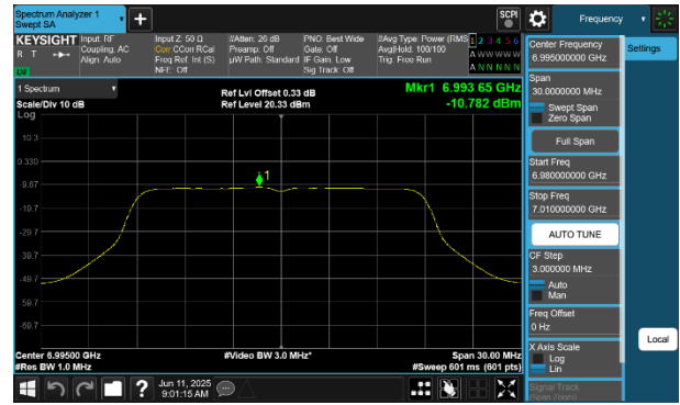
Plot 7-221 PSD CDD Primary Antenna 4a (20MHz BW 802.11a - Ch.209)
