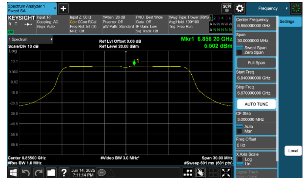
Plot 7-245 PSD CDD Diversity Antenna 2a (20MHz BW 802.11a - Ch.181)
