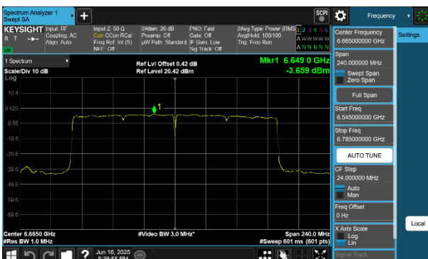
Plot 7-244 PSD CDD Diversity Antenna 4a (160MHz BW 802.11be(SU) - Ch.143)
