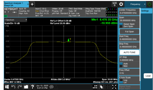
Plot 7-261 PSD CDD Diversity Antenna 2a (20MHz BW 802.11a - Ch.105)
