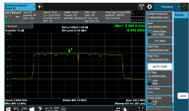
Plot 7-280 PSD SDM Diversity Antenna 2a (160MHz BW 802.11be(SU) - Ch.207)
