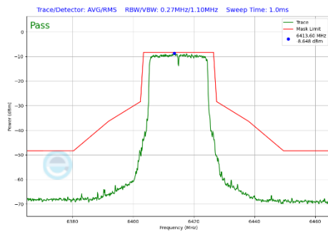
Plot 7-293 In-Band Emission Plot Antenna WF5B (20MHz BW 802.11be(SU) (UNII Band 5) - Ch.93)
