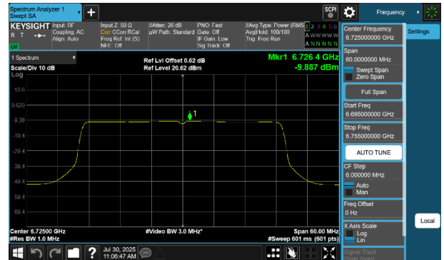
Plot 7-270 PSD SDM Diversity Antenna 2a (40MHz BW 802.11be(SU) - Ch.155)
