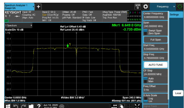
Plot 7-248 PSD CDD Diversity Antenna 2a (160MHz BW 802.11be(SU) - Ch.143)
