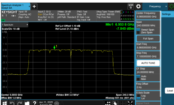
Plot 7-276 PSD SDM Diversity Antenna 4a (160MHz BW 802.11be(SU) - Ch.207)
