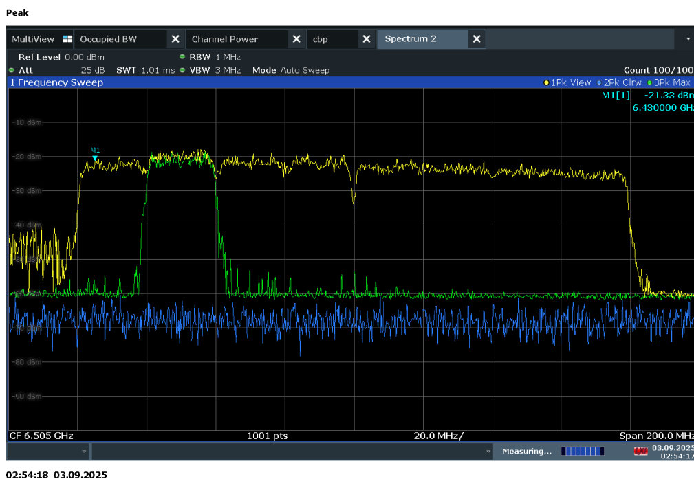
Plot 7-305. 160MHz Bandwidth, AWGN Signal Injected – 6430Mhz
