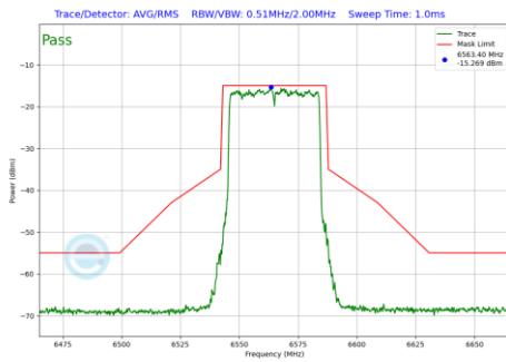
Plot 7-234 In-Band Emission Plot SDM Primary Antenna 4a (40MHz BW 802.11be(SU) (UNII Band 7) - Ch.123)
