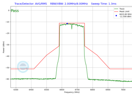
Plot 7-252 In-Band Emission Plot SDM Diversity Antenna 2a (160MHz BW 802.11be(SU) (UNII Band 7) - Ch.143)
