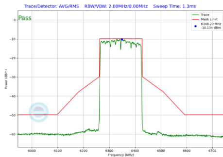
Plot 7-244 In-Band Emission Plot SDM Diversity Antenna 2a (160MHz BW 802.11be(SU) (UNII Band 5) - Ch.79)
