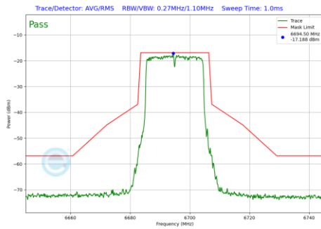
Plot 7-249 In-Band Emission Plot SDM Diversity Antenna 2a (20MHz BW 802.11be(SU) (UNII Band 7) - Ch.149)
