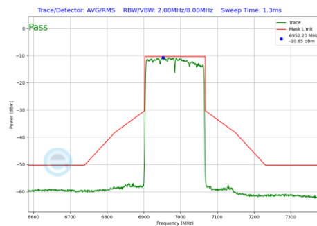
Plot 7-256 In-Band Emission Plot SDM Diversity Antenna 2a (160MHz BW 802.11be(SU) (UNII Band 8) - Ch.207)
