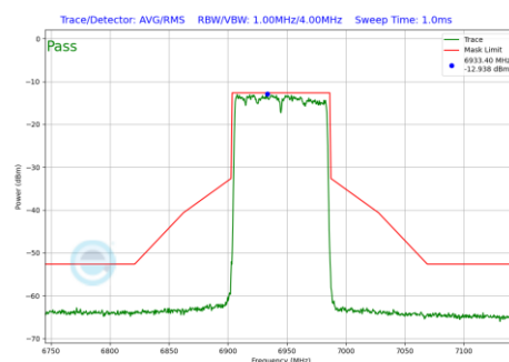
Plot 7-255 In-Band Emission Plot SDM Diversity Antenna 2a (80MHz BW 802.11be(SU) (UNII Band 8) - Ch.199)
