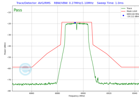
Plot 7-269 In-Band Emission Plot CDD Diversity Antenna 4a (20MHz BW 802.11a (UNII Band 8) - Ch.189)
