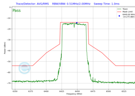
Plot 7-262 In-Band Emission Plot SDM Diversity Antenna 4a (40MHz BW 802.11be(SU) (UNII Band 6) - Ch.99)
