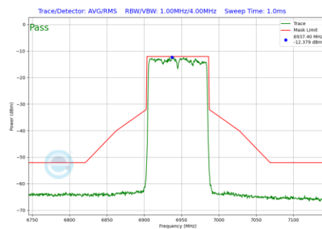
Plot 7-271 In-Band Emission Plot SDM Diversity Antenna 4a (80MHz BW 802.11be(SU) (UNII Band 8) - Ch.199)
