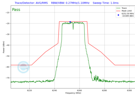
Plot 7-257 In-Band Emission Plot CDD Diversity Antenna 4a (20MHz BW 802.11a (UNII Band 5) - Ch.61)
