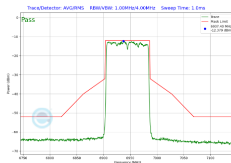
Plot 7-239 In-Band Emission Plot SDM Primary Antenna 4a (80MHz BW 802.11be(SU) (UNII Band 8) - Ch.199)
