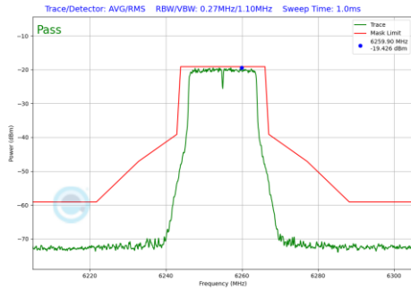
Plot 7-241 In-Band Emission Plot CDD Diversity Antenna 2a (20MHz BW 802.11a (UNII Band 5) - Ch.61)
