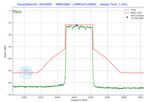
Plot 7-263 In-Band Emission Plot SDM Diversity Antenna 4a (80MHz BW 802.11be(SU) (UNII Band 6) - Ch.103)
