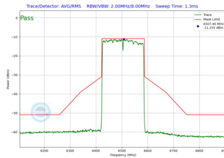
Plot 7-264 In-Band Emission Plot SDM Diversity Antenna 4a (160MHz BW 802.11be(SU) (UNII Band 6) - Ch.111)
