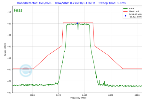
Plot 7-261 In-Band Emission Plot CDD Diversity Antenna 4a (20MHz BW 802.11a (UNII Band 6) - Ch.97)
