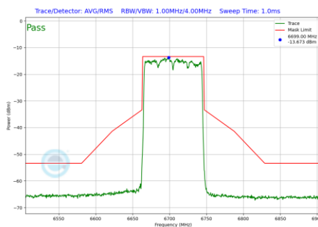
Plot 7-251 In-Band Emission Plot SDM Diversity Antenna 2a (80MHz BW 802.11be(SU) (UNII Band 7) - Ch.151)
