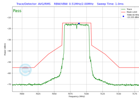
Plot 7-238 In-Band Emission Plot SDM Primary Antenna 4a (40MHz BW 802.11be(SU) (UNII Band 8) - Ch.227)
