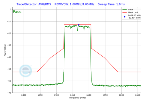
Plot 7-247 In-Band Emission Plot SDM Diversity Antenna 2a (80MHz BW 802.11be(SU) (UNII Band 6) - Ch.103)
