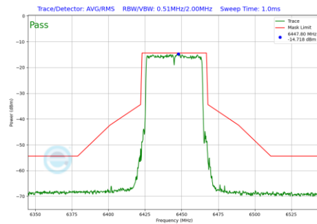
Plot 7-246 In-Band Emission Plot SDM Diversity Antenna 2a (40MHz BW 802.11be(SU) (UNII Band 6) - Ch.99)
