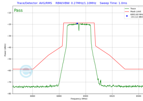
Plot 7-237 In-Band Emission Plot CDD Primary Antenna 4a (20MHz BW 802.11a (UNII Band 8) - Ch.189)
