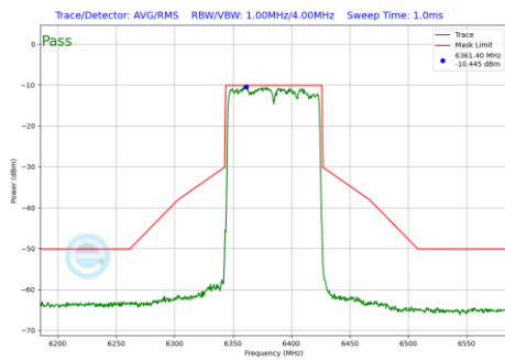
Plot 7-259 In-Band Emission Plot SDM Diversity Antenna 4a (80MHz BW 802.11be(SU) (UNII Band 5) - Ch.87)
