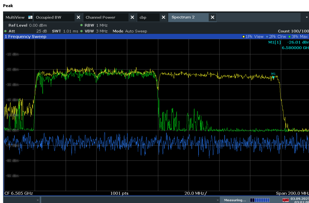
Plot 7-307. 160MHz Bandwidth, AWGN Signal Injected – 6580MHz
