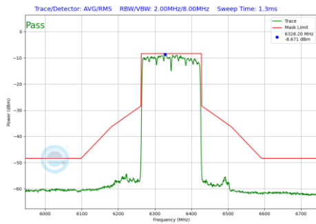
Plot 7-260 In-Band Emission Plot SDM Diversity Antenna 4a (160MHz BW 802.11be(SU) (UNII Band 5) - Ch.79)
