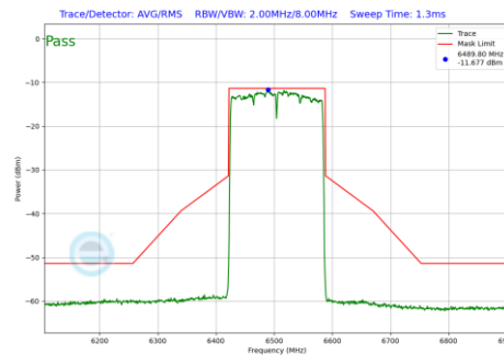
Plot 7-248 In-Band Emission Plot SDM Diversity Antenna 2a (160MHz BW 802.11be(SU) (UNII Band 6) - Ch.111)
