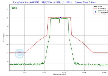
Plot 7-245 In-Band Emission Plot CDD Diversity Antenna 2a (20MHz BW 802.11a (UNII Band 6) - Ch.97)
