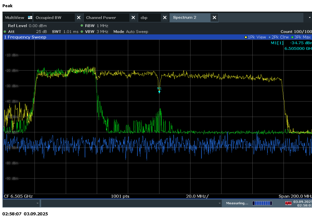
Plot 7-306. 160MHz Bandwidth, AWGN Signal Injected – 6505Mhz
