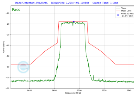
Plot 7-265 In-Band Emission Plot SDM Diversity Antenna 4a (20MHz BW 802.11be(SU) (UNII Band 7) - Ch.149)
