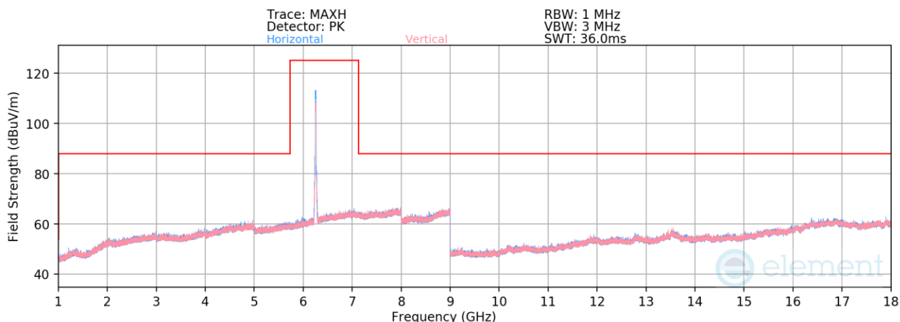
Plot 7-311. Radiated Spurious Emissions 1-18GHz SDM Primary (802.11be – Ch. 61)
