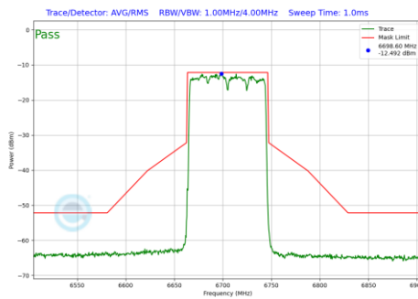
Plot 7-267 In-Band Emission Plot SDM Diversity Antenna 4a (80MHz BW 802.11be(SU) (UNII Band 7) - Ch.151)
