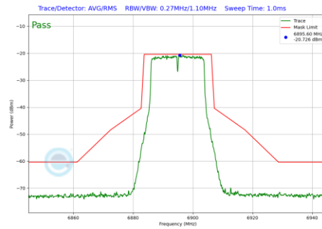
Plot 7-253 In-Band Emission Plot CDD Diversity Antenna 2a (20MHz BW 802.11a (UNII Band 8) - Ch.189)
