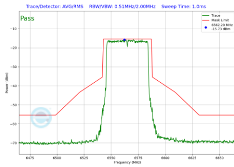
Plot 7-266 In-Band Emission Plot SDM Diversity Antenna 4a (40MHz BW 802.11be(SU) (UNII Band 7) - Ch.123)
