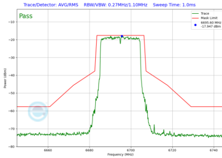
Plot 7-233 In-Band Emission Plot SDM Primary Antenna 4a (20MHz BW 802.11be(SU) (UNII Band 7) - Ch.149)
