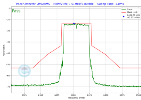
Plot 7-258 In-Band Emission Plot SDM Diversity Antenna 4a (40MHz BW 802.11be(SU) (UNII Band 5) - Ch.91)
