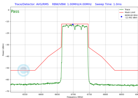
Plot 7-235 In-Band Emission Plot SDM Primary Antenna 4a (80MHz BW 802.11be(SU) (UNII Band 7) - Ch.151)
