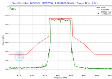
Plot 7-242 In-Band Emission Plot SDM Diversity Antenna 2a (40MHz BW 802.11be(SU) (UNII Band 5) - Ch.91)
