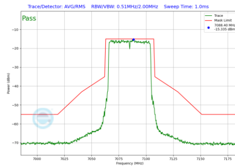
Plot 7-270 In-Band Emission Plot SDM Diversity Antenna 4a (40MHz BW 802.11be(SU) (UNII Band 8) - Ch.227)
