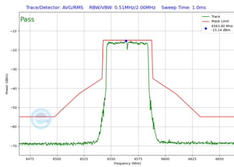
Plot 7-250 In-Band Emission Plot SDM Diversity Antenna 2a (40MHz BW 802.11be(SU) (UNII Band 7) - Ch.123)
