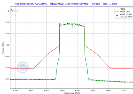
Plot 7-236 In-Band Emission Plot SDM Primary Antenna 4a (160MHz BW 802.11be(SU) (UNII Band 7) - Ch.143)
