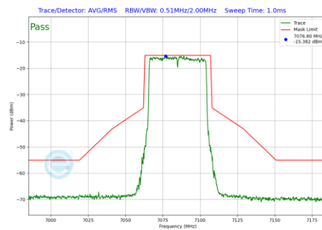
Plot 7-254 In-Band Emission Plot SDM Diversity Antenna 2a (40MHz BW 802.11be(SU) (UNII Band 8) - Ch.227)
