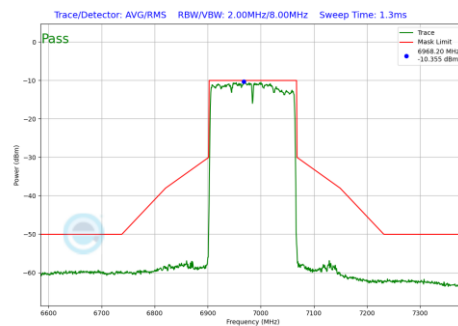
Plot 7-272 In-Band Emission Plot SDM Diversity Antenna 4a (160MHz BW 802.11be(SU) (UNII Band 8) - Ch.207)
