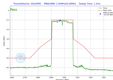
Plot 7-240 In-Band Emission Plot SDM Primary Antenna 4a (160MHz BW 802.11be(SU) (UNII Band 8) - Ch.207)
