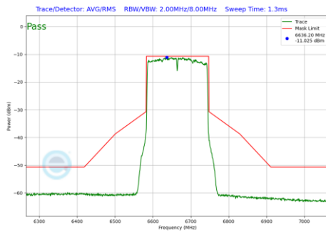
Plot 7-268 In-Band Emission Plot SDM Diversity Antenna 4a (160MHz BW 802.11be(SU) (UNII Band 7) - Ch.143)
