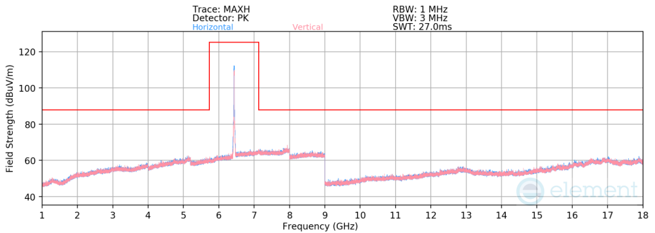
Plot 7-314. Radiated Spurious Emissions 1-18GHz SDM Primary (802.11be – Ch. 97)
