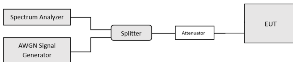
Figure 7-5. Contention-based protocol test setup, conducted method
