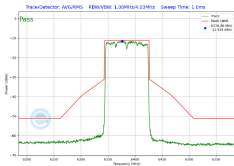
Plot 7-243 In-Band Emission Plot SDM Diversity Antenna 2a (80MHz BW 802.11be(SU) (UNII Band 5) - Ch.87)
