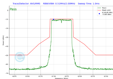
Plot 7-390 In-Band Emission Plot SDM Primary Antenna WF5B (40MHz BW 802.11be(SU) (UNII Band 5) - Ch.43)
