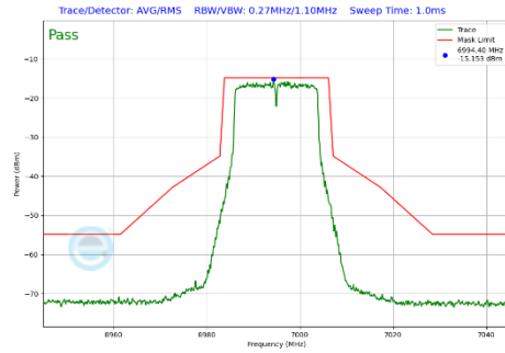
Plot 7-401 In-Band Emission Plot CDD Primary Antenna WF5B (20MHz BW 802.11a (UNII Band 8) - Ch.209)
