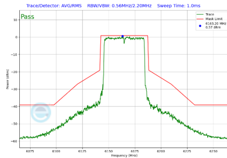
Plot 7-378 In-Band Emission Plot CDD Primary Antenna 4a (40MHz BW 802.11be(SU) (UNII Band 5) - Ch.43)
