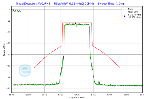
Plot 7-414 In-Band Emission Plot SDM Primary Antenna 4a (40MHz BW 802.11be(SU) (UNII Band 7) - Ch.155)
