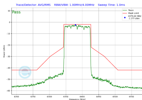
Plot 7-323 In-Band Emission Plot Antenna 4a (80MHz BW 802.11be(SU) (UNII Band 5) - Ch.87)
