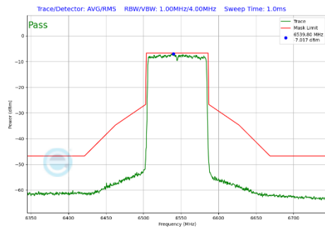
Plot 7-359 In-Band Emission Plot Antenna 2a (80MHz BW 802.11be(SU) (UNII Band 7) - Ch.119)
