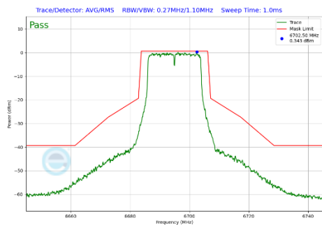
Plot 7-345 In-Band Emission Plot Antenna 2a (20MHz BW 802.11a (UNII Band 7) - Ch.149)
