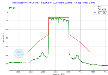
Plot 7-416 In-Band Emission Plot SDM Primary Antenna 4a (160MHz BW 802.11be(SU) (UNII Band 7) - Ch.175)
