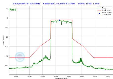
Plot 7-352 In-Band Emission Plot Antenna 2a (160MHz BW 802.11be(SU) (UNII Band 5) - Ch.79)
