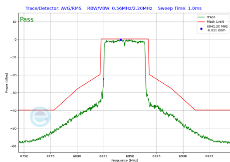
Plot 7-346 In-Band Emission Plot Antenna 2a (40MHz BW 802.11be(SU) (UNII Band 7) - Ch.179)
