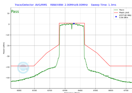
Plot 7-324 In-Band Emission Plot Antenna 4a (160MHz BW 802.11be(SU) (UNII Band 5) - Ch.79)
