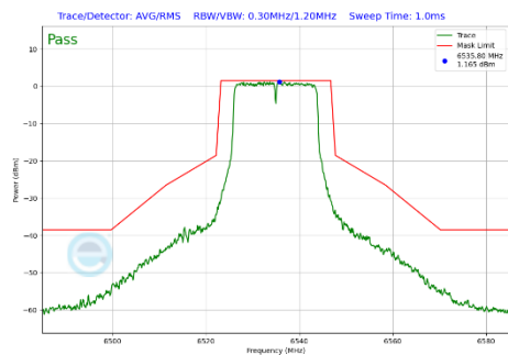
Plot 7-317 In-Band Emission Plot Antenna 4a (20MHz BW 802.11a (UNII Band 7) - Ch.117)
