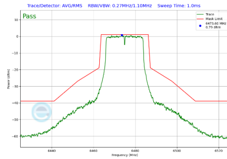
Plot 7-313 In-Band Emission Plot Antenna 4a (20MHz BW 802.11a (UNII Band 6) - Ch.105)
