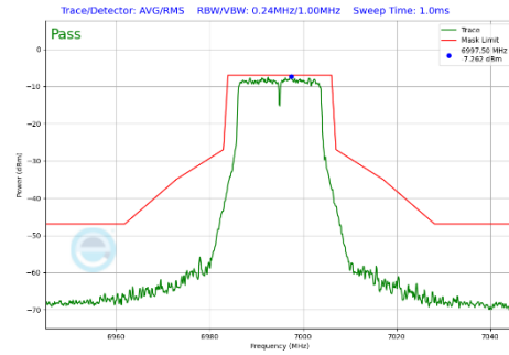
Plot 7-333 In-Band Emission Plot Antenna 4a (20MHz BW 802.11a (UNII Band 8) - Ch.209)
