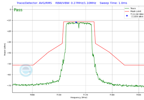
Plot 7-305 In-Band Emission Plot Antenna WF5B (20MHz BW 802.11be(SU) (UNII Band 8) - Ch.233)
