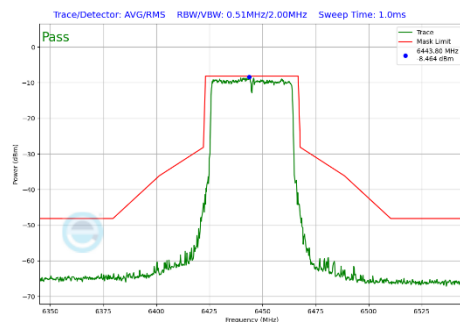
Plot 7-354 In-Band Emission Plot Antenna 2a (40MHz BW 802.11be(SU) (UNII Band 6) - Ch.99)
