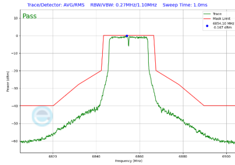
Plot 7-441 In-Band Emission Plot CDD Diversity Antenna 4a (20MHz BW 802.11a (UNII Band 7) - Ch.181)
