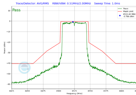
Plot 7-342 In-Band Emission Plot Antenna 2a (40MHz BW 802.11be(SU) (UNII Band 6) - Ch.115)
