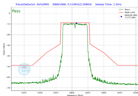
Plot 7-446 In-Band Emission Plot SDM Diversity Antenna 2a (40MHz BW 802.11be(SU) (UNII Band 5) - Ch.91)
