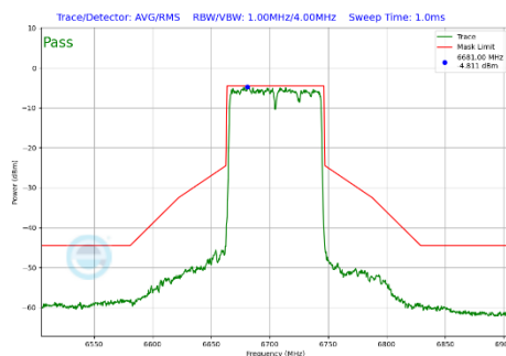
Plot 7-331 In-Band Emission Plot Antenna 4a (80MHz BW 802.11be(SU) (UNII Band 7) - Ch.151)
