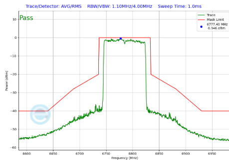
Plot 7-431 In-Band Emission Plot CDD Diversity Antenna 2a (80MHz BW 802.11be(SU) (UNII Band 7) - Ch.167)
