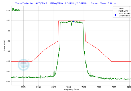
Plot 7-362 In-Band Emission Plot Antenna 2a (40MHz BW 802.11be(SU) (UNII Band 8) - Ch.211)
