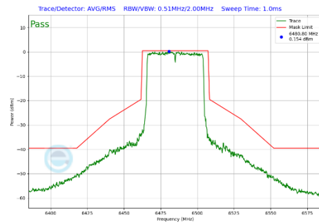
Plot 7-314 In-Band Emission Plot Antenna 4a (40MHz BW 802.11be(SU) (UNII Band 6) - Ch.107)
