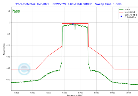
Plot 7-332 In-Band Emission Plot Antenna 4a (160MHz BW 802.11be(SU) (UNII Band 7) - Ch.143)
