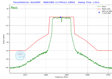
Plot 7-385 In-Band Emission Plot CDD Primary Antenna 4a (20MHz BW 802.11a (UNII Band 7) - Ch.181)
