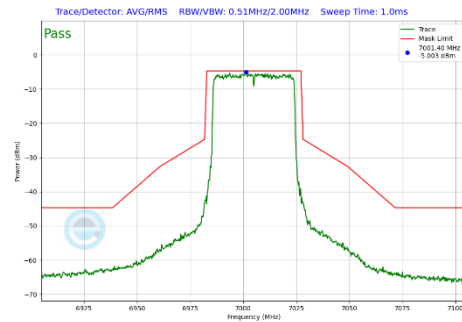
Plot 7-334 In-Band Emission Plot Antenna 4a (40MHz BW 802.11be(SU) (UNII Band 8) - Ch.211)
