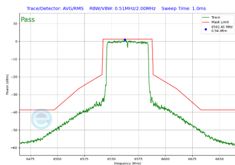
Plot 7-318 In-Band Emission Plot Antenna 4a (40MHz BW 802.11be(SU) (UNII Band 7) - Ch.123)
