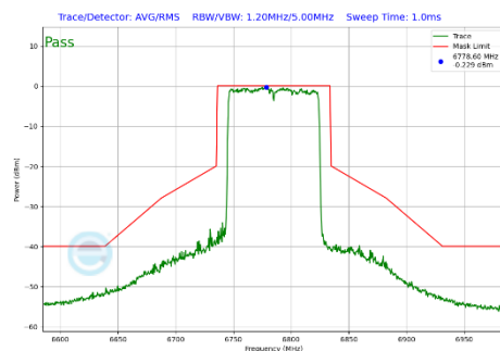
Plot 7-443 In-Band Emission Plot CDD Diversity Antenna 4a (80MHz BW 802.11be(SU) (UNII Band 7) - Ch.167)
