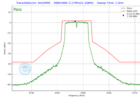
Plot 7-377 In-Band Emission Plot CDD Primary Antenna 4a (20MHz BW 802.11a (UNII Band 5) - Ch.45)
