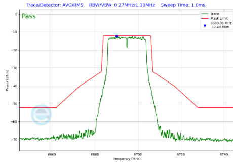
Plot 7-357 In-Band Emission Plot Antenna 2a (20MHz BW 802.11a (UNII Band 7) - Ch.149)
