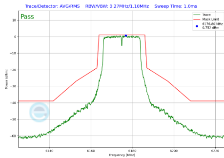
Plot 7-365 In-Band Emission Plot CDD Primary Antenna WF5B (20MHz BW 802.11a (UNII Band 5) - Ch.45)
