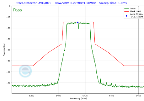
Plot 7-405 In-Band Emission Plot CDD Primary Antenna 4a (20MHz BW 802.11a (UNII Band 5) - Ch.93)
