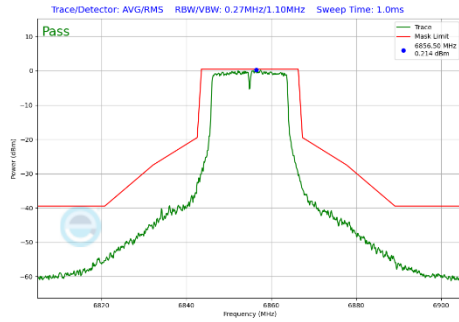
Plot 7-429 In-Band Emission Plot CDD Diversity Antenna 2a (20MHz BW 802.11a (UNII Band 7) - Ch.181)
