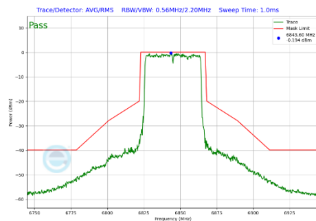
Plot 7-442 In-Band Emission Plot CDD Diversity Antenna 4a (40MHz BW 802.11be(SU) (UNII Band 7) - Ch.179)
