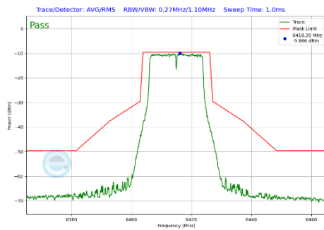
Plot 7-349 In-Band Emission Plot Antenna 2a (20MHz BW 802.11a (UNII Band 5) - Ch.93)
