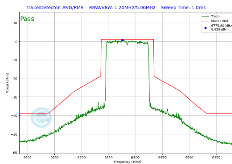
Plot 7-319 In-Band Emission Plot Antenna 4a (80MHz BW 802.11be(SU) (UNII Band 7) - Ch.167)
