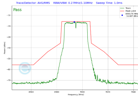
Plot 7-417 In-Band Emission Plot CDD Primary Antenna 4a (20MHz BW 802.11a (UNII Band 8) - Ch.209)
