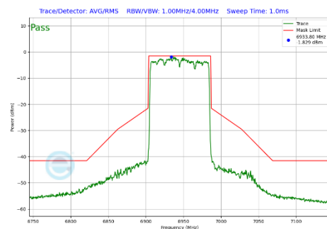
Plot 7-335 In-Band Emission Plot Antenna 4a (80MHz BW 802.11be(SU) (UNII Band 8) - Ch.199)
