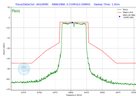
Plot 7-322 In-Band Emission Plot Antenna 4a (40MHz BW 802.11be(SU) (UNII Band 5) - Ch.91)
