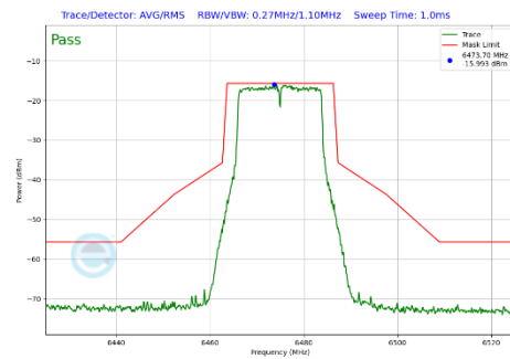
Plot 7-449 In-Band Emission Plot CDD Diversity Antenna 2a (20MHz BW 802.11a (UNII Band 6) - Ch.105)
