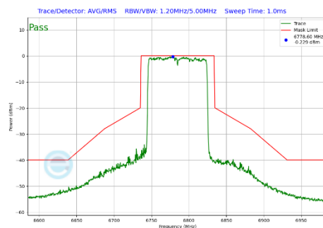
Plot 7-387 In-Band Emission Plot CDD Primary Antenna 4a (80MHz BW 802.11be(SU) (UNII Band 7) - Ch.167)
