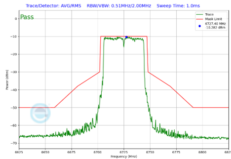
Plot 7-358 In-Band Emission Plot Antenna 2a (40MHz BW 802.11be(SU) (UNII Band 7) - Ch.155)
