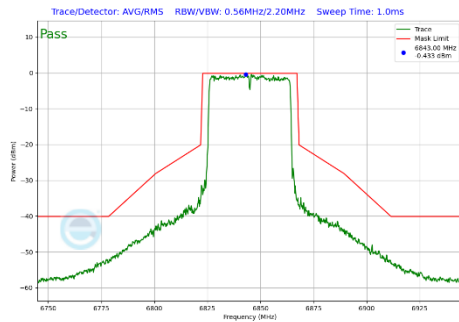
Plot 7-430 In-Band Emission Plot CDD Diversity Antenna 2a (40MHz BW 802.11be(SU) (UNII Band 7) - Ch.179)
