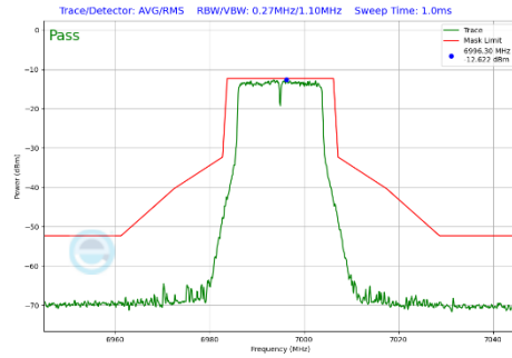
Plot 7-361 In-Band Emission Plot Antenna 2a (20MHz BW 802.11a (UNII Band 8) - Ch.209)
