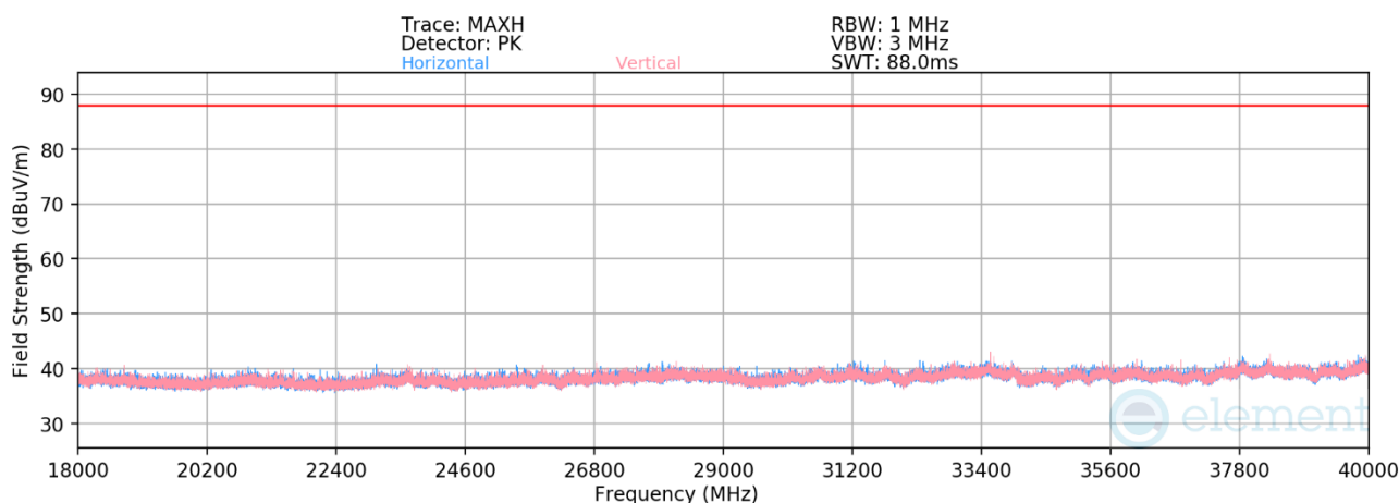
Plot 7-518. Radiated Spurious Emissions 18-40GHz CDD Primary (802.11be – Ch. 105)
