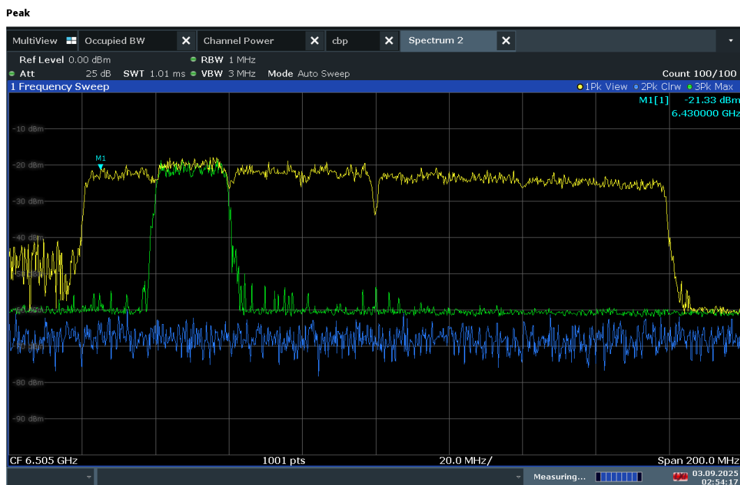
Plot 7-509. 160MHz Bandwidth, AWGN Signal Injected – 6430Mhz
