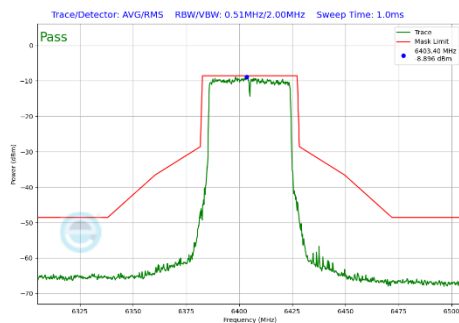
Plot 7-462 In-Band Emission Plot SDM Diversity Antenna 4a (40MHz BW 802.11be(SU) (UNII Band 5) - Ch.91)
