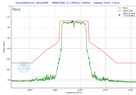
Plot 7-453 In-Band Emission Plot SDM Diversity Antenna 2a (20MHz BW 802.11be(SU) (UNII Band 7) - Ch.149)
