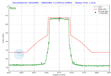
Plot 7-454 In-Band Emission Plot SDM Diversity Antenna 2a (40MHz BW 802.11be(SU) (UNII Band 7) - Ch.155)
