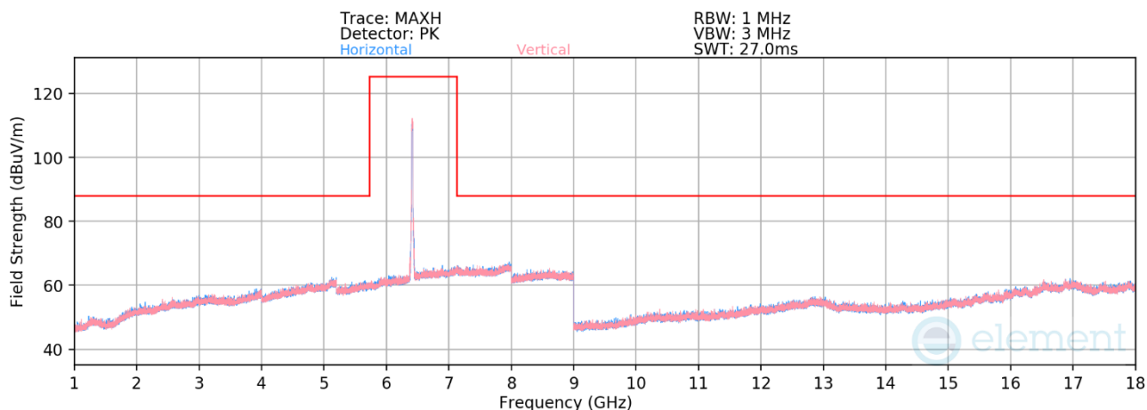
Plot 7-531. Radiated Spurious Emissions 1-18GHz CDD Diversity (802.11be – Ch. 93)
