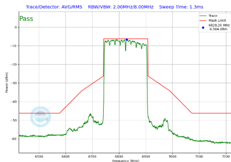
Plot 7-472 In-Band Emission Plot SDM Diversity Antenna 4a (160MHz BW 802.11be(SU) (UNII Band 7) - Ch.175)
