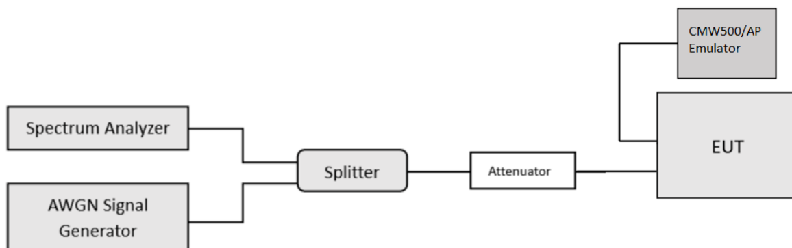
Figure 7-5. Contention-based protocol test setup, conducted method
