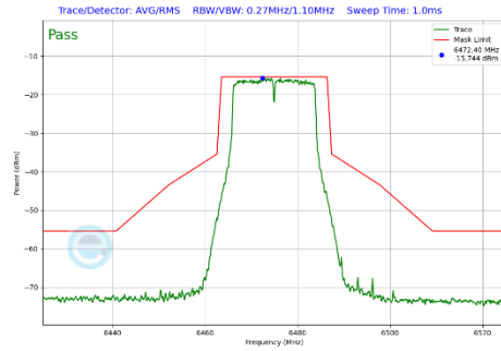
Plot 7-465 In-Band Emission Plot CDD Diversity Antenna 4a (20MHz BW 802.11a (UNII Band 6) - Ch.105)
