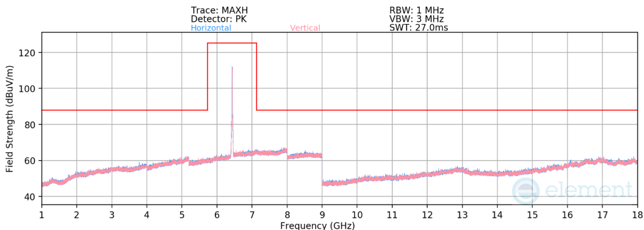
Plot 7-532. Radiated Spurious Emissions 1-18GHz CDD Diversity (802.11be – Ch. 97)
