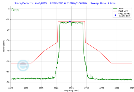
Plot 7-470 In-Band Emission Plot SDM Diversity Antenna 4a (40MHz BW 802.11be(SU) (UNII Band 7) - Ch.155)
