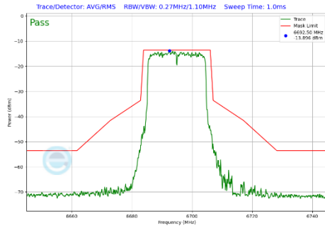
Plot 7-469 In-Band Emission Plot SDM Diversity Antenna 4a (20MHz BW 802.11be(SU) (UNII Band 7) - Ch.149)
