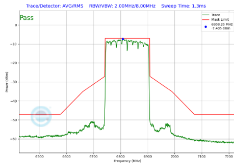
Plot 7-456 In-Band Emission Plot SDM Diversity Antenna 2a (160MHz BW 802.11be(SU) (UNII Band 7) - Ch.175)
