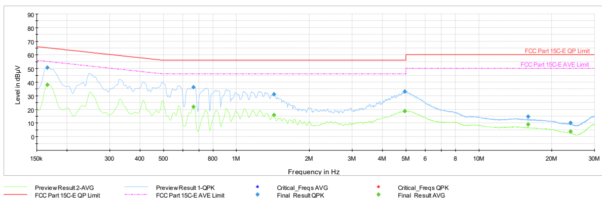
Plot 7-416. AC Line Conducted Plot with 802.11ax SDM Primary – Ch. 61 (N), with AC/DC Adaptor
