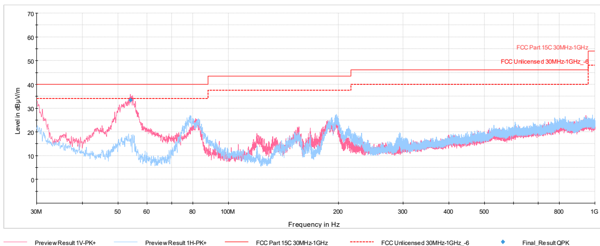
Plot 7-413. Radiated Spurious Emissions below 1GHz SDM Primary, 802.11be, Ch.61 with AC/DC Adaptor
