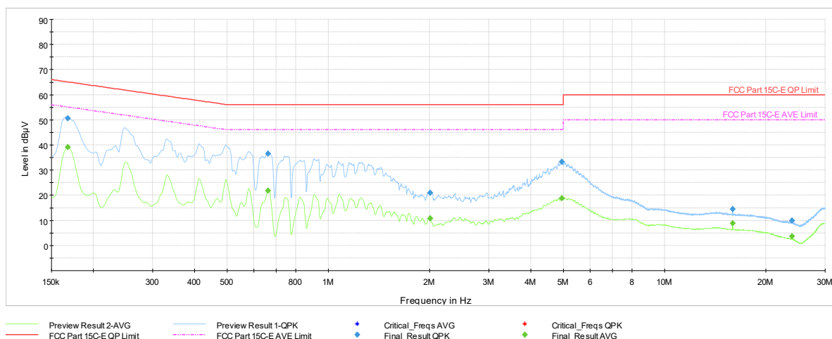
Plot 7-418. AC Line Conducted Plot with 802.11be SDM Diversity – Ch. 61 (N), with AC/DC Adaptor
