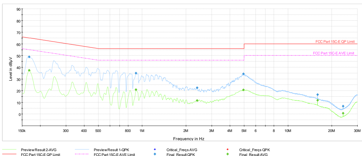
Plot 7-417. AC Line Conducted Plot with 802.11be SDM Diversity – Ch.61 (L1), with AC/DC Adaptor
