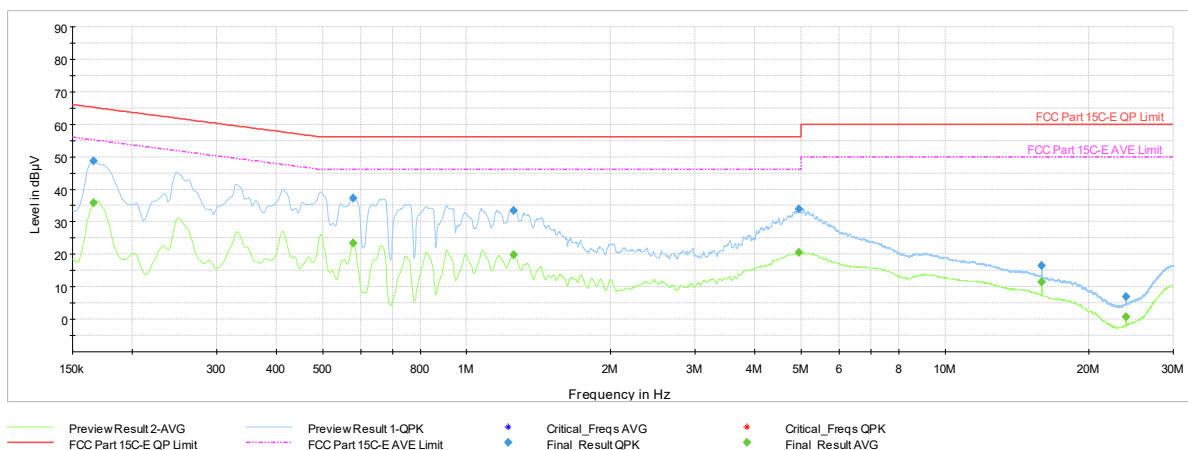
Plot 7-415. AC Line Conducted Plot with 802.11be SDM Primary – Ch.61 (L1), with AC/DC Adaptor
