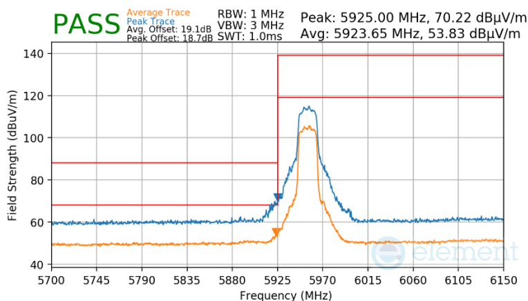
Plot 7-599 CDD Diversity Radiated Lower Band Edge (Peak & Average – UNII Band 5)
