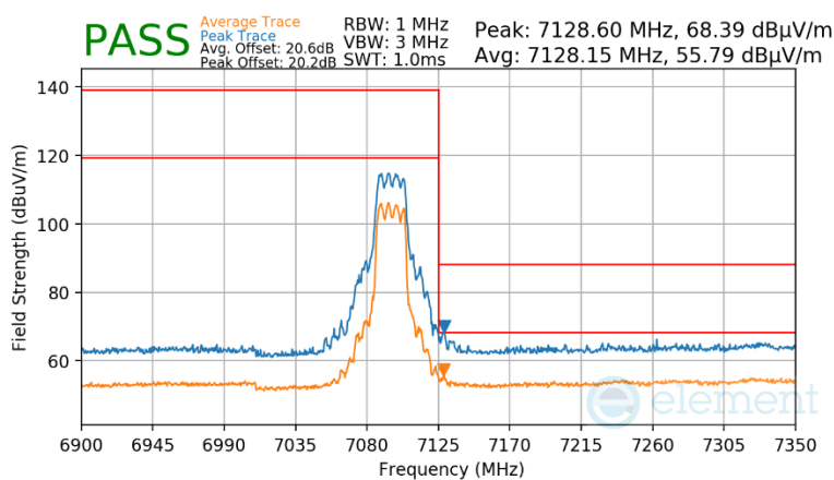
Plot 7-600 SDM Diversity Radiated Upper Band Edge (Peak & Average – UNII Band 8)
