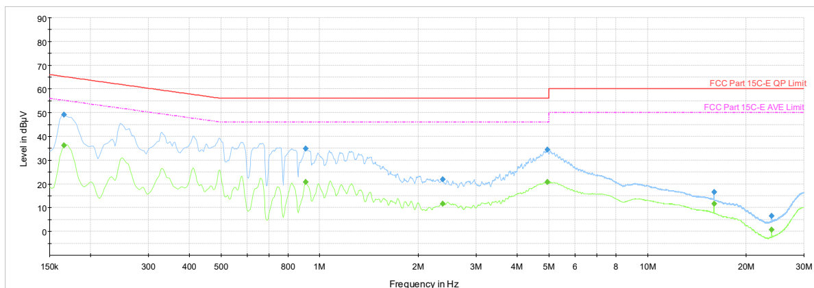
Plot 7-617. AC Line Conducted Plot with 802.11be CDD Diversity – Ch.45 (L1), with AC/DC adapter
