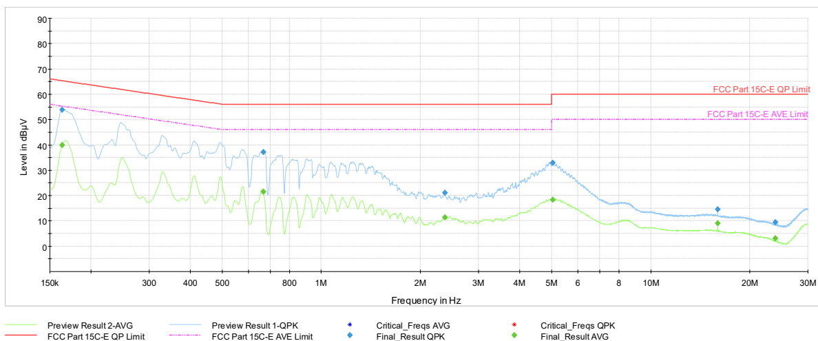
Plot 7-618. AC Line Conducted Plot with 802.11be CDD Diversity – Ch. 45 (N), with AC/DC adapter
