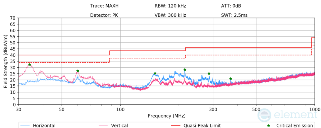
Plot 7-613. Radiated Spurious Emissions below 1GHz CDD Primary, 802.11be, Ch.45 with AC/DC adapter
