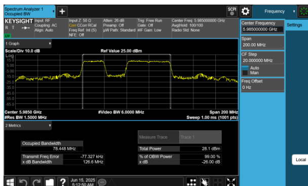
Plot 7-6 26dB BW & 99% OBW Antenna WF5B (80MHz BW 802.11be(RU) RU484+242 Index91 - Ch.7)
