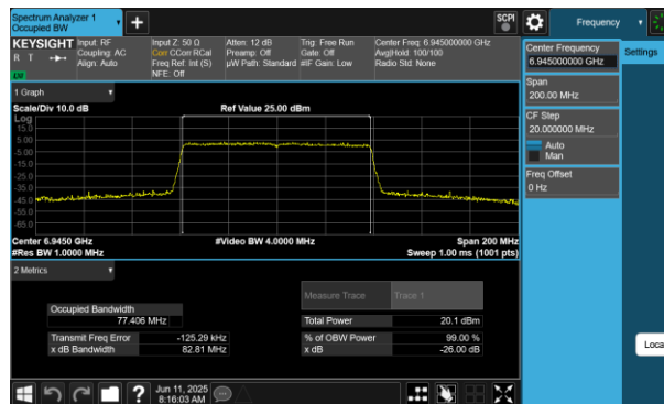
Plot 7-76 26dB BW & 99% OBW Antenna WF5B (80MHz BW 802.11be(RU) RU996 Index67 - Ch.199)
