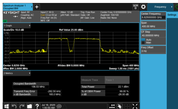
Plot 7-62 26dB BW & 99% OBW Antenna WF5B (160MHz BW 802.11be(RU) RU996+484+242 Index99 - Ch.175)
