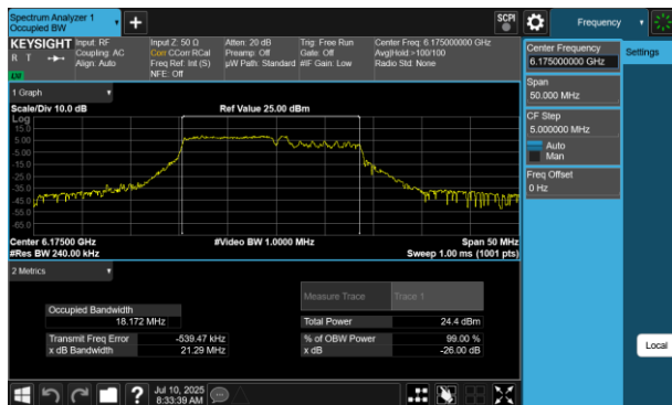
Plot 7-5 26dB BW & 99% OBW Antenna WF5B (20MHz BW 802.11be(RU) RU106+26 Index82 - Ch.45)
