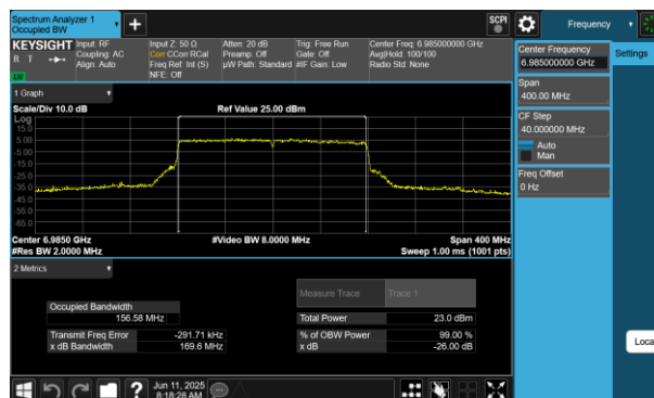
Plot 7-77 26dB BW & 99% OBW Antenna WF5B (160MHz BW 802.11be(RU) RU996X2 Index68 - Ch.207)
