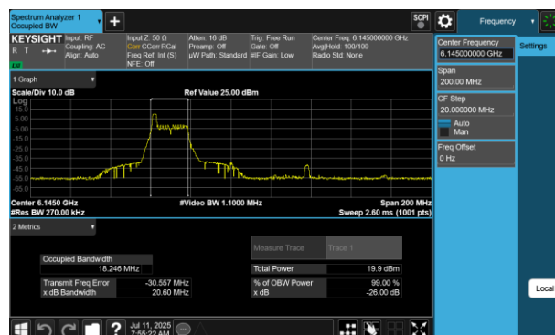
Plot 7-80 26dB BW & 99% OBW Antenna 4a(80MHz BW 802.11be(RU) RU26 Index0 - Ch.39)
