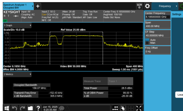
Plot 7-7 26dB BW & 99% OBW Antenna WF5B (160MHz BW 802.11be(RU) RU996+484+242 Index97 - Ch.47)
