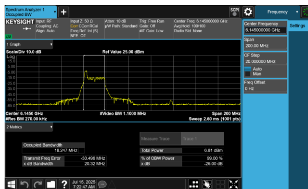
Plot 7-36 26dB BW & 99% OBW Antenna WF5B (80MHz BW 802.11be(RU) RU26 Index0 - Ch.39)
