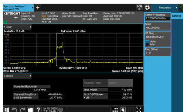
Plot 7-37 26dB BW & 99% OBW Antenna WF5B (160MHz BW 802.11be(RU) RU26 Index17 - Ch.15)
