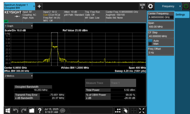
Plot 7-70 26dB BW & 99% OBW Antenna WF5B (160MHz BW 802.11be(RU) RU26 Index0 - Ch.207)
