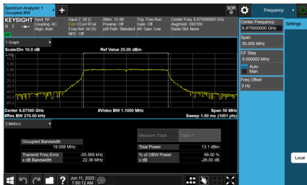
Plot 7-63 26dB BW & 99% OBW Antenna WF5B (20MHz BW 802.11be(RU) RU242 Index61 - Ch.185)
