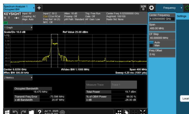
Plot 7-81 26dB BW & 99% OBW Antenna 4a(160MHz BW 802.11be(RU) RU26 Index0 - Ch.15)
