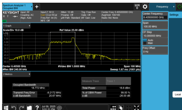
Plot 7-2 26dB BW & 99% OBW Antenna WF5B (40MHz BW 802.11be(RU) RU26 Index8 - Ch.91)
