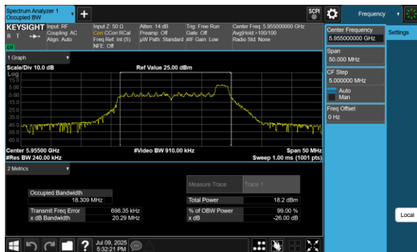
Plot 7-1 26dB BW & 99% OBW Antenna WF5B (20MHz BW 802.11be(RU) RU26 Index8 - Ch.1)
