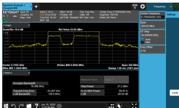
Plot 7-28 26dB BW & 99% OBW Antenna WF5B (80MHz BW 802.11be(RU) RU484+242 Index91 - Ch.151)
