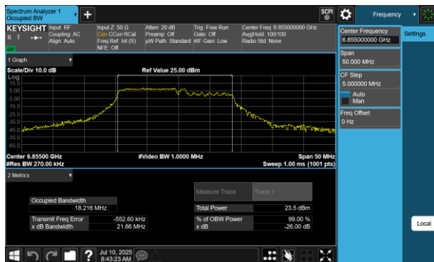
Plot 7-27 26dB BW & 99% OBW Antenna WF5B (20MHz BW 802.11be(RU) RU106+26 Index82 - Ch.181)
