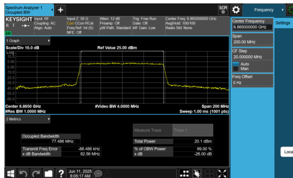
Plot 7-65 26dB BW & 99% OBW Antenna WF5B (80MHz BW 802.11be(RU) RU996 Index67 - Ch.183)
