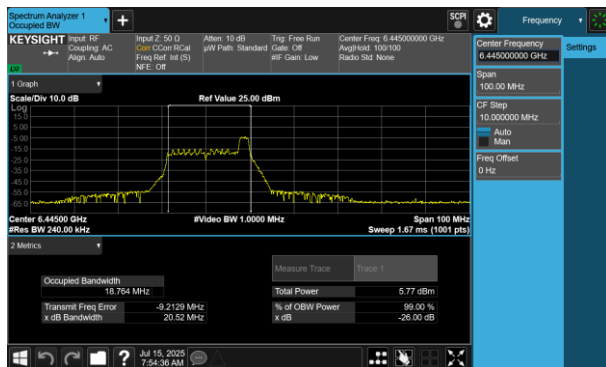
Plot 7-46 26dB BW & 99% OBW Antenna WF5B (40MHz BW 802.11be(RU) RU26 Index8 - Ch.99)
