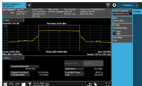
Plot 7-66 26dB BW & 99% OBW Antenna WF5B (160MHz BW 802.11be(RU) RU996X2 Index68 - Ch.143)
