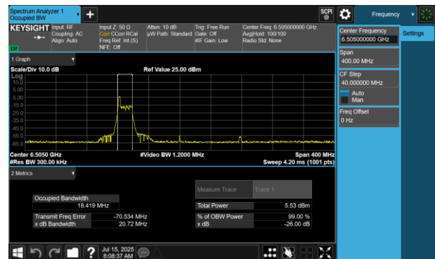
Plot 7-48 26dB BW & 99% OBW Antenna WF5B (160MHz BW 802.11be(RU) RU26 Index0 - Ch.111)
