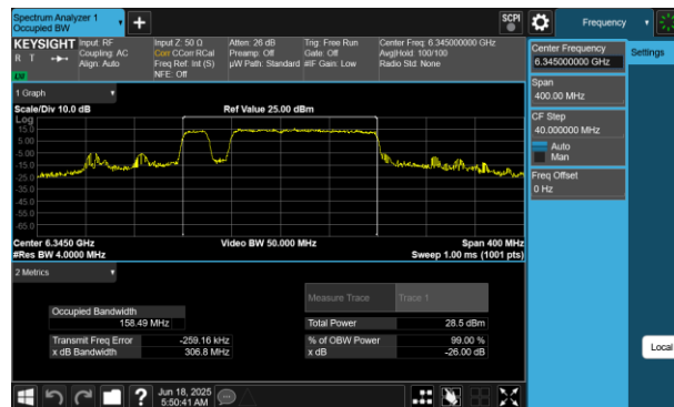
Plot 7-84 26dB BW & 99% OBW Antenna 4a(160MHz BW 802.11be(RU) RU996+484+242 Index97 - Ch.79)
