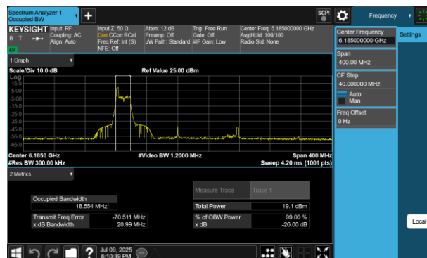
Plot 7-4 26dB BW & 99% OBW Antenna WF5B (160MHz BW 802.11be(RU) RU26 Index0 - Ch.47)
