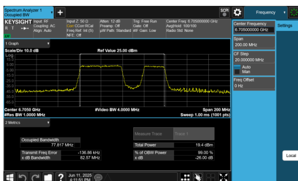
Plot 7-61 26dB BW & 99% OBW Antenna WF5B (80MHz BW 802.11be(RU) RU484+242 Index92 - Ch.151)
