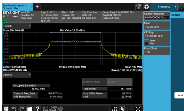
Plot 7-64 26dB BW & 99% OBW Antenna WF5B (40MHz BW 802.11be(RU) RU484 Index65 - Ch.179)
