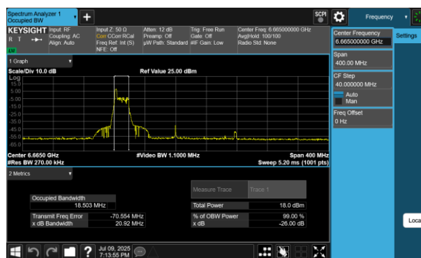
Plot 7-26 26dB BW & 99% OBW Antenna WF5B (160MHz BW 802.11be(RU) RU26 Index0 - Ch.143)
