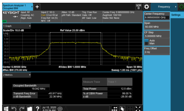
Plot 7-75 26dB BW & 99% OBW Antenna WF5B (20MHz BW 802.11be(RU) RU242 Index61 - Ch.209)
