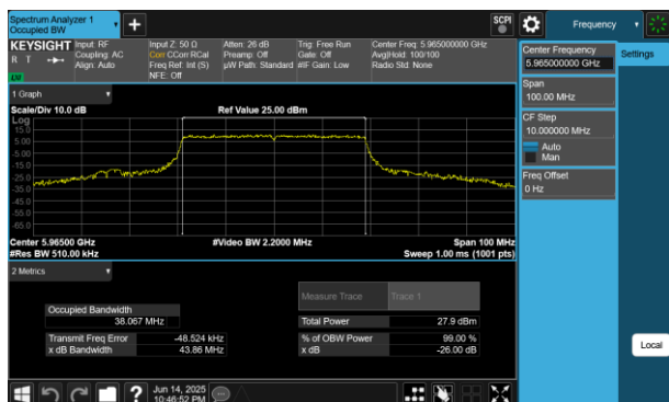
Plot 7-9 26dB BW & 99% OBW Antenna WF5B (40MHz BW 802.11be(RU) RU484 Index65 - Ch.3)
