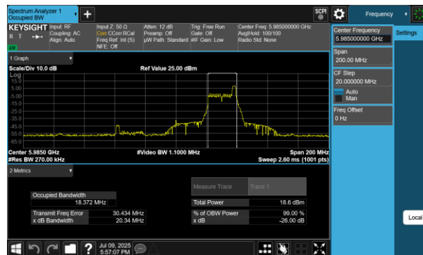
Plot 7-3 26dB BW & 99% OBW Antenna WF5B (80MHz BW 802.11be(RU) RU26 Index36 - Ch.7)
