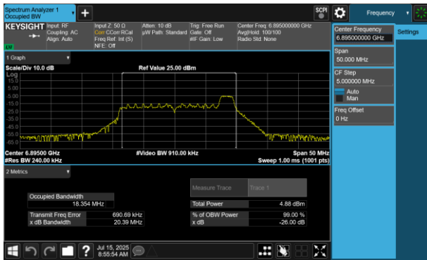
Plot 7-67 26dB BW & 99% OBW Antenna WF5B (20MHz BW 802.11be(RU) RU26 Index8 - Ch.189)
