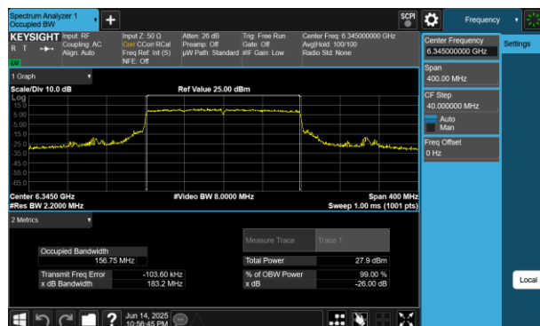
Plot 7-11 26dB BW & 99% OBW Antenna WF5B (160MHz BW 802.11be(RU) RU996X2 Index68 - Ch.79)
