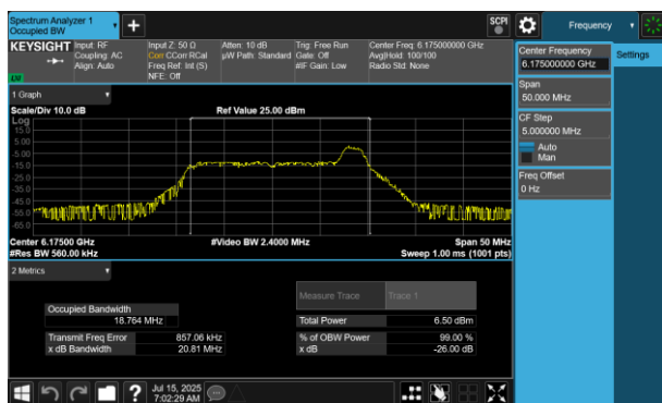
Plot 7-34 26dB BW & 99% OBW Antenna WF5B (20MHz BW 802.11be(RU) RU26 Index8 - Ch.45)
