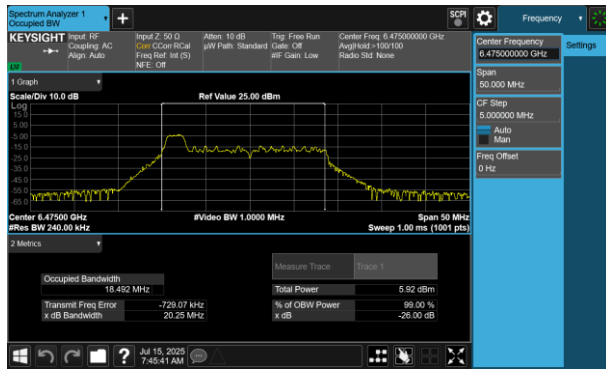
Plot 7-45 26dB BW & 99% OBW Antenna WF5B (20MHz BW 802.11be(RU) RU26 Index0 - Ch.105)
