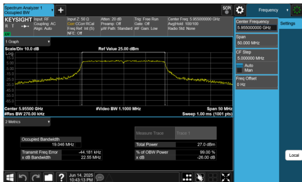
Plot 7-8 26dB BW & 99% OBW Antenna WF5B (20MHz BW 802.11be(RU) RU242 Index61 - Ch.1)
