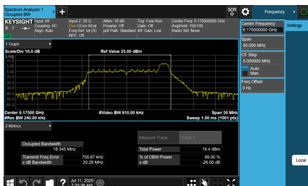
Plot 7-78 26dB BW & 99% OBW Antenna 4a(20MHz BW 802.11be(RU) RU26 Index8 - Ch.45)
