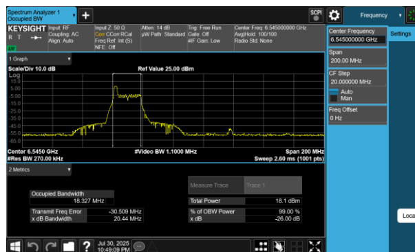
Plot 7-25 26dB BW & 99% OBW Antenna WF5B (80MHz BW 802.11be(RU) RU26 Index0 - Ch.119)
