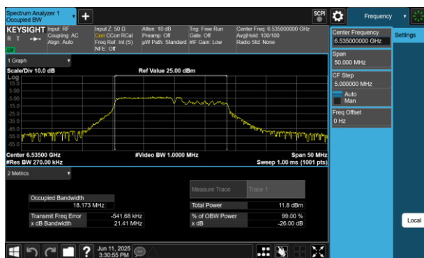
Plot 7-60 26dB BW & 99% OBW Antenna WF5B (20MHz BW 802.11be(RU) RU106+26 Index82 - Ch.117)
