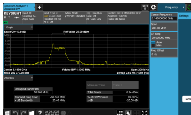
Plot 7-47 26dB BW & 99% OBW Antenna 4a (80MHz BW 802.11be(RU) RU26 Index0 - Ch.39)
