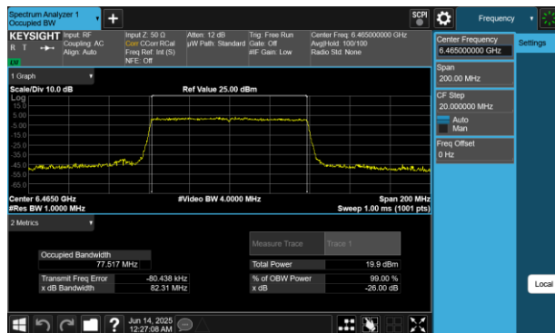
Plot 7-65 26dB BW & 99% OBW Antenna 4a (80MHz BW 802.11be(RU) RU996 Index67 - Ch.103)
