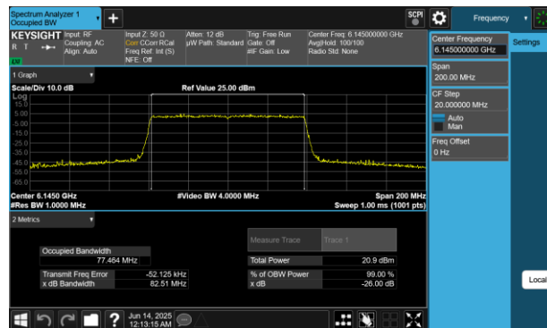
Plot 7-54 26dB BW & 99% OBW Antenna 4a (80MHz BW 802.11be(RU) RU996 Index67 - Ch.39)
