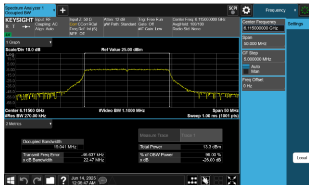
Plot 7-52 26dB BW & 99% OBW Antenna 4a (20MHz BW 802.11be(RU) RU242 Index61 - Ch.33)
