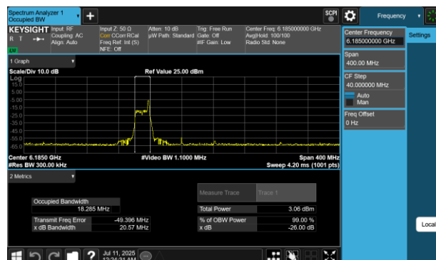
Plot 7-4 26dB BW & 99% OBW Antenna WF5B (160MHz BW 802.11be(RU) RU26 Index17 - Ch.47)
