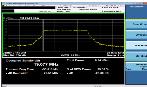
Plot 7-41 26dB BW & 99% OBW Antenna WF5B (20MHz BW 802.11be(RU) RU242 Index61 - Ch.233)
