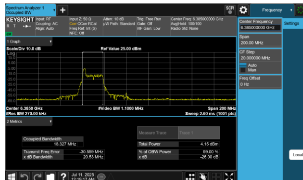
Plot 7-3 26dB BW & 99% OBW Antenna WF5B (80MHz BW 802.11be(RU) RU26 Index0 - Ch.87)
