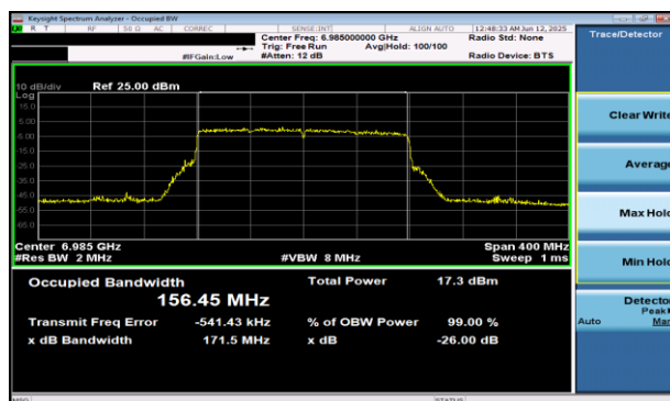
Plot 7-44 26dB BW & 99% OBW Antenna WF5B (160MHz BW 802.11be(RU) RU996X2 Index68 - Ch.207)
