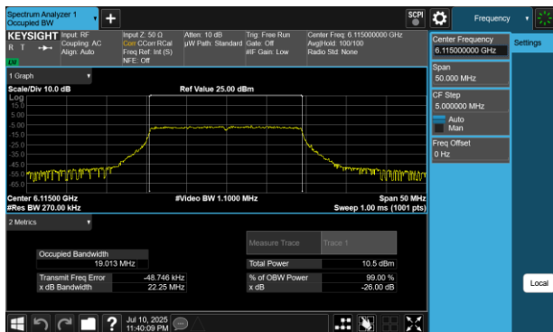
Plot 7-8 26dB BW & 99% OBW Antenna WF5B (20MHz BW 802.11be(RU) RU242 Index61 - Ch.33)
