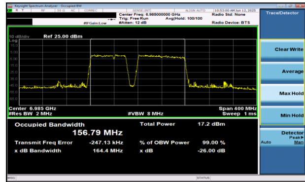
Plot 7-40 26dB BW & 99% OBW Antenna WF5B (160MHz BW 802.11be(RU) RU996+484+242 Index99 - Ch.207)
