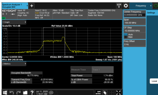
Plot 7-24 26dB BW & 99% OBW Antenna WF5B (40MHz BW 802.11be(RU) RU26 Index8 - Ch.179)
