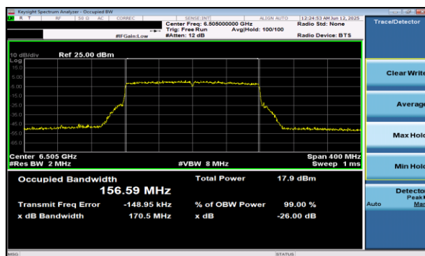
Plot 7-22 26dB BW & 99% OBW Antenna WF5B (160MHz BW 802.11be(RU) RU996X2 Index68 - Ch.111)
