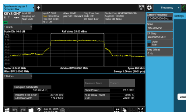
Plot 7-55 26dB BW & 99% OBW Antenna 4a (160MHz BW 802.11be(RU) RU996X2 Index68 - Ch.79)
