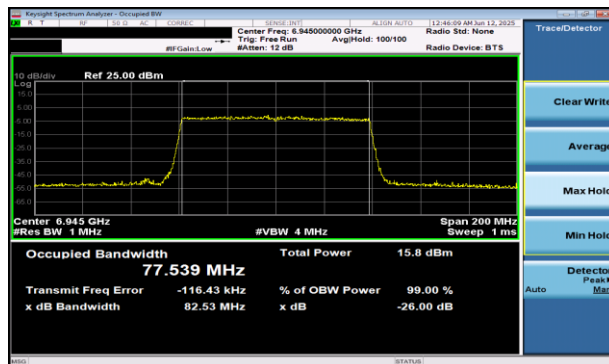
Plot 7-43 26dB BW & 99% OBW Antenna WF5B (80MHz BW 802.11be(RU) RU996 Index67 - Ch.199)
