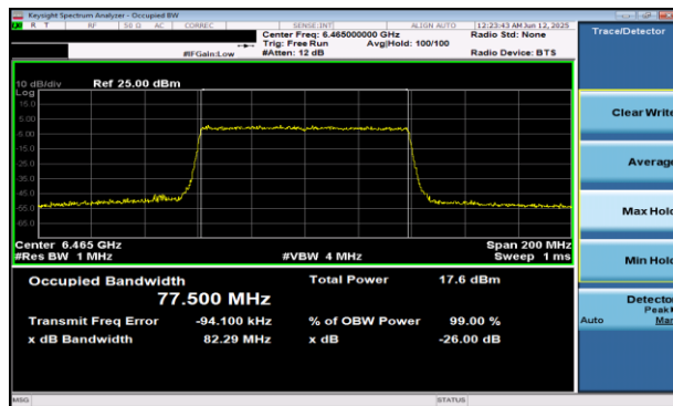
Plot 7-21 26dB BW & 99% OBW Antenna WF5B (80MHz BW 802.11be(RU) RU996 Index67 - Ch.103)
