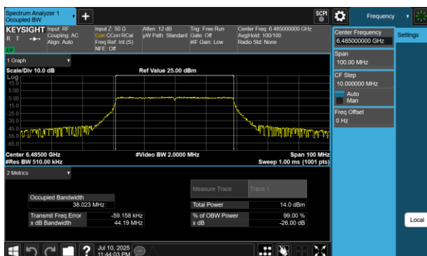
Plot 7-20 26dB BW & 99% OBW Antenna WF5B (40MHz BW 802.11be(RU) RU484 Index65 - Ch.107)
