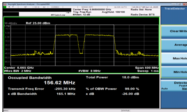
Plot 7-29 26dB BW & 99% OBW Antenna WF5B (160MHz BW 802.11be(RU) RU996+484+242 Index99 - Ch.143)
