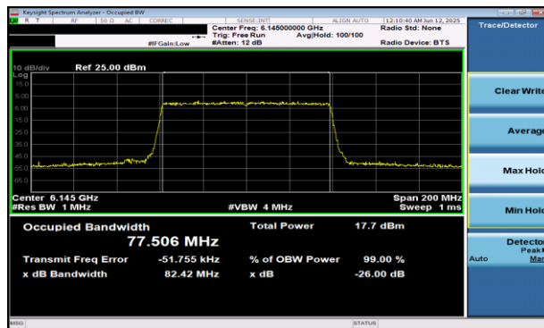
Plot 7-10 26dB BW & 99% OBW Antenna WF5B (80MHz BW 802.11be(RU) RU996 Index67 - Ch.39)
