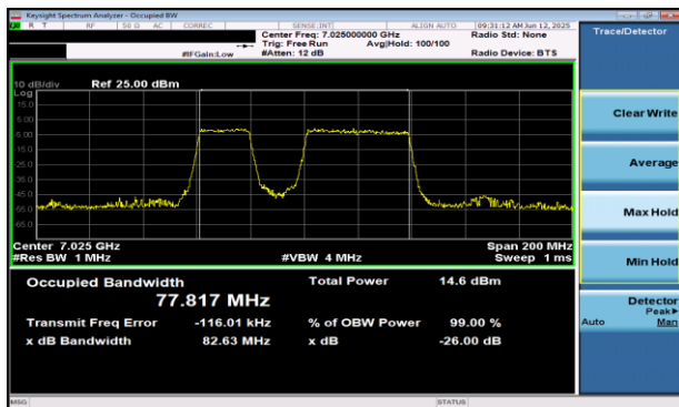
Plot 7-39 26dB BW & 99% OBW Antenna WF5B (80MHz BW 802.11be(RU) RU484+242 Index91 - Ch.215)
