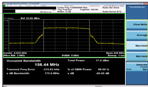
Plot 7-33 26dB BW & 99% OBW Antenna WF5B (160MHz BW 802.11be(RU) RU996X2 Index68 - Ch.175)
