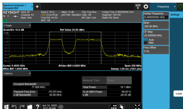
Plot 7-61 26dB BW & 99% OBW Antenna 4a (80MHz BW 802.11be(RU) RU484+242 Index91 - Ch.103)
