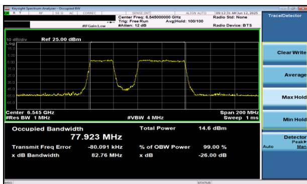
Plot 7-28 26dB BW & 99% OBW Antenna WF5B (80MHz BW 802.11be(RU) RU484+242 Index91 - Ch.119)
