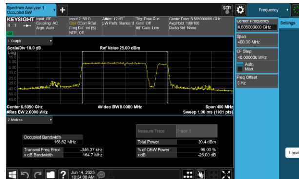
Plot 7-62 26dB BW & 99% OBW Antenna 4a (160MHz BW 802.11be(RU) RU996+484+242 Index98 - Ch.111)
