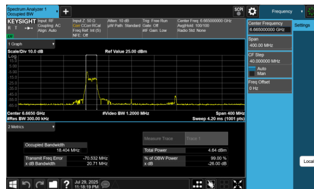
Plot 7-70 26dB BW & 99% OBW Antenna 4a (160MHz BW 802.11be(RU) RU26 Index0 - Ch.143)
