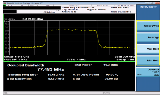
Plot 7-32 26dB BW & 99% OBW Antenna WF5B (80MHz BW 802.11be(RU) RU996 Index67 - Ch.119)
