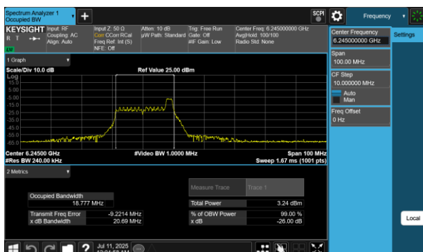
Plot 7-2 26dB BW & 99% OBW Antenna WF5B (40MHz BW 802.11be(RU) RU26 Index8 - Ch.59)
