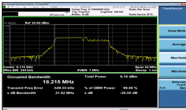
Plot 7-5 26dB BW & 99% OBW Antenna WF5B (20MHz BW 802.11be(RU) RU106+26 Index82 - Ch.33)
