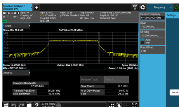
Plot 7-53 26dB BW & 99% OBW Antenna 4a (40MHz BW 802.11be(RU) RU484 Index65 - Ch.91)
