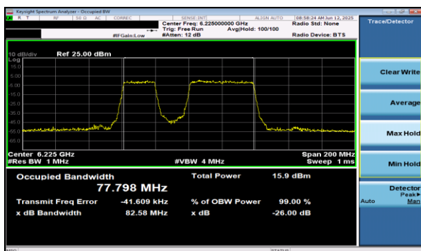
Plot 7-6 26dB BW & 99% OBW Antenna WF5B (80MHz BW 802.11be(RU) RU484+242 Index91 - Ch.55)
