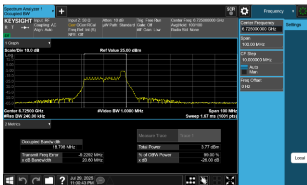
Plot 7-68 26dB BW & 99% OBW Antenna 4a (40MHz BW 802.11be(RU) RU26 Index8 - Ch.155)
