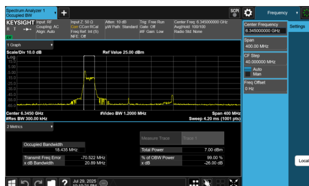
Plot 7-48 26dB BW & 99% OBW Antenna 4a (160MHz BW 802.11be(RU) RU26 Index0 - Ch.79)
