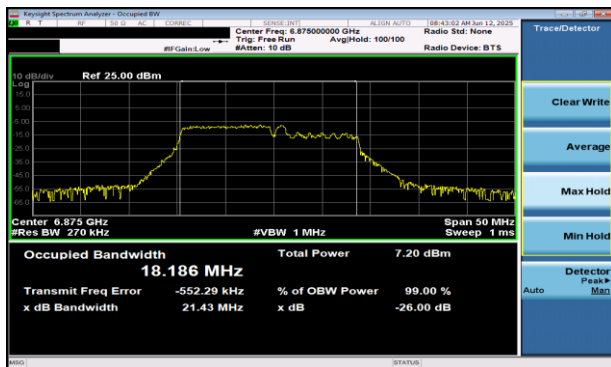
Plot 7-27 26dB BW & 99% OBW Antenna WF5B (20MHz BW 802.11be(RU) RU106+26 Index82 - Ch.185)
