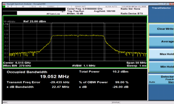
Plot 7-19 26dB BW & 99% OBW Antenna WF5B (20MHz BW 802.11be(RU) RU242 Index61 - Ch.113)
