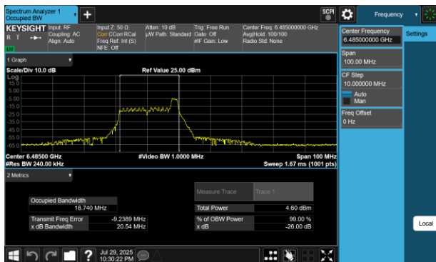
Plot 7-57 26dB BW & 99% OBW Antenna 4a (40MHz BW 802.11be(RU) RU26 Index8 - Ch.107)
