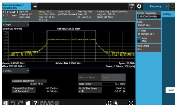
Plot 7-64 26dB BW & 99% OBW Antenna 4a (40MHz BW 802.11be(RU) RU484 Index65 - Ch.107)
