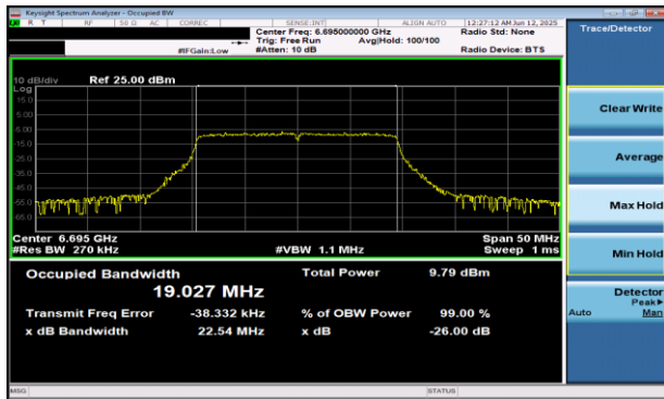
Plot 7-30 26dB BW & 99% OBW Antenna WF5B (20MHz BW 802.11be(RU) RU242 Index61 - Ch.149)
