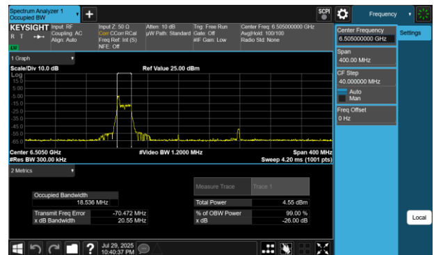
Plot 7-59 26dB BW & 99% OBW Antenna 4a (160MHz BW 802.11be(RU) RU26 Index0 - Ch.111)
