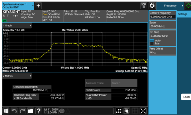
Plot 7-38 26dB BW & 99% OBW Antenna WF5B (20MHz BW 802.11be(RU) RU106+26 Index82 - Ch.209)
