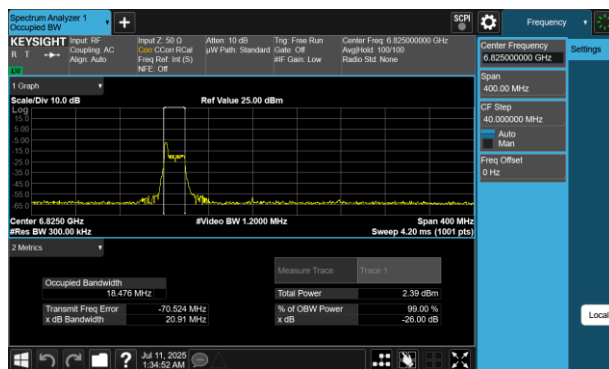
Plot 7-26 26dB BW & 99% OBW Antenna WF5B (160MHz BW 802.11be(RU) RU26 Index0 - Ch.175)
