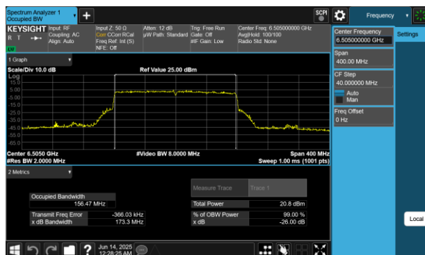
Plot 7-66 26dB BW & 99% OBW Antenna 4a (160MHz BW 802.11be(RU) RU996X2 Index68 - Ch.111)
