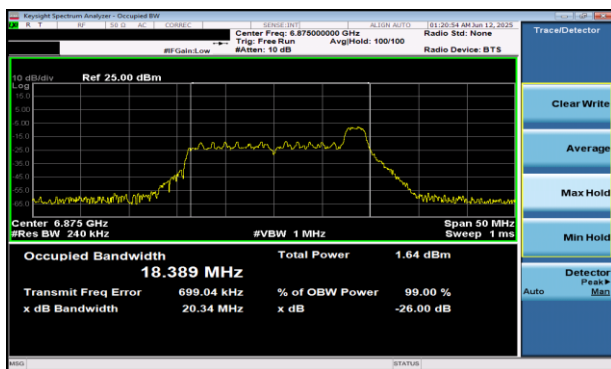
Plot 7-23 26dB BW & 99% OBW Antenna WF5B (20MHz BW 802.11be(RU) RU26 Index8 - Ch.185)
