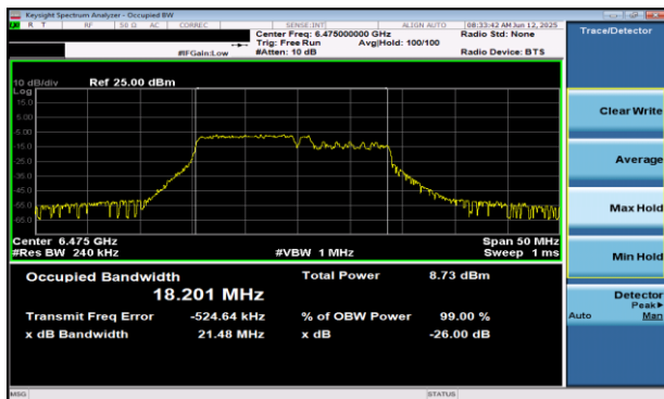
Plot 7-16 26dB BW & 99% OBW Antenna WF5B (20MHz BW 802.11be(RU) RU106+26 Index82 - Ch.105)
