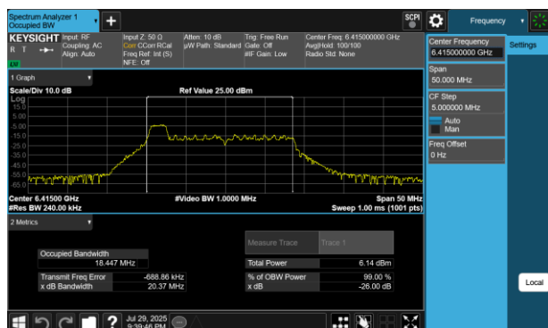
Plot 7-45 26dB BW & 99% OBW Antenna 4a (20MHz BW 802.11be(RU) RU26 Index0 - Ch.93)
