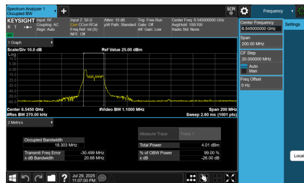
Plot 7-69 26dB BW & 99% OBW Antenna 4a (80MHz BW 802.11be(RU) RU26 Index0 - Ch.119)
