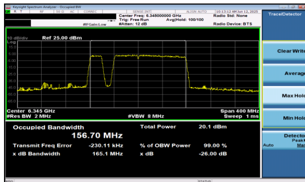
Plot 7-7 26dB BW & 99% OBW Antenna WF5B (160MHz BW 802.11be(RU) RU996+484+242 Index97 - Ch.79)
