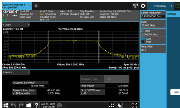
Plot 7-63 26dB BW & 99% OBW Antenna 4a (20MHz BW 802.11be(RU) RU242 Index61 - Ch.97)
