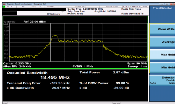
Plot 7-1 26dB BW & 99% OBW Antenna WF5B (20MHz BW 802.11be(RU) RU26 Index0 - Ch.61)
