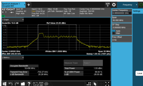
Plot 7-34 26dB BW & 99% OBW Antenna WF5B (20MHz BW 802.11be(RU) RU26 Index0 - Ch.209)
