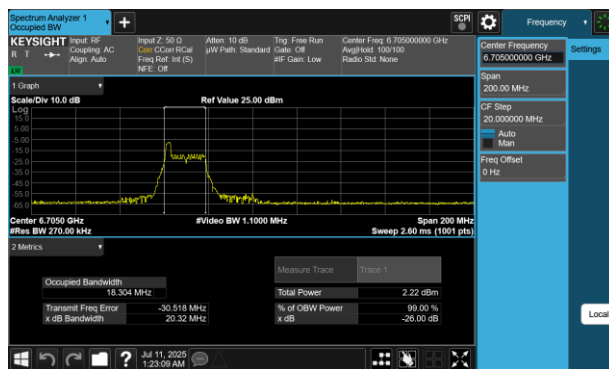
Plot 7-25 26dB BW & 99% OBW Antenna WF5B (80MHz BW 802.11be(RU) RU26 Index0 - Ch.151)
