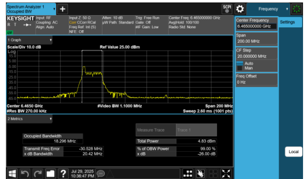
Plot 7-58 26dB BW & 99% OBW Antenna 4a (80MHz BW 802.11be(RU) RU26 Index0 - Ch.103)
