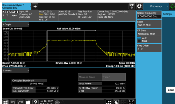
Plot 7-42 26dB BW & 99% OBW Antenna WF5B (40MHz BW 802.11be(RU) RU484 Index65 - Ch.211)
