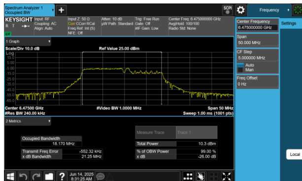
Plot 7-60 26dB BW & 99% OBW Antenna 4a (20MHz BW 802.11be(RU) RU106+26 Index82 - Ch.105)
