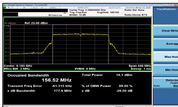
Plot 7-11 26dB BW & 99% OBW Antenna WF5B (160MHz BW 802.11be(RU) RU996X2 Index68 - Ch.47)
