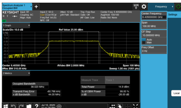
Plot 7-9 26dB BW & 99% OBW Antenna WF5B (40MHz BW 802.11be(RU) RU484 Index65 - Ch.91)
