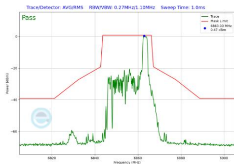
Plot 7-779 In-Band Emission Plot Antenna WF5B (20MHz BW 802.11be(RU) RU26 Index8 (UNII Band 7) - Ch.181)
