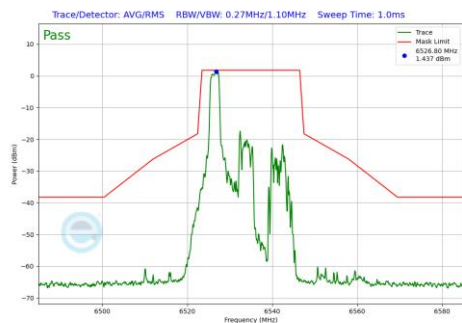
Plot 7-856 In-Band Emission Plot Antenna 4a(20MHz BW 802.11be(RU) RU26 Index0 (UNII Band 7) - Ch.117)
