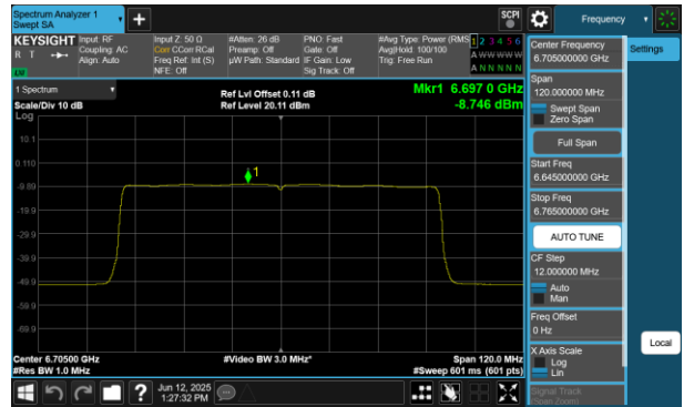
Plot 7-747 PSD SDM Diversity Antenna 2a (80MHz BW 802.11be(RU) RU996 Index67 - Ch.151)
