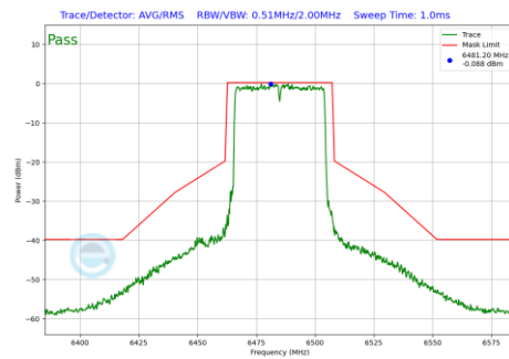
Plot 7-797 In-Band Emission Plot Antenna WF5B (40MHz BW 802.11be(RU) RU484 Index65 (UNII Band 6) - Ch.107)
