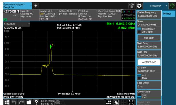
Plot 7-756 PSD SDM Diversity Antenna 2a (160MHz BW 802.11be(RU) RU26 Index17 - Ch.207)
