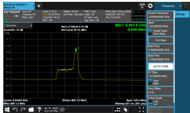
Plot 7-755 PSD SDM Diversity Antenna 2a (80MHz BW 802.11be(RU) RU26 Index17 - Ch.199)
