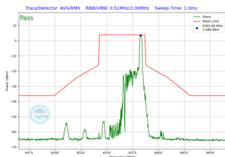
Plot 7-857 In-Band Emission Plot Antenna 4a(40MHz BW 802.11be(RU) RU26 Index17 (UNII Band 7) - Ch.123)
