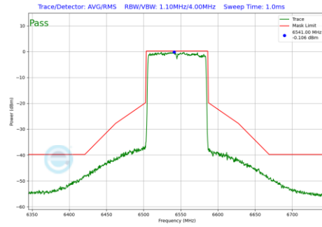
Plot 7-802 In-Band Emission Plot Antenna WF5B (80MHz BW 802.11be(RU) RU996 Index67 (UNII Band 7) - Ch.119)
