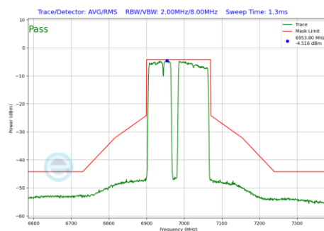
Plot 7-831 In-Band Emission Plot Antenna WF5B (160MHz BW 802.11be(RU) RU996+484+242 Index99 (UNII Band 8) - Ch.207)
