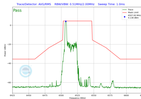
Plot 7-853 In-Band Emission Plot Antenna 4a(40MHz BW 802.11be(RU) RU26 Index0 (UNII Band 6) - Ch.115)
