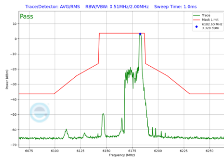
Plot 7-772 In-Band Emission Plot Antenna WF5B (40MHz BW 802.11be(RU) RU26 Index17 (UNII Band 5) - Ch.43)
