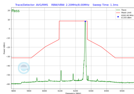
Plot 7-851 In-Band Emission Plot Antenna 4a(160MHz BW 802.11be(RU) RU26 Index36 (UNII Band 5) - Ch.47)
