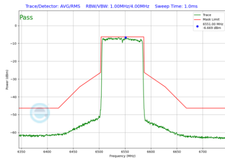
Plot 7-842 In-Band Emission Plot Antenna WF5B (80MHz BW 802.11be(RU) RU996 Index67 (UNII Band 7) - Ch.119)
