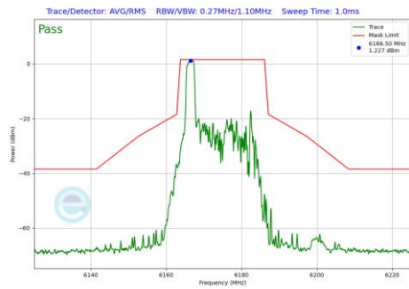
Plot 7-771 In-Band Emission Plot Antenna WF5B (20MHz BW 802.11be(RU) RU26 Index0 (UNII Band 5) - Ch.45)
