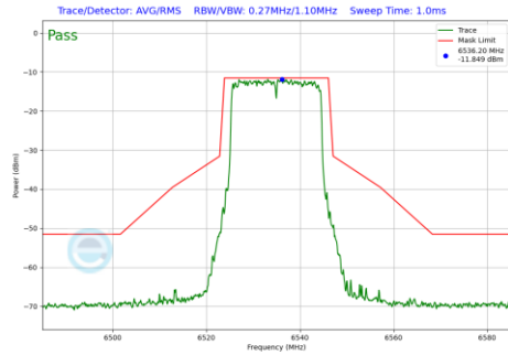
Plot 7-840 In-Band Emission Plot Antenna WF5B (20MHz BW 802.11be(RU) RU242 Index61 (UNII Band 7) - Ch.117)
