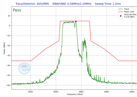
Plot 7-860 In-Band Emission Plot Antenna 4a(20MHz BW 802.11be(RU) RU106+26 Index82 (UNII Band 5) - Ch.1)
