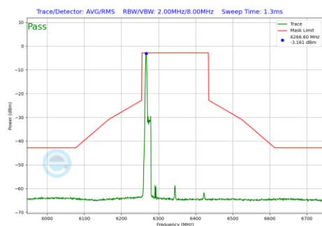
Plot 7-807 In-Band Emission Plot Antenna WF5B (160MHz BW 802.11be(RU) RU26 Index0 (UNII Band 5) - Ch.79)
