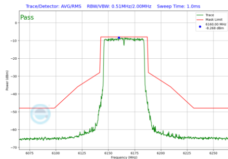
Plot 7-833 In-Band Emission Plot Antenna WF5B (40MHz BW 802.11be(RU) RU484 Index65 (UNII Band 5) - Ch.43)
