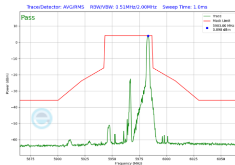
Plot 7-849 In-Band Emission Plot Antenna 4a(40MHz BW 802.11be(RU) RU26 Index17 (UNII Band 5) - Ch.3)
