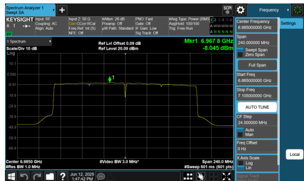
Plot 7-770 PSD SDM Diversity Antenna 2a (160MHz BW 802.11be(RU) RU996X2 Index68 - Ch.207)
