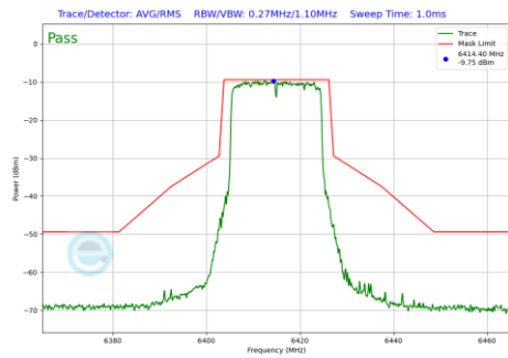
Plot 7-832 In-Band Emission Plot Antenna WF5B (20MHz BW 802.11be(RU) RU242 Index61 (UNII Band 5) - Ch.93)
