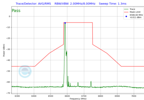
Plot 7-815 In-Band Emission Plot Antenna WF5B (160MHz BW 802.11be(RU) RU26 Index0 (UNII Band 7) - Ch.143)
