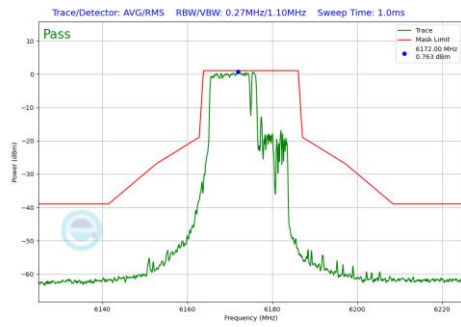
Plot 7-783 In-Band Emission Plot Antenna WF5B (20MHz BW 802.11be(RU) RU106+26 Index82 (UNII Band 5) - Ch.45)
