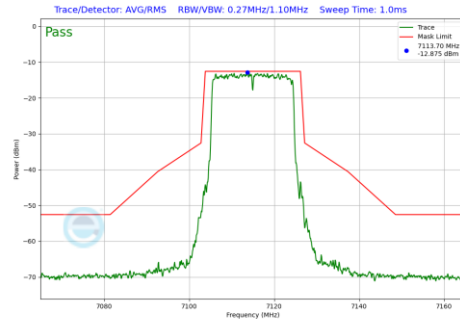
Plot 7-844 In-Band Emission Plot Antenna WF5B (20MHz BW 802.11be(RU) RU242 Index61 (UNII Band 8) - Ch.233)
