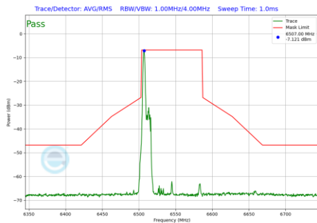
Plot 7-814 In-Band Emission Plot Antenna WF5B (80MHz BW 802.11be(RU) RU26 Index0 (UNII Band 7) - Ch.119)
