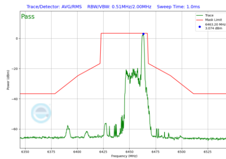
Plot 7-776 In-Band Emission Plot Antenna WF5B (40MHz BW 802.11be(RU) RU26 Index17 (UNII Band 6) - Ch.99)
