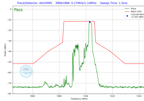
Plot 7-816 In-Band Emission Plot Antenna WF5B (20MHz BW 802.11be(RU) RU26 Index8 (UNII Band 8) - Ch.229)
