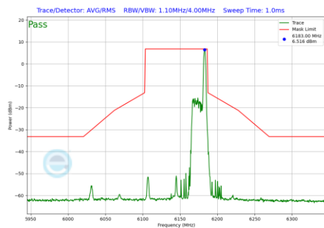
Plot 7-773 In-Band Emission Plot Antenna WF5B (80MHz BW 802.11be(RU) RU26 Index36 (UNII Band 5) - Ch.39)
