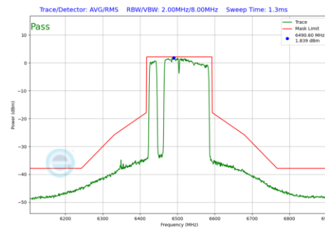
Plot 7-865 In-Band Emission Plot Antenna 4a(160MHz BW 802.11be(RU) RU996+484+242 Index97 (UNII Band 6) - Ch.111)
