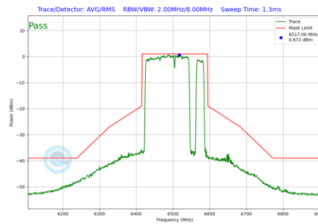
Plot 7-788 In-Band Emission Plot Antenna WF5B (160MHz BW 802.11be(RU) RU996+484+242 Index98 (UNII Band 6) - Ch.111)
