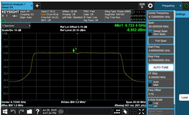
Plot 7-742 PSD SDM Diversity Antenna 4a(40MHz BW 802.11be(RU) RU484 Index65 - Ch.155)
