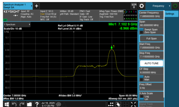
Plot 7-754 PSD SDM Diversity Antenna 2a (40MHz BW 802.11be(RU) RU26 Index17 - Ch.227)
