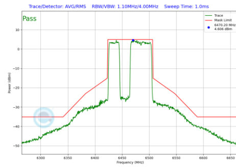
Plot 7-864 In-Band Emission Plot Antenna 4a(80MHz BW 802.11be(RU) RU484+242 Index91 (UNII Band 6) - Ch.103)
