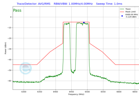
Plot 7-824 In-Band Emission Plot Antenna WF5B (80MHz BW 802.11be(RU) RU484+242 Index91 (UNII Band 6) - Ch.103)
