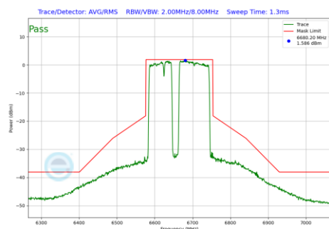
Plot 7-868 In-Band Emission Plot Antenna 4a(160MHz BW 802.11be(RU) RU996+484+242 Index99 (UNII Band 7) - Ch.143)
