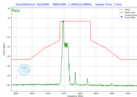
Plot 7-858 In-Band Emission Plot Antenna 4a(80MHz BW 802.11be(RU) RU26 Index0 (UNII Band 7) - Ch.167)
