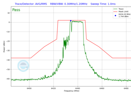
Plot 7-863 In-Band Emission Plot Antenna 4a(20MHz BW 802.11be(RU) RU106+26 Index83 (UNII Band 6) - Ch.97)
