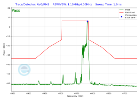
Plot 7-781 In-Band Emission Plot Antenna WF5B (80MHz BW 802.11be(RU) RU26 Index36 (UNII Band 7) - Ch.119)
