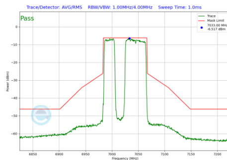
Plot 7-830 In-Band Emission Plot Antenna WF5B (80MHz BW 802.11be(RU) RU484+242 Index91 (UNII Band 8) - Ch.215)
