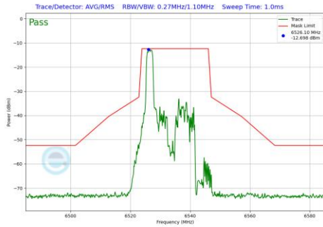
Plot 7-812 In-Band Emission Plot Antenna WF5B (20MHz BW 802.11be(RU) RU26 Index0 (UNII Band 7) - Ch.117)
