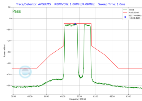
Plot 7-821 In-Band Emission Plot Antenna WF5B (80MHz BW 802.11be(RU) RU484+242 Index92 (UNII Band 5) - Ch.39)
