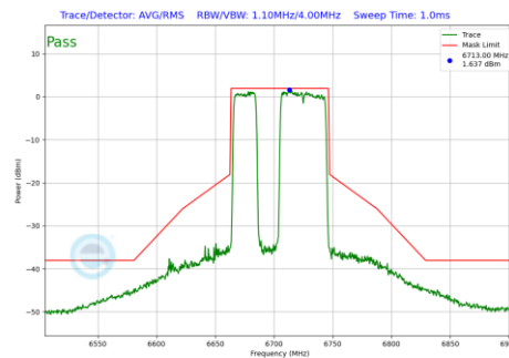
Plot 7-790 In-Band Emission Plot Antenna WF5B (80MHz BW 802.11be(RU) RU484+242 Index91 (UNII Band 7) - Ch.151)
