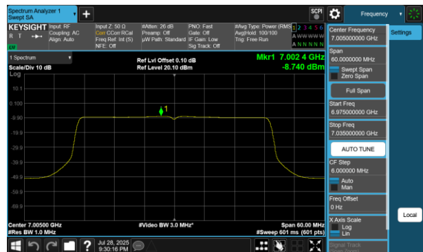
Plot 7-768 PSD SDM Diversity Antenna 2a (40MHz BW 802.11be(RU) RU484 Index65 - Ch.211)
