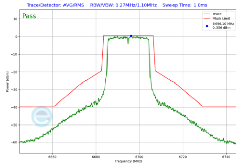
Plot 7-800 In-Band Emission Plot Antenna WF5B (20MHz BW 802.11be(RU) RU242 Index61 (UNII Band 7) - Ch.149)
