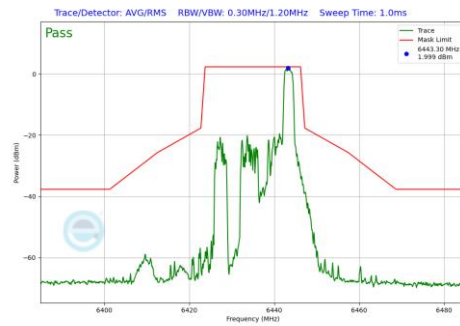
Plot 7-852 In-Band Emission Plot Antenna 4a(20MHz BW 802.11be(RU) RU26 Index8 (UNII Band 6) - Ch.97)
