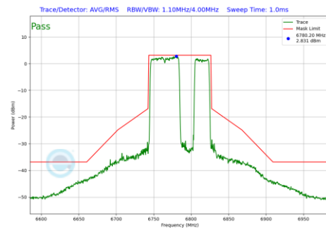
Plot 7-867 In-Band Emission Plot Antenna 4a(80MHz BW 802.11be(RU) RU484+242 Index92 (UNII Band 7) - Ch.167)
