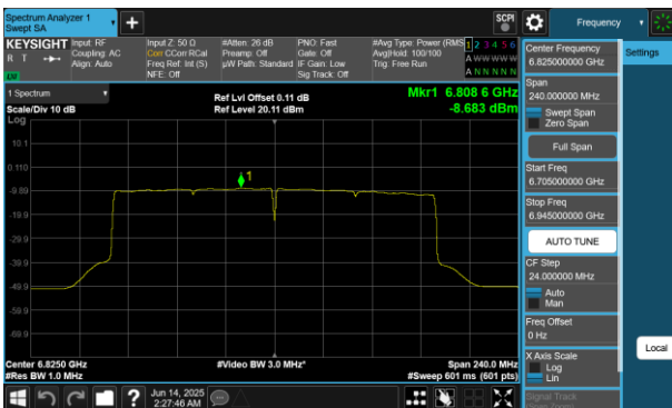
Plot 7-744 PSD SDM Diversity Antenna 4a(160MHz BW 802.11be(RU) RU996X2 Index68 - Ch.175)
