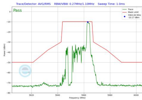
Plot 7-804 In-Band Emission Plot Antenna WF5B (20MHz BW 802.11be(RU) RU26 Index8 (UNII Band 5) - Ch.1)
