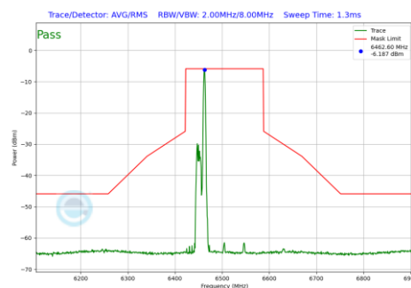
Plot 7-811 In-Band Emission Plot Antenna WF5B (160MHz BW 802.11be(RU) RU26 Index17 (UNII Band 6) - Ch.111)
