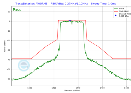
Plot 7-796 In-Band Emission Plot Antenna WF5B (20MHz BW 802.11be(RU) RU242 Index61 (UNII Band 6) - Ch.97)
