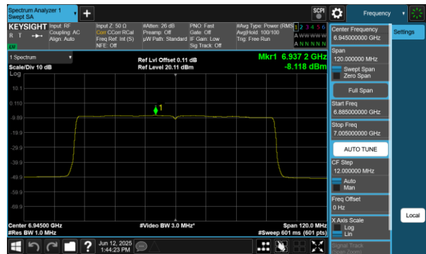
Plot 7-769 PSD SDM Diversity Antenna 2a (80MHz BW 802.11be(RU) RU996 Index67 - Ch.199)
