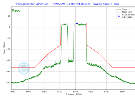
Plot 7-861 In-Band Emission Plot Antenna 4a(80MHz BW 802.11be(RU) RU484+242 Index91 (UNII Band 5) - Ch.39)
