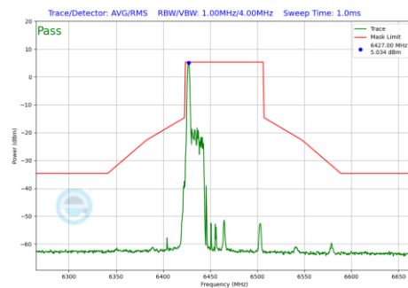
Plot 7-777 In-Band Emission Plot Antenna WF5B (80MHz BW 802.11be(RU) RU26 Index0 (UNII Band 6) - Ch.103)
