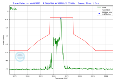
Plot 7-805 In-Band Emission Plot Antenna WF5B (40MHz BW 802.11be(RU) RU26 Index8 (UNII Band 5) - Ch.3)
