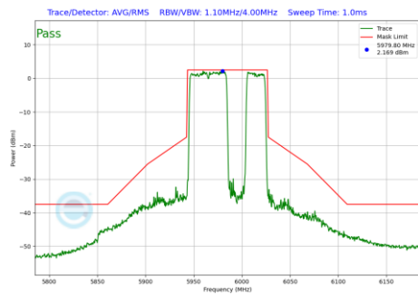
Plot 7-784 In-Band Emission Plot Antenna WF5B (80MHz BW 802.11be(RU) RU484+242 Index92 (UNII Band 5) - Ch.7)
