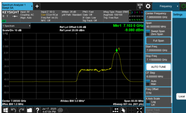
Plot 7-750 PSD SDM Diversity Antenna 4a(40MHz BW 802.11be(RU) RU26 Index17 - Ch.227)
