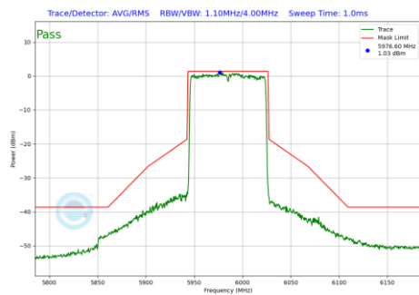
Plot 7-794 In-Band Emission Plot Antenna WF5B (80MHz BW 802.11be(RU) RU996 Index67 (UNII Band 5) - Ch.7)
