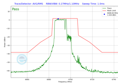
Plot 7-866 In-Band Emission Plot Antenna 4a(20MHz BW 802.11be(RU) RU106+26 Index82 (UNII Band 7) - Ch.149)
