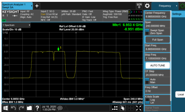
Plot 7-759 PSD SDM Diversity Antenna 4a(160MHz BW 802.11be(RU) RU996+484+242 Index99 - Ch.207)
