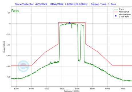
Plot 7-791 In-Band Emission Plot Antenna WF5B (160MHz BW 802.11be(RU) RU996+484+242 Index98 (UNII Band 7) - Ch.143)
