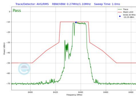
Plot 7-823 In-Band Emission Plot Antenna WF5B (20MHz BW 802.11be(RU) RU106+26 Index83 (UNII Band 6) - Ch.97)
