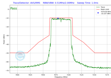
Plot 7-845 In-Band Emission Plot Antenna WF5B (40MHz BW 802.11be(RU) RU484 Index65 (UNII Band 8) - Ch.227)
