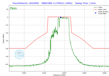
Plot 7-786 In-Band Emission Plot Antenna WF5B (20MHz BW 802.11be(RU) RU106+26 Index83 (UNII Band 6) - Ch.97)
