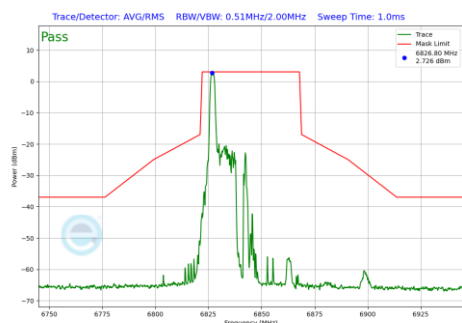
Plot 7-780 In-Band Emission Plot Antenna WF5B (40MHz BW 802.11be(RU) RU26 Index0 (UNII Band 7) - Ch.179)
