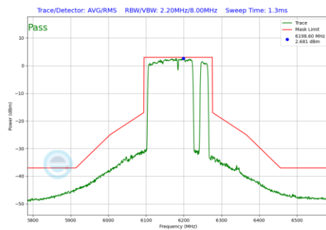
Plot 7-862 In-Band Emission Plot Antenna 4a(160MHz BW 802.11be(RU) RU996+484+242 Index98 (UNII Band 5) - Ch.47)
