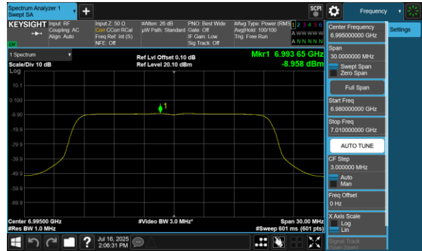
Plot 7-767 PSD SDM Diversity Antenna 2a (20MHz BW 802.11be(RU) RU242 Index61 - Ch.209)
