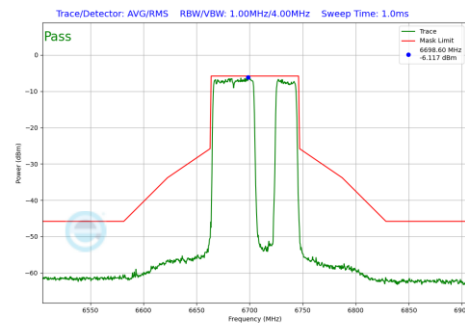
Plot 7-827 In-Band Emission Plot Antenna WF5B (80MHz BW 802.11be(RU) RU484+242 Index92 (UNII Band 7) - Ch.151)
