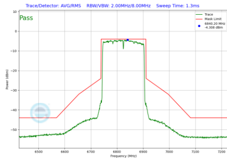
Plot 7-843 In-Band Emission Plot Antenna WF5B (160MHz BW 802.11be(RU) RU996X2 Index68 (UNII Band 7) - Ch.175)
