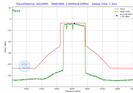
Plot 7-825 In-Band Emission Plot Antenna WF5B (160MHz BW 802.11be(RU) RU996+484+242 Index96 (UNII Band 6) - Ch.111)
