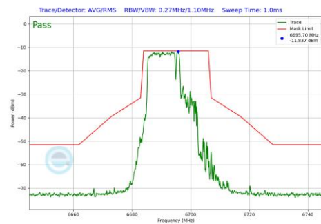
Plot 7-826 In-Band Emission Plot Antenna WF5B (20MHz BW 802.11be(RU) RU106+26 Index82 (UNII Band 7) - Ch.149)
