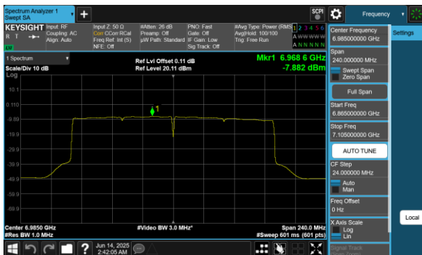
Plot 7-766 PSD SDM Diversity Antenna 4a(160MHz BW 802.11be(RU) RU996X2 Index68 - Ch.207)
