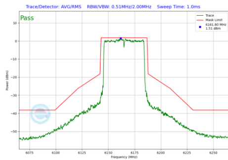
Plot 7-793 In-Band Emission Plot Antenna WF5B (40MHz BW 802.11be(RU) RU484 Index65 (UNII Band 5) - Ch.43)
