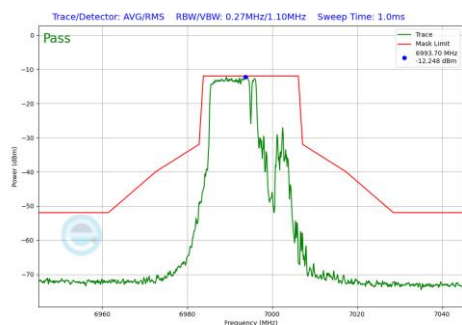
Plot 7-829 In-Band Emission Plot Antenna WF5B (20MHz BW 802.11be(RU) RU106+26 Index82 (UNII Band 8) - Ch.209)
