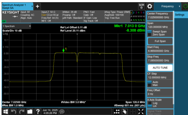
Plot 7-758 PSD SDM Diversity Antenna 4a(80MHz BW 802.11be(RU) RU484+242 Index90 - Ch.215)
