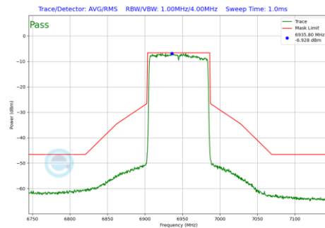
Plot 7-846 In-Band Emission Plot Antenna WF5B (80MHz BW 802.11be(RU) RU996 Index67 (UNII Band 8) - Ch.199)
