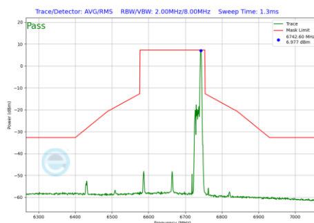
Plot 7-782 In-Band Emission Plot Antenna WF5B (160MHz BW 802.11be(RU) RU26 Index36 (UNII Band 7) - Ch.143)
