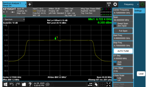
Plot 7-746 PSD SDM Diversity Antenna 2a (40MHz BW 802.11be(RU) RU484 Index65 - Ch.155)
