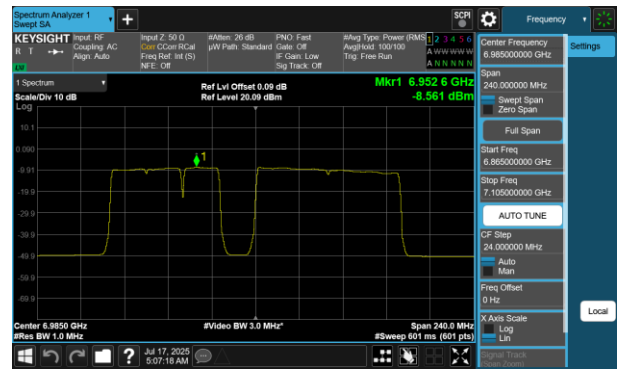
Plot 7-762 PSD SDM Diversity Antenna 2a (160MHz BW 802.11be(RU) RU996+484+242 Index99 - Ch.207)
