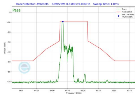
Plot 7-809 In-Band Emission Plot Antenna WF5B (40MHz BW 802.11be(RU) RU26 Index0 (UNII Band 6) - Ch.107)
