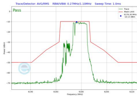
Plot 7-820 In-Band Emission Plot Antenna WF5B (20MHz BW 802.11be(RU) RU106+26 Index83 (UNII Band 5) - Ch.45)
