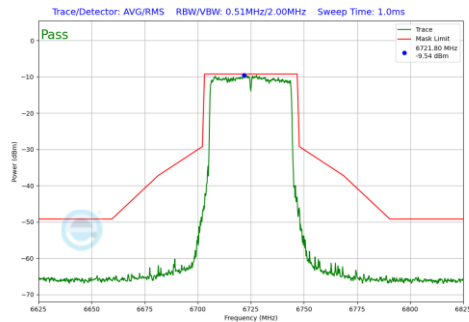
Plot 7-841 In-Band Emission Plot Antenna WF5B (40MHz BW 802.11be(RU) RU484 Index65 (UNII Band 7) - Ch.155)
