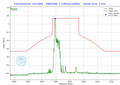
Plot 7-850 In-Band Emission Plot Antenna 4a(80MHz BW 802.11be(RU) RU26 Index0 (UNII Band 5) - Ch.7)
