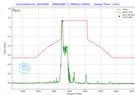
Plot 7-854 In-Band Emission Plot Antenna 4a(80MHz BW 802.11be(RU) RU26 Index0 (UNII Band 6) - Ch.103)
