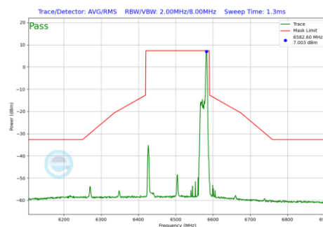
Plot 7-932 In-Band Emission Plot Antenna 2a (160MHz BW 802.11be(RU) RU26 Index36 (UNII Band 6) - Ch.111)
