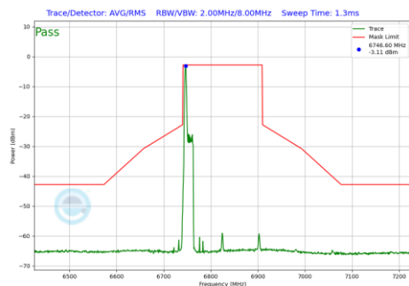
Plot 7-892 In-Band Emission Plot Antenna 4a(160MHz BW 802.11be(RU) RU26 Index0 (UNII Band 7) - Ch.175)
