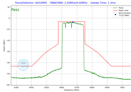
Plot 7-982 In-Band Emission Plot Antenna 2a (160MHz BW 802.11be(RU) RU996+484+242 Index96 (UNII Band 7) - Ch.143)
