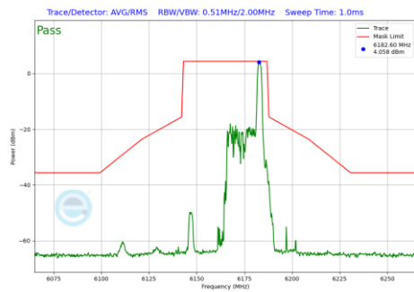
Plot 7-1002 In-Band Emission Plot CDD Primary Antenna WF5B (40MHz BW 802.11be(RU) RU26 Index17 (UNII Band 5) - Ch.43)
