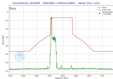
Plot 7-968 In-Band Emission Plot Antenna 2a (80MHz BW 802.11be(RU) RU26 Index0 (UNII Band 7) - Ch.119)
