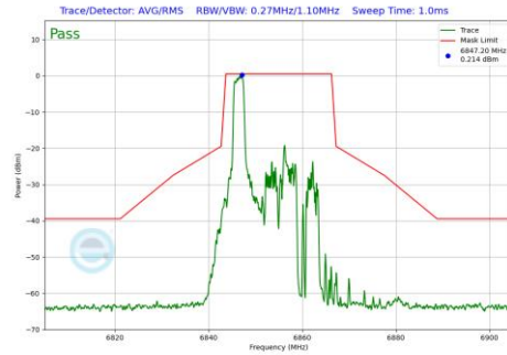
Plot 7-1021 In-Band Emission Plot CDD Primary Antenna 4a(20MHz BW 802.11be(RU) RU26 Index0 (UNII Band 7) - Ch.181)
