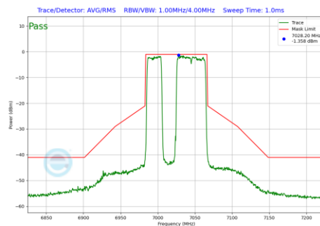
Plot 7-907 In-Band Emission Plot Antenna 4a(80MHz BW 802.11be(RU) RU484+242 Index91 (UNII Band 8) - Ch.215)
