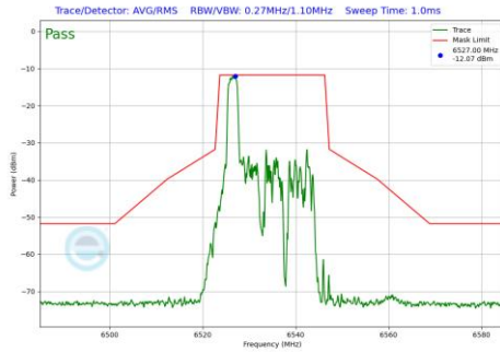
Plot 7-966 In-Band Emission Plot Antenna 2a (20MHz BW 802.11be(RU) RU26 Index0 (UNII Band 7) - Ch.117)
