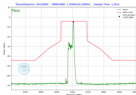
Plot 7-891 In-Band Emission Plot Antenna 4a(80MHz BW 802.11be(RU) RU26 Index17 (UNII Band 7) - Ch.151)
