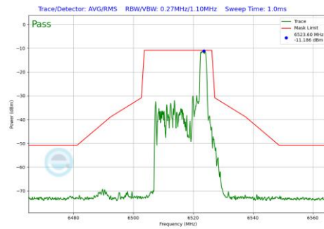
Plot 7-962 In-Band Emission Plot Antenna 2a (20MHz BW 802.11be(RU) RU26 Index8 (UNII Band 6) - Ch.113)
