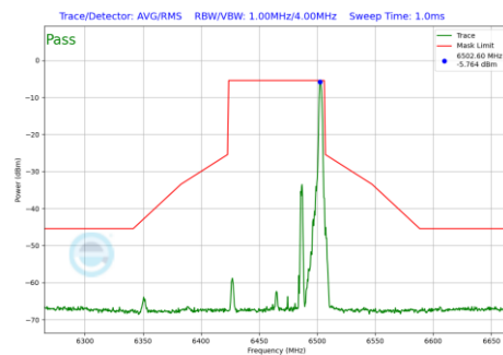
Plot 7-964 In-Band Emission Plot Antenna 2a (80MHz BW 802.11be(RU) RU26 Index36 (UNII Band 6) - Ch.103)
