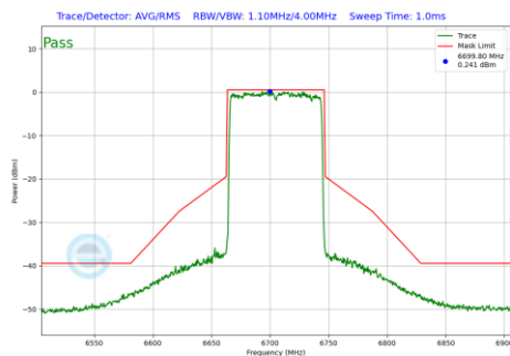
Plot 7-956 In-Band Emission Plot Antenna 2a (80MHz BW 802.11be(RU) RU996 Index67 (UNII Band 7) - Ch.151)
