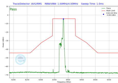
Plot 7-960 In-Band Emission Plot Antenna 2a (80MHz BW 802.11be(RU) RU26 Index17 (UNII Band 5) - Ch.87)
