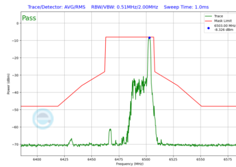
Plot 7-963 In-Band Emission Plot Antenna 2a (40MHz BW 802.11be(RU) RU26 Index17 (UNII Band 6) - Ch.107)
