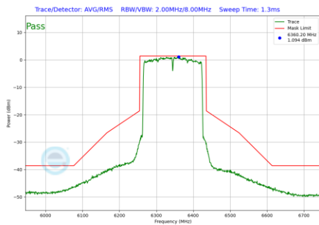
Plot 7-912 In-Band Emission Plot Antenna 4a(160MHz BW 802.11be(RU) RU996X2 Index68 (UNII Band 5) - Ch.79)
