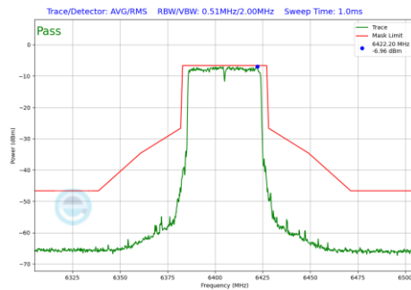
Plot 7-986 In-Band Emission Plot Antenna 2a (40MHz BW 802.11be(RU) RU484 Index65 (UNII Band 5) - Ch.91)
