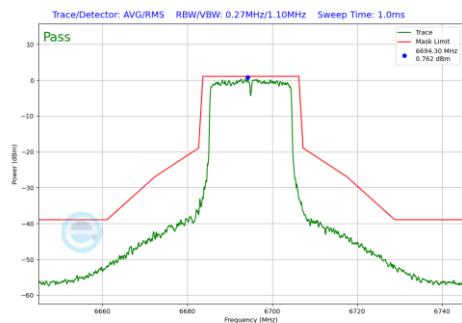
Plot 7-954 In-Band Emission Plot Antenna 2a (20MHz BW 802.11be(RU) RU242 Index61 (UNII Band 7) - Ch.149)
