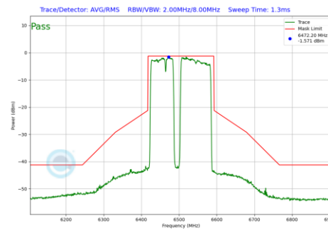
Plot 7-902 In-Band Emission Plot Antenna 4a(160MHz BW 802.11be(RU) RU996+484+242 Index99 (UNII Band 6) - Ch.111)
