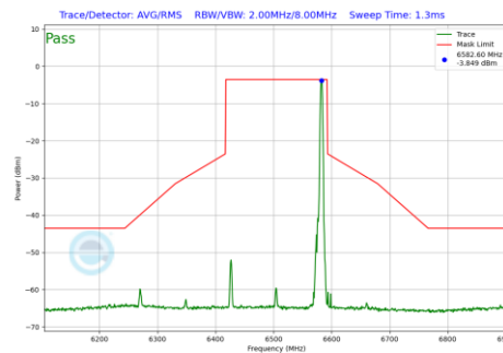
Plot 7-888 In-Band Emission Plot Antenna 4a(160MHz BW 802.11be(RU) RU26 Index36 (UNII Band 6) - Ch.111)
