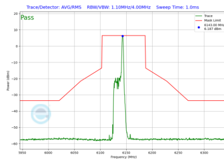
Plot 7-1015 In-Band Emission Plot CDD Primary Antenna 4a(80MHz BW 802.11be(RU) RU26 Index17 (UNII Band 5) - Ch.39)
