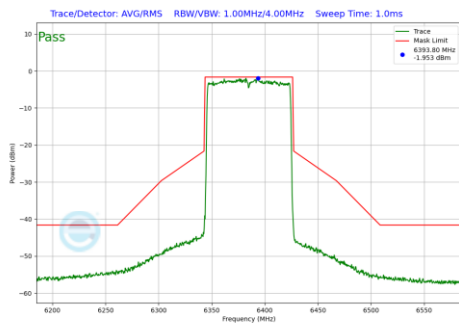
Plot 7-911 In-Band Emission Plot Antenna 4a(80MHz BW 802.11be(RU) RU996 Index67 (UNII Band 5) - Ch.87)
