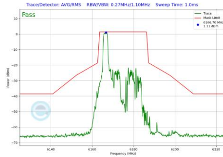
Plot 7-1013 In-Band Emission Plot CDD Primary Antenna 4a(20MHz BW 802.11be(RU) RU26 Index0 (UNII Band 5) - Ch.45)
