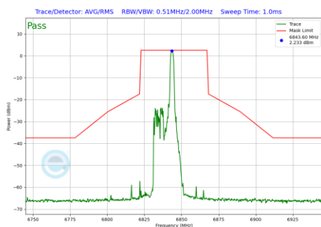
Plot 7-934 In-Band Emission Plot Antenna 2a (40MHz BW 802.11be(RU) RU26 Index8 (UNII Band 7) - Ch.179)
