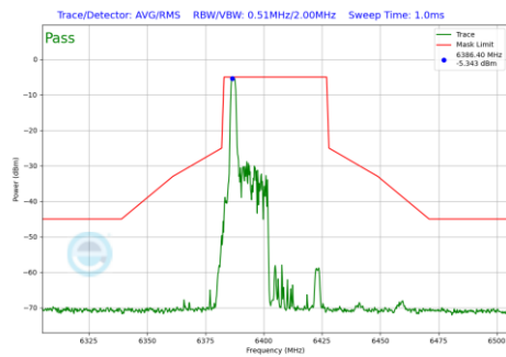
Plot 7-882 In-Band Emission Plot Antenna 4a(40MHz BW 802.11be(RU) RU26 Index0 (UNII Band 5) - Ch.91)
