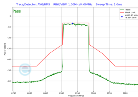
Plot 7-999 In-Band Emission Plot Antenna 2a (80MHz BW 802.11be(RU) RU996 Index67 (UNII Band 8) - Ch.199)
