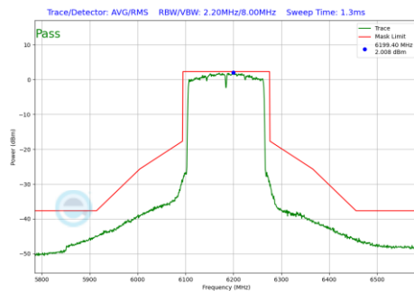
Plot 7-872 In-Band Emission Plot Antenna 4a(160MHz BW 802.11be(RU) RU996X2 Index68 (UNII Band 5) - Ch.47)
