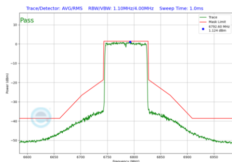
Plot 7-879 In-Band Emission Plot Antenna 4a(80MHz BW 802.11be(RU) RU996 Index67 (UNII Band 7) - Ch.167)
