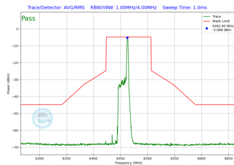
Plot 7-887 In-Band Emission Plot Antenna 4a(80MHz BW 802.11be(RU) RU26 Index17 (UNII Band 6) - Ch.103)
