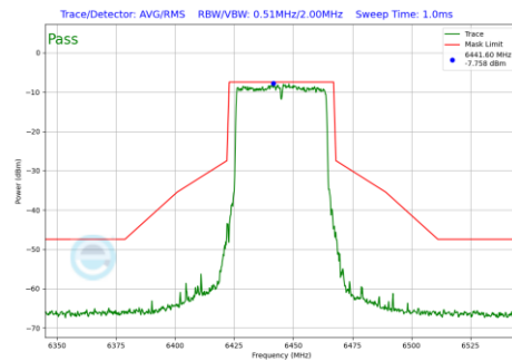
Plot 7-990 In-Band Emission Plot Antenna 2a (40MHz BW 802.11be(RU) RU484 Index65 (UNII Band 6) - Ch.99)
