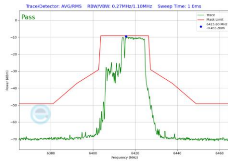
Plot 7-974 In-Band Emission Plot Antenna 2a (20MHz BW 802.11be(RU) RU106+26 Index83 (UNII Band 5) - Ch.93)
