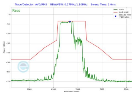
Plot 7-906 In-Band Emission Plot Antenna 4a(20MHz BW 802.11be(RU) RU106+26 Index82 (UNII Band 8) - Ch.209)
