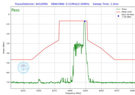
Plot 7-959 In-Band Emission Plot Antenna 2a (40MHz BW 802.11be(RU) RU26 Index17 (UNII Band 5) - Ch.91)
