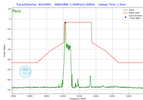
Plot 7-883 In-Band Emission Plot Antenna 4a(80MHz BW 802.11be(RU) RU26 Index0 (UNII Band 5) - Ch.39)
