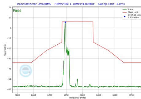
Plot 7-1023 In-Band Emission Plot CDD Primary Antenna 4a(80MHz BW 802.11be(RU) RU26 Index0 (UNII Band 7) - Ch.167)
