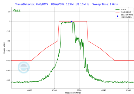
Plot 7-1028 In-Band Emission Plot CDD Primary Antenna WF5B (20MHz BW 802.11be(RU) RU106+26 Index82 (UNII Band 6) - Ch.113)
