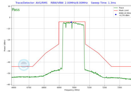
Plot 7-984 In-Band Emission Plot Antenna 2a (160MHz BW 802.11be(RU) RU996+484+242 Index96 (UNII Band 8) - Ch.207)
