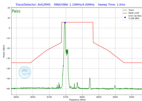
Plot 7-1011 In-Band Emission Plot CDD Primary Antenna WF5B (80MHz BW 802.11be(RU) RU26 Index0 (UNII Band 7) - Ch.167)
