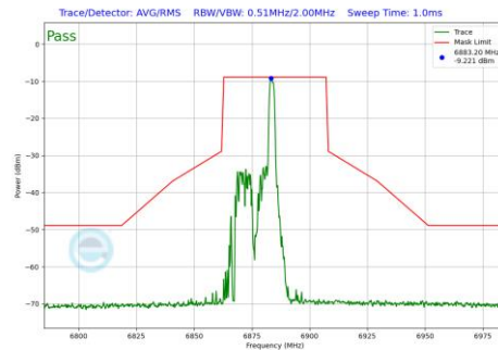
Plot 7-971 In-Band Emission Plot Antenna 2a (40MHz BW 802.11be(RU) RU26 Index8 (UNII Band 8) - Ch.187)
