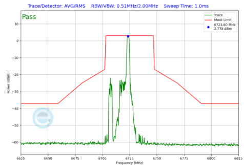
Plot 7-1022 In-Band Emission Plot CDD Primary Antenna 4a(40MHz BW 802.11be(RU) RU26 Index8 (UNII Band 7) - Ch.155)
