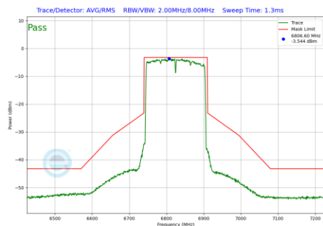
Plot 7-996 In-Band Emission Plot Antenna 2a (160MHz BW 802.11be(RU) RU996X2 Index68 (UNII Band 7) - Ch.175)
