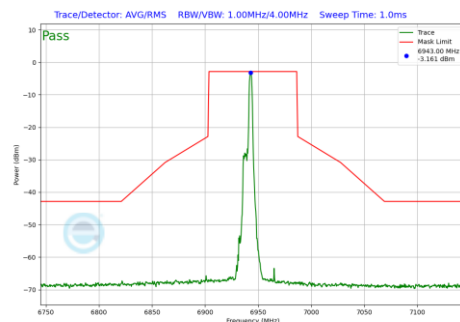
Plot 7-895 In-Band Emission Plot Antenna 4a(80MHz BW 802.11be(RU) RU26 Index17 (UNII Band 8) - Ch.199)
