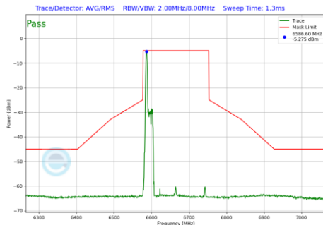
Plot 7-969 In-Band Emission Plot Antenna 2a (160MHz BW 802.11be(RU) RU26 Index0 (UNII Band 7) - Ch.143)
