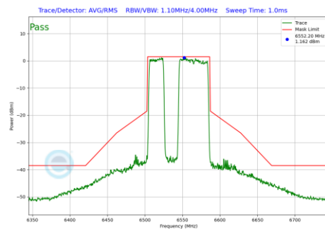
Plot 7-1032 In-Band Emission Plot CDD Primary Antenna WF5B (80MHz BW 802.11be(RU) RU484+242 Index91 (UNII Band 7) - Ch.119)
