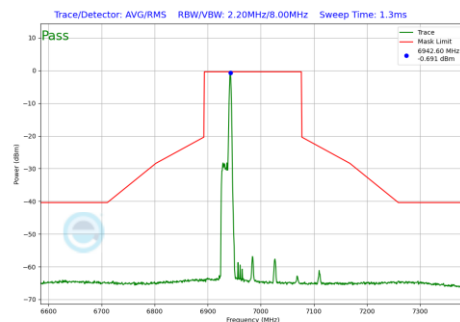
Plot 7-896 In-Band Emission Plot Antenna 4a(160MHz BW 802.11be(RU) RU26 Index17 (UNII Band 8) - Ch.207)
