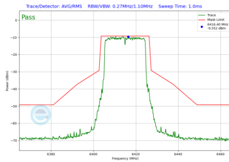
Plot 7-985 In-Band Emission Plot Antenna 2a (20MHz BW 802.11be(RU) RU242 Index61 (UNII Band 5) - Ch.93)
