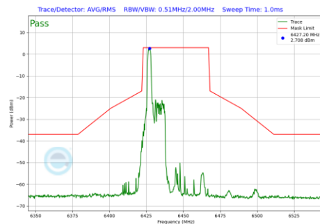
Plot 7-930 In-Band Emission Plot Antenna 2a (40MHz BW 802.11be(RU) RU26 Index0 (UNII Band 6) - Ch.99)
