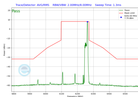
Plot 7-1004 In-Band Emission Plot CDD Primary Antenna WF5B (160MHz BW 802.11be(RU) RU26 Index36 (UNII Band 5) - Ch.47)
