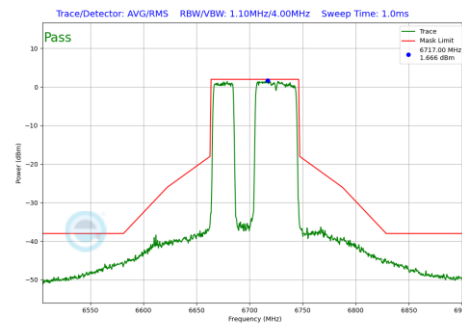
Plot 7-944 In-Band Emission Plot Antenna 2a (80MHz BW 802.11be(RU) RU484+242 Index91 (UNII Band 7) - Ch.151)
