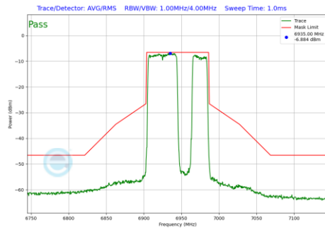
Plot 7-983 In-Band Emission Plot Antenna 2a (80MHz BW 802.11be(RU) RU484+242 Index92 (UNII Band 8) - Ch.199)
