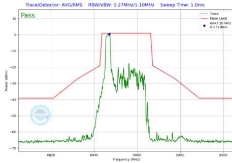
Plot 7-1009 In-Band Emission Plot CDD Primary Antenna WF5B (20MHz BW 802.11be(RU) RU26 Index0 (UNII Band 7) - Ch.181)
