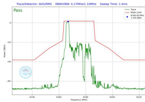
Plot 7-1001 In-Band Emission Plot CDD Primary Antenna WF5B (20MHz BW 802.11be(RU) RU26 Index0 (UNII Band 5) - Ch.45)
