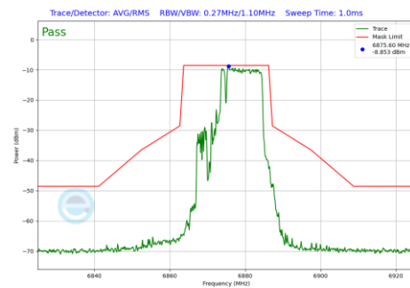
Plot 7-903 In-Band Emission Plot Antenna 4a(20MHz BW 802.11be(RU) RU106+26 Index83 (UNII Band 7) - Ch.185)
