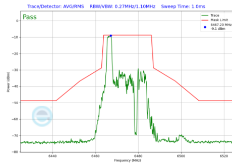
Plot 7-885 In-Band Emission Plot Antenna 4a(20MHz BW 802.11be(RU) RU26 Index0 (UNII Band 6) - Ch.105)
