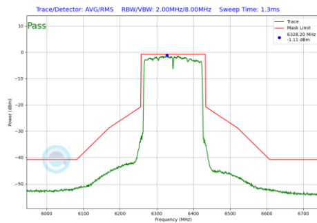
Plot 7-988 In-Band Emission Plot Antenna 2a (160MHz BW 802.11be(RU) RU996X2 Index68 (UNII Band 5) - Ch.79)
