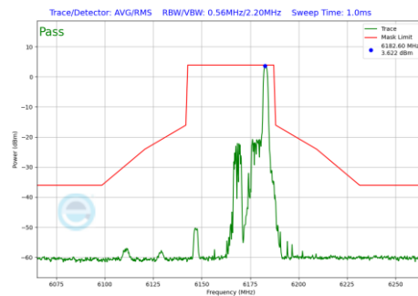
Plot 7-1014 In-Band Emission Plot CDD Primary Antenna 4a(40MHz BW 802.11be(RU) RU26 Index17 (UNII Band 5) - Ch.43)
