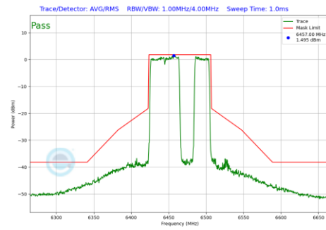
Plot 7-941 In-Band Emission Plot Antenna 2a (80MHz BW 802.11be(RU) RU484+242 Index92 (UNII Band 6) - Ch.103)
