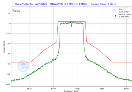
Plot 7-877 In-Band Emission Plot Antenna 4a(20MHz BW 802.11be(RU) RU242 Index61 (UNII Band 7) - Ch.181)
