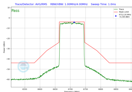
Plot 7-919 In-Band Emission Plot Antenna 4a(80MHz BW 802.11be(RU) RU996 Index67 (UNII Band 7) - Ch.151)
