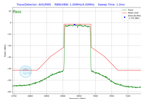
Plot 7-923 In-Band Emission Plot Antenna 4a(80MHz BW 802.11be(RU) RU996 Index67 (UNII Band 8) - Ch.199)
