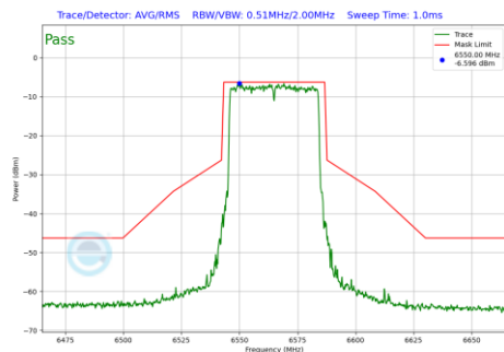
Plot 7-918 In-Band Emission Plot Antenna 4a(40MHz BW 802.11be(RU) RU484 Index65 (UNII Band 7) - Ch.123)
