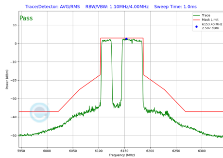
Plot 7-938 In-Band Emission Plot Antenna 2a (80MHz BW 802.11be(RU) RU484+242 Index91 (UNII Band 5) - Ch.39)
