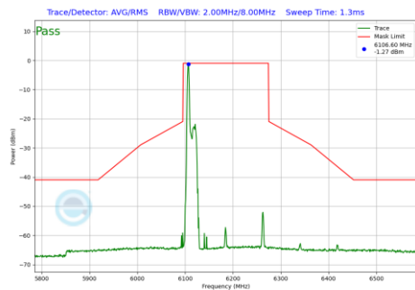
Plot 7-884 In-Band Emission Plot Antenna 4a(160MHz BW 802.11be(RU) RU26 Index0 (UNII Band 5) - Ch.47)
