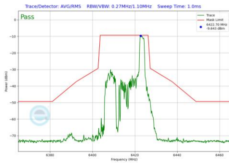
Plot 7-958 In-Band Emission Plot Antenna 2a (20MHz BW 802.11be(RU) RU26 Index8 (UNII Band 5) - Ch.93)
