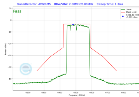
Plot 7-979 In-Band Emission Plot Antenna 2a (160MHz BW 802.11be(RU) RU996+484+242 Index96 (UNII Band 6) - Ch.111)
