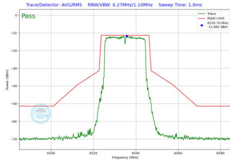
Plot 7-993 In-Band Emission Plot Antenna 2a (20MHz BW 802.11be(RU) RU242 Index61 (UNII Band 7) - Ch.117)
