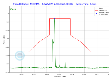
Plot 7-965 In-Band Emission Plot Antenna 2a (160MHz BW 802.11be(RU) RU26 Index17 (UNII Band 6) - Ch.111)
