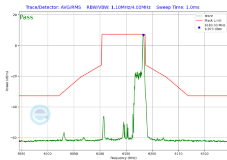
Plot 7-927 In-Band Emission Plot Antenna 2a (80MHz BW 802.11be(RU) RU26 Index36 (UNII Band 5) - Ch.39)
