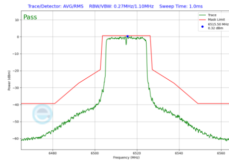
Plot 7-950 In-Band Emission Plot Antenna 2a (20MHz BW 802.11be(RU) RU242 Index61 (UNII Band 6) - Ch.113)
