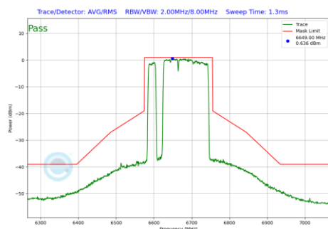
Plot 7-945 In-Band Emission Plot Antenna 2a (160MHz BW 802.11be(RU) RU996+484+242 Index97 (UNII Band 7) - Ch.143)
