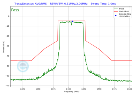
Plot 7-910 In-Band Emission Plot Antenna 4a(40MHz BW 802.11be(RU) RU484 Index65 (UNII Band 5) - Ch.91)
