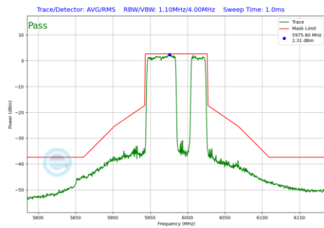
Plot 7-1026 In-Band Emission Plot CDD Primary Antenna WF5B (80MHz BW 802.11be(RU) RU484+242 Index92 (UNII Band 5) - Ch.7)
