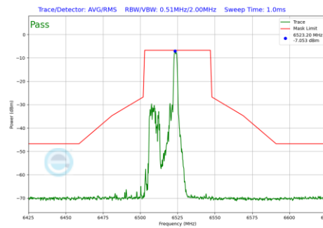
Plot 7-886 In-Band Emission Plot Antenna 4a(40MHz BW 802.11be(RU) RU26 Index8 (UNII Band 6) - Ch.115)
