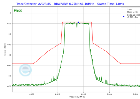
Plot 7-913 In-Band Emission Plot Antenna 4a(20MHz BW 802.11be(RU) RU242 Index61 (UNII Band 6) - Ch.97)
