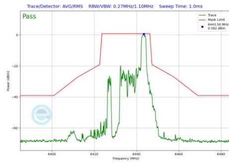
Plot 7-929 In-Band Emission Plot Antenna 2a (20MHz BW 802.11be(RU) RU26 Index8 (UNII Band 6) - Ch.97)
