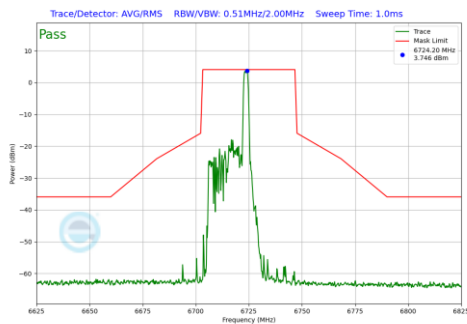
Plot 7-1010 In-Band Emission Plot CDD Primary Antenna WF5B (40MHz BW 802.11be(RU) RU26 Index8 (UNII Band 7) - Ch.155)
