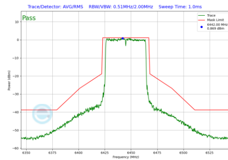
Plot 7-874 In-Band Emission Plot Antenna 4a(40MHz BW 802.11be(RU) RU484 Index65 (UNII Band 6) - Ch.99)
