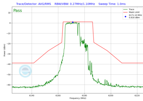
Plot 7-1025 In-Band Emission Plot CDD Primary Antenna WF5B (20MHz BW 802.11be(RU) RU106+26 Index82 (UNII Band 5) - Ch.45)
