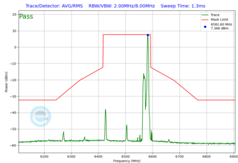
Plot 7-1020 In-Band Emission Plot CDD Primary Antenna 4a(160MHz BW 802.11be(RU) RU26 Index36 (UNII Band 6) - Ch.111)
