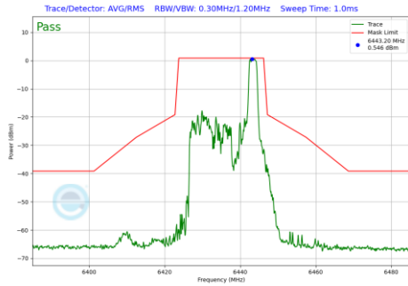
Plot 7-1017 In-Band Emission Plot CDD Primary Antenna 4a(20MHz BW 802.11be(RU) RU26 Index8 (UNII Band 6) - Ch.97)
