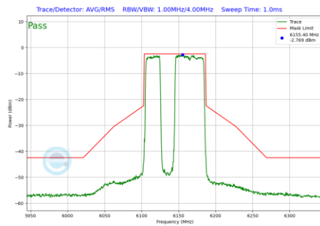
Plot 7-898 In-Band Emission Plot Antenna 4a(80MHz BW 802.11be(RU) RU484+242 Index91 (UNII Band 5) - Ch.39)
