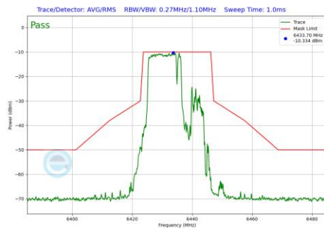
Plot 7-977 In-Band Emission Plot Antenna 2a (20MHz BW 802.11be(RU) RU106+26 Index82 (UNII Band 6) - Ch.97)
