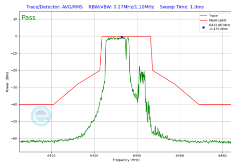
Plot 7-940 In-Band Emission Plot Antenna 2a (20MHz BW 802.11be(RU) RU106+26 Index82 (UNII Band 6) - Ch.97)
