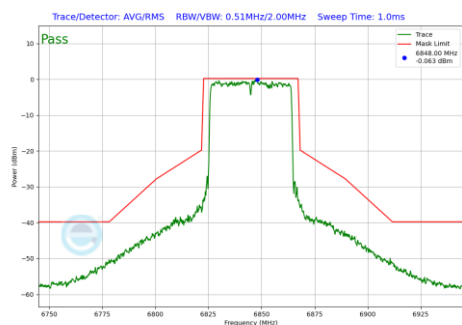
Plot 7-955 In-Band Emission Plot Antenna 2a (40MHz BW 802.11be(RU) RU484 Index65 (UNII Band 7) - Ch.179)
