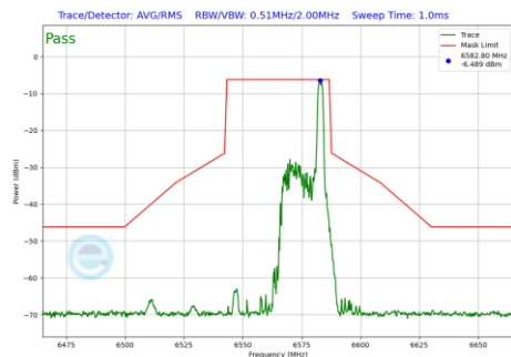
Plot 7-890 In-Band Emission Plot Antenna 4a(40MHz BW 802.11be(RU) RU26 Index17 (UNII Band 7) - Ch.123)
