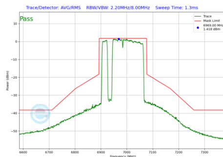
Plot 7-908 In-Band Emission Plot Antenna 4a(160MHz BW 802.11be(RU) RU996+484+242 Index97 (UNII Band 8) - Ch.207)
