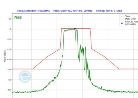
Plot 7-1031 In-Band Emission Plot CDD Primary Antenna WF5B (20MHz BW 802.11be(RU) RU106+26 Index82 (UNII Band 7) - Ch.181)
