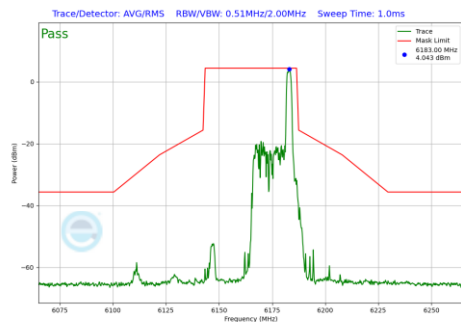
Plot 7-926 In-Band Emission Plot Antenna 2a (40MHz BW 802.11be(RU) RU26 Index17 (UNII Band 5) - Ch.43)
