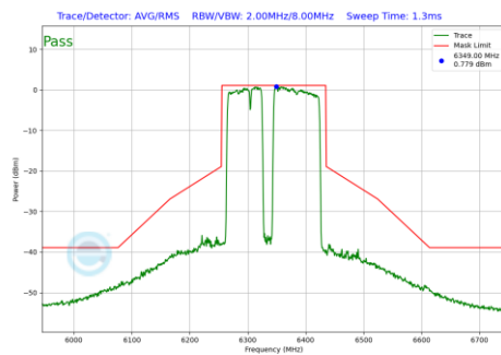
Plot 7-899 In-Band Emission Plot Antenna 4a(160MHz BW 802.11be(RU) RU996+484+242 Index99 (UNII Band 5) - Ch.79)
