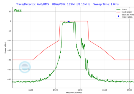
Plot 7-943 In-Band Emission Plot Antenna 2a (20MHz BW 802.11be(RU) RU106+26 Index82 (UNII Band 7) - Ch.117)
