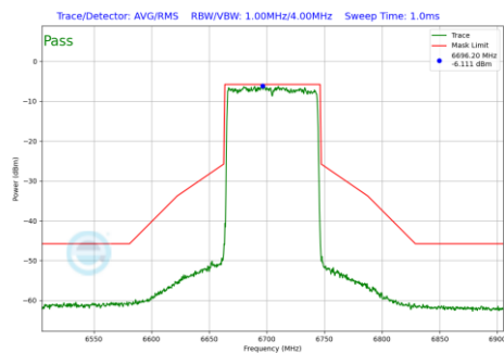
Plot 7-995 In-Band Emission Plot Antenna 2a (80MHz BW 802.11be(RU) RU996 Index67 (UNII Band 7) - Ch.151)
