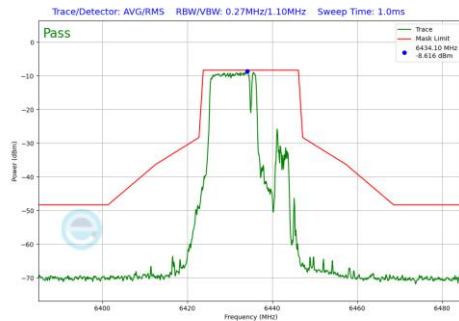
Plot 7-900 In-Band Emission Plot Antenna 4a(20MHz BW 802.11be(RU) RU106+26 Index82 (UNII Band 6) - Ch.97)
