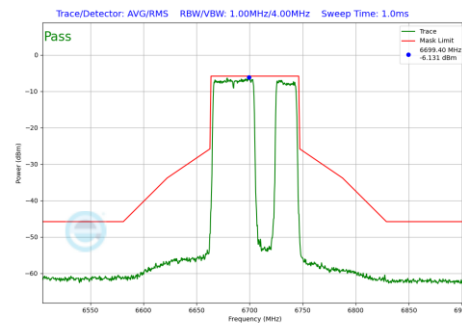
Plot 7-981 In-Band Emission Plot Antenna 2a (80MHz BW 802.11be(RU) RU484+242 Index92 (UNII Band 7) - Ch.151)
