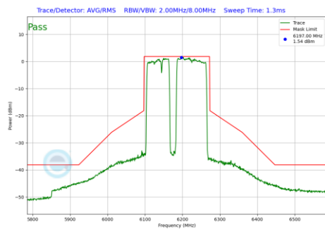
Plot 7-1027 In-Band Emission Plot CDD Primary Antenna WF5B (160MHz BW 802.11be(RU) RU996+484+242 Index99 (UNII Band 5) - Ch.47)
