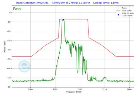
Plot 7-893 In-Band Emission Plot Antenna 4a(20MHz BW 802.11be(RU) RU26 Index0 (UNII Band 8) - Ch.229)
