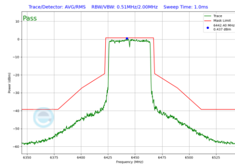
Plot 7-951 In-Band Emission Plot Antenna 2a (40MHz BW 802.11be(RU) RU484 Index65 (UNII Band 6) - Ch.99)
