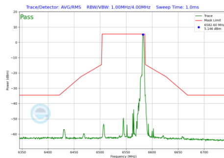
Plot 7-935 In-Band Emission Plot Antenna 2a (80MHz BW 802.11be(RU) RU26 Index36 (UNII Band 7) - Ch.119)
