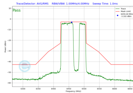
Plot 7-901 In-Band Emission Plot Antenna 4a(80MHz BW 802.11be(RU) RU484+242 Index92 (UNII Band 6) - Ch.103)
