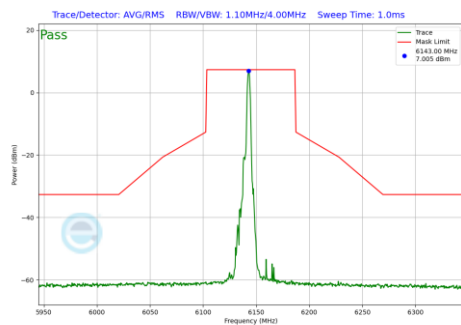
Plot 7-1003 In-Band Emission Plot CDD Primary Antenna WF5B (80MHz BW 802.11be(RU) RU26 Index17 (UNII Band 5) - Ch.39)
