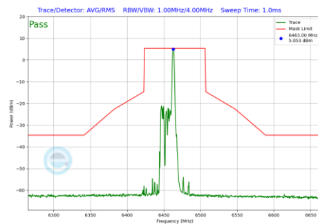
Plot 7-931 In-Band Emission Plot Antenna 2a (80MHz BW 802.11be(RU) RU26 Index17 (UNII Band 6) - Ch.103)
