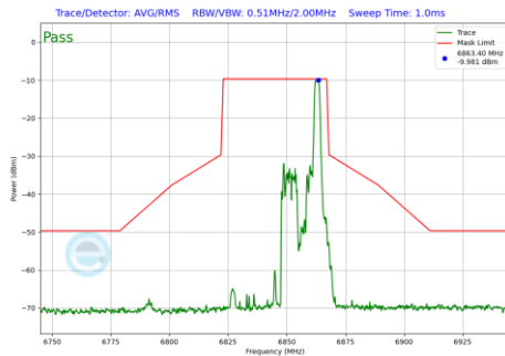
Plot 7-967 In-Band Emission Plot Antenna 2a (40MHz BW 802.11be(RU) RU26 Index17 (UNII Band 7) - Ch.179)
