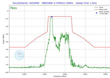
Plot 7-881 In-Band Emission Plot Antenna 4a(20MHz BW 802.11be(RU) RU26 Index0 (UNII Band 5) - Ch.93)
