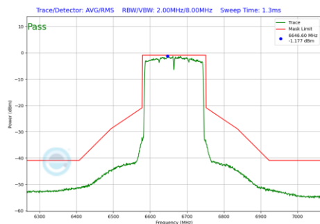
Plot 7-920 In-Band Emission Plot Antenna 4a(160MHz BW 802.11be(RU) RU996X2 Index68 (UNII Band 7) - Ch.143)
