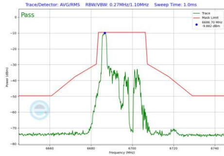
Plot 7-889 In-Band Emission Plot Antenna 4a(20MHz BW 802.11be(RU) RU26 Index0 (UNII Band 7) - Ch.149)
