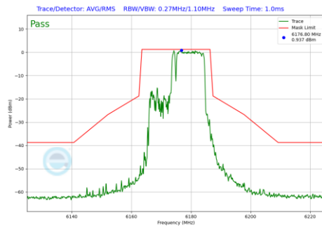
Plot 7-937 In-Band Emission Plot Antenna 2a (20MHz BW 802.11be(RU) RU106+26 Index83 (UNII Band 5) - Ch.45)
