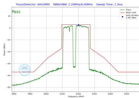
Plot 7-939 In-Band Emission Plot Antenna 2a (160MHz BW 802.11be(RU) RU996+484+242 Index99 (UNII Band 5) - Ch.47)
