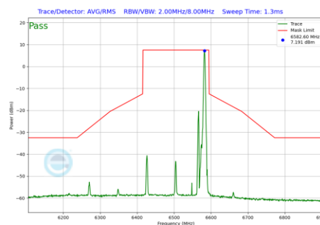
Plot 7-1008 In-Band Emission Plot CDD Primary Antenna WF5B (160MHz BW 802.11be(RU) RU26 Index36 (UNII Band 6) - Ch.111)
