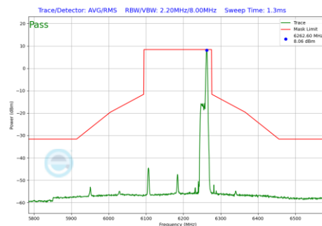
Plot 7-1016 In-Band Emission Plot CDD Primary Antenna 4a(160MHz BW 802.11be(RU) RU26 Index36 (UNII Band 5) - Ch.47)
