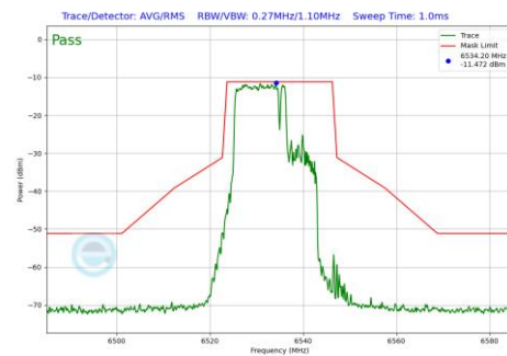
Plot 7-980 In-Band Emission Plot Antenna 2a (20MHz BW 802.11be(RU) RU106+26 Index82 (UNII Band 7) - Ch.117)
