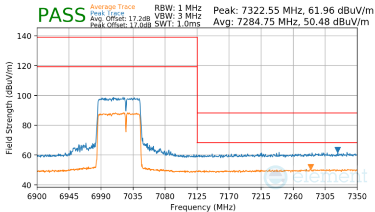
Plot 7-1001 Antenna 2a Radiated Upper Band Edge (Peak & Average – UNII Band 8) - RU484+242
