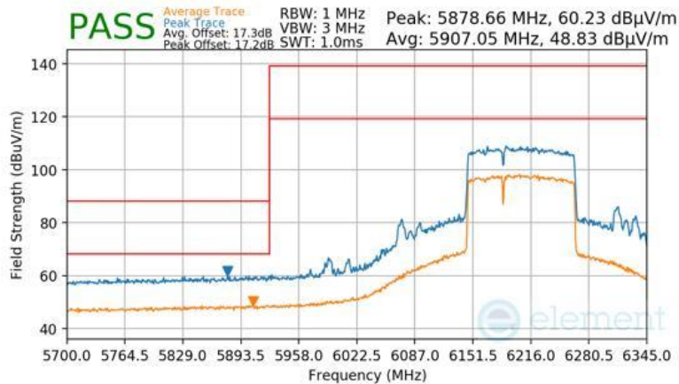
Plot 7-1008 Antenna 2a Radiated Lower Band Edge (Peak & Average – UNII Band 5) - RU996+484 (L)
