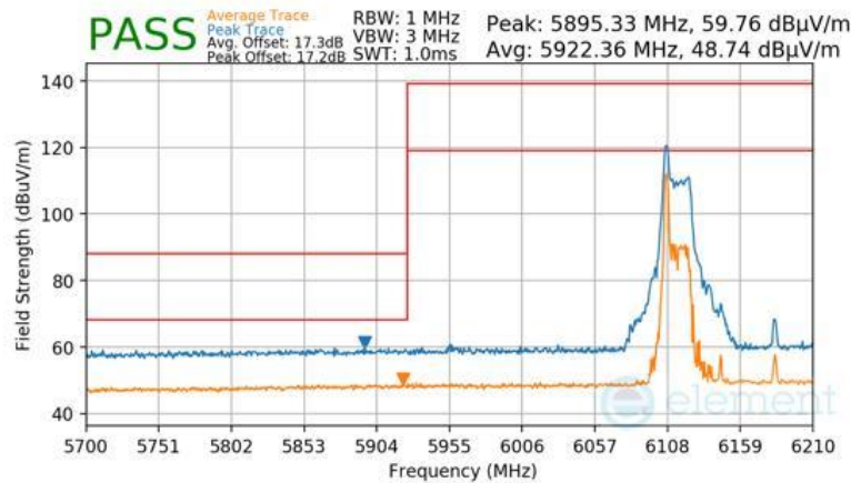
Plot 7-990 Antenna 2a Radiated Lower Band Edge (Peak & Average – UNII Band 5) - RU26
