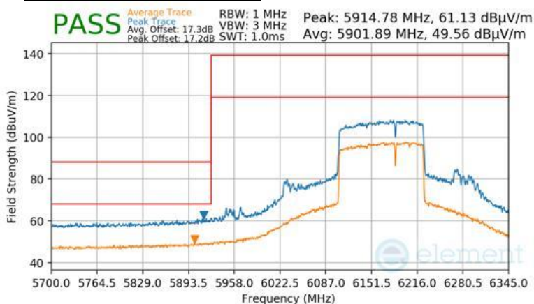
Plot 7-1011 Antenna 2a Radiated Lower Band Edge (Peak & Average – UNII Band 5) - RU996+484 (H)
