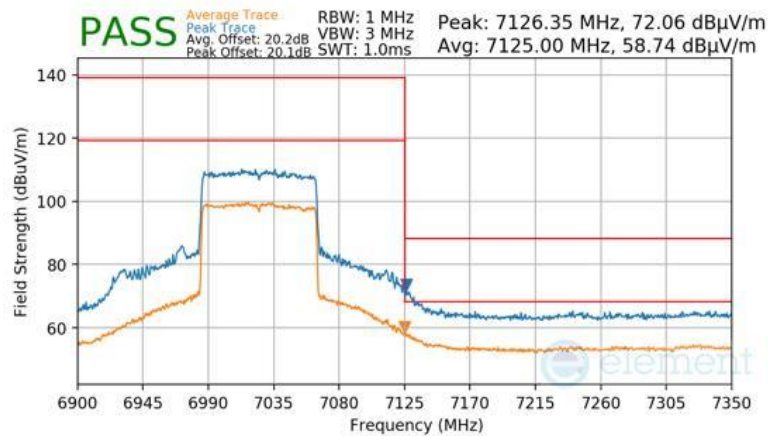
Plot 7-1003 Antenna 2a Radiated Upper Band Edge (Peak & Average – UNII Band 8) - RU996
