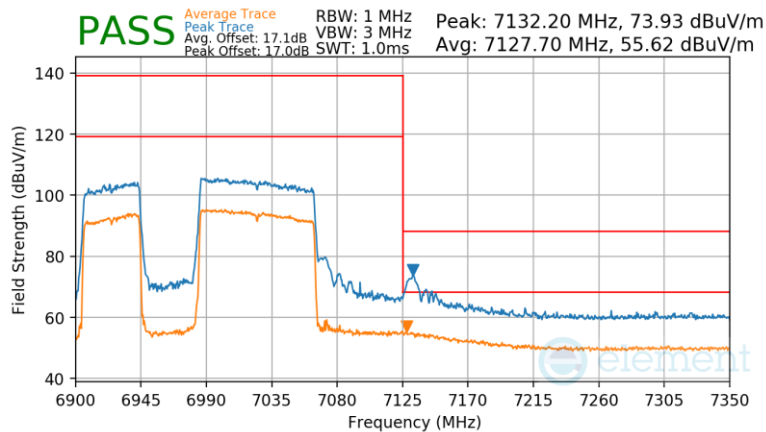
Plot 7-1015 Antenna 2a Radiated Upper Band Edge (Peak & Average – UNII Band 8) - RU996+484 (L)
