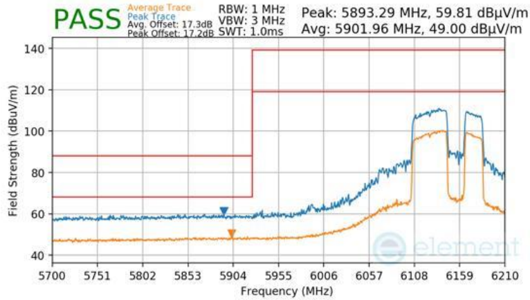
Plot 7-996 Antenna 2a Radiated Lower Band Edge (Peak & Average – UNII Band 5) - RU484+242
