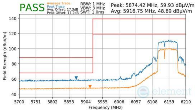
Plot 7-994 Antenna 2a Radiated Lower Band Edge (Peak & Average – UNII Band 5) - RU484+242
