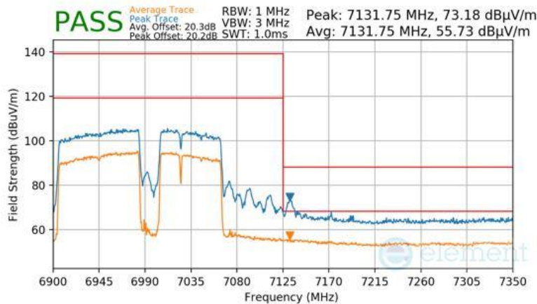
Plot 7-1025 Antenna 2a Radiated Upper Band Edge (Peak & Average – UNII Band 8) - RU996+484+242 (H)
