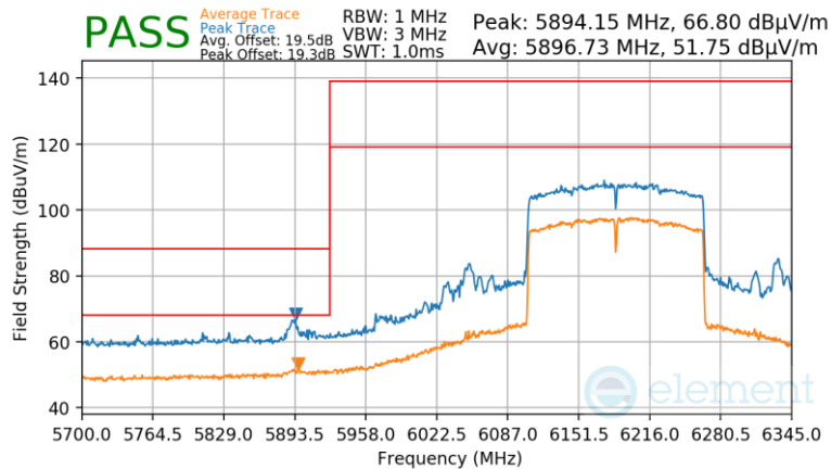
Plot 7-1032 Antenna 2a Radiated Lower Band Edge (Peak & Average – UNII Band 5) - RU996X2
