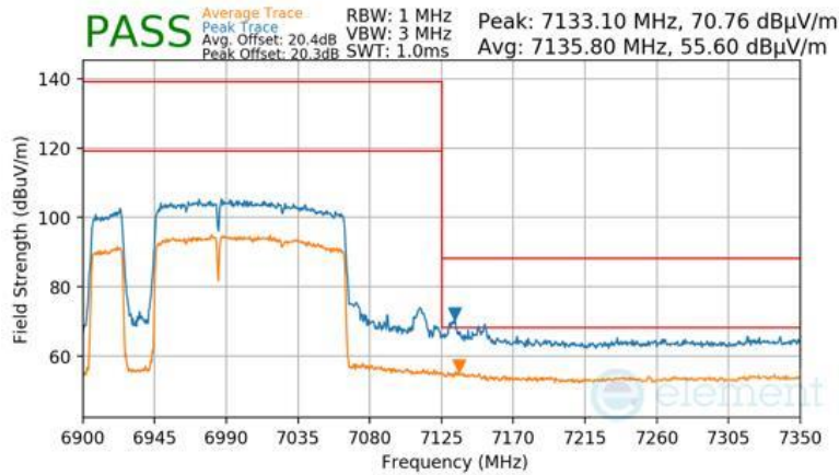
Plot 7-1026 Antenna 2a Radiated Upper Band Edge (Peak & Average – UNII Band 8) - RU996+484+242 (L)
