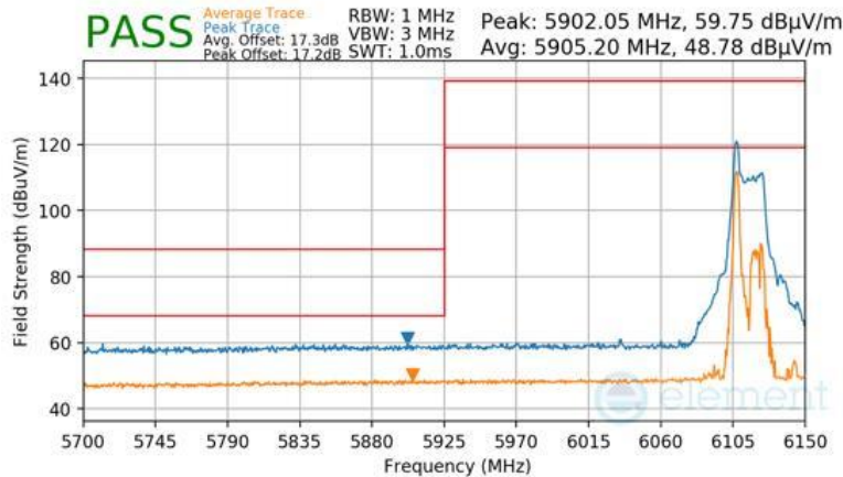
Plot 7-984 Antenna 2a Radiated Lower Band Edge (Peak & Average – UNII Band 5) - RU26
