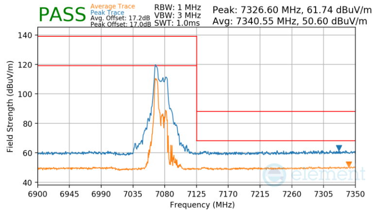
Plot 7-1048 SDM Primary Radiated Upper Band Edge (Peak & Average – UNII Band 8) – RU52
