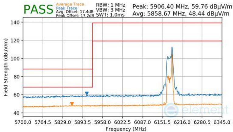
Plot 7-1005 Antenna 2a Radiated Lower Band Edge (Peak & Average – UNII Band 5) - RU26
