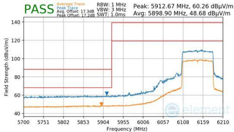
Plot 7-1002 Antenna 2a Radiated Lower Band Edge (Peak & Average – UNII Band 5) - RU996
