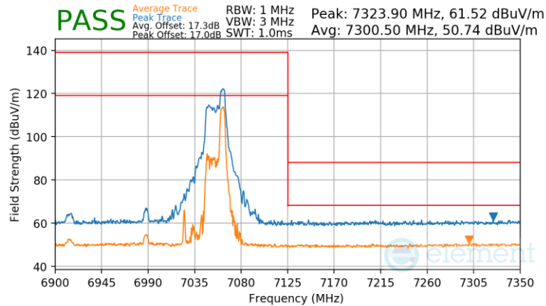
Plot 7-1055 SDM Primary Radiated Upper Band Edge (Peak & Average – UNII Band 8) – RU52
