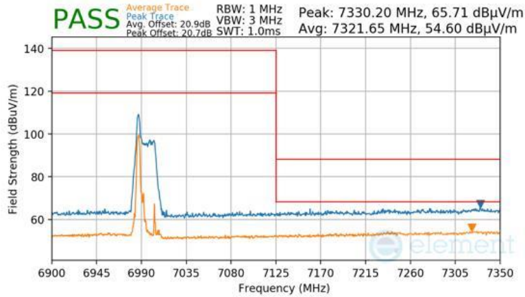
Plot 7-1006 Antenna 2a Radiated Upper Band Edge (Peak & Average – UNII Band 8) - RU26
