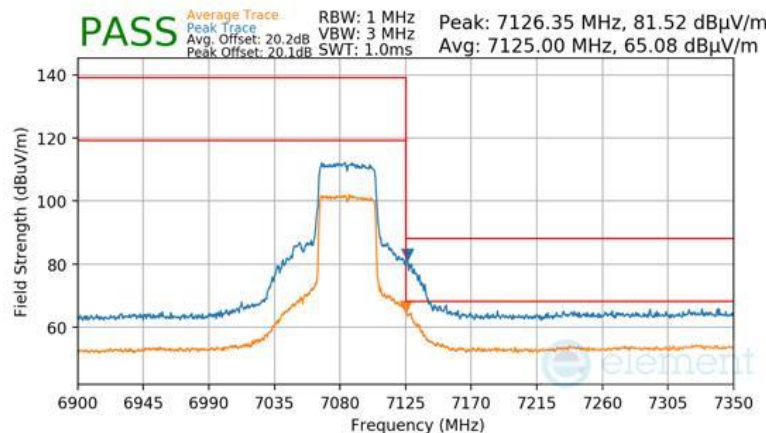
Plot 7-989 Antenna 2a Radiated Upper Band Edge (Peak & Average – UNII Band 8) - RU484
