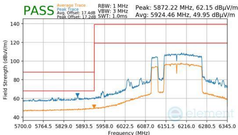
Plot 7-1018 Antenna 2a Radiated Lower Band Edge (Peak & Average – UNII Band 5) - RU996+484+242 (L)
