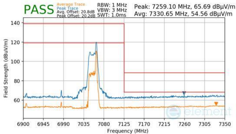
Plot 7-1007 Antenna 2a Radiated Upper Band Edge (Peak & Average – UNII Band 8) - RU26
