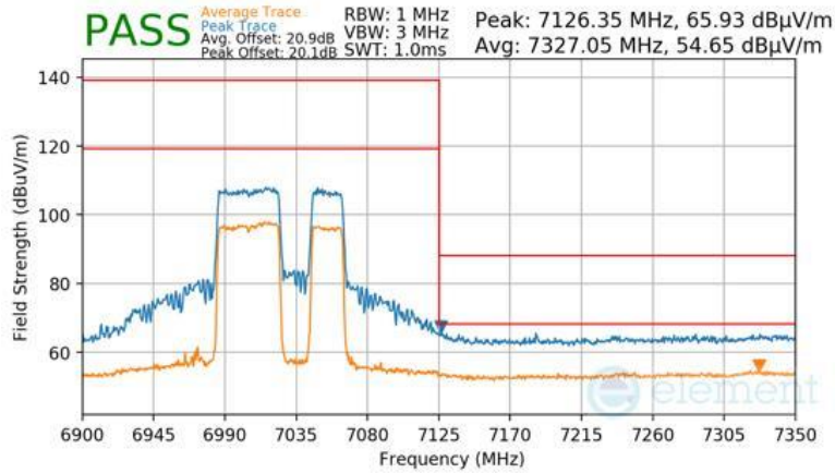
Plot 7-1000 Antenna 2a Radiated Upper Band Edge (Peak & Average – UNII Band 8) - RU484+242
