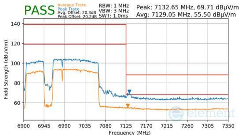
Plot 7-1028 Antenna 2a Radiated Upper Band Edge (Peak & Average – UNII Band 8) - RU996+484+242 (L)
