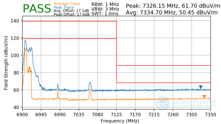
Plot 7-1068 SDM Primary Radiated Upper Band Edge (Peak & Average – UNII Band 8) – RU52
