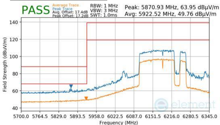
Plot 7-1021 Antenna 2a Radiated Lower Band Edge (Peak & Average – UNII Band 5) - RU996+484+242 (H)
