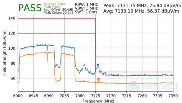
Plot 7-1027 Antenna 2a Radiated Upper Band Edge (Peak & Average – UNII Band 8) - RU996+484+242 (H)
