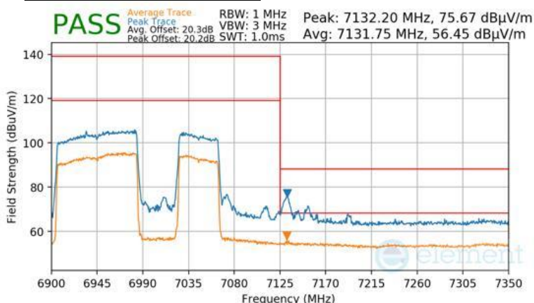
Plot 7-1013 Antenna 2a Radiated Upper Band Edge (Peak & Average – UNII Band 8) - RU996+484 (H)
