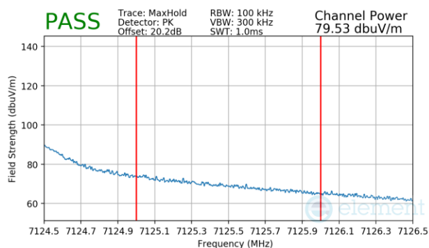
Plot 7-982 Antenna 2a Radiated Upper Band Edge (Peak – UNII Band 8)
