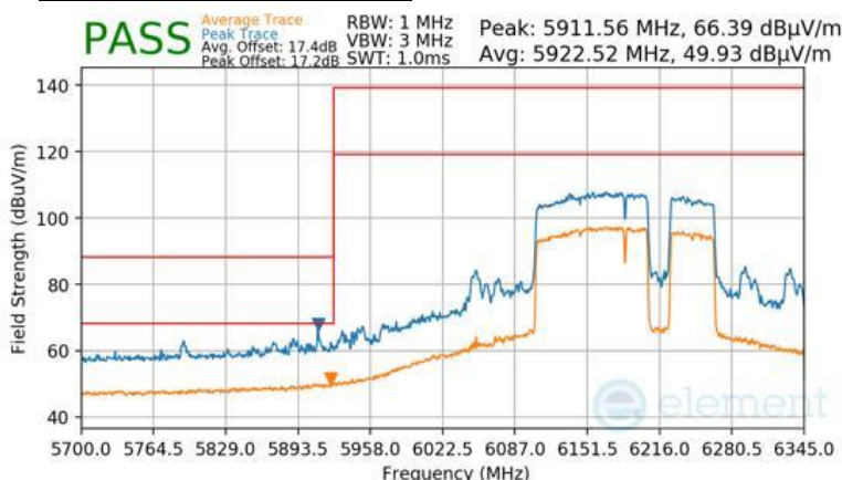
Plot 7-1019 Antenna 2a Radiated Lower Band Edge (Peak & Average – UNII Band 5) - RU996+484+242 (H)
