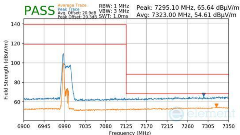
Plot 7-992 Antenna 2a Radiated Upper Band Edge (Peak & Average – UNII Band 8) - RU26
