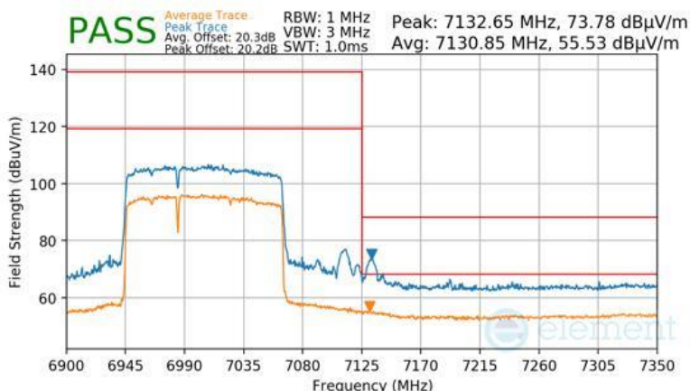
Plot 7-1012 Antenna 2a Radiated Upper Band Edge (Peak & Average – UNII Band 8) - RU996+484 (L)
