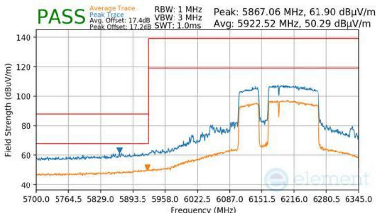
Plot 7-1020 Antenna 2a Radiated Lower Band Edge (Peak & Average – UNII Band 5) - RU996+484+242 (L)
