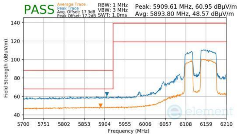
Plot 7-995 Antenna 2a Radiated Lower Band Edge (Peak & Average – UNII Band 5) - RU484+242
