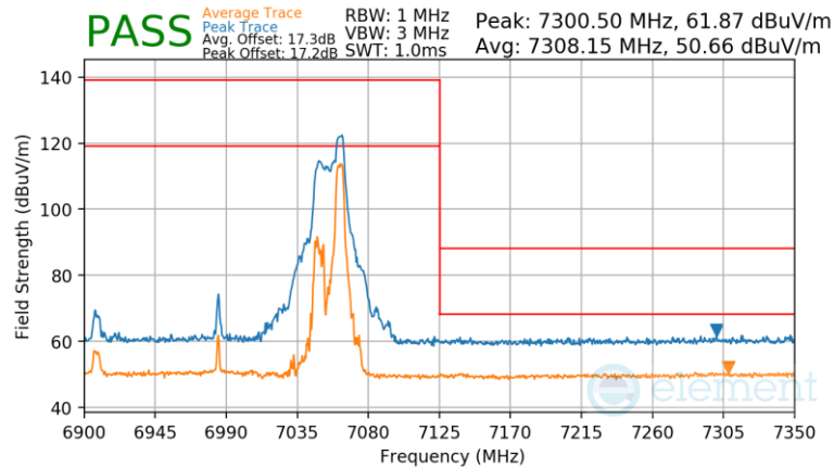
Plot 7-1069 SDM Primary Radiated Upper Band Edge (Peak & Average – UNII Band 8) – RU52
