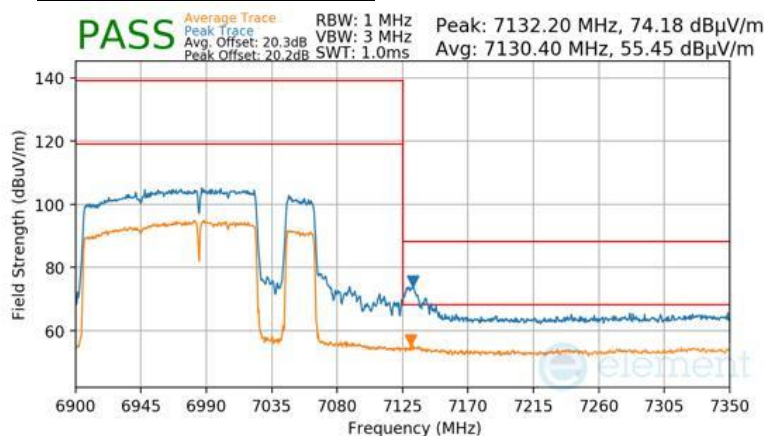
Plot 7-1029 Antenna 2a Radiated Upper Band Edge (Peak & Average – UNII Band 8) - RU996+484+242 (H)
