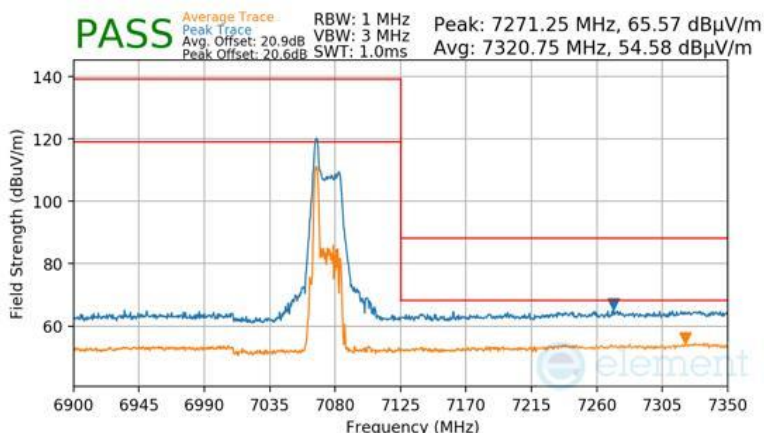
Plot 7-986 Antenna 2a Radiated Upper Band Edge (Peak & Average – UNII Band 8) - RU26
