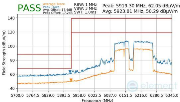
Plot 7-1022 Antenna 2a Radiated Lower Band Edge (Peak & Average – UNII Band 5) - RU996+484+242 (L)
