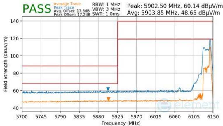
Plot 7-985 Antenna 2a Radiated Lower Band Edge (Peak & Average – UNII Band 5) - RU26
