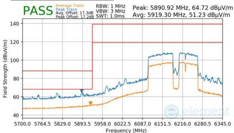
Plot 7-1017 Antenna 2a Radiated Lower Band Edge (Peak & Average – UNII Band 5) - RU996+484+242 (H)
