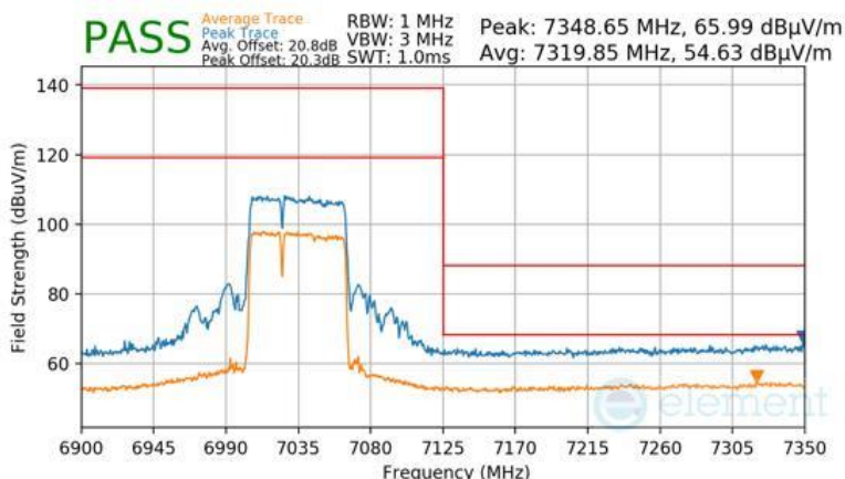
Plot 7-998 Antenna 2a Radiated Upper Band Edge (Peak & Average – UNII Band 8) - RU484+242
