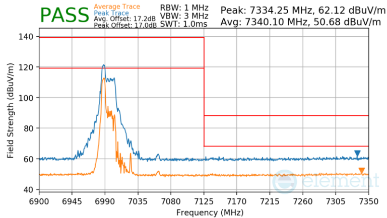
Plot 7-1054 SDM Primary Radiated Upper Band Edge (Peak & Average – UNII Band 8) – RU52
