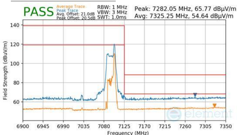
Plot 7-987 Antenna 2a Radiated Upper Band Edge (Peak & Average – UNII Band 8) - RU26
