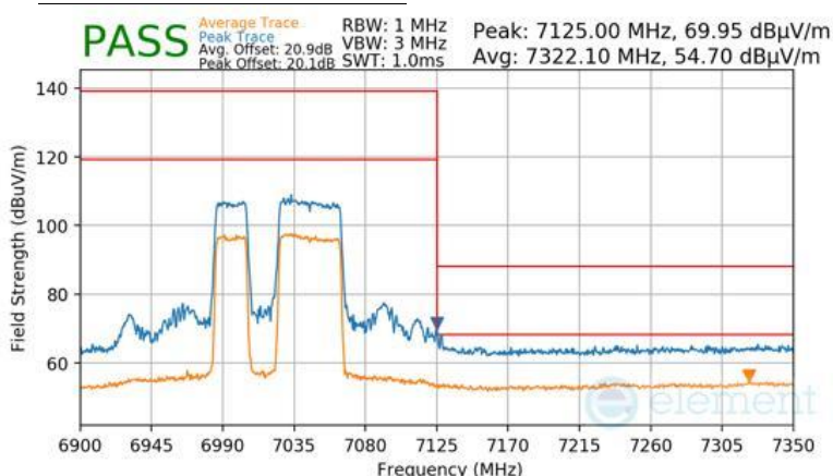
Plot 7-999 Antenna 2a Radiated Upper Band Edge (Peak & Average – UNII Band 8) - RU484+242
