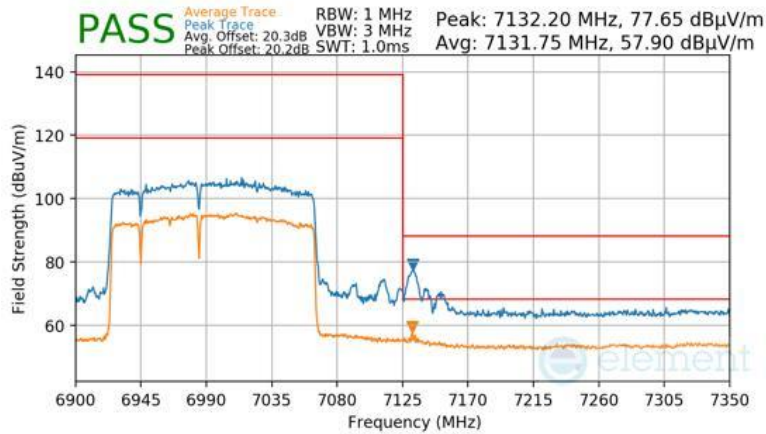
Plot 7-1024 Antenna 2a Radiated Upper Band Edge (Peak & Average – UNII Band 8) - RU996+484+242 (L)
