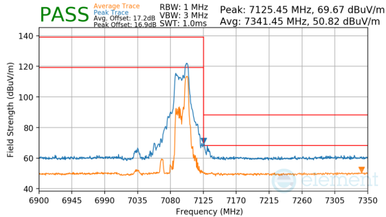
Plot 7-1049 SDM Primary Radiated Upper Band Edge (Peak & Average – UNII Band 8) – RU52
