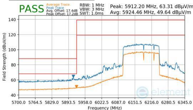
Plot 7-1023 Antenna 2a Radiated Lower Band Edge (Peak & Average – UNII Band 5) - RU996+484+242 (H)
