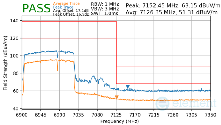
Plot 7-1014 Antenna 2a Radiated Upper Band Edge (Peak & Average – UNII Band 8) - RU996+484 (H)
