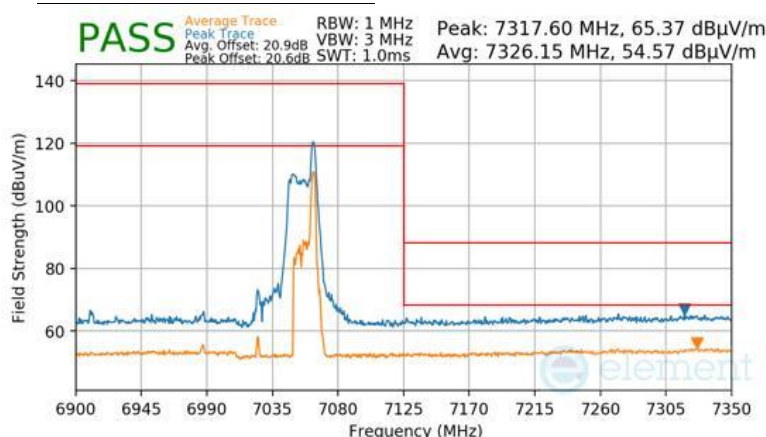
Plot 7-993 Antenna 2a Radiated Upper Band Edge (Peak & Average – UNII Band 8) - RU26
