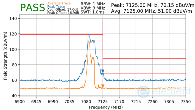
Plot 7-1036 SDM Primary Radiated Upper Band Edge (Peak & Average – UNII Band 8) – RU52
