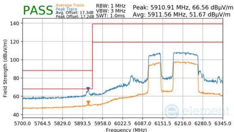
Plot 7-1010 Antenna 2a Radiated Lower Band Edge (Peak & Average – UNII Band 5) - RU996+484 (L)
