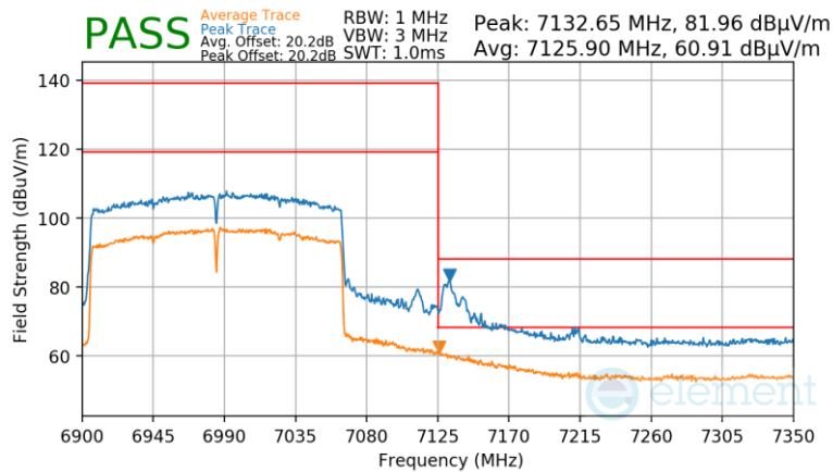
Plot 7-1033 Antenna 2a Radiated Upper Band Edge (Peak & Average – UNII Band 8) - RU996X2
