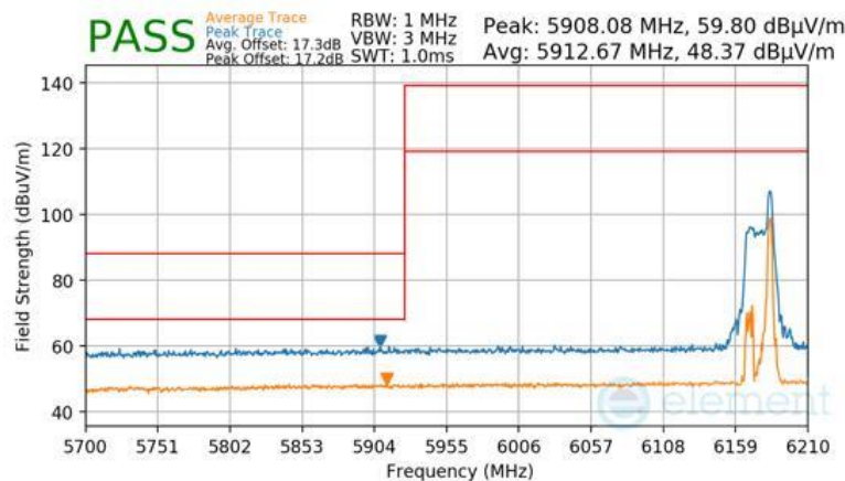
Plot 7-991 Antenna 2a Radiated Lower Band Edge (Peak & Average – UNII Band 5) - RU26
