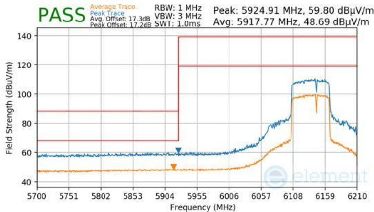
Plot 7-997 Antenna 2a Radiated Lower Band Edge (Peak & Average – UNII Band 5) - RU484+242
