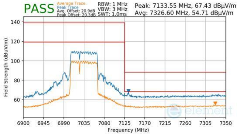
Plot 7-1060 SDM Primary Radiated Upper Band Edge (Peak & Average – UNII Band 8) - RU484+242
