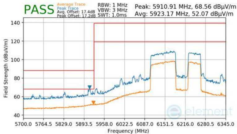
Plot 7-1009 Antenna 2a Radiated Lower Band Edge (Peak & Average – UNII Band 5) - RU996+484 (H)
