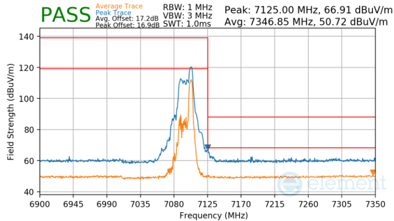
Plot 7-1037 SDM Primary Radiated Upper Band Edge (Peak & Average – UNII Band 8) – RU52
