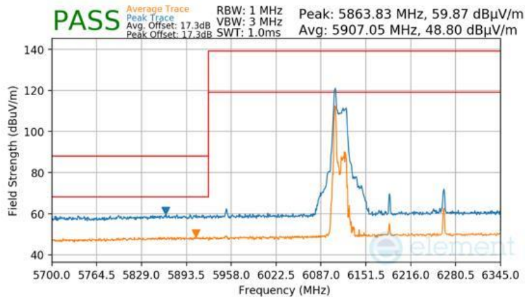
Plot 7-1004 Antenna 2a Radiated Lower Band Edge (Peak & Average – UNII Band 5) - RU26
