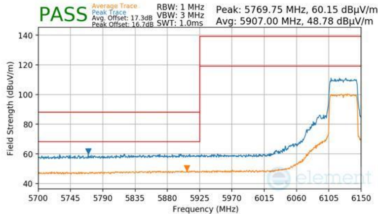
Plot 7-988 Antenna 2a Radiated Lower Band Edge (Peak & Average – UNII Band 5) - RU484
