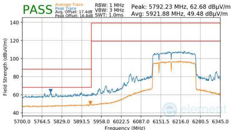
Plot 7-1016 Antenna 2a Radiated Lower Band Edge (Peak & Average – UNII Band 5) - RU996+484+242 (L)
