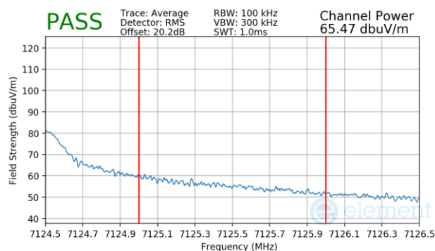
Plot 7-983 Antenna 2a Radiated Upper Band Edge (Average – UNII Band 8)
