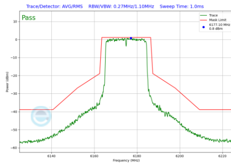
Plot 7-1197 In-Band Emission Plot CDD Diversity Antenna 2a (20MHz BW 802.11be(RU) RU242 Index61 (UNII Band 5) - Ch.45)
