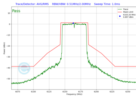
Plot 7-1198 In-Band Emission Plot CDD Diversity Antenna 2a (40MHz BW 802.11be(RU) RU484 Index65 (UNII Band 5) - Ch.43)
