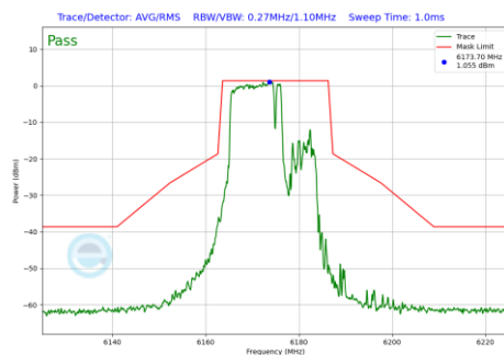
Plot 7-1034 In-Band Emission Plot CDD Primary Antenna 4a(20MHz BW 802.11be(RU) RU106+26 Index82 (UNII Band 5) - Ch.45)
