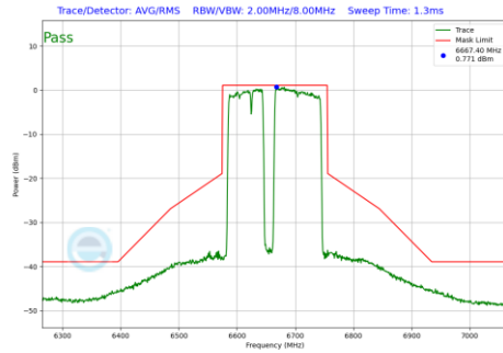
Plot 7-1187 In-Band Emission Plot CDD Diversity Antenna 2a (160MHz BW 802.11be(RU) RU996+484+242 Index99 (UNII Band 7) - Ch.143)
