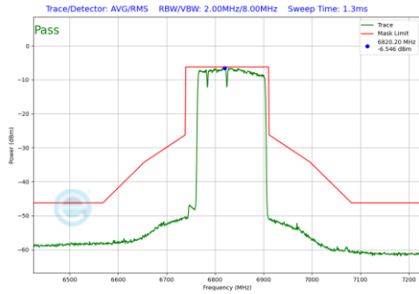
Plot 7-1107 In-Band Emission Plot SDM Primary Antenna WF5B (160MHz BW 802.11be(RU) RU996+484+242 Index96 (UNII Band 7) - Ch.175)
