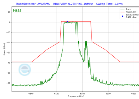
Plot 7-1179 In-Band Emission Plot CDD Diversity Antenna 2a (20MHz BW 802.11be(RU) RU106+26 Index82 (UNII Band 5) - Ch.45)
