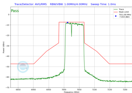
Plot 7-1109 In-Band Emission Plot SDM Primary Antenna WF5B (80MHz BW 802.11be(RU) RU484+242 Index90 (UNII Band 8) - Ch.215)
