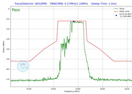
Plot 7-1099 In-Band Emission Plot SDM Primary Antenna WF5B (20MHz BW 802.11be(RU) RU106+26 Index83 (UNII Band 5) - Ch.45)
