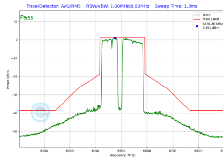
Plot 7-1193 In-Band Emission Plot CDD Diversity Antenna 4a(160MHz BW 802.11be(RU) RU996+484+242 Index99 (UNII Band 6) - Ch.111)
