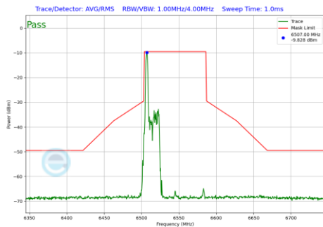
Plot 7-1093 In-Band Emission Plot SDM Primary Antenna 4a(80MHz BW 802.11be(RU) RU26 Index0 (UNII Band 7) - Ch.119)
