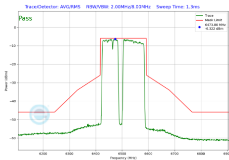
Plot 7-1116 In-Band Emission Plot SDM Primary Antenna 4a(160MHz BW 802.11be(RU) RU996+484+242 Index99 (UNII Band 6) - Ch.111)
