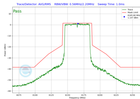
Plot 7-1056 In-Band Emission Plot CDD Primary Antenna 4a(40MHz BW 802.11be(RU) RU484 Index65 (UNII Band 5) - Ch.43)
