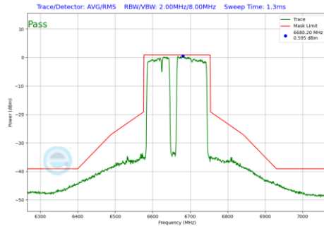
Plot 7-1033 In-Band Emission Plot CDD Primary Antenna WF5B (160MHz BW 802.11be(RU) RU996+484+242 Index99 (UNII Band 7) - Ch.143)
