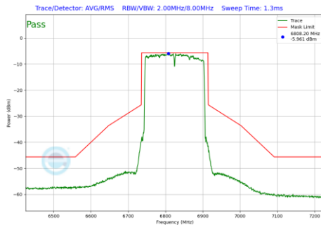
Plot 7-1150 In-Band Emission Plot SDM Primary Antenna 4a(160MHz BW 802.11be(RU) RU996X2 Index68 (UNII Band 7) - Ch.175)
