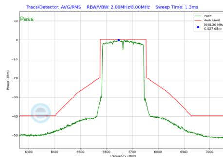
Plot 7-1066 In-Band Emission Plot CDD Primary Antenna 4a(160MHz BW 802.11be(RU) RU996X2 Index68 (UNII Band 7) - Ch.143)
