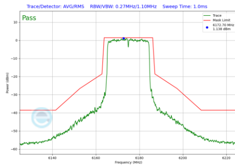
Plot 7-1043 In-Band Emission Plot CDD Primary Antenna WF5B (20MHz BW 802.11be(RU) RU242 Index61 (UNII Band 5) - Ch.45)
