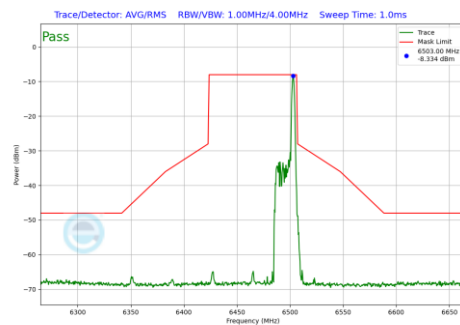
Plot 7-1089 In-Band Emission Plot SDM Primary Antenna 4a(80MHz BW 802.11be(RU) RU26 Index36 (UNII Band 6) - Ch.103)
