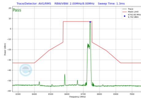
Plot 7-1178 In-Band Emission Plot CDD Diversity Antenna 4a(160MHz BW 802.11be(RU) RU26 Index36 (UNII Band 7) - Ch.143)
