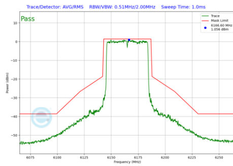
Plot 7-1044 In-Band Emission Plot CDD Primary Antenna WF5B (40MHz BW 802.11be(RU) RU484 Index65 (UNII Band 5) - Ch.43)
