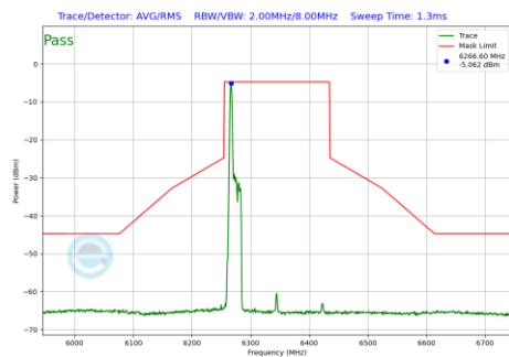
Plot 7-1086 In-Band Emission Plot SDM Primary Antenna 4a(160MHz BW 802.11be(RU) RU26 Index0 (UNII Band 5) - Ch.79)
