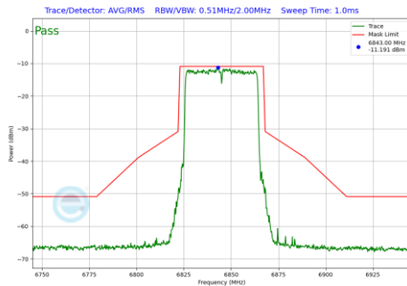
Plot 7-1148 In-Band Emission Plot SDM Primary Antenna 4a(40MHz BW 802.11be(RU) RU484 Index65 (UNII Band 7) - Ch.179)
