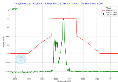
Plot 7-1068 In-Band Emission Plot SDM Primary Antenna WF5B (40MHz BW 802.11be(RU) RU26 Index8 (UNII Band 5) - Ch.3)
