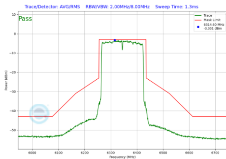
Plot 7-1126 In-Band Emission Plot SDM Primary Antenna WF5B (160MHz BW 802.11be(RU) RU996X2 Index68 (UNII Band 5) - Ch.79)
