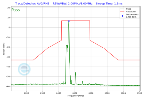
Plot 7-1174 In-Band Emission Plot CDD Diversity Antenna 4a(160MHz BW 802.11be(RU) RU26 Index17 (UNII Band 6) - Ch.111)
