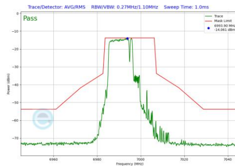
Plot 7-1120 In-Band Emission Plot SDM Primary Antenna 4a(20MHz BW 802.11be(RU) RU106+26 Index82 (UNII Band 8) - Ch.209)
