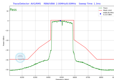
Plot 7-1062 In-Band Emission Plot CDD Primary Antenna 4a(160MHz BW 802.11be(RU) RU996X2 Index68 (UNII Band 6) - Ch.111)
