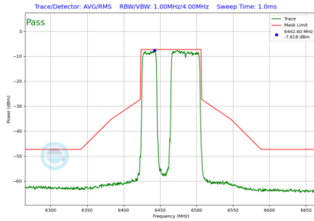
Plot 7-1115 In-Band Emission Plot SDM Primary Antenna 4a(80MHz BW 802.11be(RU) RU484+242 Index91 (UNII Band 6) - Ch.103)
