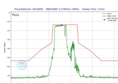
Plot 7-1105 In-Band Emission Plot SDM Primary Antenna WF5B (20MHz BW 802.11be(RU) RU106+26 Index82 (UNII Band 7) - Ch.185)
