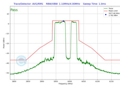
Plot 7-1035 In-Band Emission Plot CDD Primary Antenna 4a(80MHz BW 802.11be(RU) RU484+242 Index92 (UNII Band 5) - Ch.7)
