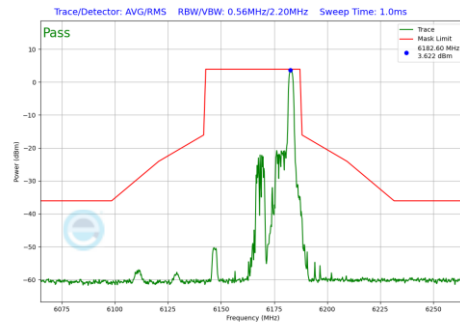
Plot 7-1168 In-Band Emission Plot CDD Diversity Antenna 4a(40MHz BW 802.11be(RU) RU26 Index17 (UNII Band 5) - Ch.43)
