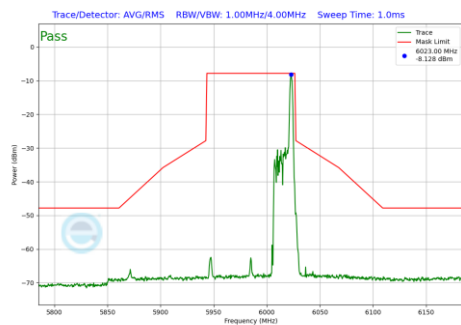
Plot 7-1085 In-Band Emission Plot SDM Primary Antenna 4a(80MHz BW 802.11be(RU) RU26 Index36 (UNII Band 5) - Ch.7)
