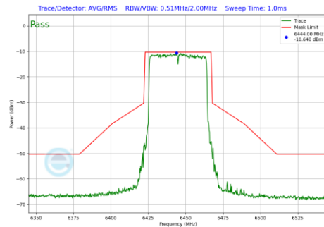
Plot 7-1144 In-Band Emission Plot SDM Primary Antenna 4a(40MHz BW 802.11be(RU) RU484 Index65 (UNII Band 6) - Ch.99)
