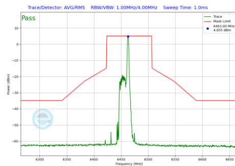
Plot 7-1161 In-Band Emission Plot CDD Diversity Antenna 2a (80MHz BW 802.11be(RU) RU26 Index17 (UNII Band 6) - Ch.103)
