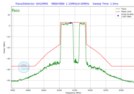
Plot 7-1189 In-Band Emission Plot CDD Diversity Antenna 4a(80MHz BW 802.11be(RU) RU484+242 Index92 (UNII Band 5) - Ch.39)
