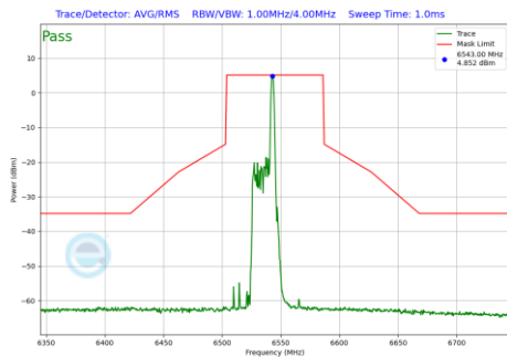
Plot 7-1165 In-Band Emission Plot CDD Diversity Antenna 2a (80MHz BW 802.11be(RU) RU26 Index17 (UNII Band 7) - Ch.119)
