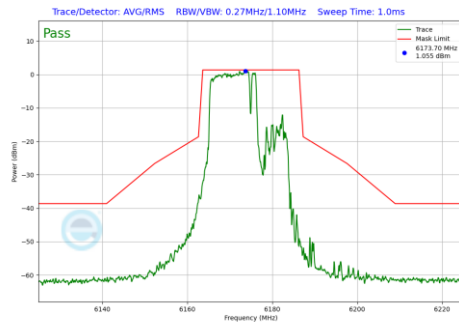
Plot 7-1188 In-Band Emission Plot CDD Diversity Antenna 4a(20MHz BW 802.11be(RU) RU106+26 Index82 (UNII Band 5) - Ch.45)
