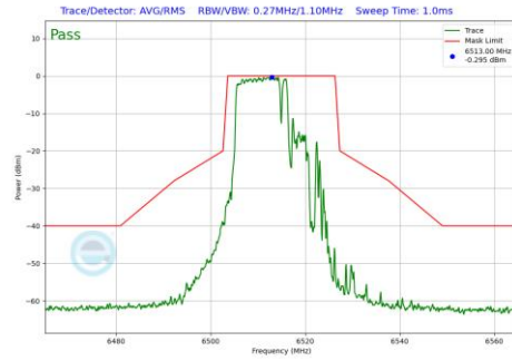
Plot 7-1037 In-Band Emission Plot CDD Primary Antenna 4a(20MHz BW 802.11be(RU) RU106+26 Index82 (UNII Band 6) - Ch.113)
