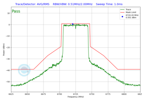
Plot 7-1052 In-Band Emission Plot CDD Primary Antenna WF5B (40MHz BW 802.11be(RU) RU484 Index65 (UNII Band 7) - Ch.155)
