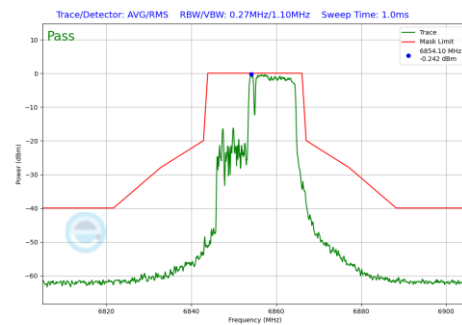
Plot 7-1185 In-Band Emission Plot CDD Diversity Antenna 2a (20MHz BW 802.11be(RU) RU106+26 Index83 (UNII Band 7) - Ch.181)
