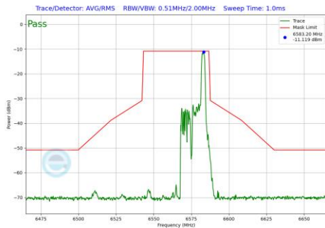
Plot 7-1092 In-Band Emission Plot SDM Primary Antenna 4a(40MHz BW 802.11be(RU) RU26 Index17 (UNII Band 7) - Ch.123)
