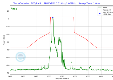
Plot 7-1160 In-Band Emission Plot CDD Diversity Antenna 2a (40MHz BW 802.11be(RU) RU26 Index0 (UNII Band 6) - Ch.115)
