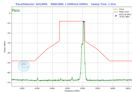
Plot 7-1073 In-Band Emission Plot SDM Primary Antenna WF5B (80MHz BW 802.11be(RU) RU26 Index36 (UNII Band 6) - Ch.103)
