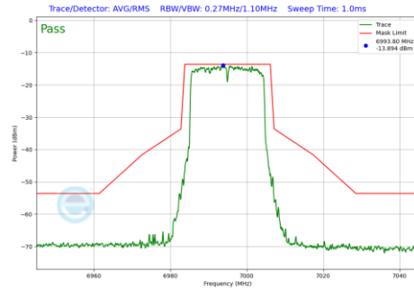
Plot 7-1135 In-Band Emission Plot SDM Primary Antenna WF5B (20MHz BW 802.11be(RU) RU242 Index61 (UNII Band 8) - Ch.209)
