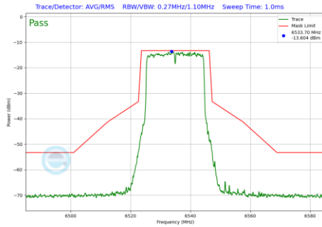
Plot 7-1147 In-Band Emission Plot SDM Primary Antenna 4a(20MHz BW 802.11be(RU) RU242 Index61 (UNII Band 7) - Ch.117)
