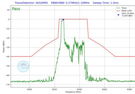
Plot 7-1163 In-Band Emission Plot CDD Diversity Antenna 2a (20MHz BW 802.11be(RU) RU26 Index0 (UNII Band 7) - Ch.117)
