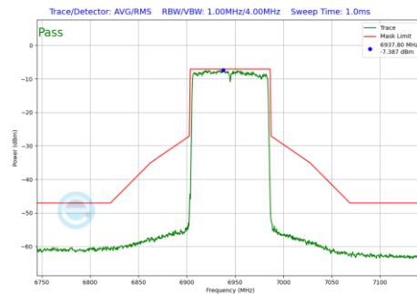
Plot 7-1153 In-Band Emission Plot SDM Primary Antenna 4a(80MHz BW 802.11be(RU) RU996 Index67 (UNII Band 8) - Ch.199)
