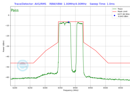
Plot 7-1100 In-Band Emission Plot SDM Primary Antenna WF5B (80MHz BW 802.11be(RU) RU484+242 Index92 (UNII Band 5) - Ch.87)
