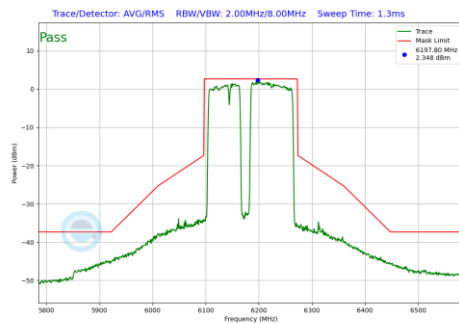
Plot 7-1036 In-Band Emission Plot CDD Primary Antenna 4a(160MHz BW 802.11be(RU) RU996+484+242 Index99 (UNII Band 5) - Ch.47)
