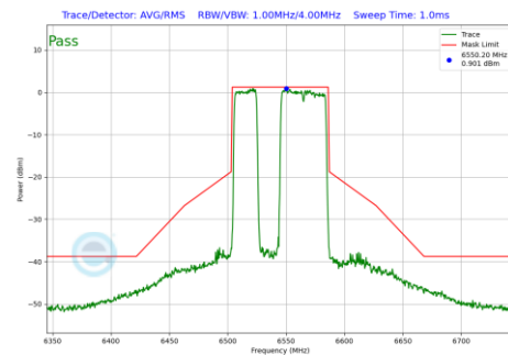
Plot 7-1186 In-Band Emission Plot CDD Diversity Antenna 2a (80MHz BW 802.11be(RU) RU484+242 Index91 (UNII Band 7) - Ch.119)
