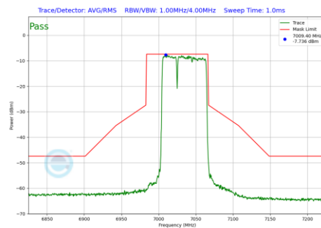
Plot 7-1121 In-Band Emission Plot SDM Primary Antenna 4a(80MHz BW 802.11be(RU) RU484+242 Index90 (UNII Band 8) - Ch.215)
