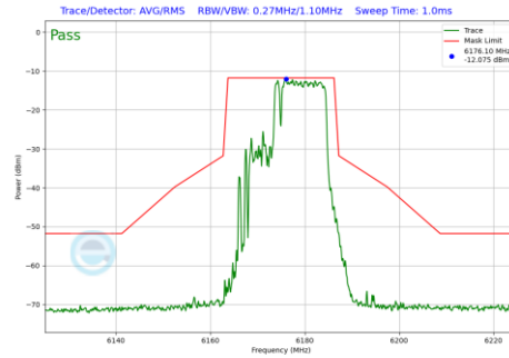
Plot 7-1111 In-Band Emission Plot SDM Primary Antenna 4a(20MHz BW 802.11be(RU) RU106+26 Index83 (UNII Band 5) - Ch.45)
