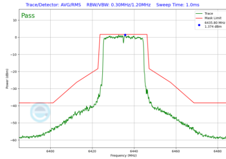
Plot 7-1059 In-Band Emission Plot CDD Primary Antenna 4a(20MHz BW 802.11be(RU) RU242 Index61 (UNII Band 6) - Ch.97)
