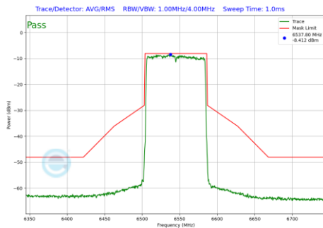
Plot 7-1149 In-Band Emission Plot SDM Primary Antenna 4a(80MHz BW 802.11be(RU) RU996 Index67 (UNII Band 7) - Ch.119)
