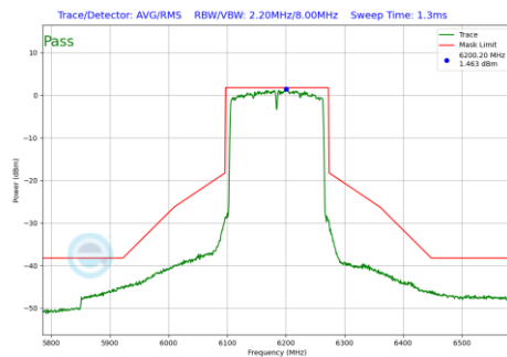
Plot 7-1200 In-Band Emission Plot CDD Diversity Antenna 2a (160MHz BW 802.11be(RU) RU996X2 Index68 (UNII Band 5) - Ch.47)
