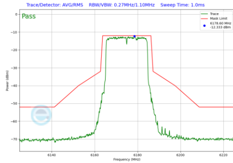
Plot 7-1139 In-Band Emission Plot SDM Primary Antenna 4a(20MHz BW 802.11be(RU) RU242 Index61 (UNII Band 5) - Ch.45)
