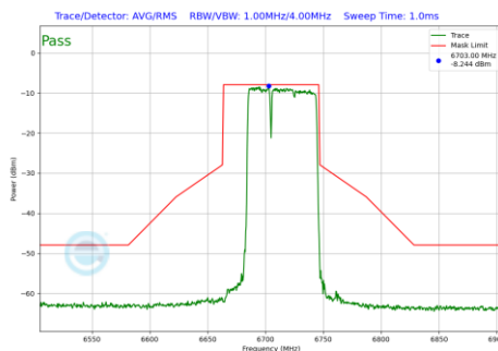
Plot 7-1118 In-Band Emission Plot SDM Primary Antenna 4a(80MHz BW 802.11be(RU) RU484+242 Index90 (UNII Band 7) - Ch.151)
