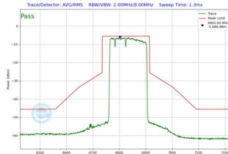
Plot 7-1119 In-Band Emission Plot SDM Primary Antenna 4a(160MHz BW 802.11be(RU) RU996+484+242 Index96 (UNII Band 7) - Ch.175)
