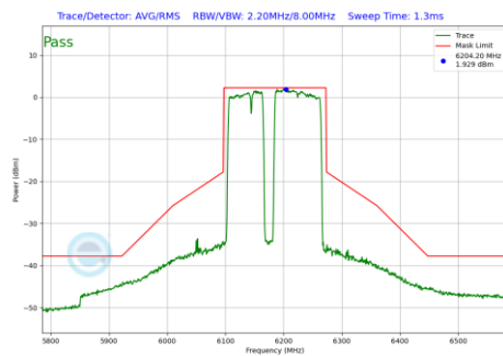
Plot 7-1181 In-Band Emission Plot CDD Diversity Antenna 2a (160MHz BW 802.11be(RU) RU996+484+242 Index99 (UNII Band 5) - Ch.47)
