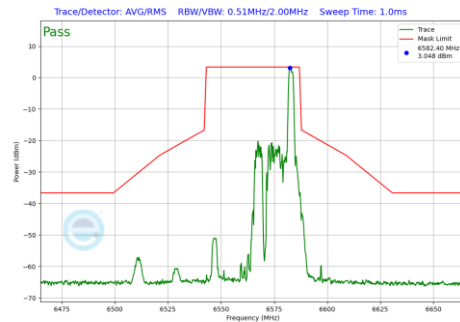
Plot 7-1176 In-Band Emission Plot CDD Diversity Antenna 4a(40MHz BW 802.11be(RU) RU26 Index17 (UNII Band 7) - Ch.123)
