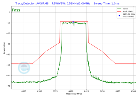
Plot 7-1140 In-Band Emission Plot SDM Primary Antenna 4a(40MHz BW 802.11be(RU) RU484 Index65 (UNII Band 5) - Ch.91)
