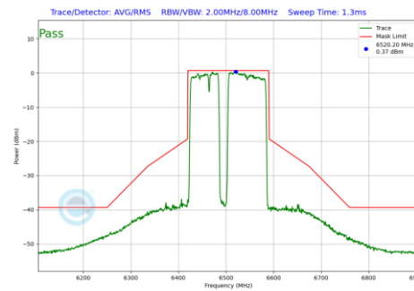
Plot 7-1184 In-Band Emission Plot CDD Diversity Antenna 2a (160MHz BW 802.11be(RU) RU996+484+242 Index99 (UNII Band 6) - Ch.111)
