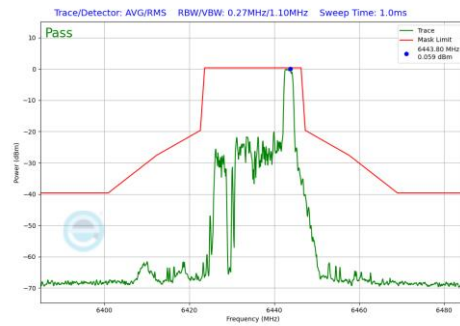
Plot 7-1159 In-Band Emission Plot CDD Diversity Antenna 2a (20MHz BW 802.11be(RU) RU26 Index8 (UNII Band 6) - Ch.97)
