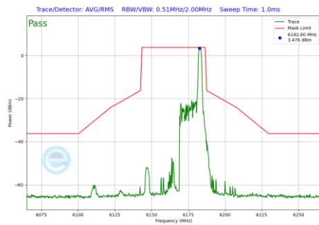
Plot 7-1156 In-Band Emission Plot CDD Diversity Antenna 2a (40MHz BW 802.11be(RU) RU26 Index17 (UNII Band 5) - Ch.43)
