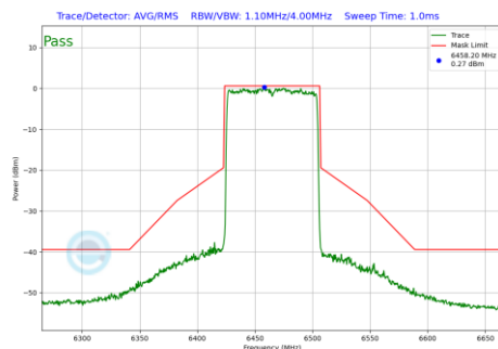
Plot 7-1061 In-Band Emission Plot CDD Primary Antenna 4a(80MHz BW 802.11be(RU) RU996 Index67 (UNII Band 6) - Ch.103)
