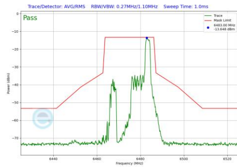
Plot 7-1071 In-Band Emission Plot SDM Primary Antenna WF5B (20MHz BW 802.11be(RU) RU26 Index8 (UNII Band 6) - Ch.105)
