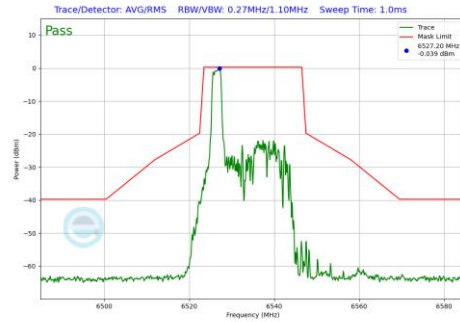
Plot 7-1175 In-Band Emission Plot CDD Diversity Antenna 4a(20MHz BW 802.11be(RU) RU26 Index0 (UNII Band 7) - Ch.117)
