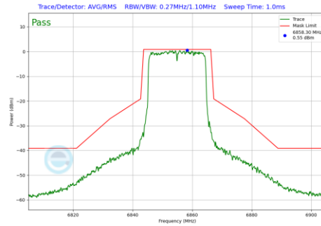
Plot 7-1063 In-Band Emission Plot CDD Primary Antenna 4a(20MHz BW 802.11be(RU) RU242 Index61 (UNII Band 7) - Ch.181)
