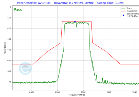
Plot 7-1151 In-Band Emission Plot SDM Primary Antenna 4a(20MHz BW 802.11be(RU) RU242 Index61 (UNII Band 8) - Ch.209)
