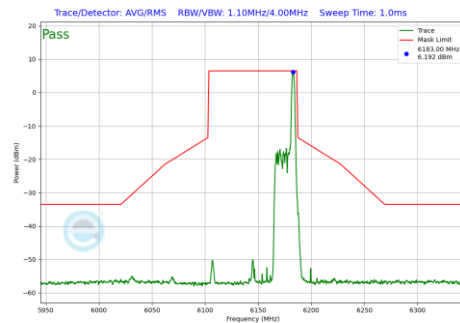
Plot 7-1169 In-Band Emission Plot CDD Diversity Antenna 4a(80MHz BW 802.11be(RU) RU26 Index36 (UNII Band 5) - Ch.39)
