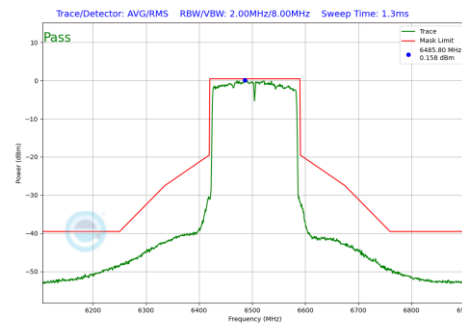
Plot 7-1204 In-Band Emission Plot CDD Diversity Antenna 2a (160MHz BW 802.11be(RU) RU996X2 Index68 (UNII Band 6) - Ch.111)
