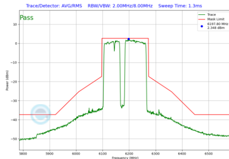
Plot 7-1190 In-Band Emission Plot CDD Diversity Antenna 4a(160MHz BW 802.11be(RU) RU996+484+242 Index99 (UNII Band 5) - Ch.47)
