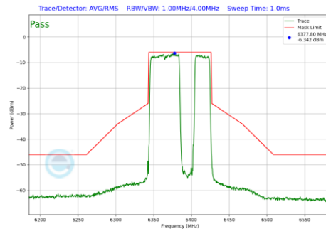
Plot 7-1112 In-Band Emission Plot SDM Primary Antenna 4a(80MHz BW 802.11be(RU) RU484+242 Index92 (UNII Band 5) - Ch.87)
