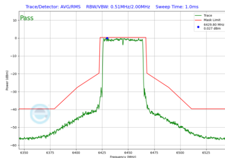
Plot 7-1060 In-Band Emission Plot CDD Primary Antenna 4a(40MHz BW 802.11be(RU) RU484 Index65 (UNII Band 6) - Ch.99)
