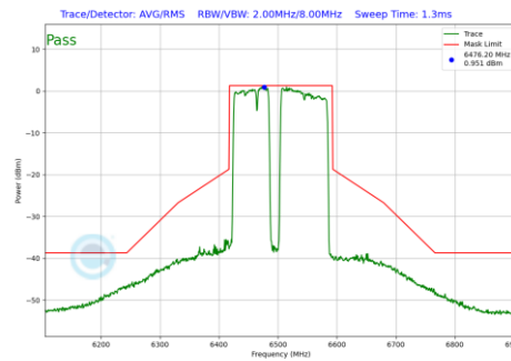
Plot 7-1039 In-Band Emission Plot CDD Primary Antenna 4a(160MHz BW 802.11be(RU) RU996+484+242 Index99 (UNII Band 6) - Ch.111)
