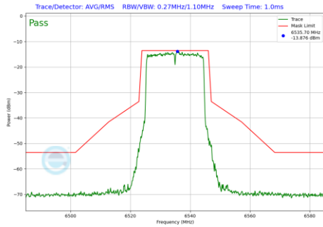
Plot 7-1131 In-Band Emission Plot SDM Primary Antenna WF5B (20MHz BW 802.11be(RU) RU242 Index61 (UNII Band 7) - Ch.117)
