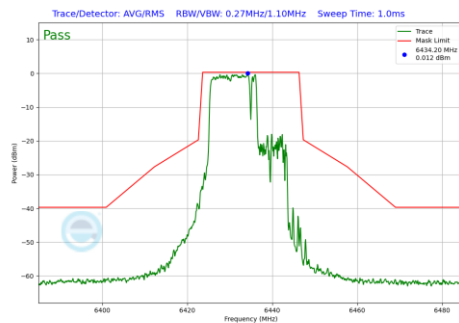
Plot 7-1182 In-Band Emission Plot CDD Diversity Antenna 2a (20MHz BW 802.11be(RU) RU106+26 Index82 (UNII Band 6) - Ch.97)
