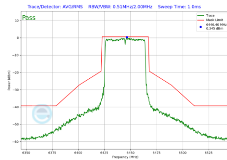
Plot 7-1202 In-Band Emission Plot CDD Diversity Antenna 2a (40MHz BW 802.11be(RU) RU484 Index65 (UNII Band 6) - Ch.99)
