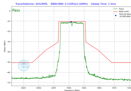
Plot 7-1136 In-Band Emission Plot SDM Primary Antenna WF5B (40MHz BW 802.11be(RU) RU484 Index65 (UNII Band 8) - Ch.211)
