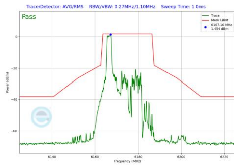
Plot 7-1155 In-Band Emission Plot CDD Diversity Antenna 2a (20MHz BW 802.11be(RU) RU26 Index0 (UNII Band 5) - Ch.45)
