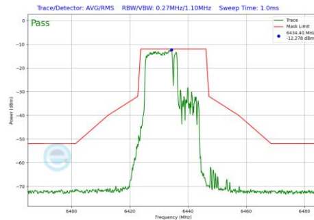
Plot 7-1114 In-Band Emission Plot SDM Primary Antenna 4a(20MHz BW 802.11be(RU) RU106+26 Index82 (UNII Band 6) - Ch.97)
