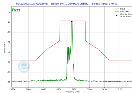
Plot 7-1097 In-Band Emission Plot SDM Primary Antenna 4a(80MHz BW 802.11be(RU) RU26 Index17 (UNII Band 8) - Ch.199)
