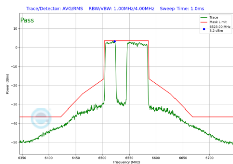
Plot 7-1195 In-Band Emission Plot CDD Diversity Antenna 4a(80MHz BW 802.11be(RU) RU484+242 Index91 (UNII Band 7) - Ch.119)
