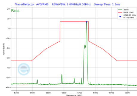
Plot 7-1166 In-Band Emission Plot CDD Diversity Antenna 2a (160MHz BW 802.11be(RU) RU26 Index36 (UNII Band 7) - Ch.143)
