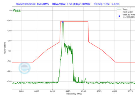
Plot 7-1088 In-Band Emission Plot SDM Primary Antenna 4a(40MHz BW 802.11be(RU) RU26 Index0 (UNII Band 6) - Ch.107)
