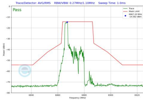
Plot 7-1091 In-Band Emission Plot SDM Primary Antenna 4a(20MHz BW 802.11be(RU) RU26 Index0 (UNII Band 7) - Ch.185)
