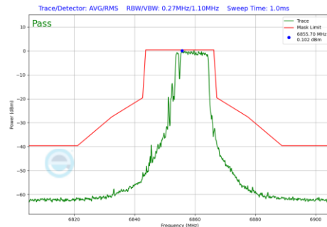
Plot 7-1194 In-Band Emission Plot CDD Diversity Antenna 4a(20MHz BW 802.11be(RU) RU106+26 Index83 (UNII Band 7) - Ch.181)
