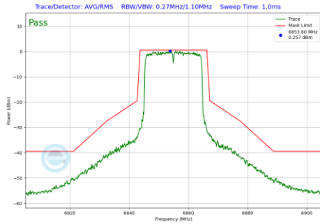
Plot 7-1051 In-Band Emission Plot CDD Primary Antenna WF5B (20MHz BW 802.11be(RU) RU242 Index61 (UNII Band 7) - Ch.181)
