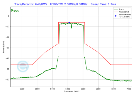
Plot 7-1134 In-Band Emission Plot SDM Primary Antenna WF5B (160MHz BW 802.11be(RU) RU996X2 Index68 (UNII Band 7) - Ch.175)
