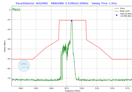
Plot 7-1096 In-Band Emission Plot SDM Primary Antenna 4a(40MHz BW 802.11be(RU) RU26 Index8 (UNII Band 8) - Ch.227)
