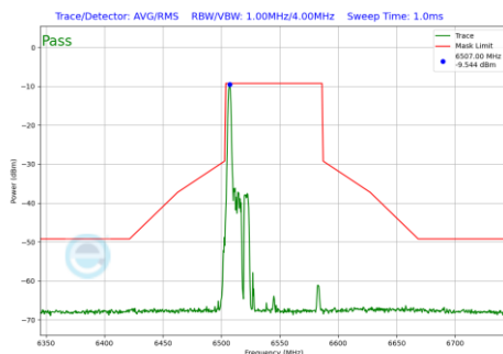
Plot 7-1077 In-Band Emission Plot SDM Primary Antenna WF5B (80MHz BW 802.11be(RU) RU26 Index0 (UNII Band 7) - Ch.119)
