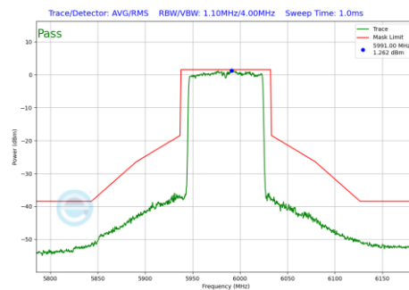
Plot 7-1057 In-Band Emission Plot CDD Primary Antenna 4a(80MHz BW 802.11be(RU) RU996 Index67 (UNII Band 5) - Ch.7)
