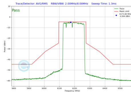
Plot 7-1113 In-Band Emission Plot SDM Primary Antenna 4a(160MHz BW 802.11be(RU) RU996+484+242 Index96 (UNII Band 5) - Ch.47)
