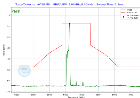
Plot 7-1078 In-Band Emission Plot SDM Primary Antenna WF5B (160MHz BW 802.11be(RU) RU26 Index17 (UNII Band 7) - Ch.143)
