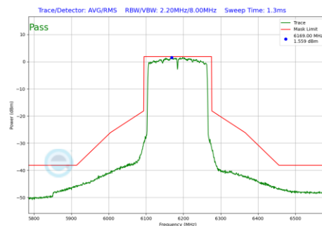
Plot 7-1058 In-Band Emission Plot CDD Primary Antenna 4a(160MHz BW 802.11be(RU) RU996X2 Index68 (UNII Band 5) - Ch.47)
