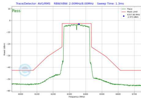
Plot 7-1142 In-Band Emission Plot SDM Primary Antenna 4a(160MHz BW 802.11be(RU) RU996X2 Index68 (UNII Band 5) - Ch.79)
