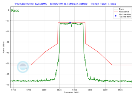
Plot 7-1132 In-Band Emission Plot SDM Primary Antenna WF5B (40MHz BW 802.11be(RU) RU484 Index65 (UNII Band 7) - Ch.179)
