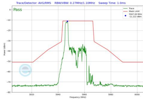
Plot 7-1083 In-Band Emission Plot SDM Primary Antenna 4a(20MHz BW 802.11be(RU) RU26 Index0 (UNII Band 5) - Ch.1)
