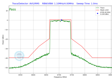
Plot 7-1053 In-Band Emission Plot CDD Primary Antenna WF5B (80MHz BW 802.11be(RU) RU996 Index67 (UNII Band 7) - Ch.151)
