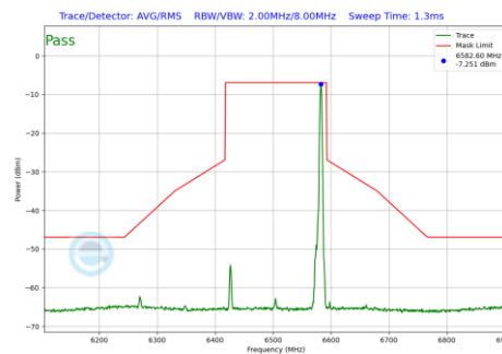
Plot 7-1090 In-Band Emission Plot SDM Primary Antenna 4a(160MHz BW 802.11be(RU) RU26 Index36 (UNII Band 6) - Ch.111)
