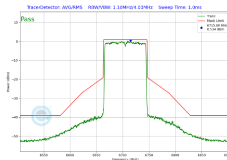
Plot 7-1065 In-Band Emission Plot CDD Primary Antenna 4a(80MHz BW 802.11be(RU) RU996 Index67 (UNII Band 7) - Ch.151)
