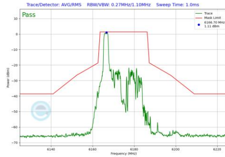
Plot 7-1167 In-Band Emission Plot CDD Diversity Antenna 4a(20MHz BW 802.11be(RU) RU26 Index0 (UNII Band 5) - Ch.45)
