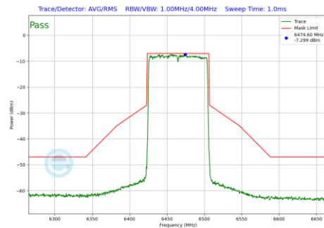
Plot 7-1145 In-Band Emission Plot SDM Primary Antenna 4a(80MHz BW 802.11be(RU) RU996 Index67 (UNII Band 6) - Ch.103)
