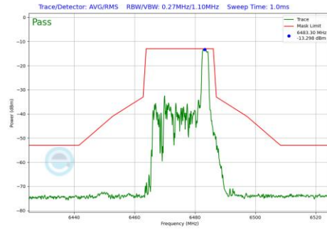
Plot 7-1087 In-Band Emission Plot SDM Primary Antenna 4a(20MHz BW 802.11be(RU) RU26 Index8 (UNII Band 6) - Ch.105)
