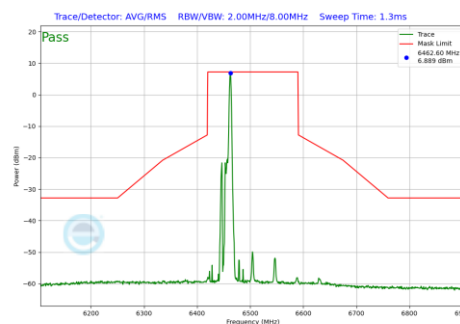
Plot 7-1162 In-Band Emission Plot CDD Diversity Antenna 2a (160MHz BW 802.11be(RU) RU26 Index17 (UNII Band 6) - Ch.111)
