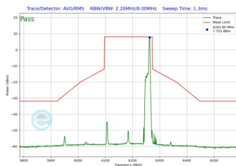
Plot 7-1158 In-Band Emission Plot CDD Diversity Antenna 2a (160MHz BW 802.11be(RU) RU26 Index36 (UNII Band 5) - Ch.47)
