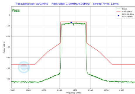
Plot 7-1141 In-Band Emission Plot SDM Primary Antenna 4a(80MHz BW 802.11be(RU) RU996 Index67 (UNII Band 5) - Ch.39)
