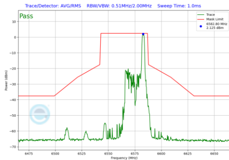
Plot 7-1164 In-Band Emission Plot CDD Diversity Antenna 2a (40MHz BW 802.11be(RU) RU26 Index17 (UNII Band 7) - Ch.123)
