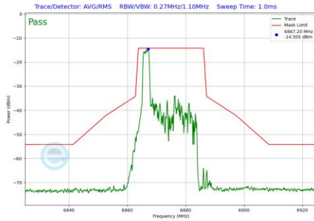
Plot 7-1075 In-Band Emission Plot SDM Primary Antenna WF5B (20MHz BW 802.11be(RU) RU26 Index0 (UNII Band 7) - Ch.185)
