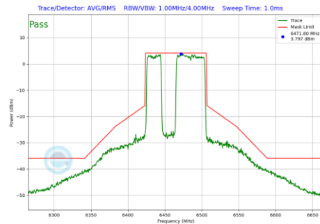
Plot 7-1192 In-Band Emission Plot CDD Diversity Antenna 4a(80MHz BW 802.11be(RU) RU484+242 Index91 (UNII Band 6) - Ch.103)
