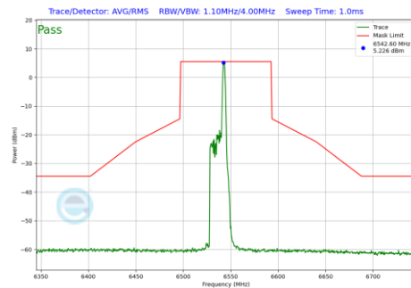
Plot 7-1177 In-Band Emission Plot CDD Diversity Antenna 4a(80MHz BW 802.11be(RU) RU26 Index17 (UNII Band 7) - Ch.119)
