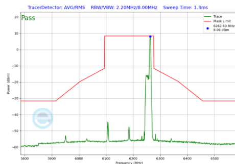
Plot 7-1170 In-Band Emission Plot CDD Diversity Antenna 4a(160MHz BW 802.11be(RU) RU26 Index36 (UNII Band 5) - Ch.47)
