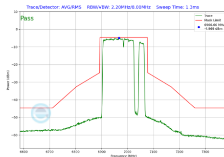
Plot 7-1122 In-Band Emission Plot SDM Primary Antenna 4a(160MHz BW 802.11be(RU) RU996+484+242 Index98 (UNII Band 8) - Ch.207)
