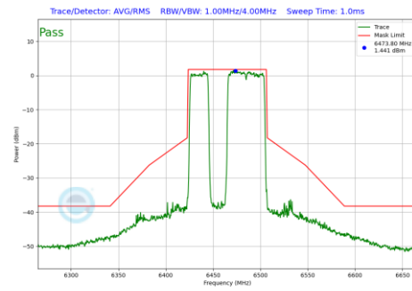
Plot 7-1183 In-Band Emission Plot CDD Diversity Antenna 2a (80MHz BW 802.11be(RU) RU484+242 Index91 (UNII Band 6) - Ch.103)
