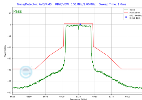
Plot 7-1064 In-Band Emission Plot CDD Primary Antenna 4a(40MHz BW 802.11be(RU) RU484 Index65 (UNII Band 7) - Ch.155)
