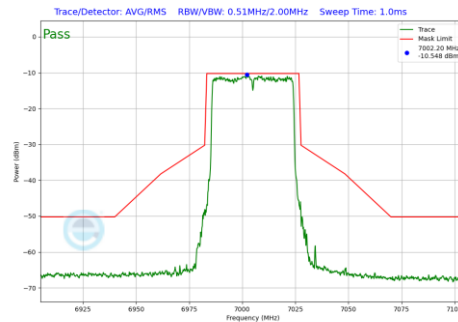
Plot 7-1152 In-Band Emission Plot SDM Primary Antenna 4a(40MHz BW 802.11be(RU) RU484 Index65 (UNII Band 8) - Ch.211)
