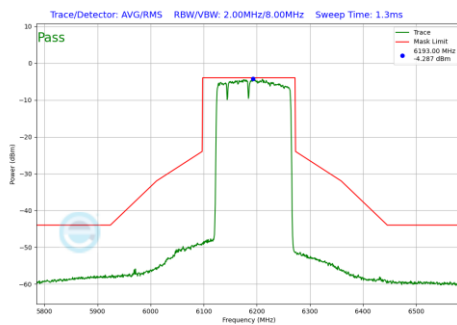
Plot 7-1101 In-Band Emission Plot SDM Primary Antenna WF5B (160MHz BW 802.11be(RU) RU996+484+242 Index96 (UNII Band 5) - Ch.47)
