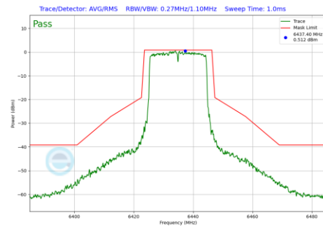
Plot 7-1201 In-Band Emission Plot CDD Diversity Antenna 2a (20MHz BW 802.11be(RU) RU242 Index61 (UNII Band 6) - Ch.97)
