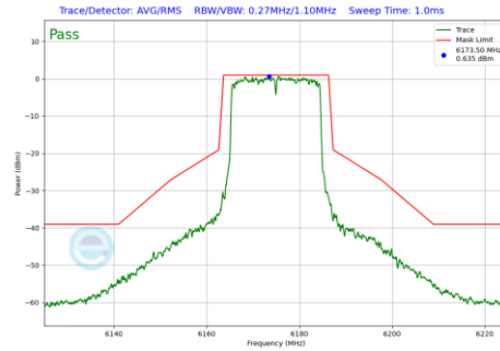
Plot 7-1055 In-Band Emission Plot CDD Primary Antenna 4a(20MHz BW 802.11be(RU) RU242 Index61 (UNII Band 5) - Ch.45)
