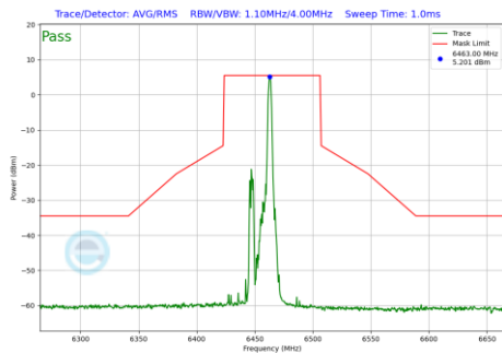
Plot 7-1173 In-Band Emission Plot CDD Diversity Antenna 4a(80MHz BW 802.11be(RU) RU26 Index17 (UNII Band 6) - Ch.103)
