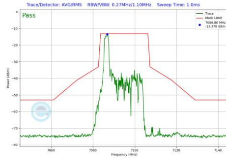
Plot 7-1095 In-Band Emission Plot SDM Primary Antenna 4a(20MHz BW 802.11be(RU) RU26 Index0 (UNII Band 8) - Ch.229)
