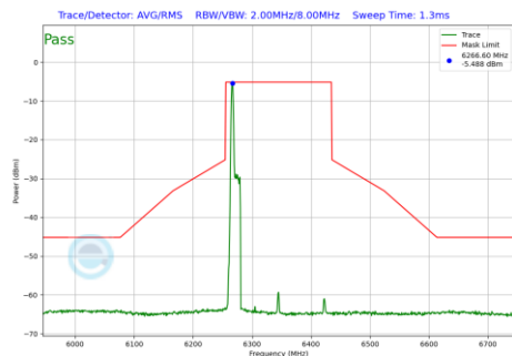
Plot 7-1070 In-Band Emission Plot SDM Primary Antenna WF5B (160MHz BW 802.11be(RU) RU26 Index0 (UNII Band 5) - Ch.79)
