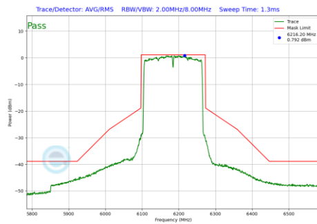
Plot 7-1046 In-Band Emission Plot CDD Primary Antenna WF5B (160MHz BW 802.11be(RU) RU996X2 Index68 (UNII Band 5) - Ch.47)
