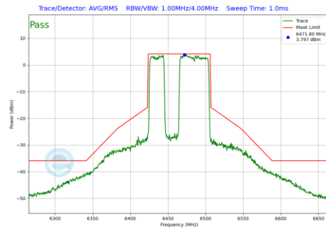
Plot 7-1038 In-Band Emission Plot CDD Primary Antenna 4a(80MHz BW 802.11be(RU) RU484+242 Index91 (UNII Band 6) - Ch.103)
