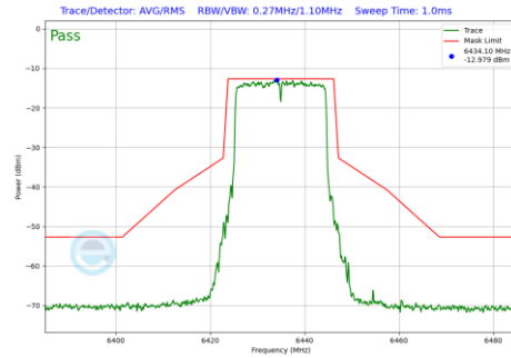
Plot 7-1143 In-Band Emission Plot SDM Primary Antenna 4a(20MHz BW 802.11be(RU) RU242 Index61 (UNII Band 6) - Ch.97)
