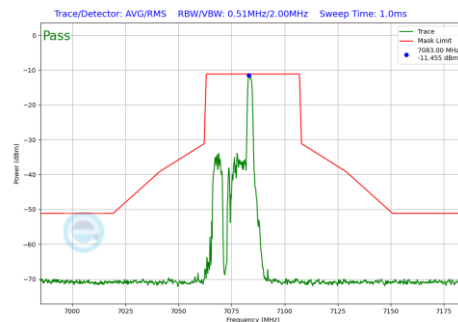
Plot 7-1080 In-Band Emission Plot SDM Primary Antenna WF5B (40MHz BW 802.11be(RU) RU26 Index8 (UNII Band 8) - Ch.227)
