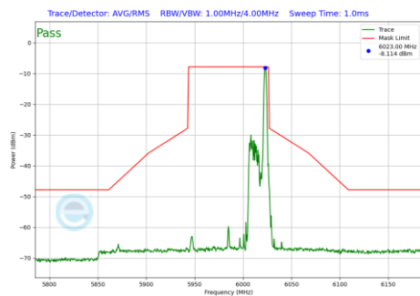
Plot 7-1069 In-Band Emission Plot SDM Primary Antenna WF5B (80MHz BW 802.11be(RU) RU26 Index36 (UNII Band 5) - Ch.7)
