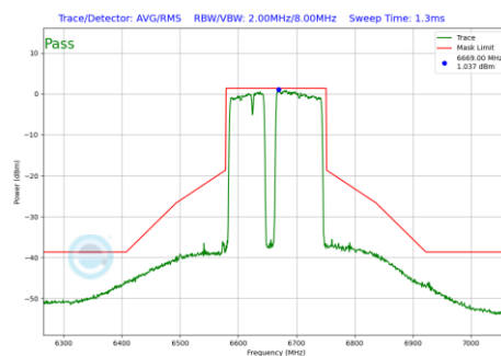
Plot 7-1196 In-Band Emission Plot CDD Diversity Antenna 4a(160MHz BW 802.11be(RU) RU996+484+242 Index99 (UNII Band 7) - Ch.143)
