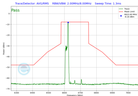
Plot 7-1094 In-Band Emission Plot SDM Primary Antenna 4a(160MHz BW 802.11be(RU) RU26 Index17 (UNII Band 7) - Ch.143)
