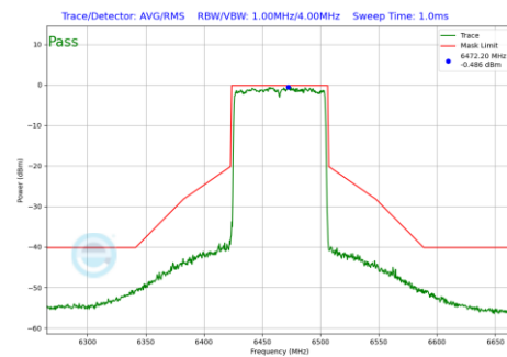
Plot 7-1203 In-Band Emission Plot CDD Diversity Antenna 2a (80MHz BW 802.11be(RU) RU996 Index67 (UNII Band 6) - Ch.103)
