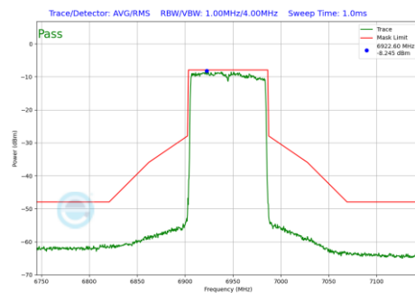
Plot 7-1137 In-Band Emission Plot SDM Primary Antenna WF5B (80MHz BW 802.11be(RU) RU996 Index67 (UNII Band 8) - Ch.199)
