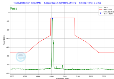
Plot 7-1098 In-Band Emission Plot SDM Primary Antenna 4a(160MHz BW 802.11be(RU) RU26 Index0 (UNII Band 8) - Ch.207)
