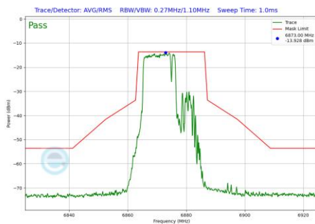
Plot 7-1117 In-Band Emission Plot SDM Primary Antenna 4a(20MHz BW 802.11be(RU) RU106+26 Index82 (UNII Band 7) - Ch.185)
