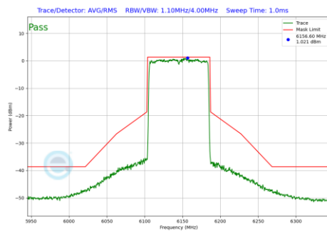
Plot 7-1199 In-Band Emission Plot CDD Diversity Antenna 2a (80MHz BW 802.11be(RU) RU996 Index67 (UNII Band 5) - Ch.39)
