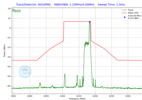
Plot 7-1157 In-Band Emission Plot CDD Diversity Antenna 2a (80MHz BW 802.11be(RU) RU26 Index36 (UNII Band 5) - Ch.39)
