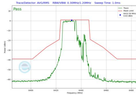
Plot 7-1191 In-Band Emission Plot CDD Diversity Antenna 4a(20MHz BW 802.11be(RU) RU106+26 Index82 (UNII Band 6) - Ch.97)
