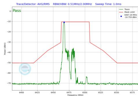
Plot 7-1072 In-Band Emission Plot SDM Primary Antenna WF5B (40MHz BW 802.11be(RU) RU26 Index0 (UNII Band 6) - Ch.107)
