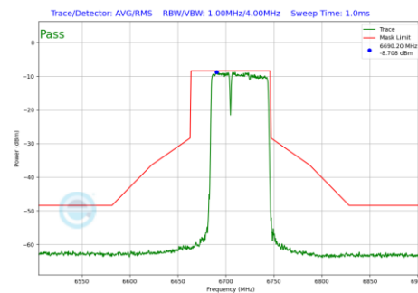
Plot 7-1106 In-Band Emission Plot SDM Primary Antenna WF5B (80MHz BW 802.11be(RU) RU484+242 Index90 (UNII Band 7) - Ch.151)
