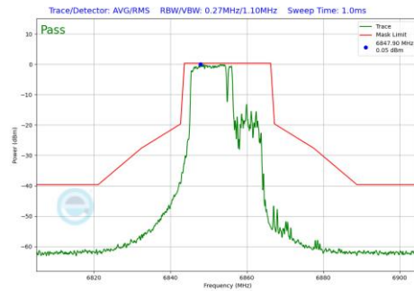
Plot 7-1040 In-Band Emission Plot CDD Primary Antenna 4a(20MHz BW 802.11be(RU) RU106+26 Index82 (UNII Band 7) - Ch.181)
