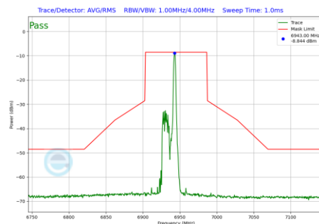
Plot 7-1081 In-Band Emission Plot SDM Primary Antenna WF5B (80MHz BW 802.11be(RU) RU26 Index17 (UNII Band 8) - Ch.199)
