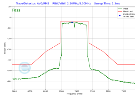
Plot 7-1154 In-Band Emission Plot SDM Primary Antenna 4a(160MHz BW 802.11be(RU) RU996X2 Index68 (UNII Band 8) - Ch.207)
