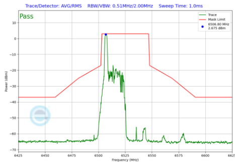
Plot 7-1172 In-Band Emission Plot CDD Diversity Antenna 4a(40MHz BW 802.11be(RU) RU26 Index0 (UNII Band 6) - Ch.115)
