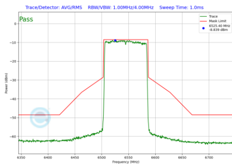
Plot 7-1133 In-Band Emission Plot SDM Primary Antenna WF5B (80MHz BW 802.11be(RU) RU996 Index67 (UNII Band 7) - Ch.119)
