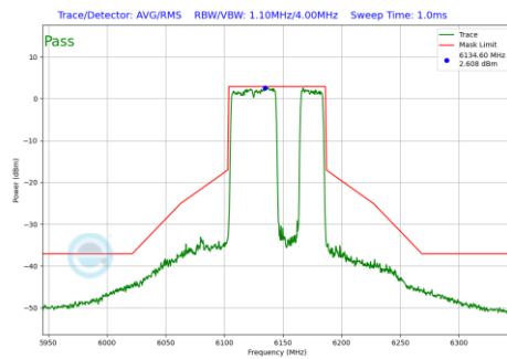
Plot 7-1180 In-Band Emission Plot CDD Diversity Antenna 2a (80MHz BW 802.11be(RU) RU484+242 Index92 (UNII Band 5) - Ch.39)
