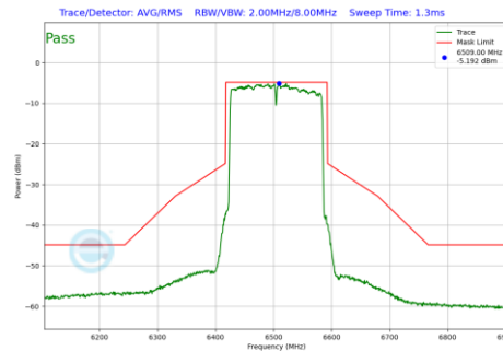
Plot 7-1146 In-Band Emission Plot SDM Primary Antenna 4a(160MHz BW 802.11be(RU) RU996X2 Index68 (UNII Band 6) - Ch.111)
