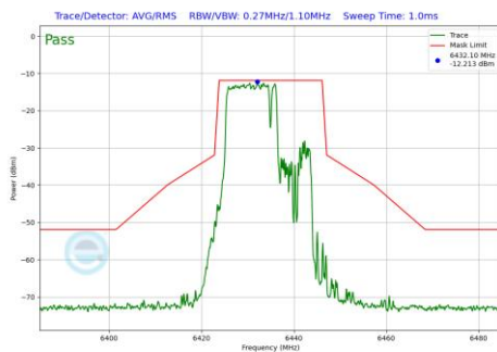
Plot 7-1102 In-Band Emission Plot SDM Primary Antenna WF5B (20MHz BW 802.11be(RU) RU106+26 Index82 (UNII Band 6) - Ch.97)
