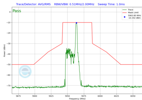
Plot 7-1084 In-Band Emission Plot SDM Primary Antenna 4a(40MHz BW 802.11be(RU) RU26 Index8 (UNII Band 5) - Ch.3)
