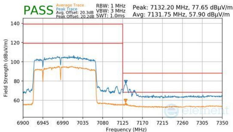
Plot 7-1583 Antenna 2a Radiated Upper Band Edge (Peak & Average – UNII Band 8) - RU996+484+242 (L)
