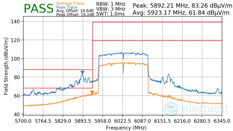
Plot 7-1591 Antenna 2a Radiated Lower Band Edge (Peak & Average – UNII Band 5) - RU996X2
