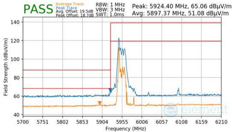
Plot 7-1611 CDD Primary Radiated Lower Band Edge (Peak & Average – UNII Band 5) - RU26
