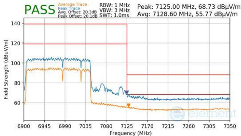
Plot 7-1652 CDD Primary Radiated Upper Band Edge (Peak & Average – UNII Band 8) - RU996+484+242 (H)
