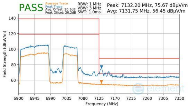
Plot 7-1572 Antenna 2a Radiated Upper Band Edge (Peak & Average – UNII Band 8) - RU996+484 (H)
