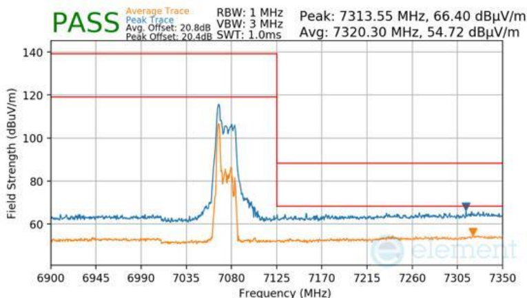
Plot 7-1669 CDD Diversity Radiated Upper Band Edge (Peak & Average – UNII Band 8) - RU26
