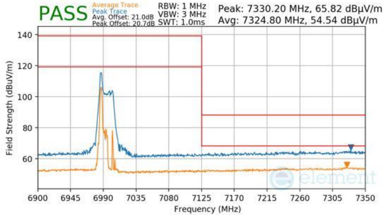
Plot 7-1627 CDD Primary Radiated Upper Band Edge (Peak & Average – UNII Band 8) - RU26
