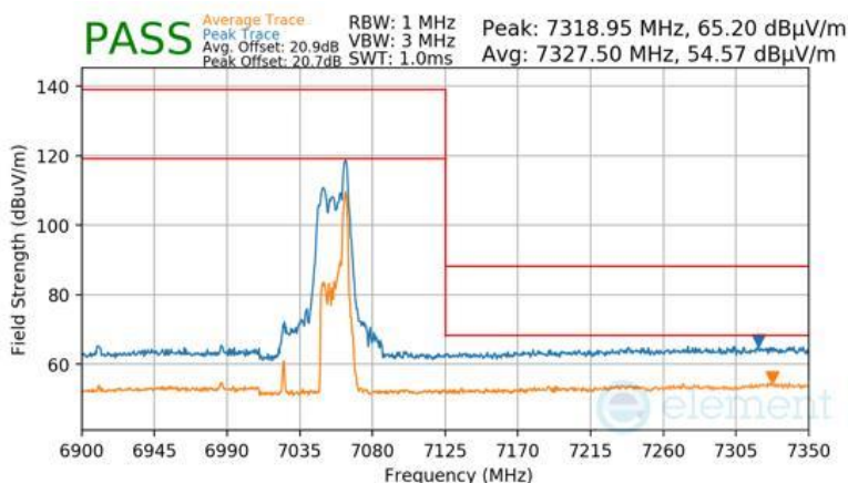
Plot 7-1676 CDD Diversity Radiated Upper Band Edge (Peak & Average – UNII Band 8) - RU26
