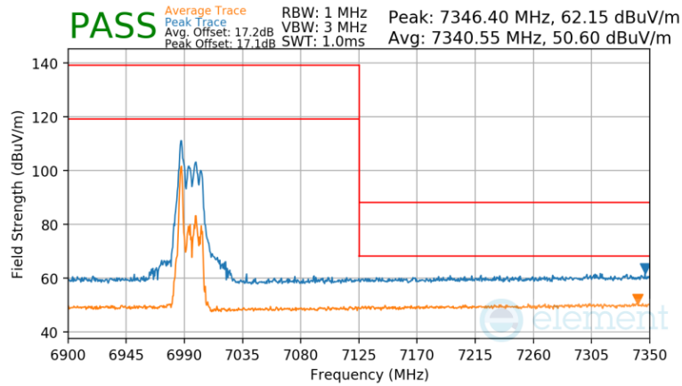
Plot 7-1689 CDD Diversity Radiated Upper Band Edge (Peak & Average – UNII Band 8) - RU26
