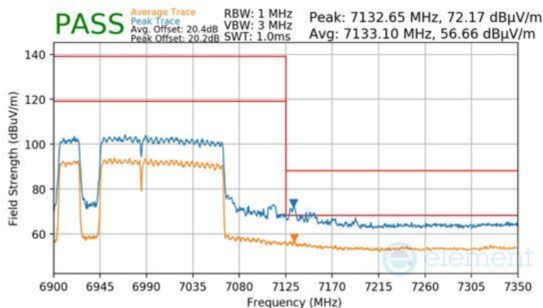
Plot 7-1647 CDD Primary Radiated Upper Band Edge (Peak & Average – UNII Band 8) - RU996+484+242 (L)
