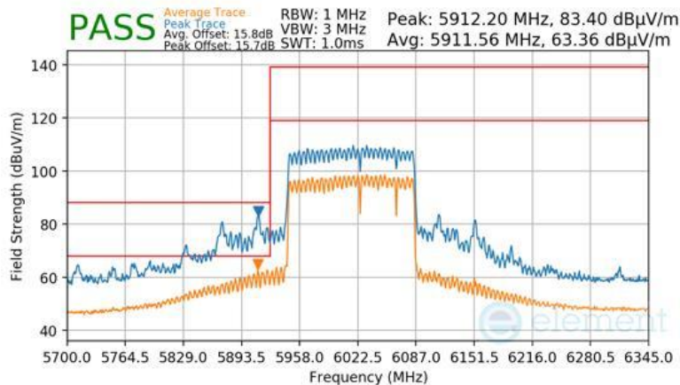
Plot 7-1644 CDD Primary Radiated Lower Band Edge (Peak & Average – UNII Band 5) - RU996+484+242 (H)
