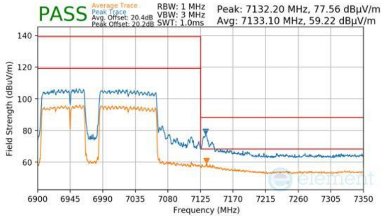
Plot 7-1651 CDD Primary Radiated Upper Band Edge (Peak & Average – UNII Band 8) - RU996+484+242 (L)
