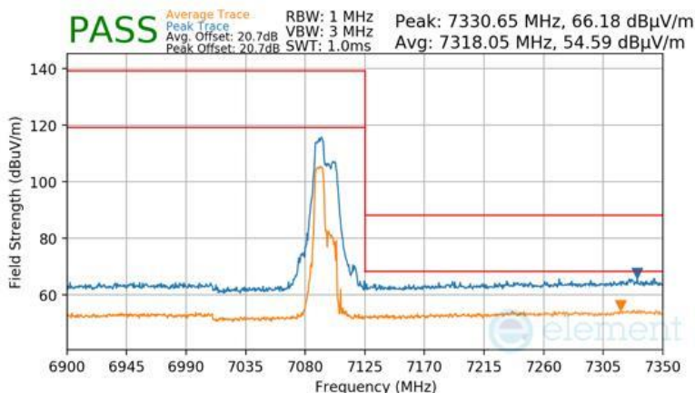
Plot 7-1599 CDD Primary Radiated Upper Band Edge (Peak & Average – UNII Band 8) - RU52+26
