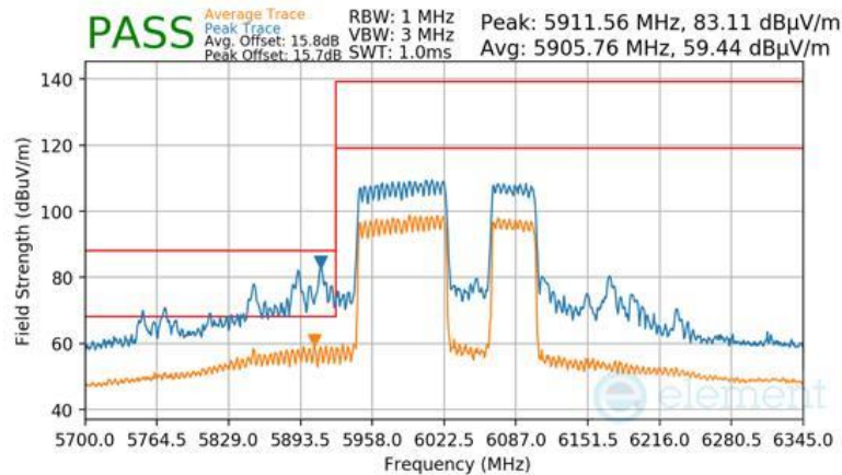
Plot 7-1630 CDD Primary Radiated Lower Band Edge (Peak & Average – UNII Band 5) - RU996+484 (H)
