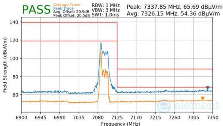
Plot 7-1657 CDD Diversity Radiated Upper Band Edge (Peak & Average – UNII Band 8) - RU26
