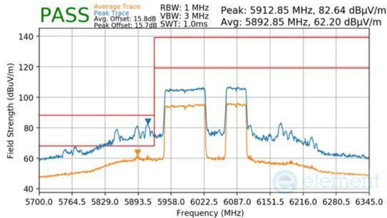
Plot 7-1568 Antenna 2a Radiated Lower Band Edge (Peak & Average – UNII Band 5) - RU996+484 (H)
