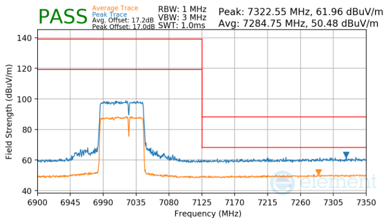
Plot 7-1560 Antenna 2a Radiated Upper Band Edge (Peak & Average – UNII Band 8) - RU484+242
