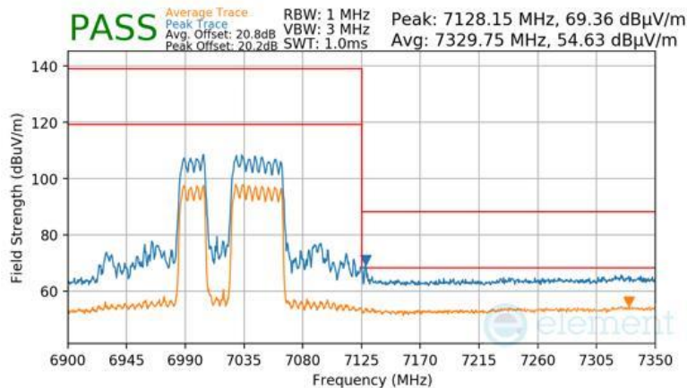
Plot 7-1682 CDD Diversity Radiated Upper Band Edge (Peak & Average – UNII Band 8) - RU484+242
