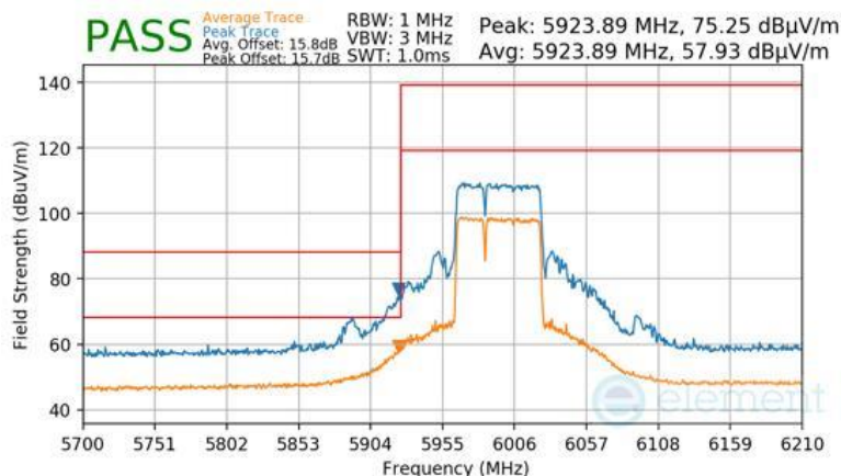
Plot 7-1553 Antenna 2a Radiated Lower Band Edge (Peak & Average – UNII Band 5) - RU484+242
