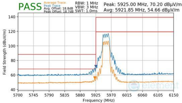
Plot 7-1601 CDD Primary Radiated Lower Band Edge (Peak & Average – UNII Band 5) - RU242
