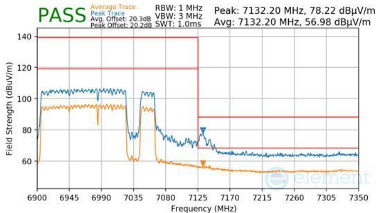
Plot 7-1650 CDD Primary Radiated Upper Band Edge (Peak & Average – UNII Band 8) - RU996+484+242 (H)
