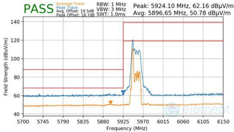
Plot 7-1655 CDD Diversity Radiated Lower Band Edge (Peak & Average – UNII Band 5) - RU26
