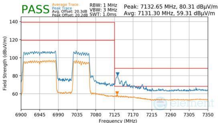
Plot 7-1634 CDD Primary Radiated Upper Band Edge (Peak & Average – UNII Band 8) - RU996+484 (H)
