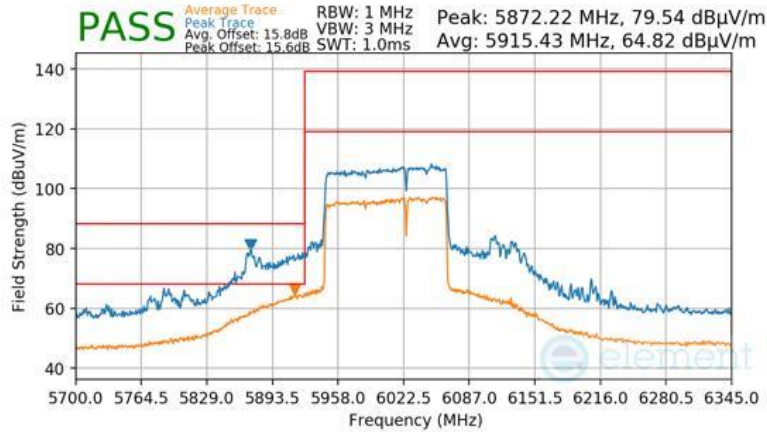
Plot 7-1569 Antenna 2a Radiated Lower Band Edge (Peak & Average – UNII Band 5) - RU996+484 (H)
