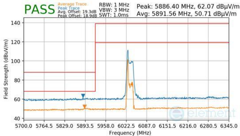
Plot 7-1563 Antenna 2a Radiated Lower Band Edge (Peak & Average – UNII Band 5) - RU26
