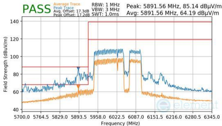
Plot 7-1640 CDD Primary Radiated Lower Band Edge (Peak & Average – UNII Band 5) - RU996+484+242 (H)
