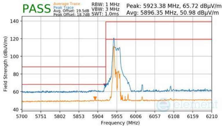
Plot 7-1673 CDD Diversity Radiated Lower Band Edge (Peak & Average – UNII Band 5) - RU26
