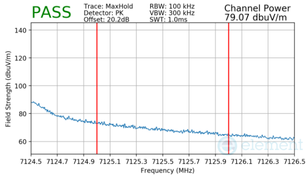
Plot 7-1603 CDD Primary Radiated Upper Band Edge (Peak – UNII Band 8)
