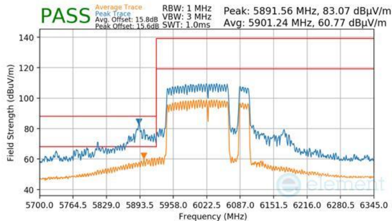
Plot 7-1642 CDD Primary Radiated Lower Band Edge (Peak & Average – UNII Band 5) - RU996+484+242 (H)
