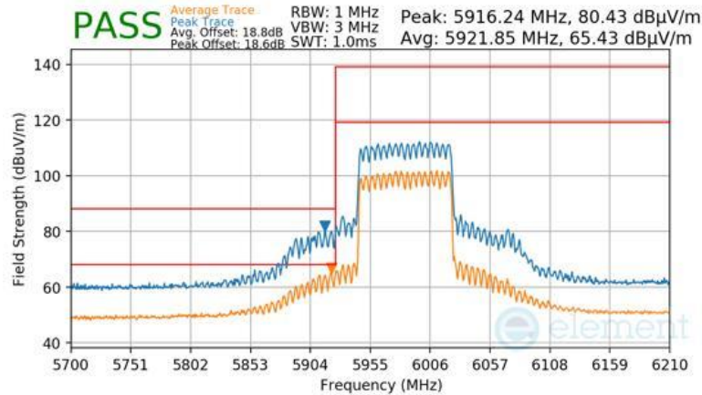
Plot 7-1623 CDD Primary Radiated Lower Band Edge (Peak & Average – UNII Band 5) - RU996
