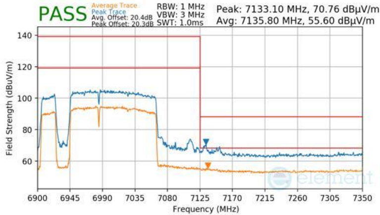
Plot 7-1585 Antenna 2a Radiated Upper Band Edge (Peak & Average – UNII Band 8) - RU996+484+242 (L)
