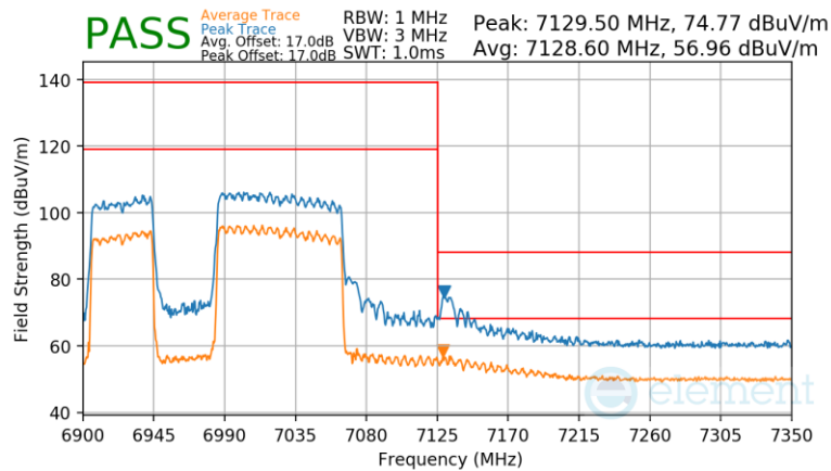
Plot 7-1698 CDD Diversity Radiated Upper Band Edge (Peak & Average – UNII Band 8) - RU996+484 (L)
