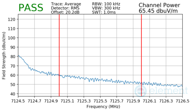
Plot 7-1666 CDD Diversity Radiated Upper Band Edge (Average – UNII Band 8)
