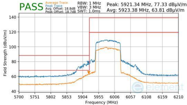
Plot 7-1561 Antenna 2a Radiated Lower Band Edge (Peak & Average – UNII Band 5) - RU996
