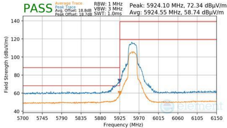
Plot 7-1663 CDD Diversity Radiated Lower Band Edge (Peak & Average – UNII Band 5) - RU242
