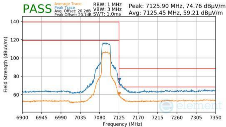
Plot 7-1602 CDD Primary Radiated Upper Band Edge (Peak & Average – UNII Band 8) - RU242
