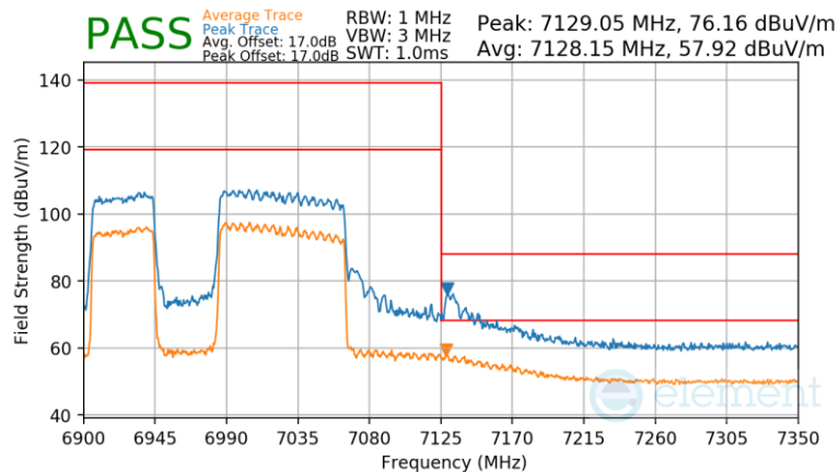
Plot 7-1636 CDD Primary Radiated Upper Band Edge (Peak & Average – UNII Band 8) - RU996+484 (L)
