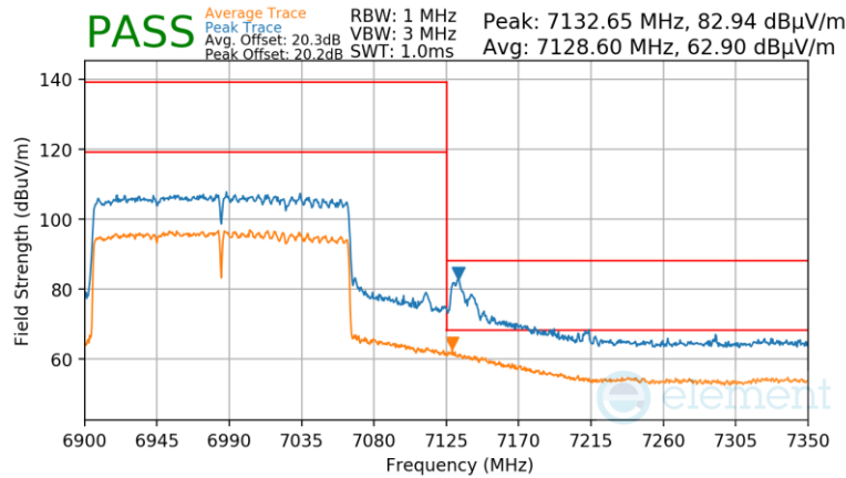
Plot 7-1654 CDD Primary Radiated Upper Band Edge (Peak & Average – UNII Band 8) - RU996X2
