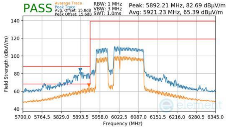
Plot 7-1641 CDD Primary Radiated Lower Band Edge (Peak & Average – UNII Band 5) - RU996+484+242 (L)
