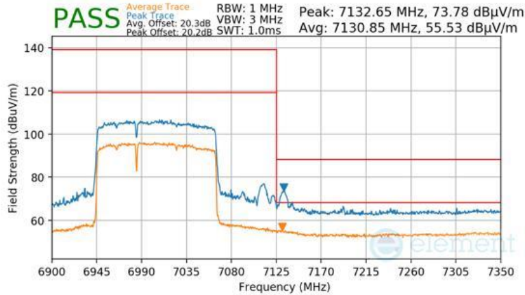
Plot 7-1571 Antenna 2a Radiated Upper Band Edge (Peak & Average – UNII Band 8) - RU996+484 (L)
