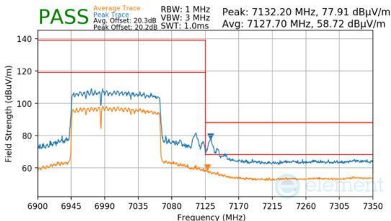
Plot 7-1633 CDD Primary Radiated Upper Band Edge (Peak & Average – UNII Band 8) - RU996+484 (L)
