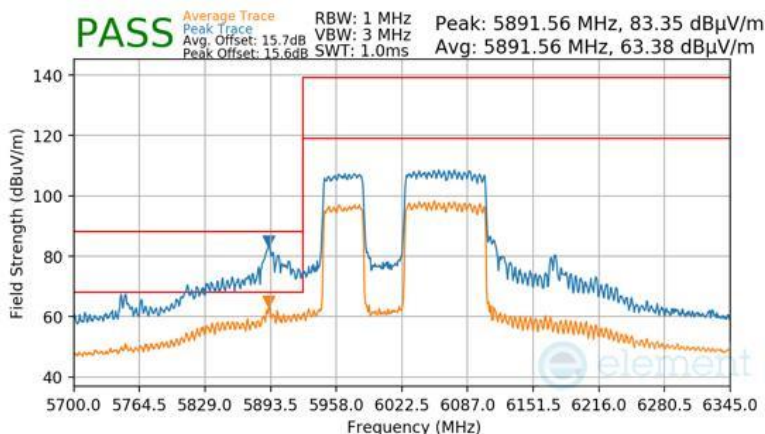
Plot 7-1694 CDD Diversity Radiated Lower Band Edge (Peak & Average – UNII Band 5) - RU996+484 (L)
