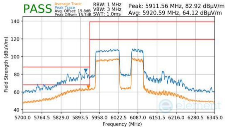
Plot 7-1692 CDD Diversity Radiated Lower Band Edge (Peak & Average – UNII Band 5) - RU996+484 (H)
