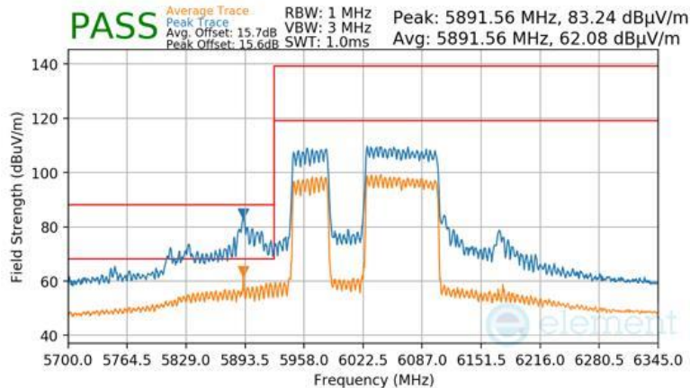
Plot 7-1632 CDD Primary Radiated Lower Band Edge (Peak & Average – UNII Band 5) - RU996+484 (L)
