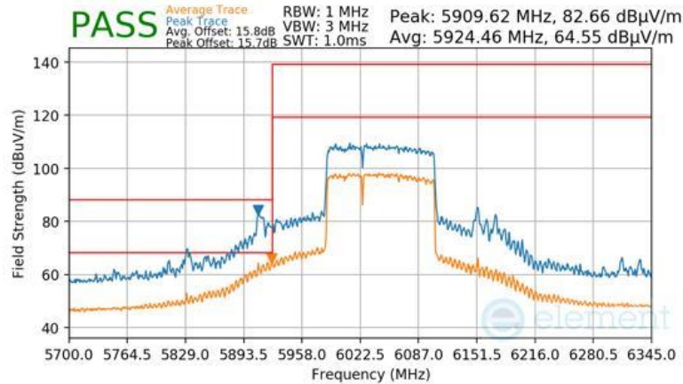
Plot 7-1691 CDD Diversity Radiated Lower Band Edge (Peak & Average – UNII Band 5) - RU996+484 (L)
