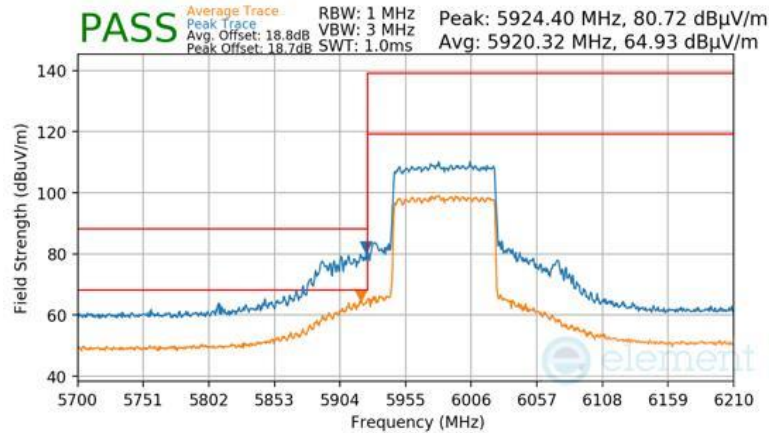
Plot 7-1685 CDD Diversity Radiated Lower Band Edge (Peak & Average – UNII Band 5) - RU996
