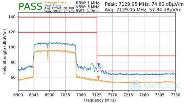
Plot 7-1695 CDD Diversity Radiated Upper Band Edge (Peak & Average – UNII Band 8) - RU996+484 (L)
