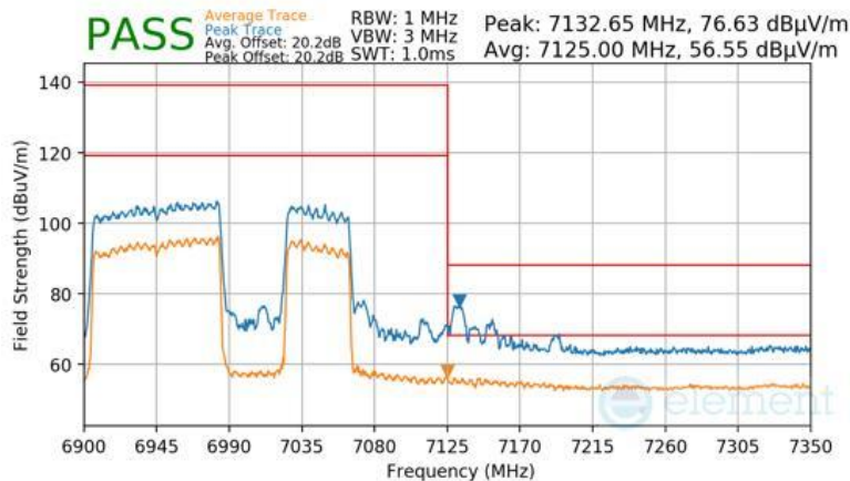
Plot 7-1696 CDD Diversity Radiated Upper Band Edge (Peak & Average – UNII Band 8) - RU996+484 (H)
