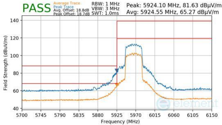
Plot 7-1671 CDD Diversity Radiated Lower Band Edge (Peak & Average – UNII Band 5) - RU484
