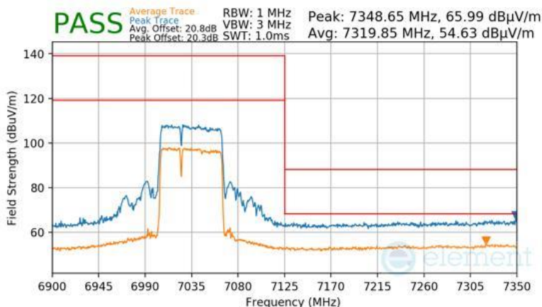
Plot 7-1557 Antenna 2a Radiated Upper Band Edge (Peak & Average – UNII Band 8) - RU484+242
