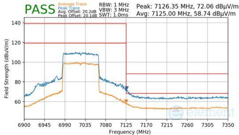
Plot 7-1562 Antenna 2a Radiated Upper Band Edge (Peak & Average – UNII Band 8) - RU996
