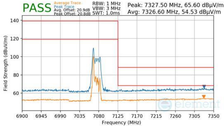
Plot 7-1607 CDD Primary Radiated Upper Band Edge (Peak & Average – UNII Band 8) - RU26
