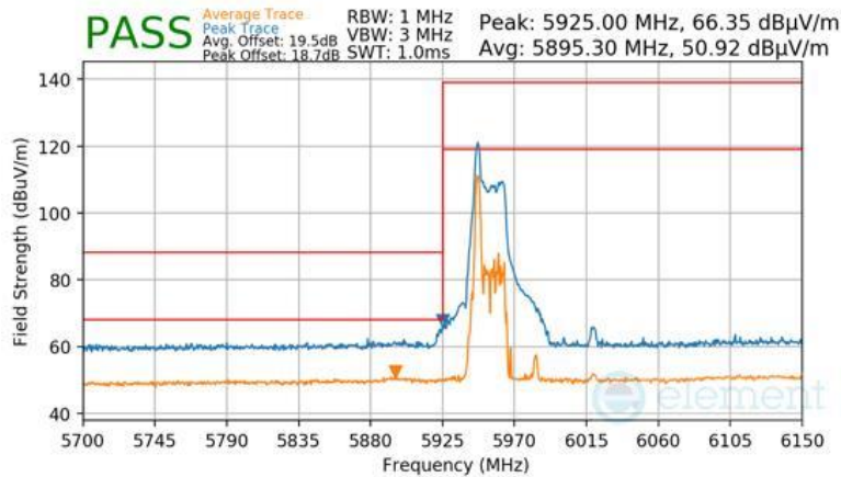
Plot 7-1667 CDD Diversity Radiated Lower Band Edge (Peak & Average – UNII Band 5) - RU26
