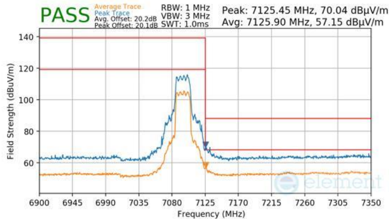
Plot 7-1664 CDD Diversity Radiated Upper Band Edge (Peak & Average – UNII Band 8) - RU242
