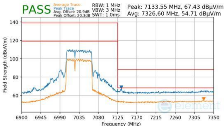
Plot 7-1619 CDD Primary Radiated Upper Band Edge (Peak & Average – UNII Band 8) - RU484+242
