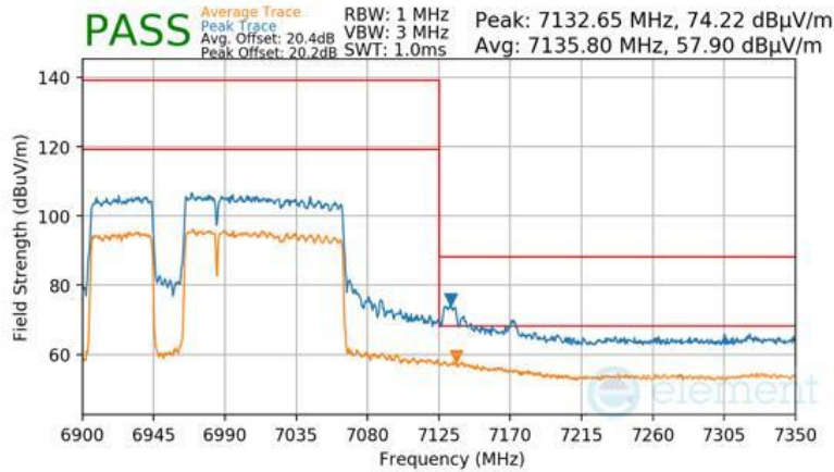
Plot 7-1649 CDD Primary Radiated Upper Band Edge (Peak & Average – UNII Band 8) - RU996+484+242 (L)
