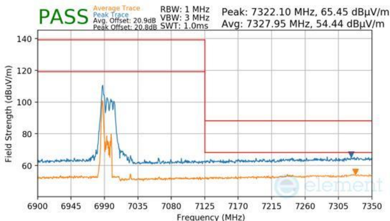
Plot 7-1675 CDD Diversity Radiated Upper Band Edge (Peak & Average – UNII Band 8) - RU26
