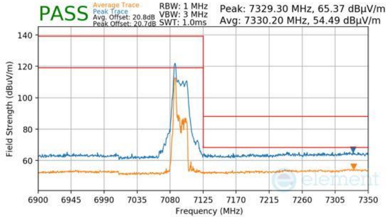
Plot 7-1595 CDD Primary Radiated Upper Band Edge (Peak & Average – UNII Band 8) - RU26
