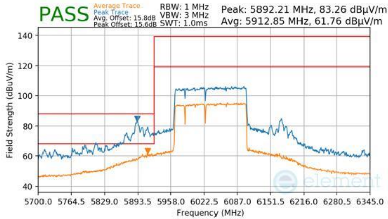
Plot 7-1575 Antenna 2a Radiated Lower Band Edge (Peak & Average – UNII Band 5) - RU996+484+242 (L)
