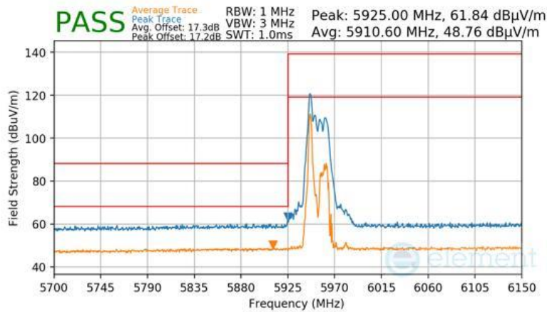
Plot 7-1593 CDD Primary Radiated Lower Band Edge (Peak & Average – UNII Band 5) - RU26
