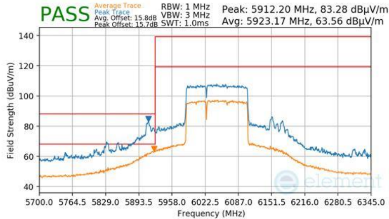
Plot 7-1567 Antenna 2a Radiated Lower Band Edge (Peak & Average – UNII Band 5) - RU996+484 (L)
