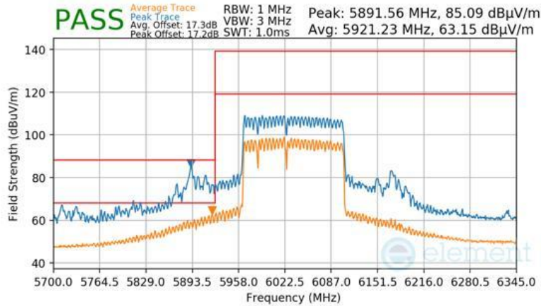
Plot 7-1637 CDD Primary Radiated Lower Band Edge (Peak & Average – UNII Band 5) - RU996+484+242 (L)
