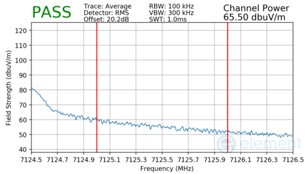
Plot 7-1604 CDD Primary Radiated Upper Band Edge (Average – UNII Band 8)
