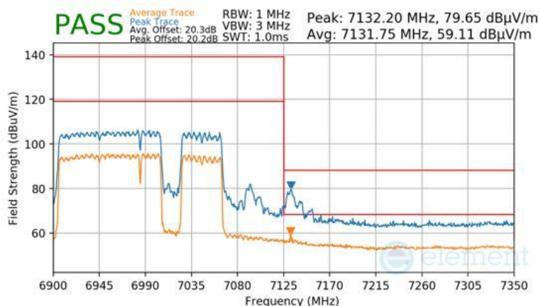
Plot 7-1648 CDD Primary Radiated Upper Band Edge (Peak & Average – UNII Band 8) - RU996+484+242 (H)
