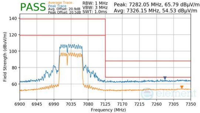
Plot 7-1681 CDD Diversity Radiated Upper Band Edge (Peak & Average – UNII Band 8) - RU484+242
