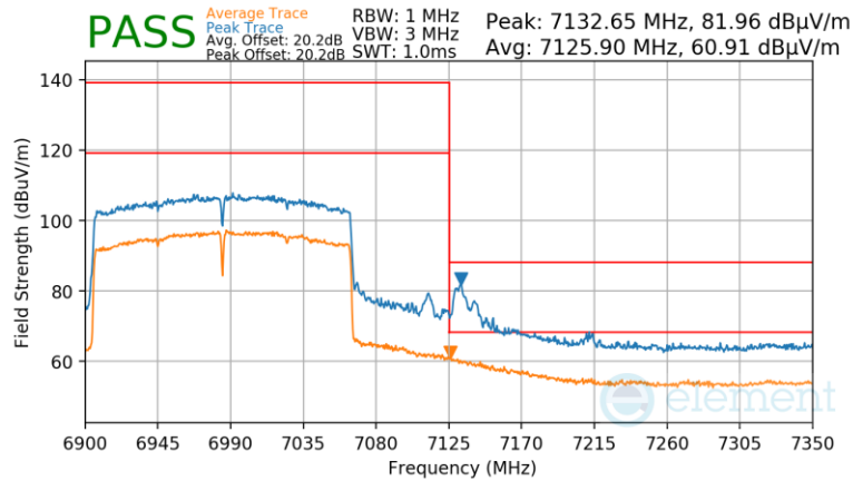
Plot 7-1592 Antenna 2a Radiated Upper Band Edge (Peak & Average – UNII Band 8) - RU996X2
