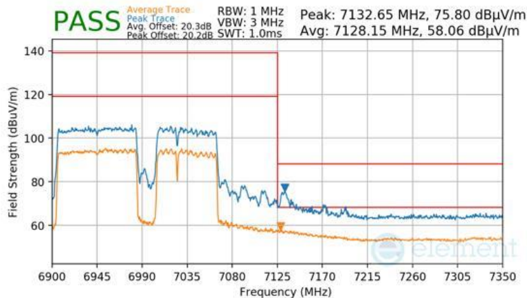
Plot 7-1646 CDD Primary Radiated Upper Band Edge (Peak & Average – UNII Band 8) - RU996+484+242 (H)
