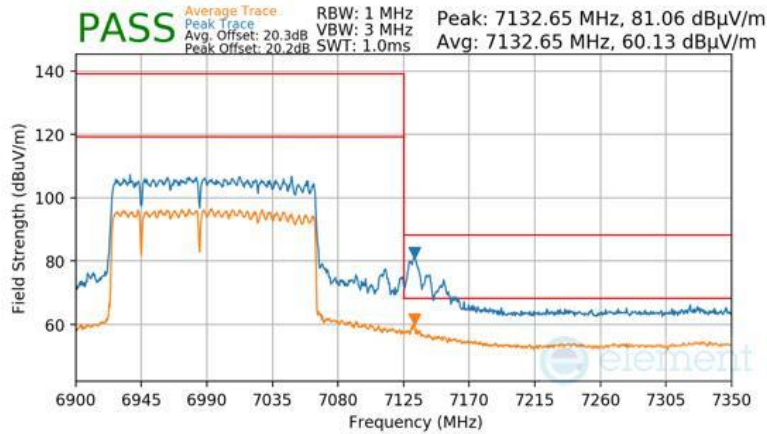
Plot 7-1645 CDD Primary Radiated Upper Band Edge (Peak & Average – UNII Band 8) - RU996+484+242 (L)
