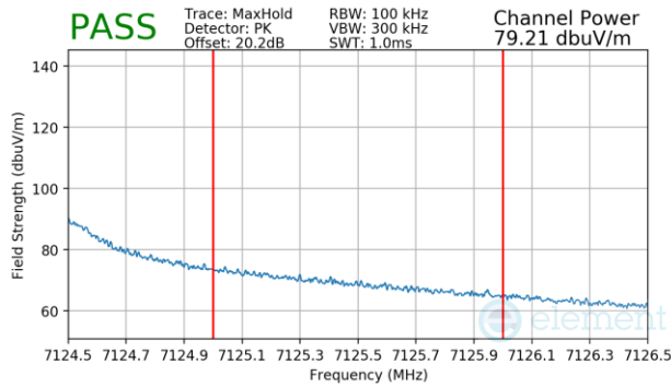
Plot 7-1665 CDD Diversity Radiated Upper Band Edge (Peak – UNII Band 8)
