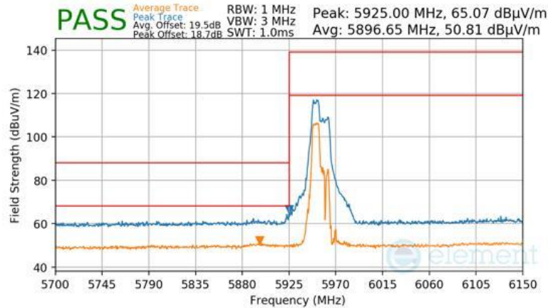
Plot 7-1659 CDD Diversity Radiated Lower Band Edge (Peak & Average – UNII Band 5) - RU52+26
