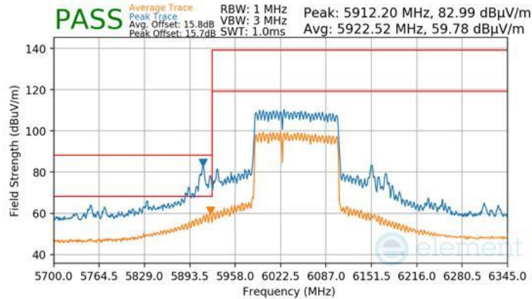
Plot 7-1629 CDD Primary Radiated Lower Band Edge (Peak & Average – UNII Band 5) - RU996+484 (L)
