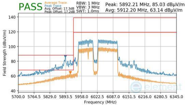
Plot 7-1643 CDD Primary Radiated Lower Band Edge (Peak & Average – UNII Band 5) - RU996+484+242 (L)
