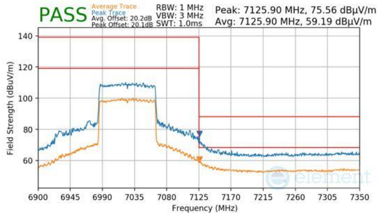
Plot 7-1686 CDD Diversity Radiated Upper Band Edge (Peak & Average – UNII Band 8) - RU996
