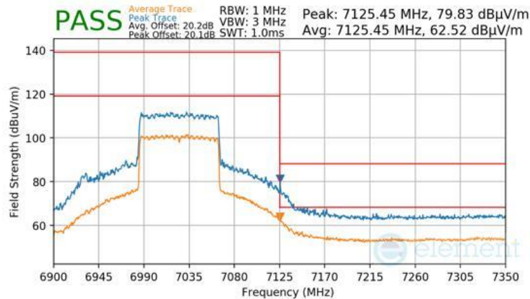
Plot 7-1624 CDD Primary Radiated Upper Band Edge (Peak & Average – UNII Band 8) - RU996
