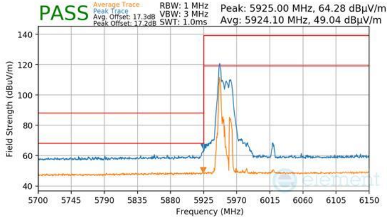
Plot 7-1605 CDD Primary Radiated Lower Band Edge (Peak & Average – UNII Band 5) - RU26
