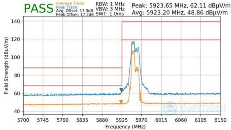
Plot 7-1597 CDD Primary Radiated Lower Band Edge (Peak & Average – UNII Band 5) - RU52+26
