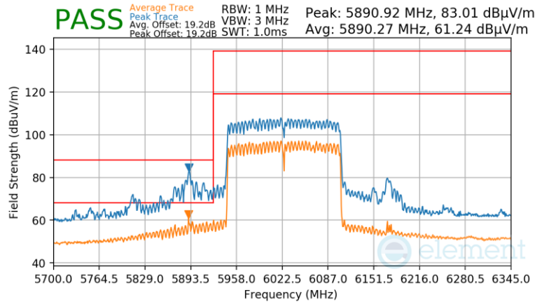
Plot 7-1653 CDD Primary Radiated Lower Band Edge (Peak & Average – UNII Band 5) - RU996X2
