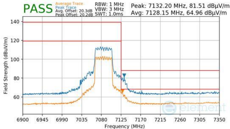
Plot 7-1672 CDD Diversity Radiated Upper Band Edge (Peak & Average – UNII Band 8) - RU484
