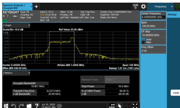
Plot 7-156 26dB BW & 99% OBW Antenna 2a (40MHz BW 802.11be(RU) RU26 Index8 - Ch.91)
