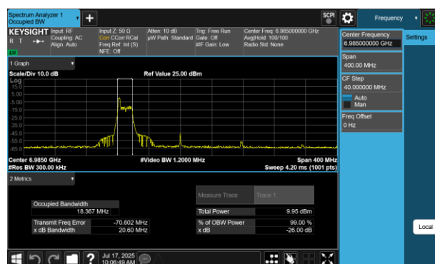
Plot 7-147 26dB BW & 99% OBW Antenna 4a(160MHz BW 802.11be(RU) RU26 Index0 - Ch.207)
