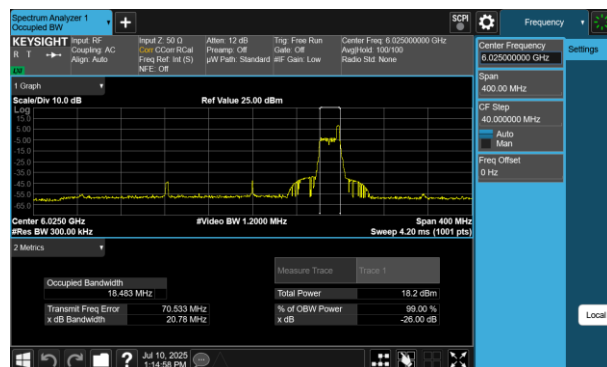
Plot 7-158 26dB BW & 99% OBW Antenna 2a (160MHz BW 802.11be(RU) RU26 Index36 - Ch.15)
