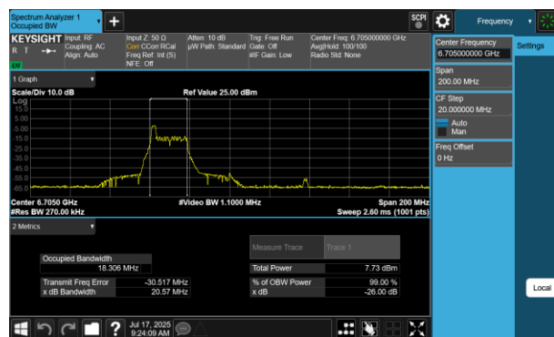
Plot 7-135 26dB BW & 99% OBW Antenna 4a(80MHz BW 802.11be(RU) RU26 Index0 - Ch.151)
