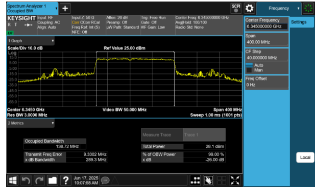
Plot 7-161 26dB BW & 99% OBW Antenna 2a (160MHz BW 802.11be(RU) RU996+484+242 Index96 - Ch.79)
