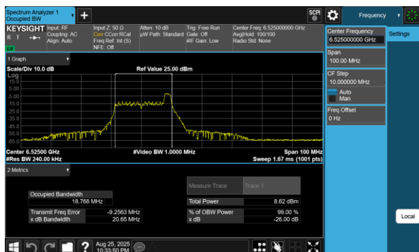
Plot 7-123 26dB BW & 99% OBW Antenna 4a(40MHz BW 802.11be(RU) RU26 Index8 - Ch.115)
