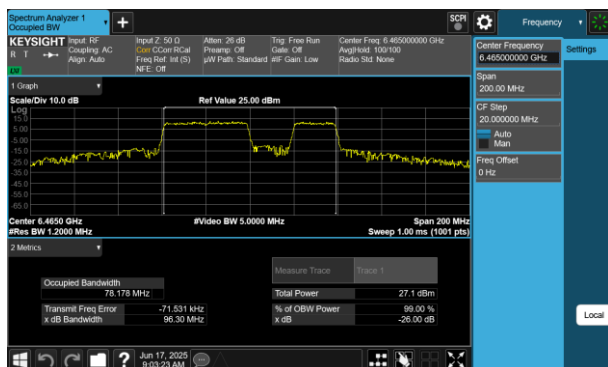
Plot 7-171 26dB BW & 99% OBW Antenna 2a (80MHz BW 802.11be(RU) RU484+242 Index92 - Ch.103)
