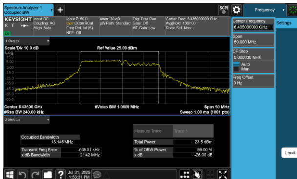
Plot 7-170 26dB BW & 99% OBW Antenna 2a (20MHz BW 802.11be(RU) RU106+26 Index82 - Ch.97)
