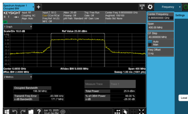
Plot 7-143 26dB BW & 99% OBW Antenna 4a(160MHz BW 802.11be(RU) RU996X2 Index68 - Ch.143)
