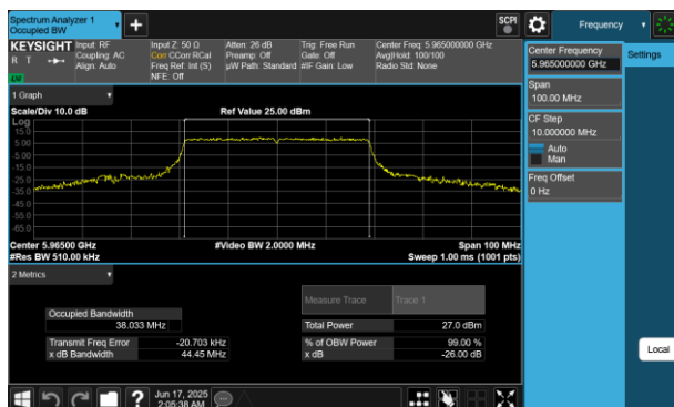
Plot 7-163 26dB BW & 99% OBW Antenna 2a (40MHz BW 802.11be(RU) RU484 Index65 - Ch.3)
