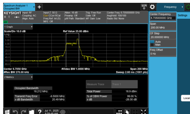
Plot 7-102 26dB BW & 99% OBW Antenna 4a(80MHz BW 802.11be(RU) RU26 Index17 - Ch.151)
