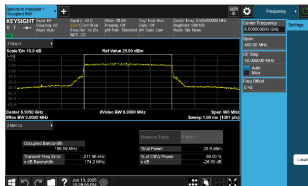
Plot 7-132 26dB BW & 99% OBW Antenna 4a(160MHz BW 802.11be(RU) RU996X2 Index68 - Ch.111)
