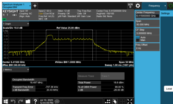
Plot 7-155 26dB BW & 99% OBW Antenna 2a (20MHz BW 802.11be(RU) RU26 Index0 - Ch.93)
