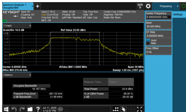
Plot 7-104 26dB BW & 99% OBW Antenna 4a(20MHz BW 802.11be(RU) RU106+26 Index82 - Ch.149)
