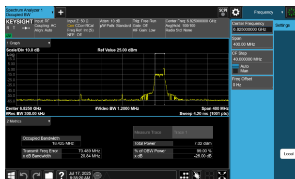
Plot 7-136 26dB BW & 99% OBW Antenna 4a(160MHz BW 802.11be(RU) RU26 Index36 - Ch.175)
