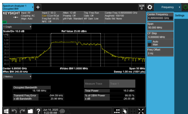
Plot 7-148 26dB BW & 99% OBW Antenna 4a(20MHz BW 802.11be(RU) RU106+26 Index82 - Ch.189)
