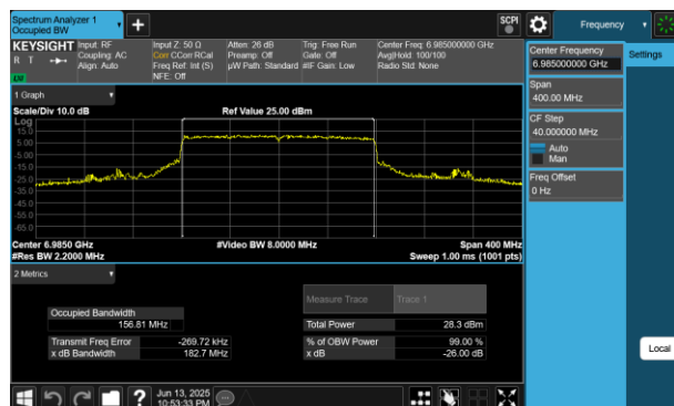
Plot 7-154 26dB BW & 99% OBW Antenna 4a(160MHz BW 802.11be(RU) RU996X2 Index68 - Ch.207)
