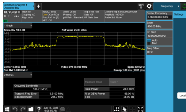
Plot 7-106 26dB BW & 99% OBW Antenna 4a(160MHz BW 802.11be(RU) RU996+484+242 Index96 - Ch.143)
