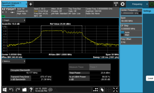
Plot 7-159 26dB BW & 99% OBW Antenna 2a (20MHz BW 802.11be(RU) RU106+26 Index82 - Ch.1)
