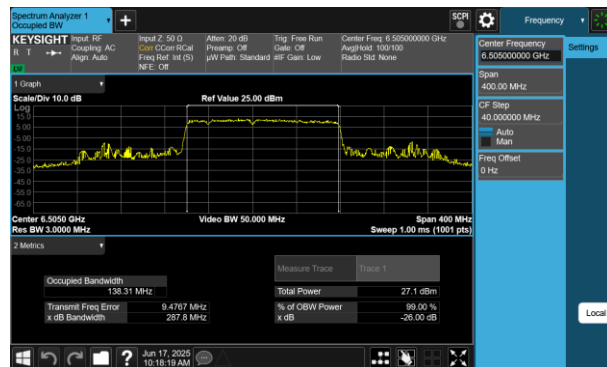
Plot 7-172 26dB BW & 99% OBW Antenna 2a (160MHz BW 802.11be(RU) RU996+484+242 Index96 - Ch.111)
