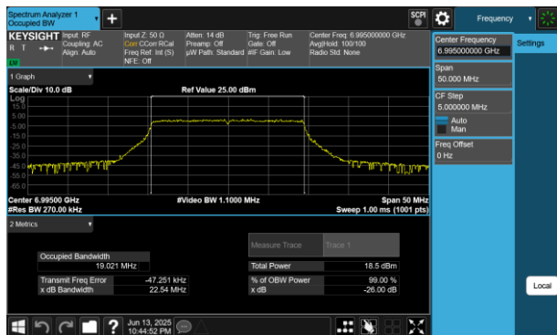
Plot 7-151 26dB BW & 99% OBW Antenna 4a(20MHz BW 802.11be(RU) RU242 Index61 - Ch.209)
