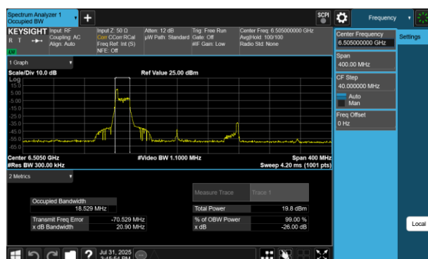
Plot 7-92 26dB BW & 99% OBW Antenna 4a(160MHz BW 802.11be(RU) RU26 Index0 - Ch.111)
