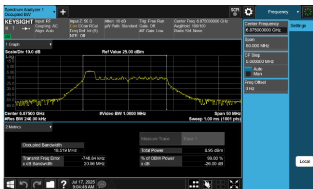
Plot 7-133 26dB BW & 99% OBW Antenna 4a(20MHz BW 802.11be(RU) RU26 Index0 - Ch.185)
