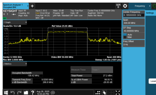
Plot 7-117 26dB BW & 99% OBW Antenna 4a(160MHz BW 802.11be(RU) RU996+484+242 Index96 - Ch.47)
