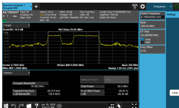
Plot 7-105 26dB BW & 99% OBW Antenna 4a(80MHz BW 802.11be(RU) RU484+242 Index91 - Ch.167)
