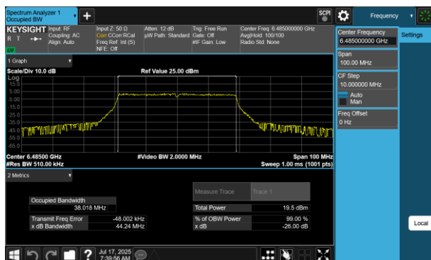
Plot 7-130 26dB BW & 99% OBW Antenna 4a(40MHz BW 802.11be(RU) RU484 Index65 - Ch.107)
