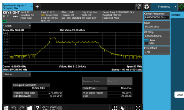
Plot 7-100 26dB BW & 99% OBW Antenna 4a(20MHz BW 802.11be(RU) RU26 Index0 - Ch.149)
