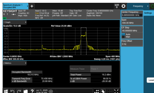
Plot 7-103 26dB BW & 99% OBW Antenna 4a(160MHz BW 802.11be(RU) RU26 Index36 - Ch.143)
