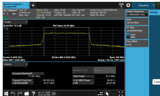
Plot 7-131 26dB BW & 99% OBW Antenna 4a(80MHz BW 802.11be(RU) RU996 Index67 - Ch.103)
