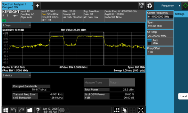
Plot 7-160 26dB BW & 99% OBW Antenna 2a (80MHz BW 802.11be(RU) RU484+242 Index91 - Ch.39)
