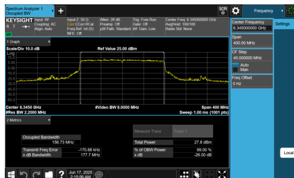
Plot 7-165 26dB BW & 99% OBW Antenna 2a (160MHz BW 802.11be(RU) RU996X2 Index68 - Ch.79)
