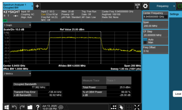
Plot 7-153 26dB BW & 99% OBW Antenna 4a(80MHz BW 802.11be(RU) RU996 Index67 - Ch.199)
