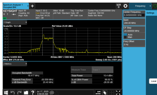
Plot 7-146 26dB BW & 99% OBW Antenna 4a(80MHz BW 802.11be(RU) RU26 Index0 - Ch.199)
