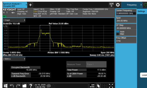
Plot 7-157 26dB BW & 99% OBW Antenna 2a (80MHz BW 802.11be(RU) RU26 Index0 - Ch.7)
