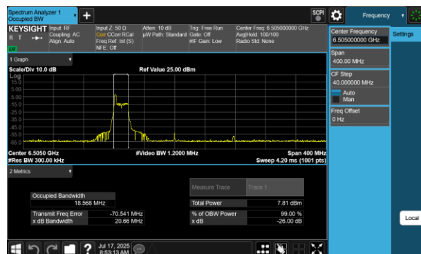
Plot 7-125 26dB BW & 99% OBW Antenna 4a(160MHz BW 802.11be(RU) RU26 Index0 - Ch.111)
