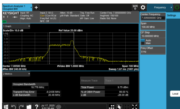
Plot 7-145 26dB BW & 99% OBW Antenna 4a(40MHz BW 802.11be(RU) RU26 Index8 - Ch.211)
