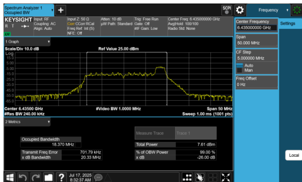
Plot 7-122 26dB BW & 99% OBW Antenna 4a(20MHz BW 802.11be(RU) RU26 Index8 - Ch.97)
