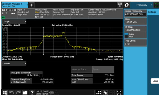
Plot 7-178 26dB BW & 99% OBW Antenna 2a (40MHz BW 802.11be(RU) RU26 Index8 - Ch.155)
