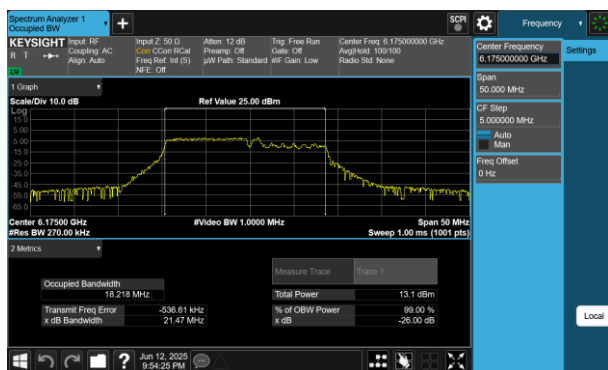
Plot 7-192 26dB BW & 99% OBW Antenna 2a (20MHz BW 802.11be(RU) RU106+26 Index82 - Ch.45)
