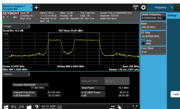
Plot 7-215 26dB BW & 99% OBW Antenna 2a (80MHz BW 802.11be(RU) RU484+242 Index91 - Ch.119)
