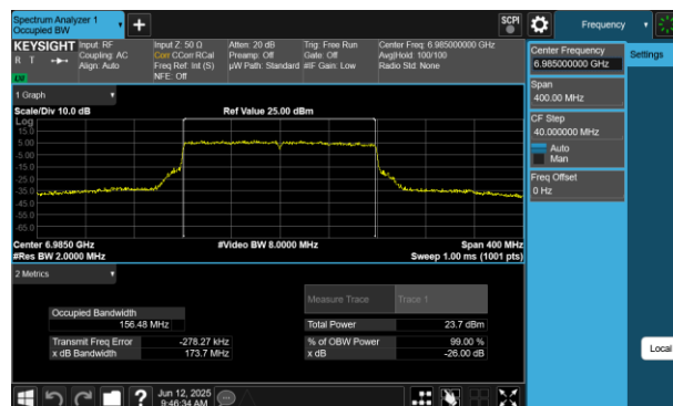
Plot 7-231 26dB BW & 99% OBW Antenna 2a (160MHz BW 802.11be(RU) RU996X2 Index68 - Ch.207)
