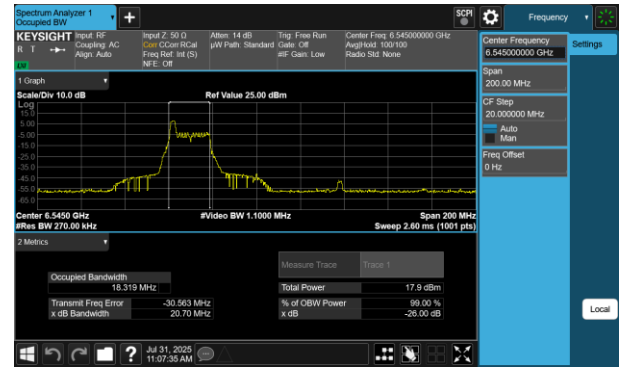
Plot 7-179 26dB BW & 99% OBW Antenna 2a (80MHz BW 802.11be(RU) RU26 Index0 - Ch.119)
