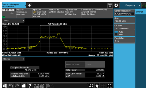
Plot 7-211 26dB BW & 99% OBW Antenna 2a (40MHz BW 802.11be(RU) RU26 Index8 - Ch.155)
