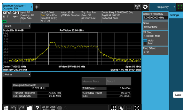
Plot 7-221 26dB BW & 99% OBW Antenna 2a (20MHz BW 802.11be(RU) RU26 Index0 - Ch.229)
