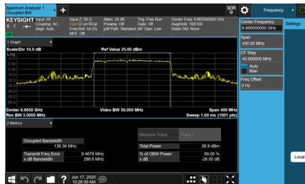
Plot 7-183 26dB BW & 99% OBW Antenna 2a (160MHz BW 802.11be(RU) RU996+484+242 Index96 - Ch.143)
