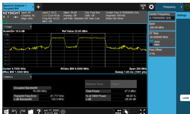
Plot 7-182 26dB BW & 99% OBW Antenna 2a (80MHz BW 802.11be(RU) RU484+242 Index91 - Ch.151)
