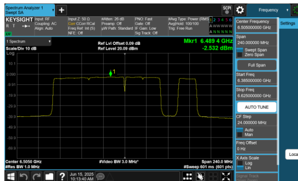
Plot 7-249 PSD Antenna WF5B (160MHz BW 802.11be(RU) RU996+484+242 Index98 - Ch.111)
