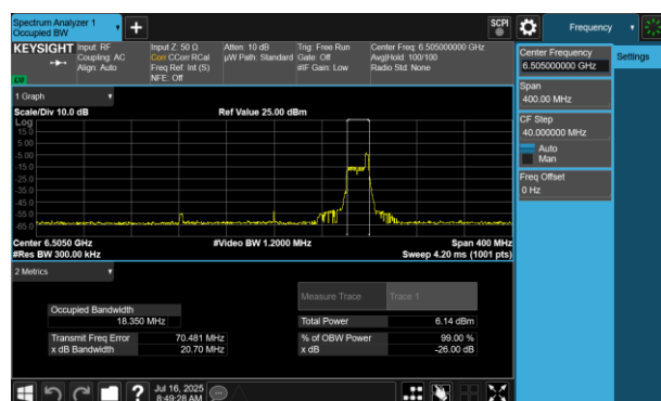
Plot 7-202 26dB BW & 99% OBW Antenna 2a (160MHz BW 802.11be(RU) RU26 Index36 - Ch.111)
