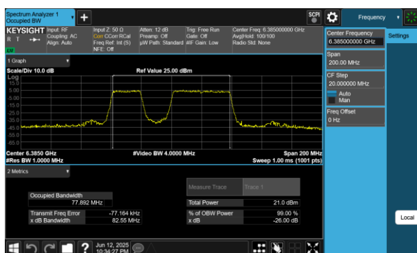
Plot 7-193 26dB BW & 99% OBW Antenna 2a (80MHz BW 802.11be(RU) RU484+242 Index91 - Ch.87)
