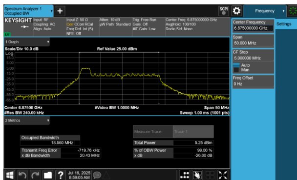
Plot 7-210 26dB BW & 99% OBW Antenna 2a (20MHz BW 802.11be(RU) RU26 Index0 - Ch.185)
