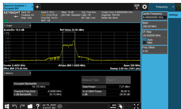
Plot 7-201 26dB BW & 99% OBW Antenna 2a (80MHz BW 802.11be(RU) RU26 Index17 - Ch.103)
