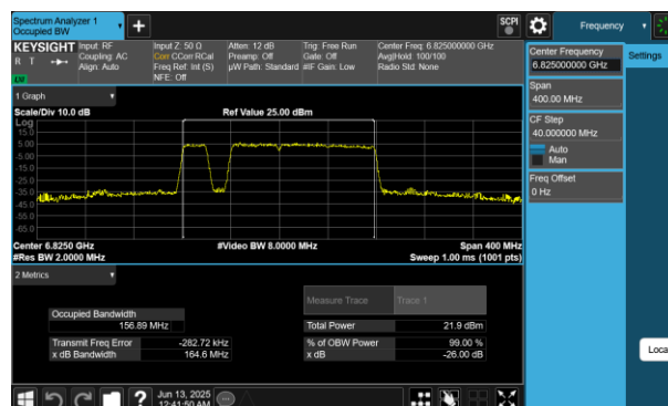
Plot 7-216 26dB BW & 99% OBW Antenna 2a (160MHz BW 802.11be(RU) RU996+484+242 Index97 - Ch.175)
