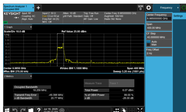
Plot 7-224 26dB BW & 99% OBW Antenna 2a (160MHz BW 802.11be(RU) RU26 Index17 - Ch.207)
