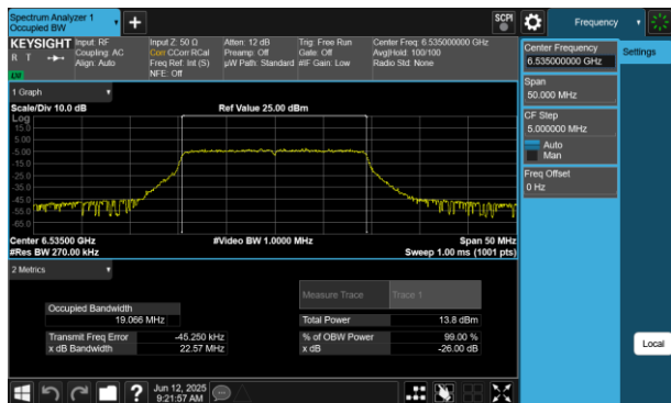
Plot 7-217 26dB BW & 99% OBW Antenna 2a (20MHz BW 802.11be(RU) RU242 Index61 - Ch.117)
