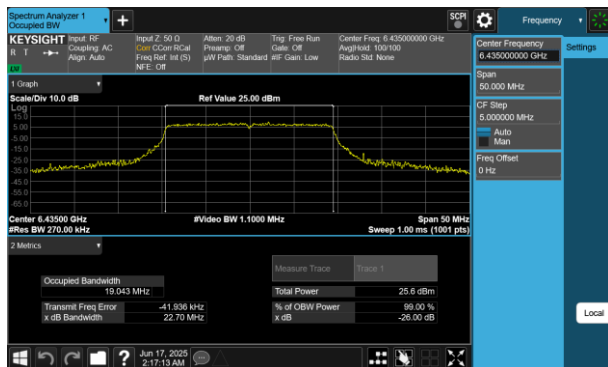
Plot 7-173 26dB BW & 99% OBW Antenna 2a (20MHz BW 802.11be(RU) RU242 Index61 - Ch.97)
