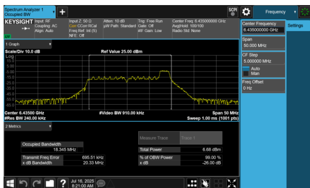
Plot 7-199 26dB BW & 99% OBW Antenna 2a (20MHz BW 802.11be(RU) RU26 Index8 - Ch.97)
