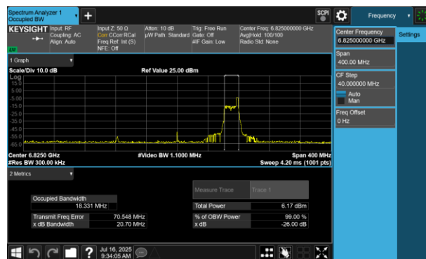
Plot 7-213 26dB BW & 99% OBW Antenna 2a (160MHz BW 802.11be(RU) RU26 Index36 - Ch.175)
