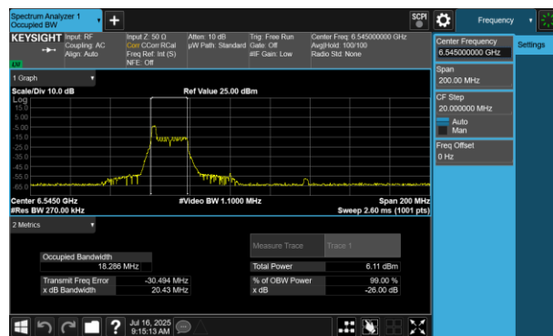
Plot 7-212 26dB BW & 99% OBW Antenna 2a (80MHz BW 802.11be(RU) RU26 Index0 - Ch.119)
