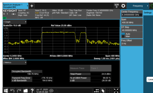
Plot 7-194 26dB BW & 99% OBW Antenna 2a (160MHz BW 802.11be(RU) RU996+484+242 Index98 - Ch.79)
