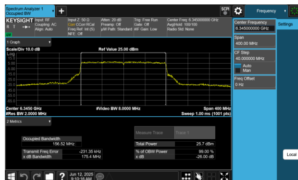
Plot 7-198 26dB BW & 99% OBW Antenna 2a (160MHz BW 802.11be(RU) RU996X2 Index68 - Ch.79)
