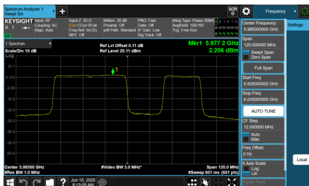
Plot 7-237 PSD Antenna WF5B (80MHz BW 802.11be(RU) RU484+242 Index92 - Ch.7)
