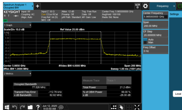
Plot 7-197 26dB BW & 99% OBW Antenna 2a (80MHz BW 802.11be(RU) RU996 Index67 - Ch.7)
