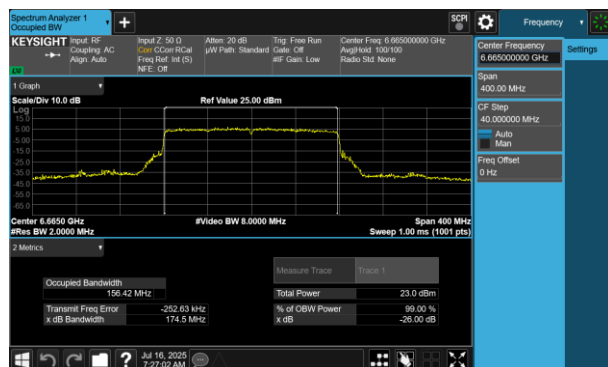
Plot 7-220 26dB BW & 99% OBW Antenna 2a (160MHz BW 802.11be(RU) RU996X2 Index68 - Ch.143)
