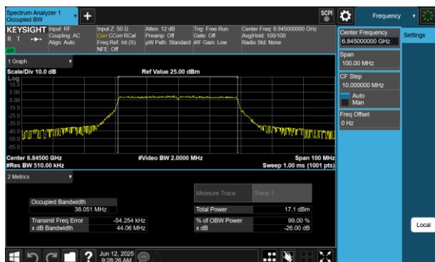
Plot 7-218 26dB BW & 99% OBW Antenna 2a (40MHz BW 802.11be(RU) RU484 Index65 - Ch.179)
