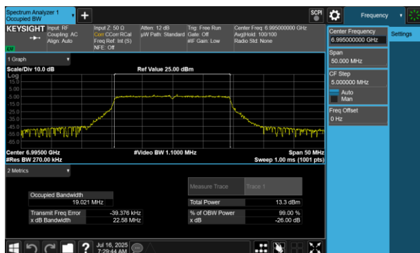
Plot 7-229 26dB BW & 99% OBW Antenna 2a (20MHz BW 802.11be(RU) RU242 Index61 - Ch.209)
