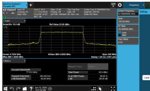
Plot 7-219 26dB BW & 99% OBW Antenna 2a (80MHz BW 802.11be(RU) RU996 Index67 - Ch.151)
