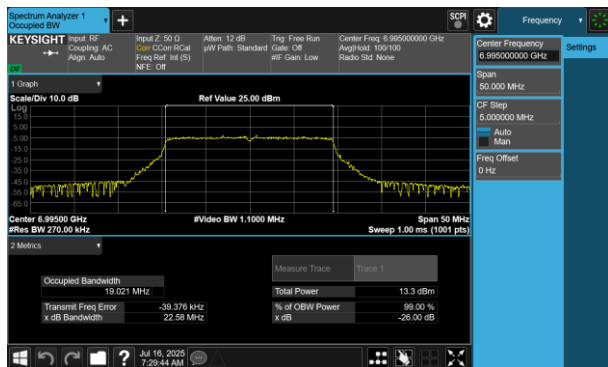
Plot 7-228 26dB BW & 99% OBW Antenna 2a (20MHz BW 802.11be(RU) RU242 Index61 - Ch.209)
