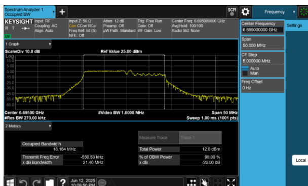
Plot 7-214 26dB BW & 99% OBW Antenna 2a (20MHz BW 802.11be(RU) RU106+26 Index82 - Ch.149)
