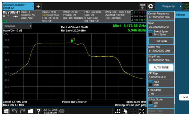
Plot 7-236 PSD Antenna WF5B (20MHz BW 802.11be(RU) RU106+26 Index82 - Ch.45)
