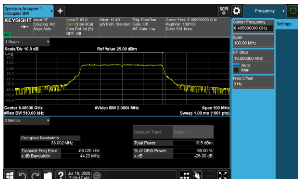
Plot 7-196 26dB BW & 99% OBW Antenna 2a (40MHz BW 802.11be(RU) RU484 Index65 - Ch.91)
