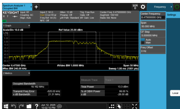
Plot 7-203 26dB BW & 99% OBW Antenna 2a (20MHz BW 802.11be(RU) RU106+26 Index82 - Ch.105)
