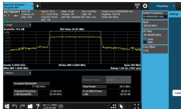
Plot 7-175 26dB BW & 99% OBW Antenna 2a (80MHz BW 802.11be(RU) RU996 Index67 - Ch.103)
