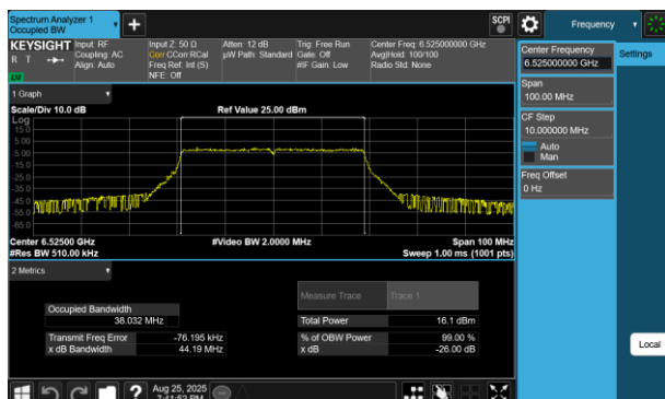
Plot 7-207 26dB BW & 99% OBW Antenna 2a (40MHz BW 802.11be(RU) RU484 Index65 - Ch.115)
