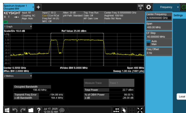
Plot 7-205 26dB BW & 99% OBW Antenna 2a (160MHz BW 802.11be(RU) RU996+484+242 Index97 - Ch.111)
