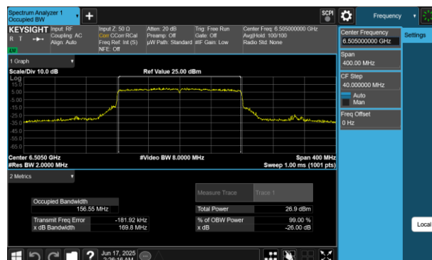
Plot 7-176 26dB BW & 99% OBW Antenna 2a (160MHz BW 802.11be(RU) RU996X2 Index68 - Ch.111)
