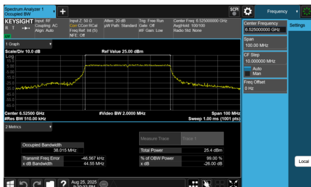
Plot 7-174 26dB BW & 99% OBW Antenna 2a (40MHz BW 802.11be(RU) RU484 Index65 - Ch.115)
