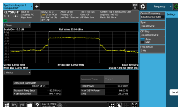
Plot 7-209 26dB BW & 99% OBW Antenna 2a (160MHz BW 802.11be(RU) RU996X2 Index68 - Ch.111)
