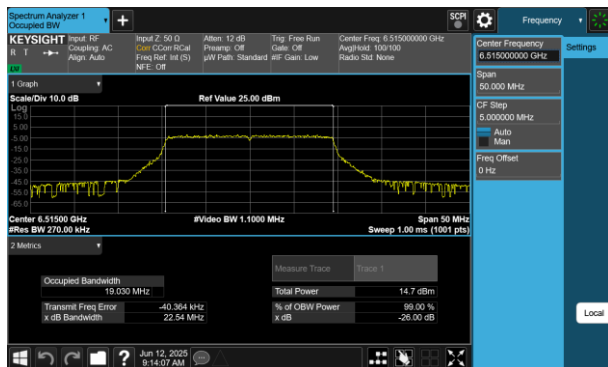
Plot 7-206 26dB BW & 99% OBW Antenna 2a (20MHz BW 802.11be(RU) RU242 Index61 - Ch.113)
