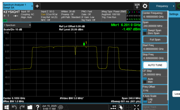
Plot 7-238 PSD Antenna WF5B (160MHz BW 802.11be(RU) RU996+484+242 Index98 - Ch.47)
