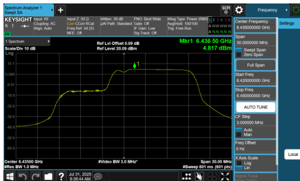
Plot 7-247 PSD Antenna WF5B (20MHz BW 802.11be(RU) RU106+26 Index83 - Ch.97)
