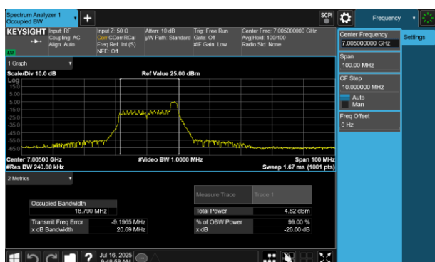
Plot 7-222 26dB BW & 99% OBW Antenna 2a (40MHz BW 802.11be(RU) RU26 Index8 - Ch.211)
