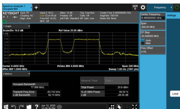
Plot 7-204 26dB BW & 99% OBW Antenna 2a (80MHz BW 802.11be(RU) RU484+242 Index91 - Ch.103)
