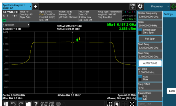
Plot 7-240 PSD Antenna WF5B (40MHz BW 802.11be(RU) RU484 Index65 - Ch.43)
