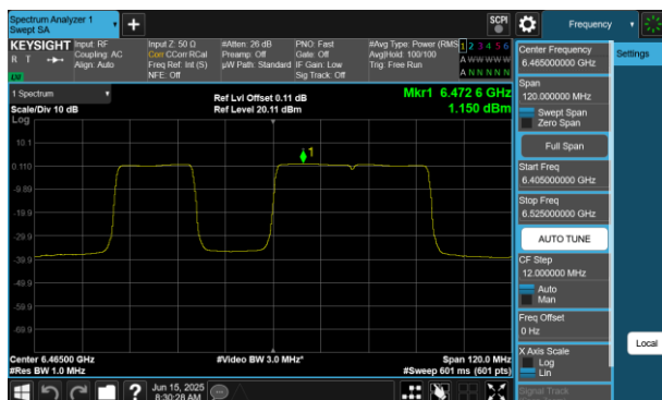
Plot 7-248 PSD Antenna WF5B (80MHz BW 802.11be(RU) RU484+242 Index91 - Ch.103)
