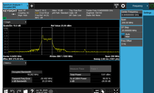
Plot 7-223 26dB BW & 99% OBW Antenna 2a (80MHz BW 802.11be(RU) RU26 Index0 - Ch.199)
