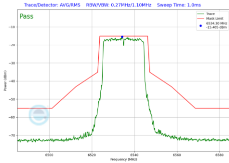
Plot 7-477 In-Band Emission Plot Antenna WF5B (20MHz BW 802.11be(RU) RU242 Index61 (UNII Band 7) - Ch.117)
