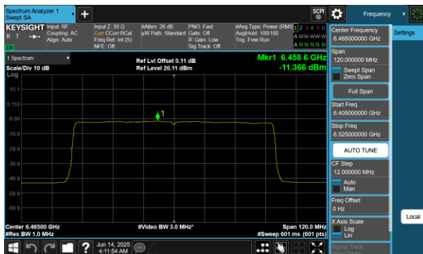
Plot 7-391 PSD SDM Diversity Antenna 4a (80MHz BW 802.11be(RU) RU996 Index67 - Ch.103)
