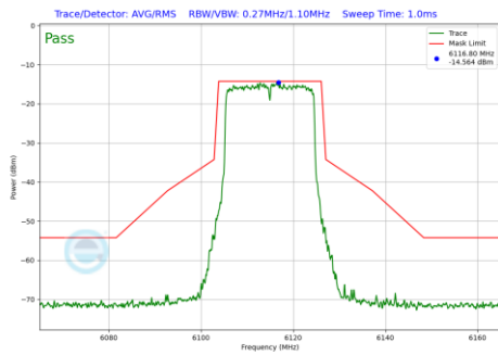
Plot 7-469 In-Band Emission Plot Antenna WF5B (20MHz BW 802.11be(RU) RU242 Index61 (UNII Band 5) - Ch.33)
