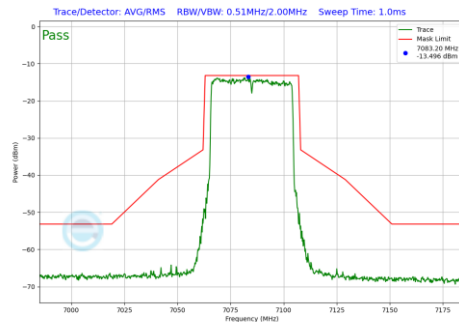
Plot 7-482 In-Band Emission Plot Antenna WF5B (40MHz BW 802.11be(RU) RU484 Index65 (UNII Band 8) - Ch.227)
