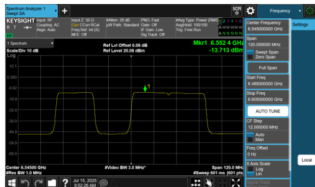
Plot 7-409 PSD SDM Diversity Antenna 2a (80MHz BW 802.11be(RU) RU484+242 Index91 - Ch.119)
