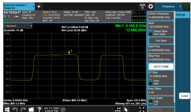
Plot 7-387 PSD SDM Diversity Antenna 2a (80MHz BW 802.11be(RU) RU484+242 Index92 - Ch.103)
