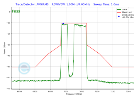
Plot 7-467 In-Band Emission Plot Antenna WF5B (80MHz BW 802.11be(RU) RU484+242 Index91 (UNII Band 8) - Ch.215)
