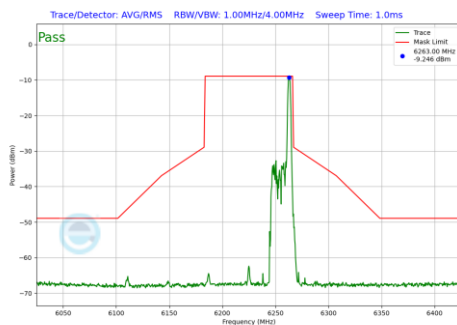
Plot 7-443 In-Band Emission Plot Antenna WF5B (80MHz BW 802.11be(RU) RU26 Index36 (UNII Band 5) - Ch.55)
