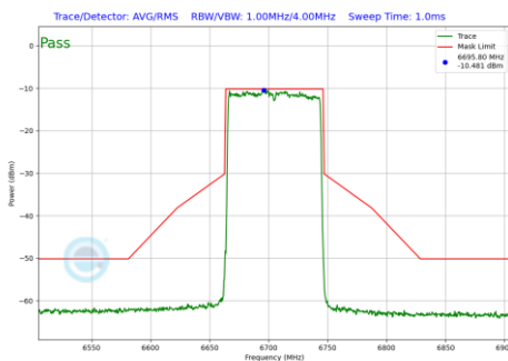
Plot 7-479 In-Band Emission Plot Antenna WF5B (80MHz BW 802.11be(RU) RU996 Index67 (UNII Band 7) - Ch.151)
