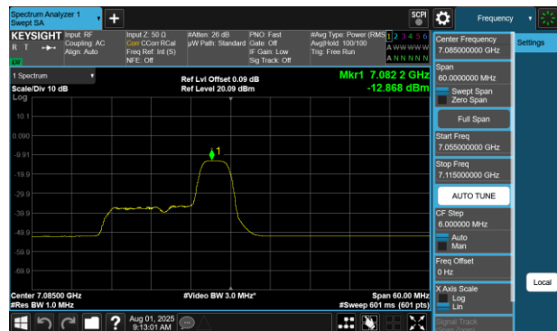
Plot 7-424 PSD SDM Diversity Antenna 2a (40MHz BW 802.11be(RU) RU52 Index40 - Ch.227)
