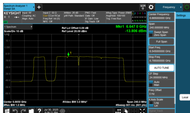
Plot 7-410 PSD SDM Diversity Antenna 2a (160MHz BW 802.11be(RU) RU996+484+242 Index97 - Ch.143)
