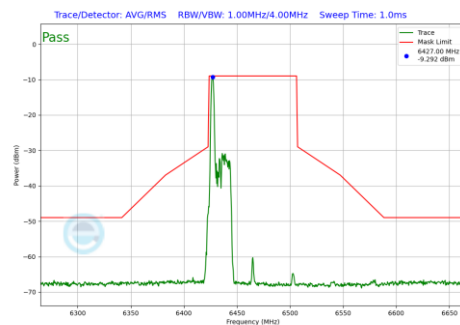
Plot 7-447 In-Band Emission Plot Antenna WF5B (80MHz BW 802.11be(RU) RU26 Index0 (UNII Band 6) - Ch.103)
