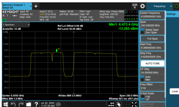
Plot 7-385 PSD SDM Diversity Antenna 4a(160MHz BW 802.11be(RU) RU996+484+242 Index99 - Ch.111)
