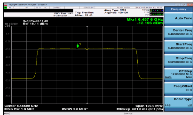
Plot 7-395 PSD SDM Diversity Antenna 2a (80MHz BW 802.11be(RU) RU996 Index67 - Ch.103)
