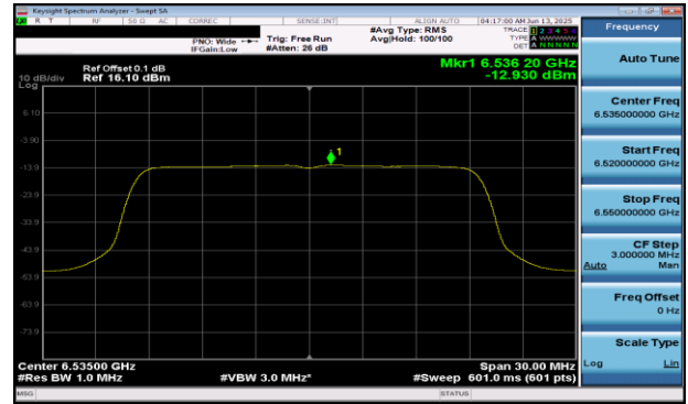
Plot 7-415 PSD SDM Diversity Antenna 2a (20MHz BW 802.11be(RU) RU242 Index61 - Ch.117)
