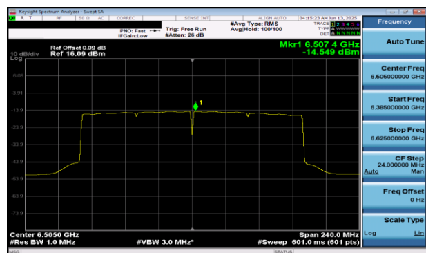
Plot 7-396 PSD SDM Diversity Antenna 2a (160MHz BW 802.11be(RU) RU996X2 Index68 - Ch.111)
