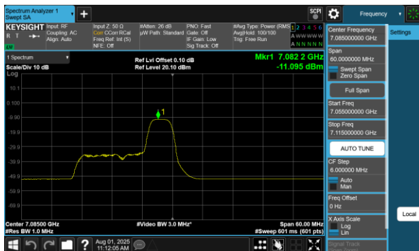
Plot 7-420 PSD SDM Diversity Antenna 4a (40MHz BW 802.11be(RU) RU52 Index40 - Ch.227)
