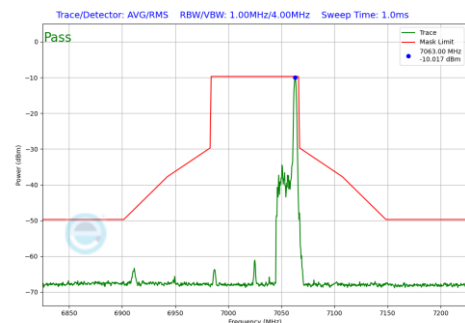
Plot 7-455 In-Band Emission Plot Antenna WF5B (80MHz BW 802.11be(RU) RU26 Index36 (UNII Band 8) - Ch.215)
