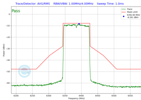
Plot 7-471 In-Band Emission Plot Antenna WF5B (80MHz BW 802.11be(RU) RU996 Index67 (UNII Band 5) - Ch.87)
