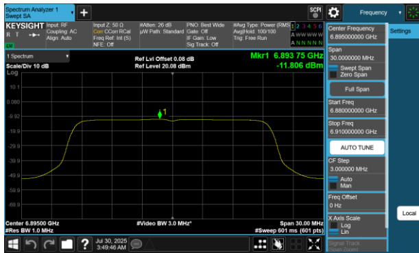
Plot 7-433 PSD SDM Diversity Antenna 4a (20MHz BW 802.11be(RU) RU242 Index61 - Ch.189)
