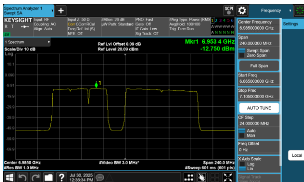
Plot 7-429 PSD SDM Diversity Antenna 4a(160MHz BW 802.11be(RU) RU996+484+242 Index99 - Ch.207)
