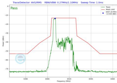
Plot 7-441 In-Band Emission Plot Antenna WF5B (20MHz BW 802.11be(RU) RU26 Index0 (UNII Band 5) - Ch.93)
