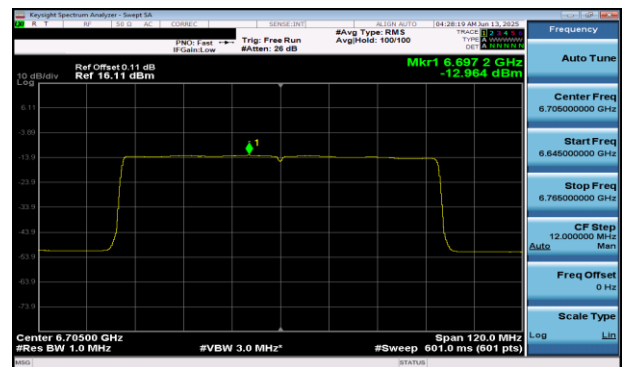
Plot 7-417 PSD SDM Diversity Antenna 2a (80MHz BW 802.11be(RU) RU996 Index67 - Ch.151)
