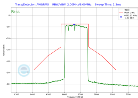
Plot 7-465 In-Band Emission Plot Antenna WF5B (160MHz BW 802.11be(RU) RU996+484+242 Index96 (UNII Band 7) - Ch.143)
