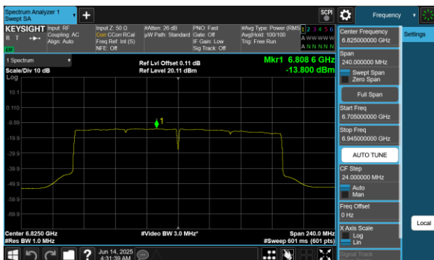
Plot 7-414 PSD SDM Diversity Antenna 4a (160MHz BW 802.11be(RU) RU996X2 Index68 - Ch.175)
