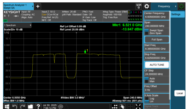
Plot 7-388 PSD SDM Diversity Antenna 2a (160MHz BW 802.11be(RU) RU996+484+242 Index99 - Ch.111)
