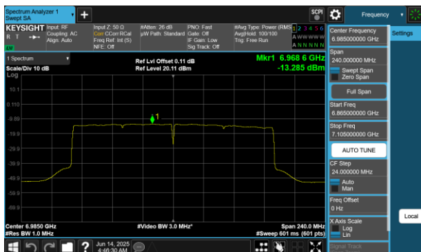
Plot 7-436 PSD SDM Diversity Antenna 4a (160MHz BW 802.11be(RU) RU996X2 Index68 - Ch.207)
