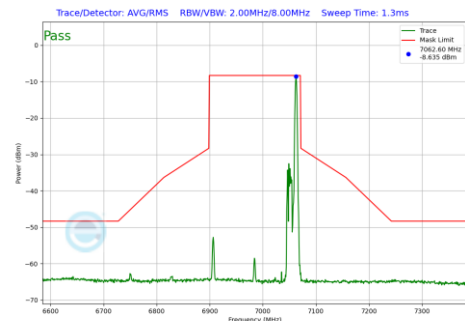
Plot 7-456 In-Band Emission Plot Antenna WF5B (160MHz BW 802.11be(RU) RU26 Index36 (UNII Band 8) - Ch.207)
