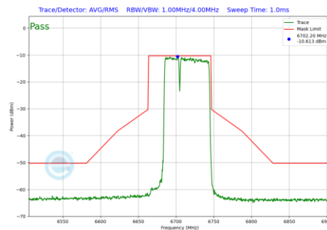
Plot 7-464 In-Band Emission Plot Antenna WF5B (80MHz BW 802.11be(RU) RU484+242 Index90 (UNII Band 7) - Ch.151)
