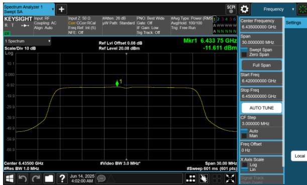
Plot 7-389 PSD SDM Diversity Antenna 4a (20MHz BW 802.11be(RU) RU242 Index61 - Ch.97)
