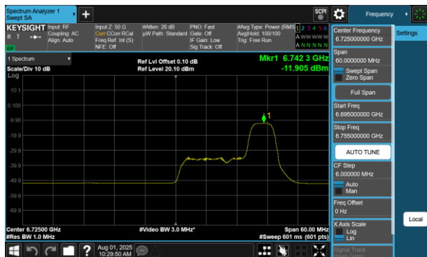
Plot 7-398 PSD SDM Diversity Antenna 4a (40MHz BW 802.11be(RU) RU52 Index44 - Ch.155)
