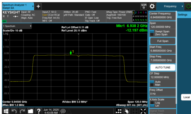
Plot 7-435 PSD SDM Diversity Antenna 4a (80MHz BW 802.11be(RU) RU996 Index67 - Ch.199)
