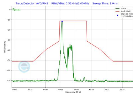
Plot 7-446 In-Band Emission Plot Antenna WF5B (40MHz BW 802.11be(RU) RU26 Index0 (UNII Band 6) - Ch.99)
