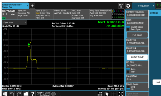
Plot 7-422 PSD SDM Diversity Antenna 4a (160MHz BW 802.11be(RU) RU52 Index37 - Ch.207)
