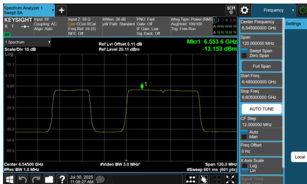
Plot 7-406 PSD SDM Diversity Antenna 4a(80MHz BW 802.11be(RU) RU484+242 Index91 - Ch.119)
