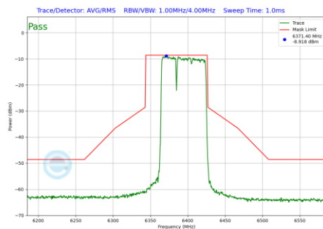
Plot 7-458 In-Band Emission Plot Antenna WF5B (80MHz BW 802.11be(RU) RU484+242 Index90 (UNII Band 5) - Ch.87)
