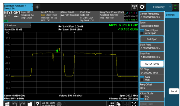
Plot 7-432 PSD SDM Diversity Antenna 2a (160MHz BW 802.11be(RU) RU996+484+242 Index99 - Ch.207)
