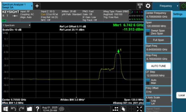
Plot 7-399 PSD SDM Diversity Antenna 4a (80MHz BW 802.11be(RU) RU52 Index52 - Ch.151)
