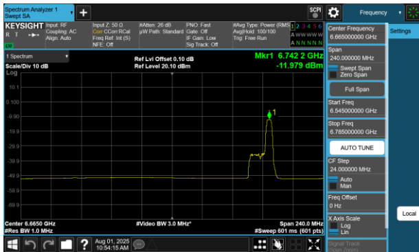
Plot 7-400 PSD SDM Diversity Antenna 4a (160MHz BW 802.11be(RU) RU52 Index52 - Ch.143)
