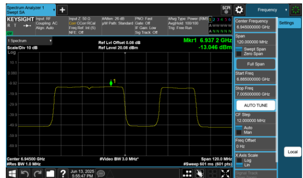
Plot 7-431 PSD SDM Diversity Antenna 2a (80MHz BW 802.11be(RU) RU484+242 Index92 - Ch.199)
