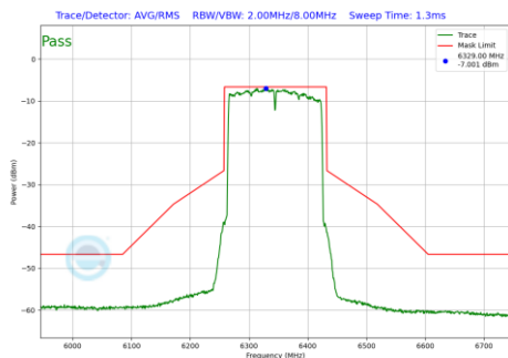
Plot 7-472 In-Band Emission Plot Antenna WF5B (160MHz BW 802.11be(RU) RU996X2 Index68 (UNII Band 5) - Ch.79)
