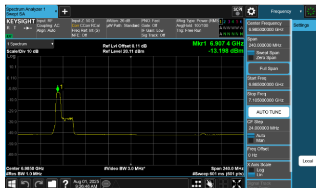
Plot 7-426 PSD SDM Diversity Antenna 2a (160MHz BW 802.11be(RU) RU52 Index37 - Ch.207)
