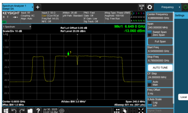
Plot 7-407 PSD SDM Diversity Antenna 4a(160MHz BW 802.11be(RU) RU996+484+242 Index97 - Ch.143)
