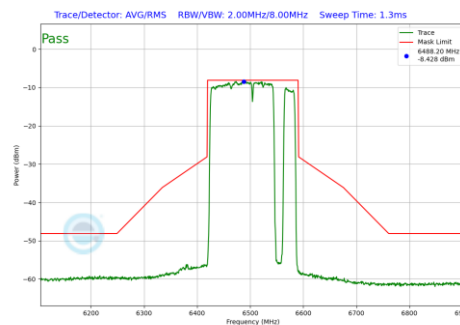
Plot 7-462 In-Band Emission Plot Antenna WF5B (160MHz BW 802.11be(RU) RU996+484+242 Index98 (UNII Band 6) - Ch.111)
