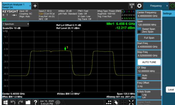
Plot 7-384 PSD SDM Diversity Antenna 4a(80MHz BW 802.11be(RU) RU484+242 Index92 - Ch.103)
