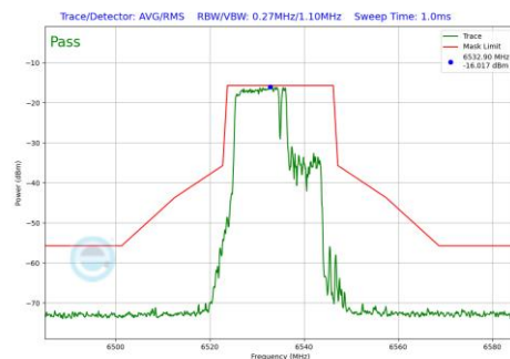
Plot 7-463 In-Band Emission Plot Antenna WF5B (20MHz BW 802.11be(RU) RU106+26 Index82 (UNII Band 7) - Ch.117)
