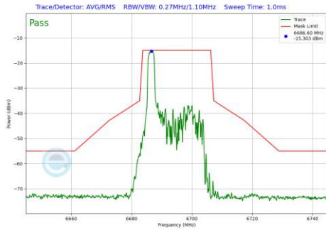
Plot 7-449 In-Band Emission Plot Antenna WF5B (20MHz BW 802.11be(RU) RU26 Index0 (UNII Band 7) - Ch.149)
