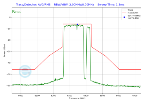
Plot 7-459 In-Band Emission Plot Antenna WF5B (160MHz BW 802.11be(RU) RU996+484+242 Index98 (UNII Band 5) - Ch.79)
