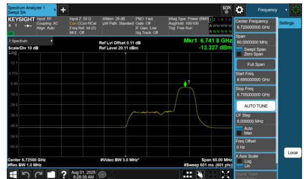
Plot 7-402 PSD SDM Diversity Antenna 2a (40MHz BW 802.11be(RU) RU52 Index44 - Ch.155)
