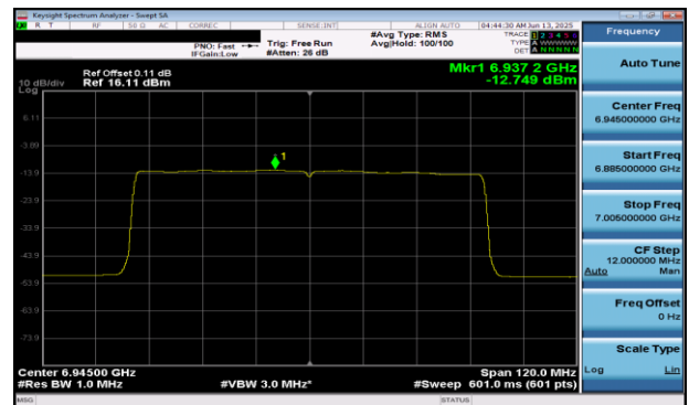
Plot 7-439 PSD SDM Diversity Antenna 2a (80MHz BW 802.11be(RU) RU996 Index67 - Ch.199)
