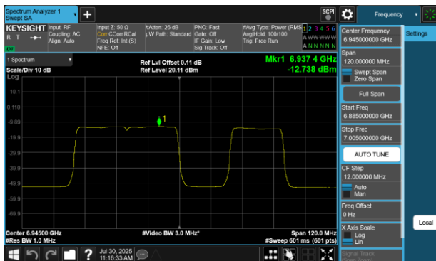
Plot 7-428 PSD SDM Diversity Antenna 4a(80MHz BW 802.11be(RU) RU484+242 Index92 - Ch.199)
