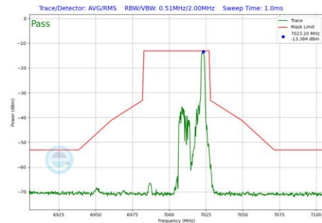
Plot 7-454 In-Band Emission Plot Antenna WF5B (40MHz BW 802.11be(RU) RU26 Index17 (UNII Band 8) - Ch.211)
