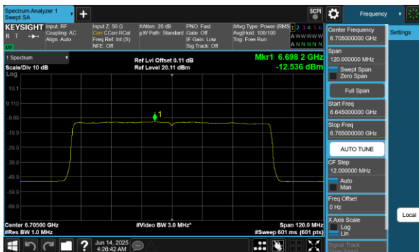
Plot 7-413 PSD SDM Diversity Antenna 4a (80MHz BW 802.11be(RU) RU996 Index67 - Ch.151)
