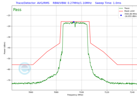
Plot 7-481 In-Band Emission Plot Antenna WF5B (20MHz BW 802.11be(RU) RU242 Index61 (UNII Band 8) - Ch.229)
