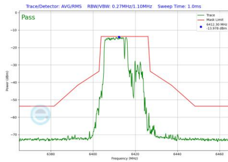
Plot 7-457 In-Band Emission Plot Antenna WF5B (20MHz BW 802.11be(RU) RU106+26 Index82 (UNII Band 5) - Ch.93)
