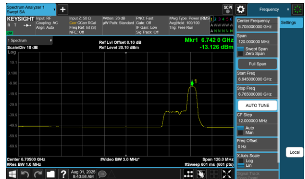
Plot 7-403 PSD SDM Diversity Antenna 2a (80MHz BW 802.11be(RU) RU52 Index52 - Ch.151)
