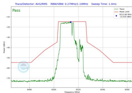
Plot 7-460 In-Band Emission Plot Antenna WF5B (20MHz BW 802.11be(RU) RU106+26 Index82 (UNII Band 6) - Ch.113)
