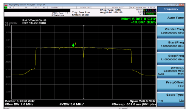
Plot 7-440 PSD SDM Diversity Antenna 2a (160MHz BW 802.11be(RU) RU996X2 Index68 - Ch.207)
