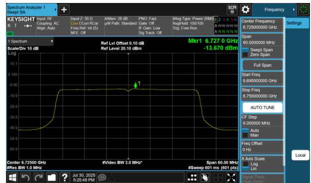
Plot 7-416 PSD SDM Diversity Antenna 2a (40MHz BW 802.11be(RU) RU484 Index65 - Ch.155)
