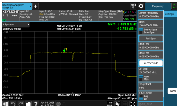
Plot 7-392 PSD SDM Diversity Antenna 4a (160MHz BW 802.11be(RU) RU996X2 Index68 - Ch.111)
