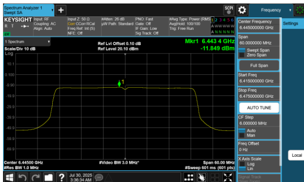
Plot 7-390 PSD SDM Diversity Antenna 4a (40MHz BW 802.11be(RU) RU484 Index65 - Ch.99)
