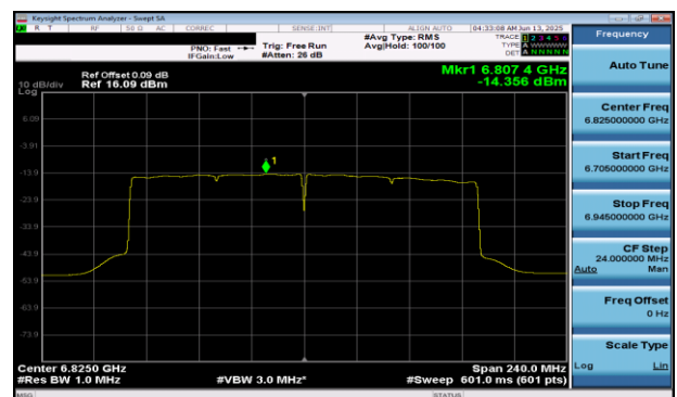
Plot 7-418 PSD SDM Diversity Antenna 2a (160MHz BW 802.11be(RU) RU996X2 Index68 - Ch.175)
