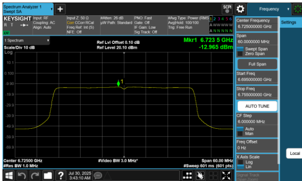
Plot 7-412 PSD SDM Diversity Antenna 4a (40MHz BW 802.11be(RU) RU484 Index65 - Ch.155)
