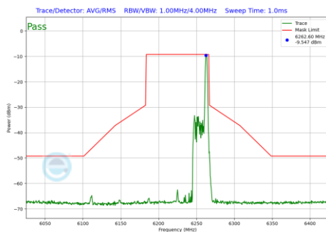
Plot 7-531 In-Band Emission Plot Antenna 2a (80MHz BW 802.11be(RU) RU26 Index36 (UNII Band 5) - Ch.55)
