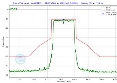
Plot 7-558 In-Band Emission Plot Antenna 2a (40MHz BW 802.11be(RU) RU484 Index65 (UNII Band 5) - Ch.91)
