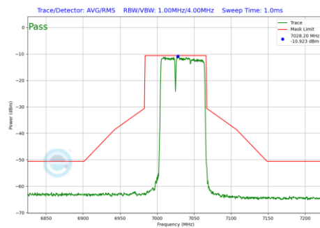
Plot 7-555 In-Band Emission Plot Antenna 2a (80MHz BW 802.11be(RU) RU484+242 Index90 (UNII Band 8) - Ch.215)
