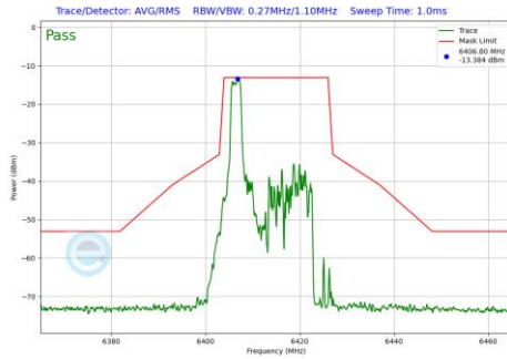
Plot 7-529 In-Band Emission Plot Antenna 2a (20MHz BW 802.11be(RU) RU26 Index0 (UNII Band 5) - Ch.93)
