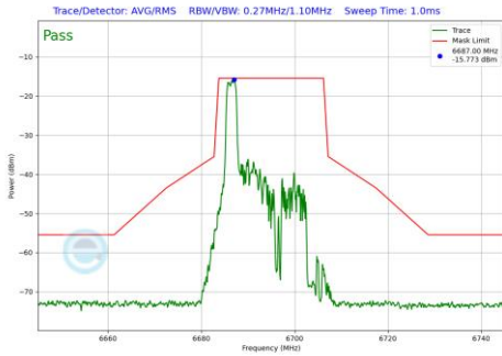
Plot 7-537 In-Band Emission Plot Antenna 2a (20MHz BW 802.11be(RU) RU26 Index0 (UNII Band 7) - Ch.149)
