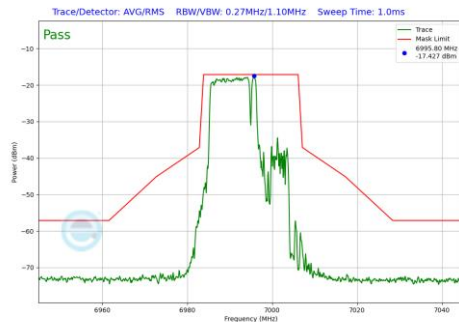
Plot 7-614 In-Band Emission Plot SDM Primary Antenna WF5B (20MHz BW 802.11be(RU) RU106+26 Index82 (UNII Band 8) - Ch.209)
