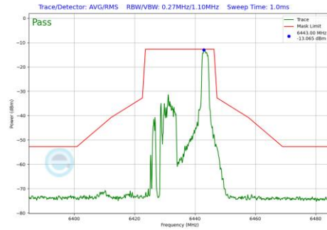
Plot 7-489 In-Band Emission Plot Antenna 4a (20MHz BW 802.11be(RU) RU26 Index8 (UNII Band 6) - Ch.97)
