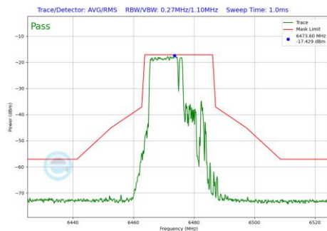
Plot 7-608 In-Band Emission Plot SDM Primary Antenna WF5B (20MHz BW 802.11be(RU) RU106+26 Index82 (UNII Band 6) - Ch.105)
