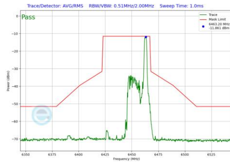
Plot 7-534 In-Band Emission Plot Antenna 2a (40MHz BW 802.11be(RU) RU26 Index17 (UNII Band 6) - Ch.99)
