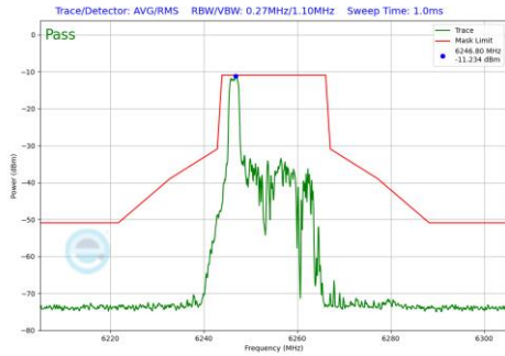
Plot 7-485 In-Band Emission Plot Antenna 4a (20MHz BW 802.11be(RU) RU26 Index0 (UNII Band 5) - Ch.61)
