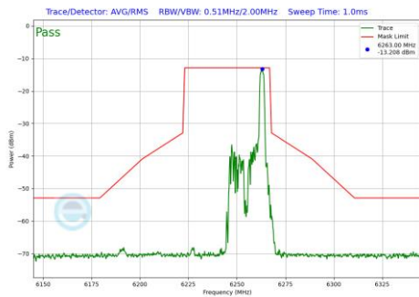
Plot 7-574 In-Band Emission Plot SDM Primary Antenna WF5B (40MHz BW 802.11be(RU) RU26 Index17 (UNII Band 5) - Ch.59)
