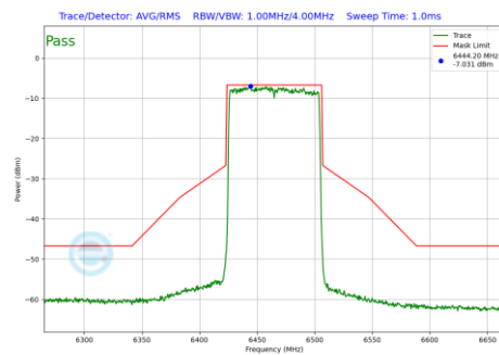
Plot 7-519 In-Band Emission Plot Antenna 4a (80MHz BW 802.11be(RU) RU996 Index67 (UNII Band 6) - Ch.103)
