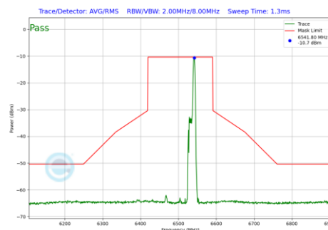
Plot 7-580 In-Band Emission Plot SDM Primary Antenna WF5B (160MHz BW 802.11be(RU) RU52 Index44 (UNII Band 6) - Ch.111)
