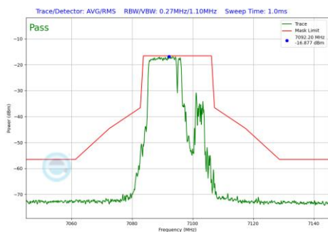
Plot 7-554 In-Band Emission Plot Antenna 2a (20MHz BW 802.11be(RU) RU106+26 Index82 (UNII Band 8) - Ch.229)
