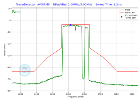
Plot 7-503 In-Band Emission Plot Antenna 4a (160MHz BW 802.11be(RU) RU996+484+242 Index98 (UNII Band 5) - Ch.79)
