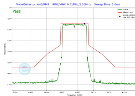
Plot 7-634 In-Band Emission Plot SDM Primary Antenna WF5B (40MHz BW 802.11be(RU) RU484 Index65 (UNII Band 6) - Ch.99)
