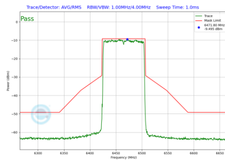
Plot 7-563 In-Band Emission Plot Antenna 2a (80MHz BW 802.11be(RU) RU996 Index67 (UNII Band 6) - Ch.103)
