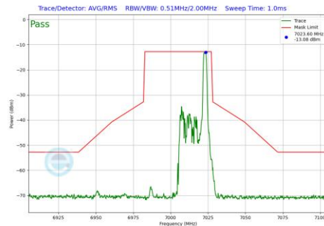
Plot 7-542 In-Band Emission Plot Antenna 2a (40MHz BW 802.11be(RU) RU26 Index17 (UNII Band 8) - Ch.211)
