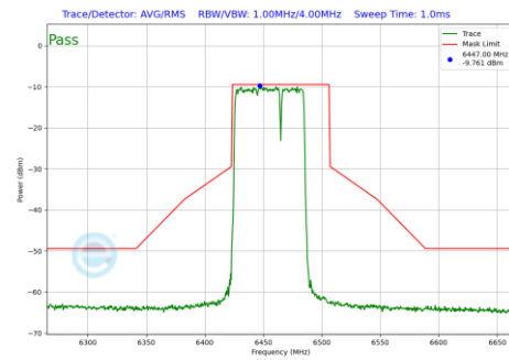
Plot 7-549 In-Band Emission Plot Antenna 2a (80MHz BW 802.11be(RU) RU484+242 Index93 (UNII Band 6) - Ch.103)
