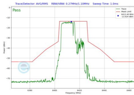
Plot 7-545 In-Band Emission Plot Antenna 2a (20MHz BW 802.11be(RU) RU106+26 Index82 (UNII Band 5) - Ch.93)
