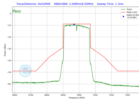
Plot 7-572 In-Band Emission Plot Antenna 2a (160MHz BW 802.11be(RU) RU996X2 Index68 (UNII Band 8) - Ch.207)
