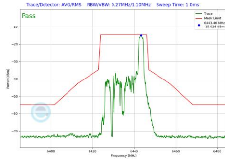
Plot 7-533 In-Band Emission Plot Antenna 2a (20MHz BW 802.11be(RU) RU26 Index8 (UNII Band 6) - Ch.97)
