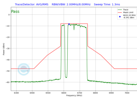
Plot 7-553 In-Band Emission Plot Antenna 2a (160MHz BW 802.11be(RU) RU996+484+242 Index97 (UNII Band 7) - Ch.143)
