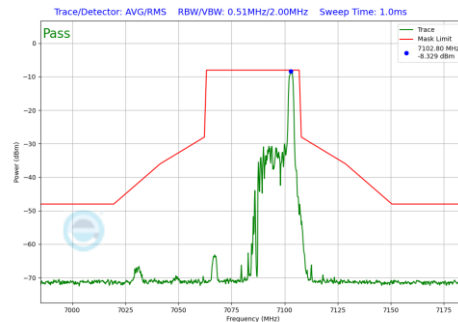
Plot 7-498 In-Band Emission Plot Antenna 4a (40MHz BW 802.11be(RU) RU26 Index17 (UNII Band 8) - Ch.227)
