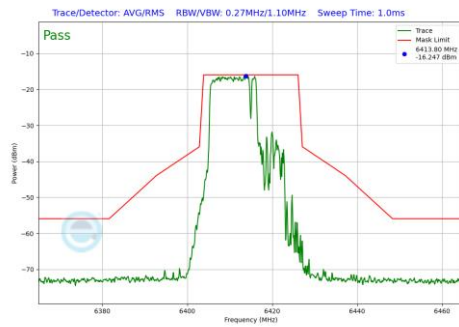
Plot 7-605 In-Band Emission Plot SDM Primary Antenna WF5B (20MHz BW 802.11be(RU) RU106+26 Index82 (UNII Band 5) - Ch.93)
