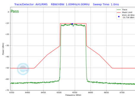
Plot 7-567 In-Band Emission Plot Antenna 2a (80MHz BW 802.11be(RU) RU996 Index67 (UNII Band 7) - Ch.119)
