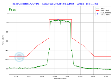
Plot 7-560 In-Band Emission Plot Antenna 2a (160MHz BW 802.11be(RU) RU996X2 Index68 (UNII Band 5) - Ch.79)
