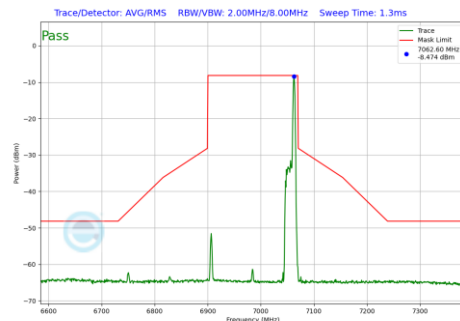
Plot 7-544 In-Band Emission Plot Antenna 2a (160MHz BW 802.11be(RU) RU26 Index36 (UNII Band 8) - Ch.207)
