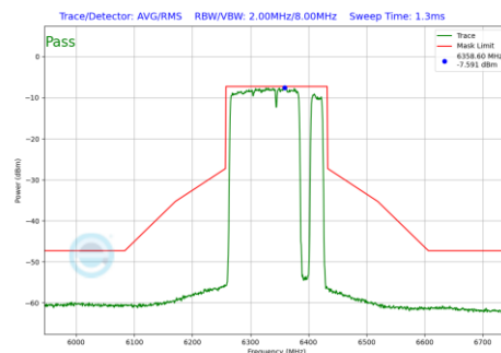
Plot 7-619 In-Band Emission Plot SDM Primary Antenna 4a (160MHz BW 802.11be(RU) RU996+484+242 Index98 (UNII Band 5) - Ch.79)
