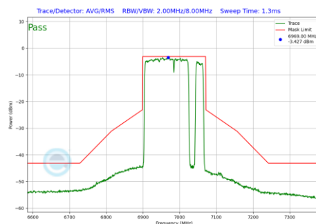
Plot 7-512 In-Band Emission Plot Antenna 4a (160MHz BW 802.11be(RU) RU996+484+242 Index98 (UNII Band 8) - Ch.207)
