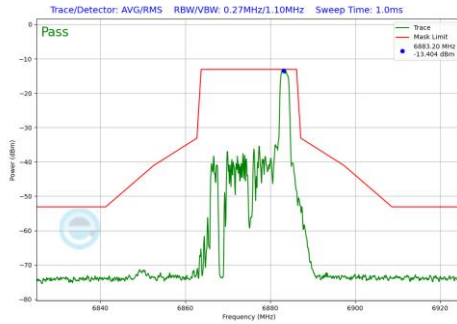
Plot 7-493 In-Band Emission Plot Antenna 4a (20MHz BW 802.11be(RU) RU26 Index8 (UNII Band 7) - Ch.185)
