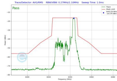
Plot 7-593 In-Band Emission Plot SDM Primary Antenna 4a (20MHz BW 802.11be(RU) RU26 Index8 (UNII Band 6) - Ch.97)
