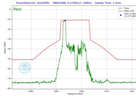
Plot 7-497 In-Band Emission Plot Antenna 4a (20MHz BW 802.11be(RU) RU26 Index0 (UNII Band 8) - Ch.229)
