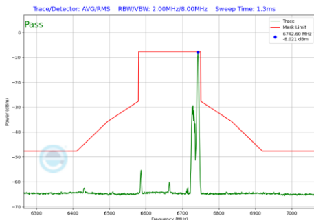
Plot 7-540 In-Band Emission Plot Antenna 2a (160MHz BW 802.11be(RU) RU26 Index36 (UNII Band 7) - Ch.143)
