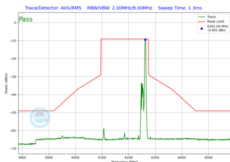
Plot 7-576 In-Band Emission Plot SDM Primary Antenna WF5B (160MHz BW 802.11be(RU) RU26 Index36 (UNII Band 5) - Ch.47)
