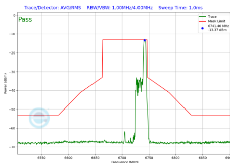
Plot 7-583 In-Band Emission Plot SDM Primary Antenna WF5B (80MHz BW 802.11be(RU) RU52 Index52 (UNII Band 7) - Ch.151)
