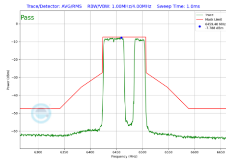
Plot 7-505 In-Band Emission Plot Antenna 4a (80MHz BW 802.11be(RU) RU484+242 Index92 (UNII Band 6) - Ch.103)
