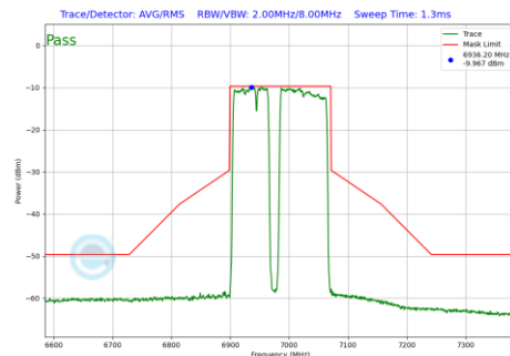
Plot 7-628 In-Band Emission Plot SDM Primary Antenna 4a (160MHz BW 802.11be(RU) RU996+484+242 Index99 (UNII Band 8) - Ch.207)
