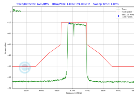
Plot 7-552 In-Band Emission Plot Antenna 2a (80MHz BW 802.11be(RU) RU484+242 Index90 (UNII Band 7) - Ch.151)
