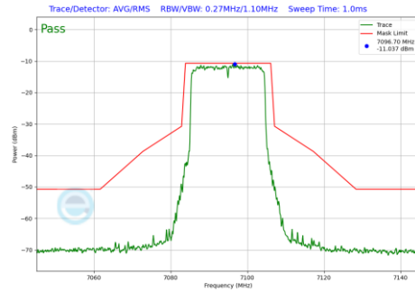
Plot 7-525 In-Band Emission Plot Antenna 4a (20MHz BW 802.11be(RU) RU242 Index61 (UNII Band 8) - Ch.229)
