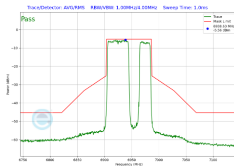
Plot 7-511 In-Band Emission Plot Antenna 4a (80MHz BW 802.11be(RU) RU484+242 Index92 (UNII Band 8) - Ch.199)
