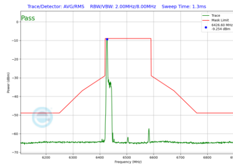
Plot 7-536 In-Band Emission Plot Antenna 2a (160MHz BW 802.11be(RU) RU26 Index0 (UNII Band 6) - Ch.111)
