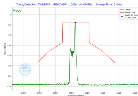
Plot 7-491 In-Band Emission Plot Antenna 4a (80MHz BW 802.11be(RU) RU26 Index17 (UNII Band 6) - Ch.103)
