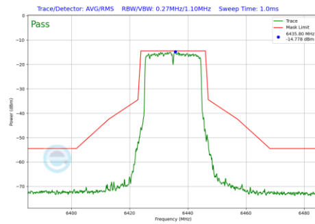
Plot 7-561 In-Band Emission Plot Antenna 2a (20MHz BW 802.11be(RU) RU242 Index61 (UNII Band 6) - Ch.97)
