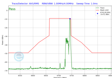
Plot 7-539 In-Band Emission Plot Antenna 2a (80MHz BW 802.11be(RU) RU26 Index36 (UNII Band 7) - Ch.151)
