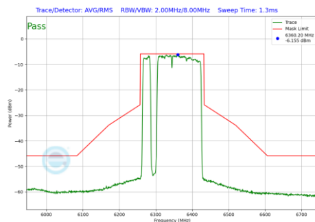
Plot 7-547 In-Band Emission Plot Antenna 2a (160MHz BW 802.11be(RU) RU996+484+242 Index97 (UNII Band 5) - Ch.79)
