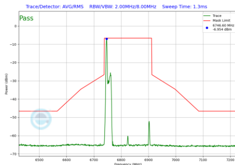
Plot 7-496 In-Band Emission Plot Antenna 4a (160MHz BW 802.11be(RU) RU26 Index0 (UNII Band 7) - Ch.175)
