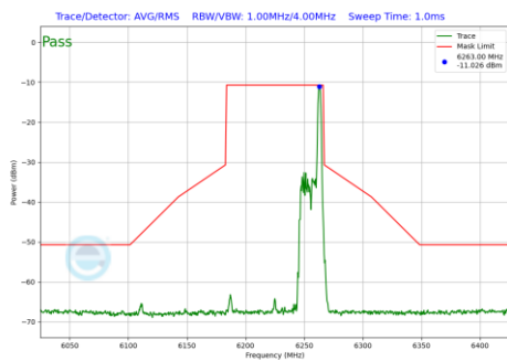
Plot 7-575 In-Band Emission Plot SDM Primary Antenna WF5B (80MHz BW 802.11be(RU) RU26 Index36 (UNII Band 5) - Ch.55)
