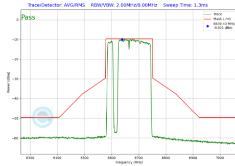
Plot 7-625 In-Band Emission Plot SDM Primary Antenna 4a (160MHz BW 802.11be(RU) RU996+484+242 Index97 (UNII Band 7) - Ch.143)
