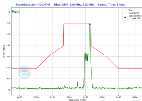
Plot 7-591 In-Band Emission Plot SDM Primary Antenna 4a (80MHz BW 802.11be(RU) RU26 Index36 (UNII Band 5) - Ch.55)
