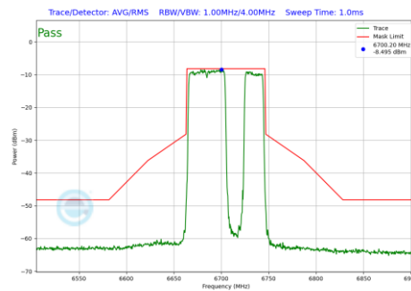
Plot 7-508 In-Band Emission Plot Antenna 4a (80MHz BW 802.11be(RU) RU484+242 Index92 (UNII Band 7) - Ch.151)
