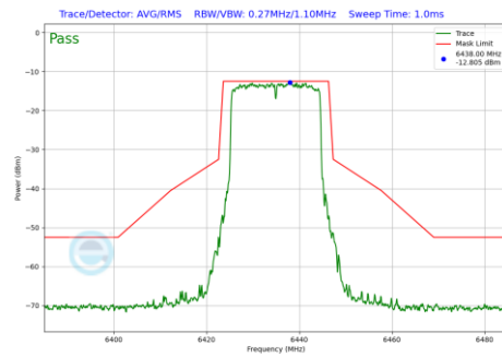
Plot 7-517 In-Band Emission Plot Antenna 4a (20MHz BW 802.11be(RU) RU242 Index61 (UNII Band 6) - Ch.97)
