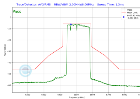
Plot 7-506 In-Band Emission Plot Antenna 4a (160MHz BW 802.11be(RU) RU996+484+242 Index96 (UNII Band 6) - Ch.111)
