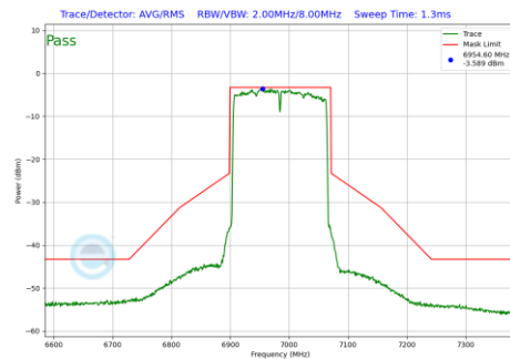
Plot 7-528 In-Band Emission Plot Antenna 4a (160MHz BW 802.11be(RU) RU996X2 Index68 (UNII Band 8) - Ch.207)
