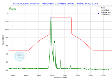
Plot 7-487 In-Band Emission Plot Antenna 4a (80MHz BW 802.11be(RU) RU26 Index0 (UNII Band 5) - Ch.87)
