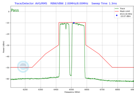
Plot 7-622 In-Band Emission Plot SDM Primary Antenna 4a (160MHz BW 802.11be(RU) RU996+484+242 Index99 (UNII Band 6) - Ch.111)
