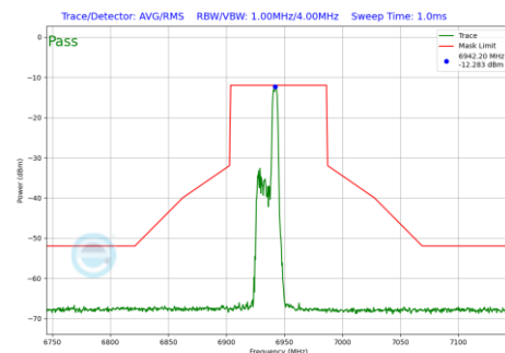
Plot 7-587 In-Band Emission Plot SDM Primary Antenna WF5B (80MHz BW 802.11be(RU) RU52 Index44 (UNII Band 8) - Ch.199)
