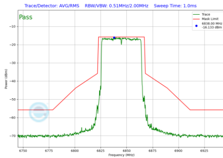
Plot 7-638 In-Band Emission Plot SDM Primary Antenna WF5B (40MHz BW 802.11be(RU) RU484 Index65 (UNII Band 7) - Ch.179)
