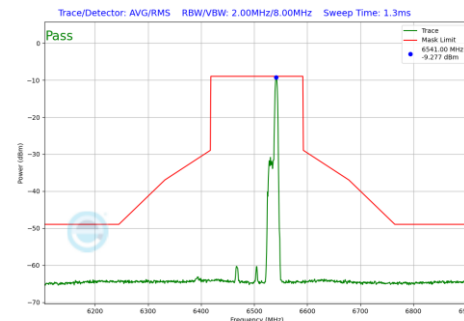
Plot 7-596 In-Band Emission Plot SDM Primary Antenna 4a (160MHz BW 802.11be(RU) RU52 Index44 (UNII Band 6) - Ch.111)
