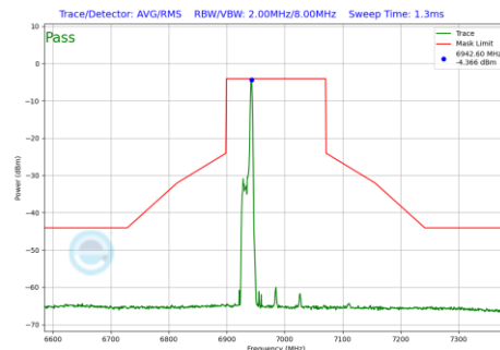
Plot 7-500 In-Band Emission Plot Antenna 4a (160MHz BW 802.11be(RU) RU26 Index17 (UNII Band 8) - Ch.207)
