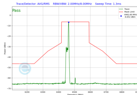
Plot 7-492 In-Band Emission Plot Antenna 4a (160MHz BW 802.11be(RU) RU26 Index17 (UNII Band 6) - Ch.111)
