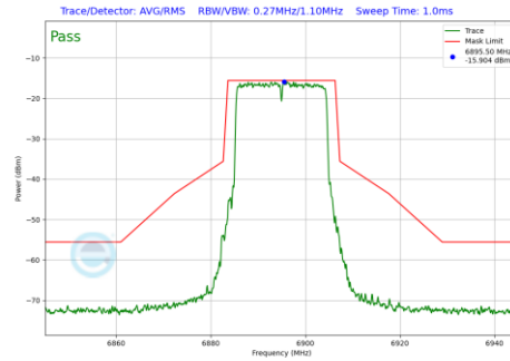
Plot 7-569 In-Band Emission Plot Antenna 2a (20MHz BW 802.11be(RU) RU242 Index61 (UNII Band 8) - Ch.189)
