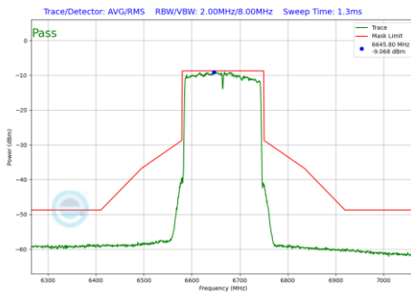
Plot 7-568 In-Band Emission Plot Antenna 2a (160MHz BW 802.11be(RU) RU996X2 Index68 (UNII Band 7) - Ch.143)
