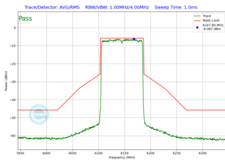
Plot 7-515 In-Band Emission Plot Antenna 4a (80MHz BW 802.11be(RU) RU996 Index67 (UNII Band 5) - Ch.39)
