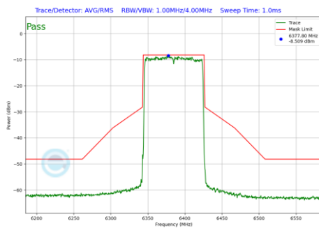
Plot 7-559 In-Band Emission Plot Antenna 2a (80MHz BW 802.11be(RU) RU996 Index67 (UNII Band 5) - Ch.87)
