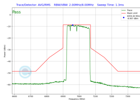
Plot 7-556 In-Band Emission Plot Antenna 2a (160MHz BW 802.11be(RU) RU996+484+242 Index96 (UNII Band 8) - Ch.207)
