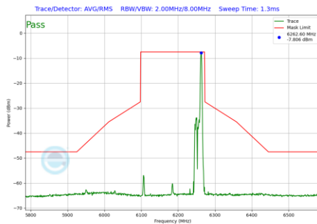
Plot 7-532 In-Band Emission Plot Antenna 2a (160MHz BW 802.11be(RU) RU26 Index36 (UNII Band 5) - Ch.47)
