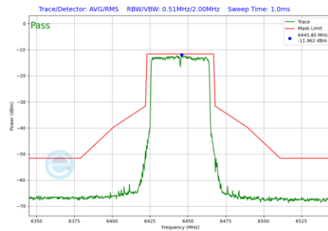
Plot 7-562 In-Band Emission Plot Antenna 2a (40MHz BW 802.11be(RU) RU484 Index65 (UNII Band 6) - Ch.99)
