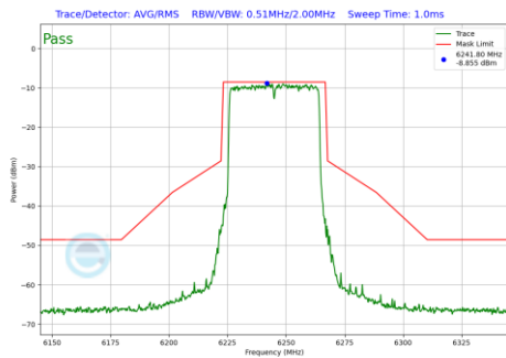
Plot 7-514 In-Band Emission Plot Antenna 4a (40MHz BW 802.11be(RU) RU484 Index65 (UNII Band 5) - Ch.59)
