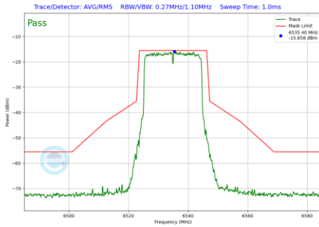
Plot 7-565 In-Band Emission Plot Antenna 2a (20MHz BW 802.11be(RU) RU242 Index61 (UNII Band 7) - Ch.117)
