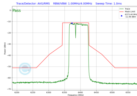
Plot 7-618 In-Band Emission Plot SDM Primary Antenna 4a (80MHz BW 802.11be(RU) RU484+242 Index90 (UNII Band 5) - Ch.87)
