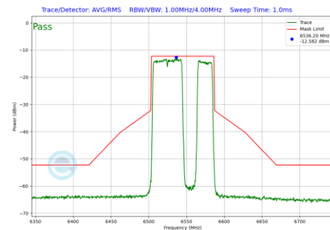
Plot 7-612 In-Band Emission Plot SDM Primary Antenna WF5B (80MHz BW 802.11be(RU) RU484+242 Index92 (UNII Band 7) - Ch.119)
