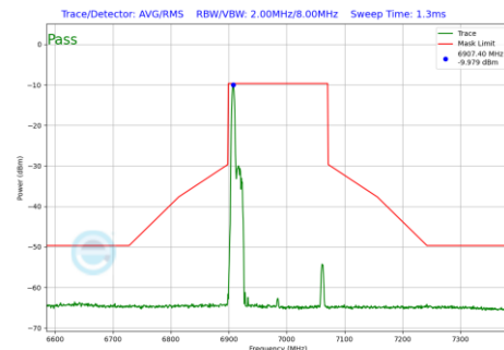
Plot 7-588 In-Band Emission Plot SDM Primary Antenna WF5B (160MHz BW 802.11be(RU) RU52 Index37 (UNII Band 8) - Ch.207)
