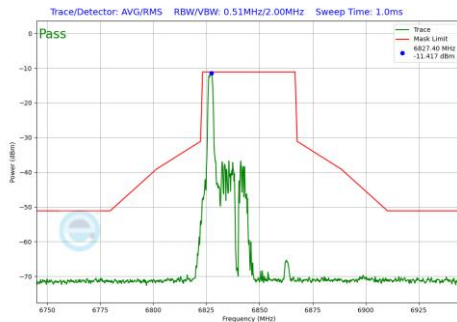
Plot 7-494 In-Band Emission Plot Antenna 4a (40MHz BW 802.11be(RU) RU26 Index0 (UNII Band 7) - Ch.179)
