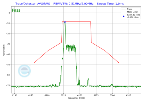
Plot 7-486 In-Band Emission Plot Antenna 4a (40MHz BW 802.11be(RU) RU26 Index0 (UNII Band 5) - Ch.59)
