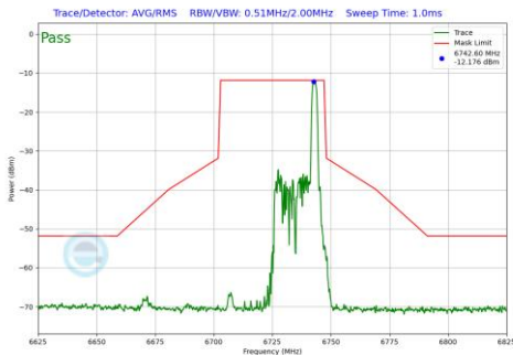
Plot 7-538 In-Band Emission Plot Antenna 2a (40MHz BW 802.11be(RU) RU26 Index17 (UNII Band 7) - Ch.155)
