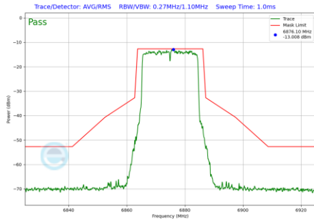
Plot 7-521 In-Band Emission Plot Antenna 4a (20MHz BW 802.11be(RU) RU242 Index61 (UNII Band 7) - Ch.185)
