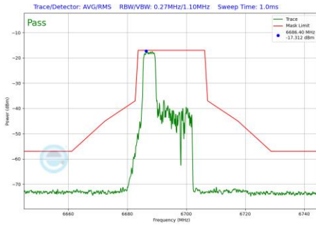
Plot 7-581 In-Band Emission Plot SDM Primary Antenna WF5B (20MHz BW 802.11be(RU) RU52 Index37 (UNII Band 7) - Ch.149)
