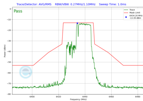
Plot 7-504 In-Band Emission Plot Antenna 4a (20MHz BW 802.11be(RU) RU106+26 Index83 (UNII Band 6) - Ch.97)
