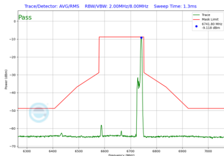
Plot 7-600 In-Band Emission Plot SDM Primary Antenna 4a (160MHz BW 802.11be(RU) RU52 Index52 (UNII Band 7) - Ch.143)
