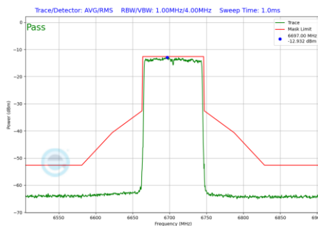
Plot 7-639 In-Band Emission Plot SDM Primary Antenna WF5B (80MHz BW 802.11be(RU) RU996 Index67 (UNII Band 7) - Ch.151)
