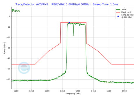
Plot 7-502 In-Band Emission Plot Antenna 4a (80MHz BW 802.11be(RU) RU484+242 Index90 (UNII Band 5) - Ch.87)
