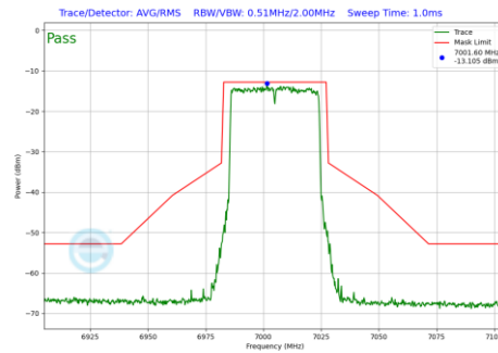
Plot 7-570 In-Band Emission Plot Antenna 2a (40MHz BW 802.11be(RU) RU484 Index65 (UNII Band 8) - Ch.211)
