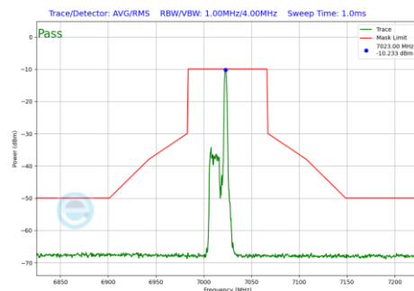
Plot 7-543 In-Band Emission Plot Antenna 2a (80MHz BW 802.11be(RU) RU26 Index17 (UNII Band 8) - Ch.215)
