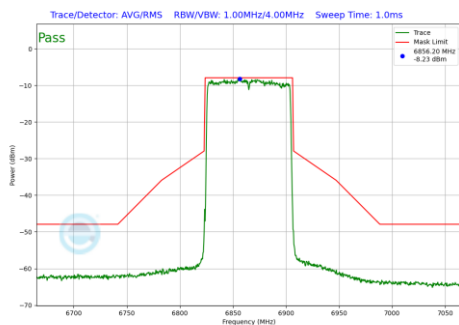
Plot 7-523 In-Band Emission Plot Antenna 4a (80MHz BW 802.11be(RU) RU996 Index67 (UNII Band 7) - Ch.183)
