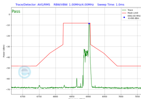
Plot 7-495 In-Band Emission Plot Antenna 4a (80MHz BW 802.11be(RU) RU26 Index36 (UNII Band 7) - Ch.183)
