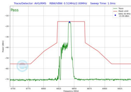
Plot 7-582 In-Band Emission Plot SDM Primary Antenna WF5B (40MHz BW 802.11be(RU) RU52 Index40 (UNII Band 7) - Ch.179)
