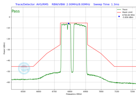
Plot 7-509 In-Band Emission Plot Antenna 4a (160MHz BW 802.11be(RU) RU996+484+242 Index99 (UNII Band 7) - Ch.175)
