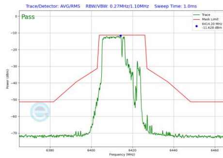
Plot 7-501 In-Band Emission Plot Antenna 4a (20MHz BW 802.11be(RU) RU106+26 Index82 (UNII Band 5) - Ch.93)
