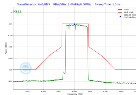
Plot 7-610 In-Band Emission Plot SDM Primary Antenna WF5B (160MHz BW 802.11be(RU) RU996+484+242 Index96 (UNII Band 6) - Ch.111)
