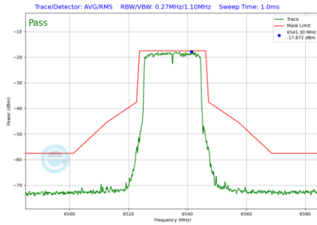
Plot 7-637 In-Band Emission Plot SDM Primary Antenna WF5B (20MHz BW 802.11be(RU) RU242 Index61 (UNII Band 7) - Ch.117)
