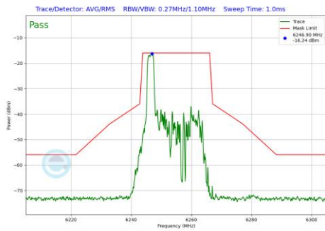
Plot 7-573 In-Band Emission Plot SDM Primary Antenna WF5B (20MHz BW 802.11be(RU) RU26 Index0 (UNII Band 5) - Ch.61)
