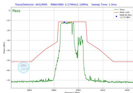
Plot 7-510 In-Band Emission Plot Antenna 4a (20MHz BW 802.11be(RU) RU106+26 Index82 (UNII Band 8) - Ch.189)
