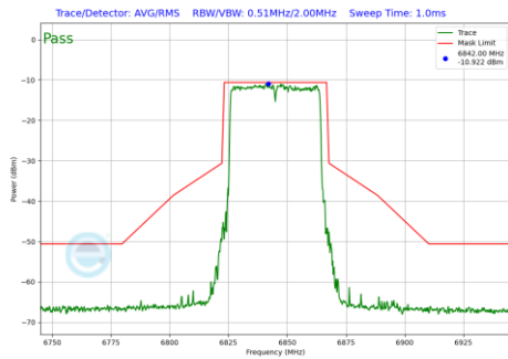
Plot 7-522 In-Band Emission Plot Antenna 4a (40MHz BW 802.11be(RU) RU484 Index65 (UNII Band 7) - Ch.179)
