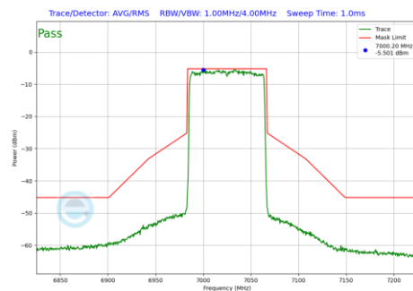
Plot 7-527 In-Band Emission Plot Antenna 4a (80MHz BW 802.11be(RU) RU996 Index67 (UNII Band 8) - Ch.215)
