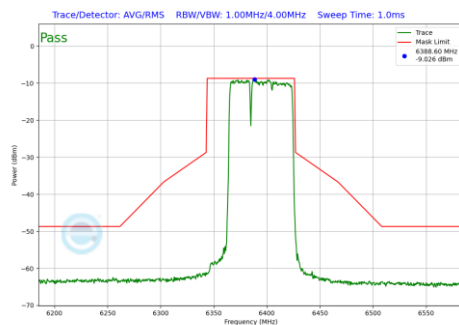
Plot 7-546 In-Band Emission Plot Antenna 2a (80MHz BW 802.11be(RU) RU484+242 Index90 (UNII Band 5) - Ch.87)
