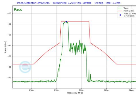
Plot 7-585 In-Band Emission Plot SDM Primary Antenna WF5B (20MHz BW 802.11be(RU) RU52 Index37 (UNII Band 8) - Ch.229)
