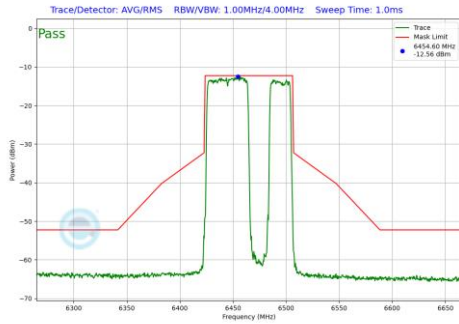
Plot 7-621 In-Band Emission Plot SDM Primary Antenna 4a (80MHz BW 802.11be(RU) RU484+242 Index92 (UNII Band 6) - Ch.103)
