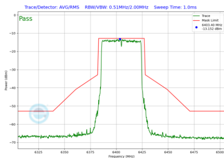
Plot 7-630 In-Band Emission Plot SDM Primary Antenna WF5B (40MHz BW 802.11be(RU) RU484 Index65 (UNII Band 5) - Ch.91)
