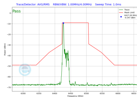
Plot 7-535 In-Band Emission Plot Antenna 2a (80MHz BW 802.11be(RU) RU26 Index0 (UNII Band 6) - Ch.103)
