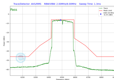
Plot 7-520 In-Band Emission Plot Antenna 4a (160MHz BW 802.11be(RU) RU996X2 Index68 (UNII Band 6) - Ch.111)
