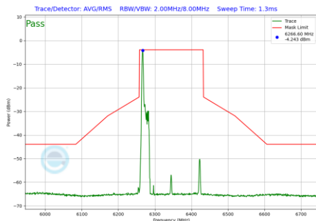
Plot 7-488 In-Band Emission Plot Antenna 4a (160MHz BW 802.11be(RU) RU26 Index0 (UNII Band 5) - Ch.79)
