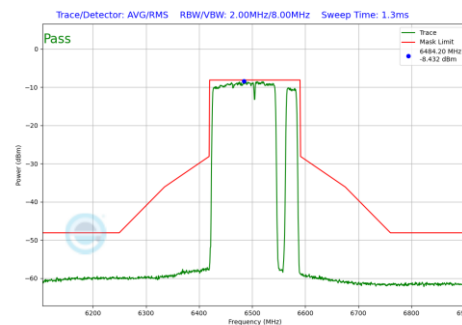
Plot 7-550 In-Band Emission Plot Antenna 2a (160MHz BW 802.11be(RU) RU996+484+242 Index98 (UNII Band 6) - Ch.111)
