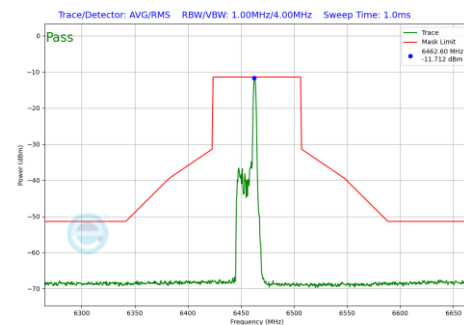
Plot 7-595 In-Band Emission Plot SDM Primary Antenna 4a (80MHz BW 802.11be(RU) RU26 Index17 (UNII Band 6) - Ch.103)
