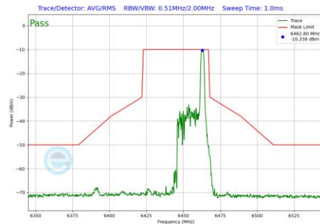
Plot 7-490 In-Band Emission Plot Antenna 4a (40MHz BW 802.11be(RU) RU26 Index17 (UNII Band 6) - Ch.99)
