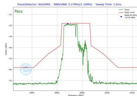
Plot 7-611 In-Band Emission Plot SDM Primary Antenna WF5B (20MHz BW 802.11be(RU) RU106+26 Index82 (UNII Band 7) - Ch.185)
