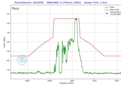
Plot 7-541 In-Band Emission Plot Antenna 2a (20MHz BW 802.11be(RU) RU26 Index8 (UNII Band 8) - Ch.209)
