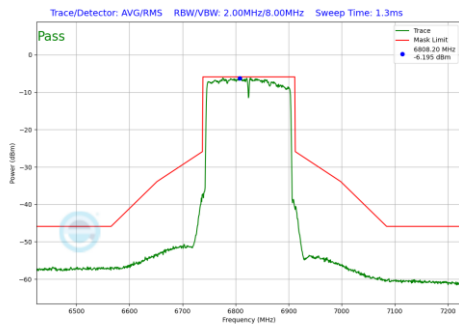
Plot 7-524 In-Band Emission Plot Antenna 4a (160MHz BW 802.11be(RU) RU996X2 Index68 (UNII Band 7) - Ch.175)
