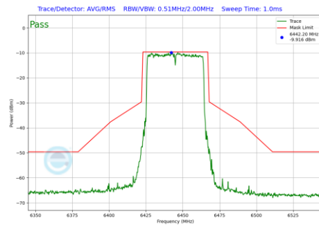
Plot 7-518 In-Band Emission Plot Antenna 4a (40MHz BW 802.11be(RU) RU484 Index65 (UNII Band 6) - Ch.99)
