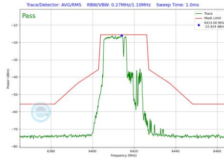
Plot 7-617 In-Band Emission Plot SDM Primary Antenna 4a (20MHz BW 802.11be(RU) RU106+26 Index82 (UNII Band 5) - Ch.93)
