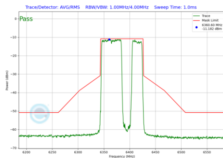
Plot 7-606 In-Band Emission Plot SDM Primary Antenna WF5B (80MHz BW 802.11be(RU) RU484+242 Index92 (UNII Band 5) - Ch.87)
