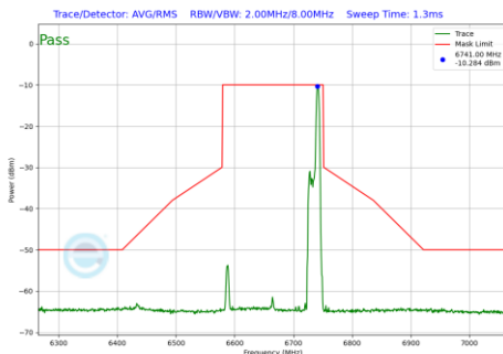
Plot 7-584 In-Band Emission Plot SDM Primary Antenna WF5B (160MHz BW 802.11be(RU) RU52 Index52 (UNII Band 7) - Ch.143)
