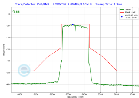
Plot 7-632 In-Band Emission Plot SDM Primary Antenna WF5B (160MHz BW 802.11be(RU) RU996X2 Index68 (UNII Band 5) - Ch.79)
