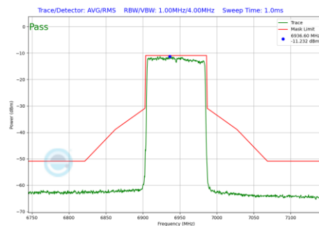
Plot 7-571 In-Band Emission Plot Antenna 2a (80MHz BW 802.11be(RU) RU996 Index67 (UNII Band 8) - Ch.199)
