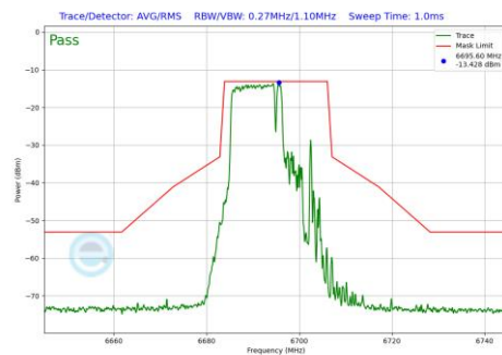
Plot 7-507 In-Band Emission Plot Antenna 4a (20MHz BW 802.11be(RU) RU106+26 Index82 (UNII Band 7) - Ch.149)
