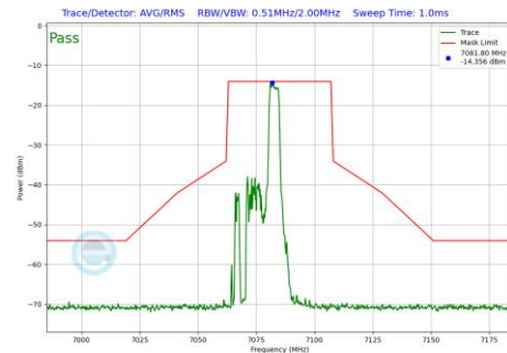
Plot 7-586 In-Band Emission Plot SDM Primary Antenna WF5B (40MHz BW 802.11be(RU) RU52 Index40 (UNII Band 8) - Ch.227)
