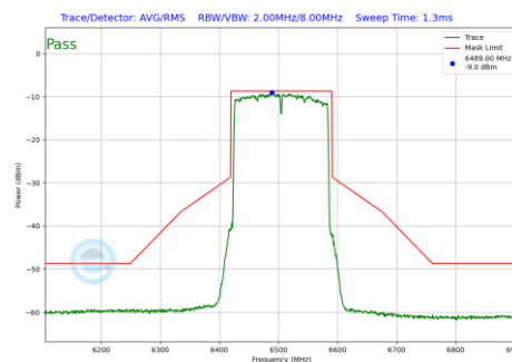
Plot 7-564 In-Band Emission Plot Antenna 2a (160MHz BW 802.11be(RU) RU996X2 Index68 (UNII Band 6) - Ch.111)
