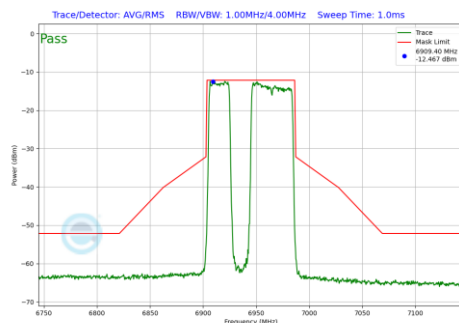
Plot 7-615 In-Band Emission Plot SDM Primary Antenna WF5B (80MHz BW 802.11be(RU) RU484+242 Index91 (UNII Band 8) - Ch.199)
