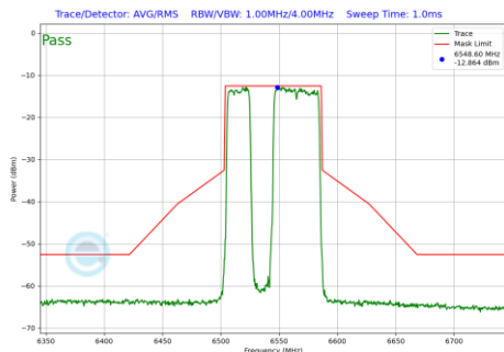
Plot 7-624 In-Band Emission Plot SDM Primary Antenna 4a (80MHz BW 802.11be(RU) RU484+242 Index91 (UNII Band 7) - Ch.119)
