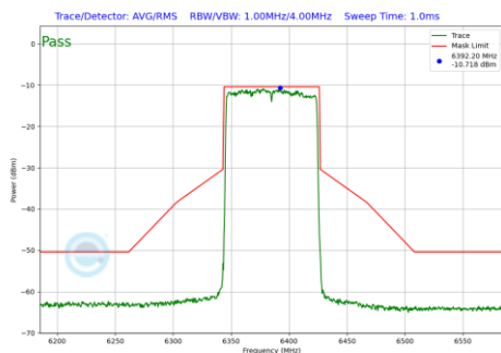
Plot 7-631 In-Band Emission Plot SDM Primary Antenna WF5B (80MHz BW 802.11be(RU) RU996 Index67 (UNII Band 5) - Ch.87)
