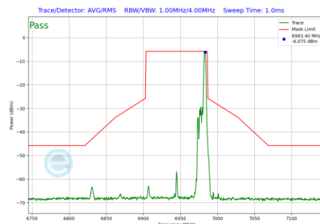
Plot 7-499 In-Band Emission Plot Antenna 4a (80MHz BW 802.11be(RU) RU26 Index36 (UNII Band 8) - Ch.199)
