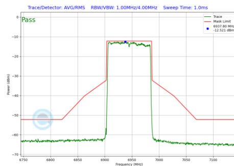
Plot 7-643 In-Band Emission Plot SDM Primary Antenna WF5B (80MHz BW 802.11be(RU) RU996 Index67 (UNII Band 8) - Ch.199)
