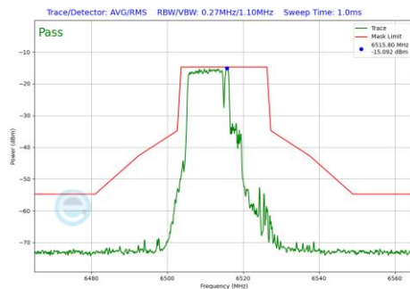
Plot 7-548 In-Band Emission Plot Antenna 2a (20MHz BW 802.11be(RU) RU106+26 Index82 (UNII Band 6) - Ch.113)
