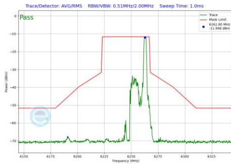
Plot 7-530 In-Band Emission Plot Antenna 2a (40MHz BW 802.11be(RU) RU26 Index17 (UNII Band 5) - Ch.59)
