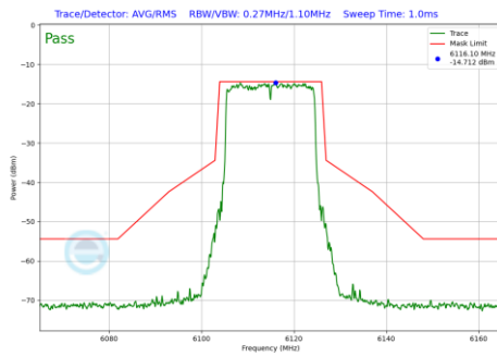
Plot 7-557 In-Band Emission Plot Antenna 2a (20MHz BW 802.11be(RU) RU242 Index61 (UNII Band 5) - Ch.33)
