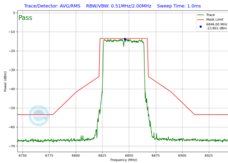
Plot 7-566 In-Band Emission Plot Antenna 2a (40MHz BW 802.11be(RU) RU484 Index65 (UNII Band 7) - Ch.179)
