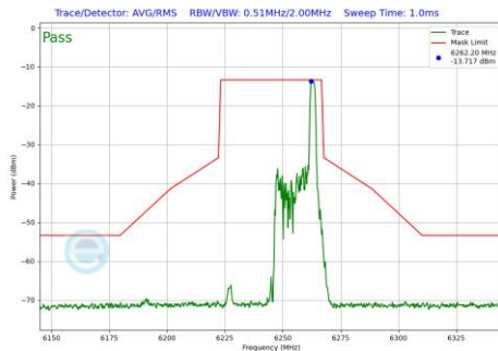
Plot 7-590 In-Band Emission Plot SDM Primary Antenna 4a (40MHz BW 802.11be(RU) RU26 Index17 (UNII Band 5) - Ch.59)
