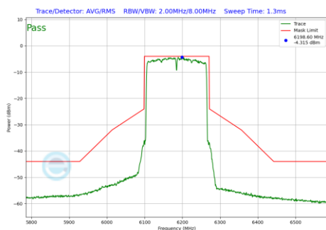
Plot 7-516 In-Band Emission Plot Antenna 4a (160MHz BW 802.11be(RU) RU996X2 Index68 (UNII Band 5) - Ch.47)
