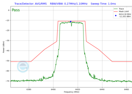
Plot 7-513 In-Band Emission Plot Antenna 4a (20MHz BW 802.11be(RU) RU242 Index61 (UNII Band 5) - Ch.93)
