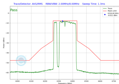
Plot 7-607 In-Band Emission Plot SDM Primary Antenna WF5B (160MHz BW 802.11be(RU) RU996+484+242 Index97 (UNII Band 5) - Ch.79)
