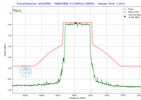
Plot 7-526 In-Band Emission Plot Antenna 4a (40MHz BW 802.11be(RU) RU484 Index65 (UNII Band 8) - Ch.211)
