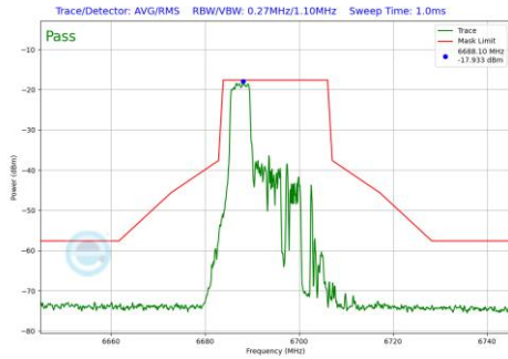
Plot 7-597 In-Band Emission Plot SDM Primary Antenna 4a (20MHz BW 802.11be(RU) RU52 Index37 (UNII Band 7) - Ch.149)
