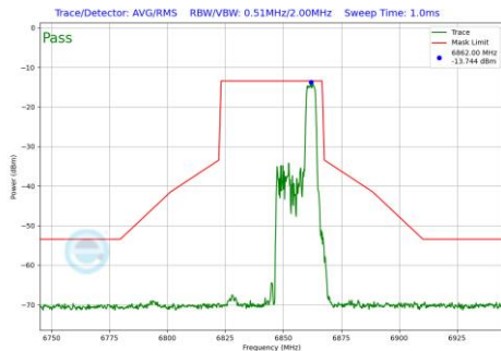
Plot 7-686 In-Band Emission Plot SDM Diversity Antenna 4a (40MHz BW 802.11be(RU) RU52 Index44 (UNII Band 7) - Ch.179)
