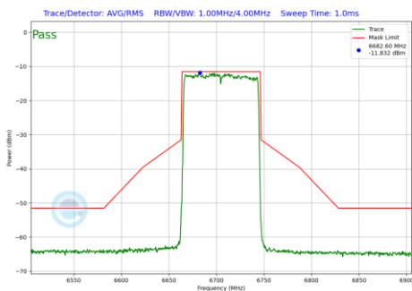
Plot 7-655 In-Band Emission Plot SDM Primary Antenna 4a (80MHz BW 802.11be(RU) RU996 Index67 (UNII Band 7) - Ch.151)
