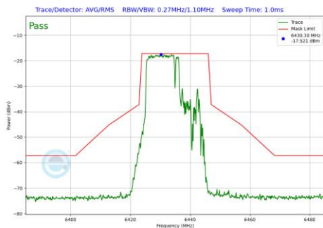
Plot 7-696 In-Band Emission Plot SDM Diversity Antenna 2a (20MHz BW 802.11be(RU) RU106+26 Index82 (UNII Band 6) - Ch.97)
