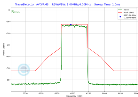
Plot 7-727 In-Band Emission Plot SDM Diversity Antenna 2a (80MHz BW 802.11be(RU) RU996 Index67 (UNII Band 7) - Ch.151)
