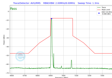
Plot 7-692 In-Band Emission Plot SDM Diversity Antenna 4a (160MHz BW 802.11be(RU) RU52 Index37 (UNII Band 8) - Ch.207)
