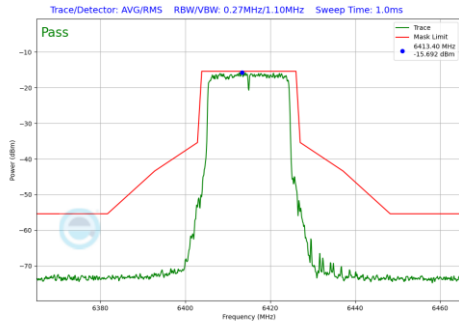
Plot 7-645 In-Band Emission Plot SDM Primary Antenna 4a (20MHz BW 802.11be(RU) RU242 Index61 (UNII Band 5) - Ch.93)
