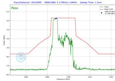
Plot 7-689 In-Band Emission Plot SDM Diversity Antenna 4a (20MHz BW 802.11be(RU) RU52 Index37 (UNII Band 8) - Ch.229)
