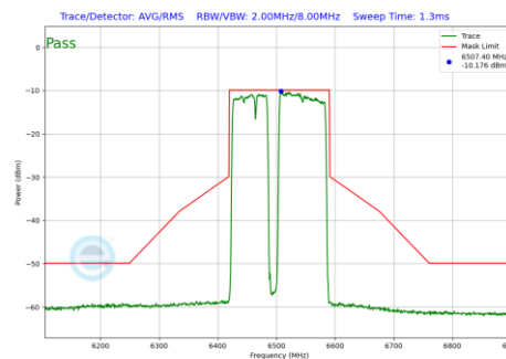
Plot 7-698 In-Band Emission Plot SDM Diversity Antenna 2a (160MHz BW 802.11be(RU) RU996+484+242 Index99 (UNII Band 6) - Ch.111)
