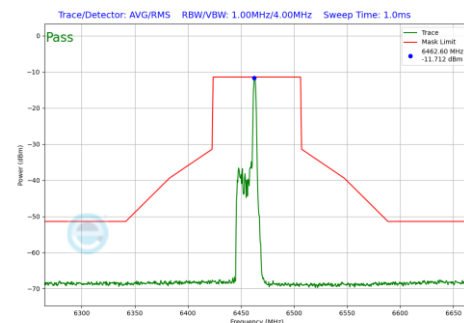
Plot 7-683 In-Band Emission Plot SDM Diversity Antenna 4a (80MHz BW 802.11be(RU) RU26 Index17 (UNII Band 6) - Ch.103)
