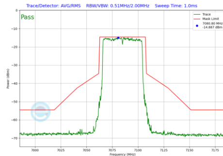
Plot 7-730 In-Band Emission Plot SDM Diversity Antenna 2a (40MHz BW 802.11be(RU) RU484 Index65 (UNII Band 8) - Ch.227)
