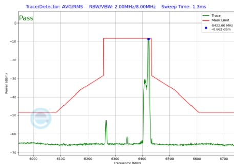
Plot 7-680 In-Band Emission Plot SDM Diversity Antenna 4a (160MHz BW 802.11be(RU) RU26 Index36 (UNII Band 5) - Ch.79)
