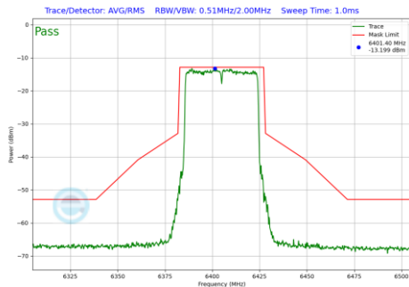
Plot 7-646 In-Band Emission Plot SDM Primary Antenna 4a (40MHz BW 802.11be(RU) RU484 Index65 (UNII Band 5) - Ch.91)
