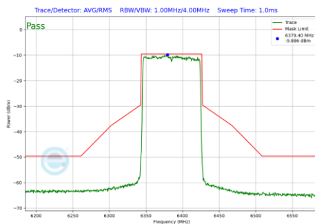
Plot 7-735 In-Band Emission Plot SDM Diversity Antenna 4a (80MHz BW 802.11be(RU) RU996 Index67 (UNII Band 5) - Ch.87)
