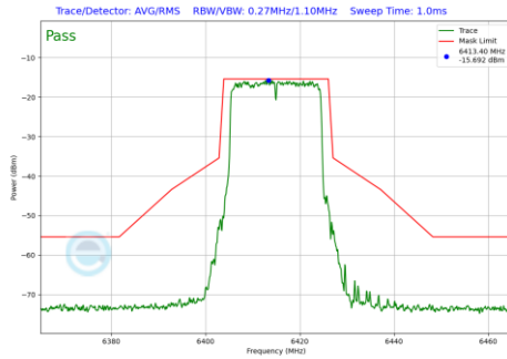
Plot 7-733 In-Band Emission Plot SDM Diversity Antenna 4a (20MHz BW 802.11be(RU) RU242 Index61 (UNII Band 5) - Ch.93)
