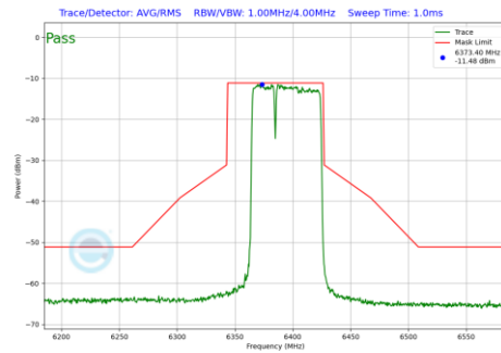
Plot 7-706 In-Band Emission Plot SDM Diversity Antenna 4a (80MHz BW 802.11be(RU) RU484+242 Index90 (UNII Band 5) - Ch.87)
