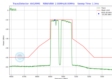
Plot 7-704 In-Band Emission Plot SDM Diversity Antenna 2a (160MHz BW 802.11be(RU) RU996+484+242 Index99 (UNII Band 8) - Ch.207)
