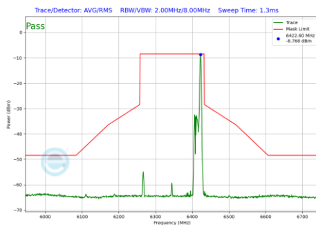
Plot 7-664 In-Band Emission Plot SDM Diversity Antenna 2a (160MHz BW 802.11be(RU) RU26 Index36 (UNII Band 5) - Ch.79)
