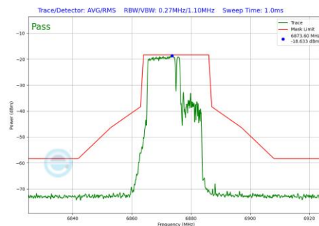
Plot 7-699 In-Band Emission Plot SDM Diversity Antenna 2a (20MHz BW 802.11be(RU) RU106+26 Index82 (UNII Band 7) - Ch.185)
