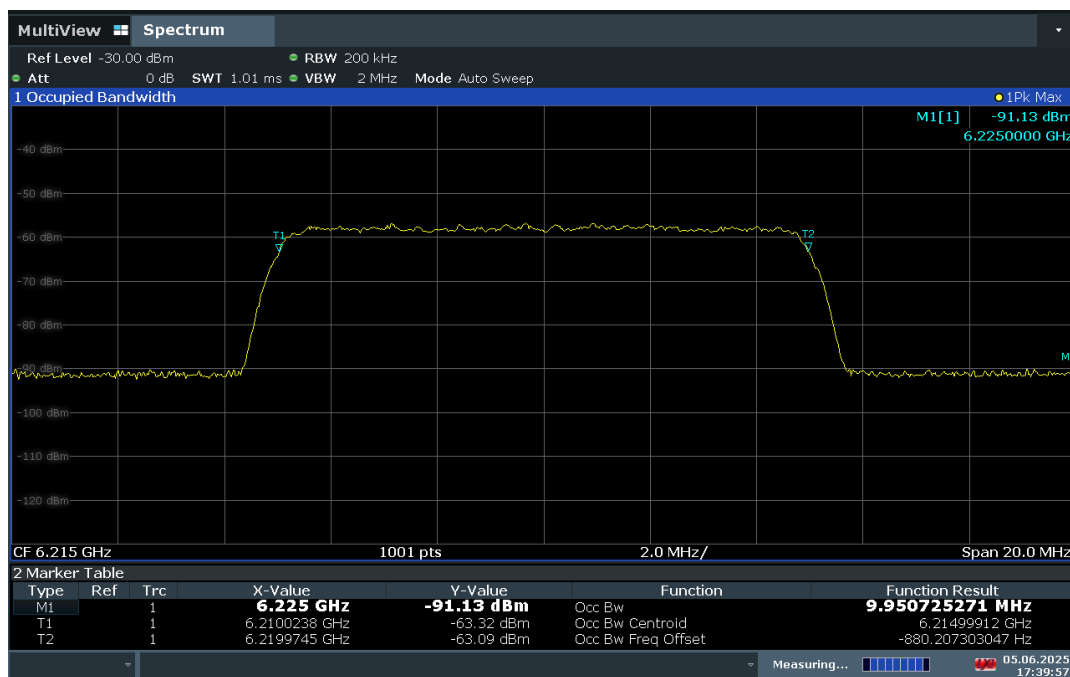
Plot 7-749. AWGN Signal – UNII 5 – 20MHz
