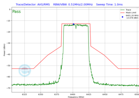
Plot 7-718 In-Band Emission Plot SDM Diversity Antenna 2a (40MHz BW 802.11be(RU) RU484 Index65 (UNII Band 5) - Ch.91)
