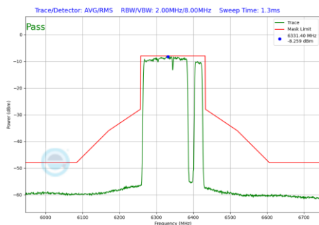
Plot 7-695 In-Band Emission Plot SDM Diversity Antenna 2a (160MHz BW 802.11be(RU) RU996+484+242 Index98 (UNII Band 5) - Ch.79)
