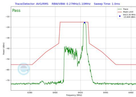
Plot 7-661 In-Band Emission Plot SDM Diversity Antenna 2a (20MHz BW 802.11be(RU) RU26 Index8 (UNII Band 5) - Ch.93)
