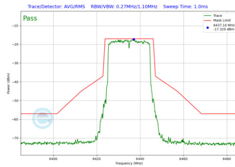
Plot 7-721 In-Band Emission Plot SDM Diversity Antenna 2a (20MHz BW 802.11be(RU) RU242 Index61 (UNII Band 6) - Ch.97)
