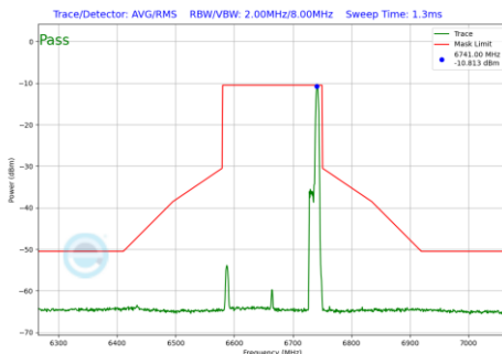
Plot 7-672 In-Band Emission Plot SDM Diversity Antenna 2a (160MHz BW 802.11be(RU) RU52 Index52 (UNII Band 7) - Ch.143)
