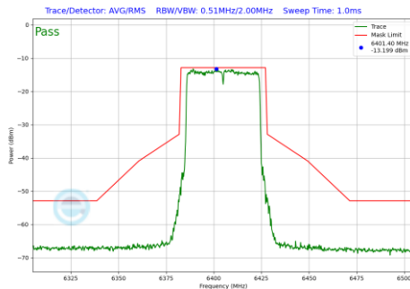
Plot 7-734 In-Band Emission Plot SDM Diversity Antenna 4a (40MHz BW 802.11be(RU) RU484 Index65 (UNII Band 5) - Ch.91)
