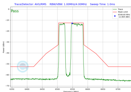
Plot 7-712 In-Band Emission Plot SDM Diversity Antenna 4a (80MHz BW 802.11be(RU) RU484+242 Index91 (UNII Band 7) - Ch.119)
