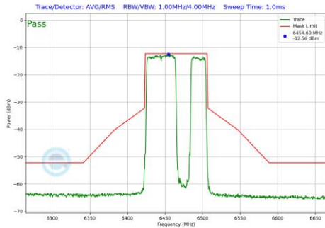
Plot 7-709 In-Band Emission Plot SDM Diversity Antenna 4a (80MHz BW 802.11be(RU) RU484+242 Index92 (UNII Band 6) - Ch.103)
