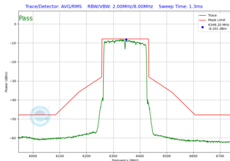
Plot 7-736 In-Band Emission Plot SDM Diversity Antenna 4a (160MHz BW 802.11be(RU) RU996X2 Index68 (UNII Band 5) - Ch.79)
