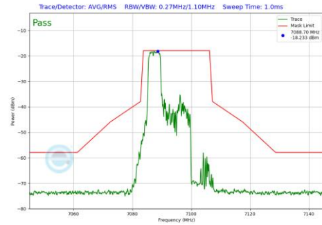
Plot 7-673 In-Band Emission Plot SDM Diversity Antenna 2a (20MHz BW 802.11be(RU) RU52 Index37 (UNII Band 8) - Ch.229)
