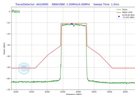
Plot 7-719 In-Band Emission Plot SDM Diversity Antenna 2a (80MHz BW 802.11be(RU) RU996 Index67 (UNII Band 5) - Ch.87)
