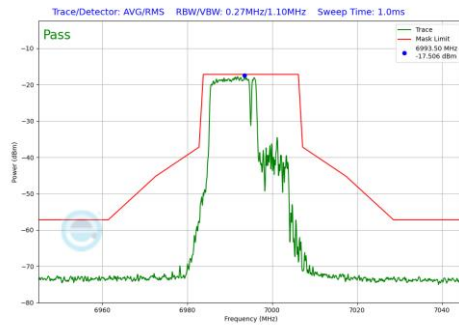
Plot 7-702 In-Band Emission Plot SDM Diversity Antenna 2a (20MHz BW 802.11be(RU) RU106+26 Index82 (UNII Band 8) - Ch.209)
