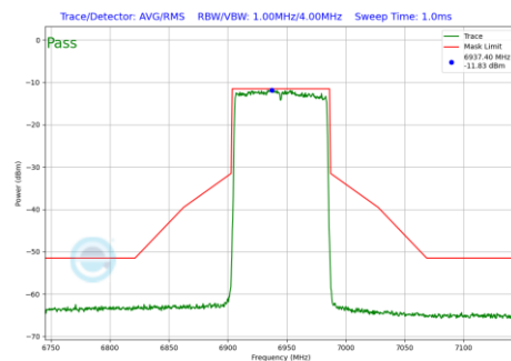
Plot 7-659 In-Band Emission Plot SDM Primary Antenna 4a (80MHz BW 802.11be(RU) RU996 Index67 (UNII Band 8) - Ch.199)
