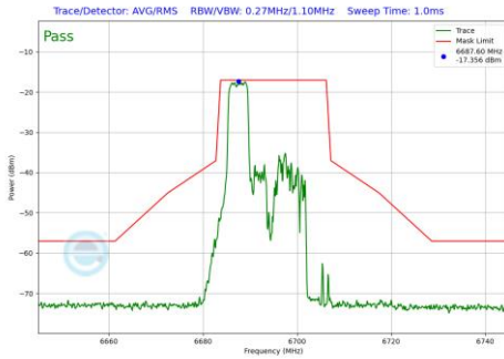
Plot 7-669 In-Band Emission Plot SDM Diversity Antenna 2a (20MHz BW 802.11be(RU) RU52 Index37 (UNII Band 7) - Ch.149)
