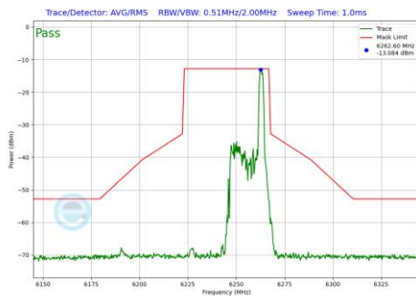
Plot 7-662 In-Band Emission Plot SDM Diversity Antenna 2a (40MHz BW 802.11be(RU) RU26 Index17 (UNII Band 5) - Ch.59)
