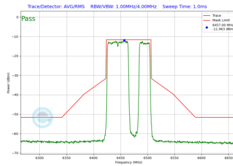
Plot 7-697 In-Band Emission Plot SDM Diversity Antenna 2a (80MHz BW 802.11be(RU) RU484+242 Index92 (UNII Band 6) - Ch.103)
