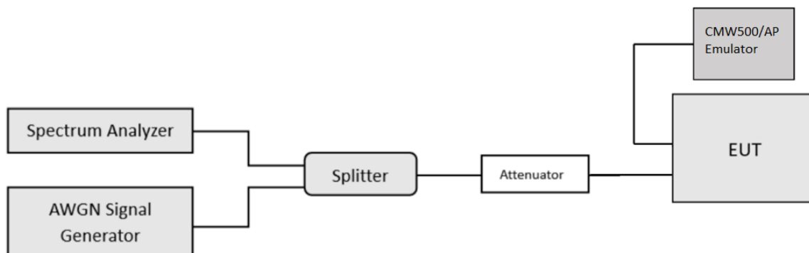
Figure 2. Contention-based protocol test setup, conducted method
