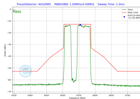
Plot 7-700 In-Band Emission Plot SDM Diversity Antenna 2a (80MHz BW 802.11be(RU) RU484+242 Index91 (UNII Band 7) - Ch.119)
