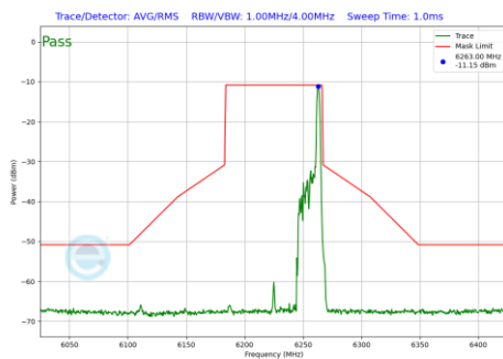
Plot 7-663 In-Band Emission Plot SDM Diversity Antenna 2a (80MHz BW 802.11be(RU) RU26 Index36 (UNII Band 5) - Ch.55)
