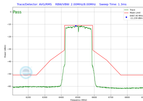
Plot 7-724 In-Band Emission Plot SDM Diversity Antenna 2a (160MHz BW 802.11be(RU) RU996X2 Index68 (UNII Band 6) - Ch.111)
