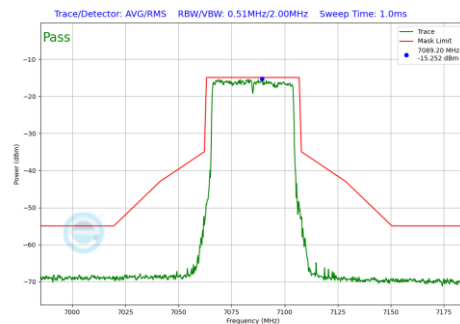
Plot 7-746 In-Band Emission Plot SDM Diversity Antenna 4a (40MHz BW 802.11be(RU) RU484 Index65 (UNII Band 8) - Ch.227)
