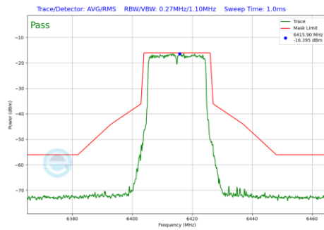
Plot 7-717 In-Band Emission Plot SDM Diversity Antenna 2a (20MHz BW 802.11be(RU) RU242 Index61 (UNII Band 5) - Ch.93)
