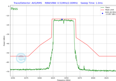
Plot 7-650 In-Band Emission Plot SDM Primary Antenna 4a (40MHz BW 802.11be(RU) RU484 Index65 (UNII Band 6) - Ch.99)
