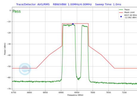
Plot 7-715 In-Band Emission Plot SDM Diversity Antenna 4a (80MHz BW 802.11be(RU) RU484+242 Index92 (UNII Band 8) - Ch.199)
