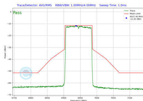
Plot 7-747 In-Band Emission Plot SDM Diversity Antenna 4a (80MHz BW 802.11be(RU) RU996 Index67 (UNII Band 8) - Ch.199)
