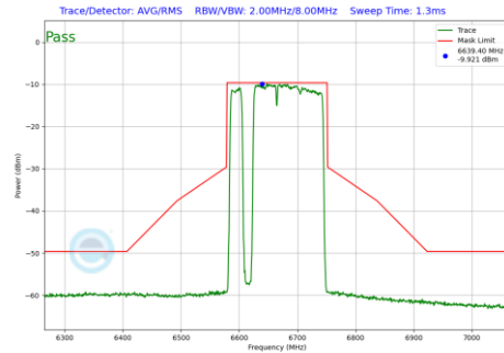
Plot 7-713 In-Band Emission Plot SDM Diversity Antenna 4a (160MHz BW 802.11be(RU) RU996+484+242 Index97 (UNII Band 7) - Ch.143)
