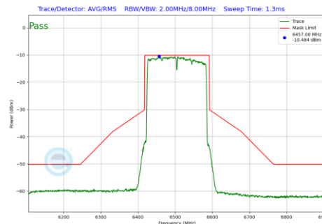
Plot 7-652 In-Band Emission Plot SDM Primary Antenna 4a (160MHz BW 802.11be(RU) RU996X2 Index68 (UNII Band 6) - Ch.111)
