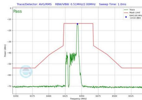
Plot 7-666 In-Band Emission Plot SDM Diversity Antenna 2a (40MHz BW 802.11be(RU) RU26 Index8 (UNII Band 6) - Ch.99)
