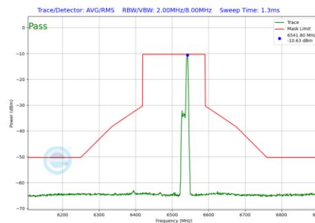
Plot 7-668 In-Band Emission Plot SDM Diversity Antenna 2a (160MHz BW 802.11be(RU) RU52 Index44 (UNII Band 6) - Ch.111)
