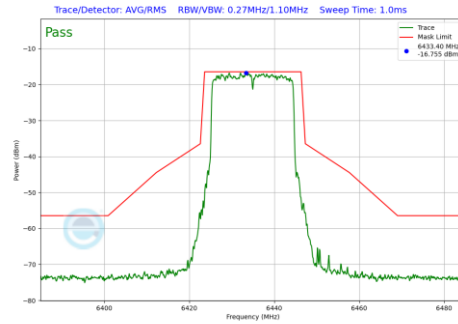
Plot 7-737 In-Band Emission Plot SDM Diversity Antenna 4a (20MHz BW 802.11be(RU) RU242 Index61 (UNII Band 6) - Ch.97)
