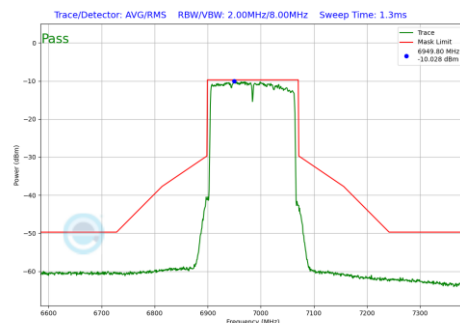
Plot 7-660 In-Band Emission Plot SDM Primary Antenna 4a (160MHz BW 802.11be(RU) RU996X2 Index68 (UNII Band 8) - Ch.207)
