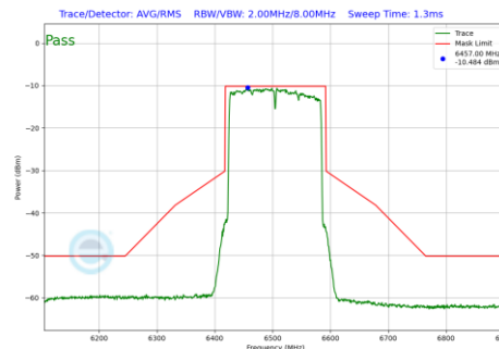
Plot 7-740 In-Band Emission Plot SDM Diversity Antenna 4a (160MHz BW 802.11be(RU) RU996X2 Index68 (UNII Band 6) - Ch.111)
