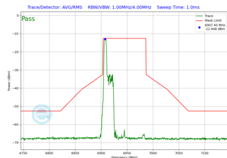
Plot 7-675 In-Band Emission Plot SDM Diversity Antenna 2a (80MHz BW 802.11be(RU) RU52 Index37 (UNII Band 8) - Ch.199)
