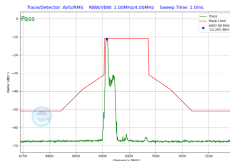
Plot 7-691 In-Band Emission Plot SDM Diversity Antenna 4a (80MHz BW 802.11be(RU) RU52 Index37 (UNII Band 8) - Ch.199)
