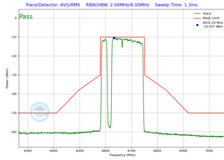
Plot 7-701 In-Band Emission Plot SDM Diversity Antenna 2a (160MHz BW 802.11be(RU) RU996+484+242 Index97 (UNII Band 7) - Ch.143)
