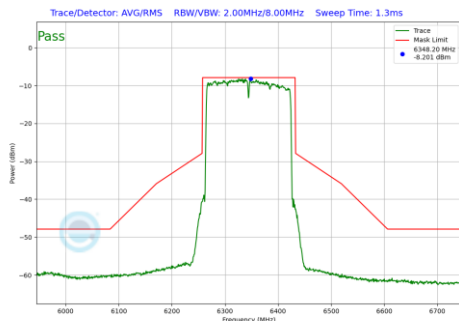
Plot 7-648 In-Band Emission Plot SDM Primary Antenna 4a (160MHz BW 802.11be(RU) RU996X2 Index68 (UNII Band 5) - Ch.79)
