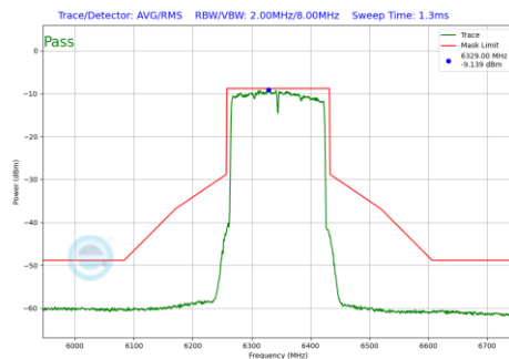
Plot 7-720 In-Band Emission Plot SDM Diversity Antenna 2a (160MHz BW 802.11be(RU) RU996X2 Index68 (UNII Band 5) - Ch.79)
