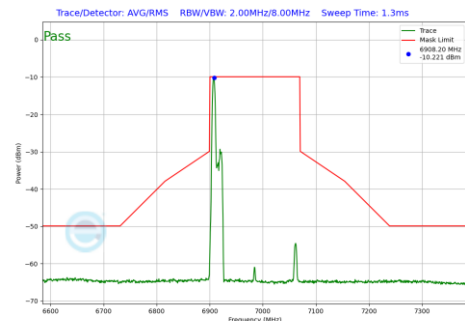
Plot 7-676 In-Band Emission Plot SDM Diversity Antenna 2a (160MHz BW 802.11be(RU) RU52 Index37 (UNII Band 8) - Ch.207)
