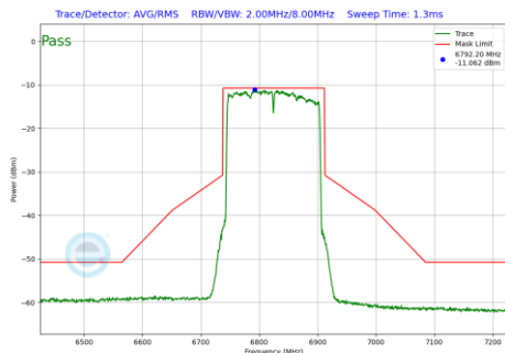
Plot 7-728 In-Band Emission Plot SDM Diversity Antenna 2a (160MHz BW 802.11be(RU) RU996X2 Index68 (UNII Band 7) - Ch.175)
