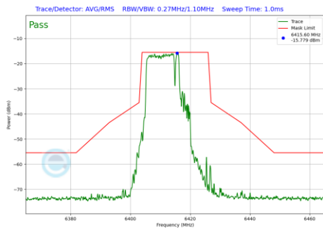
Plot 7-693 In-Band Emission Plot SDM Diversity Antenna 2a (20MHz BW 802.11be(RU) RU106+26 Index82 (UNII Band 5) - Ch.93)
