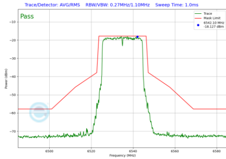
Plot 7-725 In-Band Emission Plot SDM Diversity Antenna 2a (20MHz BW 802.11be(RU) RU242 Index61 (UNII Band 7) - Ch.117)
