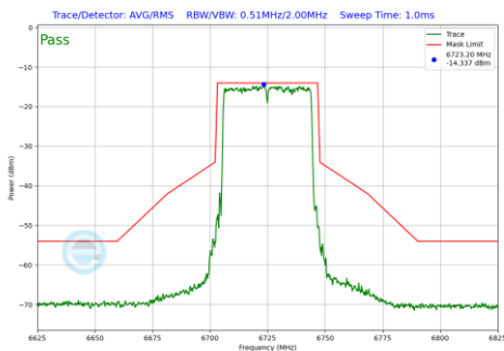
Plot 7-742 In-Band Emission Plot SDM Diversity Antenna 4a (40MHz BW 802.11be(RU) RU484 Index65 (UNII Band 7) - Ch.155)
