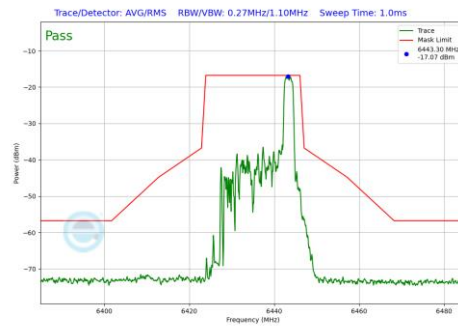
Plot 7-665 In-Band Emission Plot SDM Diversity Antenna 2a (20MHz BW 802.11be(RU) RU26 Index8 (UNII Band 6) - Ch.97)
