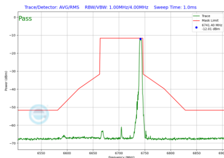
Plot 7-687 In-Band Emission Plot SDM Diversity Antenna 4a (80MHz BW 802.11be(RU) RU52 Index52 (UNII Band 7) - Ch.151)
