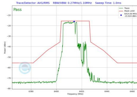
Plot 7-705 In-Band Emission Plot SDM Diversity Antenna 4a (20MHz BW 802.11be(RU) RU106+26 Index82 (UNII Band 5) - Ch.93)
