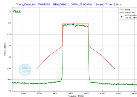
Plot 7-739 In-Band Emission Plot SDM Diversity Antenna 4a (80MHz BW 802.11be(RU) RU996 Index67 (UNII Band 6) - Ch.103)
