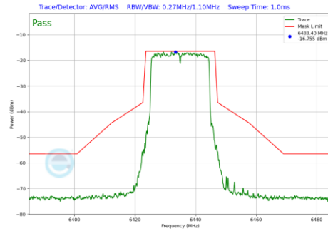
Plot 7-649 In-Band Emission Plot SDM Primary Antenna 4a (20MHz BW 802.11be(RU) RU242 Index61 (UNII Band 6) - Ch.97)
