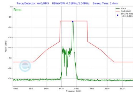
Plot 7-682 In-Band Emission Plot SDM Diversity Antenna 4a (40MHz BW 802.11be(RU) RU26 Index8 (UNII Band 6) - Ch.99)
