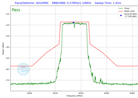
Plot 7-653 In-Band Emission Plot SDM Primary Antenna 4a (20MHz BW 802.11be(RU) RU242 Index61 (UNII Band 7) - Ch.117)
