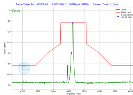
Plot 7-667 In-Band Emission Plot SDM Diversity Antenna 2a (80MHz BW 802.11be(RU) RU26 Index17 (UNII Band 6) - Ch.103)
