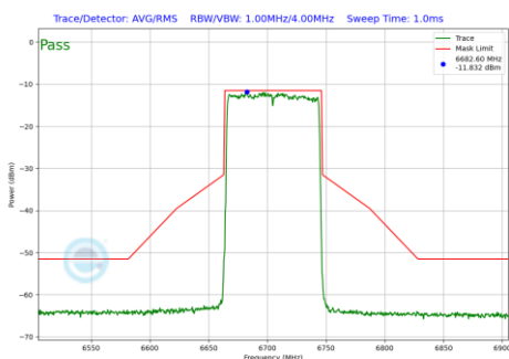
Plot 7-743 In-Band Emission Plot SDM Diversity Antenna 4a (80MHz BW 802.11be(RU) RU996 Index67 (UNII Band 7) - Ch.151)
