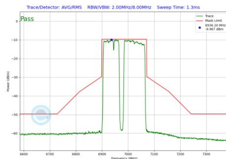
Plot 7-716 In-Band Emission Plot SDM Diversity Antenna 4a (160MHz BW 802.11be(RU) RU996+484+242 Index99 (UNII Band 8) - Ch.207)
