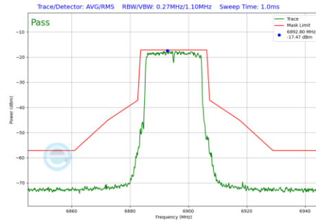
Plot 7-729 In-Band Emission Plot SDM Diversity Antenna 2a (20MHz BW 802.11be(RU) RU242 Index61 (UNII Band 8) - Ch.189)
