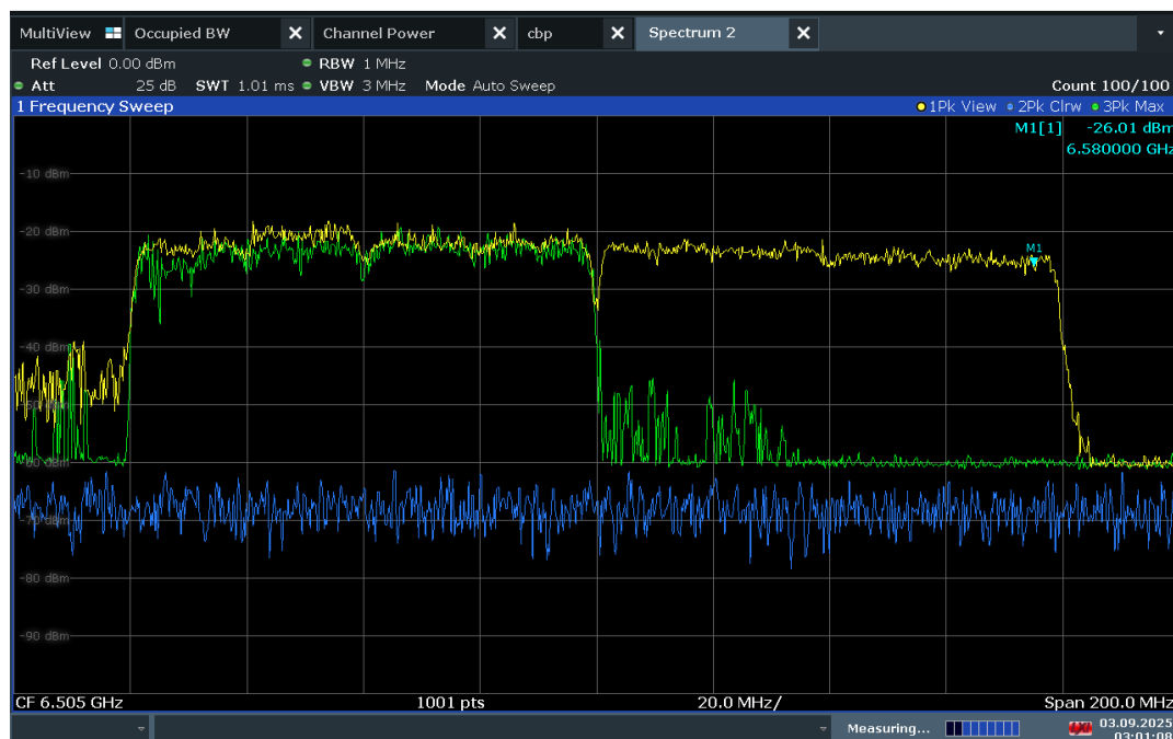
Plot 7-783. 160MHz Bandwidth, AWGN Signal Injected – 6580MHz
