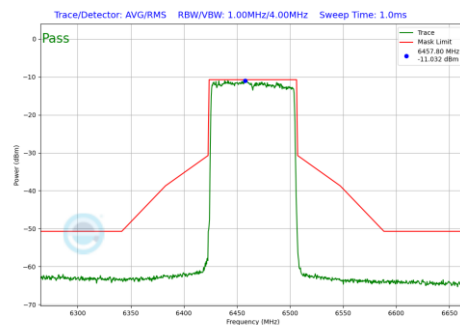
Plot 7-651 In-Band Emission Plot SDM Primary Antenna 4a (80MHz BW 802.11be(RU) RU996 Index67 (UNII Band 6) - Ch.103)
