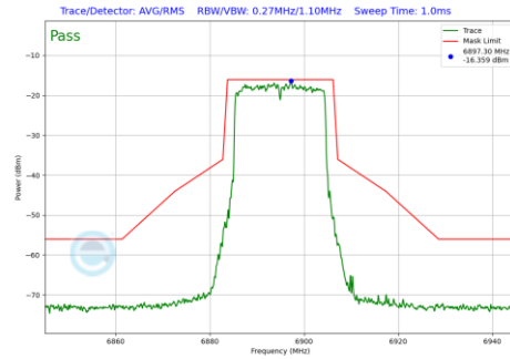
Plot 7-745 In-Band Emission Plot SDM Diversity Antenna 4a (20MHz BW 802.11be(RU) RU242 Index61 (UNII Band 8) - Ch.189)
