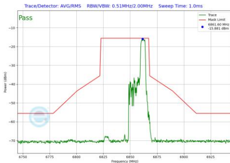
Plot 7-670 In-Band Emission Plot SDM Diversity Antenna 2a (40MHz BW 802.11be(RU) RU52 Index44 (UNII Band 7) - Ch.179)
