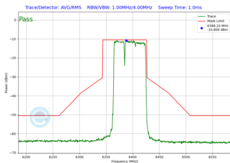
Plot 7-694 In-Band Emission Plot SDM Diversity Antenna 2a (80MHz BW 802.11be(RU) RU484+242 Index90 (UNII Band 5) - Ch.87)
