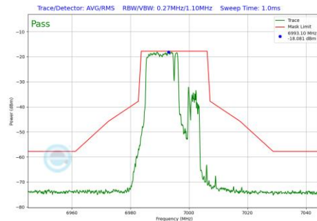
Plot 7-714 In-Band Emission Plot SDM Diversity Antenna 4a (20MHz BW 802.11be(RU) RU106+26 Index82 (UNII Band 8) - Ch.209)
