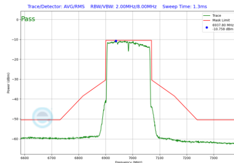
Plot 7-732 In-Band Emission Plot SDM Diversity Antenna 2a (160MHz BW 802.11be(RU) RU996X2 Index68 (UNII Band 8) - Ch.207)
