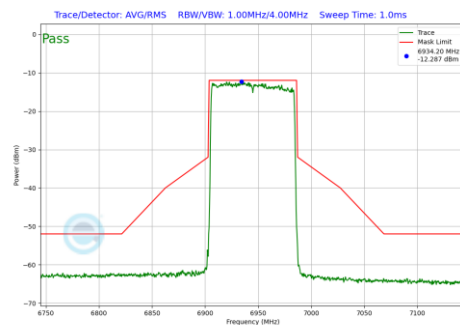
Plot 7-731 In-Band Emission Plot SDM Diversity Antenna 2a (80MHz BW 802.11be(RU) RU996 Index67 (UNII Band 8) - Ch.199)
