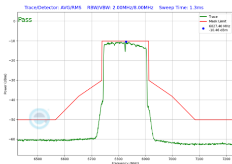
Plot 7-656 In-Band Emission Plot SDM Primary Antenna 4a (160MHz BW 802.11be(RU) RU996X2 Index68 (UNII Band 7) - Ch.175)
