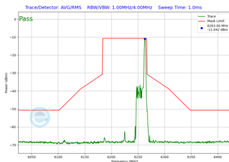
Plot 7-679 In-Band Emission Plot SDM Diversity Antenna 4a (80MHz BW 802.11be(RU) RU26 Index36 (UNII Band 5) - Ch.55)
