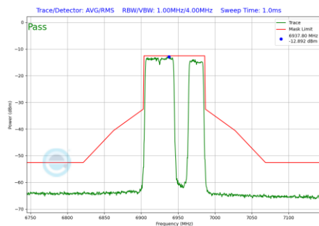
Plot 7-703 In-Band Emission Plot SDM Diversity Antenna 2a (80MHz BW 802.11be(RU) RU484+242 Index92 (UNII Band 8) - Ch.199)
