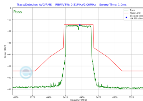
Plot 7-722 In-Band Emission Plot SDM Diversity Antenna 2a (40MHz BW 802.11be(RU) RU484 Index65 (UNII Band 6) - Ch.99)
