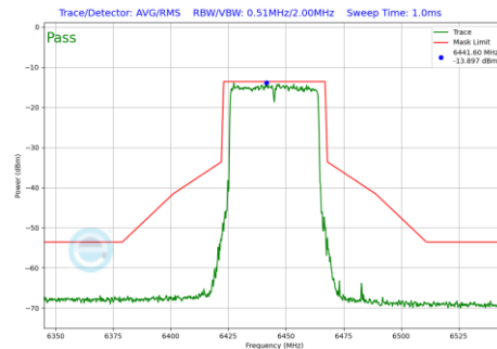
Plot 7-738 In-Band Emission Plot SDM Diversity Antenna 4a (40MHz BW 802.11be(RU) RU484 Index65 (UNII Band 6) - Ch.99)
