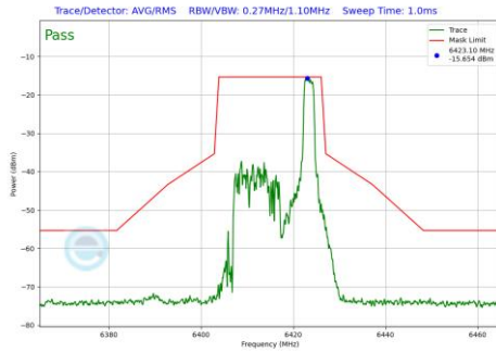
Plot 7-677 In-Band Emission Plot SDM Diversity Antenna 4a (20MHz BW 802.11be(RU) RU26 Index8 (UNII Band 5) - Ch.93)
