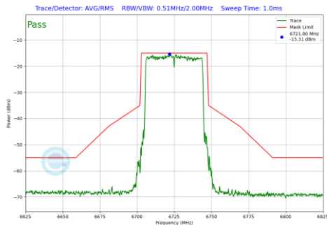
Plot 7-726 In-Band Emission Plot SDM Diversity Antenna 2a (40MHz BW 802.11be(RU) RU484 Index65 (UNII Band 7) - Ch.155)
