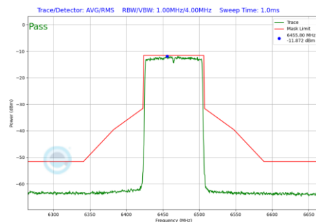
Plot 7-723 In-Band Emission Plot SDM Diversity Antenna 2a (80MHz BW 802.11be(RU) RU996 Index67 (UNII Band 6) - Ch.103)
