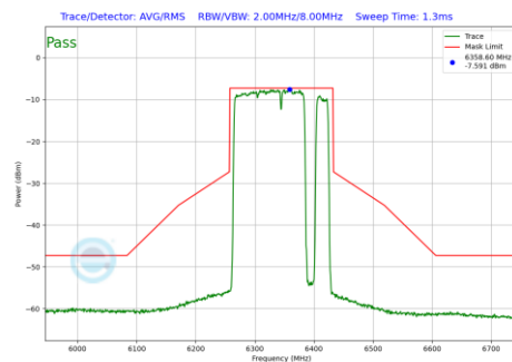
Plot 7-707 In-Band Emission Plot SDM Diversity Antenna 4a (160MHz BW 802.11be(RU) RU996+484+242 Index98 (UNII Band 5) - Ch.79)
