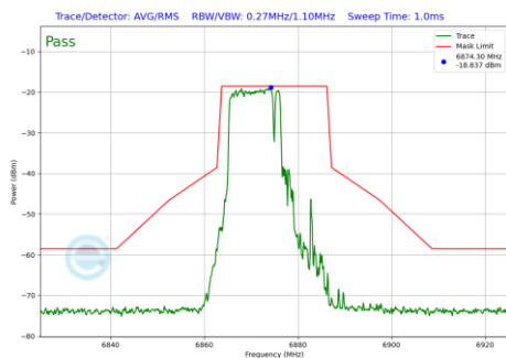
Plot 7-711 In-Band Emission Plot SDM Diversity Antenna 4a (20MHz BW 802.11be(RU) RU106+26 Index82 (UNII Band 7) - Ch.185)
