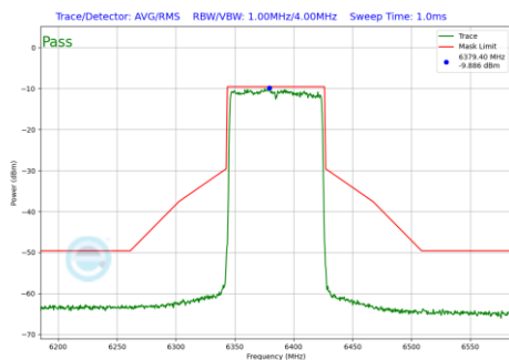
Plot 7-647 In-Band Emission Plot SDM Primary Antenna 4a (80MHz BW 802.11be(RU) RU996 Index67 (UNII Band 5) - Ch.87)
