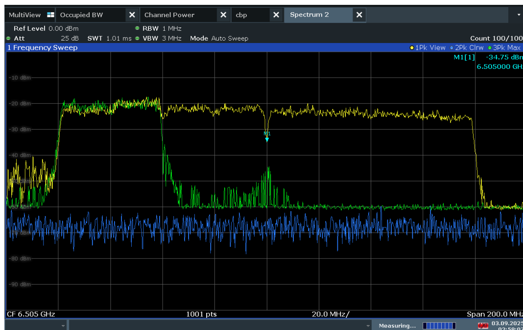
Plot 7-782. 160MHz Bandwidth, AWGN Signal Injected – 6505MHz
