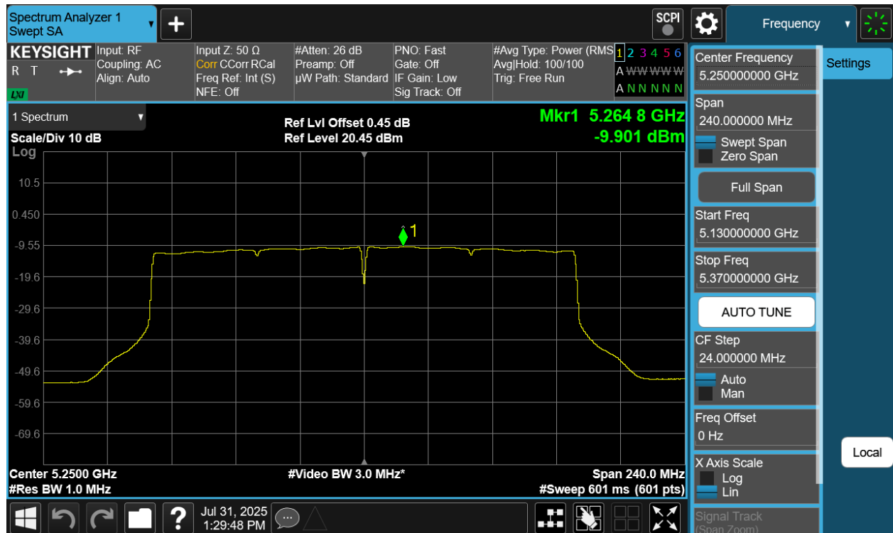
Plot 7-94 PSD CDD Diversity Antenna 4a (160MHz BW 802.11be(SU) - Ch.50)
