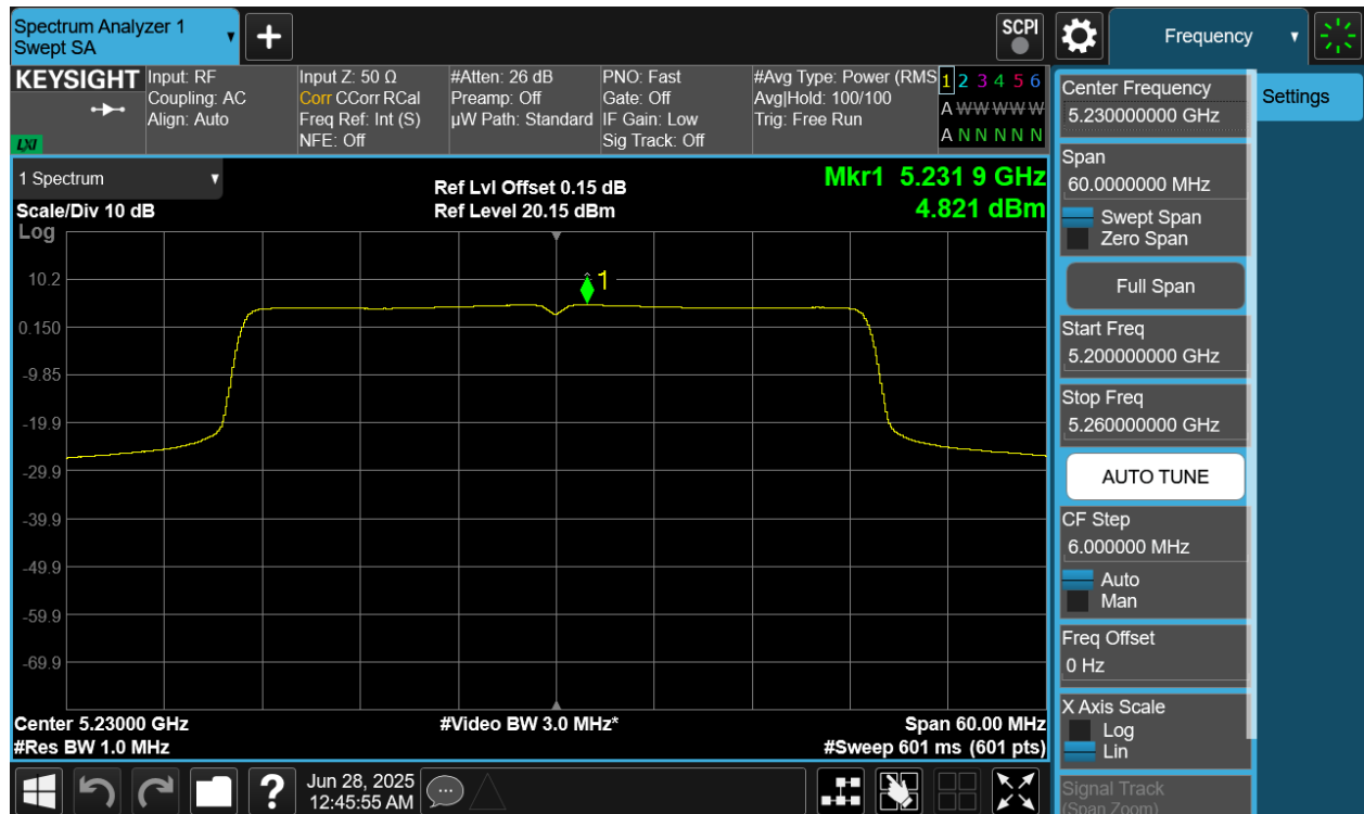
Plot 7-82 PSD CDD Diversity Antenna 2a (40MHz BW 802.11be(SU) - Ch.46)
