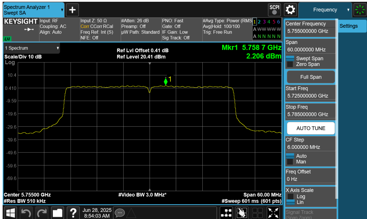
Plot 7-86 PSD CDD Diversity Antenna 4a (40MHz BW 802.11be(SU) - Ch.151)
