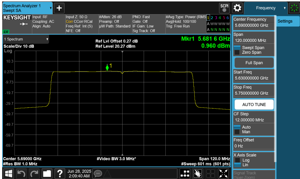
Plot 7-83 PSD CDD Diversity Antenna 2a (80MHz BW 802.11be(SU) - Ch.138)
