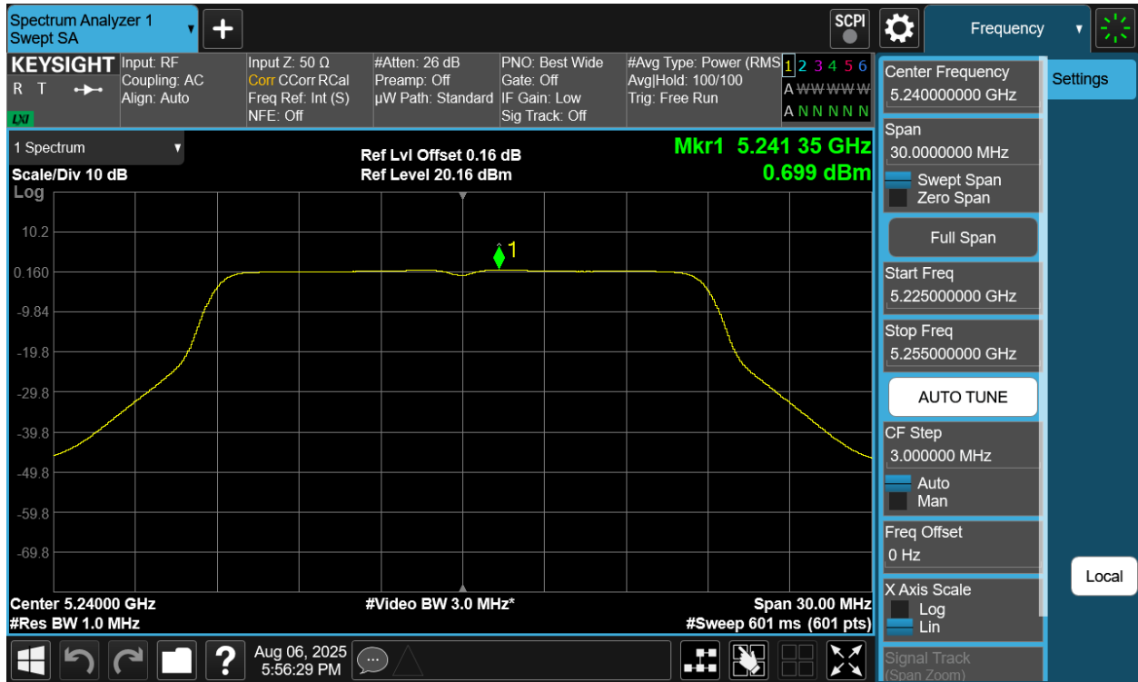
Plot 7-95 PSD CDD Diversity Antenna 2a (20MHz BW 802.11a - Ch.48)
