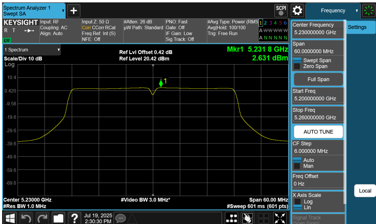
Plot 7-70 PSD CDD Primary Antenna WF5B (40MHz BW 802.11n - Ch.46)
