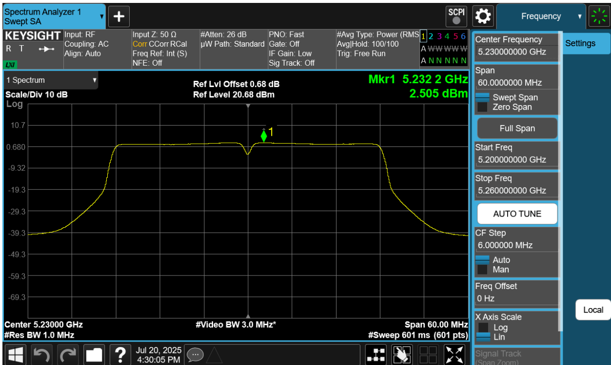
Plot 7-96 PSD CDD Diversity Antenna 2a (40MHz BW 802.11n - Ch.46)
