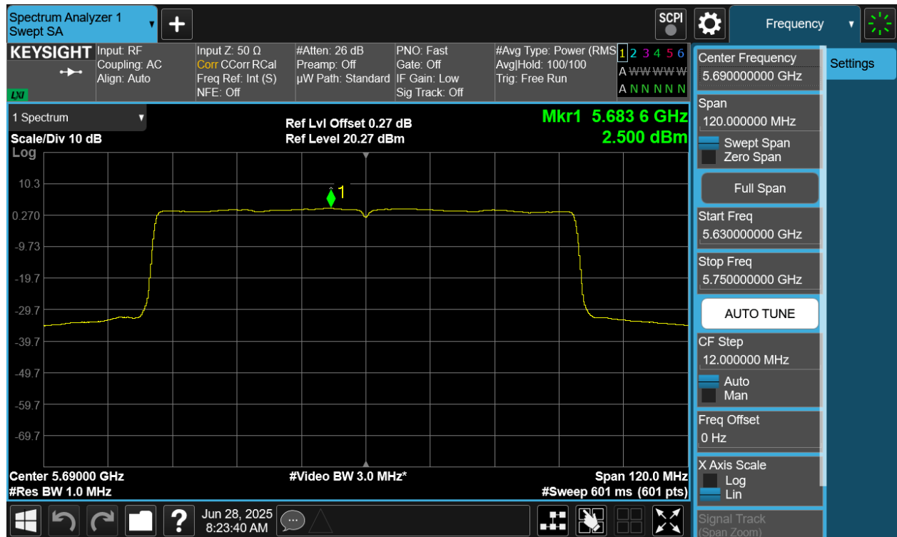
Plot 7-79 PSD CDD Diversity Antenna 4a (80MHz BW 802.11be(SU) - Ch.138)
