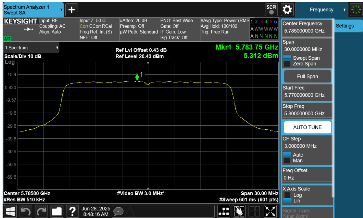
Plot 7-85 PSD CDD Diversity Antenna 4a (20MHz BW 802.11be(SU) - Ch.157)
