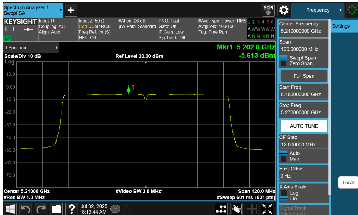
Plot 7-97 PSD CDD Diversity Antenna 2a (80MHz BW 802.11ac - Ch.42)
