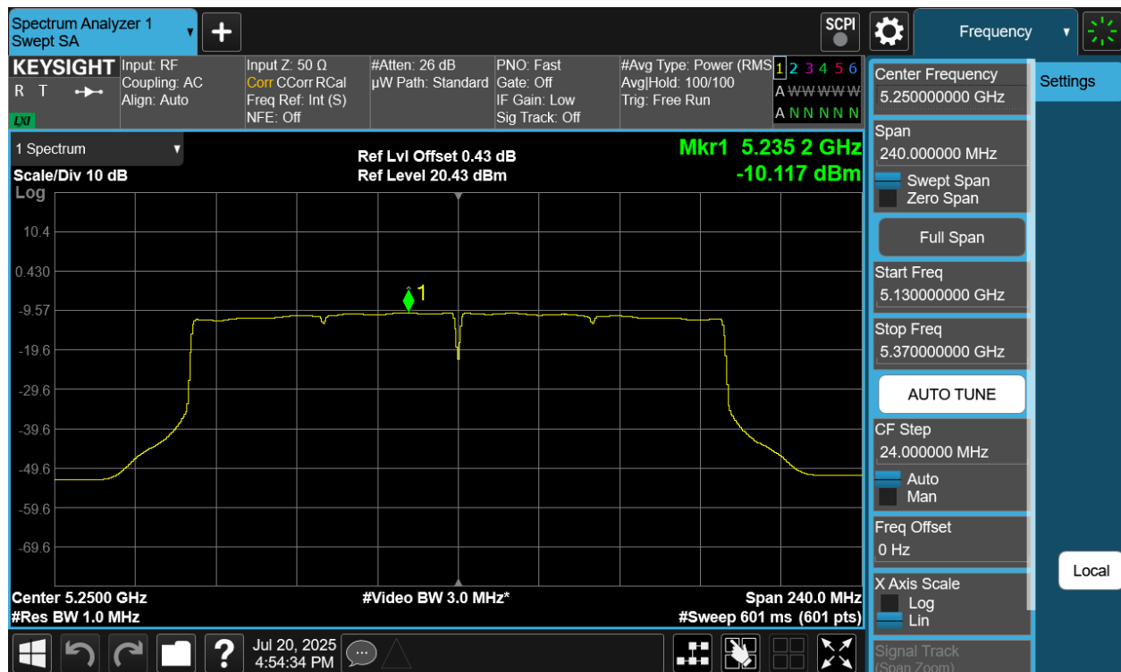
Plot 7-98 PSD CDD Diversity Antenna 2a (160MHz BW 802.11be(SU) - Ch.50)
