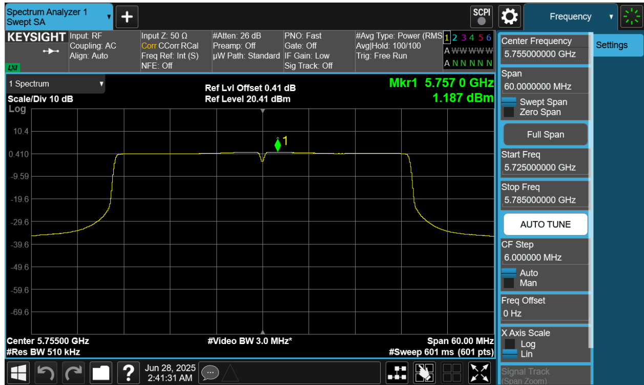
Plot 7-89 PSD CDD Diversity Antenna 2a (40MHz BW 802.11be(SU) - Ch.151)
