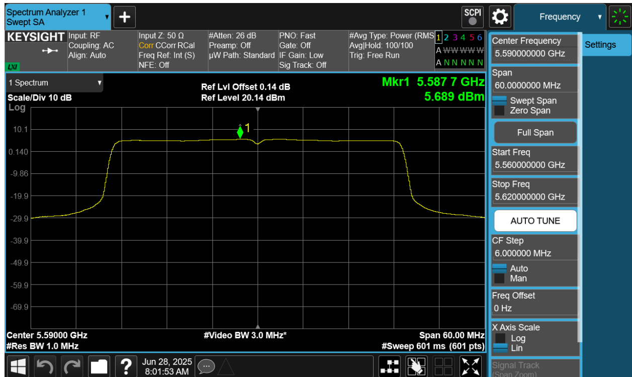
Plot 7-60 PSD CDD Primary Antenna 4a (40MHz BW 802.11be(SU) - Ch.118)
