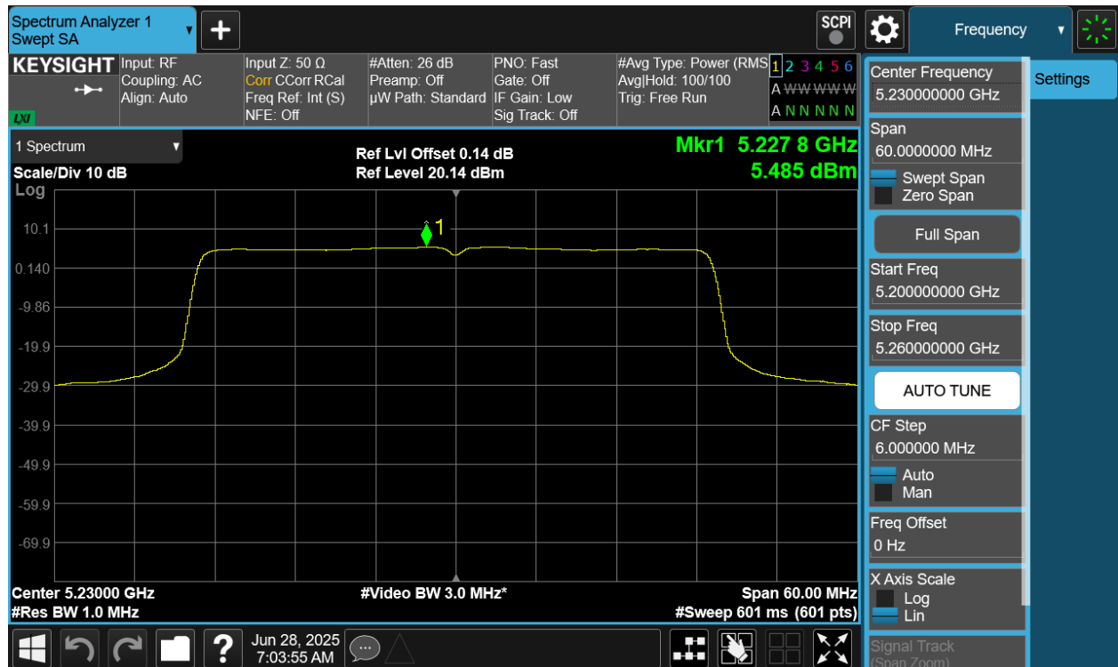
Plot 7-78 PSD CDD Diversity Antenna 4a (40MHz BW 802.11be(SU) - Ch.46)
