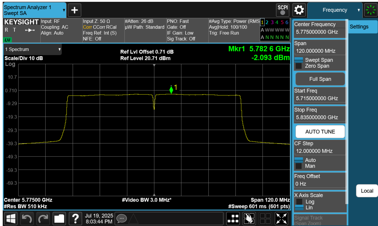
Plot 7-90 PSD CDD Diversity Antenna 2a (80MHz BW 802.11ac - Ch.155)
