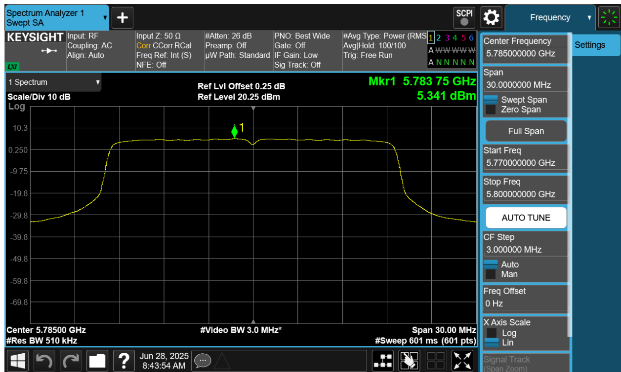
Plot 7-66 PSD CDD Primary Antenna 4a (20MHz BW 802.11be(SU) - Ch.157)
