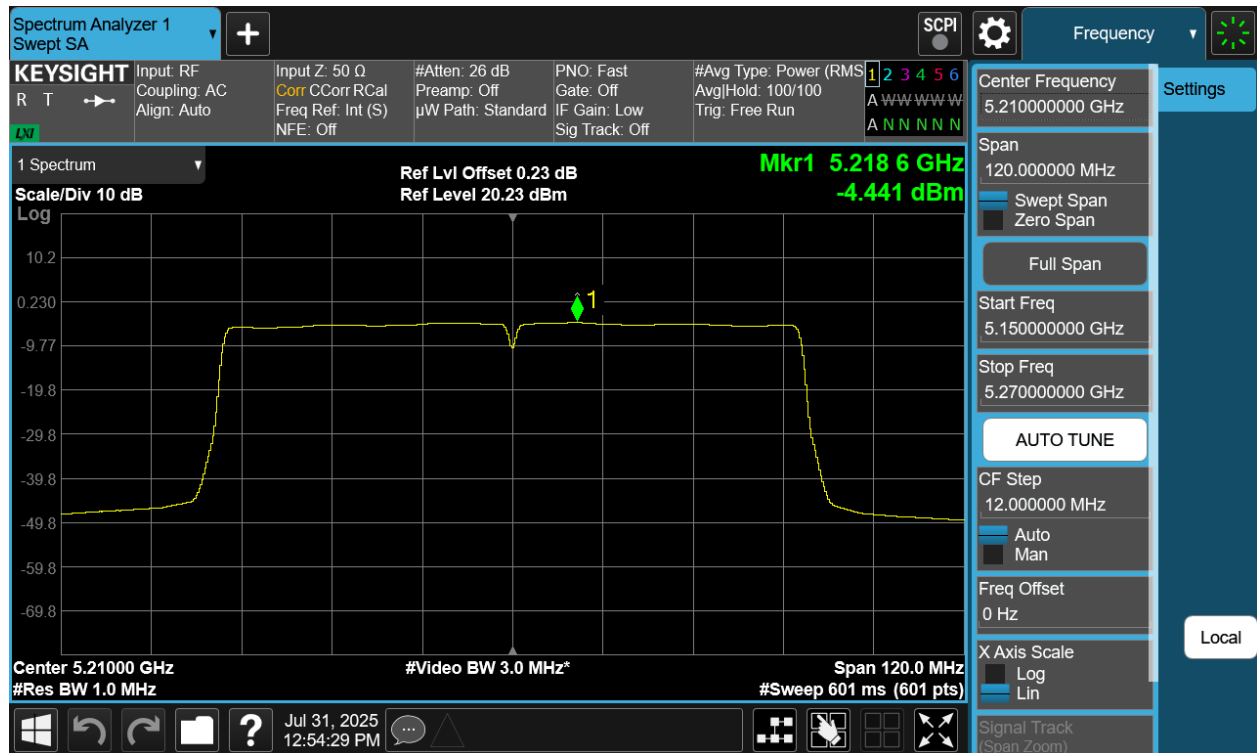
Plot 7-93 PSD CDD Diversity Antenna 4a (80MHz BW 802.11ac - Ch.42)
