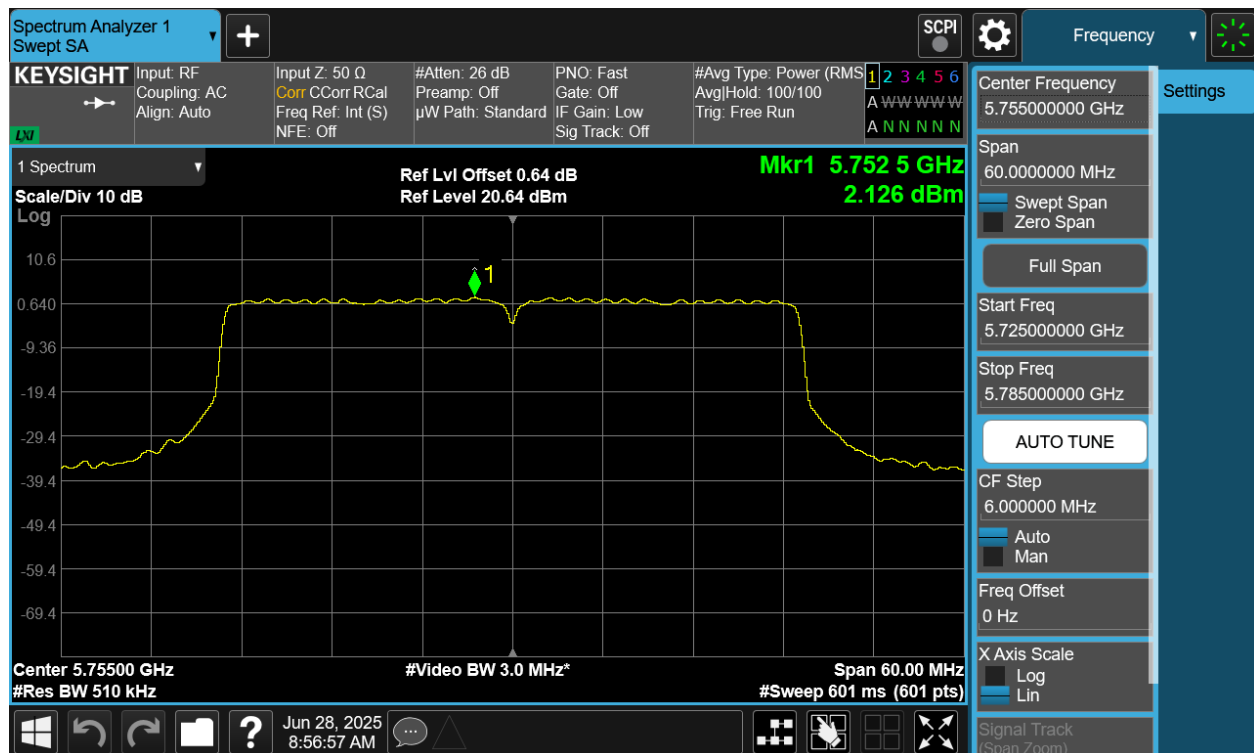
Plot 7-67 PSD CDD Primary Antenna 4a (40MHz BW 802.11be(SU) - Ch.151)
