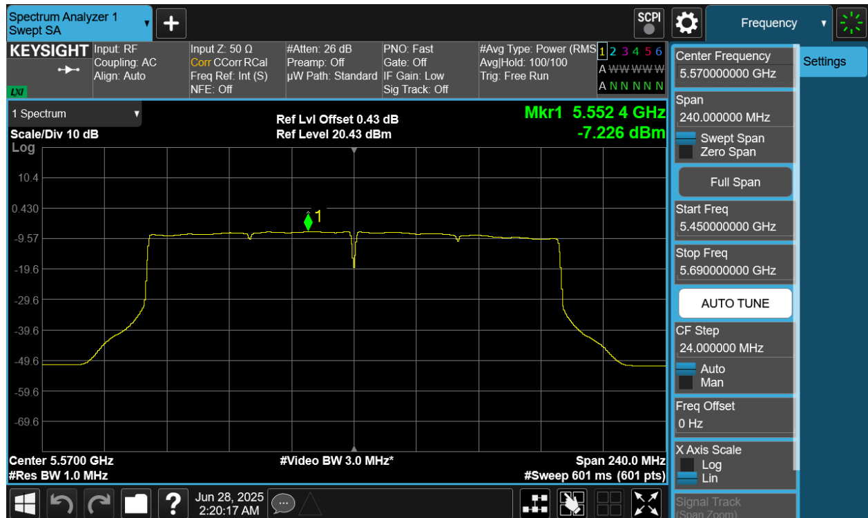
Plot 7-84 PSD CDD Diversity Antenna 2a (160MHz BW 802.11be(SU) - Ch.114)
