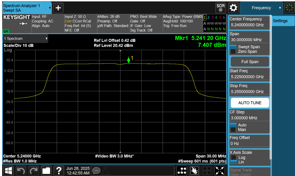
Plot 7-81 PSD CDD Diversity Antenna 2a (20MHz BW 802.11be(SU) - Ch.48)
