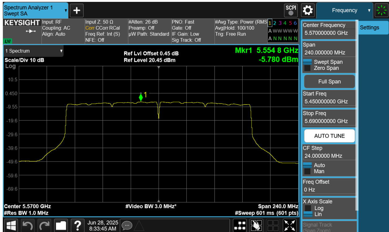
Plot 7-80 PSD CDD Diversity Antenna 4a (160MHz BW 802.11be(SU) - Ch.114)
