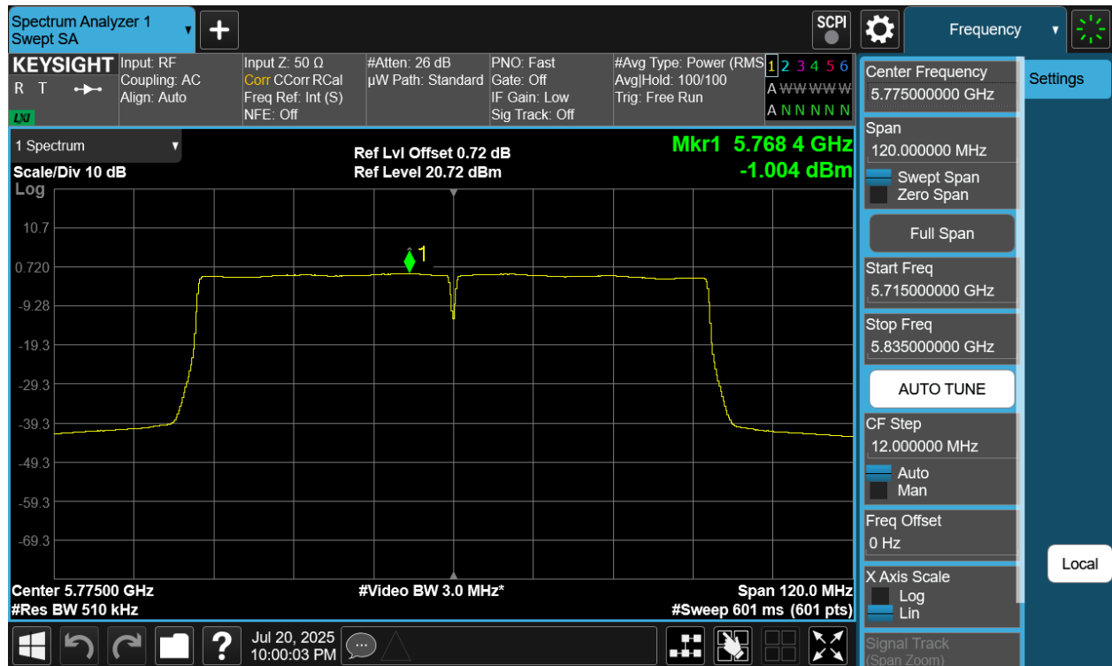
Plot 7-87 PSD CDD Diversity Antenna 4a (80MHz BW 802.11ac - Ch.155)
