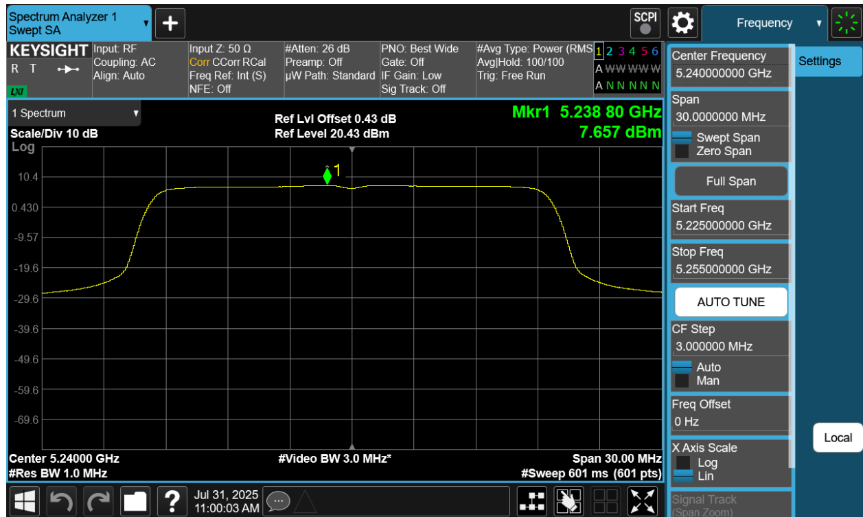
Plot 7-59 PSD CDD Primary Antenna 4a (20MHz BW 802.11be(SU) - Ch.48)
