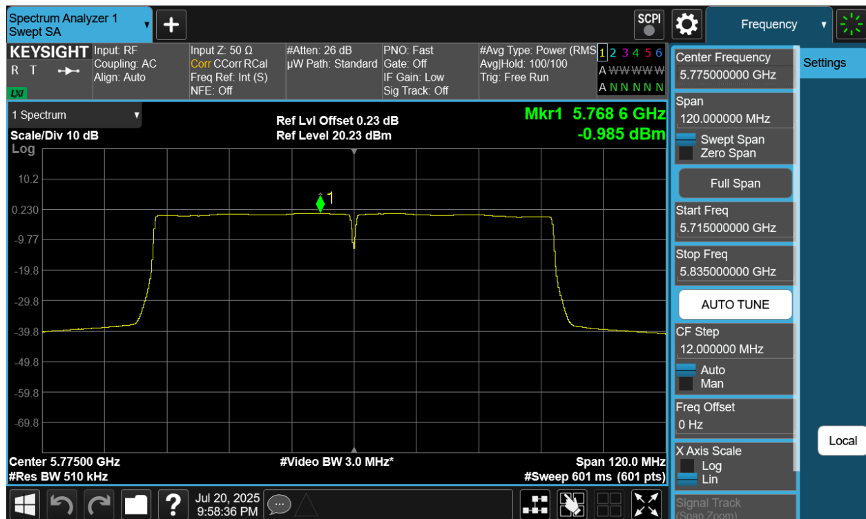
Plot 7-68 PSD CDD Primary Antenna 4a (80MHz BW 802.11ac - Ch.155)
