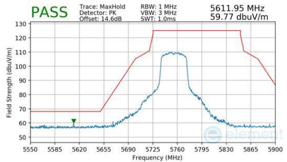
Plot 7-333. Antenna 2a (Peak, Ch.151, 802.11n, MCS7)
