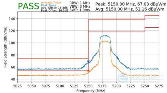
Plot 7-233. Antenna 4a (Peak & Average, Ch.36, 802.11n, MCS7)
