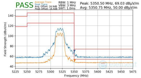
Plot 7-372. CDD Primary (Peak & Average, Ch.64, 802.11n, MCS7)
