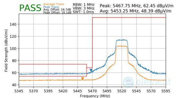
Plot 7-249. Antenna 4a (Peak & Average, Ch.104, 802.11be(SU), MCS11)
