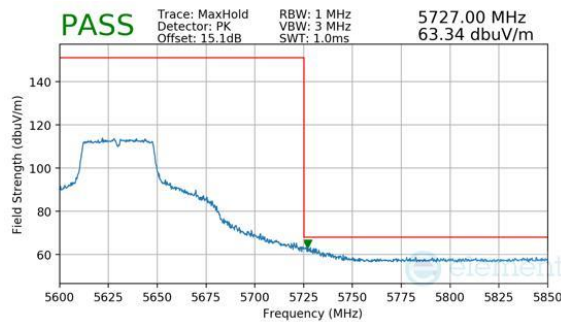
Plot 7-331. Antenna 2a (Peak, Ch.126 (FCC ONLY), 802.11n, MCS7)
