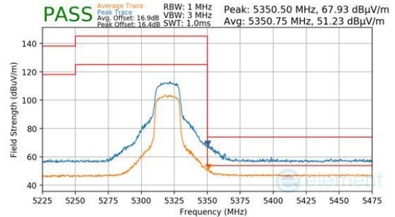
Plot 7-304. Antenna 2a (Peak & Average, Ch.64, 802.11n, MCS7)
