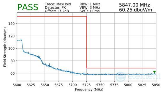
Plot 7-274. Antenna 4a (Peak, Ch.118 (FCC ONLY), 802.11be(SU), MCS11)
