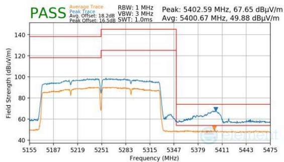
Plot 7-362. Antenna 2a (Peak & Average, Ch.50, 802.11ac, MCS9)
