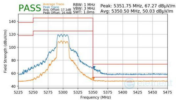
Plot 7-382. CDD Primary (Peak & Average, Ch.60, 802.11be(SU), MCS11)
