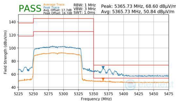
Plot 7-287. Antenna 4a (Peak & Average, Ch.58, 802.11be(SU), MCS11)
