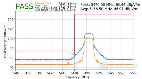
Plot 7-305. Antenna 2a (Peak & Average, Ch.100, 802.11n, MCS7)
