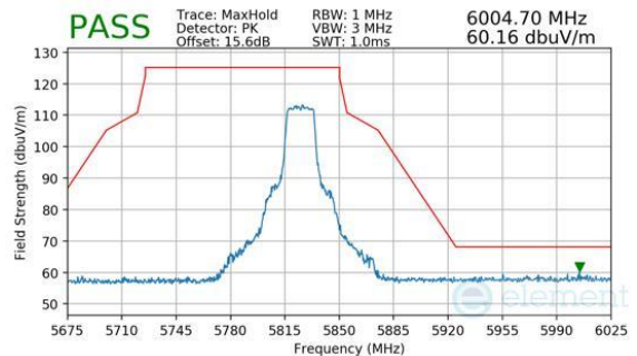
Plot 7-311. Antenna 2a (Peak, Ch.165, 802.11n, MCS7)
