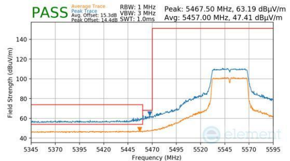
Plot 7-328. Antenna 2a (Peak & Average, Ch.110, 802.11n, MCS7)
