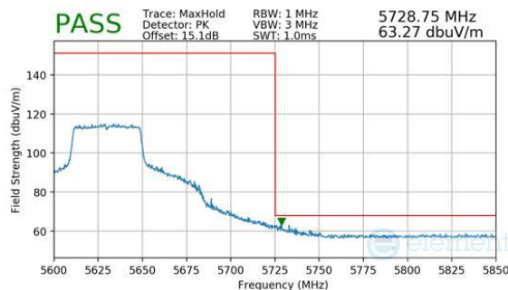
Plot 7-343. Antenna 2a (Peak, Ch.126 (FCC ONLY), 802.11be(SU), MCS11)
