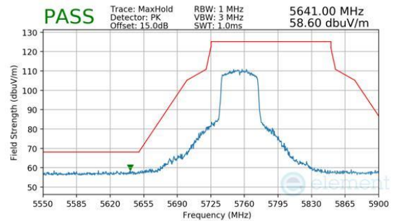
Plot 7-345. Antenna 2a (Peak, Ch.151, 802.11be(SU), MCS11)
