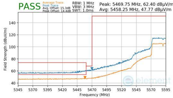
Plot 7-329. Antenna 2a (Peak & Average, Ch.118 (FCC ONLY), 802.11n, MCS7)
