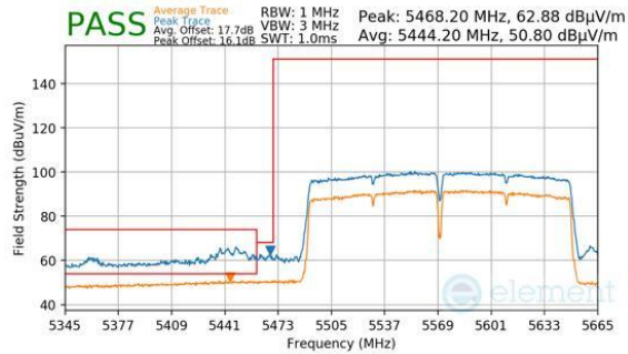
Plot 7-295. Antenna 4a (Peak & Average, Ch.114 (FCC ONLY), 802.11ac, MCS9)
