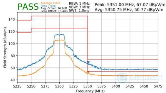
Plot 7-303. Antenna 2a (Peak & Average, Ch.60, 802.11n, MCS7)
