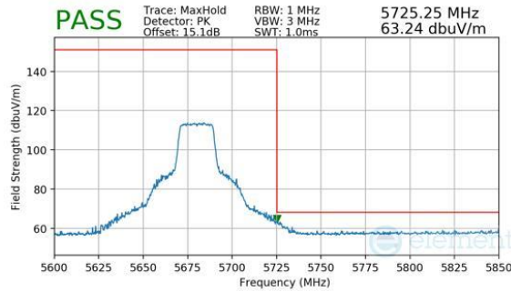
Plot 7-319. Antenna 2a (Peak, Ch.136, 802.11be(SU), MCS11)
