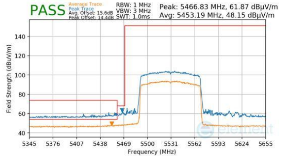
Plot 7-356. Antenna 2a (Peak & Average, Ch.106, 802.11be(SU), MCS11)
