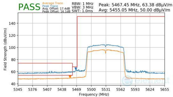
Plot 7-213. Antenna WF5B (Peak & Average, Ch.106, 802.11ac, MCS9)
