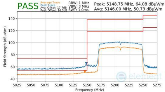
Plot 7-279. Antenna 4a (Peak & Average, Ch.42, 802.11ac, MCS9)
