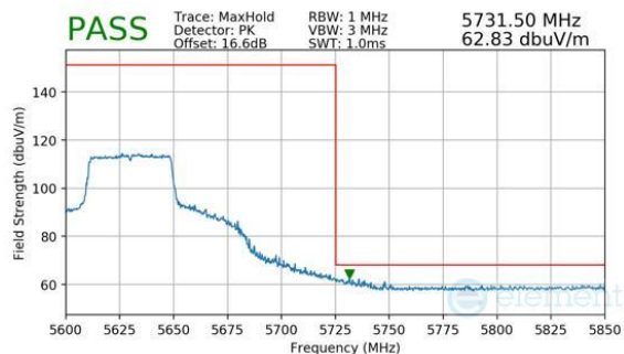
Plot 7-275. Antenna 4a (Peak, Ch.126 (FCC ONLY), 802.11be(SU), MCS11)
