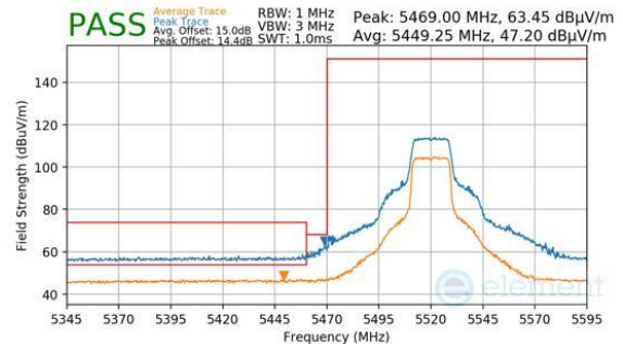
Plot 7-306. Antenna 2a (Peak & Average, Ch.104, 802.11n, MCS7)
