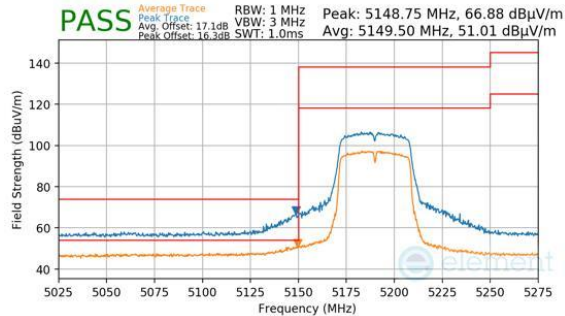
Plot 7-323. Antenna 2a (Peak & Average, Ch.38, 802.11n, MCS7)
