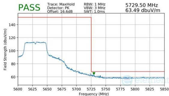
Plot 7-263. Antenna 4a (Peak, Ch.126 (FCC ONLY), 802.11n, MCS7)
