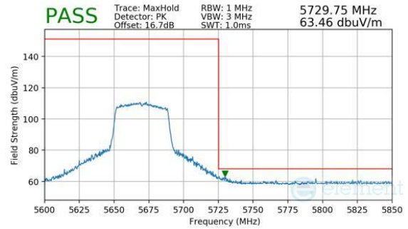
Plot 7-344. Antenna 2a (Peak, Ch.134, 802.11be(SU), MCS11)
