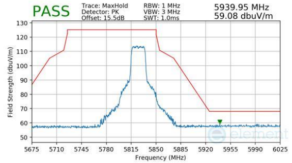
Plot 7-322. Antenna 2a (Peak, Ch.165, 802.11be(SU), MCS11)
