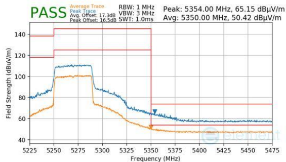
Plot 7-337. Antenna 2a (Peak & Average, Ch.54, 802.11be(SU), MCS11)
