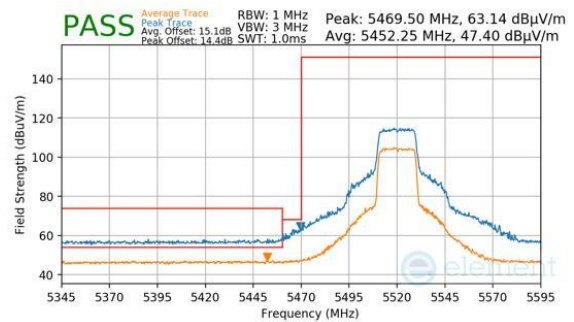
Plot 7-317. Antenna 2a (Peak & Average, Ch.104, 802.11be(SU), MCS11)
