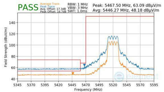
Plot 7-385. CDD Primary (Peak & Average, Ch.104, 802.11be(SU), MCS11)
