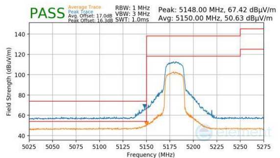
Plot 7-312. Antenna 2a (Peak & Average, Ch.36, 802.11be(SU), MCS11)
