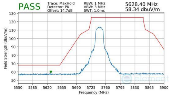
Plot 7-310. Antenna 2a (Peak, Ch.149, 802.11n, MCS7)
