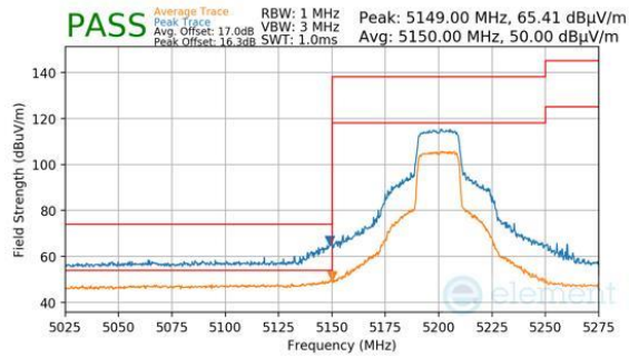
Plot 7-313. Antenna 2a (Peak & Average, Ch.40, 802.11be(SU), MCS11)
