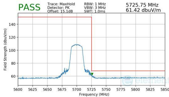
Plot 7-320. Antenna 2a (Peak, Ch.140, 802.11be(SU), MCS11)
