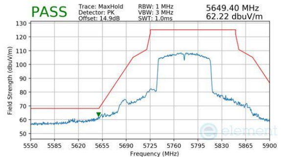
Plot 7-284. Antenna 4a (Peak, Ch.155, 802.11ac, MCS9)
