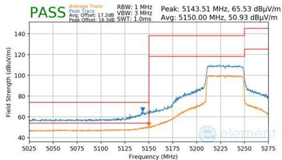
Plot 7-268. Antenna 4a (Peak & Average, Ch.46, 802.11be(SU), MCS11)
