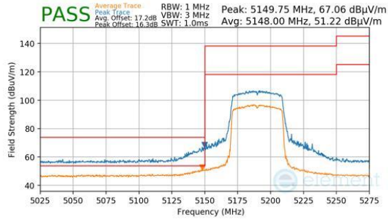
Plot 7-335. Antenna 2a (Peak & Average, Ch.38, 802.11be(SU), MCS11)
