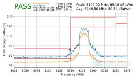
Plot 7-380. CDD Primary (Peak & Average, Ch.36, 802.11be(SU), MCS11)
