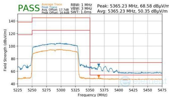
Plot 7-355. Antenna 2a (Peak & Average, Ch.58, 802.11be(SU), MCS11)
