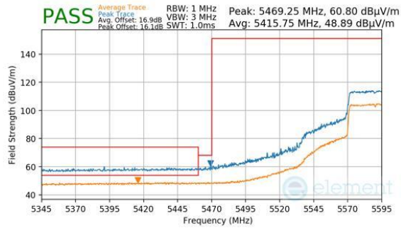
Plot 7-273. Antenna 4a (Peak & Average, Ch.118 (FCC ONLY), 802.11be(SU), MCS11)
