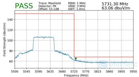
Plot 7-351. Antenna 2a (Peak, Ch.122 (FCC ONLY), 802.11ac, MCS9)
