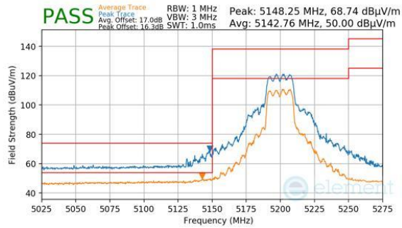
Plot 7-381. CDD Primary (Peak & Average, Ch.40, 802.11be(SU), MCS11)
