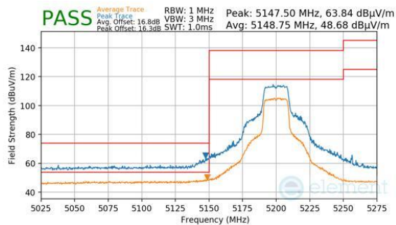
Plot 7-302. Antenna 2a (Peak & Average, Ch.40, 802.11n, MCS7)
