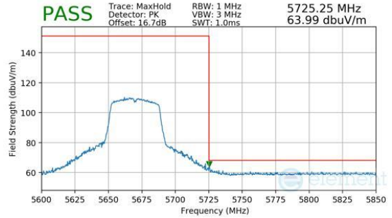
Plot 7-332. Antenna 2a (Peak, Ch.134, 802.11n, MCS7)
