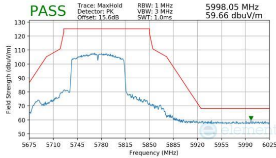
Plot 7-285. Antenna 4a (Peak, Ch.155, 802.11ac, MCS9)
