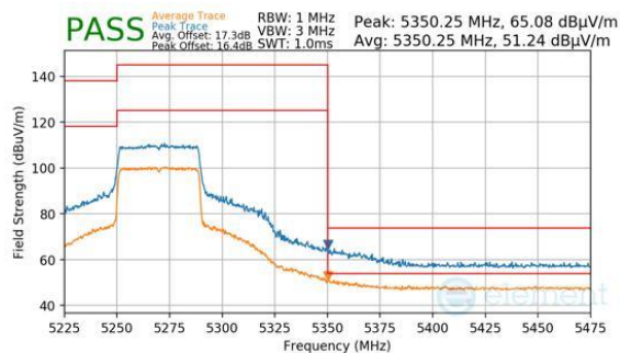
Plot 7-269. Antenna 4a (Peak & Average, Ch.54, 802.11be(SU), MCS11)
