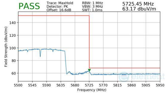
Plot 7-296. Antenna 4a (Peak, Ch.114 (FCC ONLY), 802.11ac, MCS9)
