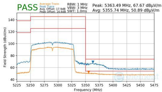
Plot 7-280. Antenna 4a (Peak & Average, Ch.58, 802.11ac, MCS9)
