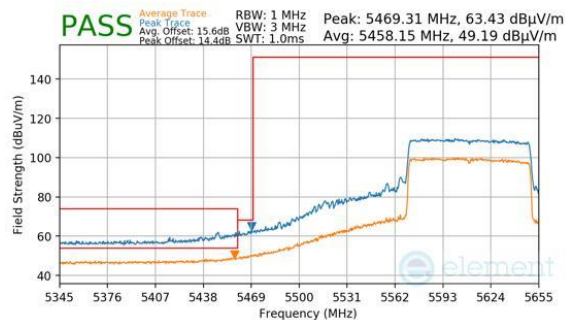
Plot 7-357. Antenna 2a (Peak & Average, Ch.122 (FCC ONLY), 802.11be(SU), MCS11)
