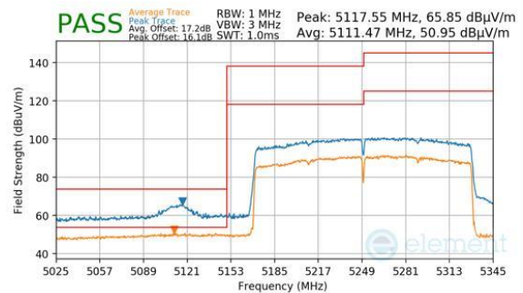
Plot 7-365. Antenna 2a (Peak & Average, Ch.50, 802.11be(SU), MCS11)
