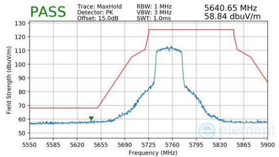
Plot 7-277. Antenna 4a (Peak, Ch.151, 802.11be(SU), MCS11)
