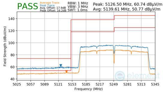
Plot 7-293. Antenna 4a (Peak & Average, Ch.50, 802.11ac, MCS9)
