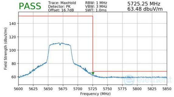
Plot 7-264. Antenna 4a (Peak, Ch.134, 802.11n, MCS7)
