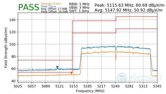
Plot 7-297. Antenna 4a (Peak & Average, Ch.50, 802.11be(SU), MCS11)
