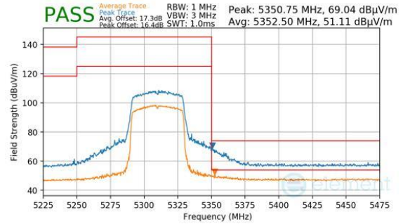
Plot 7-338. Antenna 2a (Peak & Average, Ch.62, 802.11be(SU), MCS11)
