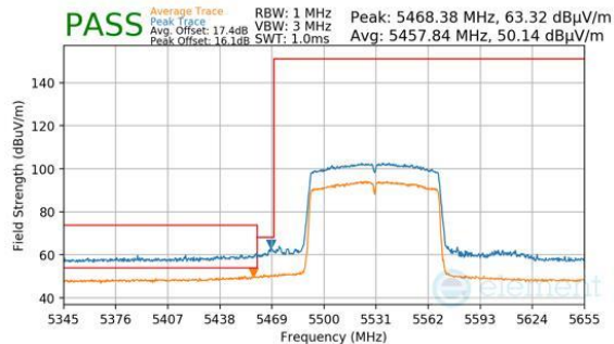
Plot 7-281. Antenna 4a (Peak & Average, Ch.106, 802.11ac, MCS9)
