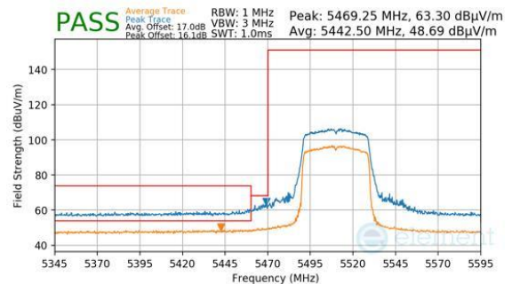
Plot 7-271. Antenna 4a (Peak & Average, Ch.102, 802.11be(SU), MCS11)
