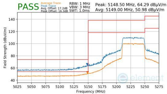
Plot 7-336. Antenna 2a (Peak & Average, Ch.46, 802.11be(SU), MCS11)
