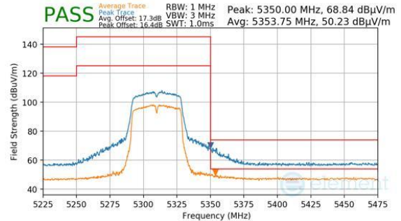
Plot 7-326. Antenna 2a (Peak & Average, Ch.62, 802.11n, MCS7)
