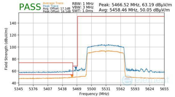
Plot 7-288. Antenna 4a (Peak & Average, Ch.106, 802.11be(SU), MCS11)
