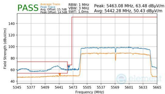
Plot 7-367. Antenna 2a (Peak & Average, Ch.114 (FCC ONLY), 802.11be(SU), MCS11)
