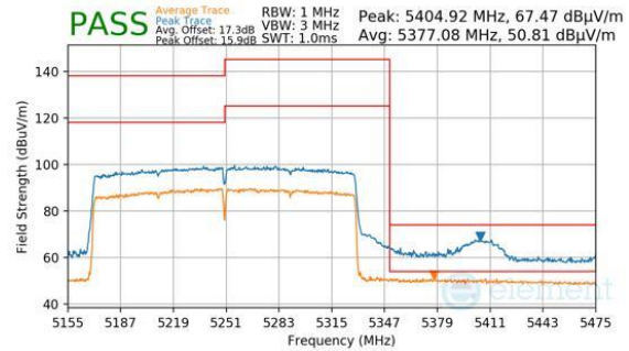
Plot 7-298. Antenna 4a (Peak & Average, Ch.50, 802.11be(SU), MCS11)
