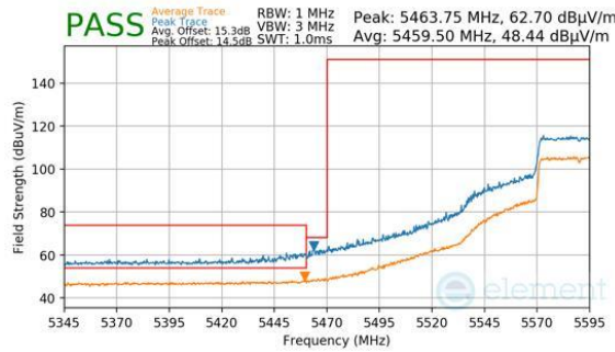
Plot 7-341. Antenna 2a (Peak & Average, Ch.118 (FCC ONLY), 802.11be(SU), MCS11)
