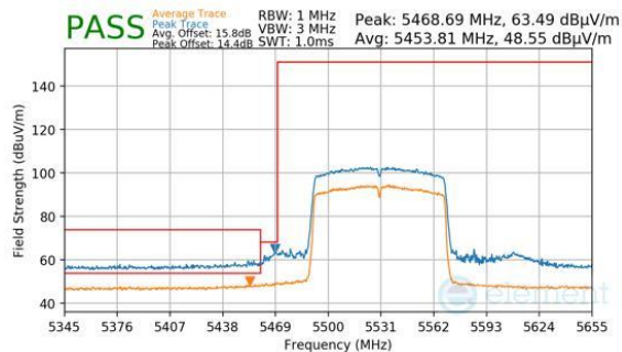
Plot 7-349. Antenna 2a (Peak & Average, Ch.106, 802.11ac, MCS9)
