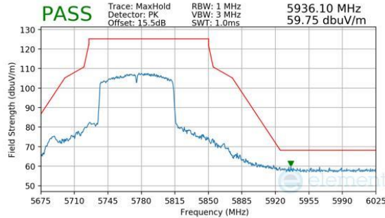
Plot 7-353. Antenna 2a (Peak, Ch.155, 802.11ac, MCS9)
