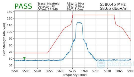
Plot 7-321. Antenna 2a (Peak, Ch.149, 802.11be(SU), MCS11)
