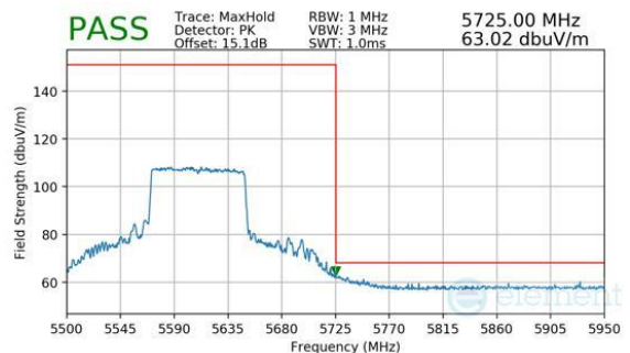
Plot 7-358. Antenna 2a (Peak, Ch.122 (FCC ONLY), 802.11be(SU), MCS11)
