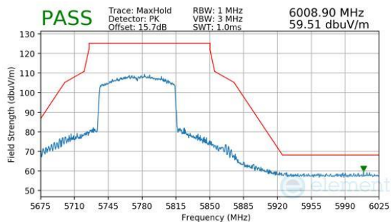
Plot 7-360. Antenna 2a (Peak, Ch.155, 802.11be(SU), MCS11)
