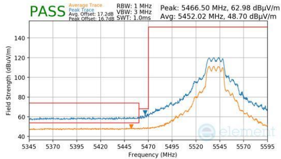
Plot 7-375. CDD Primary (Peak & Average, Ch.108, 802.11n, MCS7)
