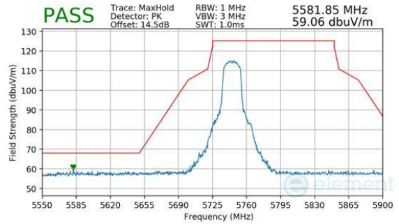
Plot 7-242. Antenna 4a (Peak, Ch.149, 802.11n, MCS7)
