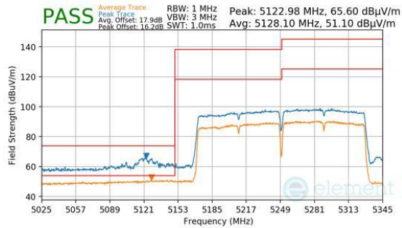
Plot 7-361. Antenna 2a (Peak & Average, Ch.50, 802.11ac, MCS9)
