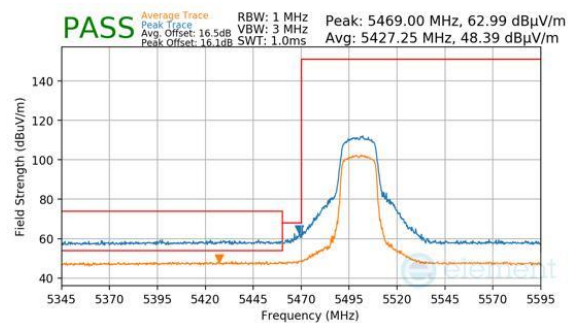
Plot 7-237. Antenna 4a (Peak & Average, Ch.100, 802.11n, MCS7)
