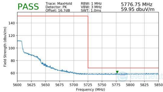
Plot 7-262. Antenna 4a (Peak, Ch.118 (FCC ONLY), 802.11n, MCS7)
