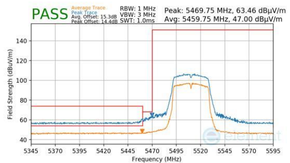
Plot 7-327. Antenna 2a (Peak & Average, Ch.102, 802.11n, MCS7)
