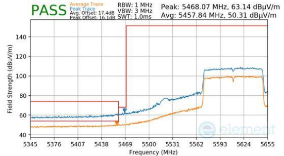
Plot 7-282. Antenna 4a (Peak & Average, Ch.122 (FCC ONLY), 802.11ac, MCS9)
