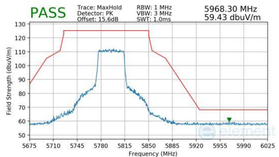
Plot 7-278. Antenna 4a (Peak, Ch.159, 802.11be(SU), MCS11)
