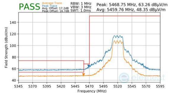
Plot 7-374. CDD Primary (Peak & Average, Ch.104, 802.11n, MCS7)
