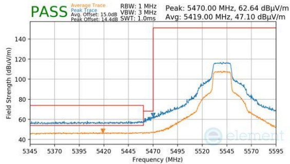
Plot 7-307. Antenna 2a (Peak & Average, Ch.108, 802.11n, MCS7)
