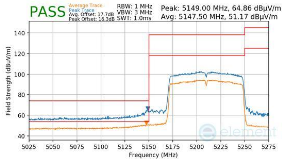
Plot 7-347. Antenna 2a (Peak & Average, Ch.42, 802.11ac, MCS9)
