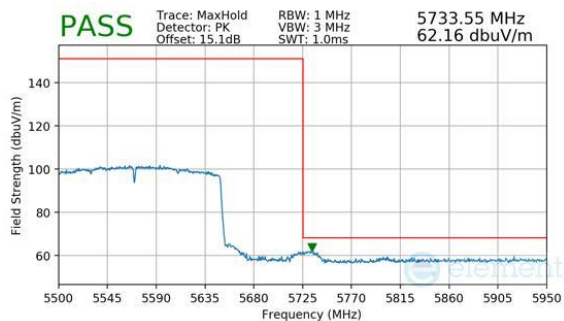
Plot 7-368. Antenna 2a (Peak, Ch.114 (FCC ONLY), 802.11be(SU), MCS11)
