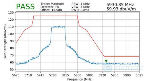
Plot 7-346. Antenna 2a (Peak, Ch.159, 802.11be(SU), MCS11)
