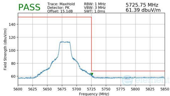
Plot 7-308. Antenna 2a (Peak, Ch.136, 802.11n, MCS7)
