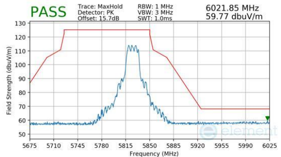
Plot 7-379. CDD Primary (Peak, Ch.165, 802.11n, MCS7)
