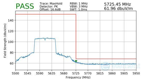
Plot 7-283. Antenna 4a (Peak, Ch.122 (FCC ONLY), 802.11ac, MCS9)
