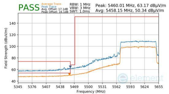
Plot 7-289. Antenna 4a (Peak & Average, Ch.122 (FCC ONLY), 802.11be(SU), MCS11)
