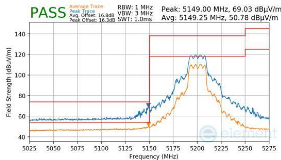
Plot 7-370. CDD Primary (Peak & Average, Ch.40, 802.11n, MCS7)
