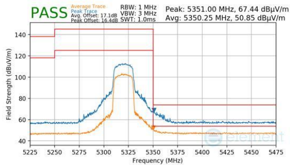
Plot 7-315. Antenna 2a (Peak & Average, Ch.64, 802.11be(SU), MCS11)
