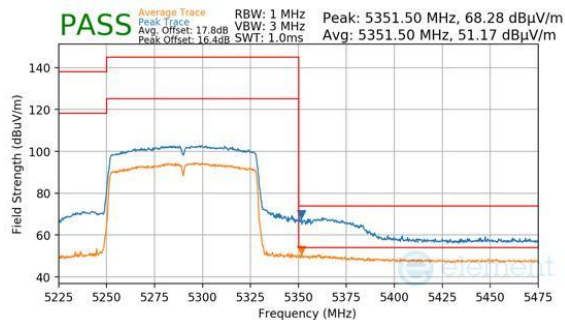
Plot 7-348. Antenna 2a (Peak & Average, Ch.58, 802.11ac, MCS9)
