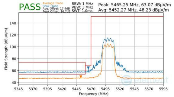
Plot 7-384. CDD Primary (Peak & Average, Ch.100, 802.11be(SU), MCS11)
