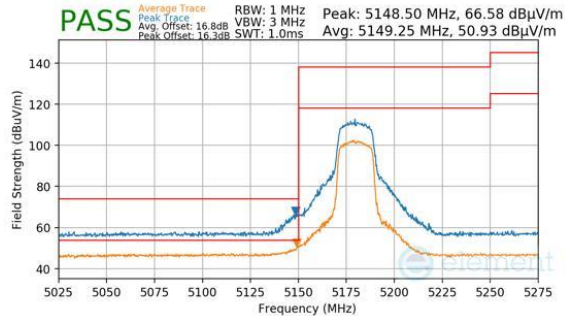
Plot 7-301. Antenna 2a (Peak & Average, Ch.36, 802.11n, MCS7)
