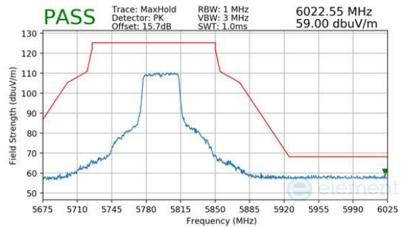
Plot 7-334. Antenna 2a (Peak, Ch.159, 802.11n, MCS7)
