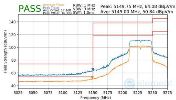
Plot 7-324. Antenna 2a (Peak & Average, Ch.46, 802.11n, MCS7)
