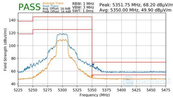
Plot 7-371. CDD Primary (Peak & Average, Ch.60, 802.11n, MCS7)
