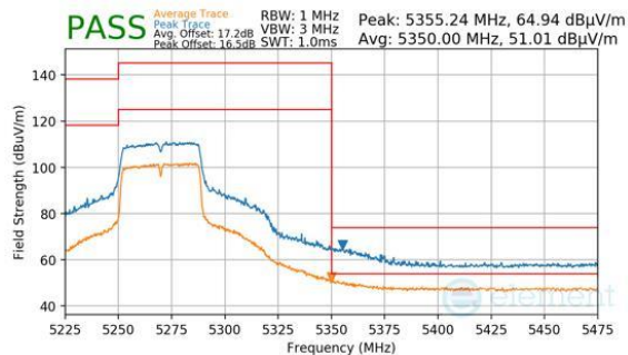
Plot 7-325. Antenna 2a (Peak & Average, Ch.54, 802.11n, MCS7)
