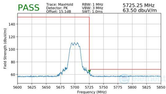
Plot 7-377. CDD Primary (Peak, Ch.140, 802.11n, MCS7)
