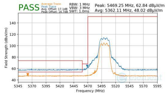
Plot 7-373. CDD Primary (Peak & Average, Ch.100, 802.11n, MCS7)
