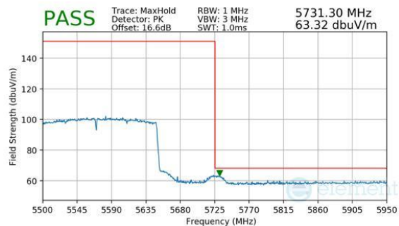
Plot 7-300. Antenna 4a (Peak, Ch.114 (FCC ONLY), 802.11be(SU), MCS11)
