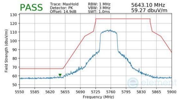
Plot 7-209. Antenna WF5B (Peak, Ch.151, 802.11be(SU), MCS11)
