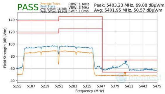
Plot 7-294. Antenna 4a (Peak & Average, Ch.50, 802.11ac, MCS9)
