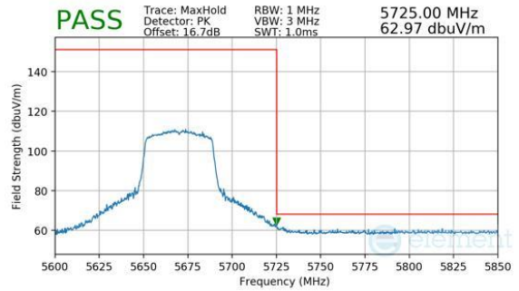
Plot 7-276. Antenna 4a (Peak, Ch.134, 802.11be(SU), MCS11)
