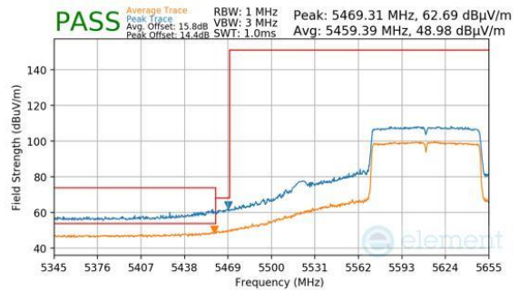
Plot 7-350. Antenna 2a (Peak & Average, Ch.122 (FCC ONLY), 802.11ac, MCS9)
