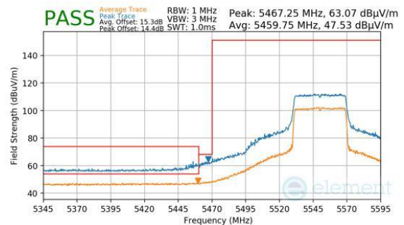
Plot 7-340. Antenna 2a (Peak & Average, Ch.110, 802.11be(SU), MCS11)
