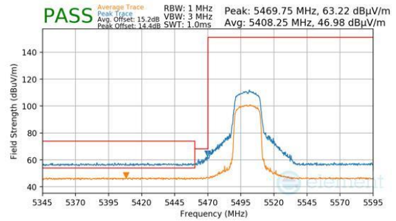
Plot 7-316. Antenna 2a (Peak & Average, Ch.100, 802.11be(SU), MCS11)
