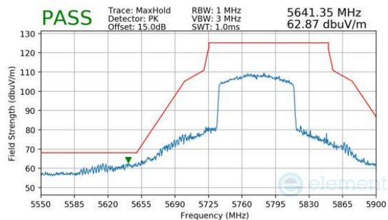
Plot 7-359. Antenna 2a (Peak, Ch.155, 802.11be(SU), MCS11)
