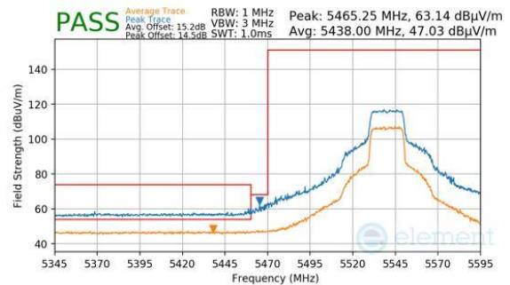
Plot 7-318. Antenna 2a (Peak & Average, Ch.108, 802.11be(SU), MCS11)
