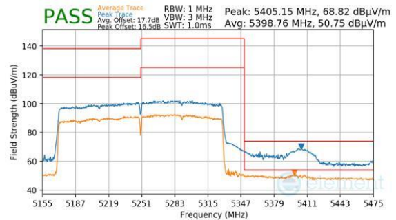
Plot 7-366. Antenna 2a (Peak & Average, Ch.50, 802.11be(SU), MCS11)
