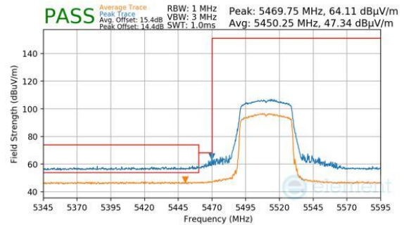
Plot 7-339. Antenna 2a (Peak & Average, Ch.102, 802.11be(SU), MCS11)
