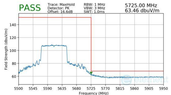
Plot 7-290. Antenna 4a (Peak, Ch.122 (FCC ONLY), 802.11be(SU), MCS11)
