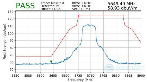
Plot 7-265. Antenna 4a (Peak, Ch.151, 802.11n, MCS7)
