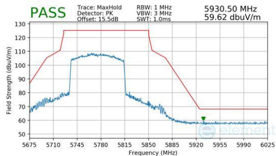
Plot 7-292. Antenna 4a (Peak, Ch.155, 802.11be(SU), MCS11)
