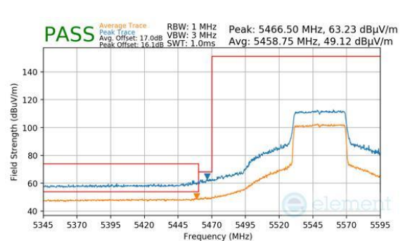
Plot 7-272. Antenna 4a (Peak & Average, Ch.110, 802.11be(SU), MCS11)
