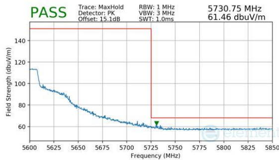
Plot 7-330. Antenna 2a (Peak, Ch.118 (FCC ONLY), 802.11n, MCS7)
