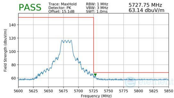
Plot 7-376. CDD Primary (Peak, Ch.136, 802.11n, MCS7)
