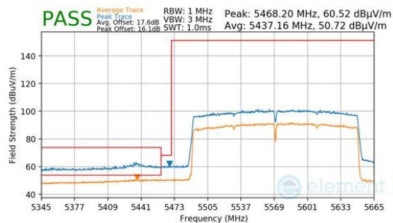
Plot 7-299. Antenna 4a (Peak & Average, Ch.114 (FCC ONLY), 802.11be(SU), MCS11)
