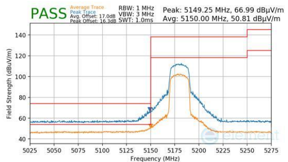
Plot 7-244. Antenna 4a (Peak & Average, Ch.36, 802.11be(SU), MCS11)
