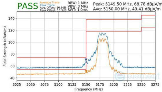
Plot 7-369. CDD Primary (Peak & Average, Ch.36, 802.11n, MCS7)
