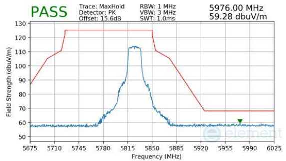
Plot 7-243. Antenna 4a (Peak, Ch.165, 802.11n, MCS7)
