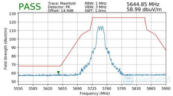
Plot 7-378. CDD Primary (Peak, Ch.149, 802.11n, MCS7)
