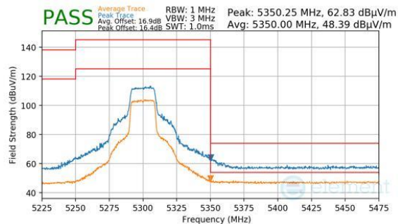
Plot 7-235. Antenna 4a (Peak & Average, Ch.60, 802.11n, MCS7)
