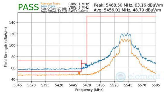
Plot 7-386. CDD Primary (Peak & Average, Ch.108, 802.11be(SU), MCS11)
