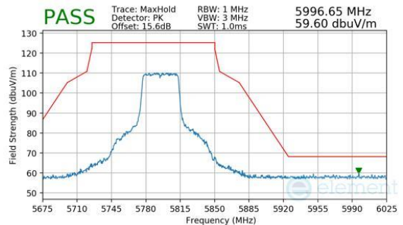
Plot 7-266. Antenna 4a (Peak, Ch.159, 802.11n, MCS7)
