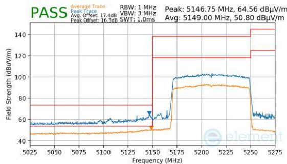
Plot 7-354. Antenna 2a (Peak & Average, Ch.42, 802.11be(SU), MCS11)
