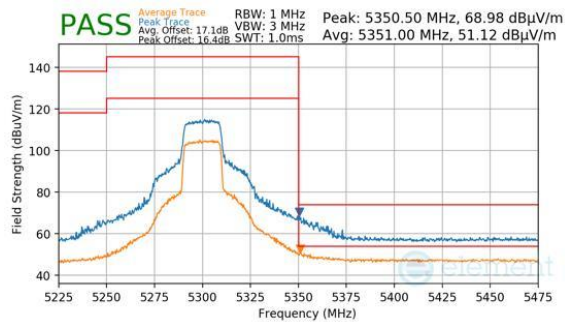
Plot 7-314. Antenna 2a (Peak & Average, Ch.60, 802.11be(SU), MCS11)
