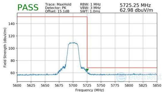
Plot 7-309. Antenna 2a (Peak, Ch.140, 802.11n, MCS7)
