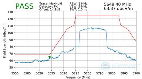
Plot 7-352. Antenna 2a (Peak, Ch.155, 802.11ac, MCS9)
