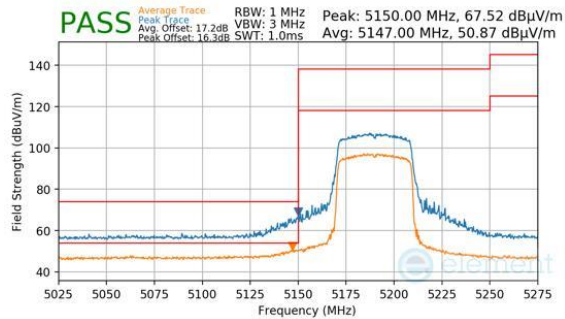
Plot 7-267. Antenna 4a (Peak & Average, Ch.38, 802.11be(SU), MCS11)
