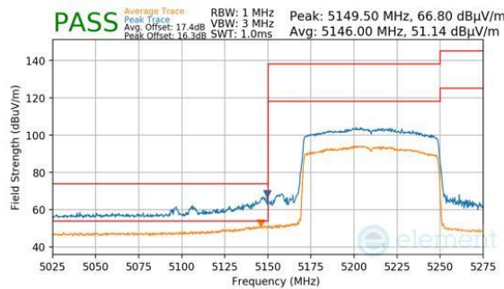
Plot 7-286. Antenna 4a (Peak & Average, Ch.42, 802.11be(SU), MCS11)
