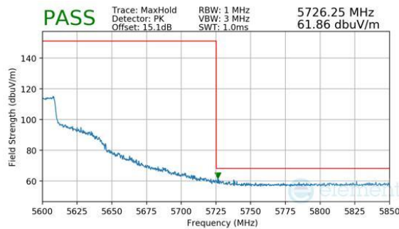
Plot 7-342. Antenna 2a (Peak, Ch.118 (FCC ONLY), 802.11be(SU), MCS11)
