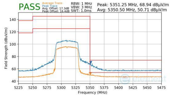
Plot 7-270. Antenna 4a (Peak & Average, Ch.62, 802.11be(SU), MCS11)
