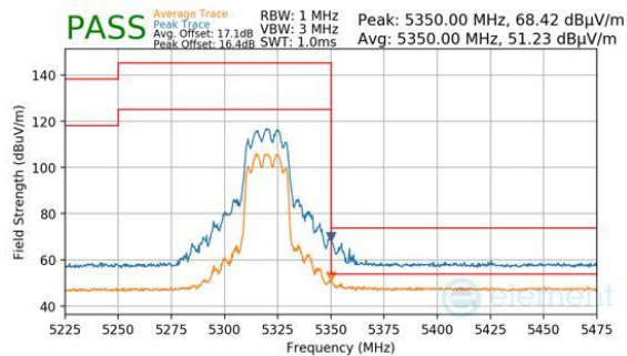
Plot 7-383. CDD Primary (Peak & Average, Ch.64, 802.11be(SU), MCS11)
