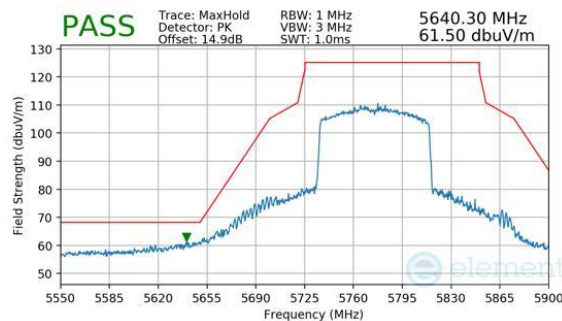
Plot 7-291. Antenna 4a (Peak, Ch.155, 802.11be(SU), MCS11)
