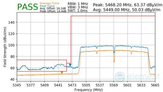
Plot 7-363. Antenna 2a (Peak & Average, Ch.114 (FCC ONLY), 802.11ac, MCS9)
