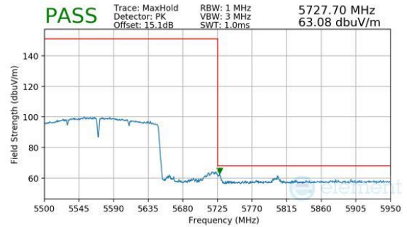
Plot 7-364. Antenna 2a (Peak, Ch.114 (FCC ONLY), 802.11ac, MCS9)
