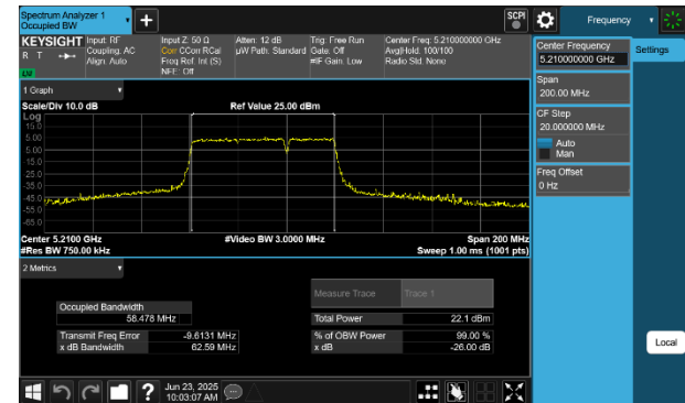
Plot 7-6 26dB BW & 99% OBW Antenna WF5B (80MHz BW 802.11be(RU) RU484+242 Index93 - Ch.42)
