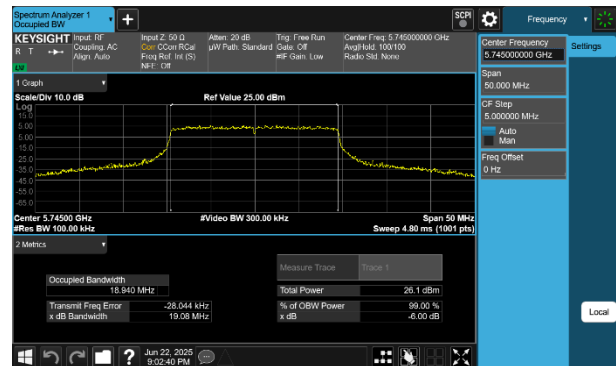
Plot 7-39 6dB BW & 99% OBW Antenna WF5B (20MHz BW 802.11be(RU) RU242 Index61 - Ch.149)
