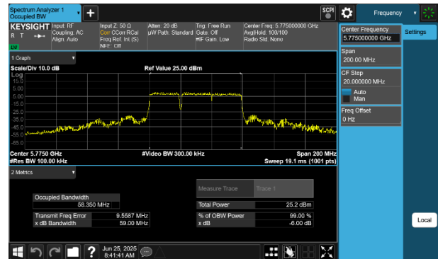
Plot 7-46 6dB BW & 99% OBW Antenna 4a (80MHz BW 802.11be(RU) RU484+242 Index90 - Ch.155)
