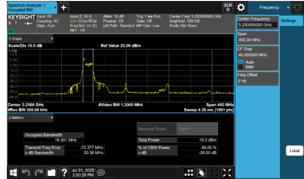
Plot 7-26 26dB BW & 99% OBW Antenna 2a (160MHz BW 802.11be(RU) RU52 Index37 - Ch.50)
