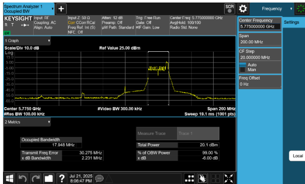
Plot 7-44 6dB BW & 99% OBW Antenna 4a (80MHz BW 802.11be(RU) RU26 Index36 - Ch.155)
