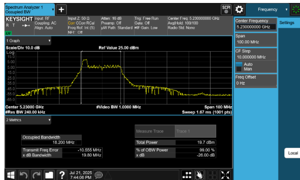
Plot 7-13 26dB BW & 99% OBW Antenna 4a (40MHz BW 802.11be(RU) RU26 Index0 - Ch.46)
