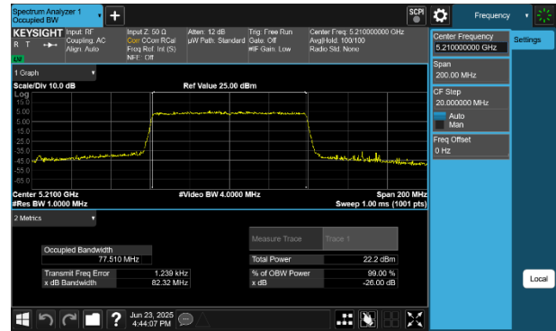
Plot 7-32 26dB BW & 99% OBW Antenna 2a (80MHz BW 802.11be(RU) RU996 Index67 - Ch.42)
