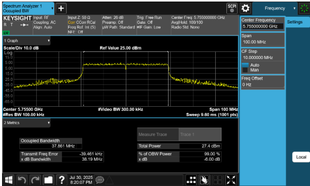
Plot 7-48 6dB BW & 99% OBW Antenna 4a (40MHz BW 802.11be(RU) RU484 Index65 - Ch.151)
