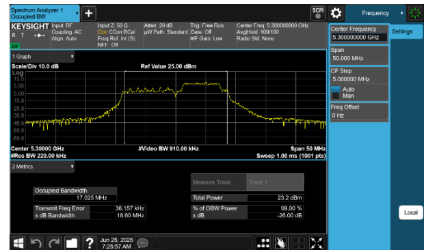
Plot 7-16 26dB BW & 99% OBW Antenna 4a (20MHz BW 802.11be(RU) RU52+26 Index72 - Ch.60)
