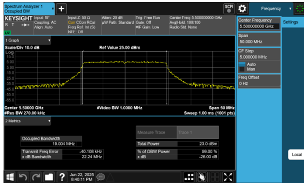
Plot 7-8 26dB BW & 99% OBW Antenna WF5B (20MHz BW 802.11be(RU) RU242 Index61 - Ch.100)
