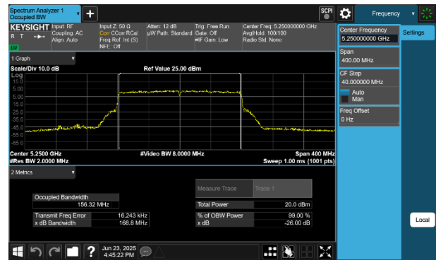
Plot 7-33 26dB BW & 99% OBW Antenna 2a (160MHz BW 802.11be(RU) RU996X2 Index68 - Ch.50)
