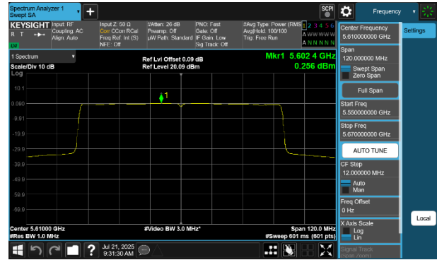
Plot 7-67 PSD Antenna WF5B (80MHz BW 802.11be(RU) RU996 Index67 - Ch.122)
