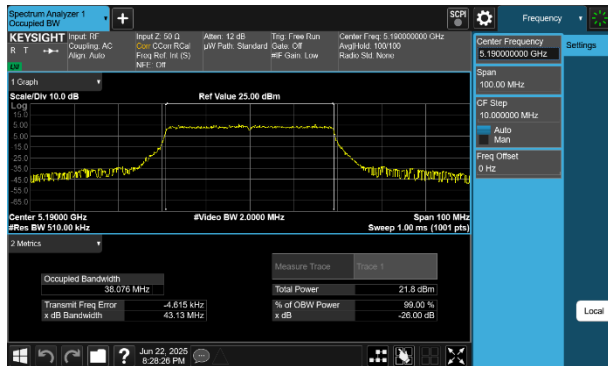
Plot 7-9 26dB BW & 99% OBW Antenna WF5B (40MHz BW 802.11be(RU) RU484 Index65 - Ch.38)
