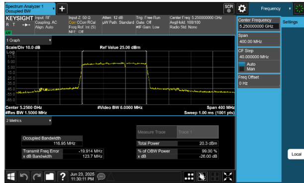
Plot 7-29 26dB BW & 99% OBW Antenna 2a (160MHz BW 802.11be(RU) RU996+484 Index95 - Ch.50)
