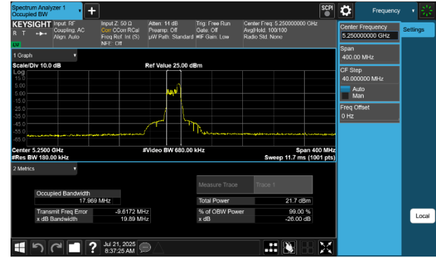
Plot 7-4 26dB BW & 99% OBW Antenna WF5B (160MHz BW 802.11be(RU) RU52 Index52 - Ch.50)
