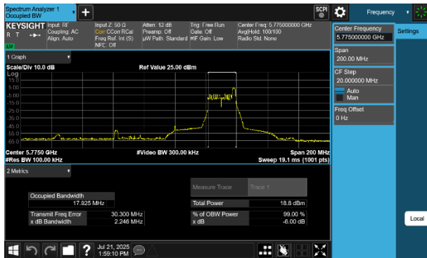
Plot 7-52 6dB BW & 99% OBW Antenna 2a (80MHz BW 802.11be(RU) RU26 Index36 - Ch.155)
