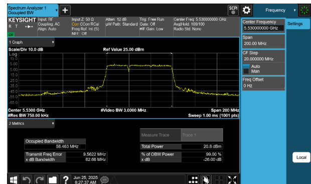
Plot 7-17 26dB BW & 99% OBW Antenna 4a (80MHz BW 802.11be(RU) RU484+242 Index90 - Ch.106)
