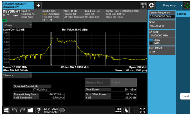
Plot 7-2 26dB BW & 99% OBW Antenna WF5B (40MHz BW 802.11be(RU) RU52 Index37 - Ch.102)
