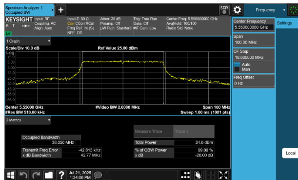
Plot 7-31 26dB BW & 99% OBW Antenna 2a (40MHz BW 802.11be(RU) RU484 Index65 - Ch.110)
