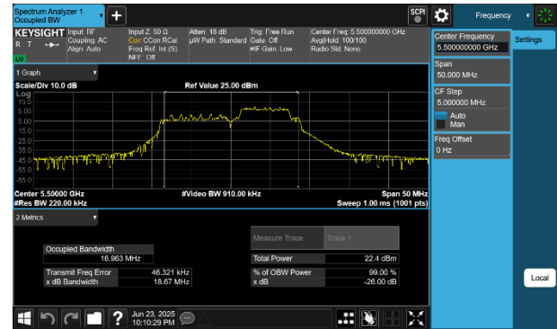
Plot 7-27 26dB BW & 99% OBW Antenna 2a (20MHz BW 802.11be(RU) RU52+26 Index72 - Ch.100)
