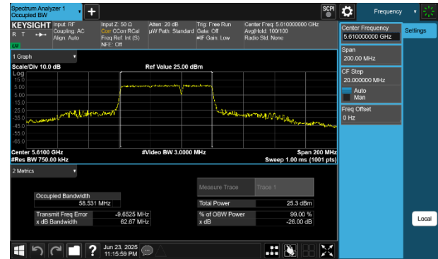
Plot 7-28 26dB BW & 99% OBW Antenna 2a (80MHz BW 802.11be(RU) RU484+242 Index93 - Ch.122)
