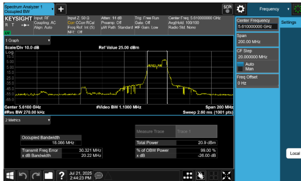
Plot 7-25 26dB BW & 99% OBW Antenna 2a (80MHz BW 802.11be(RU) RU52 Index52 - Ch.122)
