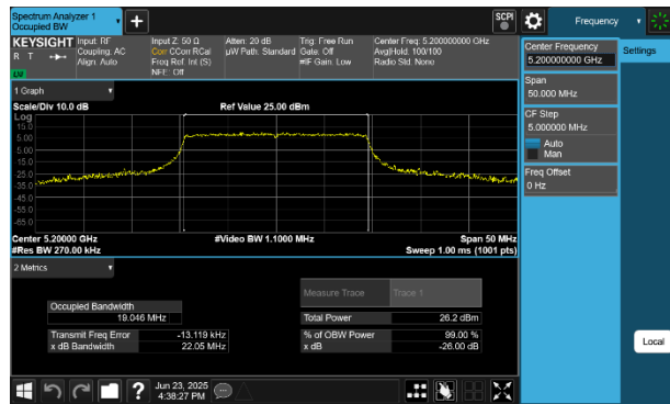
Plot 7-30 26dB BW & 99% OBW Antenna 2a (20MHz BW 802.11be(RU) RU242 Index61 - Ch.40)
