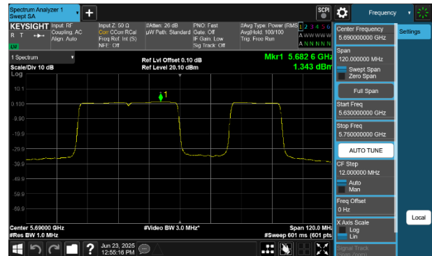
Plot 7-63 PSD Antenna WF5B (80MHz BW 802.11be(RU) RU484+242 Index92 - Ch.138)
