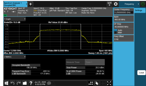
Plot 7-11 26dB BW & 99% OBW Antenna WF5B (160MHz BW 802.11be(RU) RU996X2 Index68 - Ch.50)
