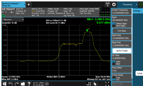
Plot 7-59 PSD Antenna WF5B (40MHz BW 802.11be(RU) RU52 Index44 - Ch.54)
