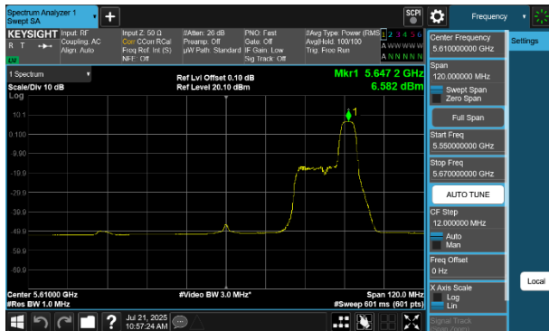
Plot 7-60 PSD Antenna WF5B (80MHz BW 802.11be(RU) RU52 Index52 - Ch.122)
