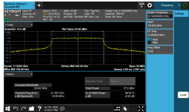
Plot 7-47 6dB BW & 99% OBW Antenna 4a (20MHz BW 802.11be(RU) RU242 Index61 - Ch.149)
