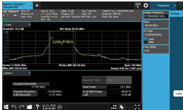
Plot 7-35 6dB BW & 99% OBW Antenna WF5B (40MHz BW 802.11be(RU) RU26 Index0 - Ch.159)
