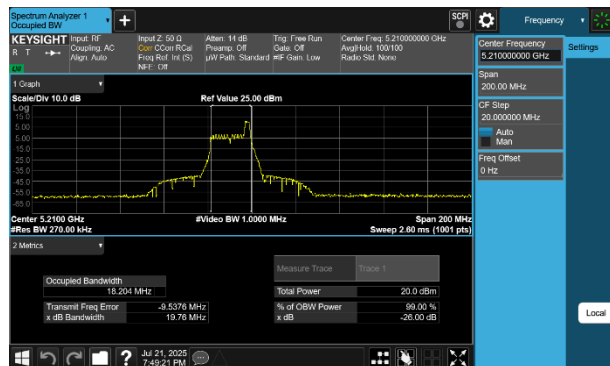
Plot 7-14 26dB BW & 99% OBW Antenna 4a (80MHz BW 802.11be(RU) RU26 Index17 - Ch.42)
