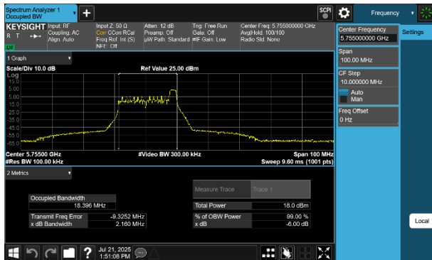
Plot 7-51 6dB BW & 99% OBW Antenna 2a (40MHz BW 802.11be(RU) RU26 Index8 - Ch.151)
