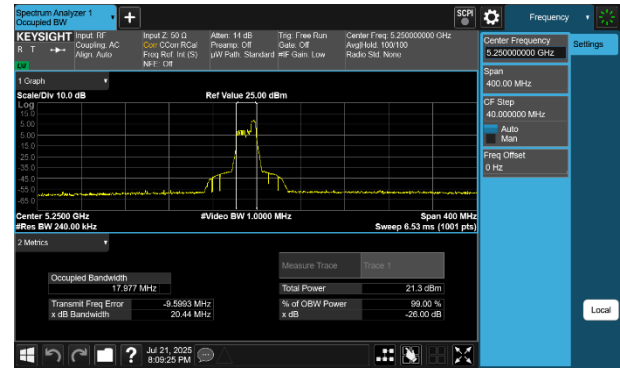
Plot 7-15 26dB BW & 99% OBW Antenna 4a (160MHz BW 802.11be(RU) RU52 Index52 - Ch.50)
