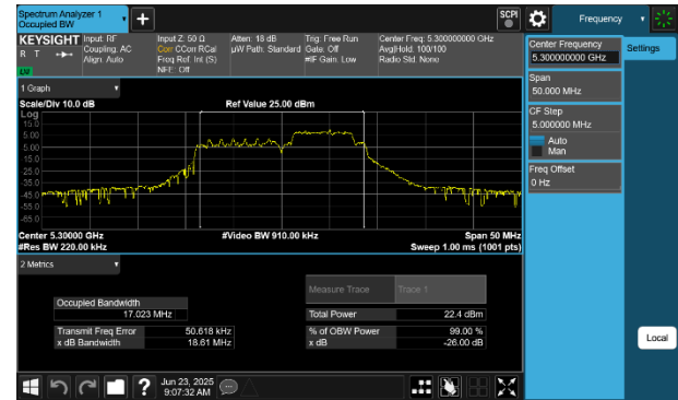
Plot 7-5 26dB BW & 99% OBW Antenna WF5B (20MHz BW 802.11be(RU) RU52+26 Index72 - Ch.60)
