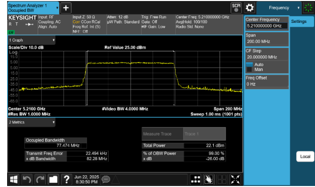
Plot 7-10 26dB BW & 99% OBW Antenna WF5B (80MHz BW 802.11be(RU) RU996 Index67 - Ch.42)
