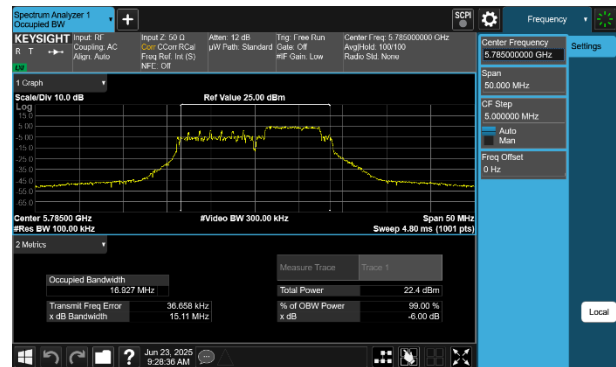
Plot 7-37 6dB BW & 99% OBW Antenna WF5B (20MHz BW 802.11be(RU) RU52+26 Index72 - Ch.157)
