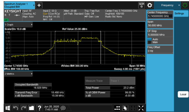
Plot 7-45 6dB BW & 99% OBW Antenna 4a (20MHz BW 802.11be(RU) RU52+26 Index72 - Ch.149)
