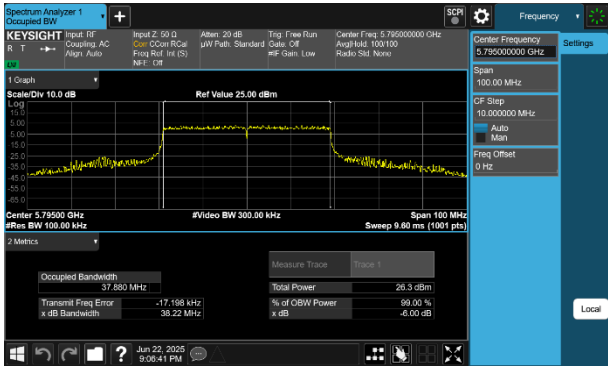
Plot 7-40 6dB BW & 99% OBW Antenna WF5B (40MHz BW 802.11be(RU) RU484 Index65 - Ch.159)
