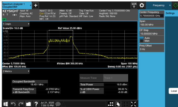
Plot 7-43 6dB BW & 99% OBW Antenna 4a (40MHz BW 802.11be(RU) RU26 Index8 - Ch.151)
