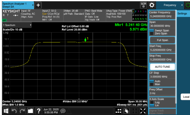
Plot 7-65 PSD Antenna WF5B (20MHz BW 802.11be(RU) RU242 Index61 - Ch.48)
