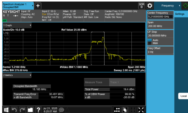
Plot 7-3 26dB BW & 99% OBW Antenna WF5B (80MHz BW 802.11be(RU) RU26 Index36 - Ch.42)
