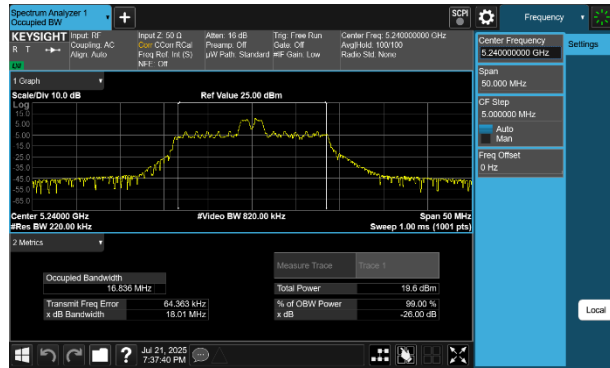
Plot 7-12 26dB BW & 99% OBW Antenna 4a (20MHz BW 802.11be(RU) RU26 Index4 - Ch.48)
