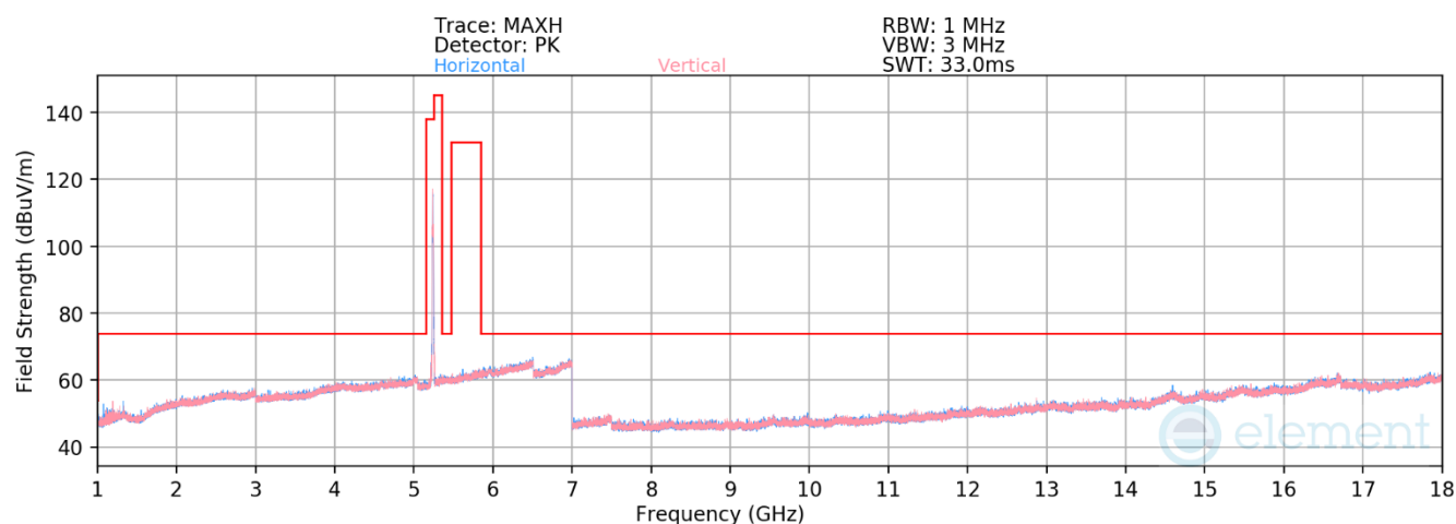
Plot 7-303. RSE above 1GHz CDD Diversity (11be – Ch.48 – RU26)
