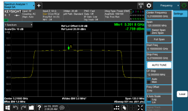
Plot 7-262 PSD SDM Diversity Antenna 2a (80MHz BW 802.11be(RU) RU996 Index67 - Ch.42)
