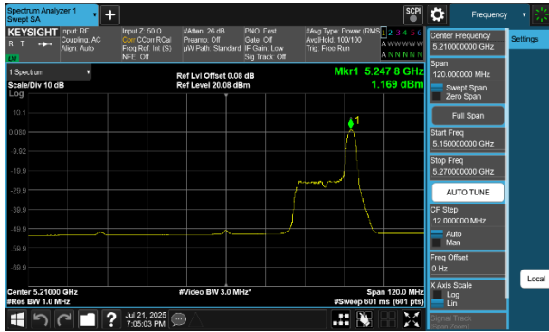
Plot 7-248 PSD SDM Diversity Antenna 2a (80MHz BW 802.11be(RU) RU26 Index36 - Ch.42)
