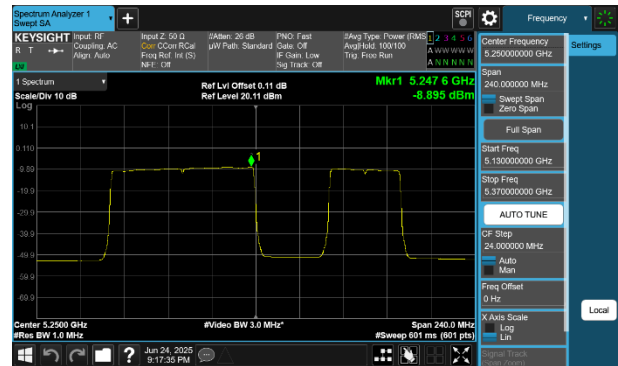
Plot 7-256 PSD CDD Diversity Antenna 2a (160MHz BW 802.11be(RU) RU996+484 Index94 - Ch.50)
