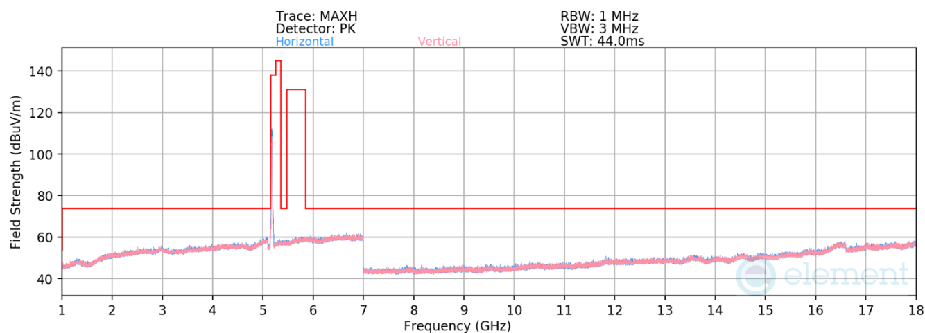
Plot 7-284. RSE above 1GHz CDD Primary (11be – Ch.36 – RU242)
