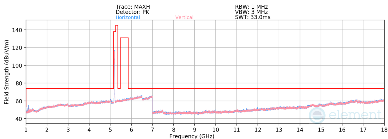
Plot 7-301. RSE above 1GHz CDD Diversity (11be - Ch.40 - RU26)
