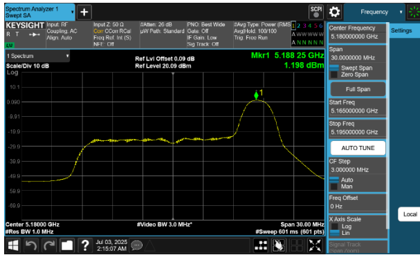
Plot 7-246 PSD SDM Diversity Antenna 2a (20MHz BW 802.11be(RU) RU26 Index8 - Ch.36)
