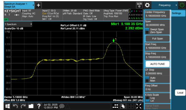
Plot 7-250 PSD SDM Diversity Antenna 4a (20MHz BW 802.11be(RU) RU26 Index8 - Ch.36)
