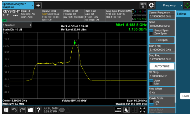
Plot 7-247 PSD SDM Diversity Antenna 2a (40MHz BW 802.11be(RU) RU26 Index8 - Ch.38)
