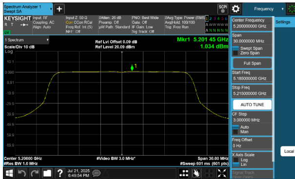
Plot 7-260 PSD SDM Diversity Antenna 2a (20MHz BW 802.11be(RU) RU242 Index61 - Ch.40)
