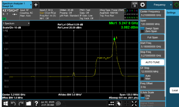
Plot 7-252 PSD SDM Diversity Antenna 4a (80MHz BW 802.11be(RU) RU26 Index36 - Ch.42)
