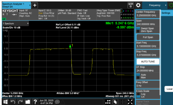
Plot 7-259 PSD CDD Diversity Antenna 4a (160MHz BW 802.11be(RU) RU996+484 Index94 - Ch.50)
