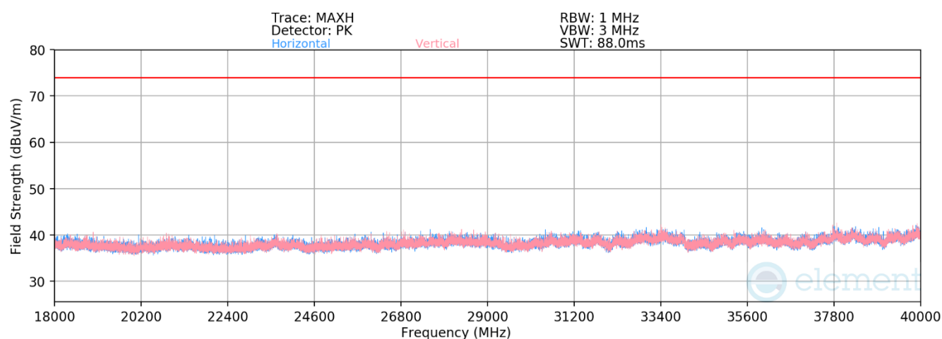
Plot 7-302. RSE 18GHz - 40 GHz CDD Diversity (11be Ch.40 - RU26)
