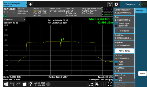
Plot 7-263 PSD SDM Diversity Antenna 2a (160MHz BW 802.11be(RU) RU996X2 Index68 - Ch.50)
