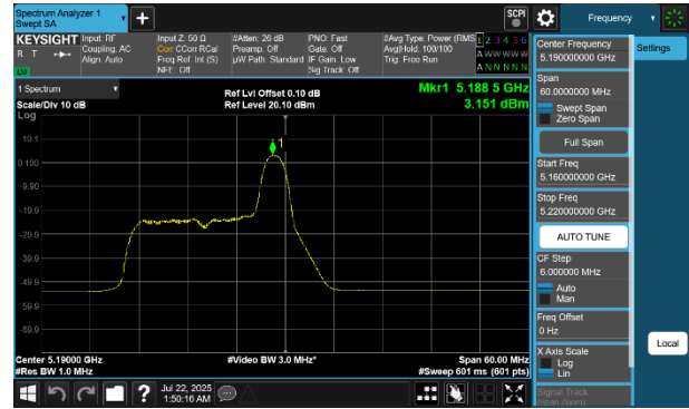
Plot 7-251 PSD SDM Diversity Antenna 4a (40MHz BW 802.11be(RU) RU26 Index8 - Ch.38)
