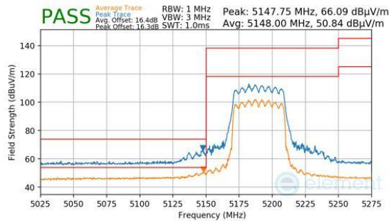
Plot 7-898. CDD Primary (Peak & Average, RU484, Index 65, Ch.38, MCS11)
