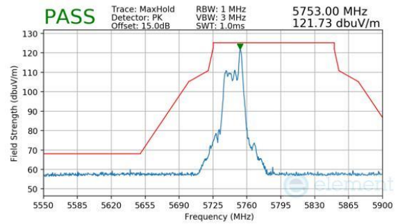
Plot 7-847. CDD Primary (Peak, RU26, Index 8, Ch.149, MCS11)
