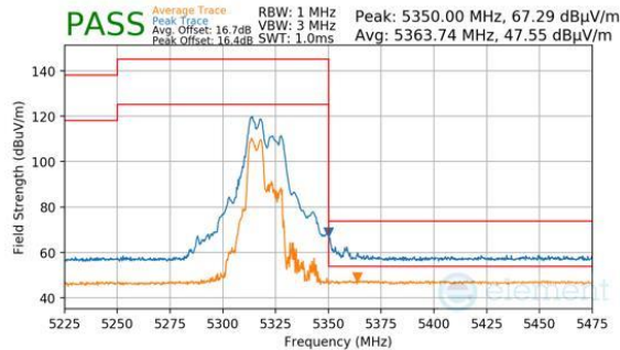
Plot 7-858. CDD Primary (Peak & Average, RU52+26, Index 70, Ch.64, MCS11)
