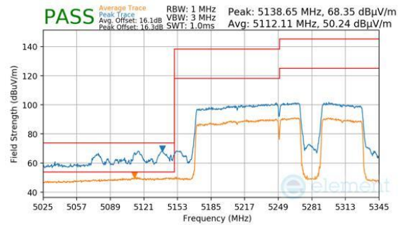
Plot 7-811. Antenna 2a (Peak & Average, RU996+484+242, Index 97 (H), Ch.50, MCS11)
