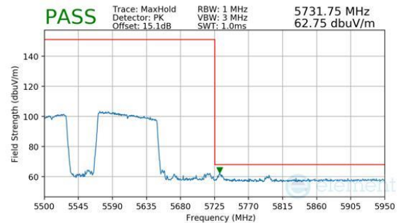
Plot 7-807. Antenna 2a (Peak, RU996+484, Index 95 (L), Ch.114 (FCC ONLY), MCS11)
