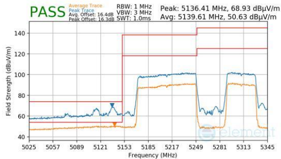
Plot 7-792. Antenna 2a (Peak & Average, RU996+484, Index 94 (H), Ch.50, MCS11)
