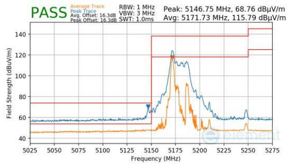
Plot 7-909. CDD Primary (Peak & Average, RU26, Index 0, Ch.42, MCS11)
