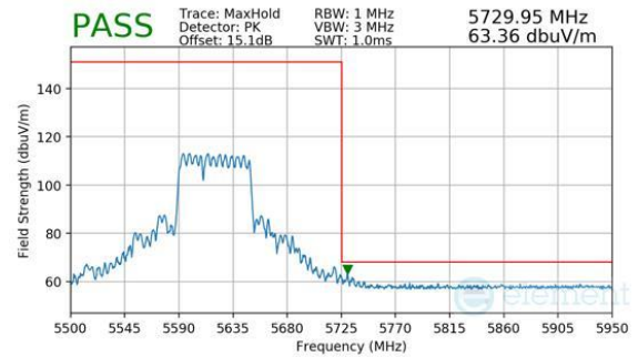
Plot 7-937. CDD Primary (Peak, RU484+242, Index 90, Ch.122 (FCC ONLY), MCS11)
