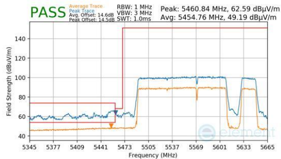
Plot 7-828. Antenna 2a (Peak & Average, RU996+484+242, Index 98 (H), Ch.114 (FCC ONLY), MCS11)
