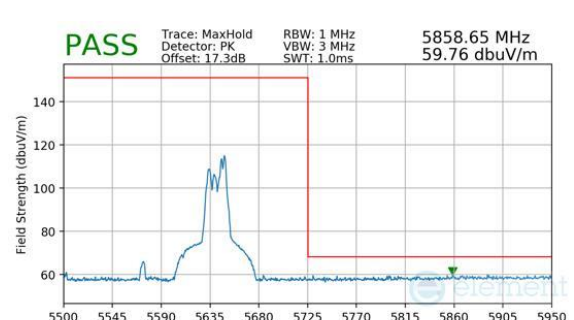
Plot 7-920. CDD Primary (Peak, RU52, Index 52, Ch.122 (FCC ONLY), MCS11)
