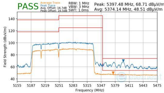
Plot 7-816. Antenna 2a (Peak & Average, RU996+484+242, Index 96 (L), Ch.50, MCS11)
