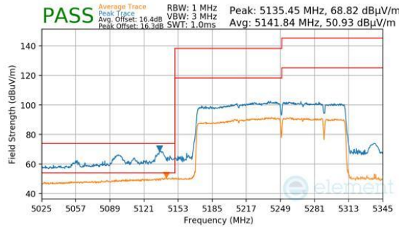
Plot 7-815. Antenna 2a (Peak & Average, RU996+484+242, Index 99 (H), Ch.50, MCS11)
