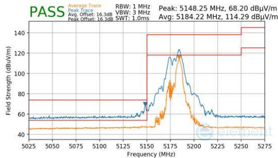
Plot 7-857. CDD Primary (Peak & Average, RU52+26, Index 72, Ch.36, MCS11)
