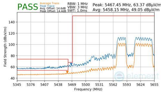
Plot 7-934. CDD Primary (Peak & Average, RU484+242, Index 91, Ch.122 (FCC ONLY), MCS11)
