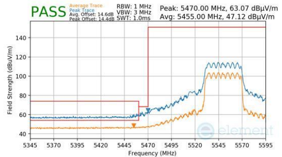
Plot 7-903. CDD Primary (Peak & Average, RU484, Index 65, Ch.110, MCS11)
