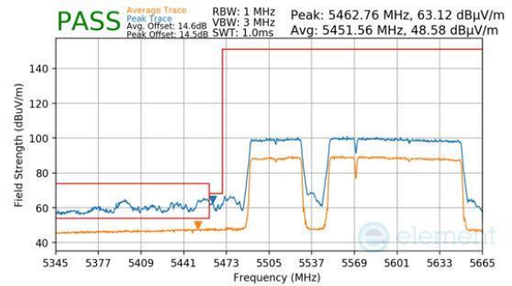
Plot 7-829. Antenna 2a (Peak & Average, RU996+484+242, Index 98 (L), Ch.114 (FCC ONLY), MCS11)
