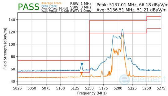
Plot 7-885. CDD Primary (Peak & Average, RU26, Index 17, Ch.38, MCS11)
