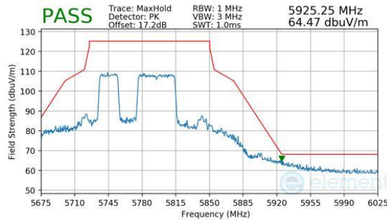
Plot 7-771. Antenna 2a (Peak, RU484+242, Index 91, Ch.155, MCS11)
