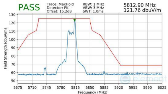
Plot 7-889. CDD Primary (Peak, RU26, Index 17, Ch.159, MCS11)
