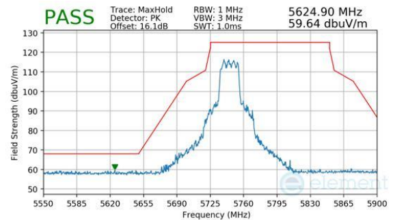
Plot 7-782. CDD Primary (Peak, RU242, Index 61, Ch.149, MCS11)
