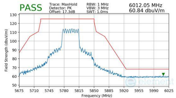
Plot 7-908. CDD Primary (Peak, RU484, Index 65, Ch.159, MCS11)
