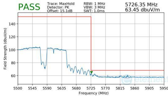
Plot 7-832. Antenna 2a (Peak, RU996+484+242, Index 96 (H), Ch.114 (FCC ONLY), MCS11)
