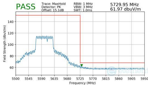
Plot 7-940. CDD Primary (Peak, RU484+242, Index 93, Ch.122 (FCC ONLY), MCS11)
