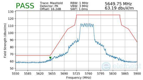
Plot 7-907. CDD Primary (Peak, RU484, Index 65, Ch.151, MCS11)
