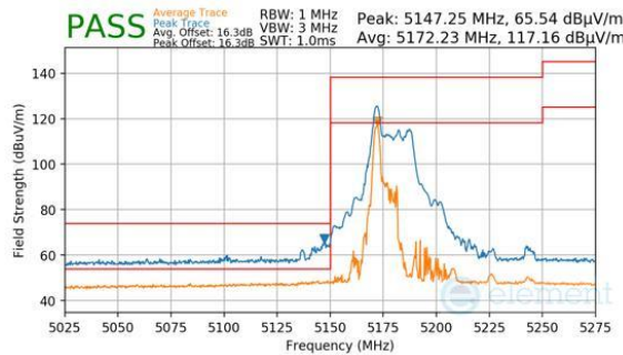
Plot 7-884. CDD Primary (Peak & Average, RU26, Index 0, Ch.38, MCS11)
