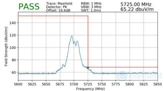
Plot 7-866. CDD Primary (Peak, RU52+26, Index 70, Ch.140, MCS11)
