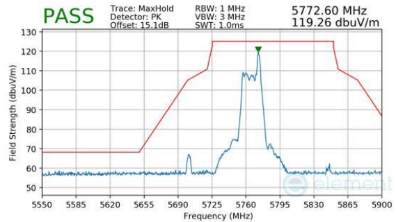
Plot 7-887. CDD Primary (Peak, RU26, Index 17, Ch.151, MCS11)
