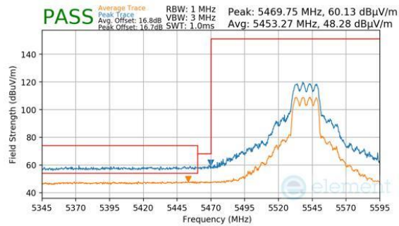
Plot 7-778. CDD Primary (Peak & Average, RU242, Index 61, Ch.108, MCS11)
