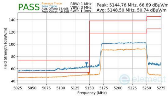
Plot 7-774. Antenna 2a (Peak & Average, RU996, Index 67, Ch.42, MCS11)
