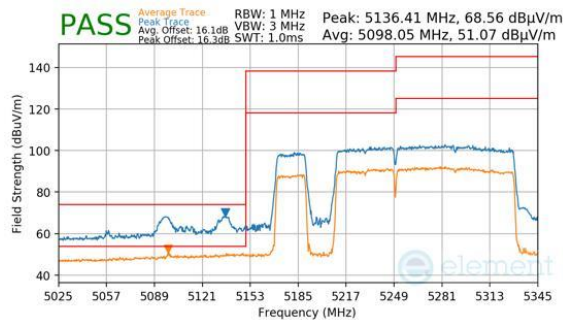
Plot 7-810. Antenna 2a (Peak & Average, RU996+484+242, Index 97 (L), Ch.50, MCS11)
