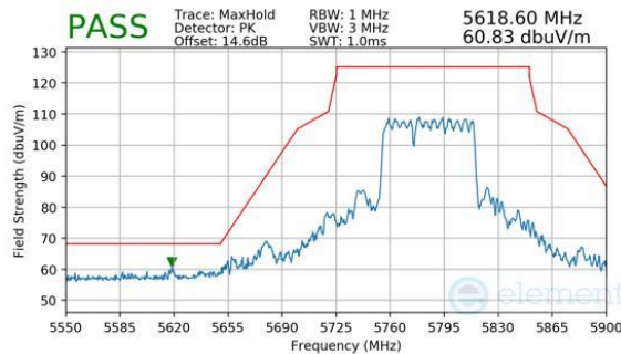
Plot 7-941. CDD Primary (Peak, RU484+242, Index 90, Ch.155, MCS11)
