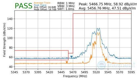
Plot 7-863. CDD Primary (Peak & Average, RU52+26, Index 72, Ch.104, MCS11)
