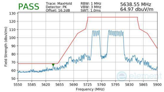
Plot 7-942. CDD Primary (Peak, RU484+242, Index 91, Ch.155, MCS11)
