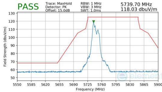
Plot 7-868. CDD Primary (Peak, RU52+26, Index 70, Ch.149, MCS11)
