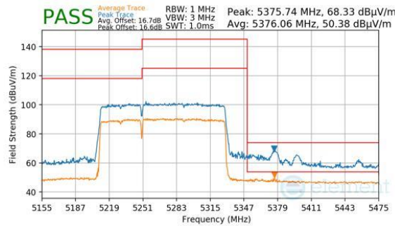
Plot 7-796. Antenna 2a (Peak & Average, RU996+484, Index 94 (L), Ch.50, MCS11)
