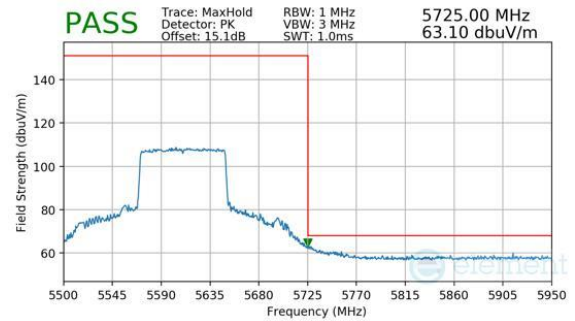
Plot 7-778. Antenna 2a (Peak, RU996, Index 67, Ch.122 (FCC ONLY), MCS11)
