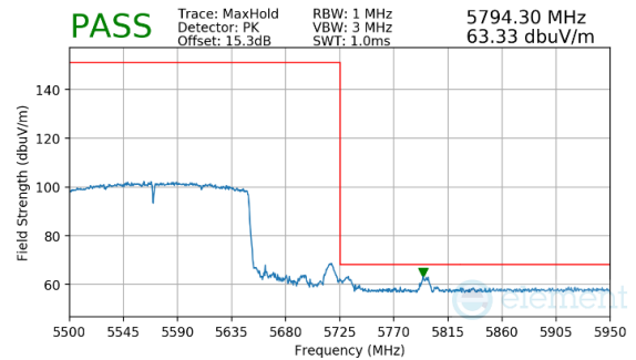
Plot 7-843. Antenna 2a (Peak & Average, RU996X2, Index 68, Ch. 114 (FCC ONLY), MCS11)
