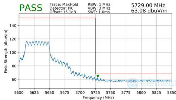
Plot 7-905. CDD Primary (Peak, RU484, Index 65, Ch.126 (FCC ONLY), MCS11)
