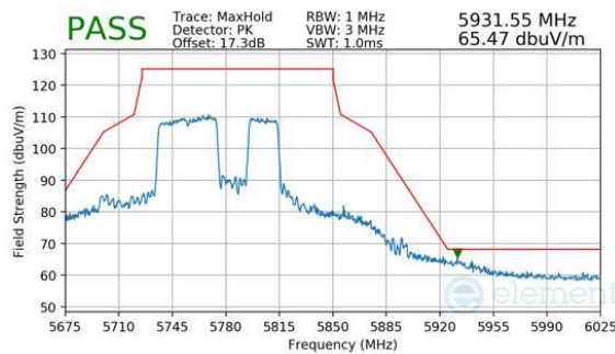
Plot 7-772. Antenna 2a (Peak, RU484+242, Index 92, Ch.155, MCS11)
