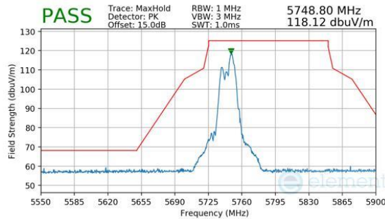
Plot 7-869. CDD Primary (Peak, RU52+26, Index 72, Ch.149, MCS11)
