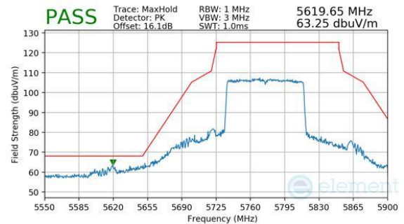
Plot 7-779. Antenna 2a (Peak, RU996, Index 67, Ch.155, MCS11)
