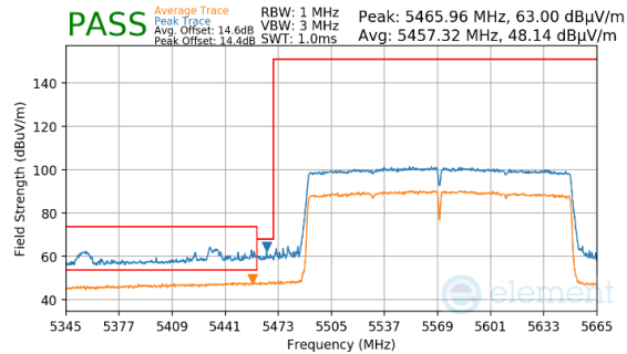
Plot 7-842. Antenna 2a (Peak & Average, RU996X2, Index 68, Ch.114 (FCC ONLY), MCS11)
