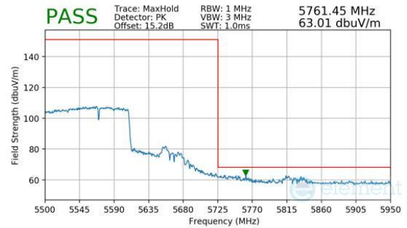
Plot 7-806. Antenna 2a (Peak, RU996+484, Index 95 (H), Ch.114 (FCC ONLY), MCS11)
