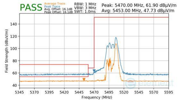
Plot 7-853. CDD Primary (Peak & Average, RU52, Index 40, Ch.100, MCS11)
