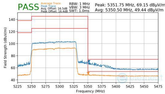
Plot 7-775. Antenna 2a (Peak & Average, RU996, Index 67, Ch.58, MCS11)
