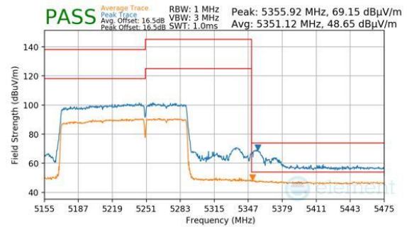
Plot 7-799. Antenna 2a (Peak & Average, RU996+484, Index 95 (H), Ch.50, MCS11)
