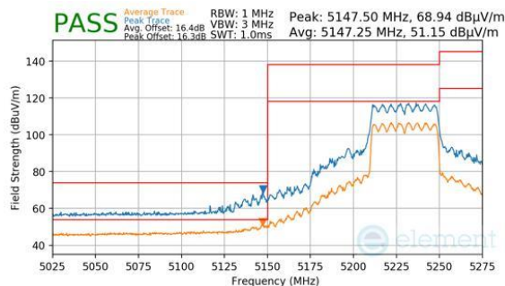
Plot 7-899. CDD Primary (Peak & Average, RU484, Index 65, Ch.46, MCS11)
