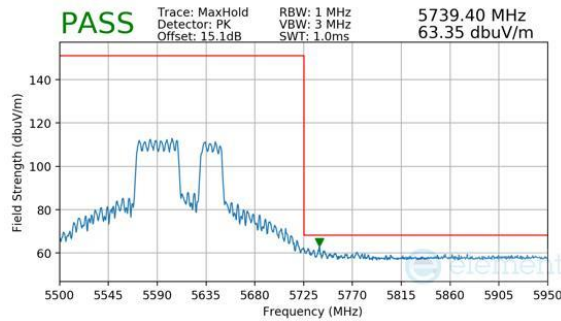
Plot 7-939. CDD Primary (Peak, RU484+242, Index 92, Ch.122 (FCC ONLY), MCS11)
