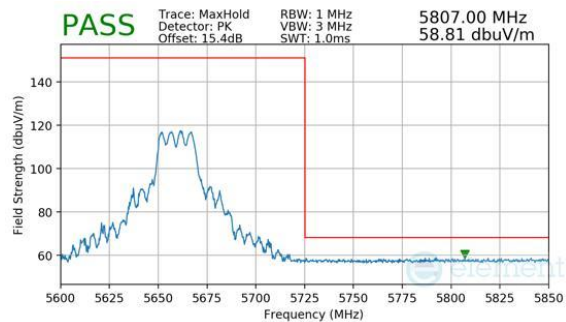
Plot 7-779. CDD Primary (Peak, RU242, Index 61, Ch.132, MCS11)
