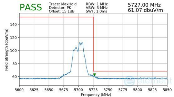
Plot 7-867. CDD Primary (Peak, RU52+26, Index 72, Ch.140, MCS11)
