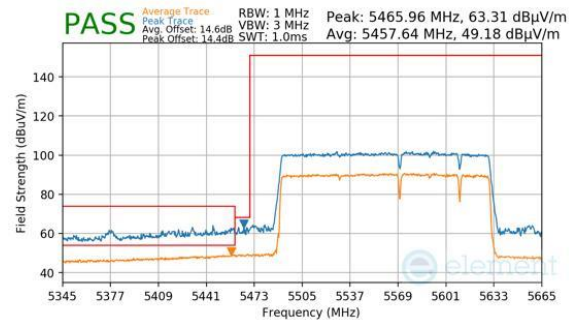
Plot 7-830. Antenna 2a (Peak & Average, RU996+484+242, Index 99 (H), Ch.114 (FCC ONLY), MCS11)
