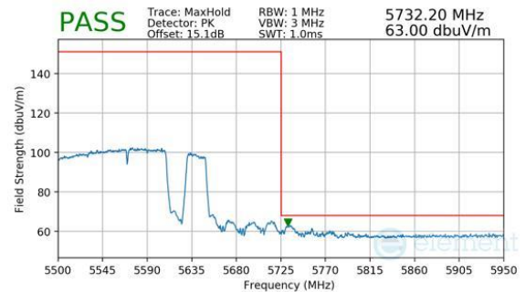
Plot 7-837. Antenna 2a (Peak, RU996+484+242, Index 98 (H), Ch.114 (FCC ONLY), MCS11)
