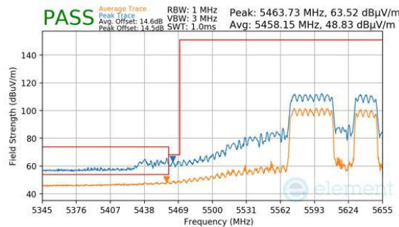
Plot 7-935. CDD Primary (Peak & Average, RU484+242, Index 92, Ch.122 (FCC ONLY), MCS11)
