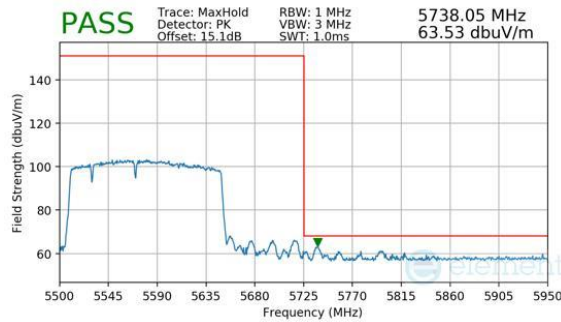
Plot 7-833. Antenna 2a (Peak, RU996+484+242, Index 96 (L), Ch.114 (FCC ONLY), MCS11)
