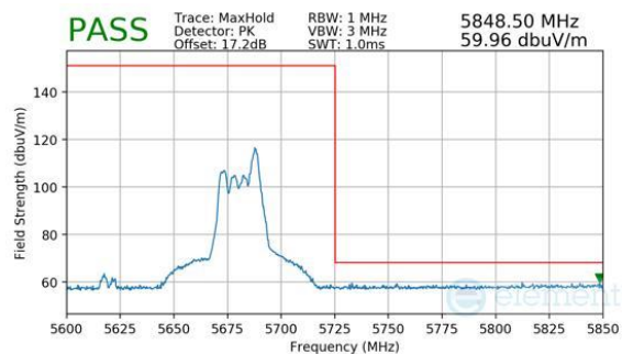
Plot 7-897. CDD Primary (Peak, RU52, Index 44, Ch.134, MCS11)
