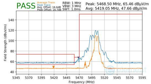
Plot 7-861. CDD Primary (Peak & Average, RU52+26, Index 72, Ch.100, MCS11)
