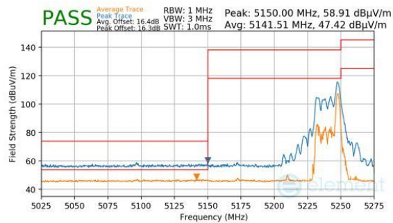
Plot 7-910. CDD Primary (Peak & Average, RU26, Index 36, Ch.42, MCS11)
