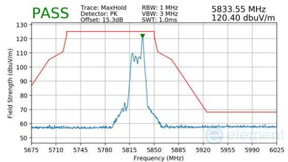
Plot 7-849. CDD Primary (Peak, RU26, Index 8, Ch.165, MCS11)
