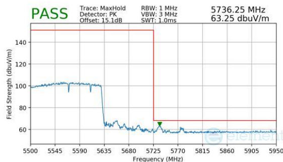
Plot 7-839. Antenna 2a (Peak, RU996+484+242, Index 99 (H), Ch.114 (FCC ONLY), MCS11)
