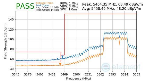
Plot 7-936. CDD Primary (Peak & Average, RU484+242, Index 93, Ch.122 (FCC ONLY), MCS11)
