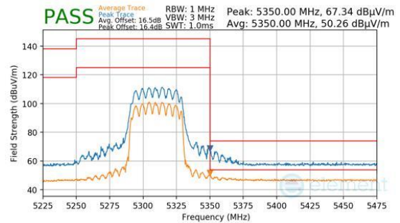
Plot 7-901. CDD Primary (Peak & Average, RU484, Index 65, Ch.62, MCS11)
