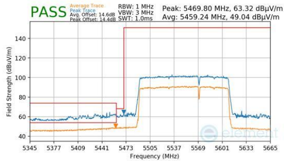
Plot 7-803. Antenna 2a (Peak & Average, RU996+484, Index 95 (H), Ch.114 (FCC ONLY), MCS11)
