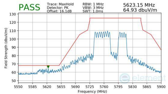
Plot 7-943. CDD Primary (Peak, RU484+242, Index 92, Ch.155, MCS11)
