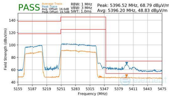
Plot 7-798. Antenna 2a (Peak & Average, RU996+484, Index 95 (L), Ch.50, MCS11)
