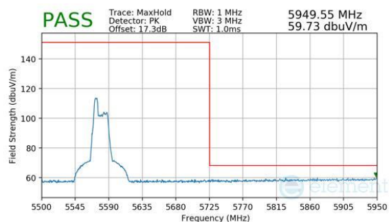
Plot 7-788. Antenna 2a (Peak, RU52, Index 37, Ch.114 (FCC ONLY), MCS11)
