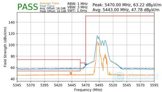
Plot 7-852. CDD Primary (Peak & Average, RU52, Index 37, Ch.100, MCS11)
