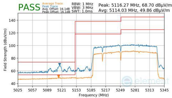
Plot 7-809. Antenna 2a (Peak & Average, RU996+484+242, Index 96 (L), Ch.50, MCS11)
