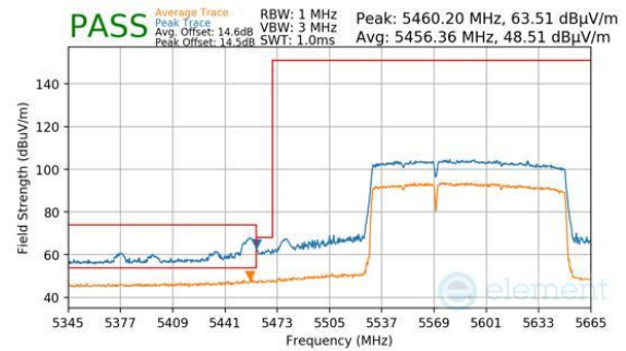
Plot 7-800. Antenna 2a (Peak & Average, RU996+484, Index 94 (L), Ch.114 (FCC ONLY), MCS11)
