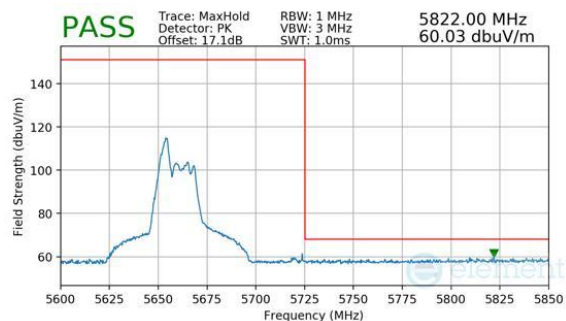
Plot 7-896. CDD Primary (Peak, RU52, Index 37, Ch.134, MCS11)
