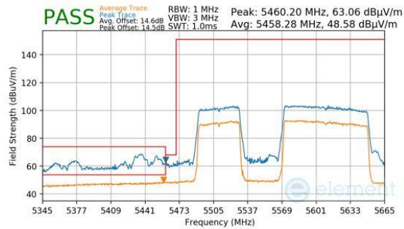
Plot 7-802. Antenna 2a (Peak & Average, RU996+484, Index 95 (L), Ch.114 (FCC ONLY), MCS11)
