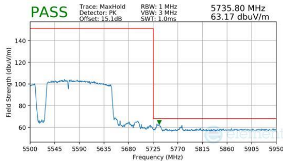
Plot 7-834. Antenna 2a (Peak, RU996+484+242, Index 97 (L), Ch.114 (FCC ONLY), MCS11)
