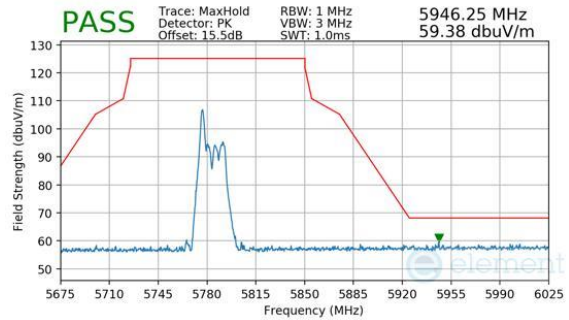
Plot 7-888. CDD Primary (Peak, RU26, Index 0, Ch.159, MCS11)
