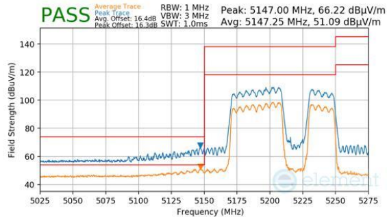
Plot 7-923. CDD Primary (Peak & Average, RU484+242, Index 92, Ch.42, MCS11)
