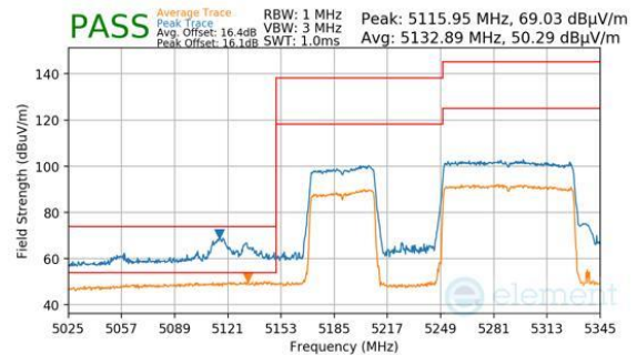
Plot 7-795. Antenna 2a (Peak & Average, RU996+484, Index 95 (L), Ch.50, MCS11)
