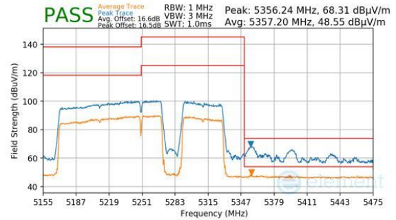
Plot 7-819. Antenna 2a (Peak & Average, RU996+484+242, Index 97 (H), Ch.50, MCS11)
