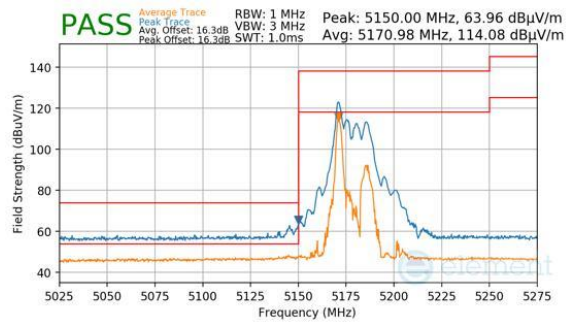
Plot 7-844. CDD Primary (Peak & Average, RU26, Index 0, Ch.36, MCS11)
