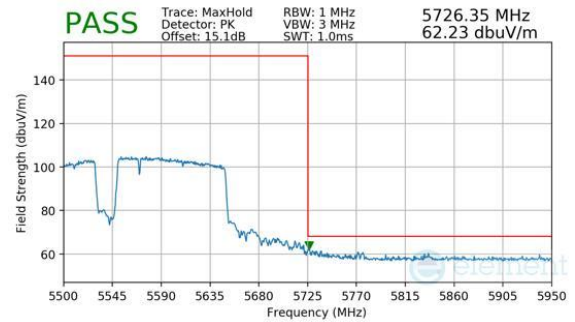
Plot 7-836. Antenna 2a (Peak, RU996+484+242, Index 98 (L), Ch.114 (FCC ONLY), MCS11)
