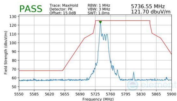
Plot 7-911. CDD Primary (Peak, RU26, Index 0, Ch.155, MCS11)
