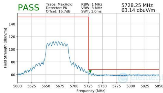
Plot 7-906. CDD Primary (Peak, RU484, Index 65, Ch.134, MCS11)
