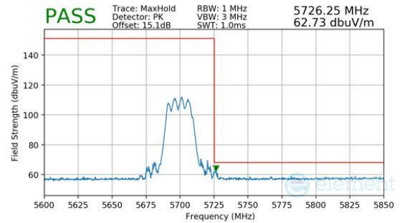
Plot 7-781. CDD Primary (Peak, RU242, Index 61, Ch.140, MCS11)
