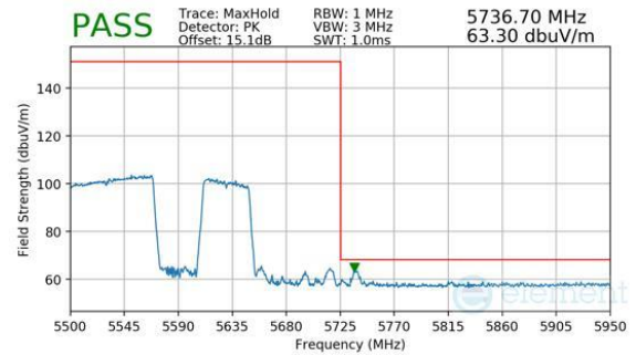
Plot 7-805. Antenna 2a (Peak, RU996+484, Index 94 (H), Ch.114 (FCC ONLY), MCS11)
