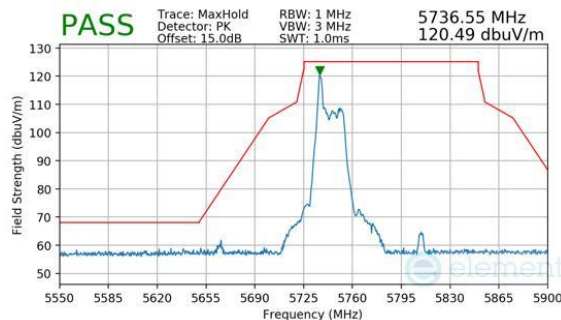
Plot 7-886. CDD Primary (Peak, RU26, Index 0, Ch.151, MCS11)
