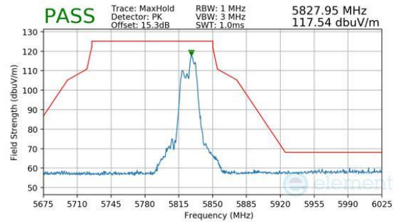
Plot 7-871. CDD Primary (Peak, RU52+26, Index 72, Ch.165, MCS11)
