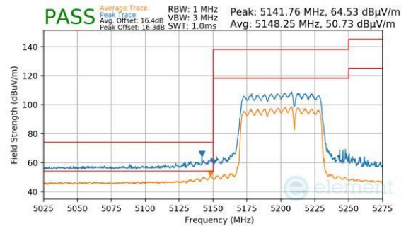
Plot 7-924. CDD Primary (Peak & Average, RU484+242, Index 93, Ch.42, MCS11)
