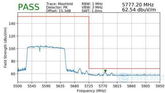
Plot 7-804. Antenna 2a (Peak, RU996+484, Index 94 (L), Ch.114 (FCC ONLY), MCS11)
