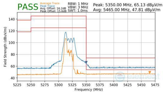
Plot 7-850. CDD Primary (Peak & Average, RU52, Index 37, Ch.64, MCS11)
