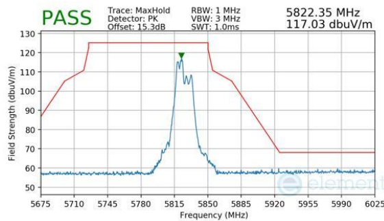
Plot 7-870. CDD Primary (Peak, RU52+26, Index 70, Ch.165, MCS11)
