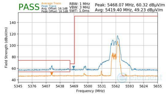
Plot 7-918. CDD Primary (Peak & Average, RU52, Index 52, Ch.106, MCS11)
