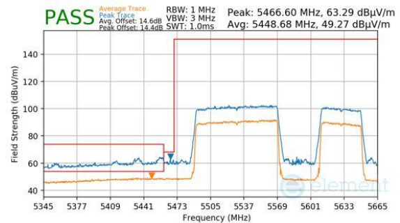
Plot 7-801. Antenna 2a (Peak & Average, RU996+484, Index 94 (H), Ch.114 (FCC ONLY), MCS11)
