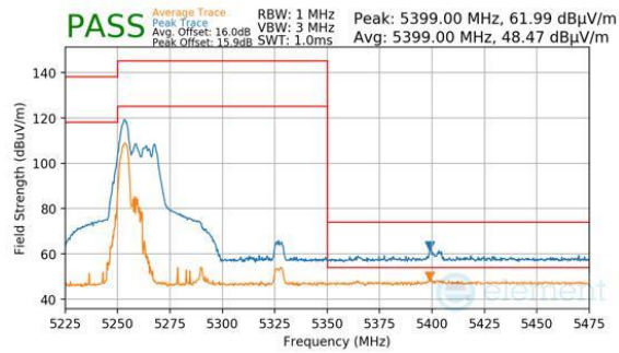
Plot 7-915. CDD Primary (Peak & Average, RU52, Index 37, Ch.58, MCS11)
