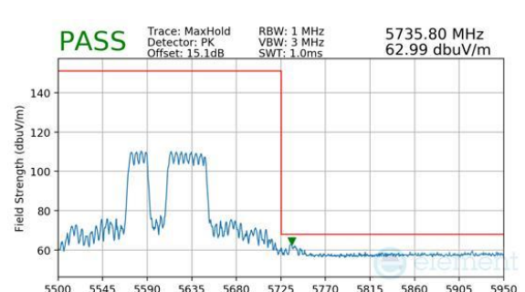
Plot 7-938. CDD Primary (Peak, RU484+242, Index 91, Ch.122 (FCC ONLY), MCS11)
