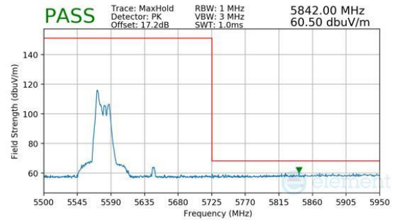
Plot 7-919. CDD Primary (Peak, RU52, Index 37, Ch.122 (FCC ONLY), MCS11)
