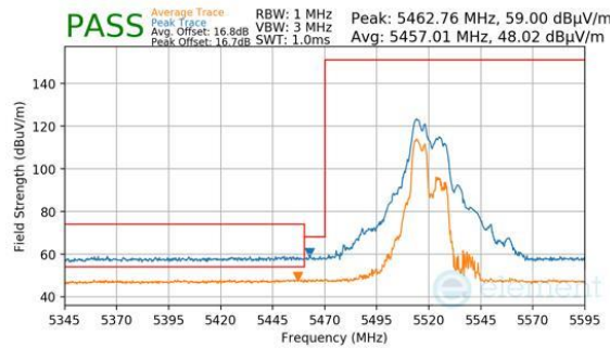
Plot 7-862. CDD Primary (Peak & Average, RU52+26, Index 70, Ch.104, MCS11)
