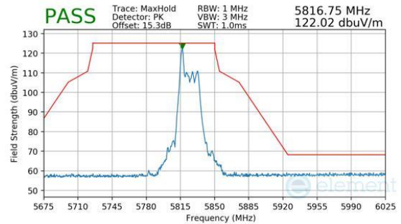
Plot 7-848. CDD Primary (Peak, RU26, Index 0, Ch.165, MCS11)
