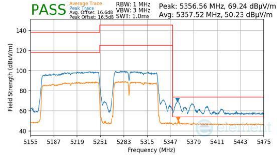
Plot 7-817. Antenna 2a (Peak & Average, RU996+484+242, Index 96 (H), Ch.50, MCS11)
