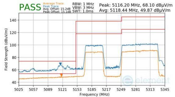
Plot 7-793. Antenna 2a (Peak & Average, RU996+484, Index 95, Ch.50, MCS11)
