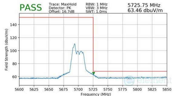
Plot 7-854. CDD Primary (Peak, RU52, Index 37, Ch.140, MCS11)
