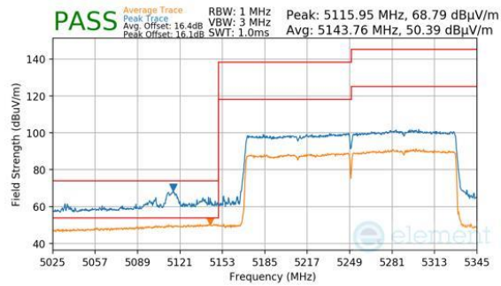
Plot 7-840. Antenna 2a (Peak & Average, RU996X2, Index 68, Ch.50, MCS11)
