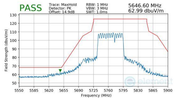
Plot 7-944. CDD Primary (Peak, RU484+242, Index 93, Ch.155, MCS11)
