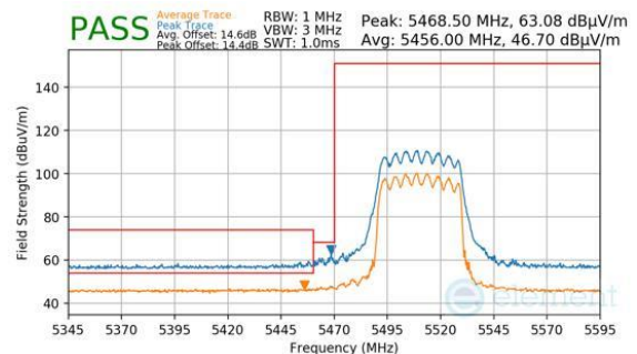
Plot 7-902. CDD Primary (Peak & Average, RU484, Index 65, Ch.102, MCS11)
