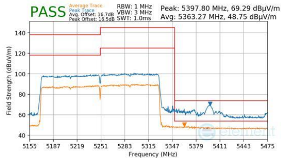
Plot 7-841. Antenna 2a (Peak & Average, RU996X2, Index 68, Ch.50, MCS11)
