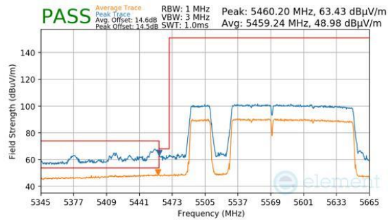
Plot 7-826. Antenna 2a (Peak & Average, RU996+484+242, Index 97 (L), Ch.114 (FCC ONLY), MCS11)
