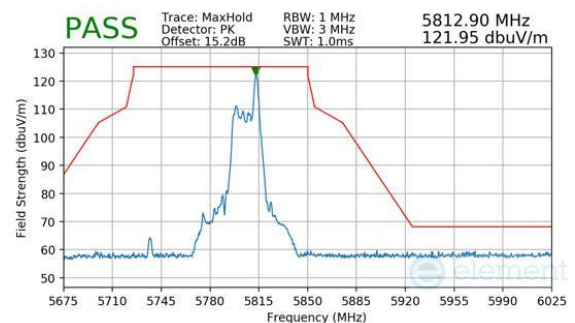
Plot 7-914. CDD Primary (Peak, RU26, Index 36, Ch.155, MCS11)
