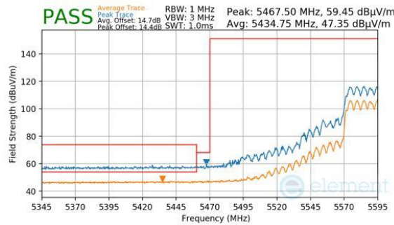
Plot 7-904. CDD Primary (Peak & Average, RU484, Index 65, Ch.118 (FCC ONLY), MCS11)
