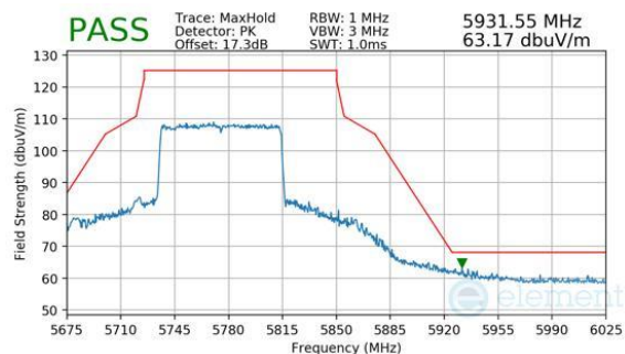
Plot 7-780. Antenna 2a (Peak, RU996, Index 67, Ch.155, MCS11)
