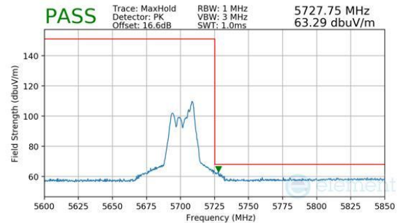
Plot 7-855. CDD Primary (Peak, RU52, Index 40, Ch.140, MCS11)
