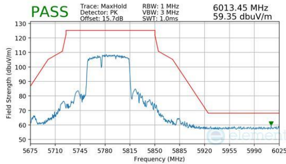
Plot 7-770. Antenna 2a (Peak, RU484+242, Index 90, Ch.155, MCS11)
