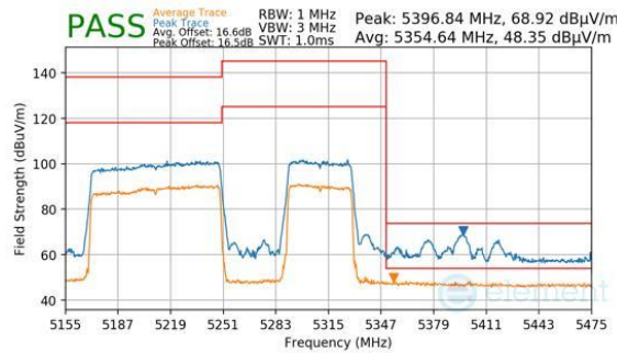
Plot 7-797. Antenna 2a (Peak & Average, RU996+484, Index 94 (H), Ch.50, MCS11)
