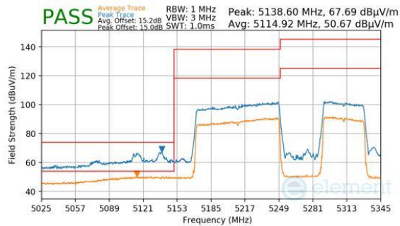
Plot 7-790. Antenna 2a (Peak & Average, RU996+484, Index 94, Ch.50, MCS11)
