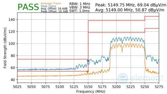
Plot 7-921. CDD Primary (Peak & Average, RU484+242, Index 90, Ch.42, MCS11)
