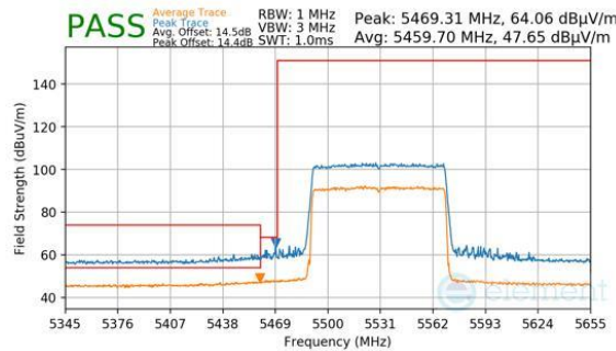
Plot 7-776. Antenna 2a (Peak & Average, RU996, Index 67, Ch.106, MCS11)
