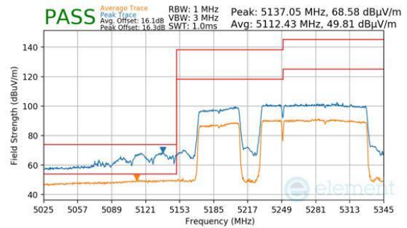
Plot 7-812. Antenna 2a (Peak & Average, RU996+484+242, Index 98 (L), Ch.50, MCS11)
