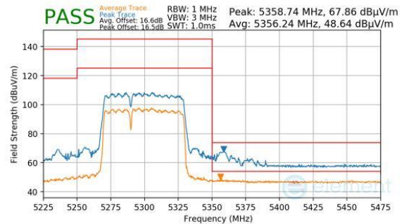
Plot 7-925. CDD Primary (Peak & Average, RU484+242, Index 90, Ch.58, MCS11)
