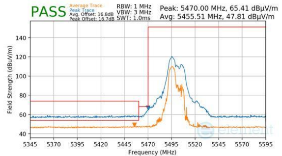
Plot 7-860. CDD Primary (Peak & Average, RU52+26, Index 70, Ch.100, MCS11)
