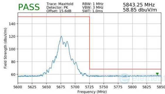
Plot 7-864. CDD Primary (Peak, RU52+26, Index 70, Ch.136, MCS11)
