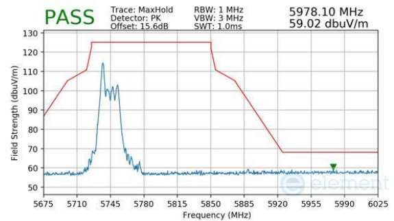
Plot 7-913. CDD Primary (Peak, RU26, Index 0, Ch.155, MCS11)
