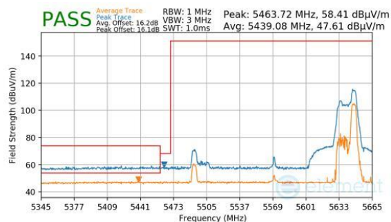
Plot 7-787. Antenna 2a (Peak & Average, RU52, Index 52 (H), Ch.114 (FCC ONLY), MCS11)
