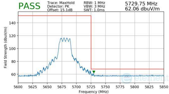
Plot 7-780. CDD Primary (Peak, RU242, Index 61, Ch.136, MCS11)
