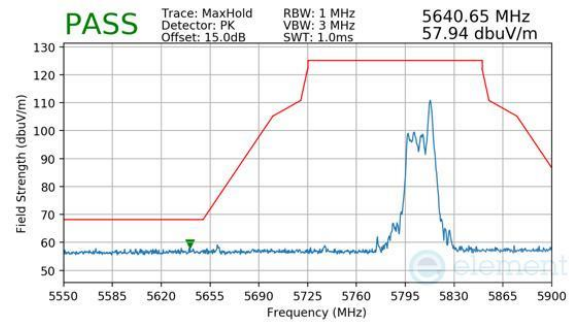
Plot 7-912. CDD Primary (Peak, RU26, Index 36, Ch.155, MCS11)
