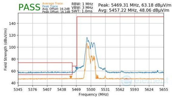
Plot 7-917. CDD Primary (Peak & Average, RU52, Index 37, Ch.106, MCS11)
