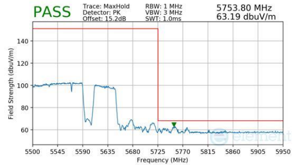
Plot 7-835. Antenna 2a (Peak, RU996+484+242, Index 97 (H), Ch.114 (FCC ONLY), MCS11)
