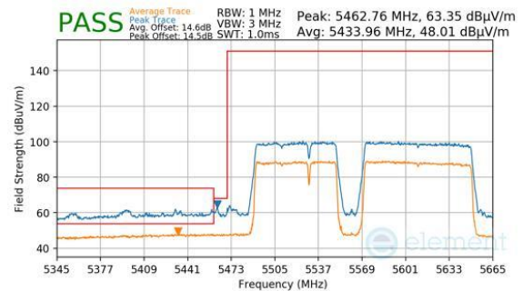
Plot 7-831. Antenna 2a (Peak & Average, RU996+484+242, Index 99 (L), Ch.114 (FCC ONLY), MCS11)
