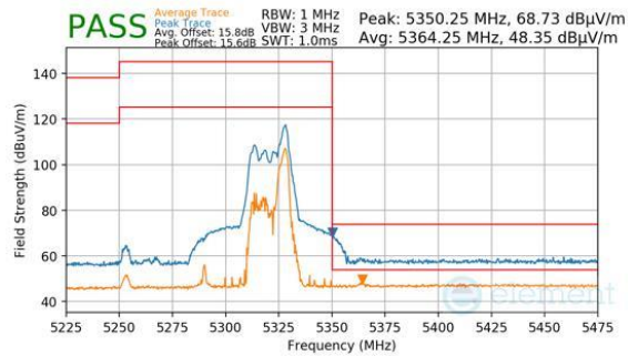
Plot 7-916. CDD Primary (Peak & Average, RU52, Index 52, Ch.58, MCS11)
