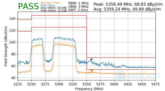
Plot 7-926. CDD Primary (Peak & Average, RU484+242, Index 91, Ch.58, MCS11)
