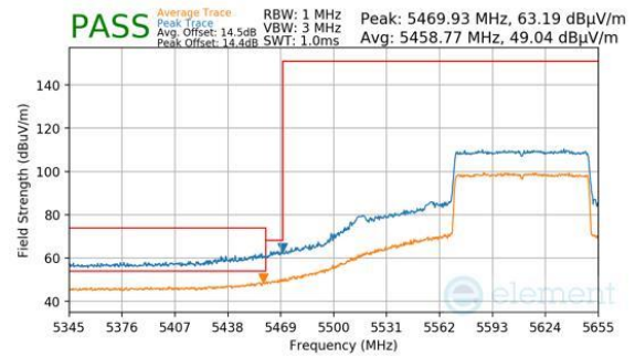
Plot 7-777. Antenna 2a (Peak & Average, RU996, Index 67, Ch.122 (FCC ONLY), MCS11)
