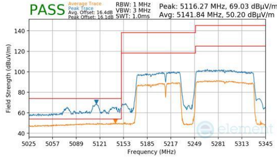
Plot 7-814. Antenna 2a (Peak & Average, RU996+484+242, Index 99 (L), Ch.50, MCS11)
