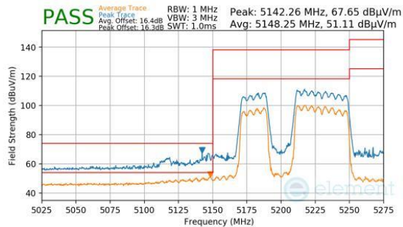
Plot 7-922. CDD Primary (Peak & Average, RU484+242, Index 91, Ch.42, MCS11)
