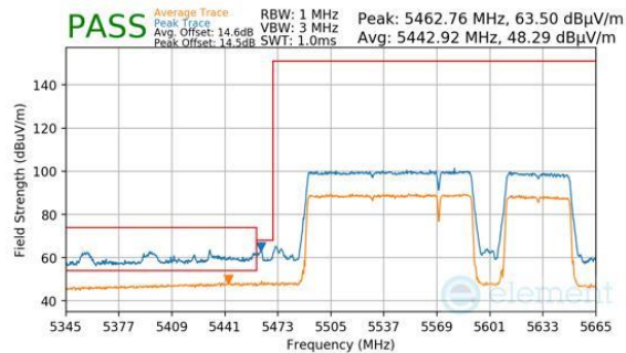
Plot 7-827. Antenna 2a (Peak & Average, RU996+484+242, Index 97 (H), Ch.114 (FCC ONLY), MCS11)
