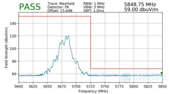
Plot 7-865. CDD Primary (Peak, RU52+26, Index 72, Ch.136, MCS11)
