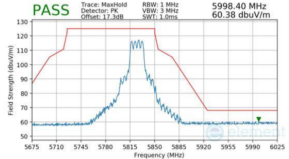
Plot 7-783. CDD Primary (Peak, RU242, Index 61, Ch.165, MCS11)
