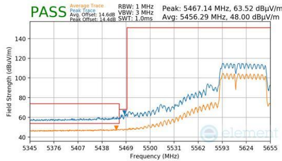
Plot 7-933. CDD Primary (Peak & Average, RU484+242, Index 90, Ch.122 (FCC ONLY), MCS11)
