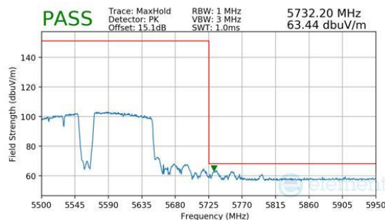
Plot 7-838. Antenna 2a (Peak, RU996+484+242, Index 99 (L), Ch.114 (FCC ONLY), MCS11)
