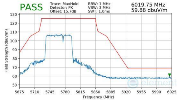
Plot 7-773. Antenna 2a (Peak, RU484+242, Index 93, Ch.155, MCS11)
