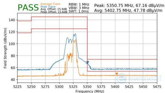
Plot 7-851. CDD Primary (Peak & Average, RU52, Index 40, Ch.64, MCS11)
