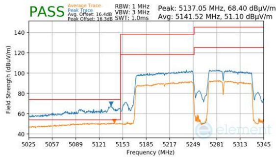
Plot 7-808. Antenna 2a (Peak & Average, RU996+484+242, Index 96 (H), Ch.50, MCS11)
