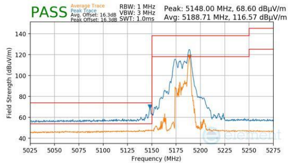
Plot 7-845. CDD Primary (Peak & Average, RU26, Index 8, Ch.36, MCS11)
