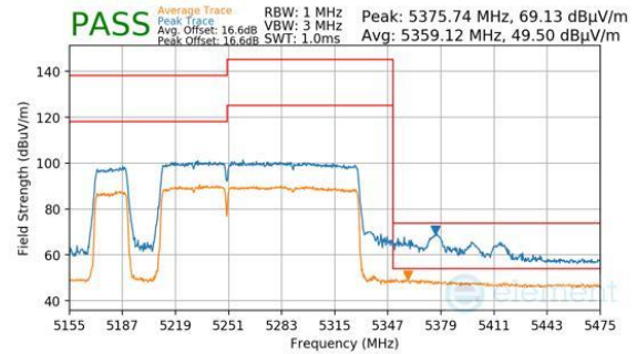
Plot 7-818. Antenna 2a (Peak & Average, RU996+484+242, Index 97 (L), Ch.50, MCS11)
