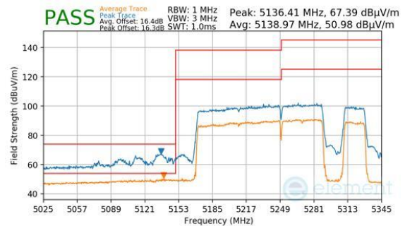
Plot 7-813. Antenna 2a (Peak & Average, RU996+484+242, Index 98 (H), Ch.50, MCS11)
