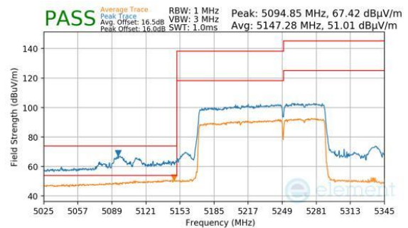
Plot 7-794. Antenna 2a (Peak & Average, RU996+484, Index 95 (H), Ch.50, MCS11)
