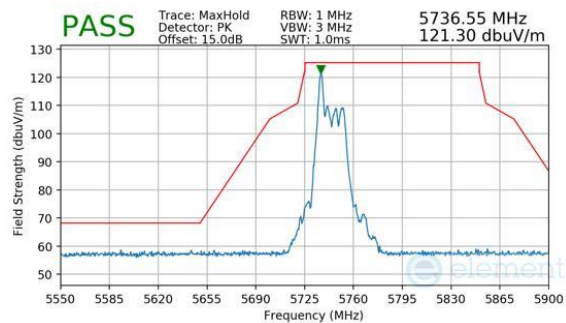
Plot 7-846. CDD Primary (Peak, RU26, Index 0, Ch.149, MCS11)
