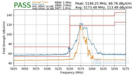
Plot 7-856. CDD Primary (Peak & Average, RU52+26, Index 70, Ch.36, MCS11)
