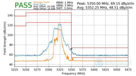
Plot 7-859. CDD Primary (Peak & Average, RU52+26, Index 72, Ch.64, MCS11)
