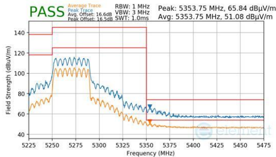
Plot 7-900. CDD Primary (Peak & Average, RU484, Index 65, Ch.54, MCS11)
