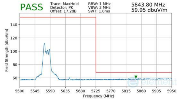
Plot 7-1086. CDD Diversity (Peak, RU52, Index 37, Ch.122 (FCC ONLY), MCS11)
