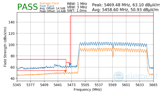
Plot 7-1007. CDD Primary (Peak & Average, RU996X2, Index 68, Ch.114 (FCC ONLY), MCS11)
