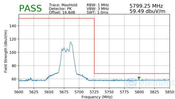
Plot 7-1064. CDD Diversity (Peak, RU52, Index 44, Ch.134, MCS11)
