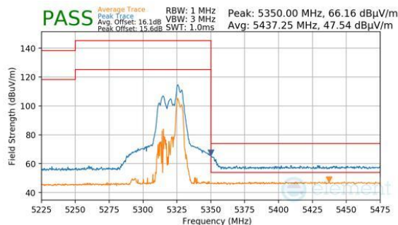
Plot 7-1058. CDD Diversity (Peak & Average, RU52, Index 44, Ch.62, MCS11)
