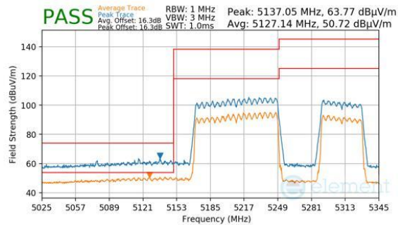
Plot 7-965. CDD Primary (Peak & Average, RU996+484, Index 94, Ch.50, MCS11)
