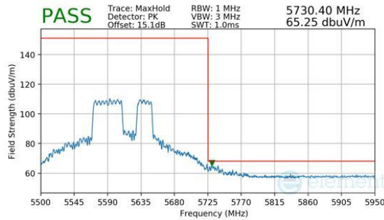
Plot 7-1106. CDD Diversity (Peak, RU484+242, Index 92, Ch.122 (FCC ONLY), MCS11)
