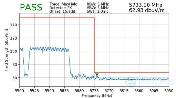
Plot 7-1000. CDD Primary (Peak, RU996+484+242, Index 97 (L), Ch.114 (FCC ONLY), MCS11)
