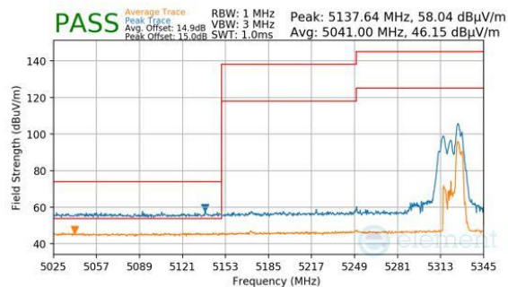
Plot 7-957. CDD Primary (Peak & Average, RU52, Index 52 (H), Ch.50, MCS11)
