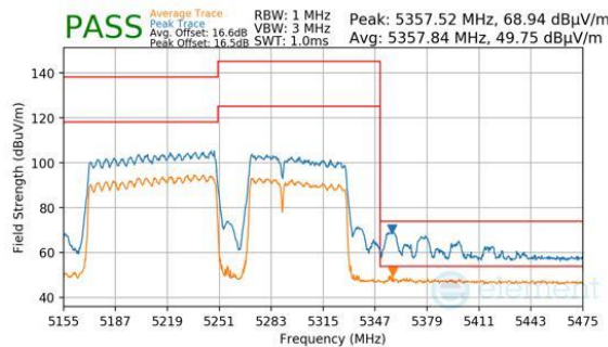
Plot 7-985. CDD Primary (Peak & Average, RU996+484+242, Index 96, Ch.50, MCS11)
