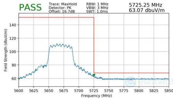
Plot 7-1073. CDD Diversity (Peak, RU484, Index 65, Ch.134, MCS11)
