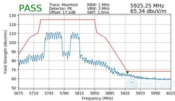
Plot 7-947. CDD Primary (Peak, RU484+242, Index 92, Ch.155, MCS11)
