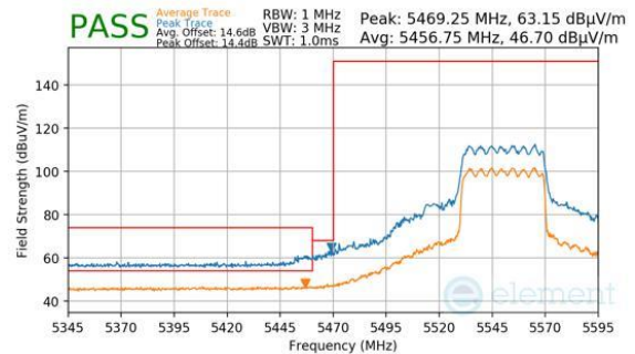
Plot 7-1070. CDD Diversity (Peak & Average, RU484, Index 65, Ch.110, MCS11)
