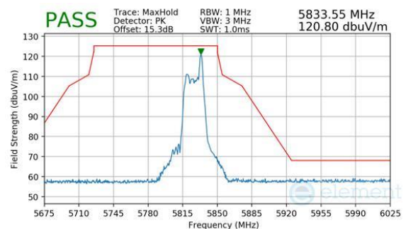
Plot 7-1014. CDD Diversity (Peak, RU26, Index 8, Ch.165, MCS11)
