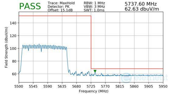
Plot 7-998. CDD Primary (Peak, RU996+484+242, Index 96 (L), Ch.114 (FCC ONLY), MCS11)
