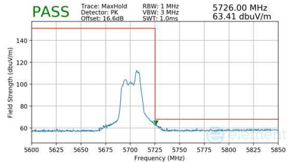
Plot 7-1020. CDD Diversity (Peak, RU52, Index 40, Ch.140, MCS11)
