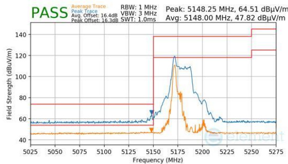
Plot 7-1009. CDD Diversity (Peak & Average, RU26, Index 0, Ch.36, MCS11)
