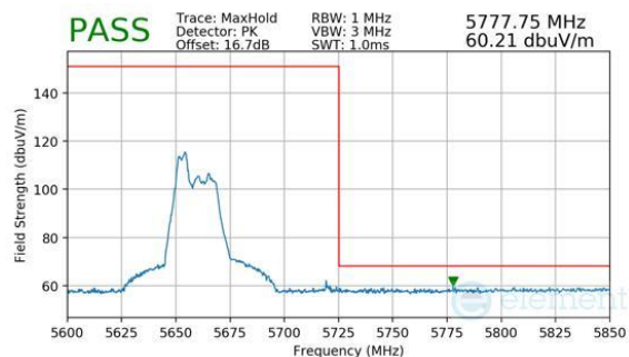
Plot 7-1063. CDD Diversity (Peak, RU52, Index 37, Ch.134, MCS11)
