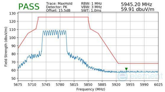
Plot 7-948. CDD Primary (Peak, RU484+242, Index 93, Ch.155, MCS11)
