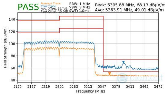
Plot 7-1006. CDD Primary (Peak & Average, RU996X2, Index 68, Ch.50, MCS11)
