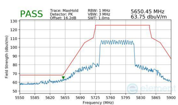
Plot 7-1121. CDD Diversity (Peak, RU996, Index 67, Ch.155, MCS11)
