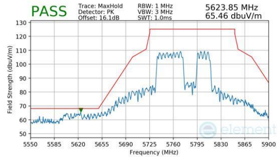
Plot 7-1110. CDD Diversity (Peak, RU484+242, Index 92, Ch.155, MCS11)
