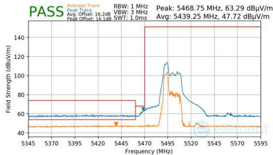
Plot 7-1059. CDD Diversity (Peak & Average, RU52, Index 37, Ch.102, MCS11)
