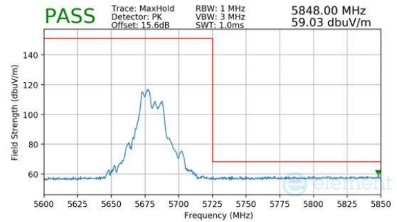
Plot 7-1031. CDD Diversity (Peak, RU52+26, Index 70, Ch.136, MCS11)
