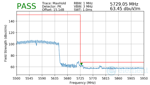
Plot 7-1008. CDD Primary (Peak & Average, RU996X2, Index 68, Ch.114 (FCC ONLY), MCS11)
