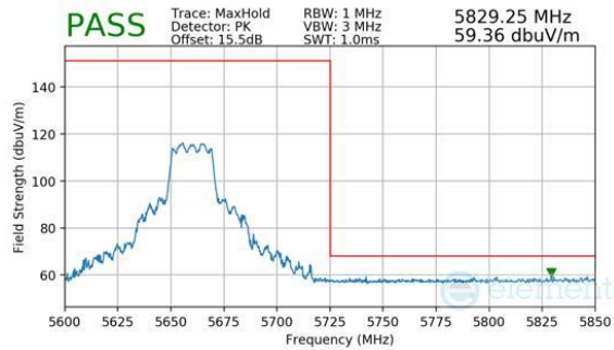
Plot 7-1046. CDD Diversity (Peak, RU242, Index 61, Ch.132, MCS11)
