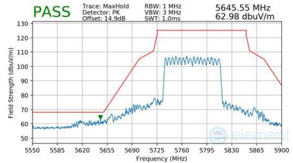
Plot 7-954. CDD Primary (Peak, RU996, Index 67, Ch.155, MCS11)
