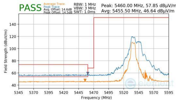
Plot 7-1029. CDD Diversity (Peak & Average, RU52+26, Index 70, Ch.108, MCS11)
