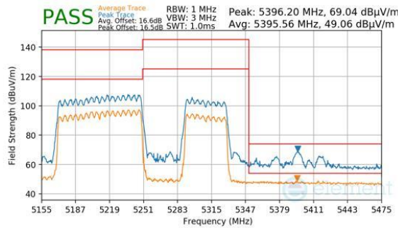
Plot 7-983. CDD Primary (Peak & Average, RU996+484+242, Index 94, Ch.50, MCS11)
