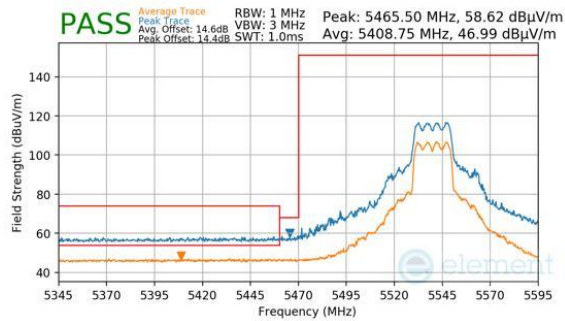
Plot 7-1045. CDD Diversity (Peak & Average, RU242, Index 61, Ch.108, MCS11)
