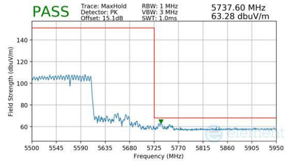
Plot 7-975. CDD Primary (Peak, RU996+484, Index 95 (H), Ch.114 (FCC ONLY), MCS11)
