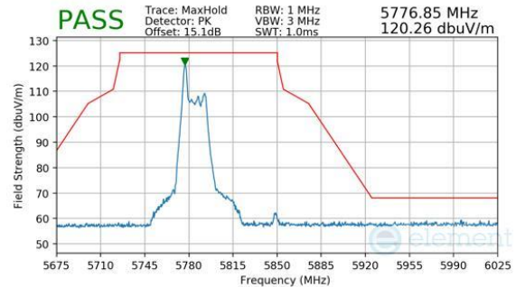
Plot 7-1055. CDD Diversity (Peak, RU26, Index 0, Ch.159, MCS11)
