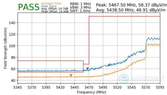
Plot 7-1071. CDD Diversity (Peak & Average, RU484, Index 65, Ch.118 (FCC ONLY), MCS11)
