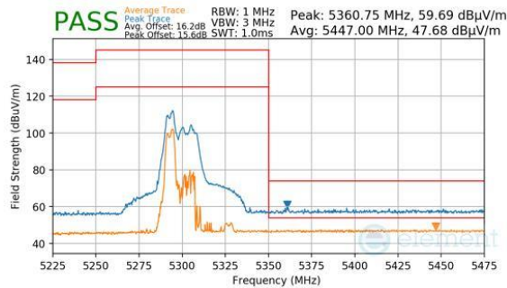
Plot 7-1057. CDD Diversity (Peak & Average, RU52, Index 37, Ch.62, MCS11)
