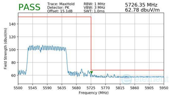
Plot 7-973. CDD Primary (Peak, RU996+484, Index 94 (L), Ch.114 (FCC ONLY), MCS11)
