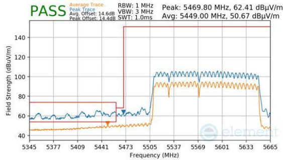
Plot 7-989. CDD Primary (Peak & Average, RU996+484+242, Index 96 (L), Ch.114 (FCC ONLY), MCS11)
