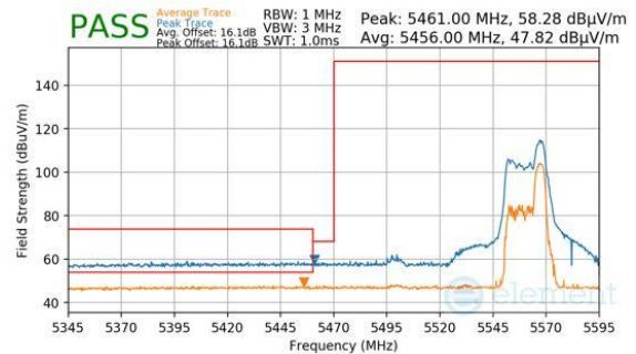
Plot 7-1062. CDD Diversity (Peak & Average, RU52, Index 44, Ch.110, MCS11)
