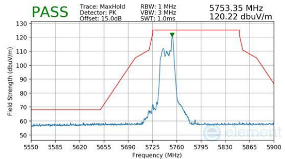
Plot 7-1012. CDD Diversity (Peak, RU26, Index 8, Ch.149, MCS11)
