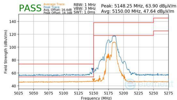
Plot 7-1022. CDD Diversity (Peak & Average, RU52+26, Index 72, Ch.36, MCS11)
