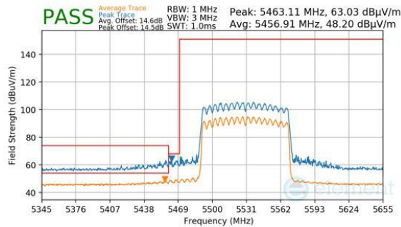
Plot 7-1118. CDD Diversity (Peak & Average, RU996, Index 67, Ch.106, MCS11)
