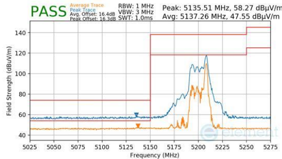
Plot 7-1052. CDD Diversity (Peak & Average, RU26, Index 17, Ch.38, MCS11)
