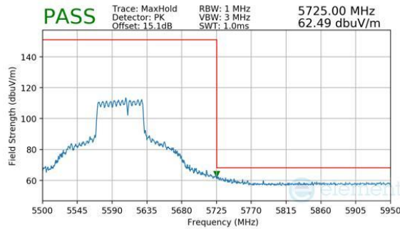
Plot 7-1107. CDD Diversity (Peak, RU484+242, Index 93, Ch.122 (FCC ONLY), MCS11)
