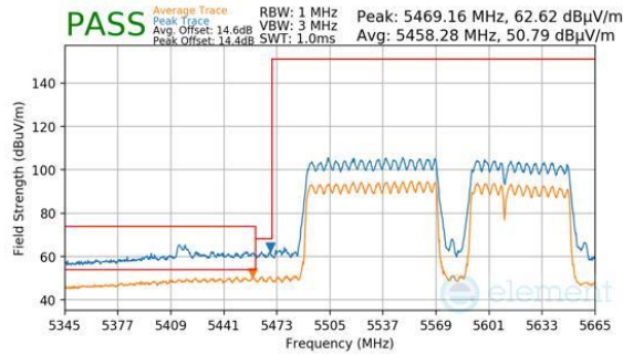
Plot 7-990. CDD Primary (Peak & Average, RU996+484+242, Index 96 (H), Ch.114 (FCC ONLY), MCS11)
