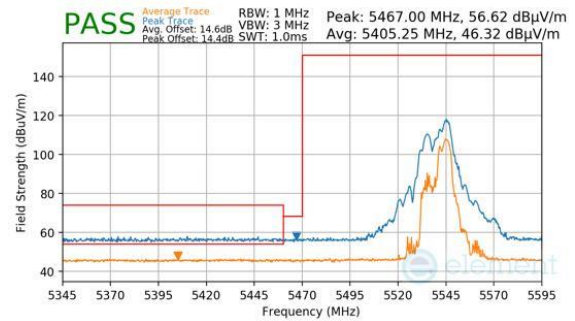
Plot 7-1030. CDD Diversity (Peak & Average, RU52+26, Index 72, Ch.108, MCS11)
