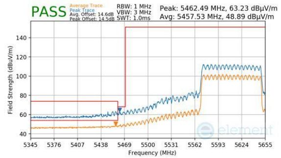
Plot 7-952. CDD Primary (Peak & Average, RU996, Index 67, Ch.122 (FCC ONLY), MCS11)
