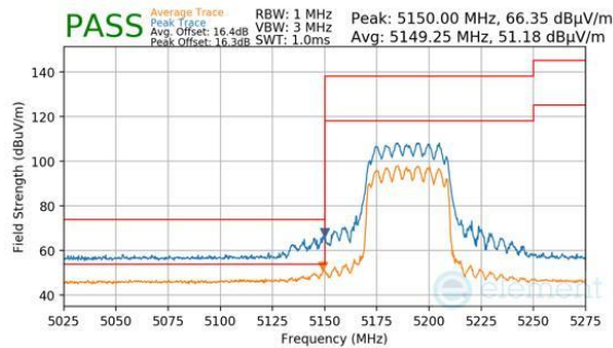
Plot 7-1065. CDD Diversity (Peak & Average, RU484, Index 65, Ch.38, MCS11)
