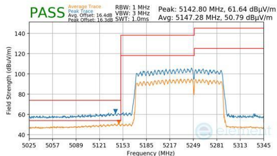
Plot 7-966. CDD Primary (Peak & Average, RU996+484, Index 95, Ch.50, MCS11)
