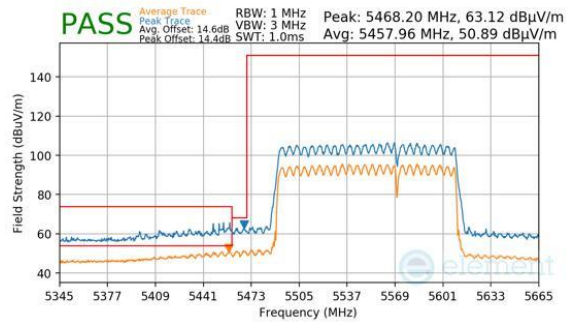
Plot 7-972. CDD Primary (Peak & Average, RU996+484, Index 95 (H), Ch.114 (FCC ONLY), MCS11)
