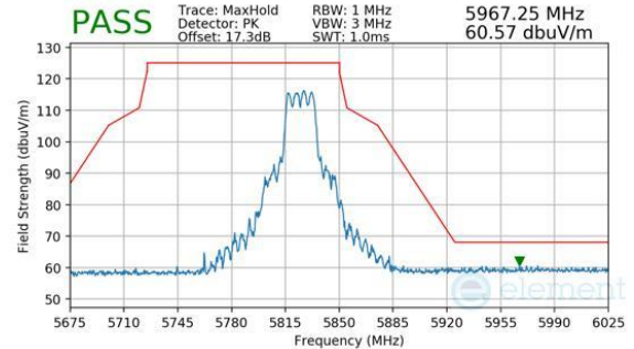
Plot 7-1050. CDD Diversity (Peak, RU242, Index 61, Ch.165, MCS11)
