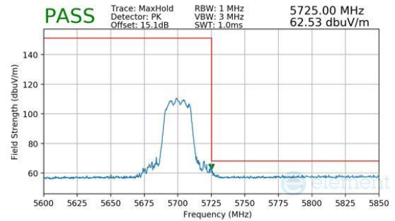
Plot 7-1048. CDD Diversity (Peak, RU242, Index 61, Ch.140, MCS11)
