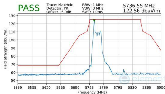
Plot 7-1053. CDD Diversity (Peak, RU26, Index 0, Ch.151, MCS11)
