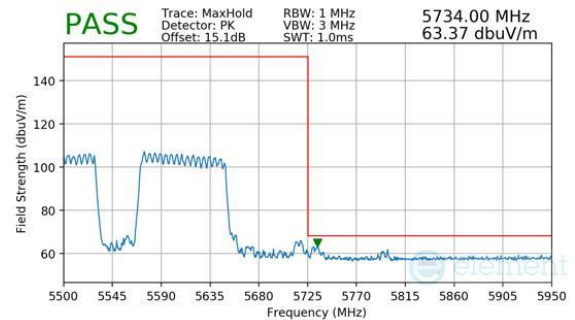
Plot 7-976. CDD Primary (Peak, RU996+484, Index 95 (L), Ch.114 (FCC ONLY), MCS11)
