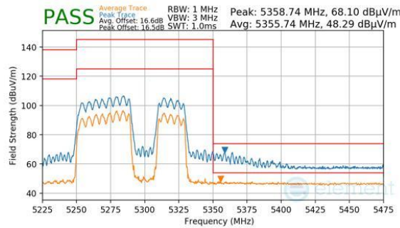
Plot 7-1094. CDD Diversity (Peak & Average, RU484+242, Index 92, Ch.58, MCS11)
