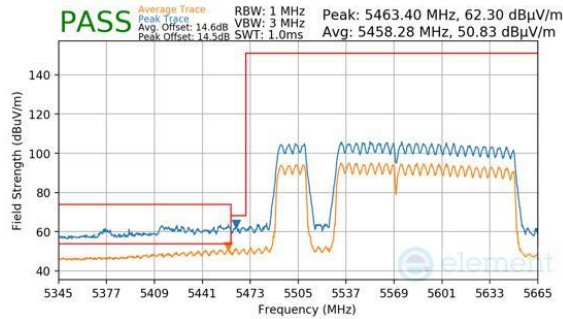
Plot 7-991. CDD Primary (Peak & Average, RU996+484+242, Index 97 (L), Ch.114 (FCC ONLY), MCS11)
