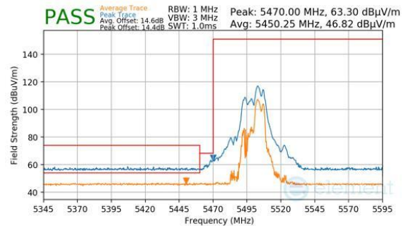
Plot 7-1026. CDD Diversity (Peak & Average, RU52+26, Index 72, Ch.100, MCS11)
