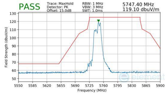
Plot 7-1036. CDD Diversity (Peak, RU52+26, Index 72, Ch.149, MCS11)
