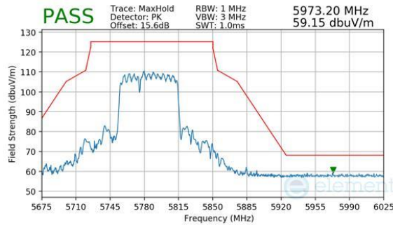
Plot 7-1112. CDD Diversity (Peak, RU484+242, Index 90, Ch.155, MCS11)
