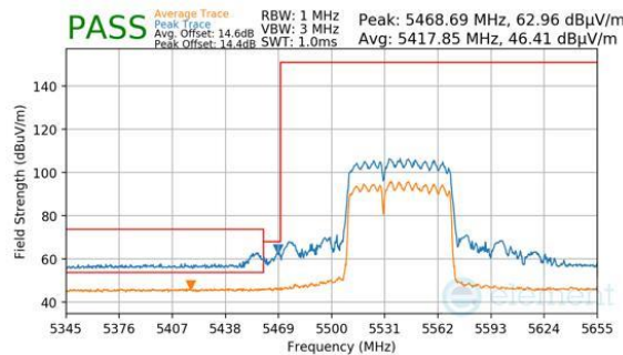
Plot 7-1096. CDD Diversity (Peak & Average, RU484+242, Index 90, Ch.106, MCS11)
