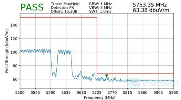
Plot 7-999. CDD Primary (Peak, RU996+484+242, Index 97 (H), Ch.114 (FCC ONLY), MCS11)
