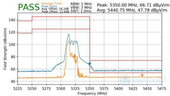
Plot 7-1015. CDD Diversity (Peak & Average, RU52, Index 37, Ch.64, MCS11)
