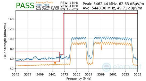
Plot 7-993. CDD Primary (Peak & Average, RU996+484+242, Index 98 (L), Ch.114 (FCC ONLY), MCS11)
