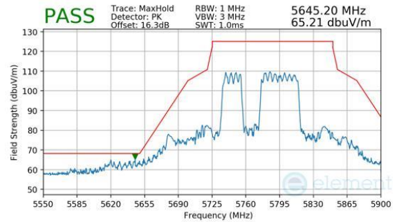
Plot 7-1109. CDD Diversity (Peak, RU484+242, Index 91, Ch.155, MCS11)
