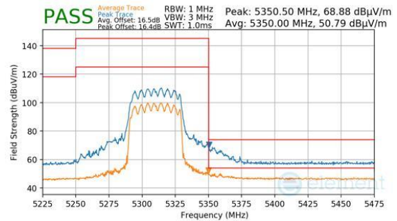
Plot 7-1068. CDD Diversity (Peak & Average, RU484, Index 65, Ch.62, MCS11)
