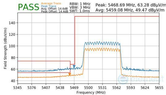
Plot 7-951. CDD Primary (Peak & Average, RU996, Index 67, Ch.106, MCS11)
