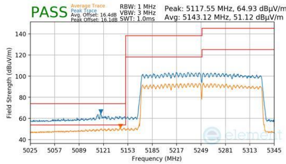
Plot 7-1005. CDD Primary (Peak & Average, RU996X2, Index 68, Ch.50, MCS11)
