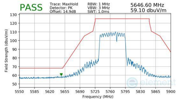
Plot 7-1111. CDD Diversity (Peak, RU484+242, Index 93, Ch.155, MCS11)
