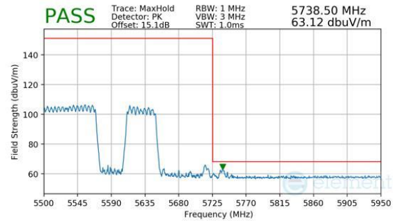
Plot 7-974. CDD Primary (Peak, RU996+484, Index 94 (H), Ch.114 (FCC ONLY), MCS11)
