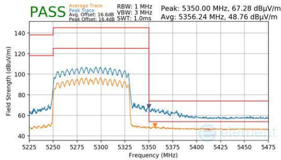
Plot 7-1117. CDD Diversity (Peak & Average, RU996, Index 67, Ch.58, MCS11)
