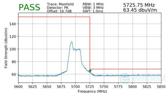
Plot 7-1019. CDD Diversity (Peak, RU52, Index 37, Ch.140, MCS11)
