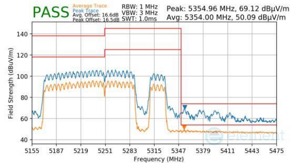
Plot 7-987. CDD Primary (Peak & Average, RU996+484+242, Index 98, Ch.50, MCS11)
