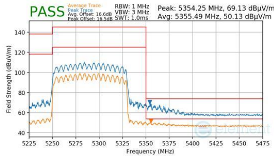
Plot 7-950. CDD Primary (Peak & Average, RU996, Index 67, Ch.58, MCS11)
