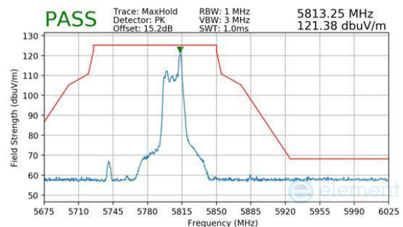
Plot 7-1056. CDD Diversity (Peak, RU26, Index 17, Ch.159, MCS11)
