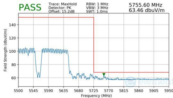
Plot 7-1003. CDD Primary (Peak, RU996+484+242, Index 99 (L), Ch.114 (FCC ONLY), MCS11)
