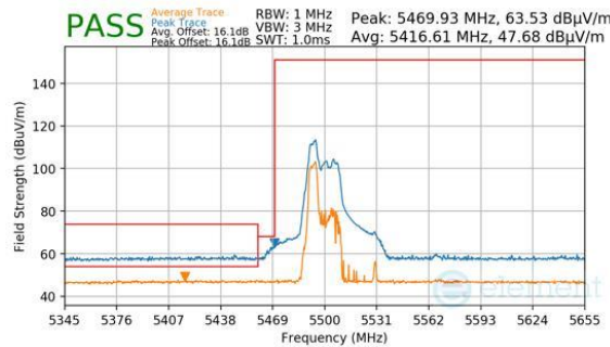
Plot 7-1084. CDD Diversity (Peak & Average, RU52, Index 37, Ch.106, MCS11)
