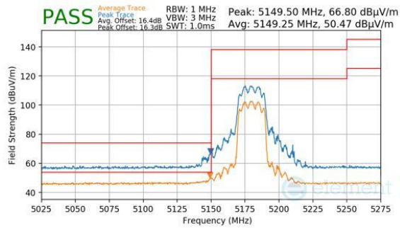
Plot 7-1039. CDD Diversity (Peak & Average, RU242, Index 61, Ch.36, MCS11)
