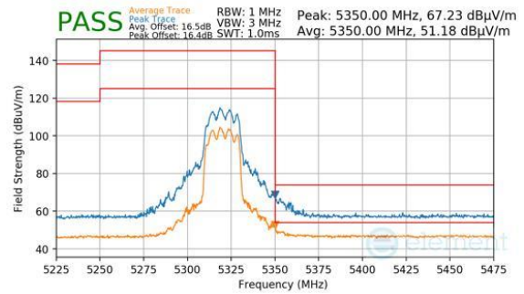
Plot 7-1042. CDD Diversity (Peak & Average, RU242, Index 61, Ch.64, MCS11)
