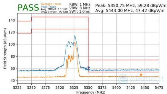
Plot 7-1016. CDD Diversity (Peak & Average, RU52, Index 40, Ch.64, MCS11)
