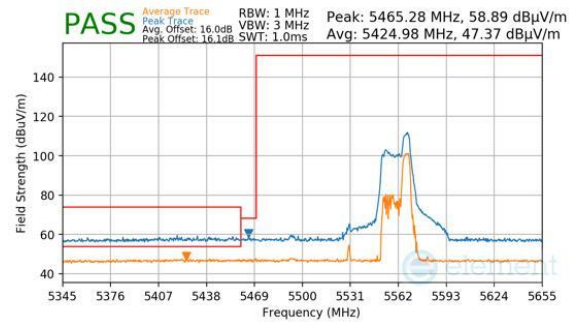
Plot 7-1085. CDD Diversity (Peak & Average, RU52, Index 52, Ch.106, MCS11)
