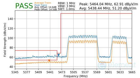
Plot 7-970. CDD Primary (Peak & Average, RU996+484, Index 94 (H), Ch.114 (FCC ONLY), MCS11)
