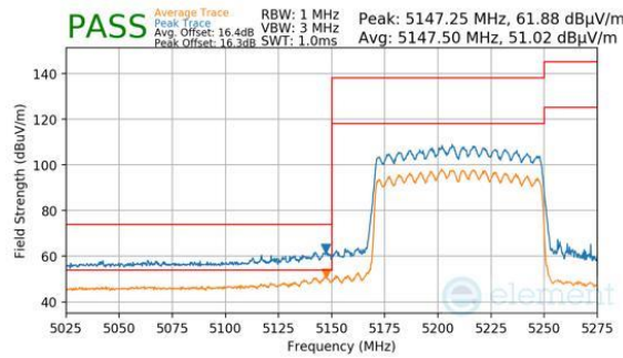
Plot 7-949. CDD Primary (Peak & Average, RU996, Index 67, Ch.42, MCS11)
