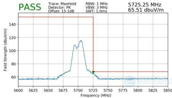
Plot 7-1034. CDD Diversity (Peak, RU52+26, Index 72, Ch.140, MCS11)
