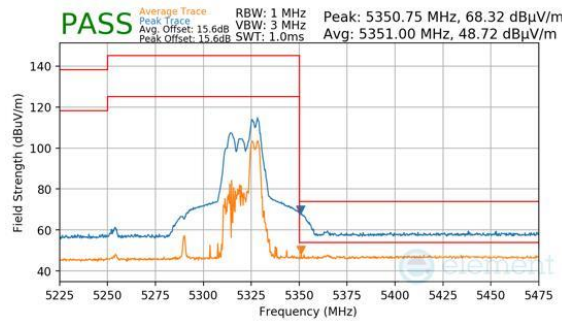
Plot 7-1083. CDD Diversity (Peak & Average, RU52, Index 52, Ch.58, MCS11)
