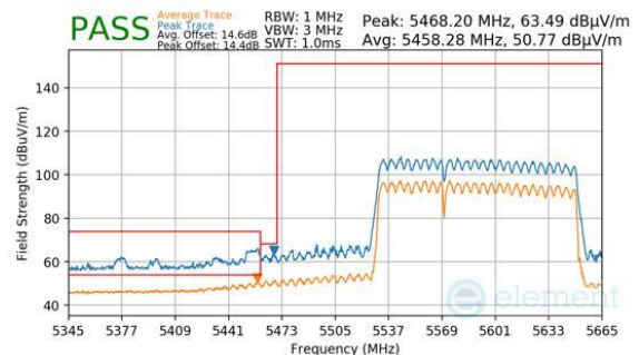
Plot 7-969. CDD Primary (Peak & Average, RU996+484, Index 94 (L), Ch.114 (FCC ONLY), MCS11)
