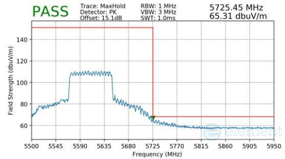
Plot 7-1120. CDD Diversity (Peak, RU996, Index 67, Ch.122 (FCC ONLY), MCS11)
