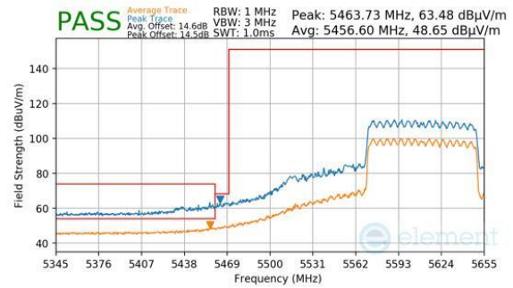
Plot 7-1119. CDD Diversity (Peak & Average, RU996, Index 67, Ch.122 (FCC ONLY), MCS11)
