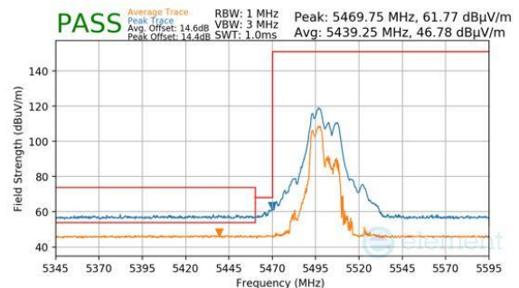
Plot 7-1025. CDD Diversity (Peak & Average, RU52+26, Index 70, Ch.100, MCS11)
