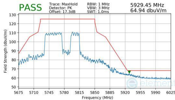
Plot 7-1114. CDD Diversity (Peak, RU484+242, Index 92, Ch.155, MCS11)
