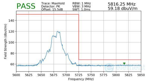
Plot 7-1032. CDD Diversity (Peak, RU52+26, Index 72, Ch.136, MCS11)
