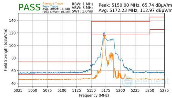
Plot 7-1051. CDD Diversity (Peak & Average, RU26, Index 0, Ch.38, MCS11)
