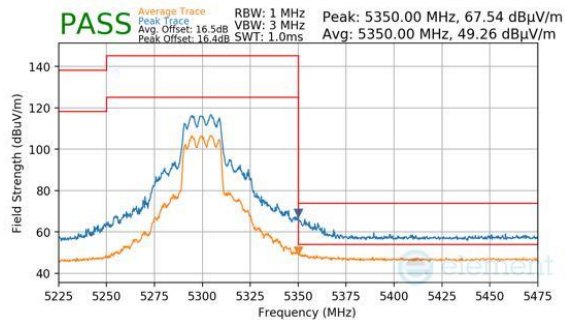
Plot 7-1041. CDD Diversity (Peak & Average, RU242, Index 61, Ch.60, MCS11)
