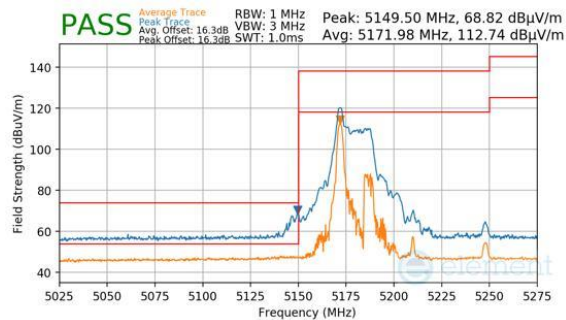
Plot 7-1076. CDD Diversity (Peak & Average, RU26, Index 0, Ch.42, MCS11)
