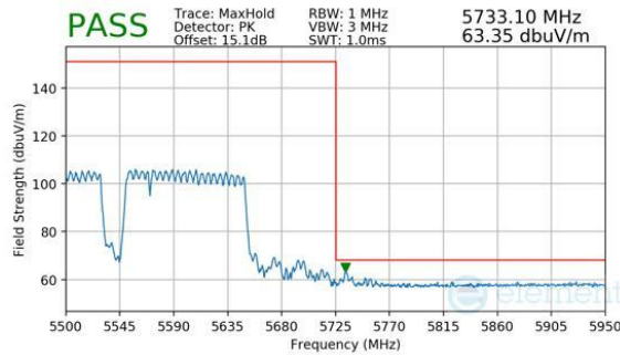
Plot 7-1001. CDD Primary (Peak, RU996+484+242, Index 98 (L), Ch.114 (FCC ONLY), MCS11)
