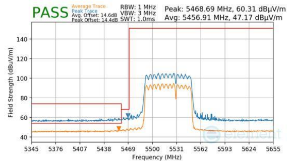
Plot 7-1099. CDD Diversity (Peak & Average, RU484+242, Index 93, Ch.106, MCS11)
