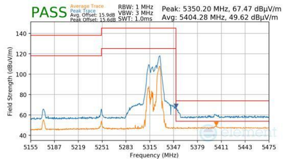
Plot 7-959. CDD Primary (Peak & Average, RU52, Index 52 (H), Ch.50, MCS11)
