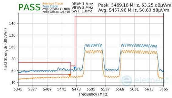
Plot 7-971. CDD Primary (Peak & Average, RU996+484, Index 95 (L), Ch.114 (FCC ONLY), MCS11)
