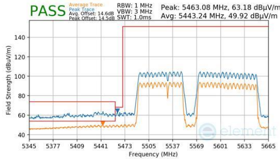
Plot 7-995. CDD Primary (Peak & Average, RU996+484+242, Index 99 (L), Ch.114 (FCC ONLY), MCS11)
