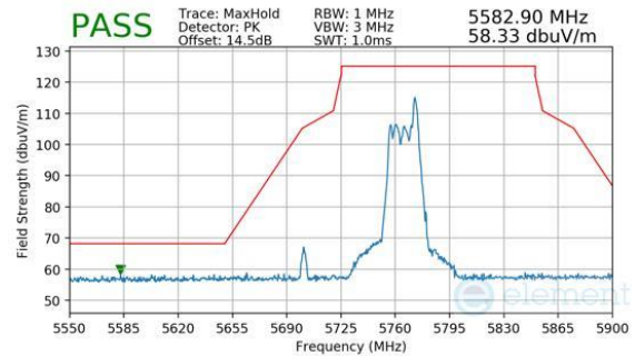
Plot 7-1054. CDD Diversity (Peak, RU26, Index 17, Ch.151, MCS11)
