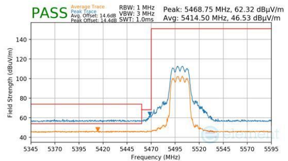
Plot 7-1043. CDD Diversity (Peak & Average, RU242, Index 61, Ch.100, MCS11)
