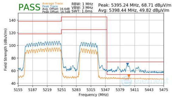
Plot 7-967. CDD Primary (Peak & Average, RU996+484, Index 94, Ch.50, MCS11)
