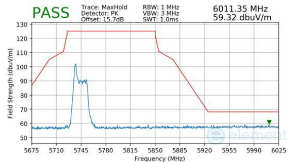
Plot 7-1080. CDD Diversity (Peak, RU26, Index 0, Ch.155, MCS11)
