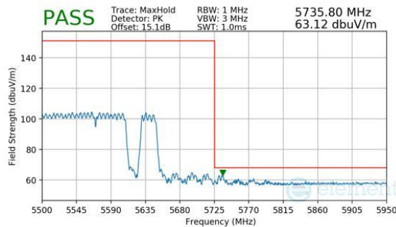
Plot 7-1002. CDD Primary (Peak, RU996+484+242, Index 98 (H), Ch.114 (FCC ONLY), MCS11)
