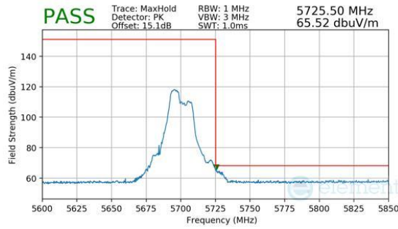
Plot 7-1033. CDD Diversity (Peak, RU52+26, Index 70, Ch.140, MCS2)
