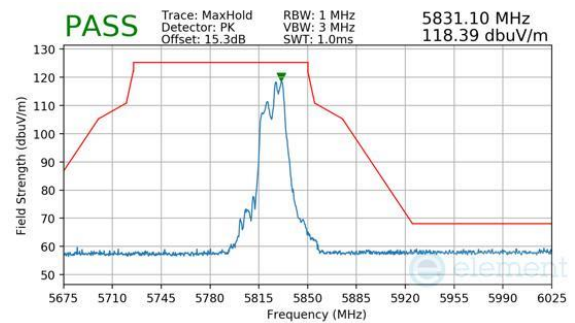
Plot 7-1038. CDD Diversity (Peak, RU52+26, Index 72, Ch.165, MCS11)
