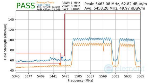
Plot 7-992. CDD Primary (Peak & Average, RU996+484+242, Index 97 (H), Ch.114 (FCC ONLY), MCS11)
