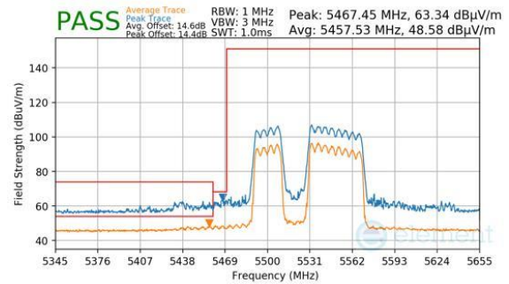
Plot 7-1097. CDD Diversity (Peak & Average, RU484+242, Index 91, Ch.106, MCS11)
