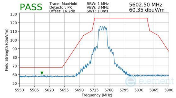
Plot 7-1049. CDD Diversity (Peak, RU242, Index 61, Ch.149, MCS11)
