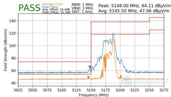
Plot 7-1010. CDD Diversity (Peak & Average, RU26, Index 8, Ch.36, MCS11)
