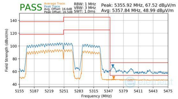
Plot 7-986. CDD Primary (Peak & Average, RU996+484+242, Index 97, Ch.50, MCS11)
