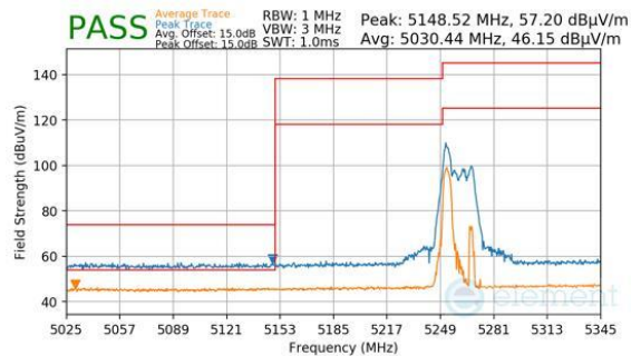
Plot 7-956. CDD Primary (Peak & Average, RU52, Index 37, Ch.50, MCS11)
