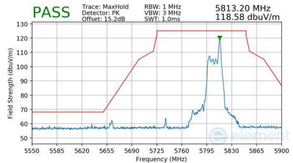
Plot 7-1079. CDD Diversity (Peak, RU26, Index 36, Ch.155, MCS11)
