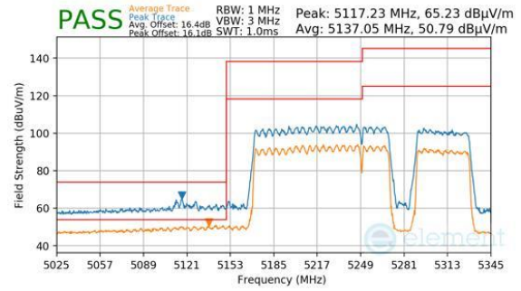
Plot 7-980. CDD Primary (Peak & Average, RU996+484+242, Index 97, Ch.50, MCS11)
