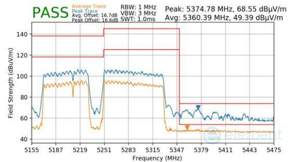
Plot 7-988. CDD Primary (Peak & Average, RU996+484+242, Index 99, Ch.50, MCS11)
