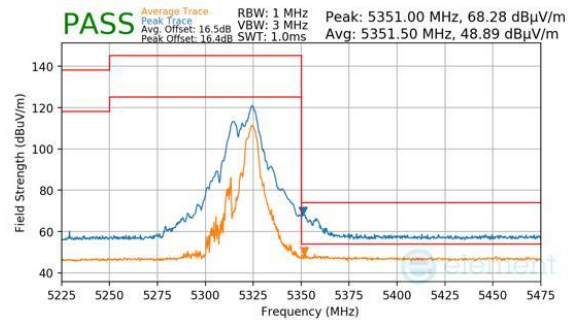
Plot 7-1024. CDD Diversity (Peak & Average, RU52+26, Index 72, Ch.64, MCS11)
