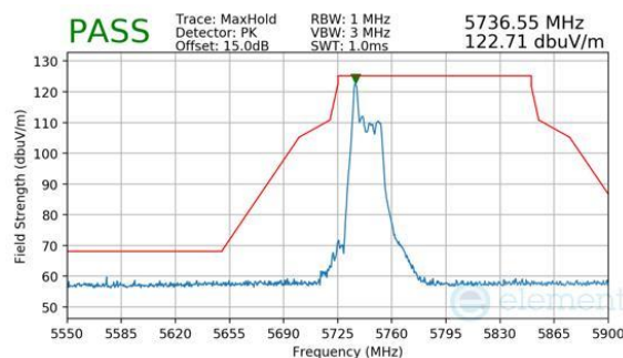
Plot 7-1011. CDD Diversity (Peak, RU26, Index 0, Ch.149, MCS11)
