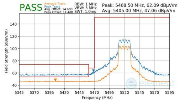
Plot 7-1044. CDD Diversity (Peak & Average, RU242, Index 61, Ch.104, MCS11)
