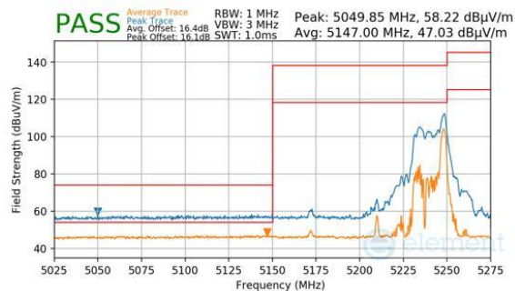
Plot 7-1077. CDD Diversity (Peak & Average, RU26, Index 36, Ch.42, MCS11)
