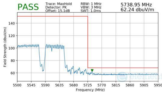
Plot 7-997. CDD Primary (Peak, RU996+484+242, Index 96 (H), Ch.114 (FCC ONLY), MCS11)
