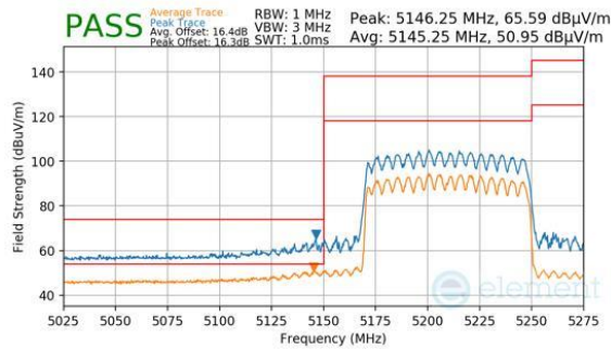
Plot 7-1116. CDD Diversity (Peak & Average, RU996, Index 67, Ch.42, MCS11)
