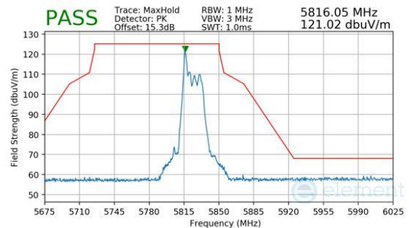
Plot 7-1013. CDD Diversity (Peak, RU26, Index 0, Ch.165, MCS11)
