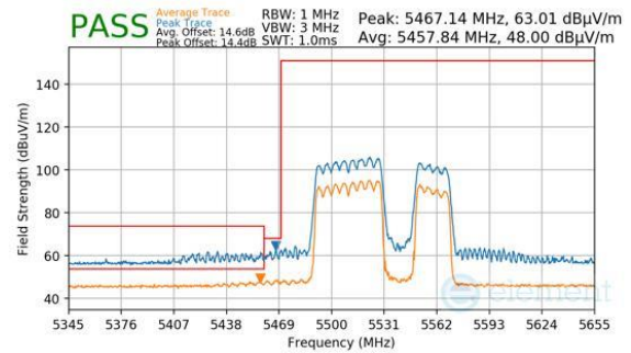
Plot 7-1098. CDD Diversity (Peak & Average, RU484+242, Index 92, Ch.106, MCS11)
