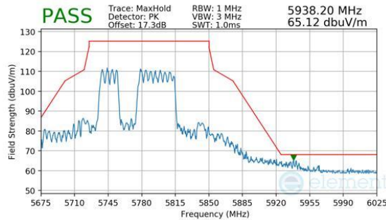
Plot 7-946. CDD Primary (Peak, RU484+242, Index 91, Ch.155, MCS11)
