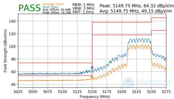
Plot 7-1066. CDD Diversity (Peak & Average, RU484, Index 65, Ch.46, MCS11)
