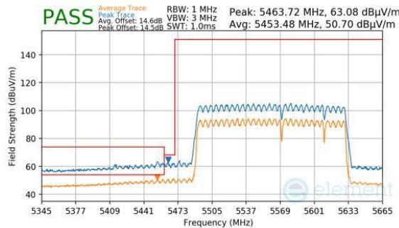
Plot 7-996. CDD Primary (Peak & Average, RU996+484+242, Index 99 (H), Ch.114 (FCC ONLY), MCS11)
