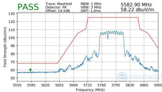
Plot 7-1108. CDD Diversity (Peak, RU484+242, Index 90, Ch.155, MCS11)
