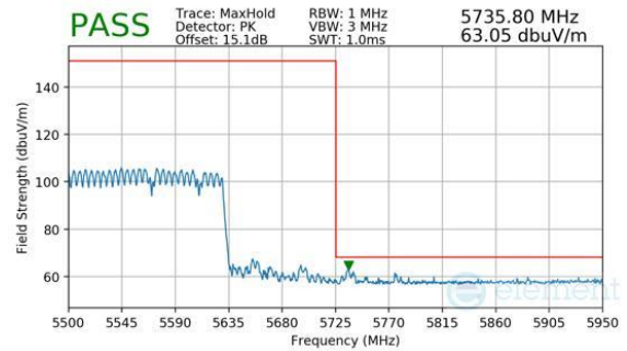
Plot 7-1004. CDD Primary (Peak, RU996+484+242, Index 99 (H), Ch.114 (FCC ONLY), MCS11)
