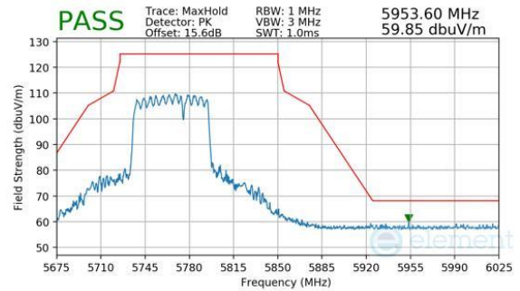
Plot 7-1115. CDD Diversity (Peak, RU484+242, Index 93, Ch.155, MCS11)
