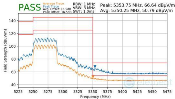
Plot 7-1067. CDD Diversity (Peak & Average, RU484, Index 65, Ch.54, MCS11)
