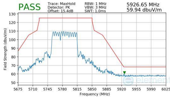
Plot 7-945. CDD Primary (Peak, RU484+242, Index 90, Ch.155, MCS11)
