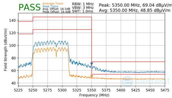
Plot 7-1095. CDD Diversity (Peak & Average, RU484+242, Index 93, Ch.58, MCS11)
