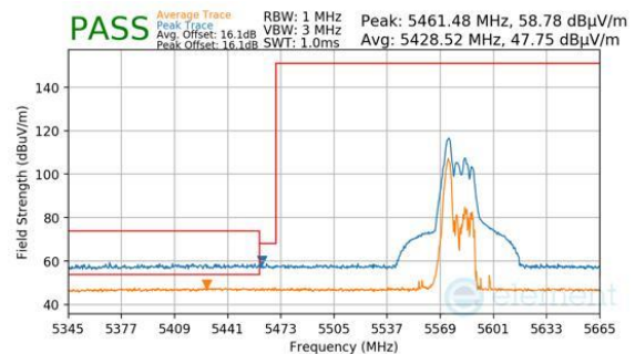
Plot 7-960. CDD Primary (Peak & Average, RU52, Index 37, Ch.114 (FCC ONLY), MCS11)
