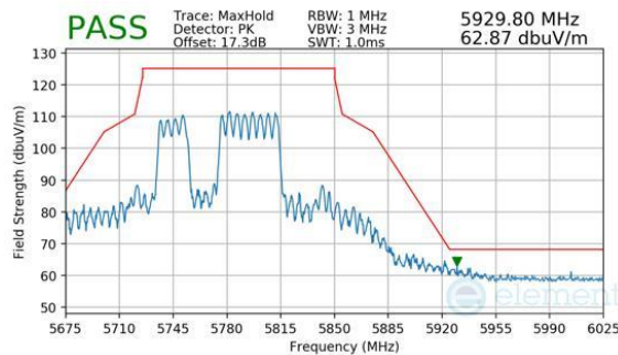
Plot 7-1113. CDD Diversity (Peak, RU484+242, Index 91, Ch.155, MCS11)
