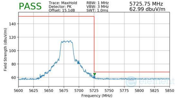
Plot 7-1047. CDD Diversity (Peak, RU242, Index 61, Ch.136, MCS11)
