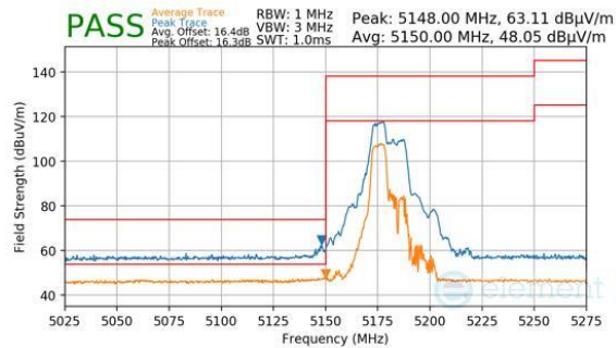
Plot 7-1021. CDD Diversity (Peak & Average, RU52+26, Index 70, Ch.36, MCS11)
