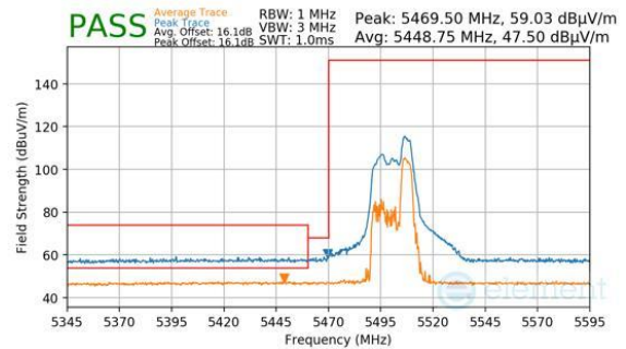
Plot 7-1018. CDD Diversity (Peak & Average, RU52, Index 40, Ch.100, MCS11)
