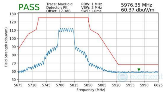
Plot 7-1075. CDD Diversity (Peak, RU484, Index 65, Ch.159, MCS11)
