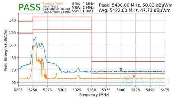
Plot 7-1082. CDD Diversity (Peak & Average, RU52, Index 37, Ch.58, MCS11)
