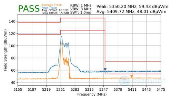
Plot 7-958. CDD Primary (Peak & Average, RU52, Index 37, Ch.50, MCS11)
