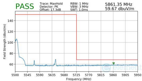
Plot 7-963. CDD Primary (Peak, RU52, Index 37, Ch.114 (FCC ONLY), MCS11)
