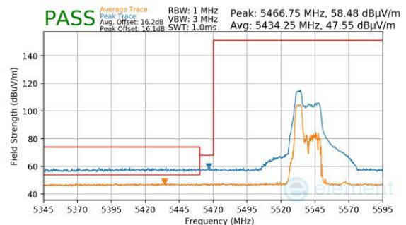
Plot 7-1061. CDD Diversity (Peak & Average, RU52, Index 37, Ch.110, MCS11)
