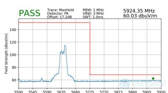
Plot 7-1087. CDD Diversity (Peak, RU52, Index 52, Ch.122 (FCC ONLY), MCS11)
