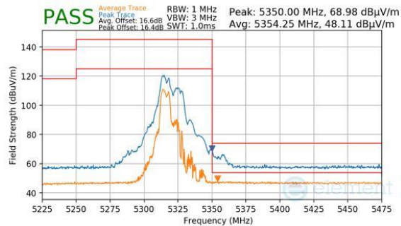
Plot 7-1023. CDD Diversity (Peak & Average, RU52+26, Index 70, Ch.64, MCS11)
