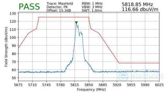
Plot 7-1037. CDD Diversity (Peak, RU52+26, Index 70, Ch.165, MCS11)
