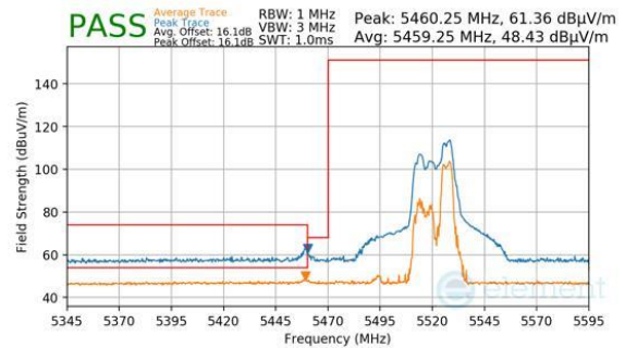
Plot 7-1060. CDD Diversity (Peak & Average, RU52, Index 44, Ch.102, MCS11)
