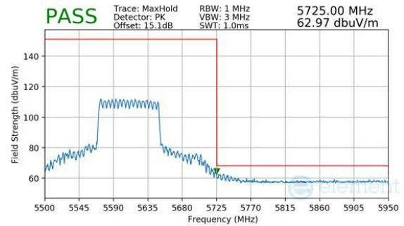
Plot 7-953. CDD Primary (Peak, RU996, Index 67, Ch.122 (FCC ONLY), MCS11)
