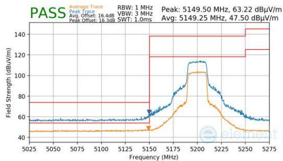
Plot 7-1040. CDD Diversity (Peak & Average, RU242, Index 61, Ch.40, MCS11)
