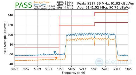
Plot 7-982. CDD Primary (Peak & Average, RU996+484+242, Index 99, Ch.50, MCS11)
