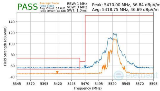
Plot 7-1028. CDD Diversity (Peak & Average, RU52+26, Index 72, Ch.104, MCS11)
