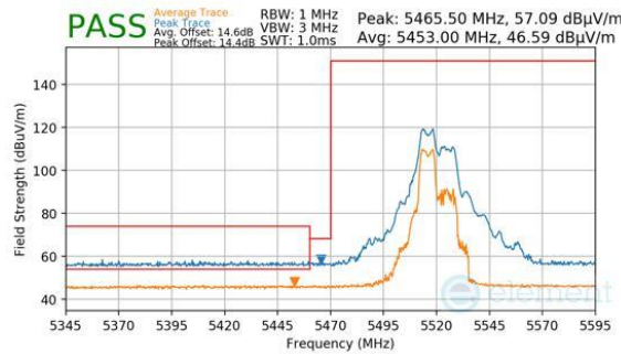
Plot 7-1027. CDD Diversity (Peak & Average, RU52+26, Index 70, Ch.104, MCS11)
