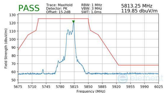
Plot 7-1081. CDD Diversity (Peak, RU26, Index 36, Ch.155, MCS11)
