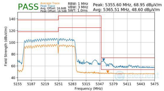
Plot 7-968. CDD Primary (Peak & Average, RU996+484, Index 95, Ch.50, MCS11)
