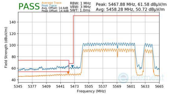
Plot 7-994. CDD Primary (Peak & Average, RU996+484+242, Index 98 (H), Ch.114 (FCC ONLY), MCS11)
