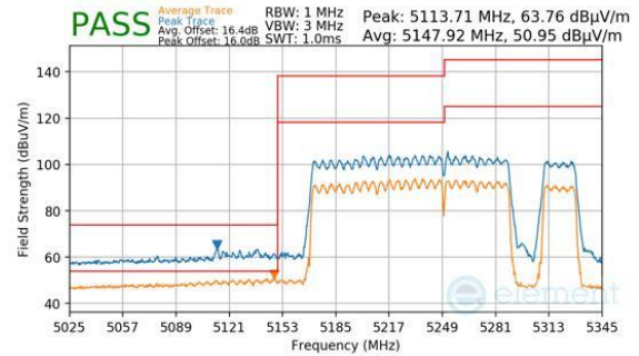
Plot 7-981. CDD Primary (Peak & Average, RU996+484+242, Index 98, Ch.50, MCS11)
