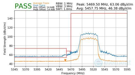
Plot 7-1069. CDD Diversity (Peak & Average, RU484, Index 65, Ch.102, MCS11)
