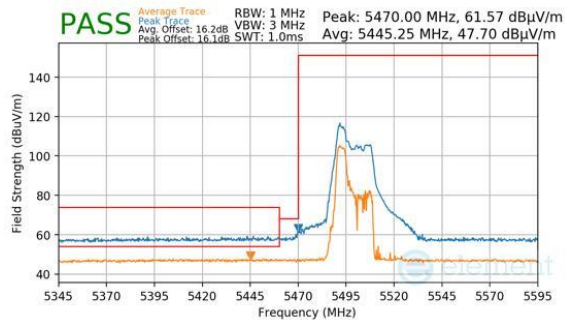
Plot 7-1017. CDD Diversity (Peak & Average, RU52, Index 37, Ch.100, MCS11)
