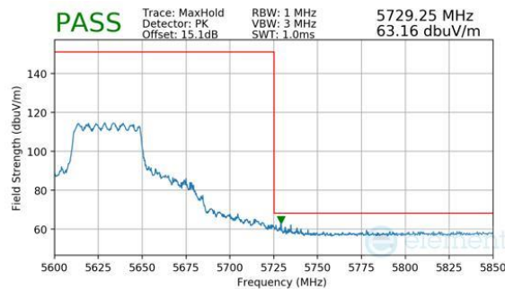
Plot 7-1072. CDD Diversity (Peak, RU484, Index 65, Ch.126 (FCC ONLY), MCS11)
