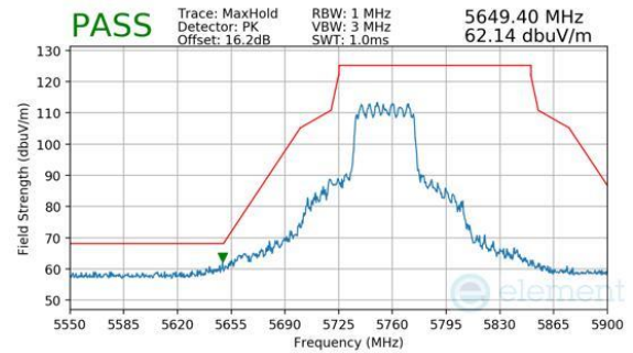
Plot 7-1074. CDD Diversity (Peak, RU484, Index 65, Ch.151, MCS11)
