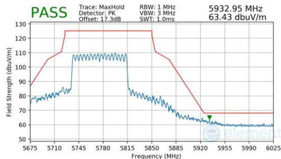
Plot 7-955. CDD Primary (Peak, RU996, Index 67, Ch.155, MCS11)
