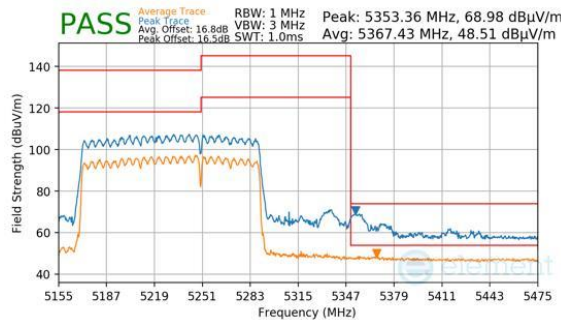
Plot 7-984. CDD Primary (Peak & Average, RU996+484+242, Index 95, Ch.50, MCS11)
