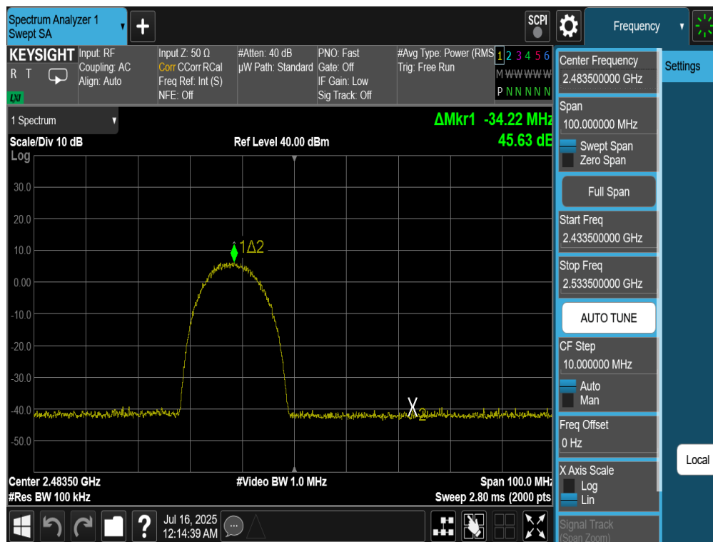
Plot 7-28. Band Edge Plot Antenna 4a (802.11b – Ch. 13)
