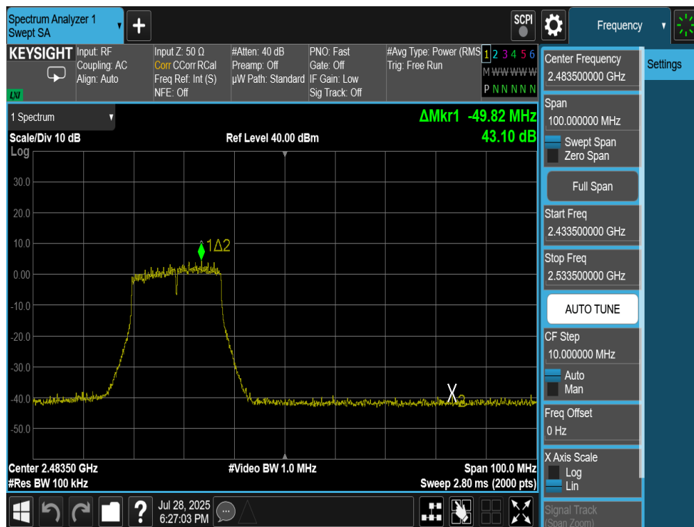
Plot 7-40. Band Edge Plot Antenna 4a (802.11g – Ch. 11)
