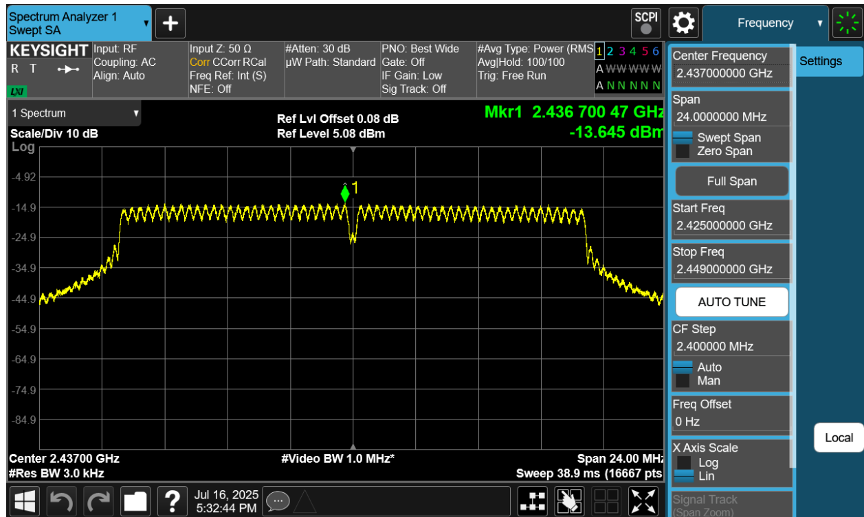
Plot 7-23 PSD CDD Antenna 2a (20MHz BW 802.11n - Ch.6)
