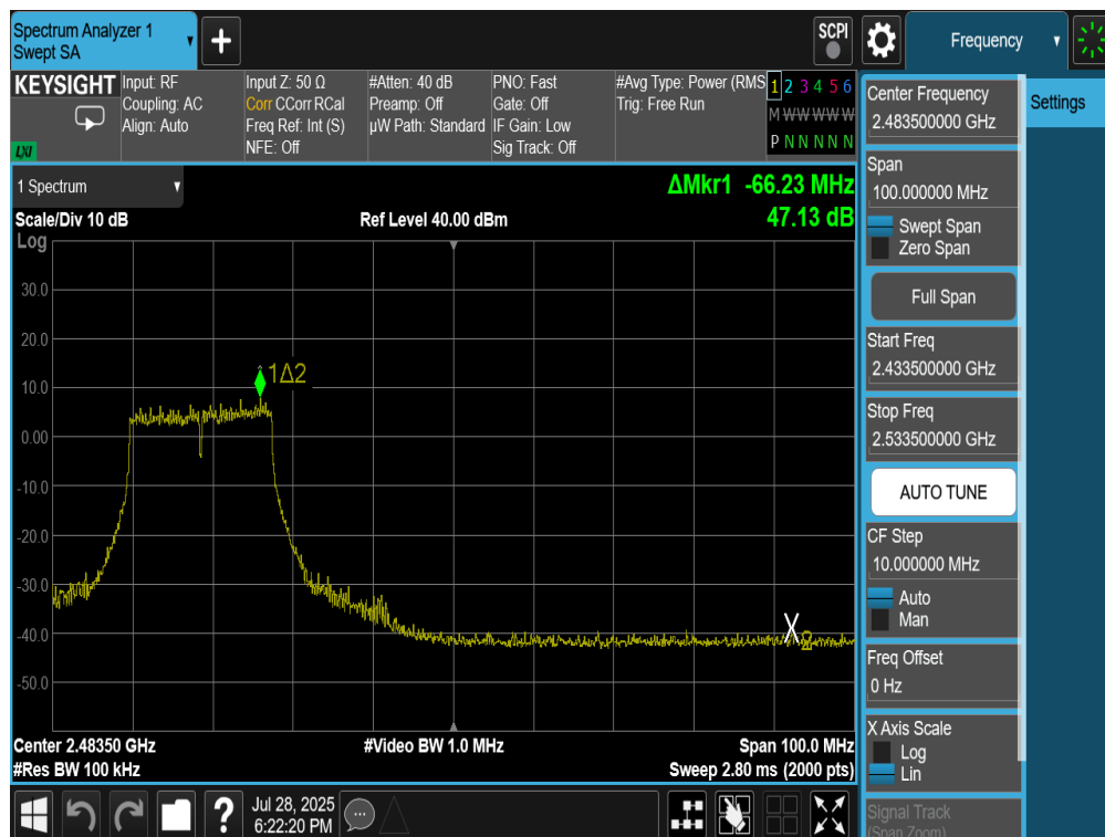
Plot 7-38. Band Edge Plot Antenna 4a (802.11g – Ch. 9)
