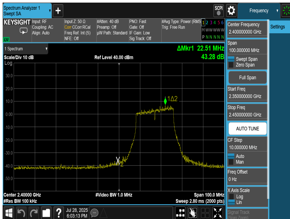
Plot 7-30. Band Edge Plot Antenna 4a (802.11g – Ch. 2)
