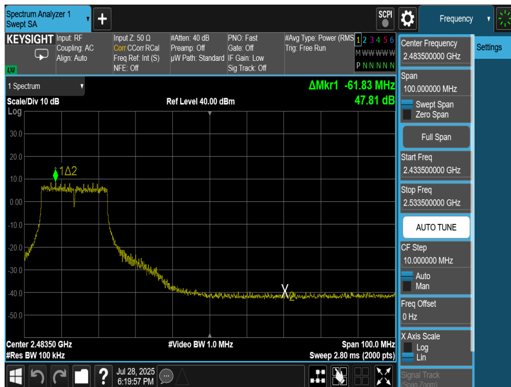
Plot 7-37. Band Edge Plot Antenna 4a (802.11g – Ch. 8)
