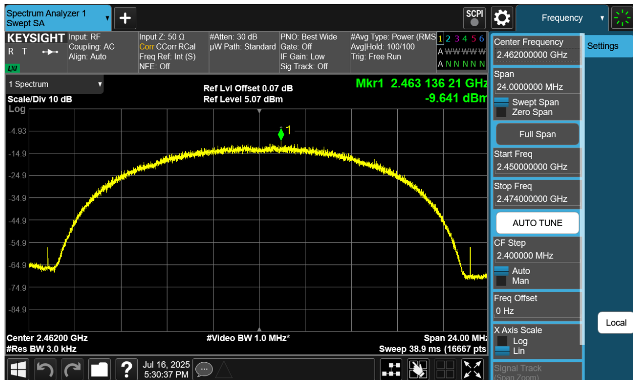
Plot 7-21 PSD CDD Antenna 2a (20MHz BW 802.11b - Ch.11)
