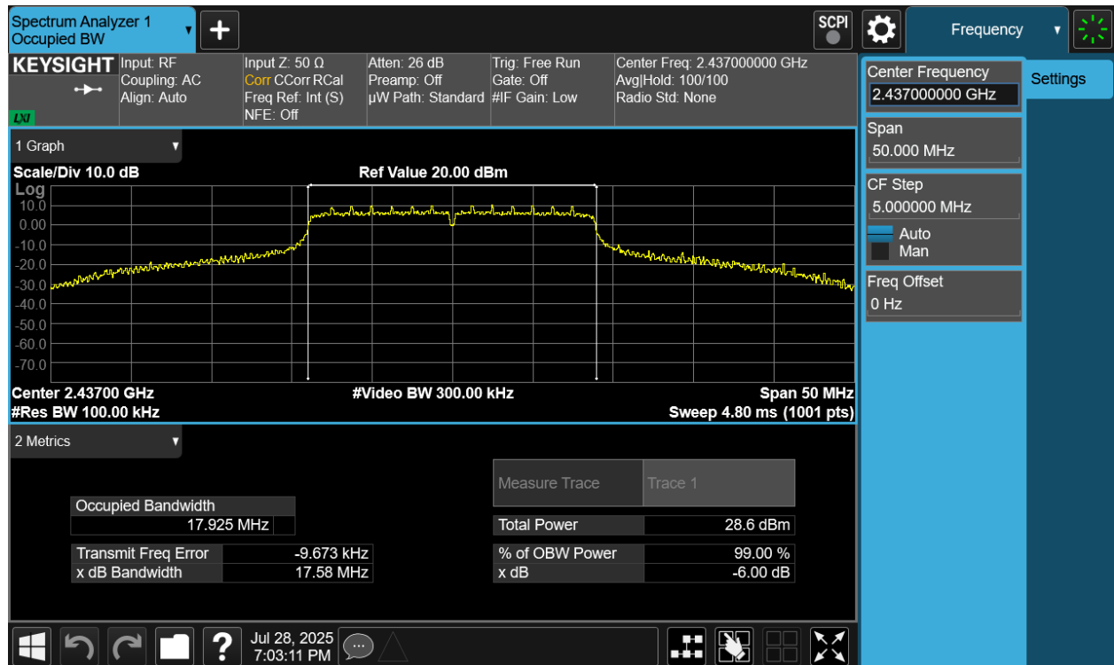
Plot 7-6 6dB BW & 99% OBW Antenna 2a (20MHz BW 802.11g - Ch.6)
