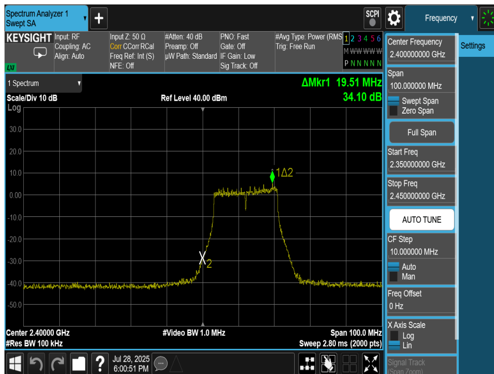
Plot 7-29. Band Edge Plot Antenna 4a (802.11g – Ch. 1)
