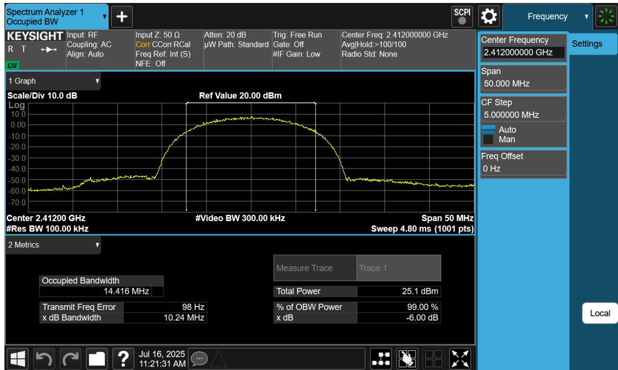
Plot 7-5 6dB BW & 99% OBW Antenna 2a (20MHz BW 802.11b - Ch.1)
