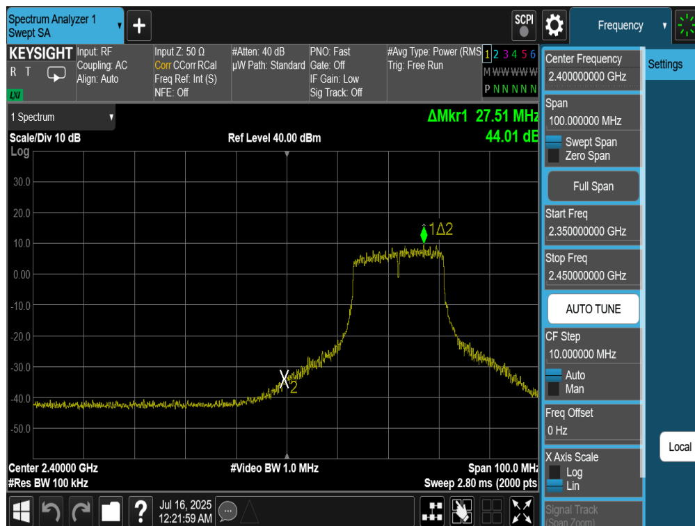
Plot 7-45. Band Edge Plot Antenna 4a (802.11n (2.4GHz) – Ch. 3)
