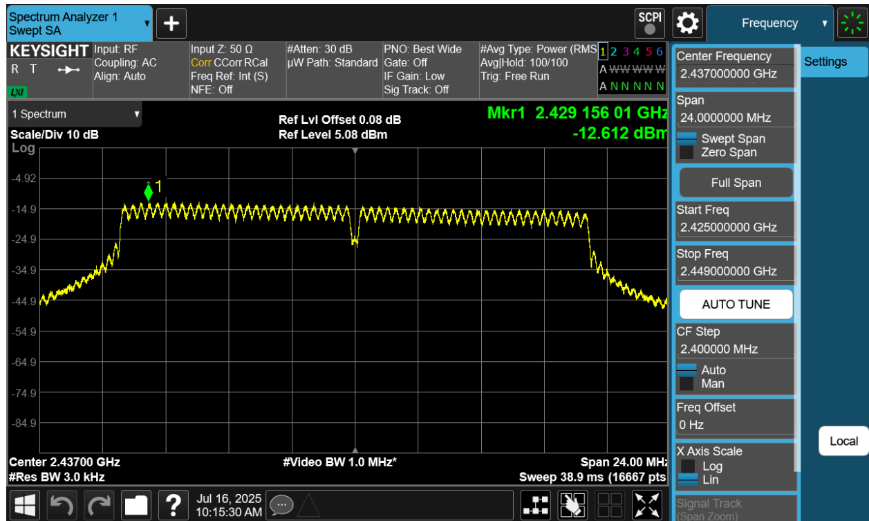
Plot 7-19 PSD CDD Antenna 4a (20MHz BW 802.11n - Ch.6)
