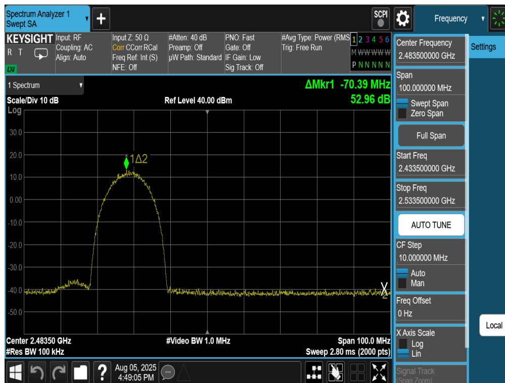
Plot 7-26. Band Edge Plot Antenna 4a (802.11b – Ch. 11)
