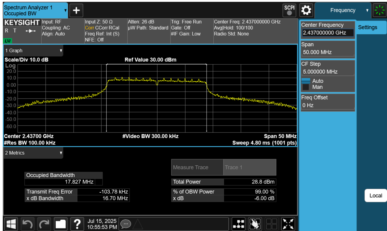
Plot 7-3 6dB BW & 99% OBW Antenna 4a (20MHz BW 802.11n - Ch.6)
