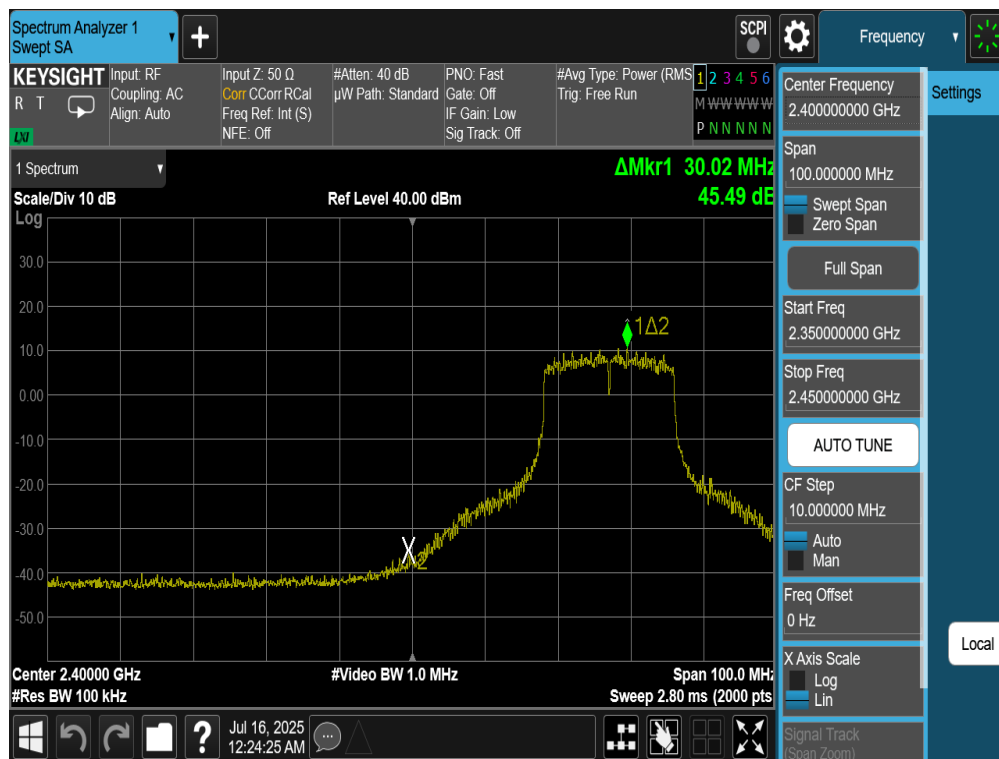
Plot 7-46. Band Edge Plot Antenna 4a (802.11n – Ch. 4)
