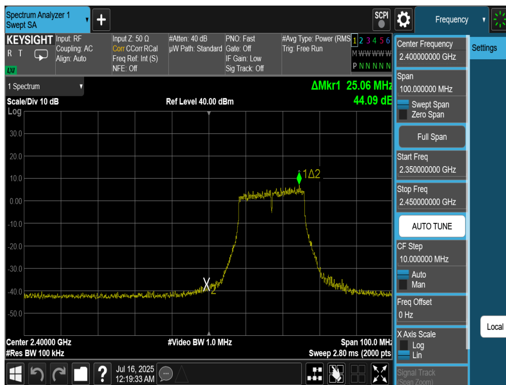
Plot 7-44. Band Edge Plot Antenna 4a (802.11n (2.4GHz) – Ch. 2)
