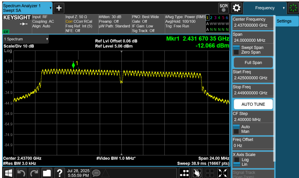
Plot 7-10 PSD Antenna 4a (20MHz BW 802.11g - Ch.6)
