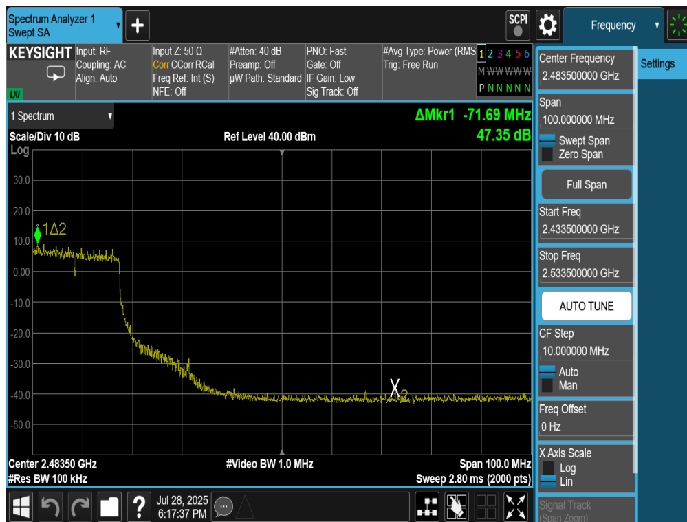
Plot 7-36. Band Edge Plot Antenna 4a (802.11g – Ch. 7)
