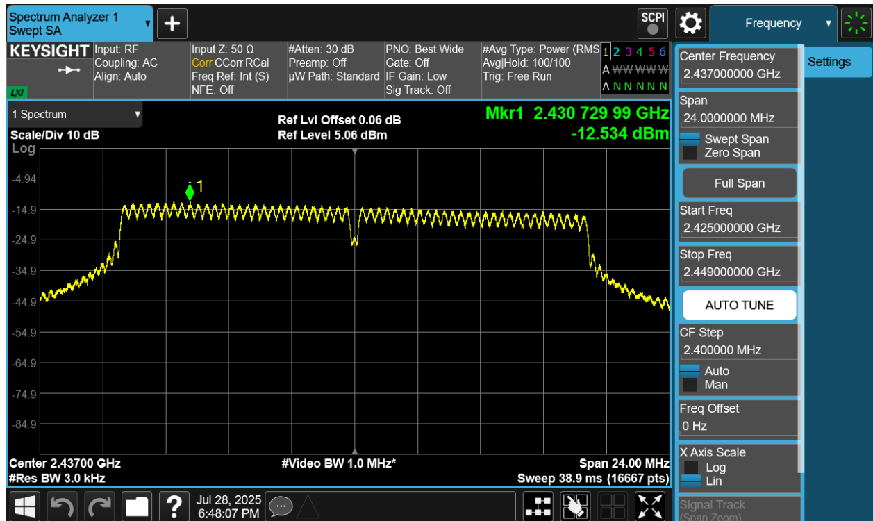
Plot 7-18 PSD CDD Antenna 4a (20MHz BW 802.11g - Ch.6)
