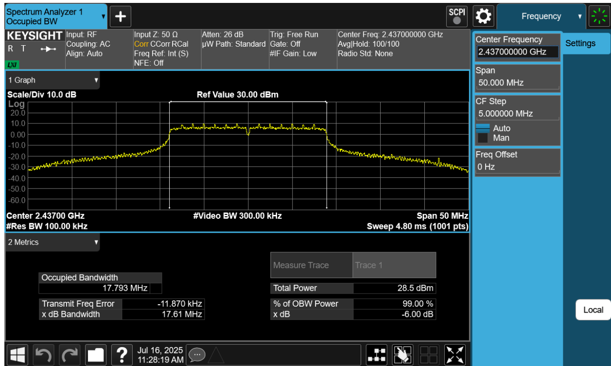
Plot 7-7 6dB BW & 99% OBW Antenna 2a (20MHz BW 802.11n - Ch.6)
