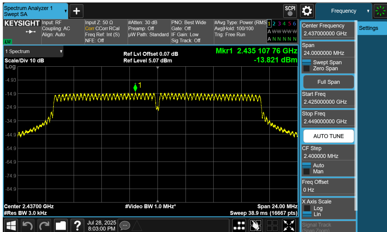
Plot 7-22 PSD CDD Antenna 2a (20MHz BW 802.11g - Ch.6)
