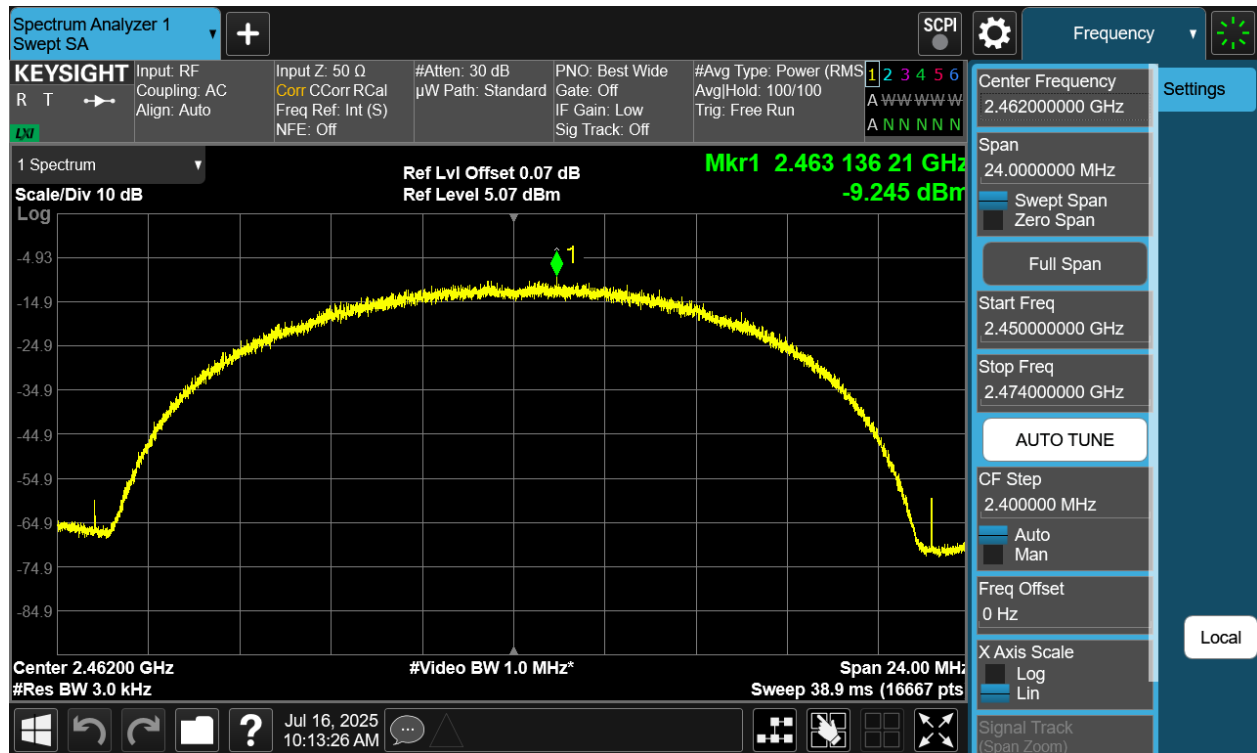
Plot 7-17 PSD CDD Antenna 4a (20MHz BW 802.11b - Ch.11)
