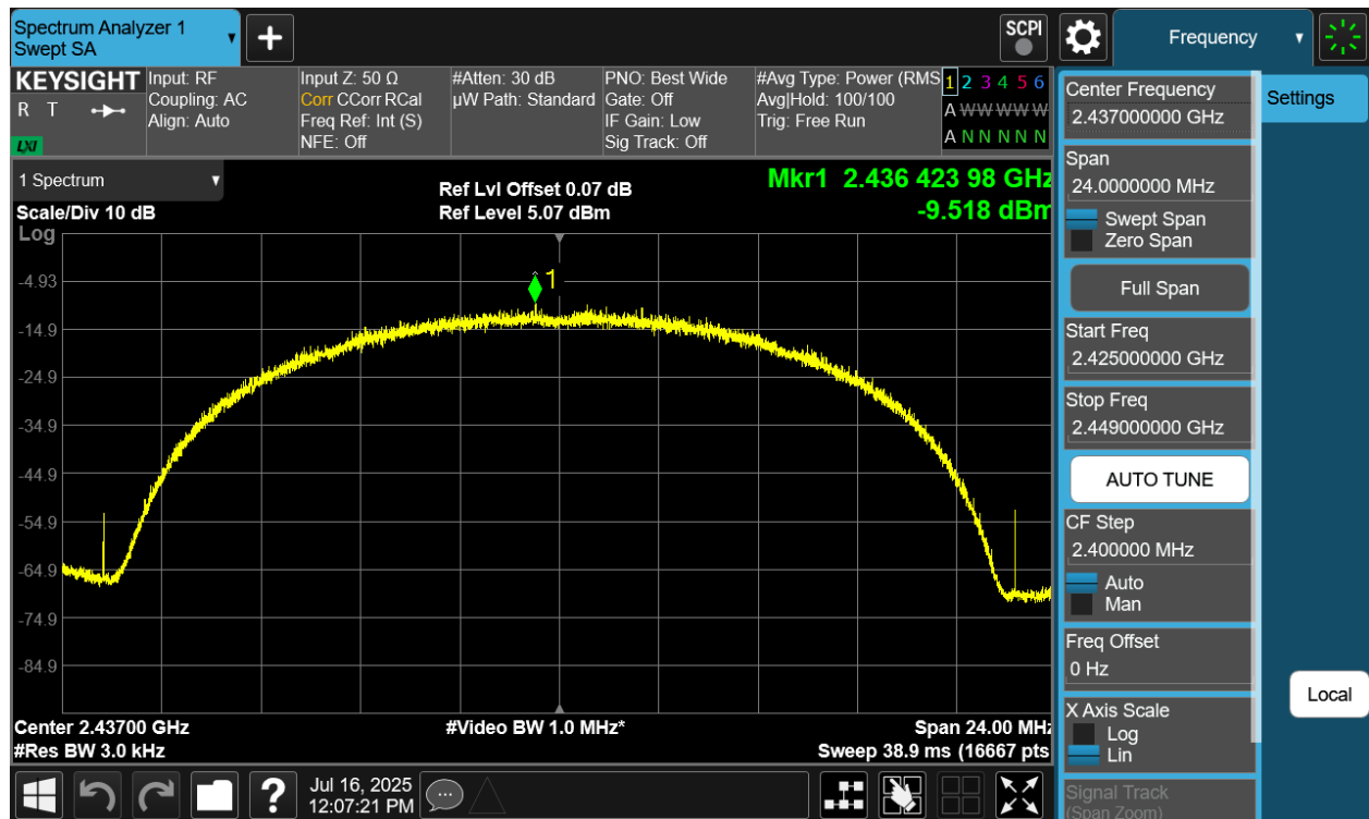
Plot 7-13 PSD Antenna 2a (20MHz BW 802.11b - Ch.6)
