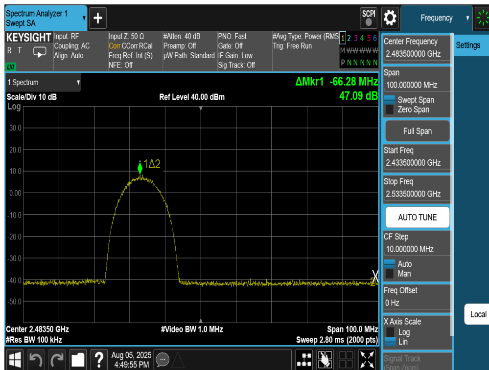
Plot 7-27. Band Edge Plot Antenna 4a (802.11b – Ch. 12)
