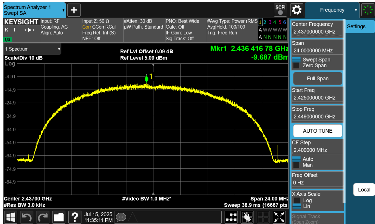
Plot 7-9 PSD Antenna 4a (20MHz BW 802.11b - Ch.6)
