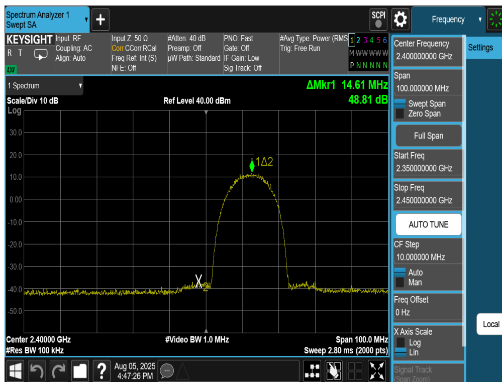
Plot 7-25. Band Edge Plot Antenna 4a (802.11b – Ch. 1)
