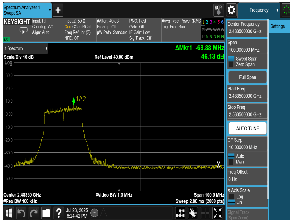
Plot 7-39. Band Edge Plot Antenna 4a (802.11g – Ch. 10)
