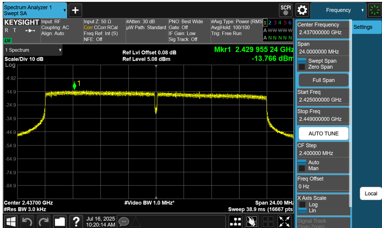
Plot 7-20 PSD CDD Antenna 4a (20MHz BW 802.11be(SU) - Ch.6)
