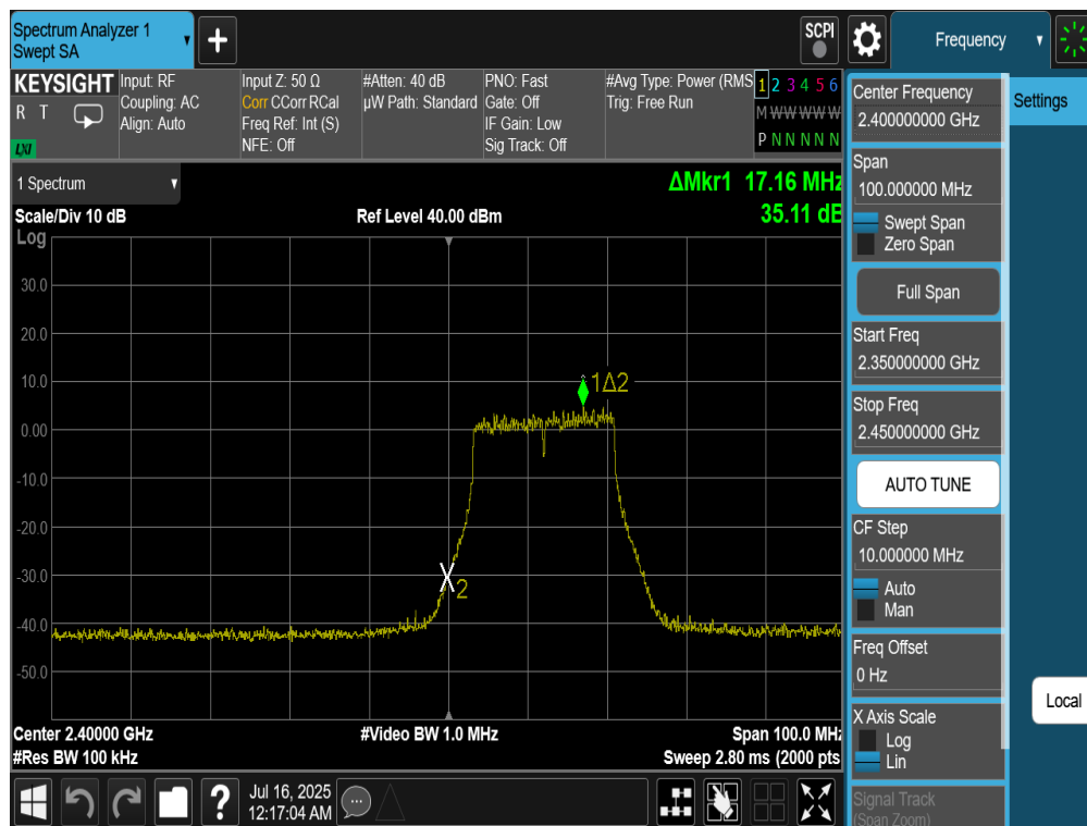
Plot 7-43. Band Edge Plot Antenna 4a (802.11n (2.4GHz) – Ch. 1)
