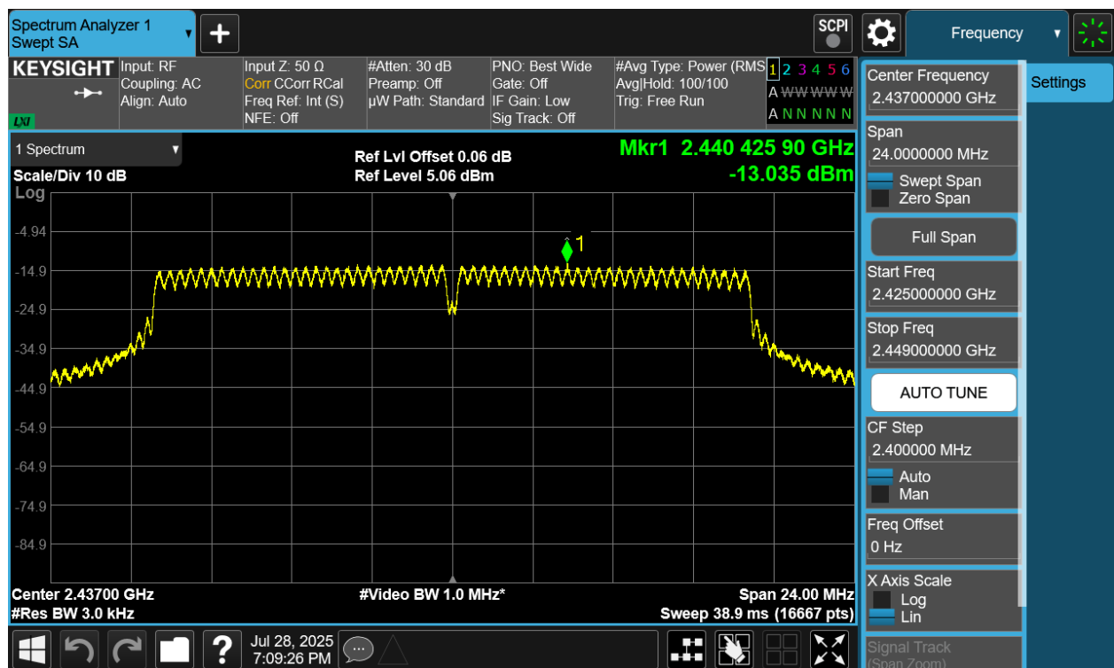
Plot 7-14 PSD Antenna 2a (20MHz BW 802.11g - Ch.6)
