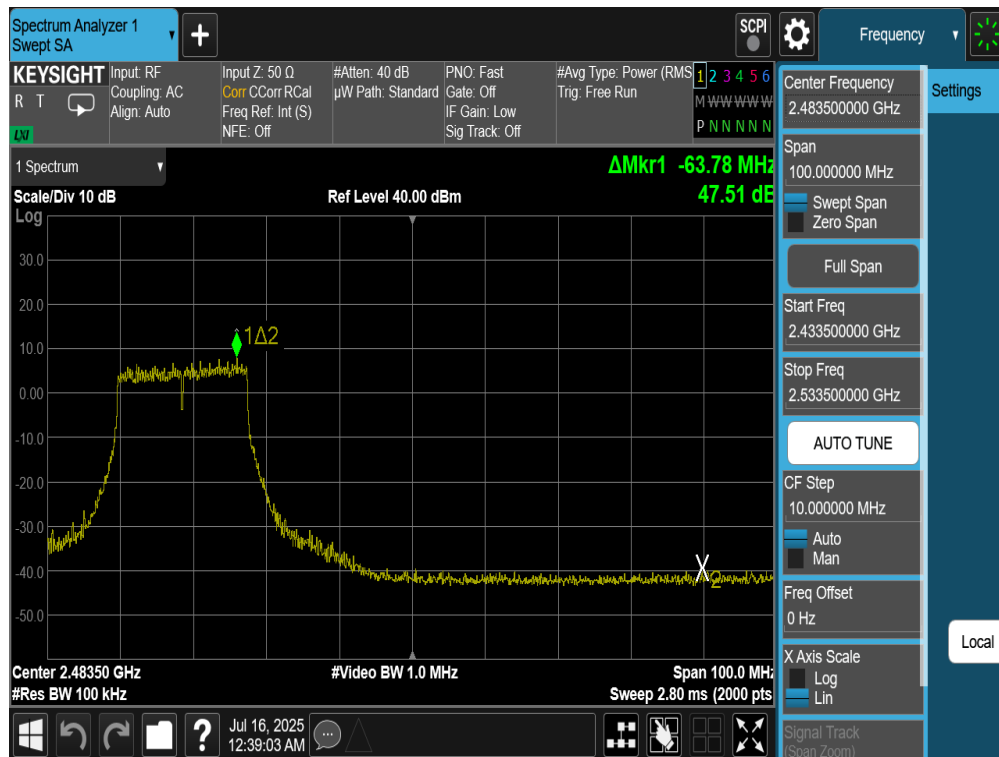
Plot 7-52. Band Edge Plot Antenna 4a (802.11n (2.4GHz) – Ch. 9)
