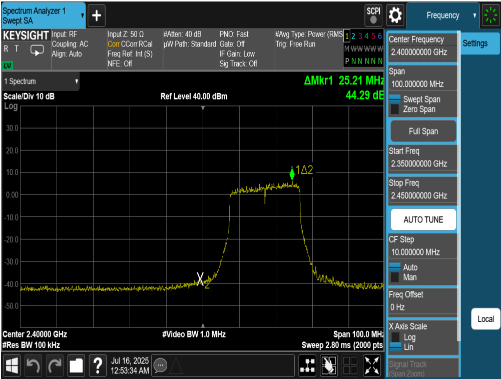
Plot 7-58. Band Edge Plot Antenna 4a (802.11be (SU - 2.4GHz) – Ch. 2)
