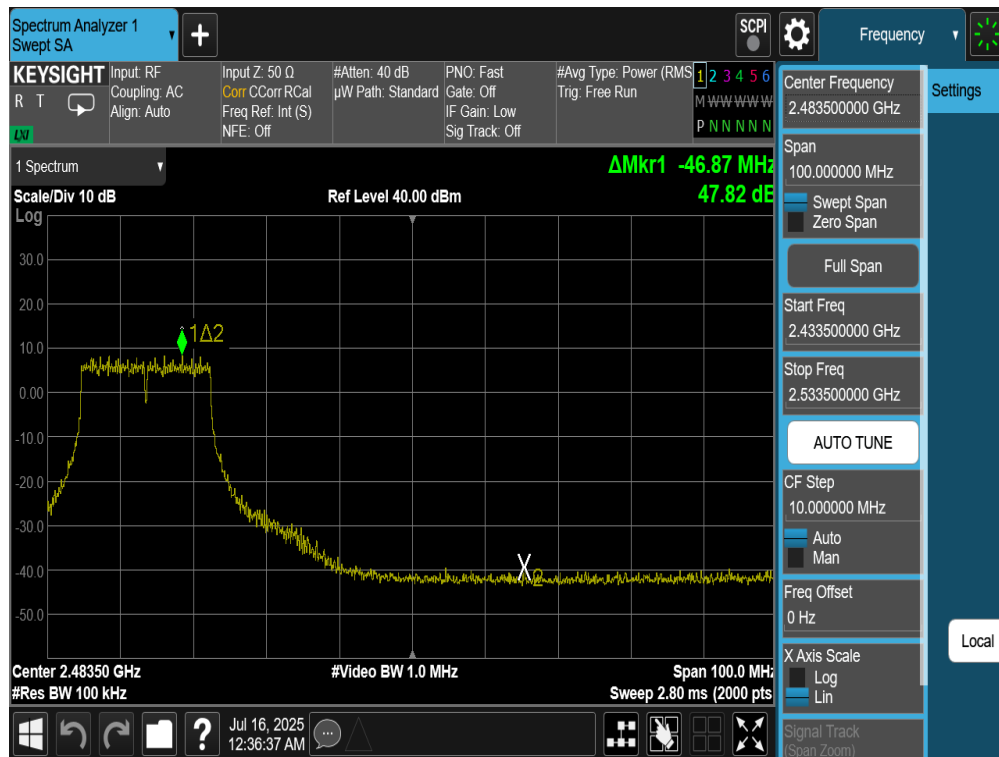
Plot 7-51. Band Edge Plot Antenna 4a (802.11n – Ch. 8)
