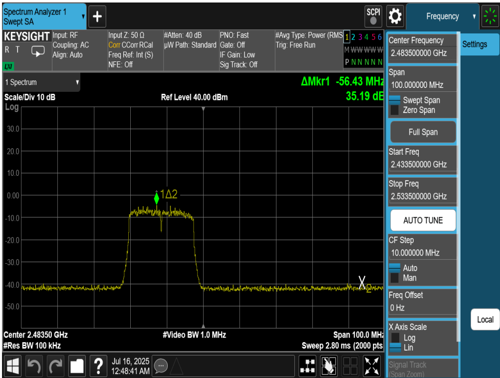
Plot 7-56. Band Edge Plot Antenna 4a (802.11n (2.4GHz) – Ch. 13)
