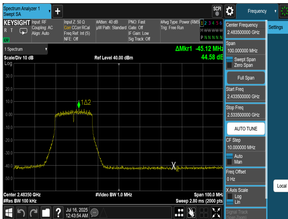
Plot 7-54. Band Edge Plot Antenna 4a (802.11n (2.4GHz) – Ch. 11)
