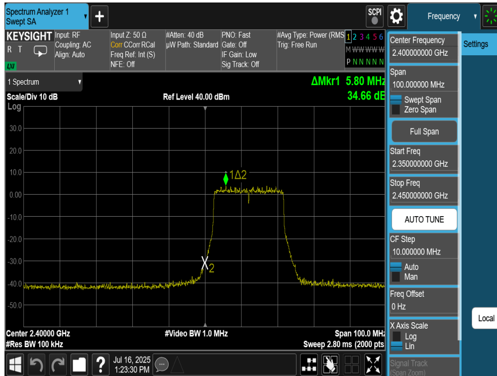
Plot 7-103. Band Edge Plot Antenna 2a (802.11be (SU - 2.4GHz) – Ch. 1)
