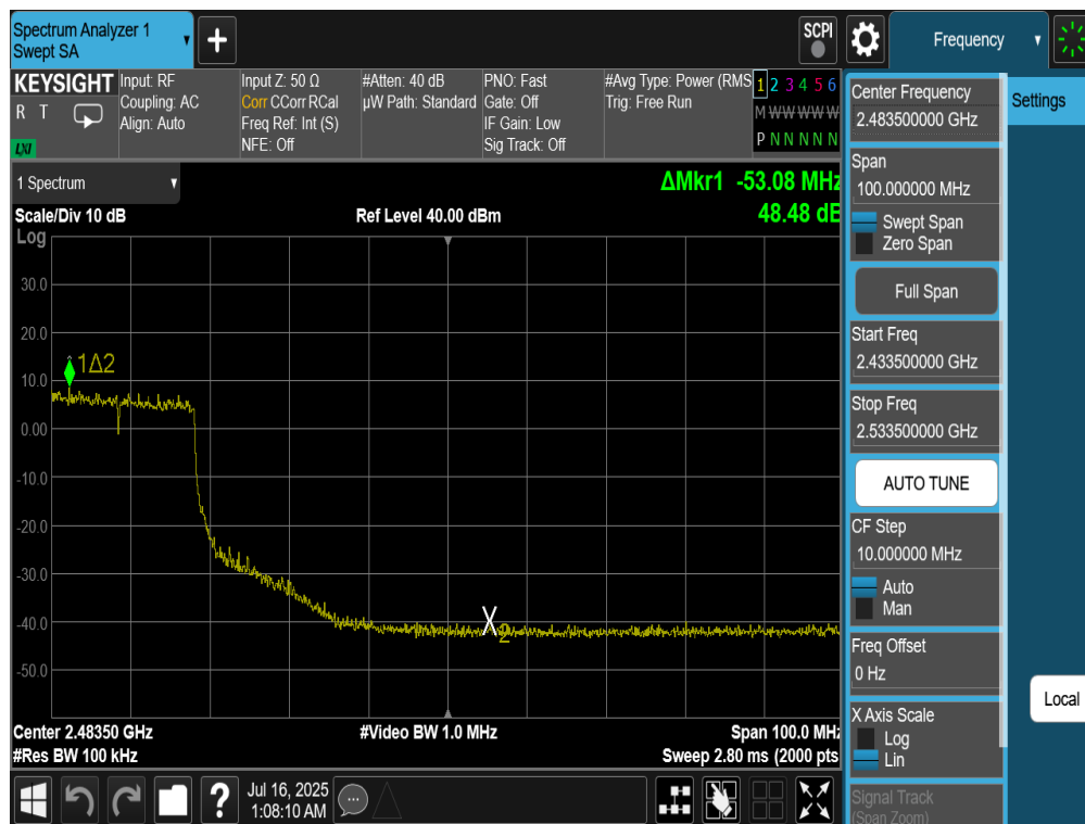
Plot 7-64. Band Edge Plot Antenna 4a (802.11be (SU - 2.4GHz) – Ch. 7)
