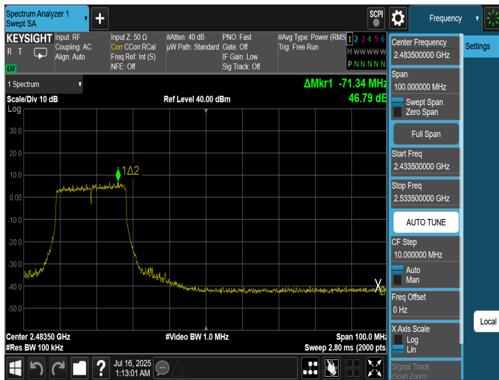
Plot 7-66. Band Edge Plot Antenna 4a (802.11be (SU - 2.4GHz) – Ch. 9)
