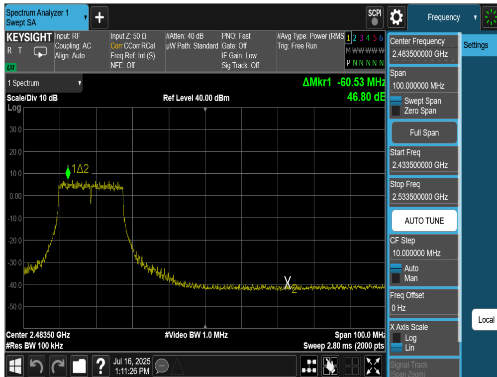
Plot 7-98. Band Edge Plot Antenna 2a (802.11n (2.4GHz) – Ch. 9)
