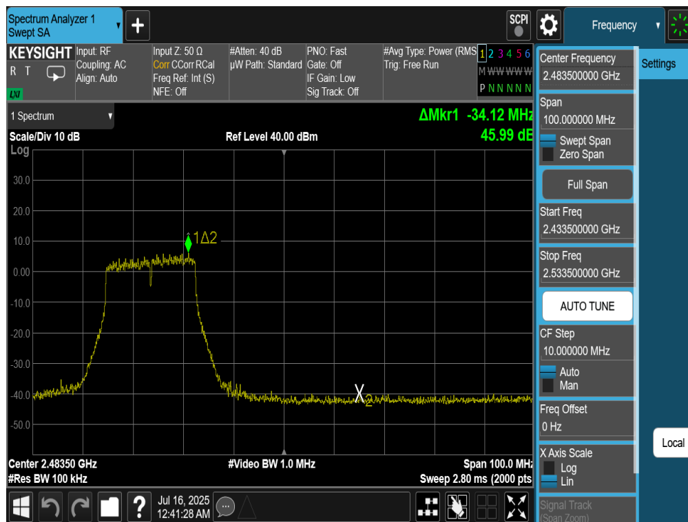
Plot 7-53. Band Edge Plot Antenna 4a (802.11n (2.4GHz) – Ch. 10)
