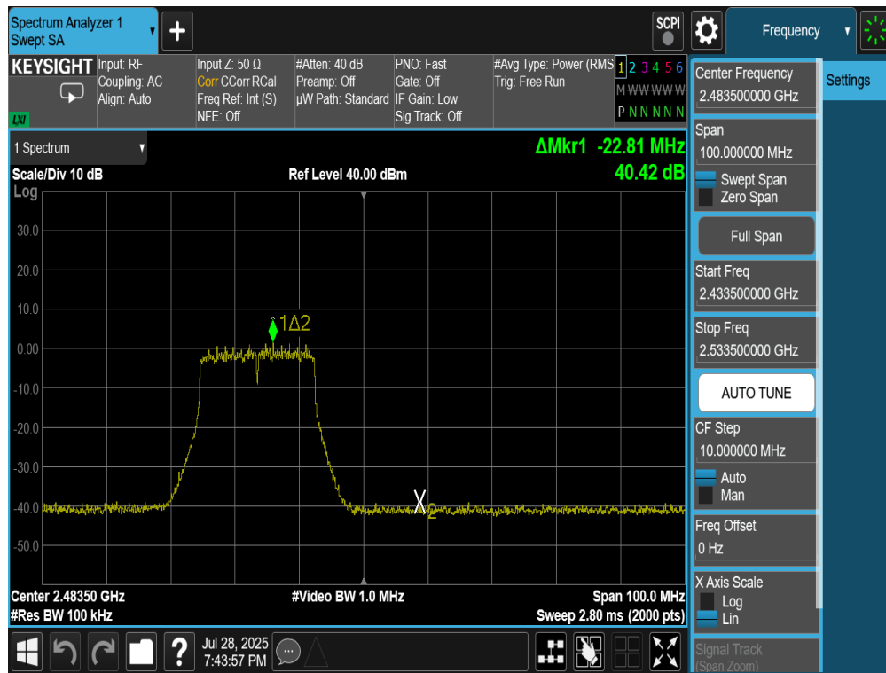
Plot 7-87. Band Edge Plot Antenna 2a (802.11g – Ch. 12)
