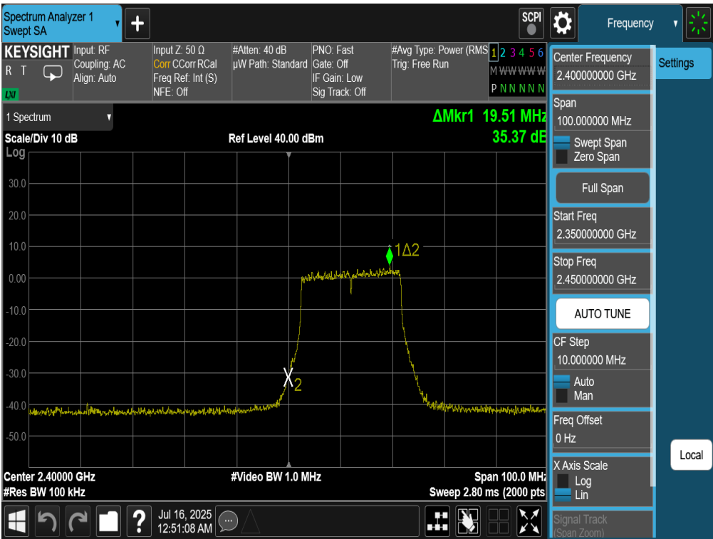
Plot 7-57. Band Edge Plot Antenna 4a (802.11be (SU - 2.4GHz) – Ch. 1)
