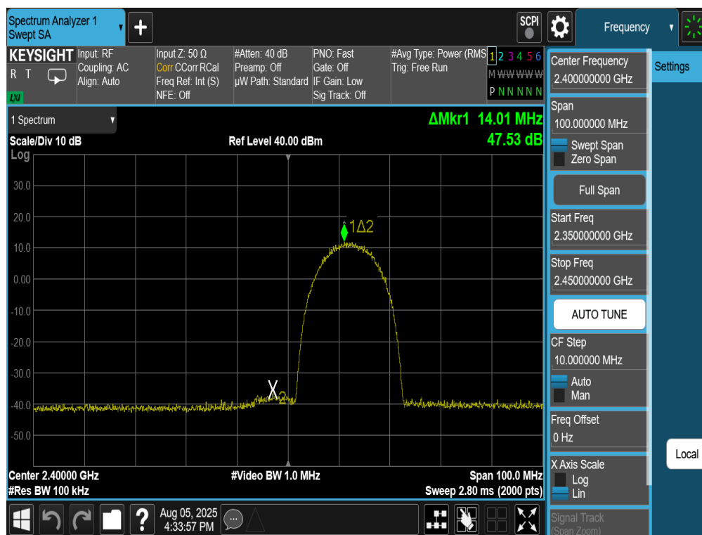
Plot 7-71. Band Edge Plot Antenna 2a (802.11b – Ch. 1)
