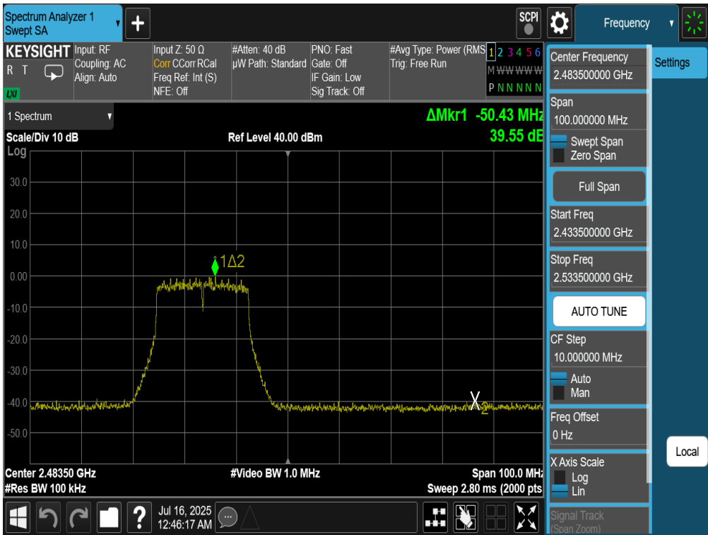
Plot 7-55. Band Edge Plot Antenna 4a (802.11n (2.4GHz) – Ch. 12)
