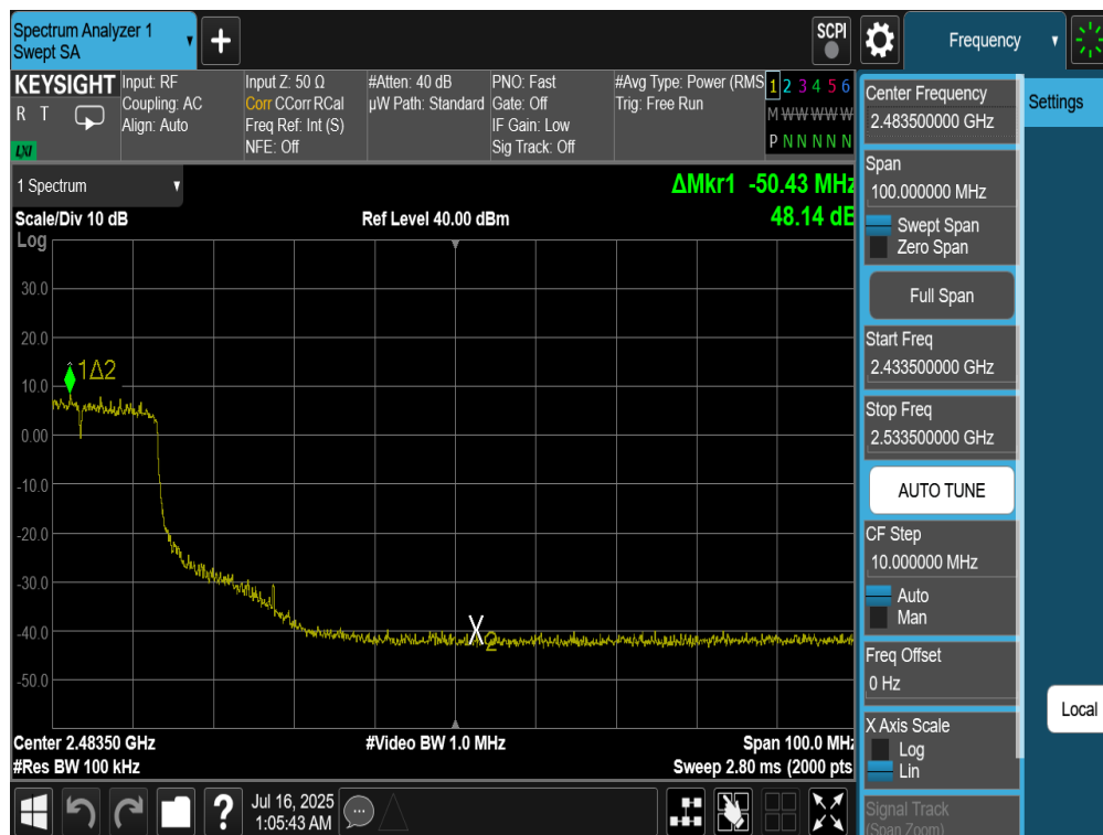
Plot 7-63. Band Edge Plot Antenna 4a (802. 11be (SU - 2.4GHz) – Ch. 6(high))
