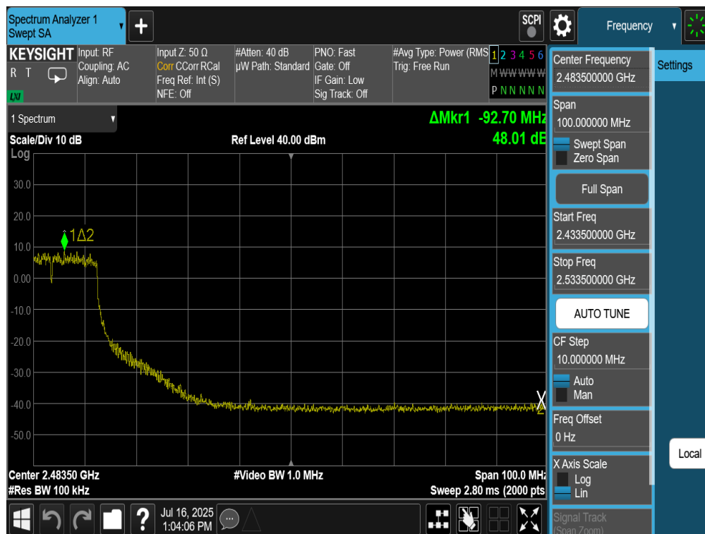
Plot 7-95. Band Edge Plot Antenna 2a (802.11n – Ch. 6(high))
