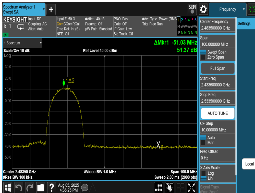
Plot 7-72. Band Edge Plot Antenna 2a (802.11b – Ch. 11)
