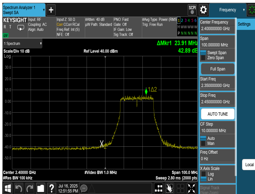
Plot 7-90. Band Edge Plot Antenna 2a (802.11n (2.4GHz) – Ch. 2)
