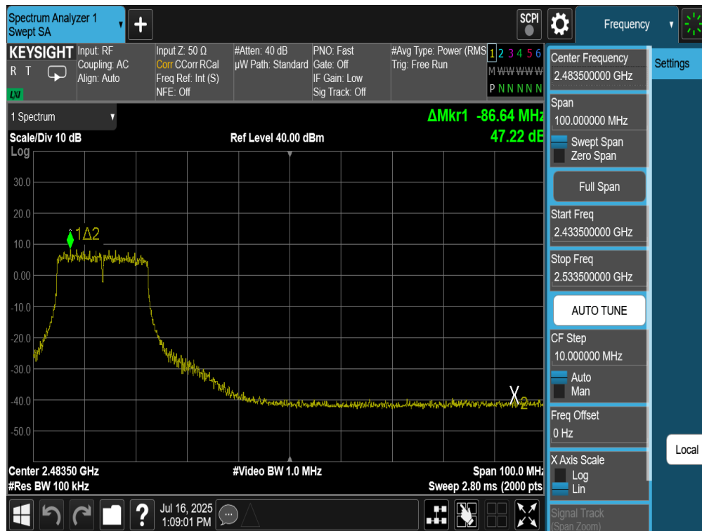
Plot 7-97. Band Edge Plot Antenna 2a (802.11n – Ch. 8)
