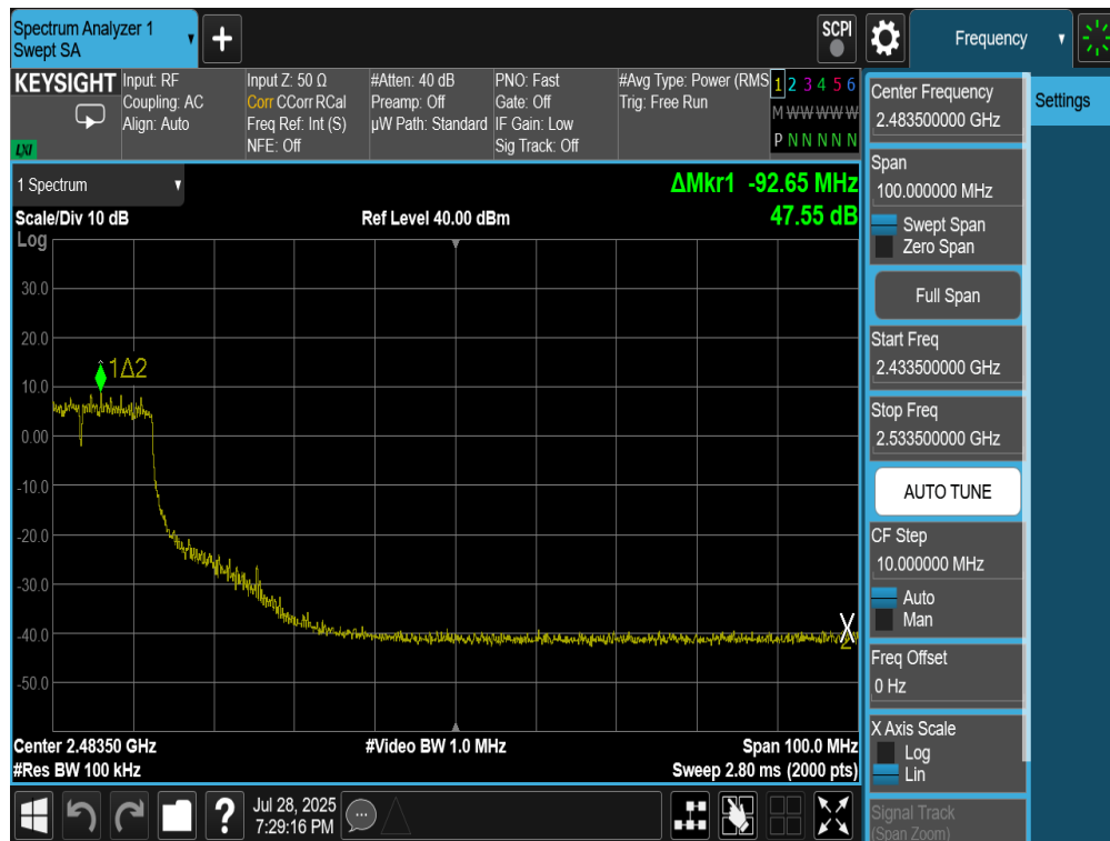
Plot 7-81. Band Edge Plot Antenna 2a (802.11g – Ch. 6(high))
