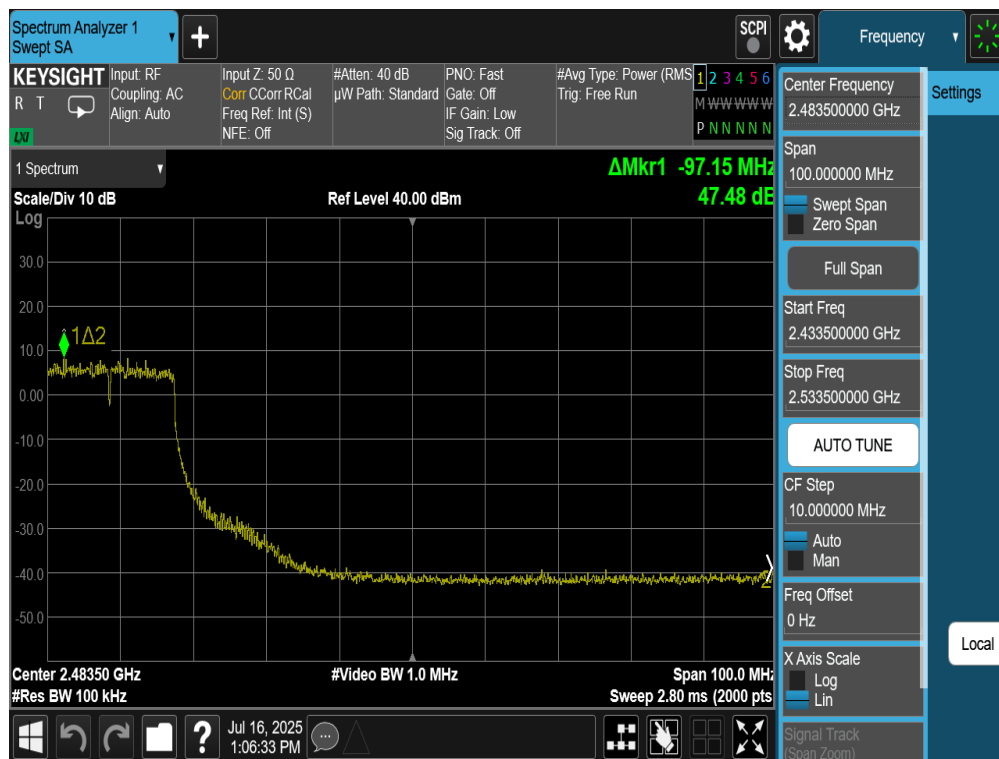
Plot 7-96. Band Edge Plot Antenna 2a (802.11n – Ch. 7)
