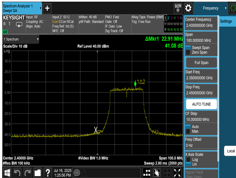
Plot 7-104. Band Edge Plot Antenna 2a (802.11be (SU - 2.4GHz) – Ch. 2)
