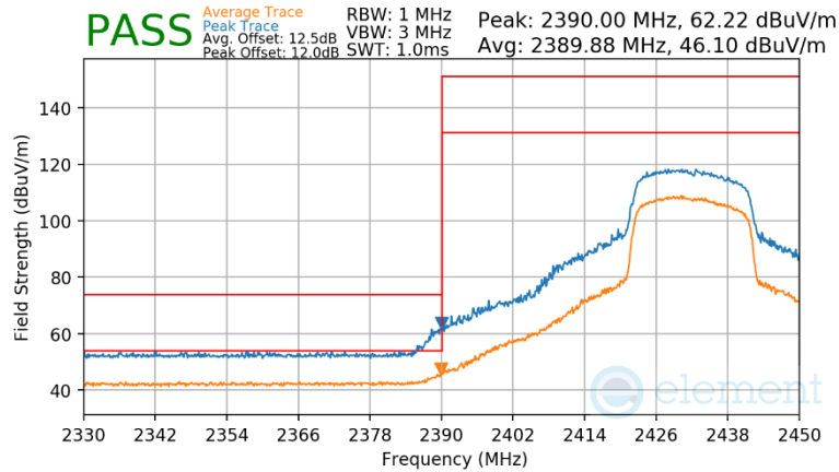
Plot 7-163 Radiated Restricted Lower Band Edge Measurement Antenna 4a
