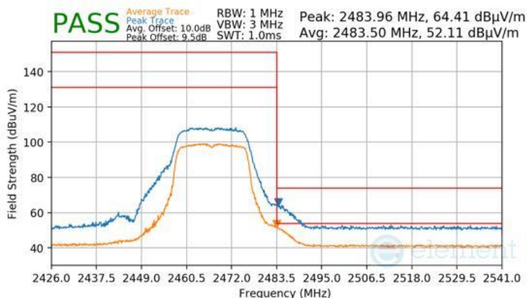
Plot 7-157 Radiated Restricted Upper Band Edge Measurement Antenna 4a
