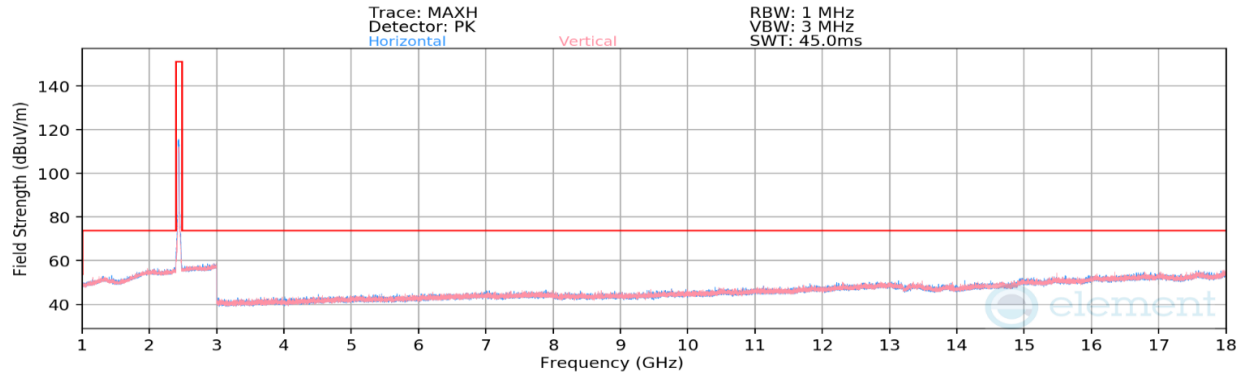
Plot 7-134. Radiated Spurious Emissions above 1GHz CDD (802.11n – Ch. 6)
