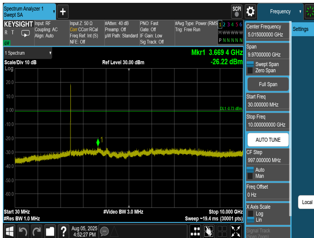
Plot 7-121. Conducted Spurious Plot Antenna 4a (802.11b – Ch. 11)
