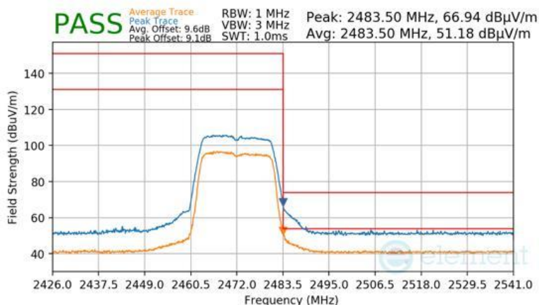
Plot 7-158 Radiated Restricted Upper Band Edge Measurement Antenna 4a
