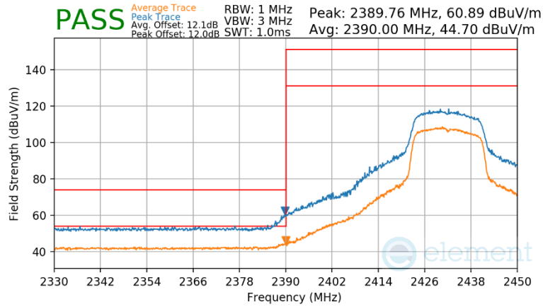
Plot 7-149 Radiated Restricted Lower Band Edge Measurement Antenna 4a
