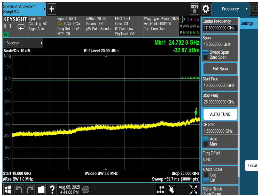
Plot 7-128. Conducted Spurious Plot Antenna 2a (802.11b – Ch. 11)
