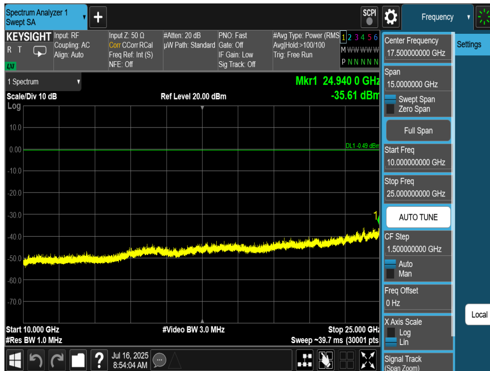
Plot 7-120. Conducted Spurious Plot Antenna 4a (802.11b – Ch. 6)
