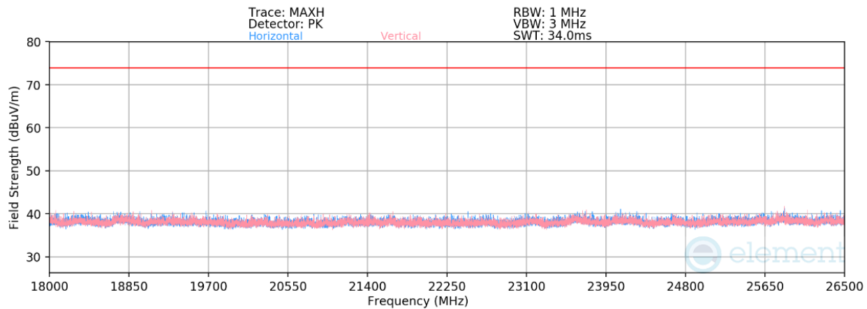
Plot 7-139. Radiated Spurious Emissions above 18GHz CDD (802.11be (SU) – Ch.6)
