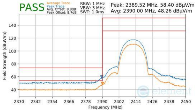
Plot 7-141 Radiated Restricted Lower Band Edge Measurement Antenna 4a
