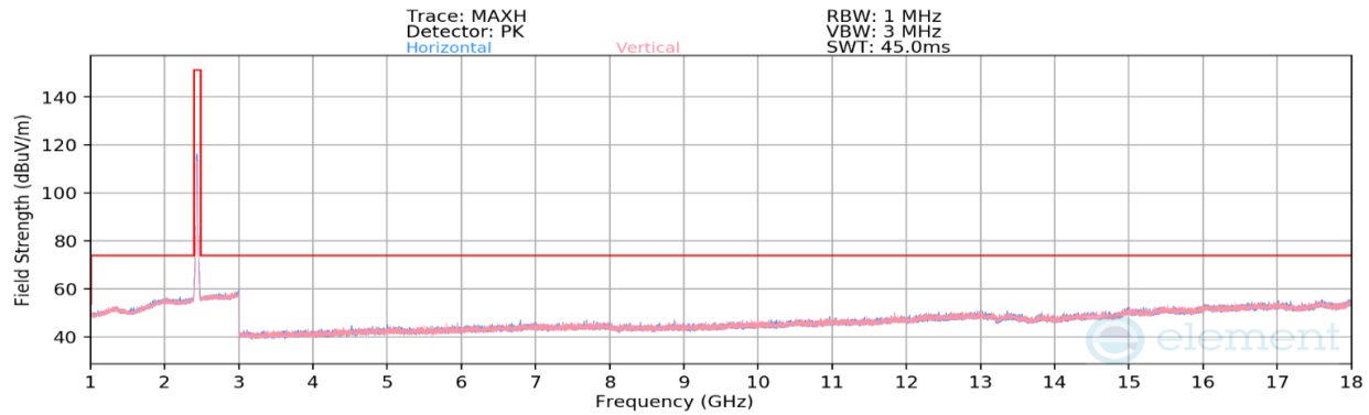
Plot 7-138. Radiated Spurious Emissions above 1GHz CDD (802.11be (SU) – Ch. 6)
