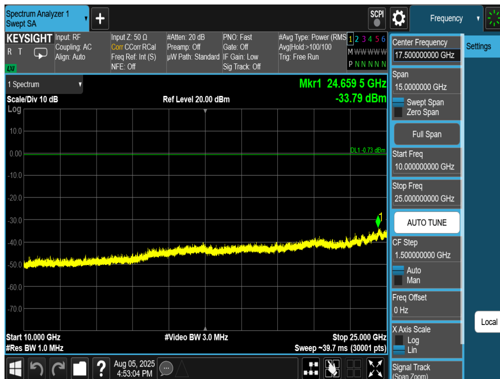
Plot 7-122. Conducted Spurious Plot Antenna 4a (802.11b – Ch. 11)
