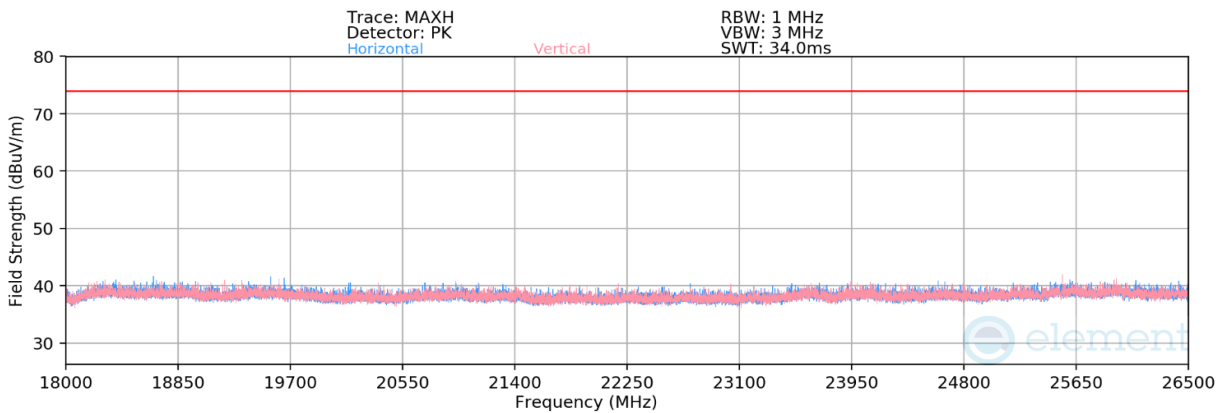
Plot 7-131. Radiated Spurious Emissions above 18GHz CDD (802.11b – Ch.6)
