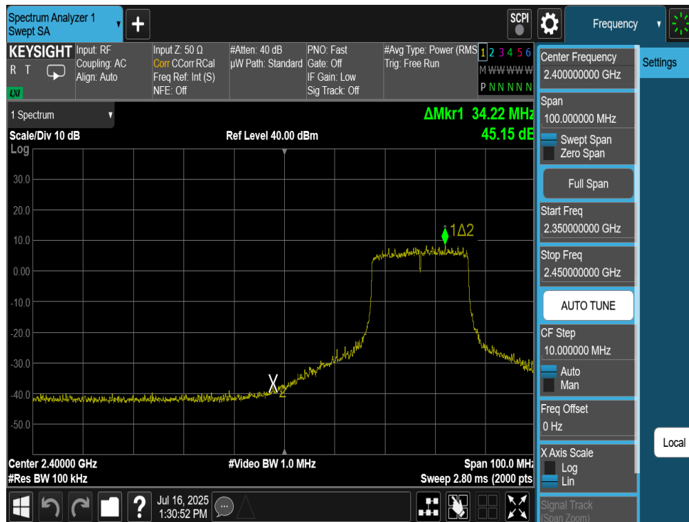
Plot 7-106. Band Edge Plot Antenna 2a (802.11be (SU - 2.4GHz) – Ch. 4)
