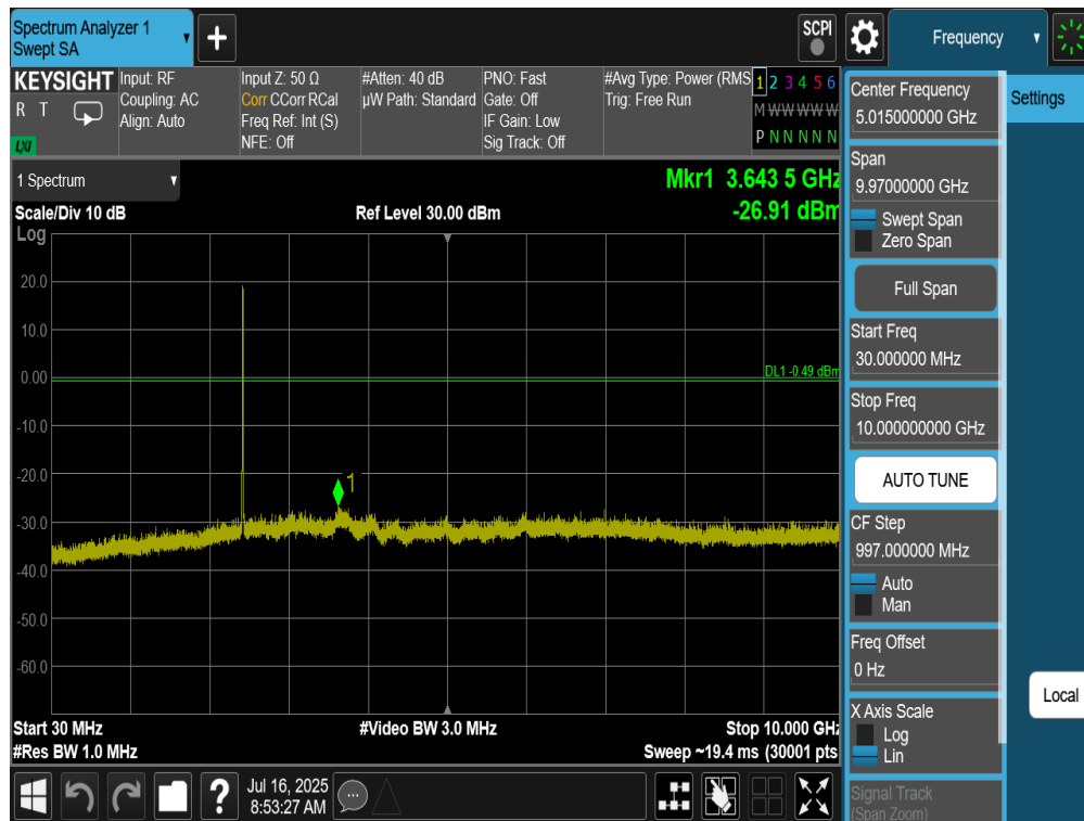
Plot 7-119. Conducted Spurious Plot Antenna 4a (802.11b – Ch. 6)
