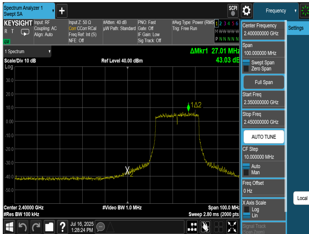
Plot 7-105. Band Edge Plot Antenna 2a (802.11be (SU - 2.4GHz) – Ch. 3)
