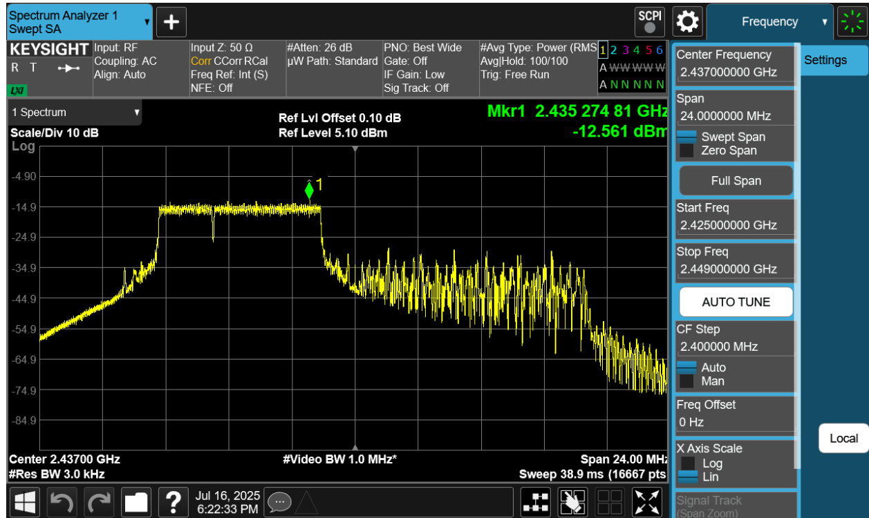
Plot 7-15 PSD Antenna 2a (20MHz BW 802.11be(RU) RU52+26 Index70 - Ch.6)
