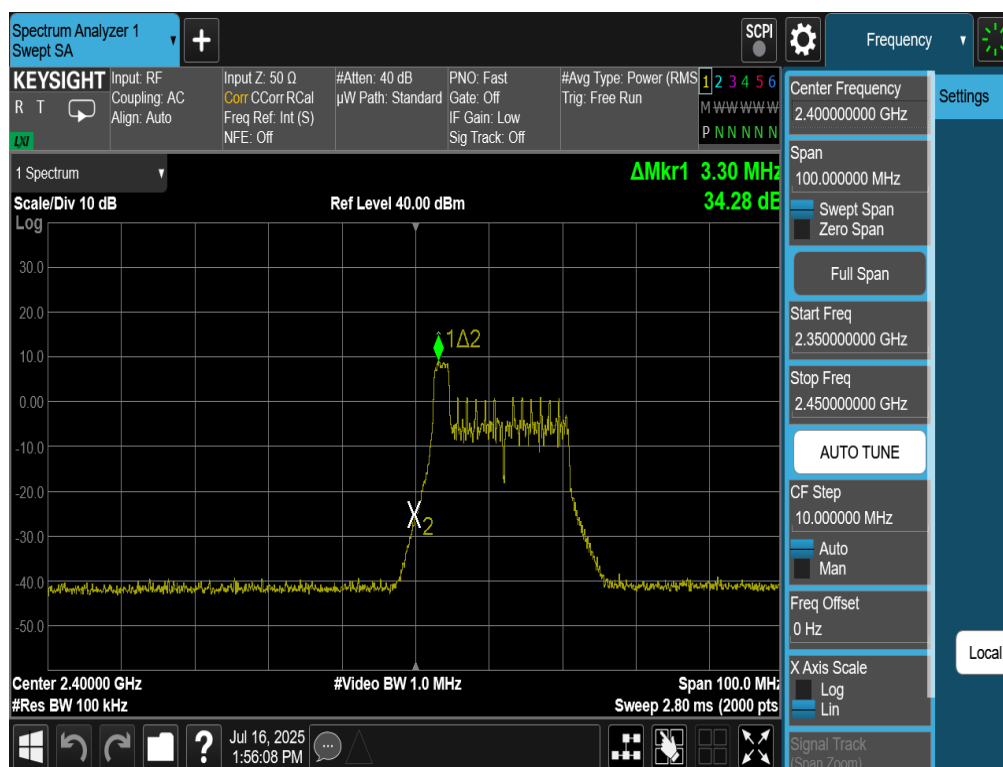
Plot 7-43. Band Edge Antenna 2a (802.11be OFDMA – RU26 Index 0 – Ch. 1)
