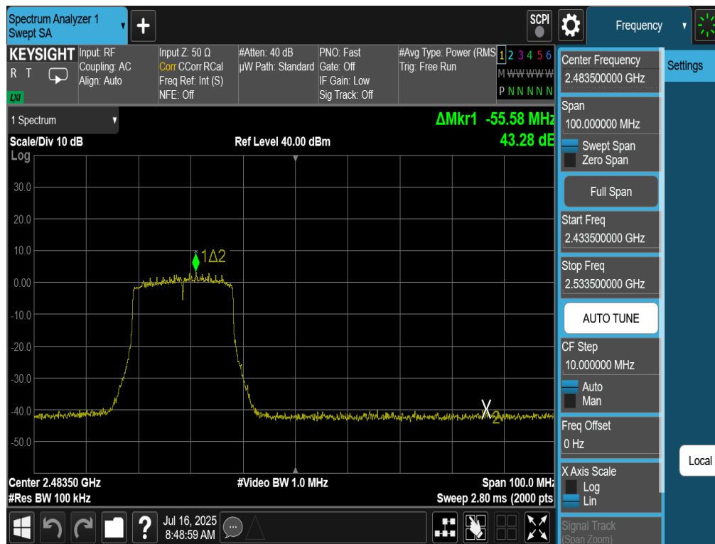
Plot 7-40. Band Edge Antenna 4a (802.11be OFDMA – RU242 – Ch. 11)
