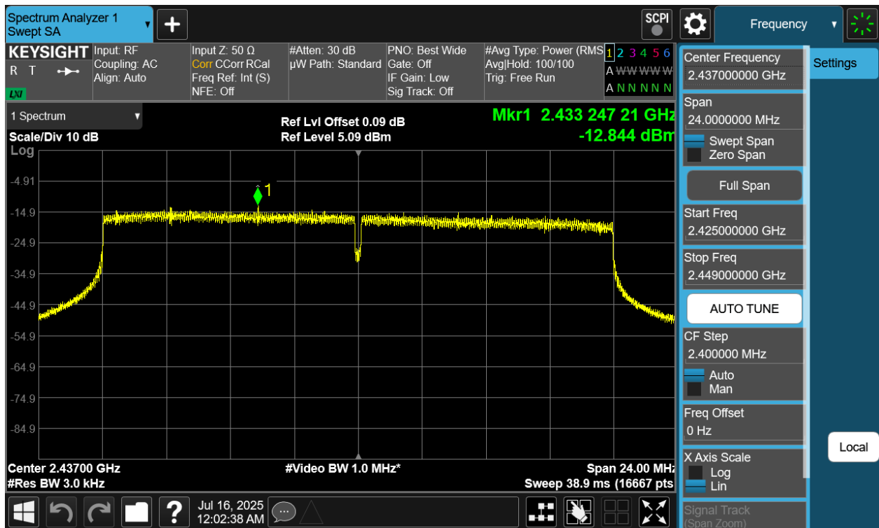
Plot 7-10 PSD Antenna 4a (20MHz BW 802.11be(RU) RU242 Index61 - Ch.6)
