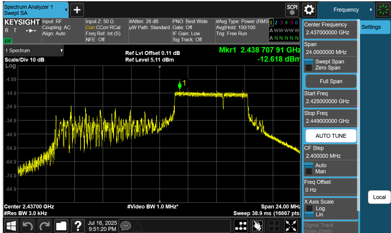
Plot 7-11 PSD Antenna 4a (20MHz BW 802.11be(RU) RU52+26 Index72 - Ch.6)
