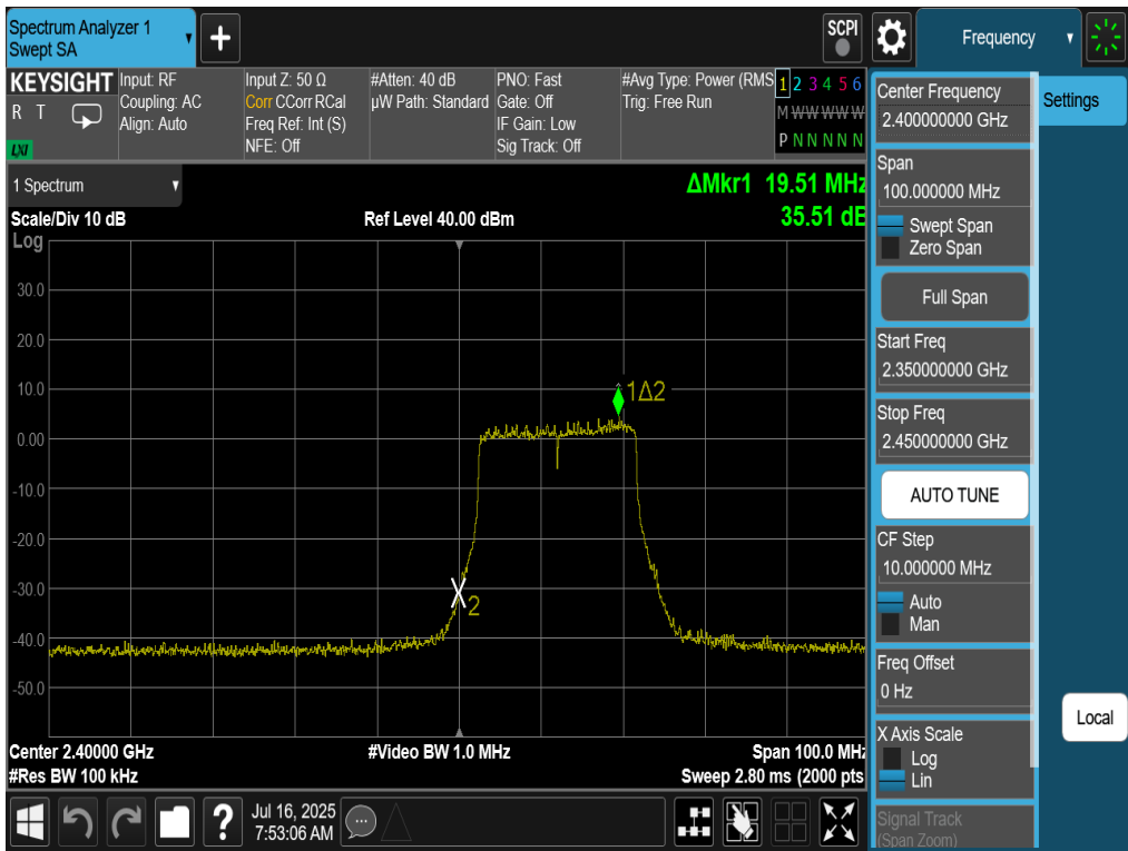
Plot 7-29. Band Edge Antenna 4a (802.11be OFDMA – RU242 – Ch. 1)
