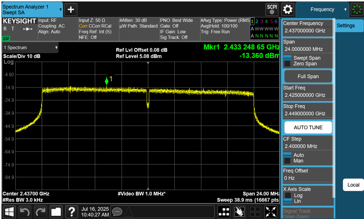
Plot 7-18 PSD CDD Antenna 4a (20MHz BW 802.11be(RU) RU242 Index61 - Ch.6)
