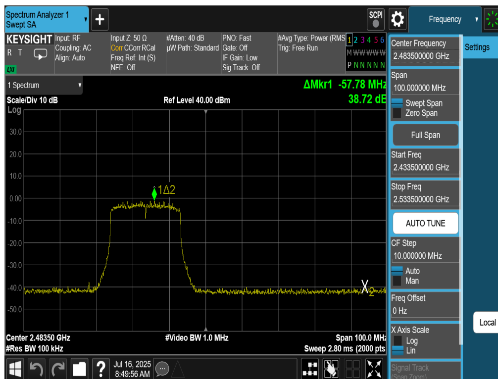
Plot 7-41. Band Edge Antenna 4a (802.11be OFDMA – RU242 – Ch. 12)
