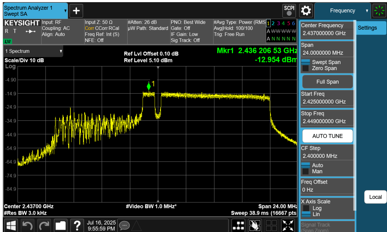
Plot 7-12 PSD Antenna 4a (20MHz BW 802.11be(RU) RU106+26 Index83 - Ch.6)
