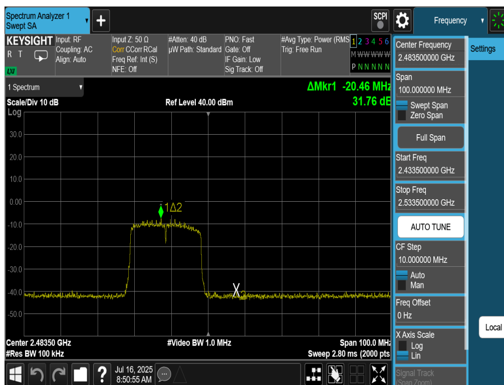
Plot 7-42. Band Edge Antenna 4a (802.11be OFDMA – RU242 – Ch. 13)
