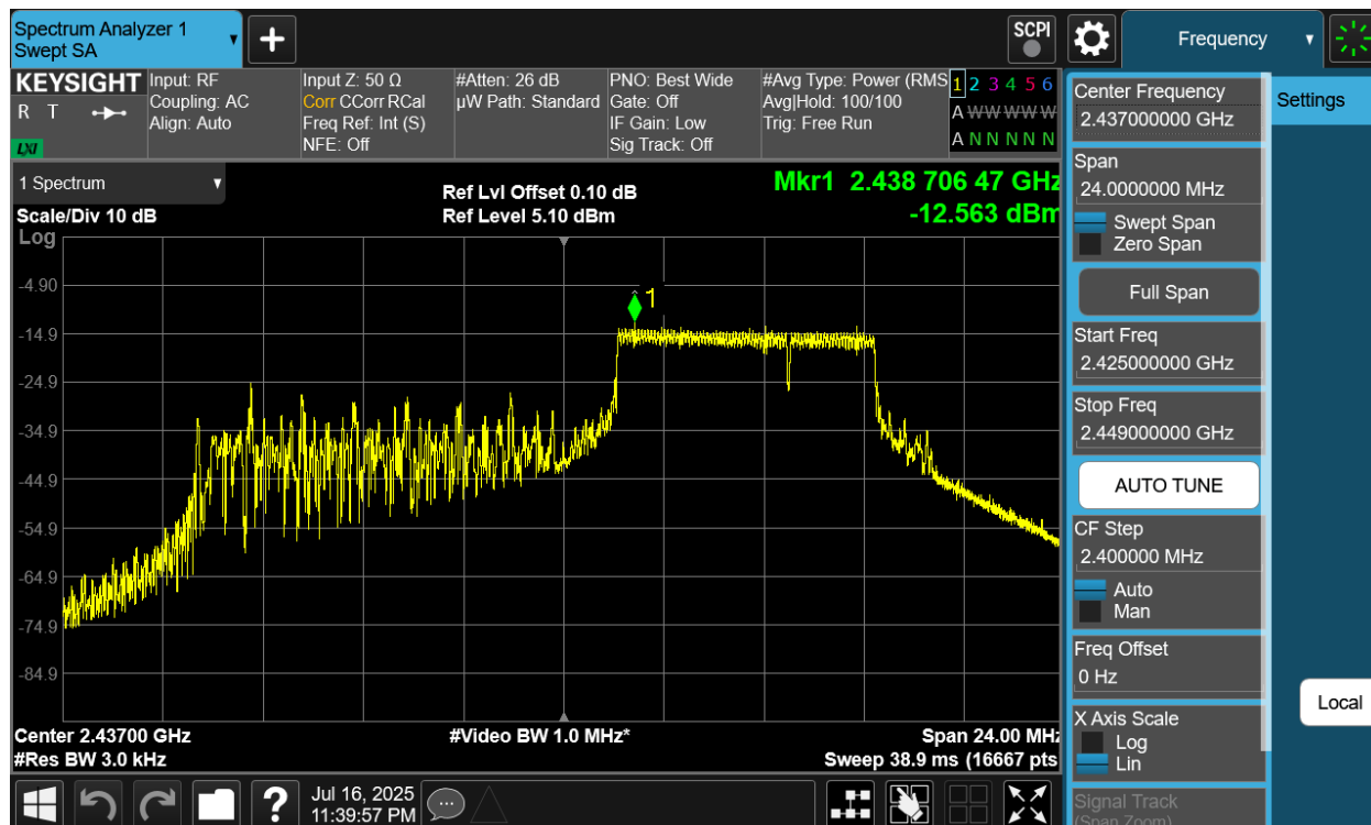
Plot 7-19 PSD CDD Antenna 4a (20MHz BW 802.11be(RU) RU52+26 Index72 - Ch.6)
