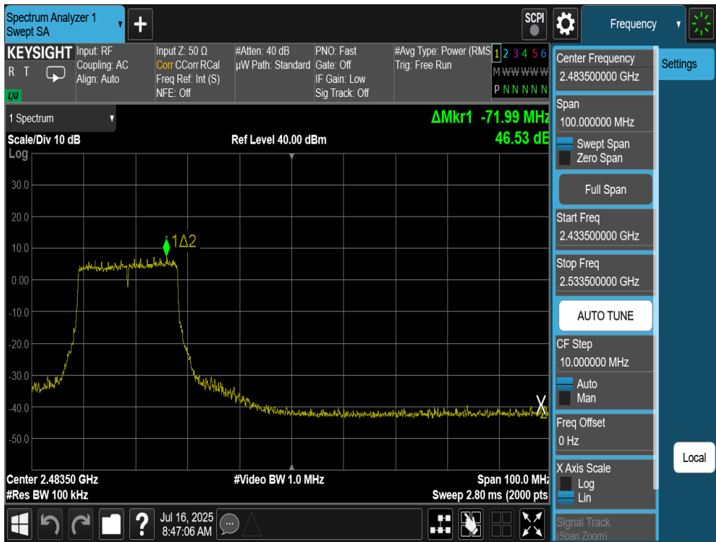
Plot 7-38. Band Edge Antenna 4a (802.11be OFDMA – RU242 – Ch. 9)
