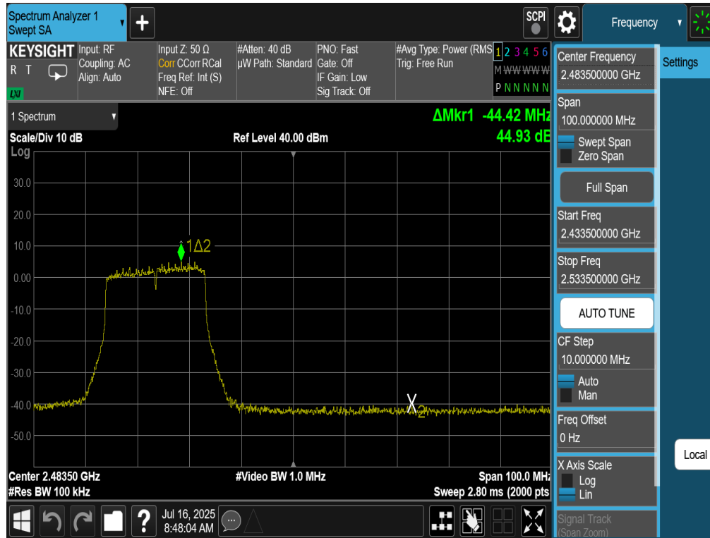
Plot 7-39. Band Edge Antenna 4a (802.11be OFDMA – RU242 – Ch. 10)
