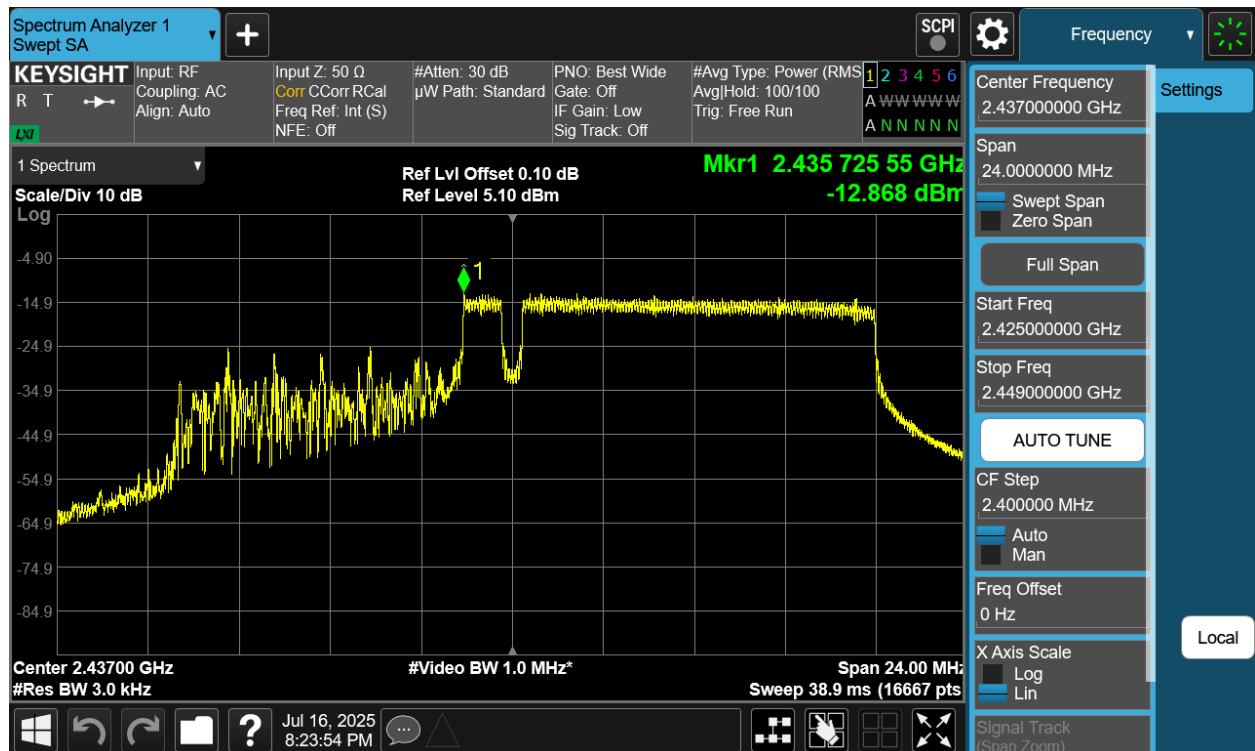
Plot 7-24 PSD CDD Antenna 2a (20MHz BW 802.11be(RU) RU106+26 Index83 - Ch.6)
