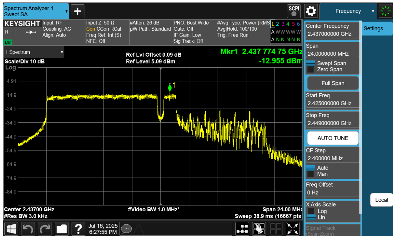
Plot 7-16 PSD Antenna 2a (20MHz BW 802.11be(RU) RU106+26 Index82 - Ch.6)
