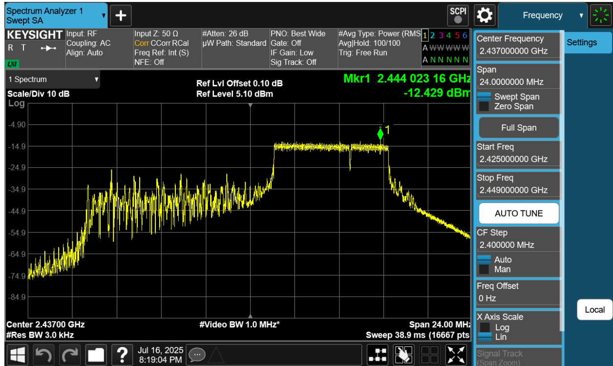
Plot 7-23 PSD CDD Antenna 2a (20MHz BW 802.11be(RU) RU52+26 Index72 - Ch.6)
