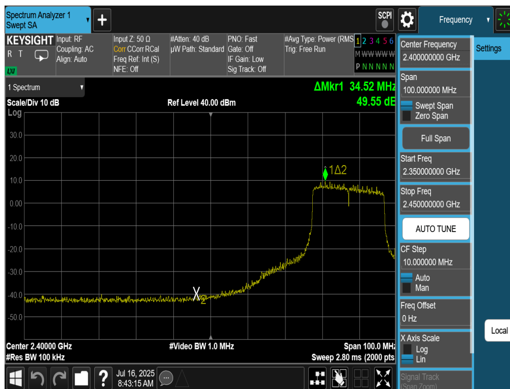
Plot 7-34. Band Edge Antenna 4a (802.11be OFDMA – RU242 – Ch. 6(Low Channel))
