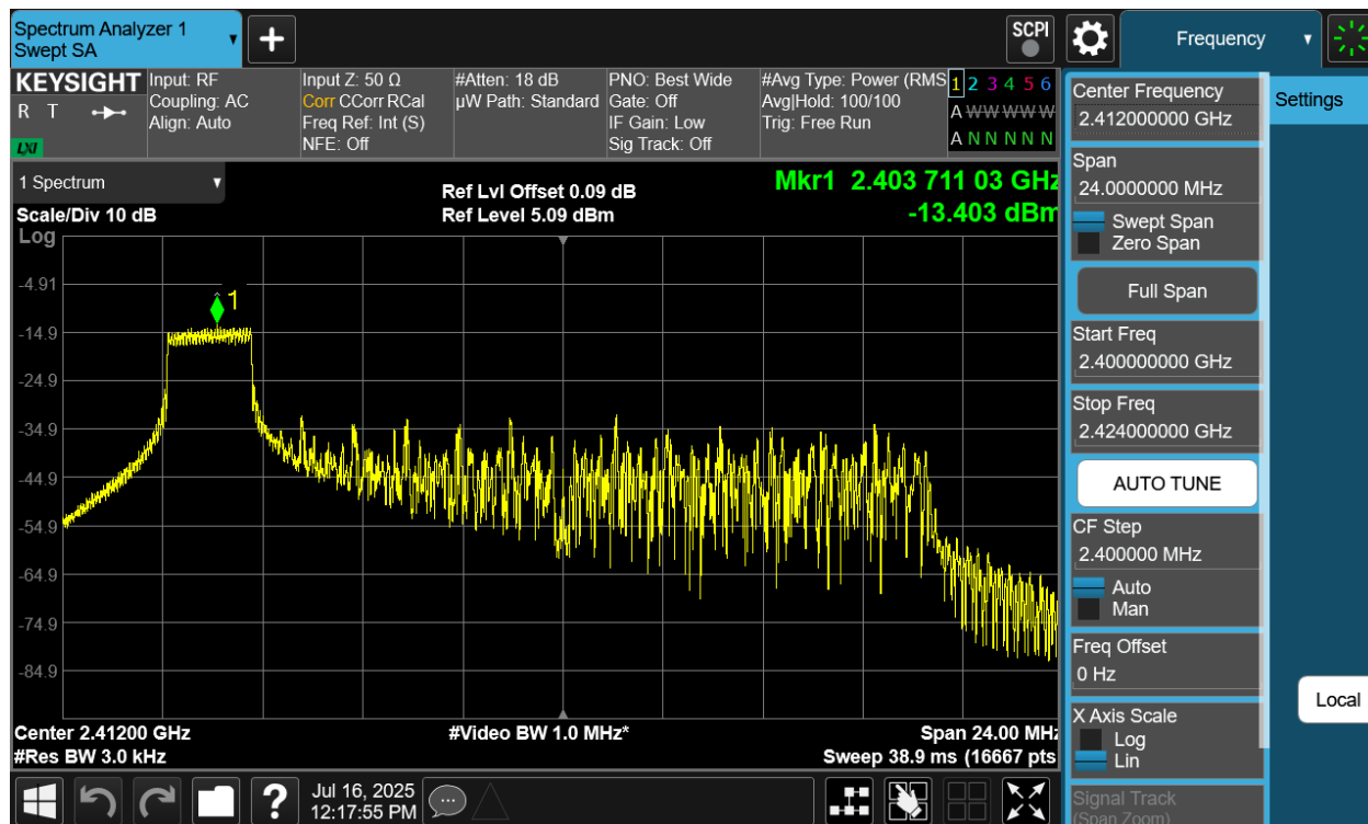
Plot 7-13 PSD Antenna 2a (20MHz BW 802.11be(RU) RU26 Index0 - Ch.1)
