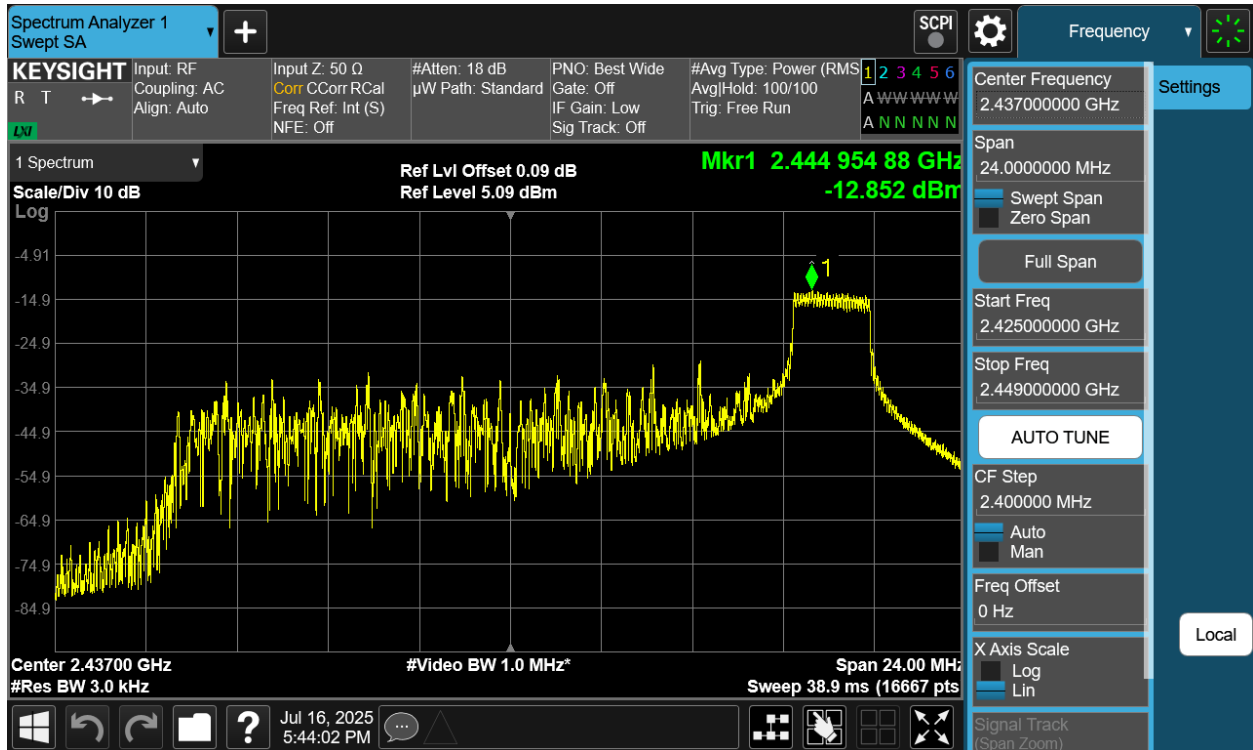
Plot 7-21 PSD CDD Antenna 2a (20MHz BW 802.11be(RU) RU26 Index8 - Ch.6)
