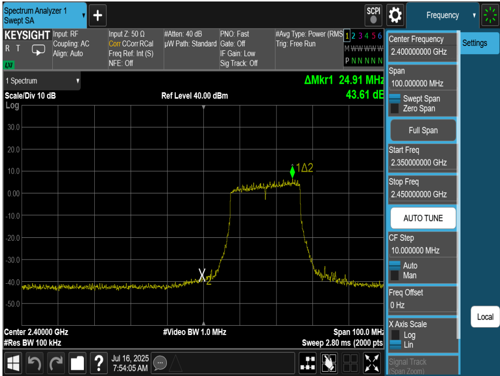
Plot 7-30. Band Edge Antenna 4a (802.11be OFDMA – RU242 – Ch. 2)
