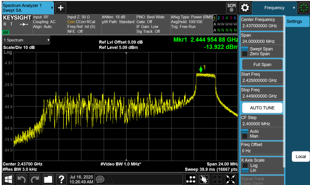
Plot 7-17 PSD CDD Antenna 4a (20MHz BW 802.11be(RU) RU26 Index8 - Ch.6)
