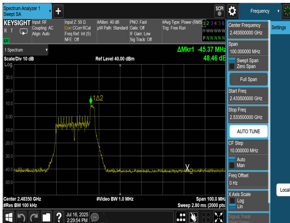
Plot 7-44. Band Edge Antenna 2a (802.11be OFDMA – RU26 Index 8 – Ch. 11)
