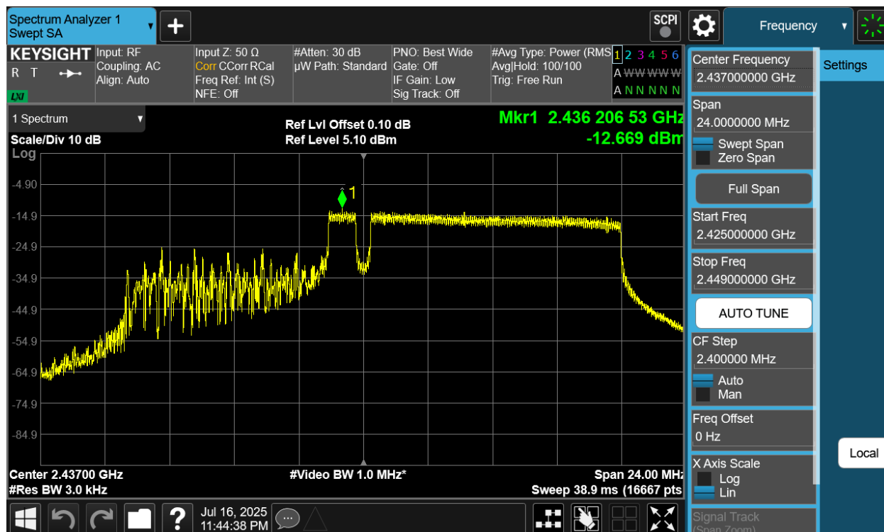
Plot 7-20 PSD CDD Antenna 4a (20MHz BW 802.11be(RU) RU106+26 Index83 - Ch.6)
