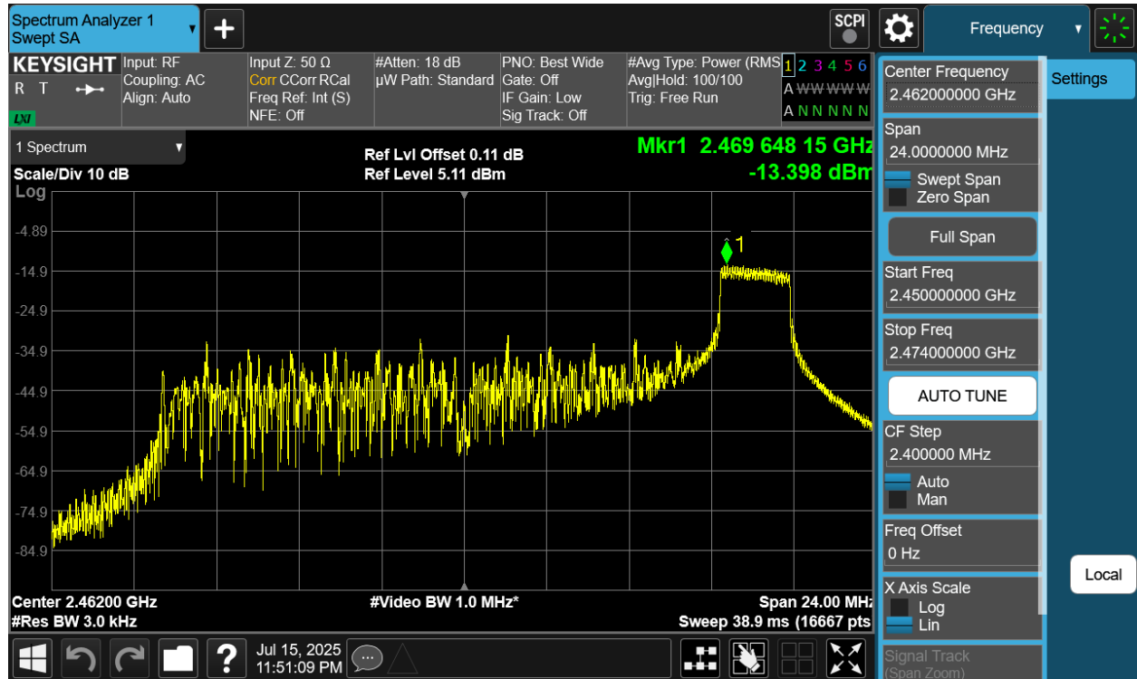
Plot 7-9 PSD Antenna 4a (20MHz BW 802.11be(RU) RU26 Index8 - Ch.11)
