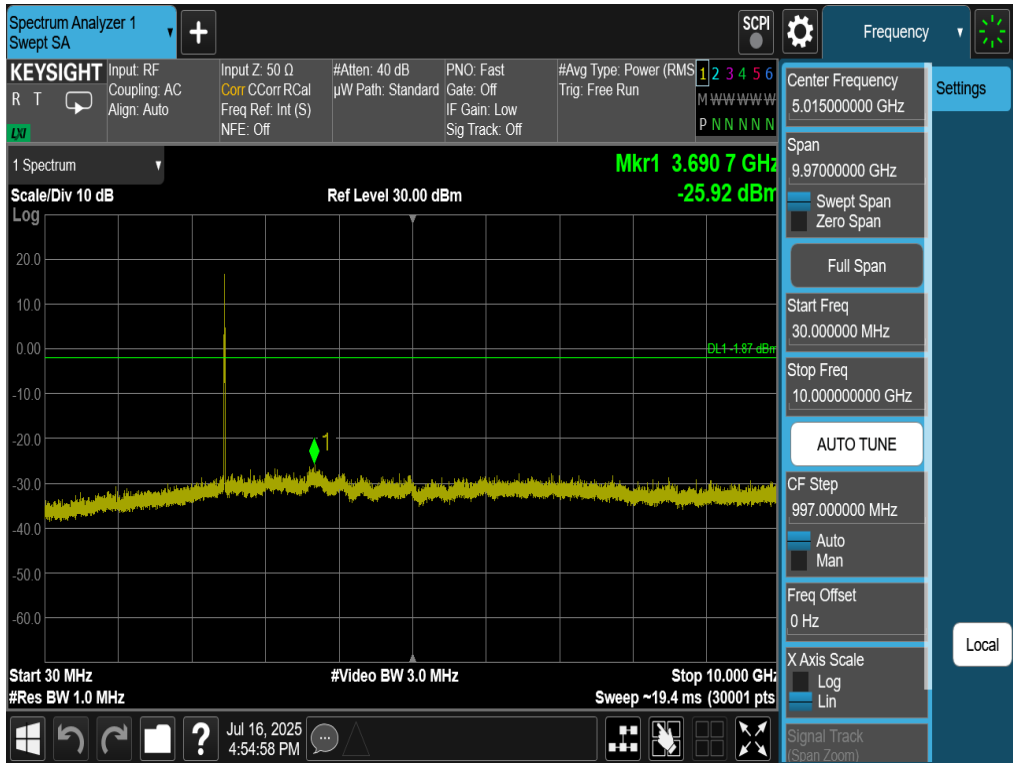
Plot 7-77. Conducted Spurious Plot Antenna 2a (802.11be OFDMA – RU26 – Ch. 11)
