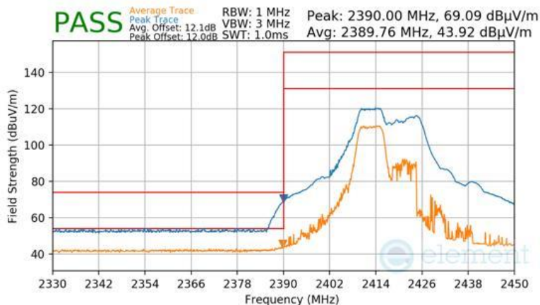
Plot 7-98 Radiated Restricted Lower Band Edge Measurement Antenna 4a (Peak & Average – RU52+26)
