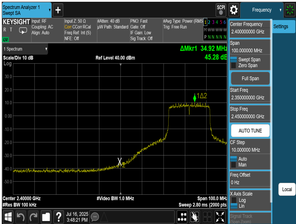
Plot 7-51. Band Edge Antenna 2a (802.11be OFDMA – RU242 – Ch. 5)
