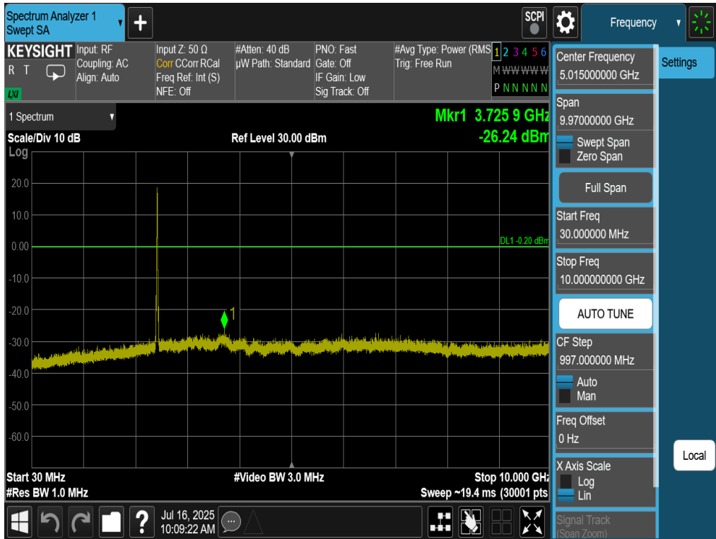
Plot 7-69. Conducted Spurious Plot Antenna 4a (802.11be OFDMA – RU242 – Ch. 6)
