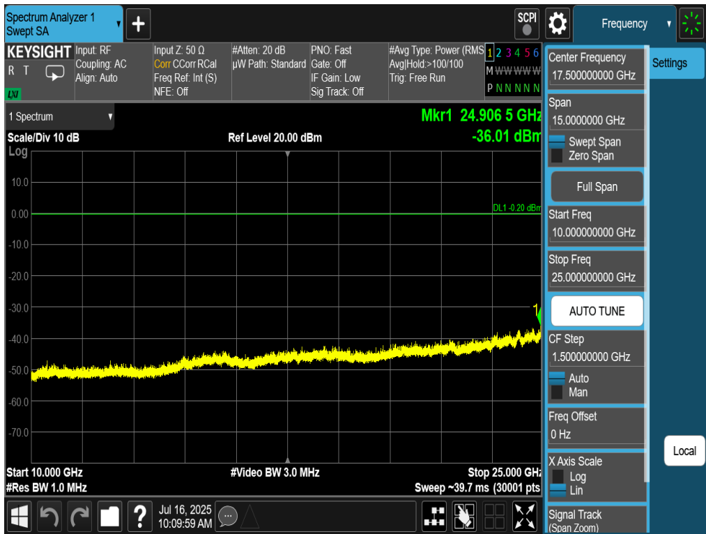
Plot 7-70. Conducted Spurious Plot Antenna 4a (802.11be OFDMA – RU242 – Ch. 6)
