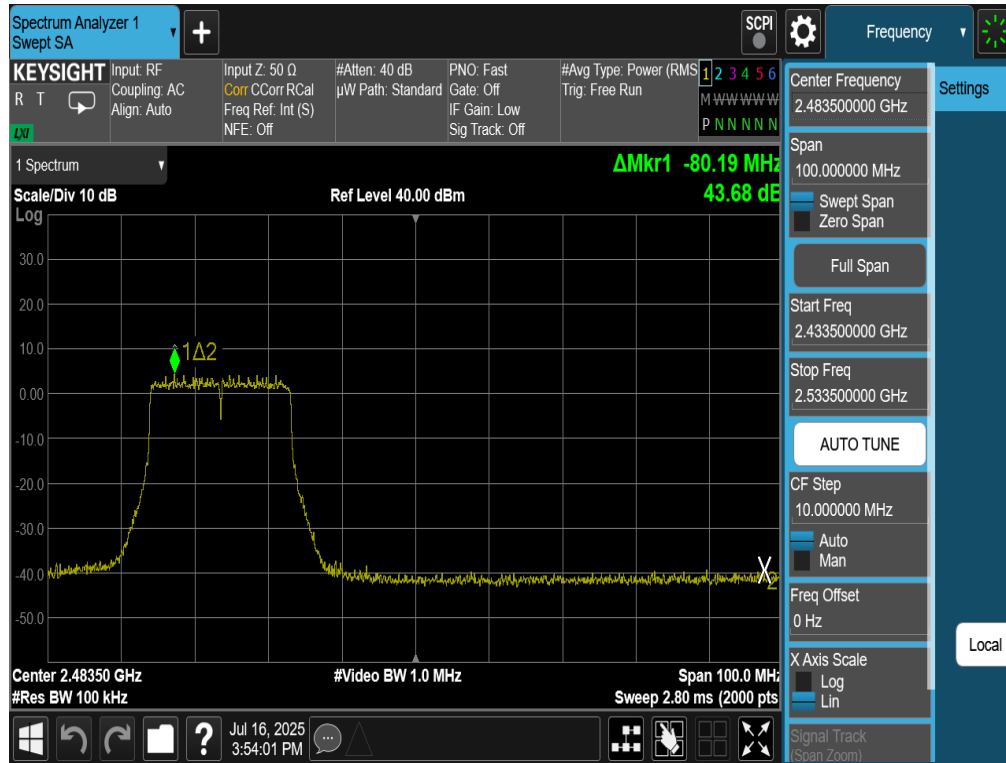
Plot 7-57. Band Edge Antenna 2a (802.11be OFDMA – RU242 – Ch. 10)
