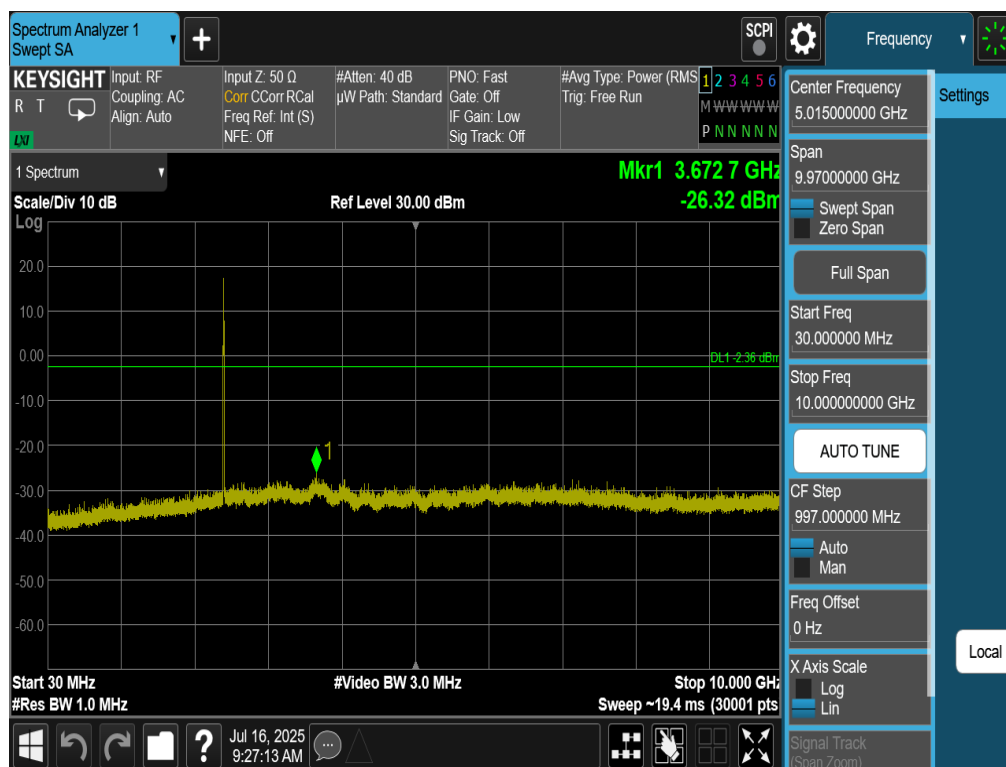
Plot 7-61. Conducted Spurious Plot Antenna 4a (802.11be OFDMA – RU26 – Ch. 1)
