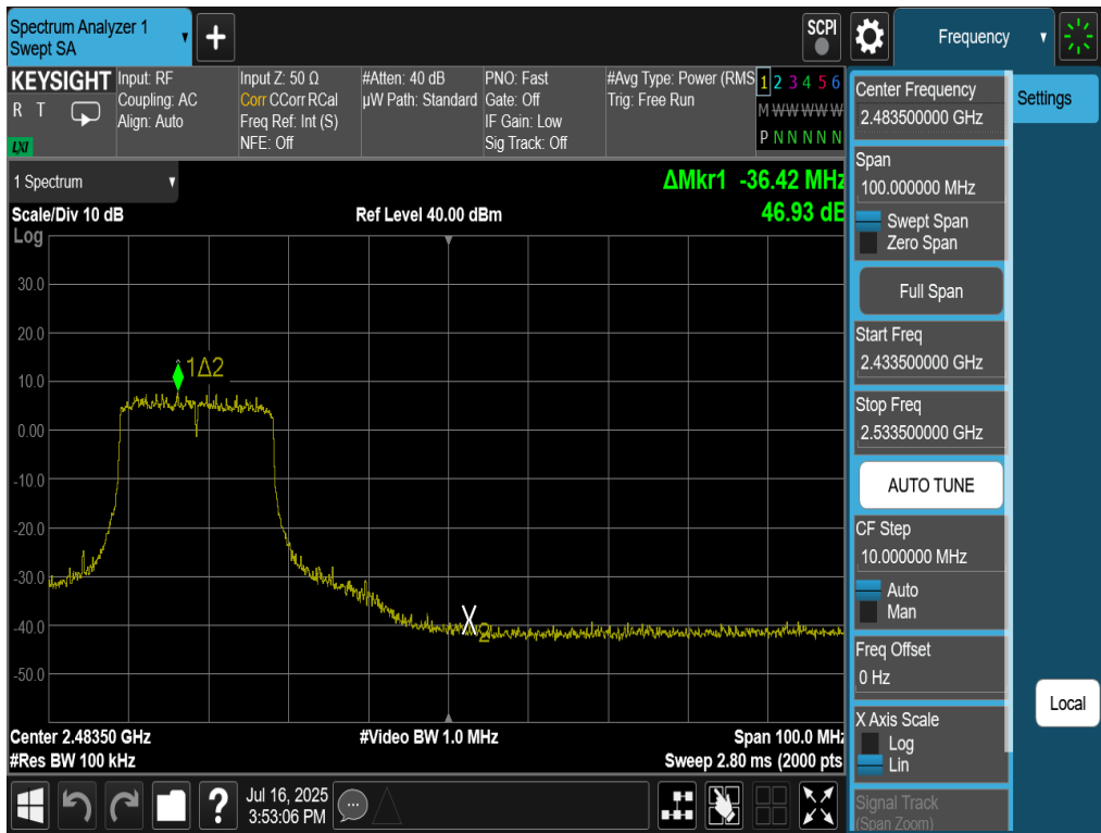
Plot 7-56. Band Edge Antenna 2a (802.11be OFDMA – RU242 – Ch. 9)
