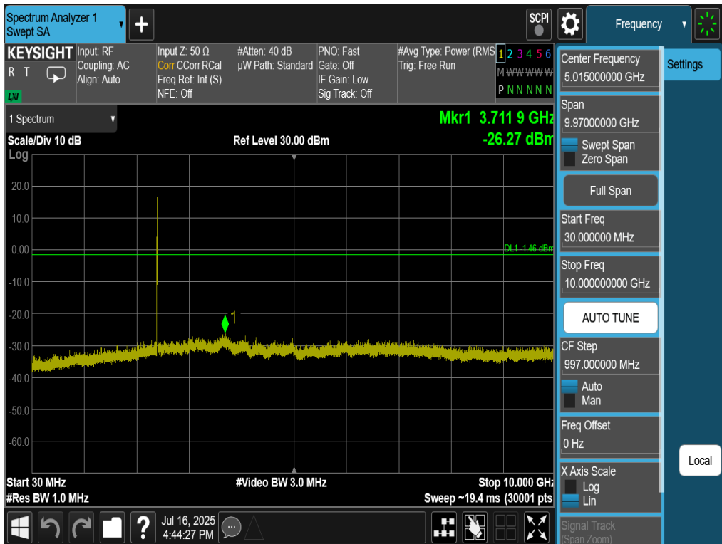
Plot 7-73. Conducted Spurious Plot Antenna 2a (802.11be OFDMA – RU26 – Ch. 1)
