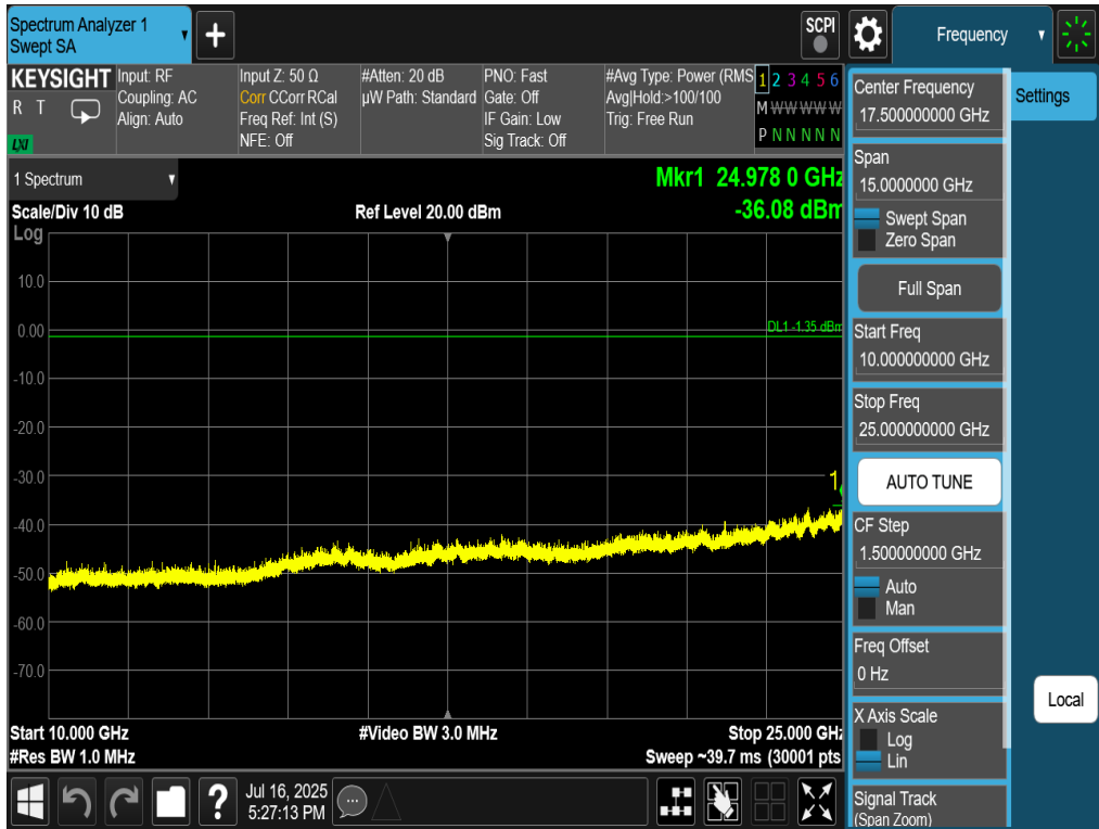
Plot 7-82. Conducted Spurious Plot Antenna 2a (802.11be OFDMA – RU242 – Ch. 6)
