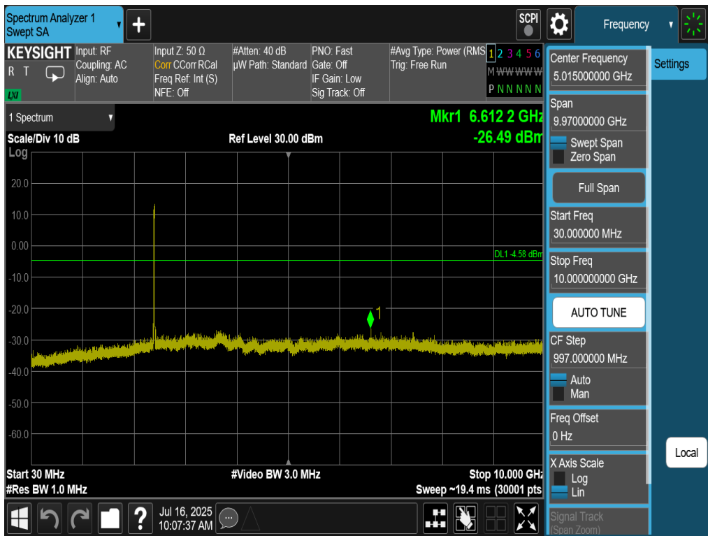
Plot 7-67. Conducted Spurious Plot Antenna 4a (802.11be OFDMA – RU242 – Ch. 1)
