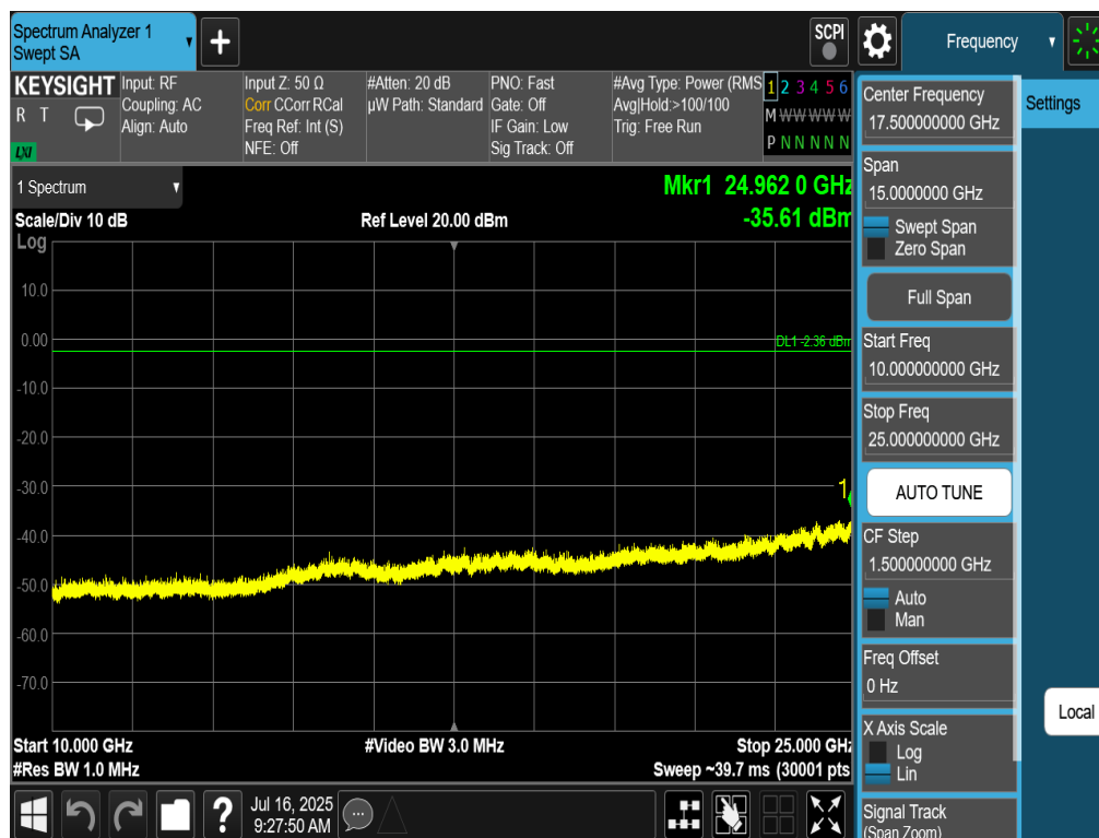
Plot 7-62. Conducted Spurious Plot Antenna 4a (802.11be OFDMA – RU26 – Ch. 1)
