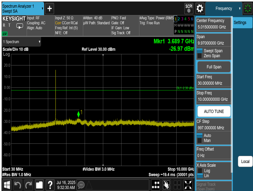
Plot 7-63. Conducted Spurious Plot Antenna 4a (802.11be OFDMA – RU26 – Ch. 6)
