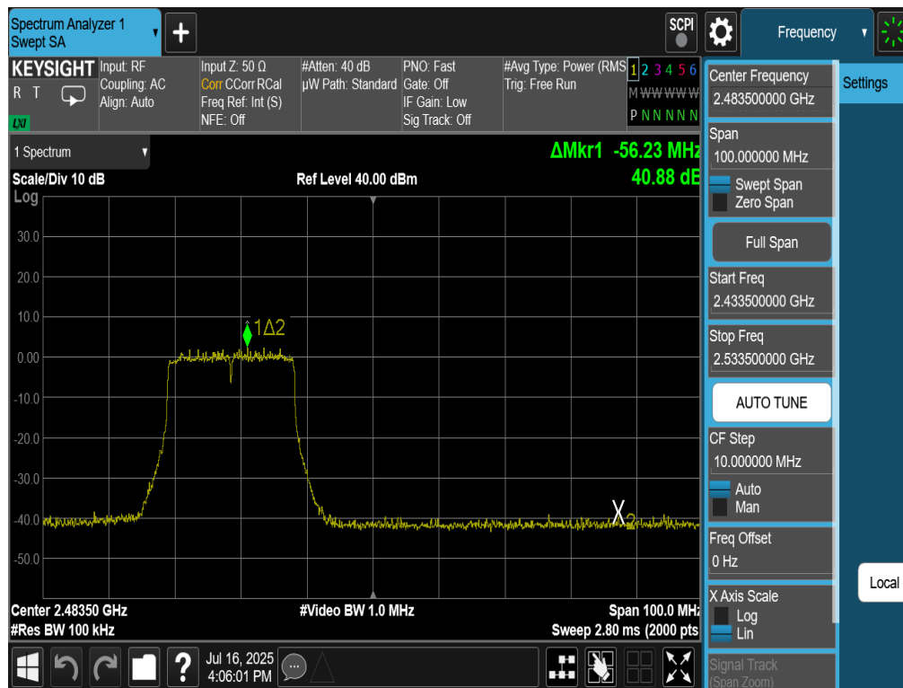
Plot 7-58. Band Edge Antenna 2a (802.11be OFDMA – RU242 – Ch. 11)
