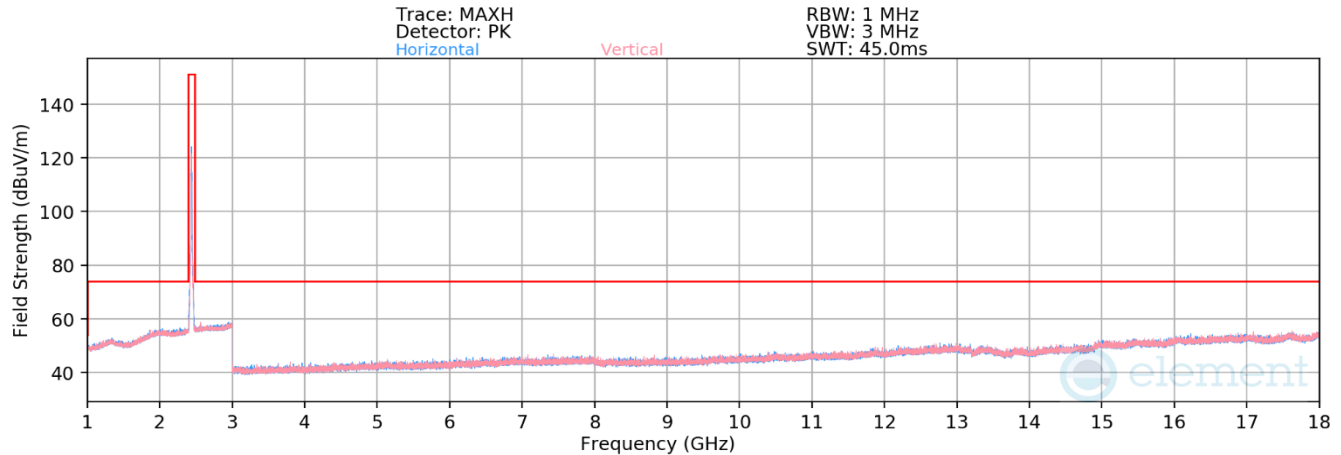
Plot 7-86. Radiated Spurious Emissions above 1GHz CDD (802.11be OFDMA – RU26 – Ch. 6)
