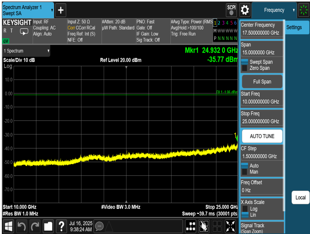
Plot 7-66. Conducted Spurious Plot Antenna 4a (802.11be OFDMA – RU26 – Ch. 11)
