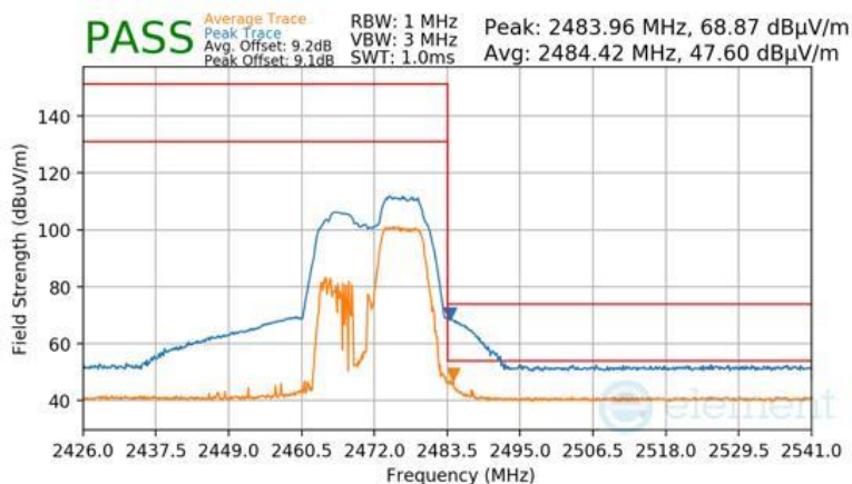
Plot 7-103 Radiated Restricted Upper Band Edge Measurement Antenna 4a (Peak & Average – RU52+26)
