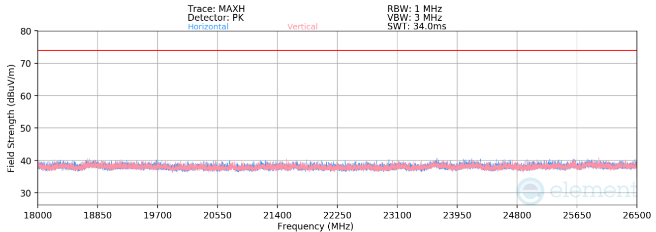
Plot 7-87. Radiated Spurious Emissions above 18GHz CDD (802.11be OFDMA – RU26 – Ch. 6)
