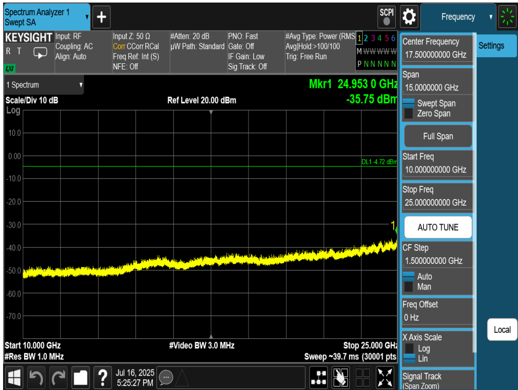
Plot 7-80. Conducted Spurious Plot Antenna 2a (802.11be OFDMA – RU242 – Ch. 1)
