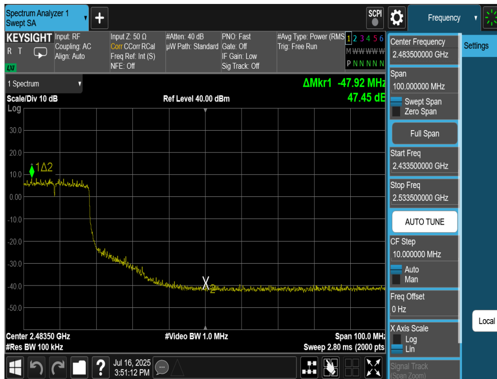
Plot 7-54. Band Edge Antenna 2a (802.11be OFDMA – RU242 – Ch. 7)
