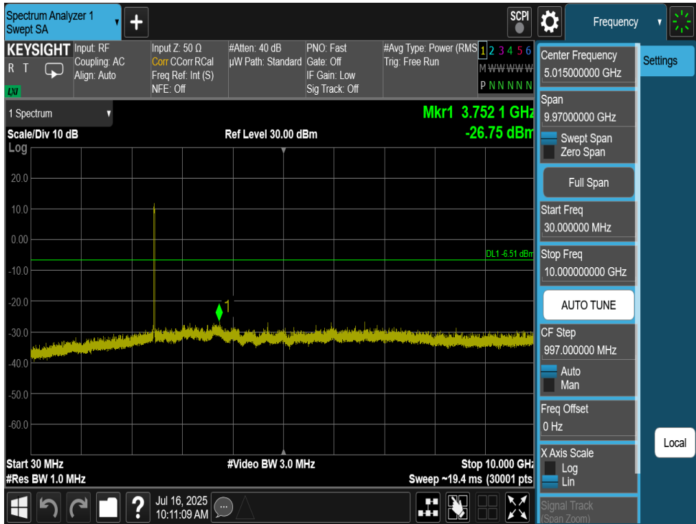
Plot 7-71. Conducted Spurious Plot Antenna 4a (802.11be OFDMA – RU242 – Ch. 11)
