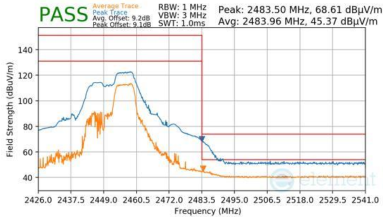
Plot 7-99 Radiated Restricted Upper Band Edge Measurement Antenna 4a (Peak & Average – RU52+26)
