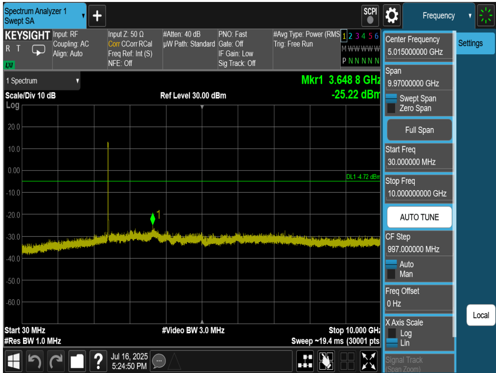
Plot 7-79. Conducted Spurious Plot Antenna 2a (802.11be OFDMA – RU242 – Ch. 1)
