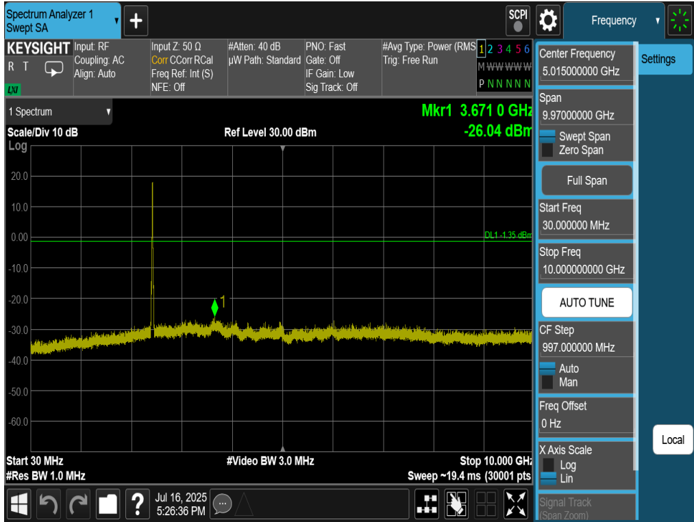
Plot 7-81. Conducted Spurious Plot Antenna 2a (802.11be OFDMA – RU242 – Ch. 6)
