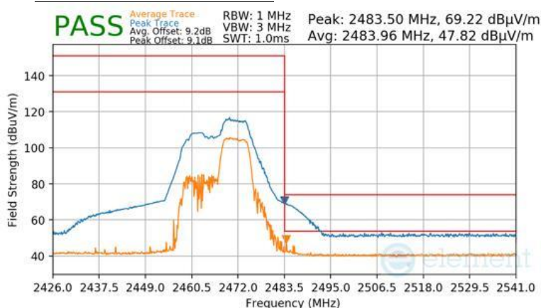
Plot 7-102 Radiated Restricted Upper Band Edge Measurement Antenna 4a (Peak & Average – RU52+26)
