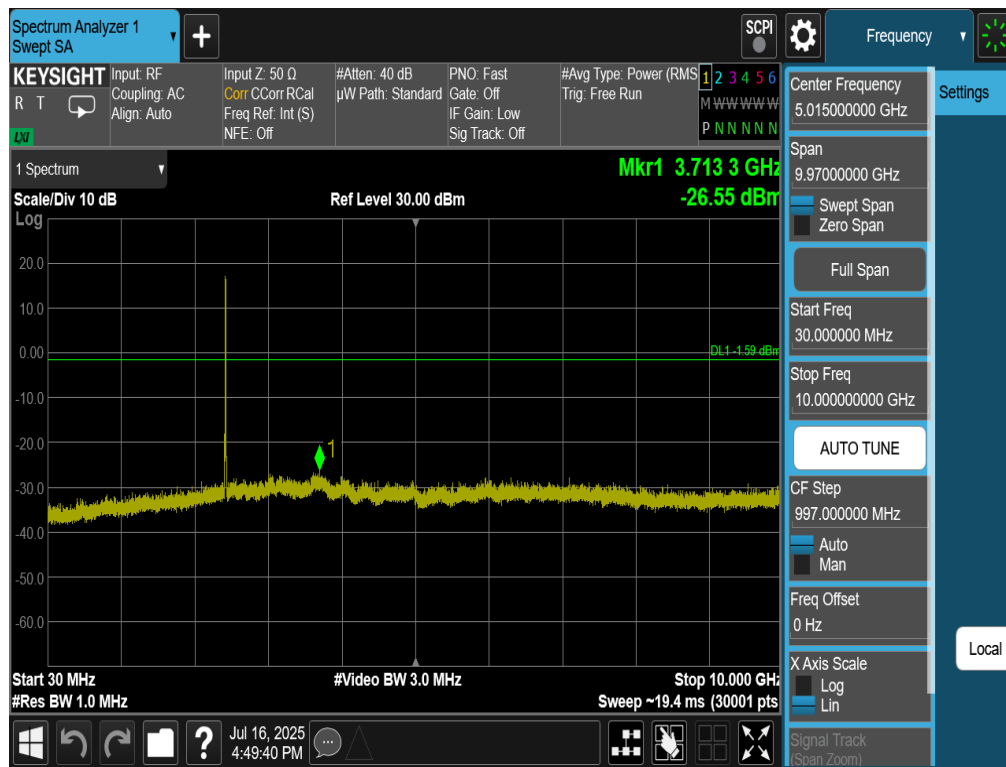
Plot 7-75. Conducted Spurious Plot Antenna 2a (802.11be OFDMA – RU26 – Ch. 6)
