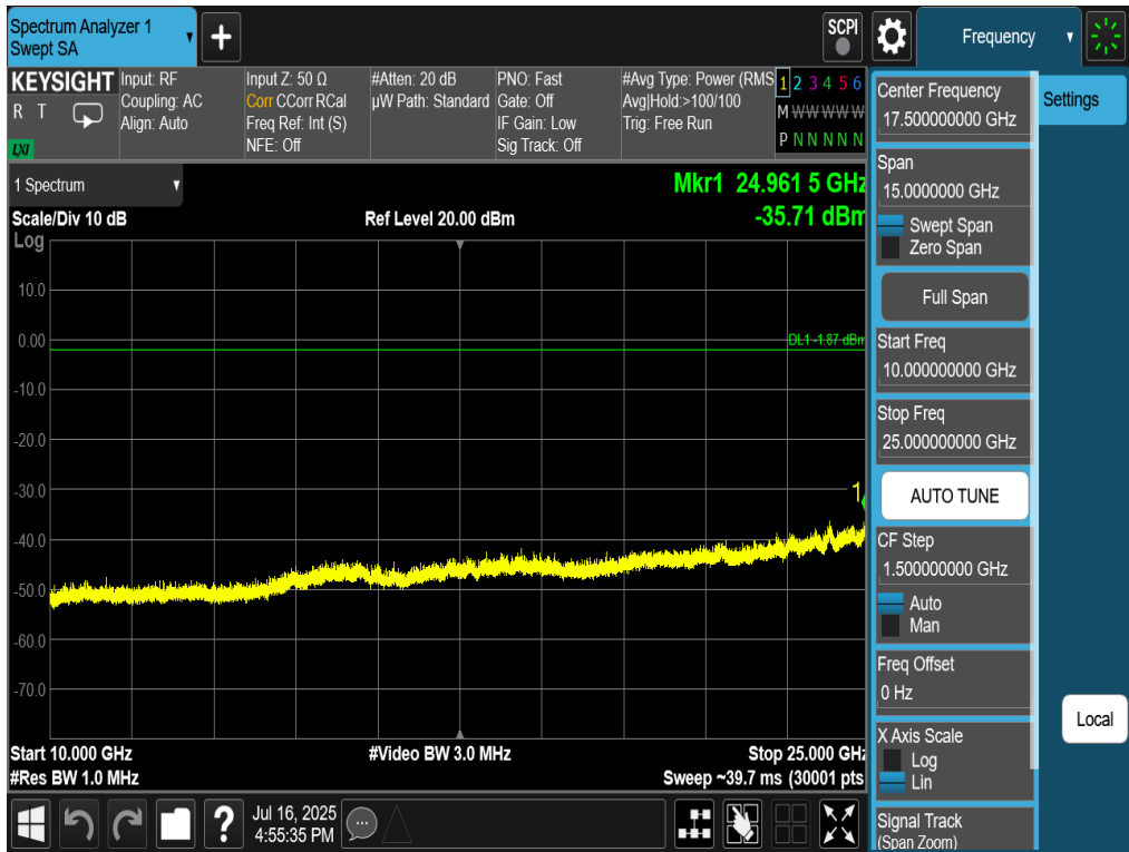
Plot 7-78. Conducted Spurious Plot Antenna 2a (802.11be OFDMA – RU26 – Ch. 11)
