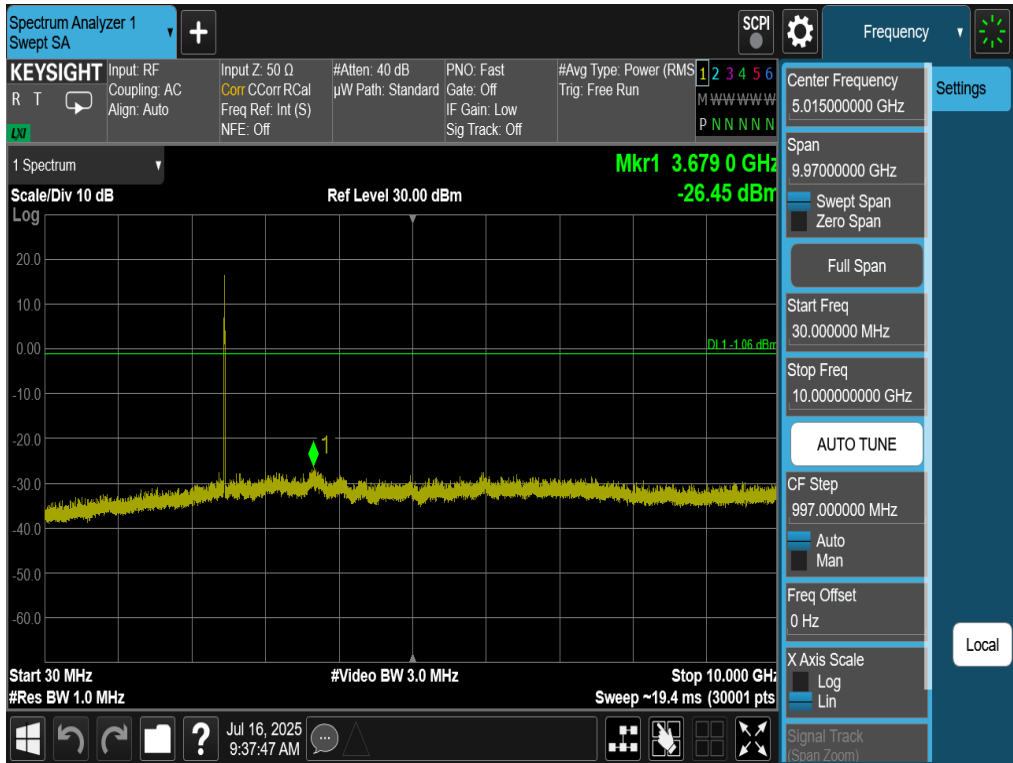
Plot 7-65. Conducted Spurious Plot Antenna 4a (802.11be OFDMA – RU26 – Ch. 11)
