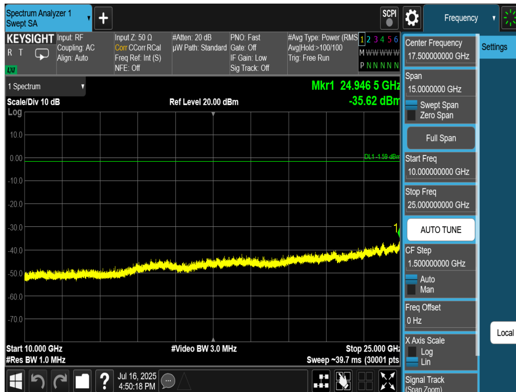
Plot 7-76. Conducted Spurious Plot Antenna 2a (802.11be OFDMA – RU26 – Ch. 6)
