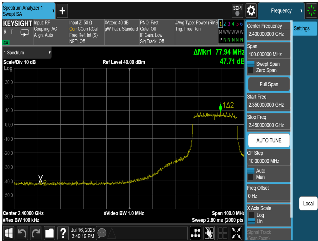
Plot 7-52. Band Edge Antenna 2a (802.11be OFDMA – RU242 – Ch. 6(Low Channel))
