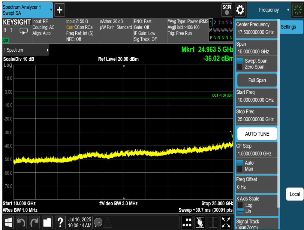
Plot 7-68. Conducted Spurious Plot Antenna 4a (802.11be OFDMA – RU242 – Ch. 1)
