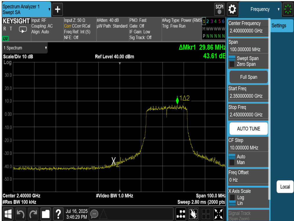
Plot 7-49. Band Edge Antenna 2a (802.11be OFDMA – RU242 – Ch. 3)
