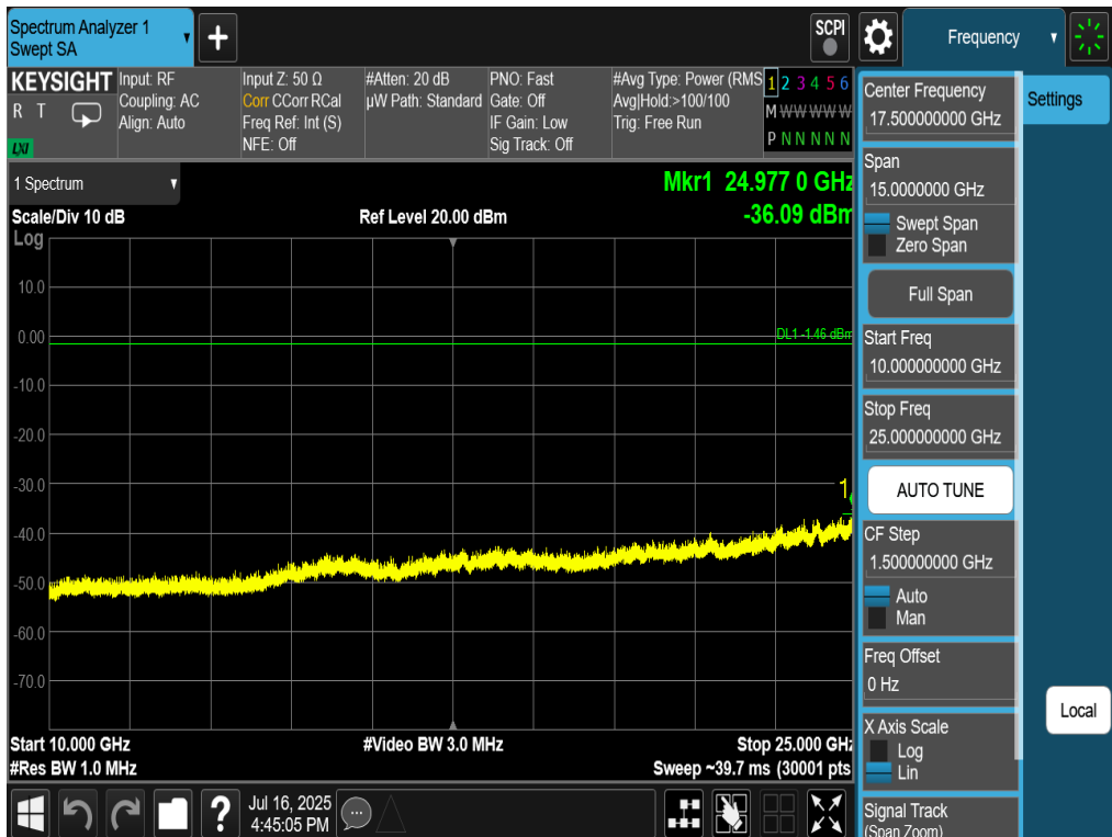
Plot 7-74. Conducted Spurious Plot Antenna 2a (802.11be OFDMA – RU26 – Ch. 1)
