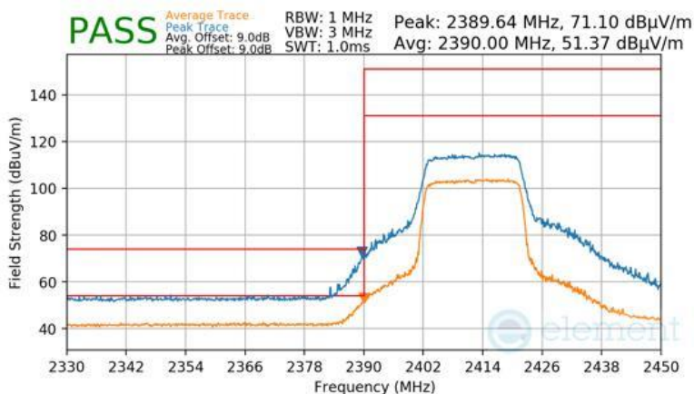
Plot 7-104 Radiated Restricted Lower Band Edge Measurement Antenna 4a (Peak & Average – RU242)
