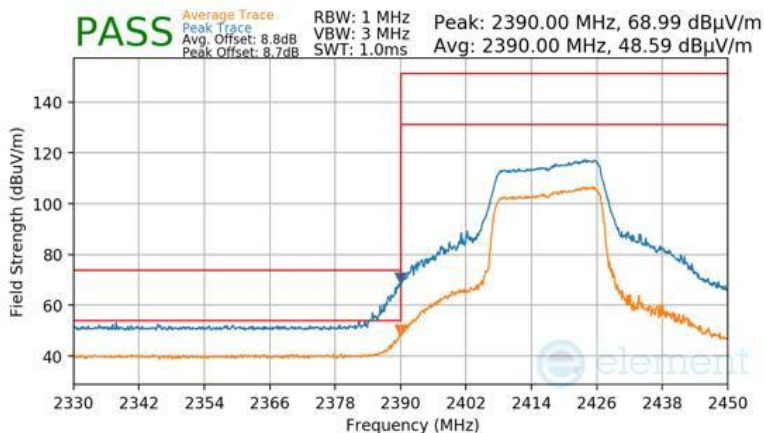
Plot 7-105 Radiated Restricted Lower Band Edge Measurement Antenna 4a (Peak & Average – RU242)
