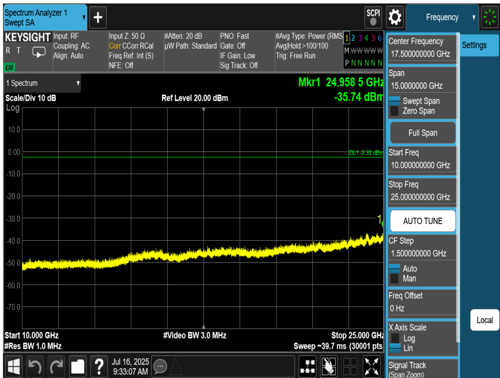
Plot 7-64. Conducted Spurious Plot Antenna 4a (802.11be OFDMA – RU26 – Ch. 6)
