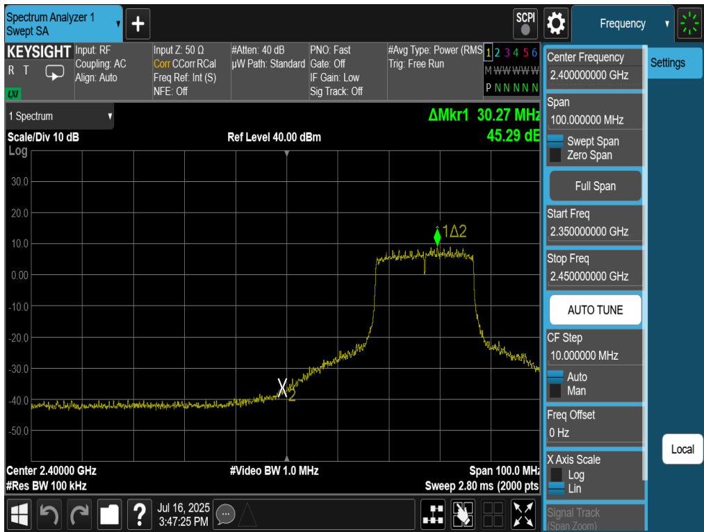
Plot 7-50. Band Edge Antenna 2a (802.11be OFDMA – RU242 – Ch. 4)
