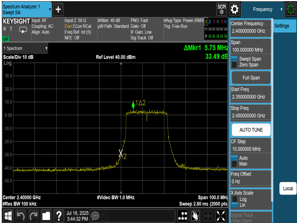
Plot 7-47. Band Edge Antenna 2a (802.11be OFDMA – RU242 – Ch. 1)
