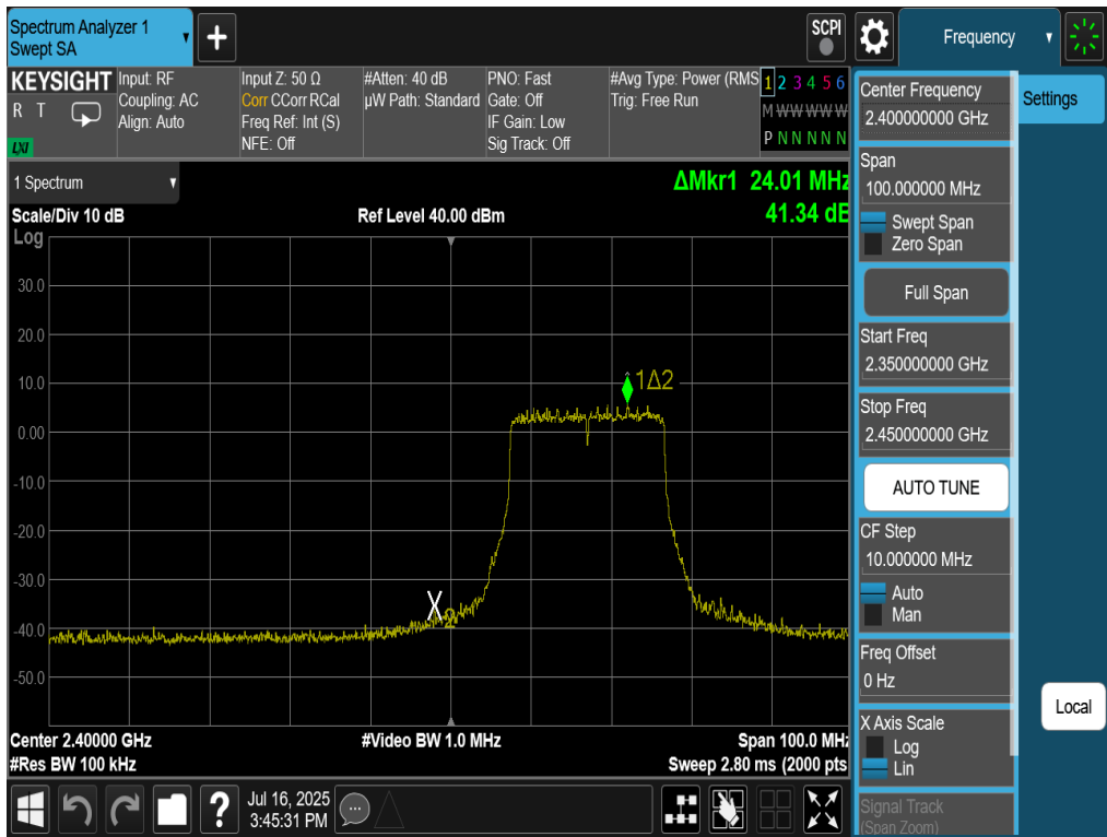
Plot 7-48. Band Edge Antenna 2a (802.11be OFDMA – RU242 – Ch. 2)
