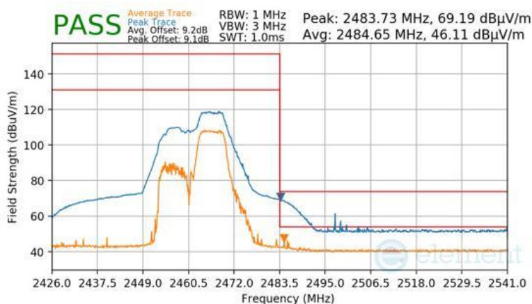
Plot 7-101 Radiated Restricted Upper Band Edge Measurement Antenna 4a (Peak & Average – RU52+26)
