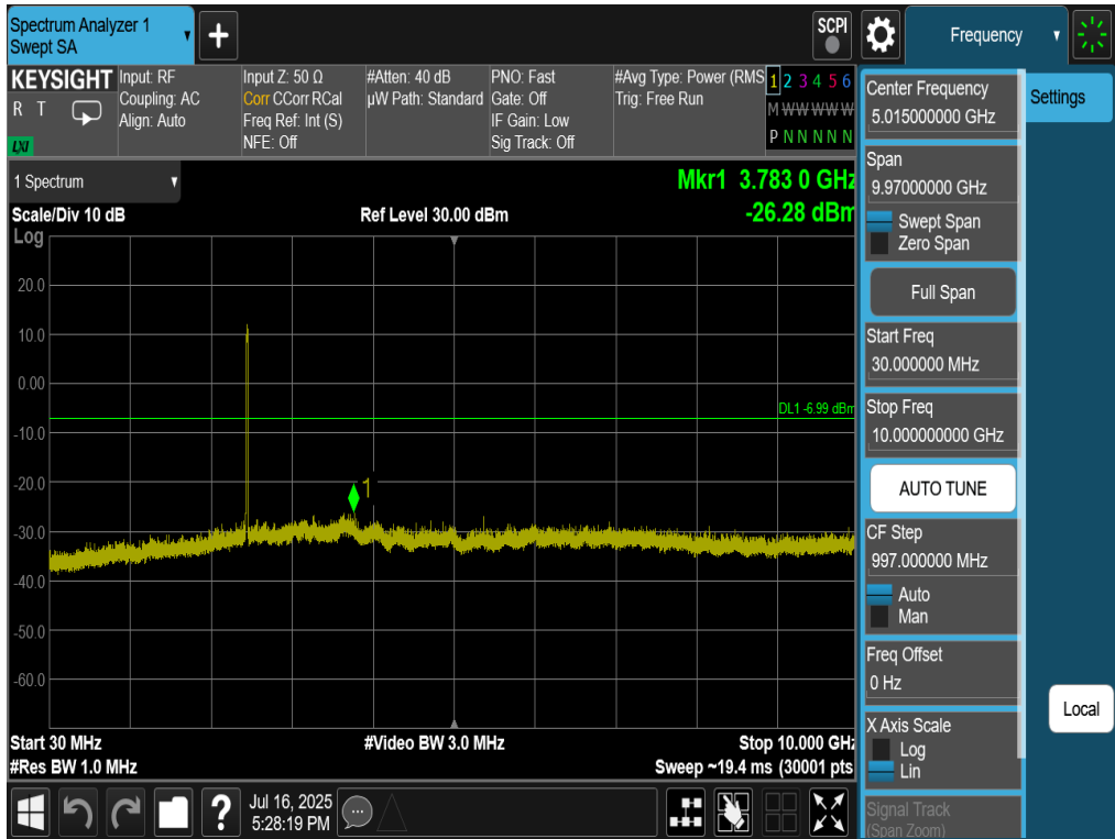
Plot 7-83. Conducted Spurious Plot Antenna 2a (802.11be OFDMA – RU242 – Ch. 11)
