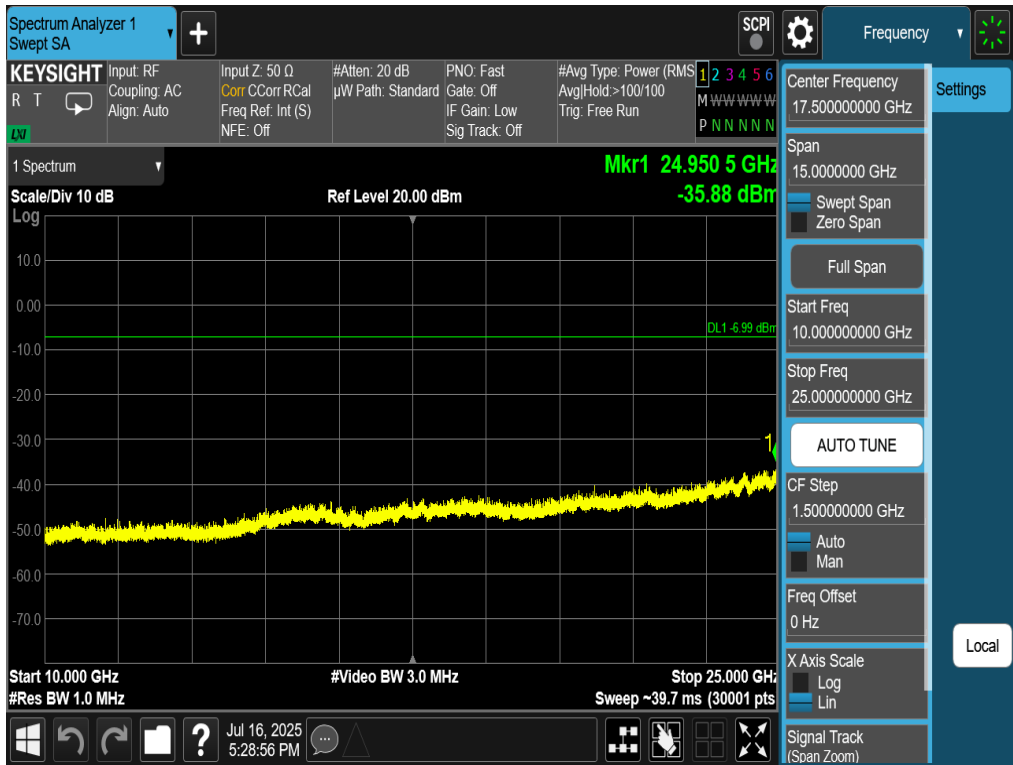
Plot 7-84. Conducted Spurious Plot Antenna 2a (802.11be OFDMA – RU242 – Ch. 11)
