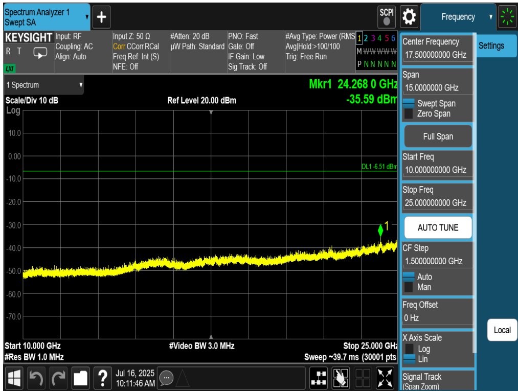
Plot 7-72. Conducted Spurious Plot Antenna 4a (802.11be OFDMA – RU242 – Ch. 11)
