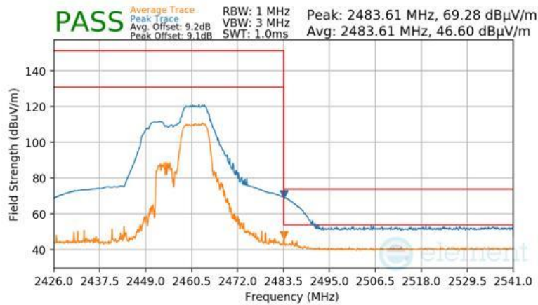
Plot 7-100 Radiated Restricted Upper Band Edge Measurement Antenna 4a (Peak & Average – RU52+26)
