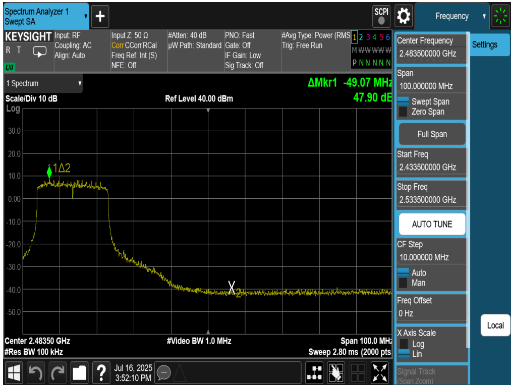
Plot 7-55. Band Edge Antenna 2a (802.11be OFDMA – RU242 – Ch. 8)
