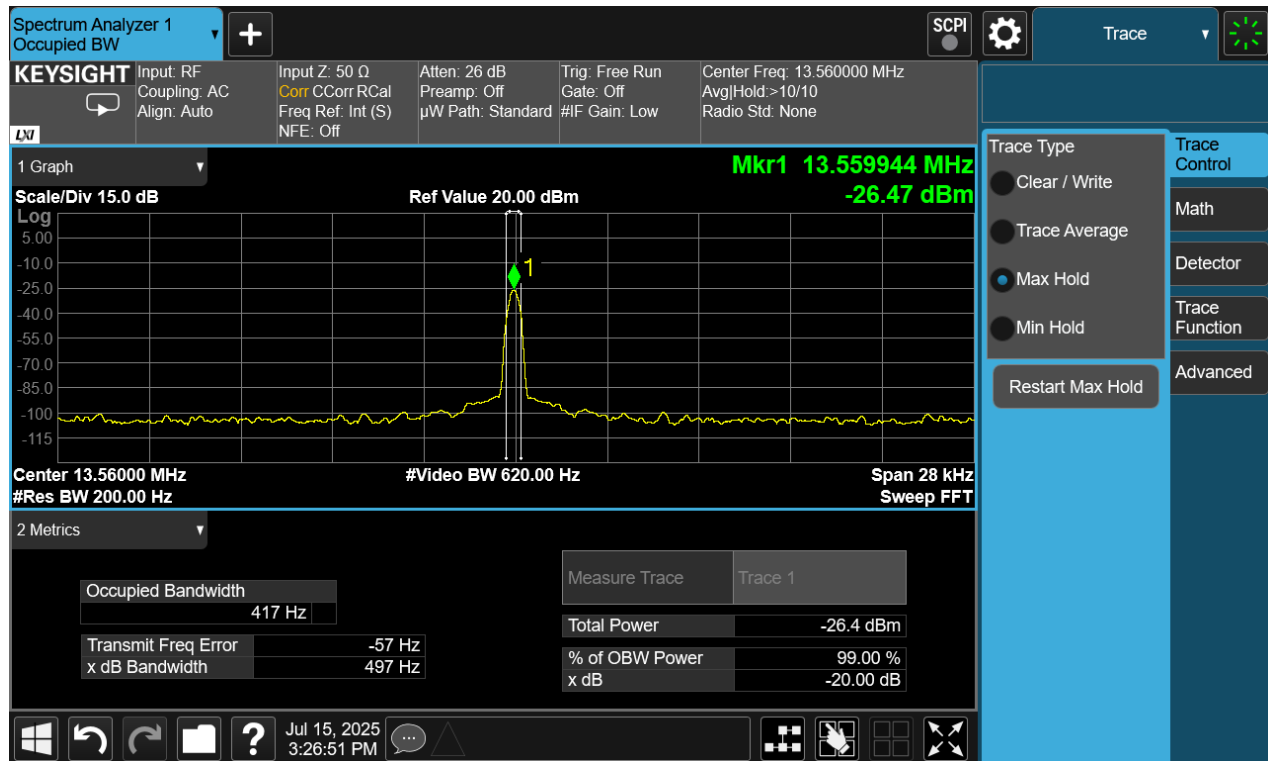
Figure 7-2. 20dB and 99% Bandwidth WPT Plot (Charging Rate 2.6C)
