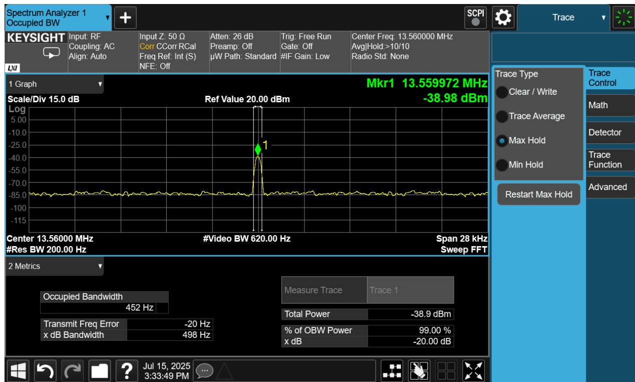
Figure 7-3. 20dB and 99% Bandwidth Communication Mode Plot
