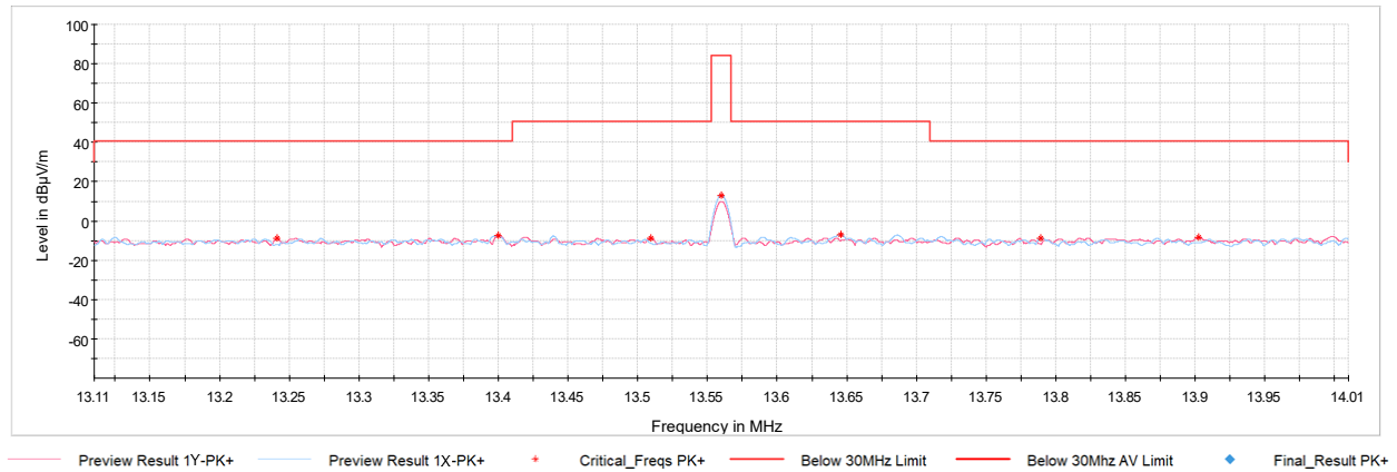
Plot 7-1. In Band Radiated Spurious Emissions (Charging Rate 2.6C, with AC/DC Adapter)
