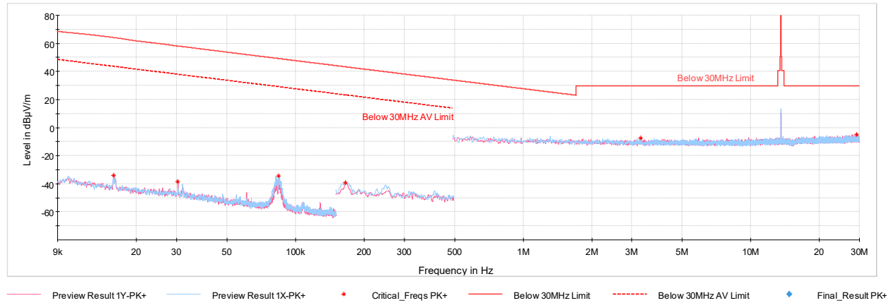
Plot 7-2. Radiated Spurious Plot 9kHz – 30MHz (Charging Rate 2.6C, with AC/DC Adapter)
