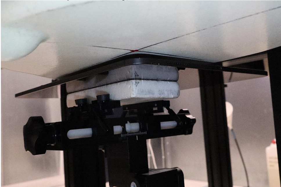
SAR Test Setup Photo 4: Body, Back Side at 5mm– Antenna 2a/WF5b
