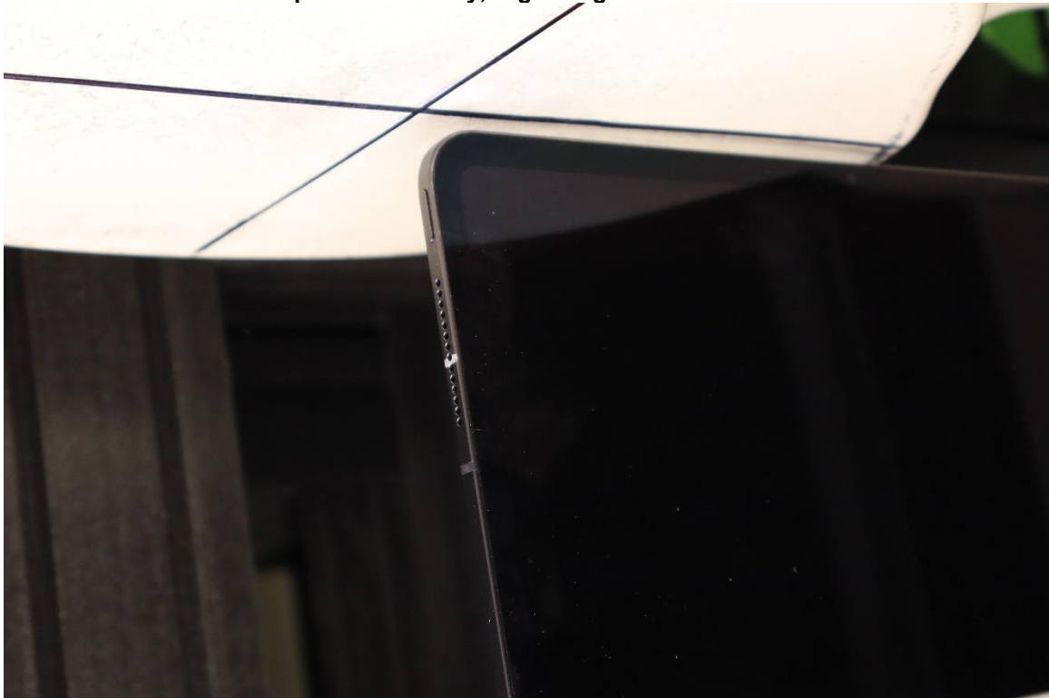
SAR Test Setup Photo 9: Body, Right Edge at 5mm – Antenna 3/4a/4b
