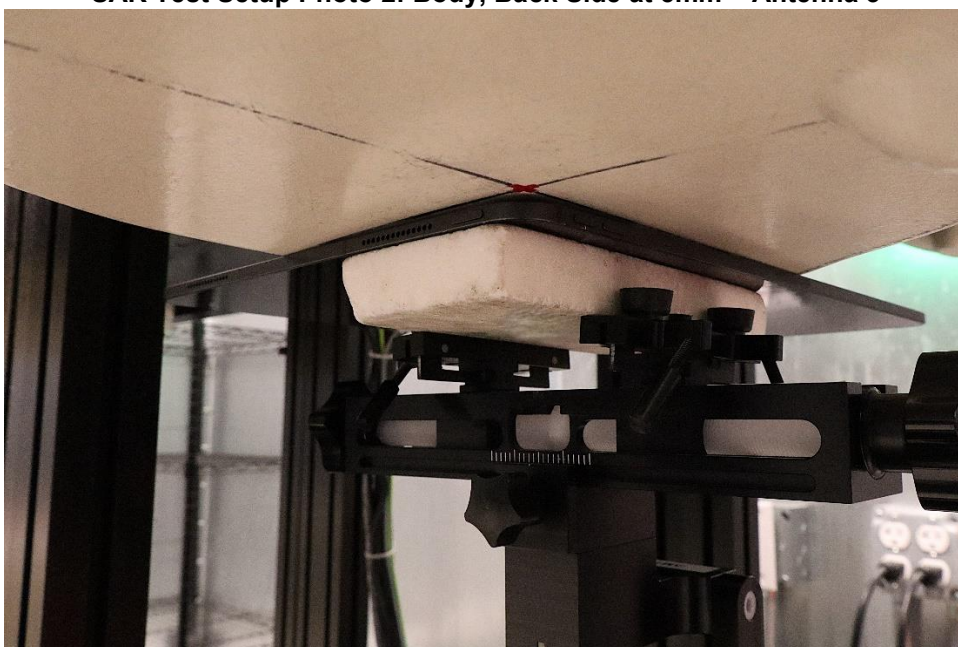
SAR Test Setup Photo 2: Body, Back Side at 5mm – Antenna 3
