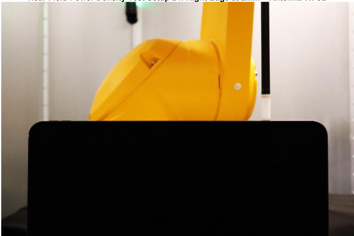
Near Field Power Density Test Setup 24: Right Edge at 2mm – Antenna WF5B
