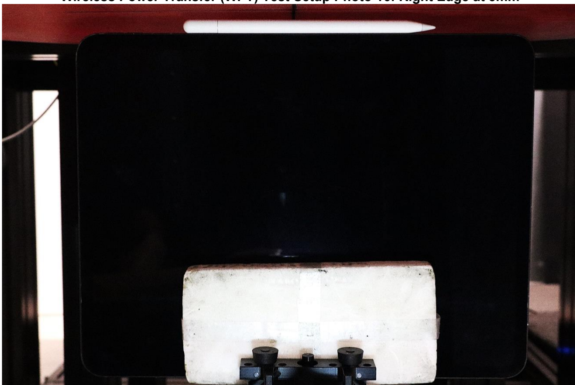
Wireless Power Transfer (WPT) Test Setup Photo 16: Right Edge at 5mm
