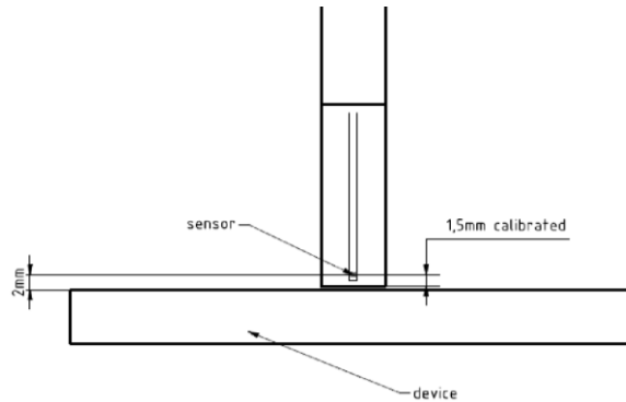
Figure K-2 EUMmWVx Probe
