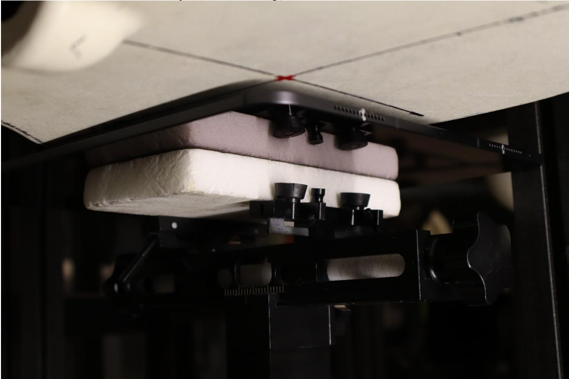
SAR Test Setup Photo 5: Body, Back Side at 5mm– Antenna 4a
