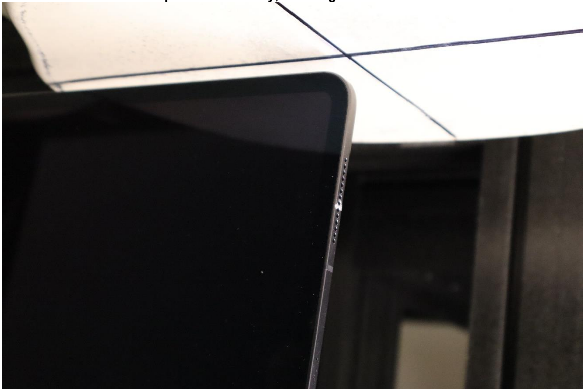
SAR Test Setup Photo 12: Body, Left Edge at 5mm – Antenna 1/2a/2b/WF5B
