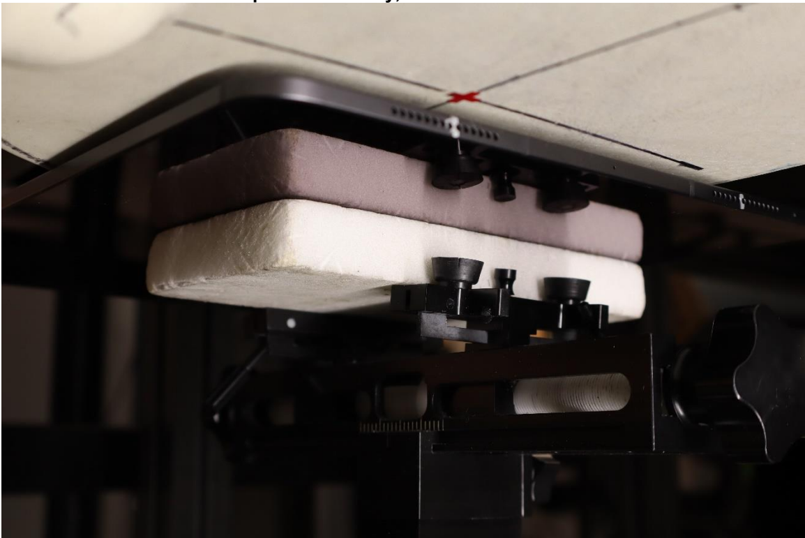
SAR Test Setup Photo 6: Body, Back Side at 5mm– Antenna 4b
