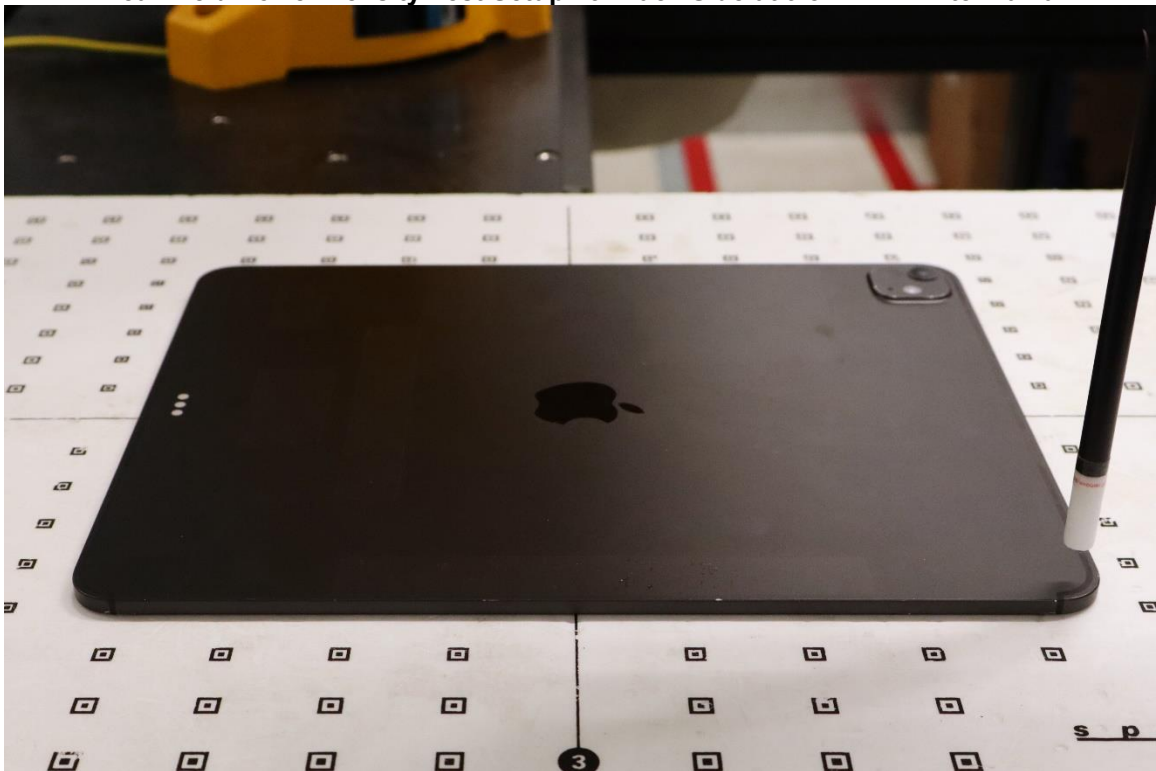
Near Field Power Density Test Setup 23: Back Side at 9.82mm – Antenna 4a
