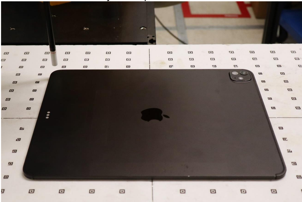
Near Field Power Density Test Setup 20: Back Side at 9.95mm – Antenna 2a
