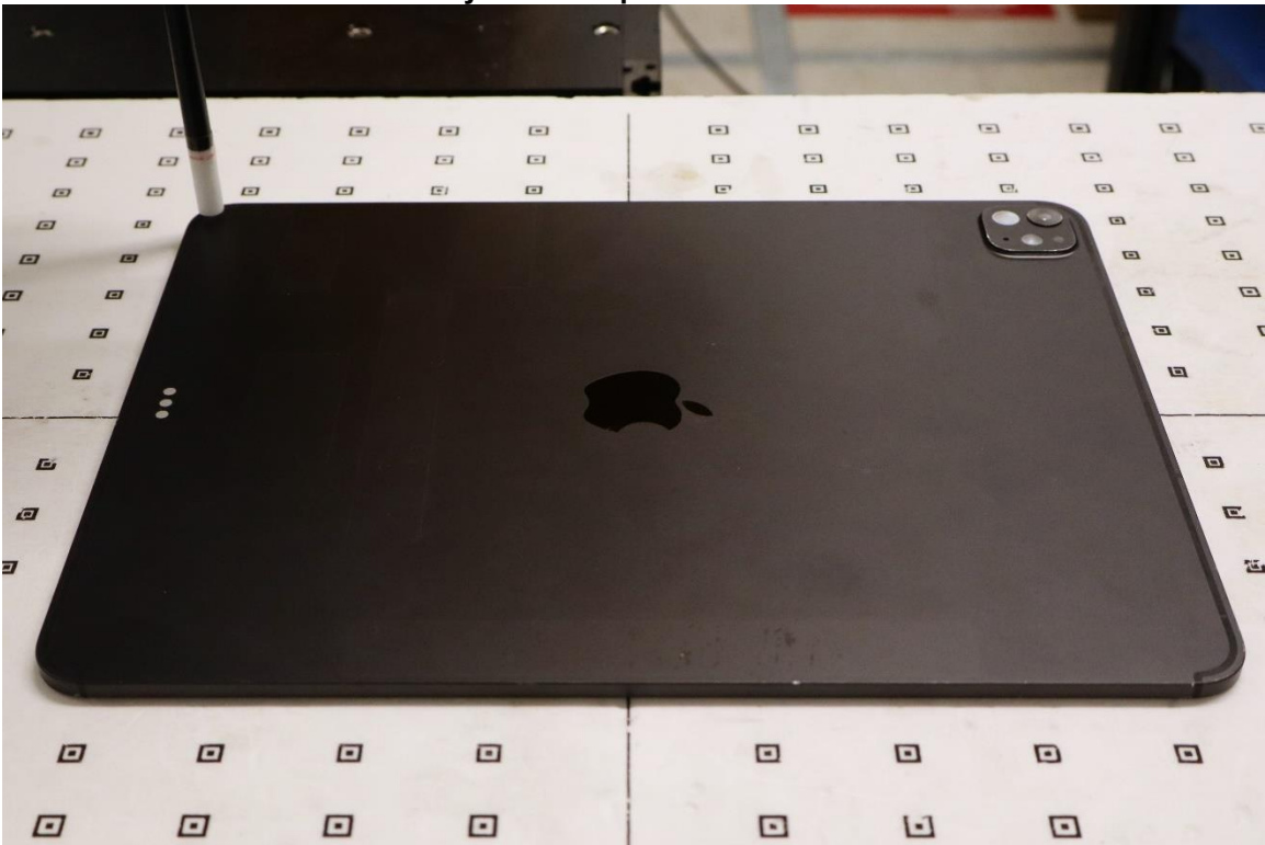
Near Field Power Density Test Setup 18: Back Side at 2mm – Antenna 2a
