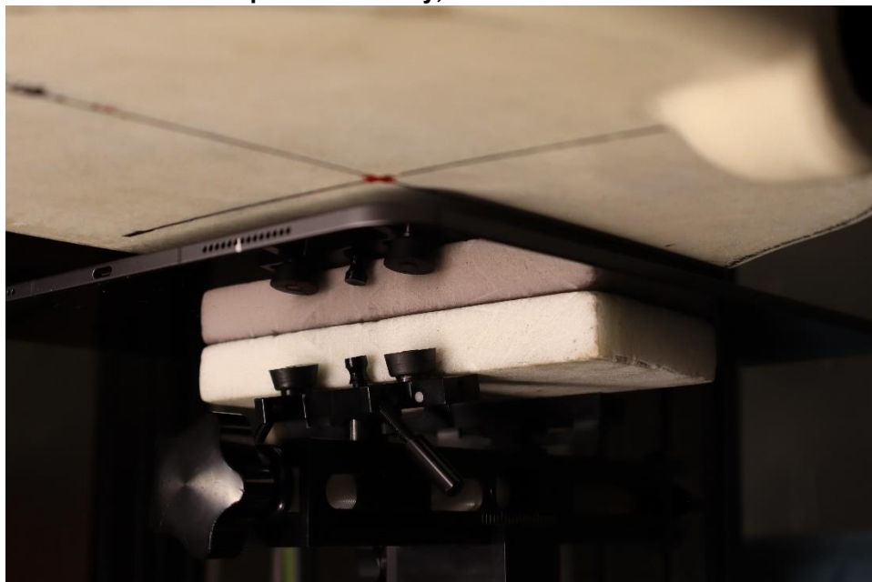
SAR Test Setup Photo 1: Body, Back Side at 5mm – Antenna 1
