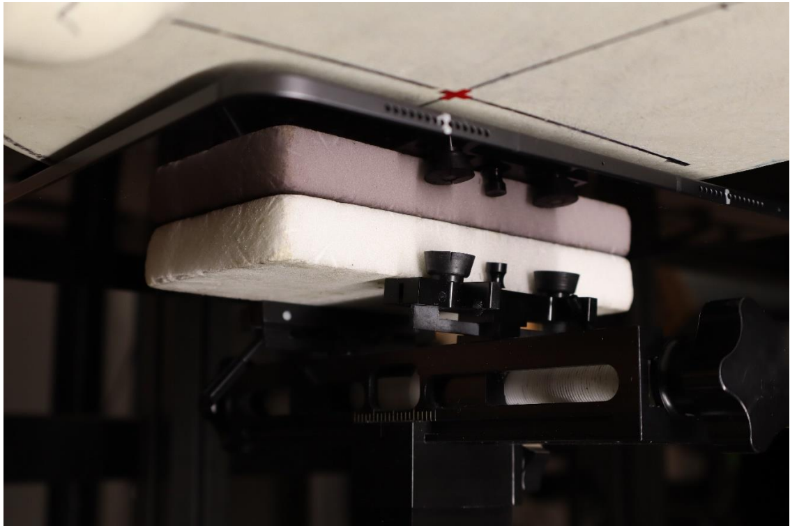
Test Setup Photo 8 – Body, Back Side at 5mm – Antenna 4b
