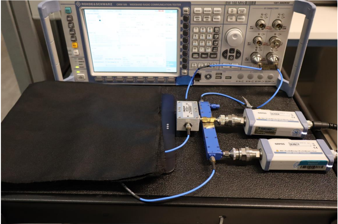
Test Setup Photo 5 – Conducted Test Setup (Figure 6-1d)
