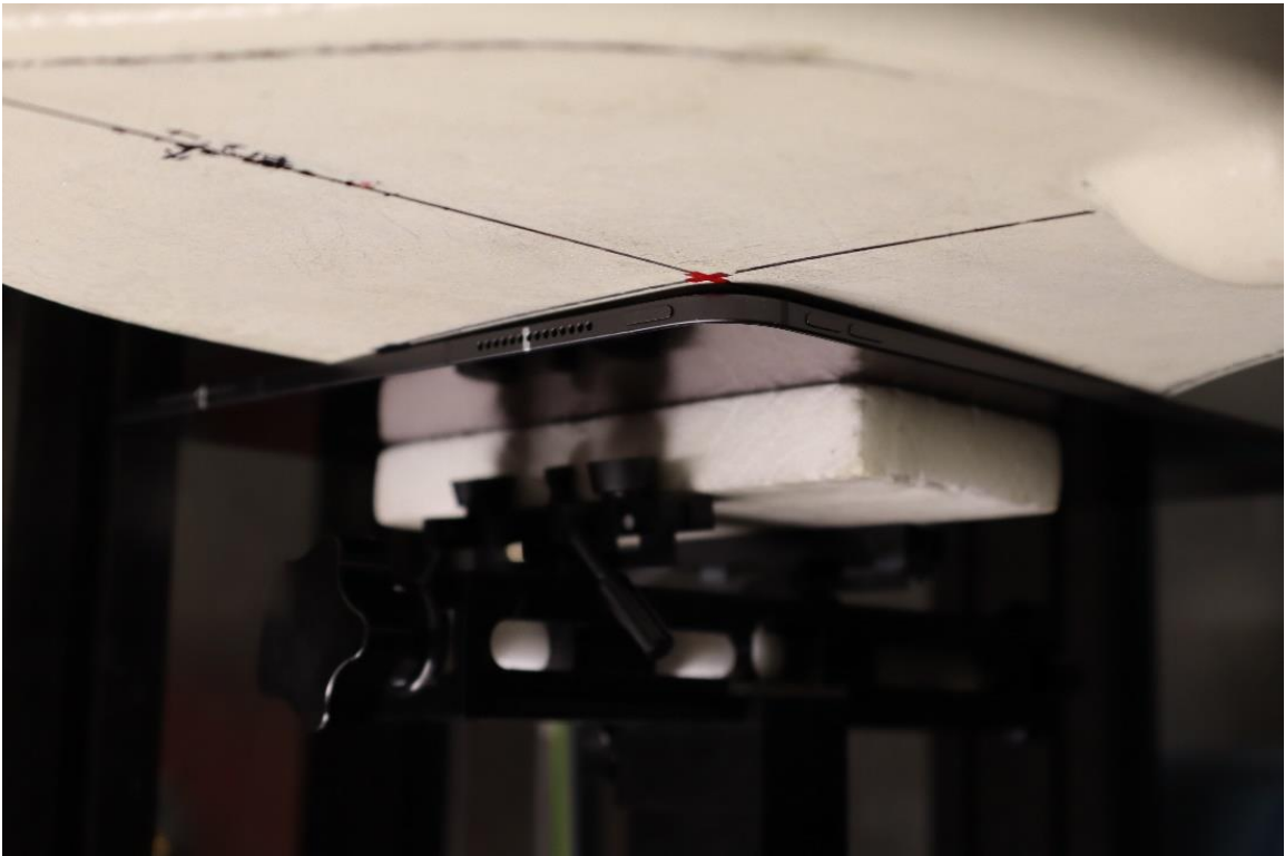
Test Setup Photo 9 – Body, Back Side at 5mm – Antenna 3
