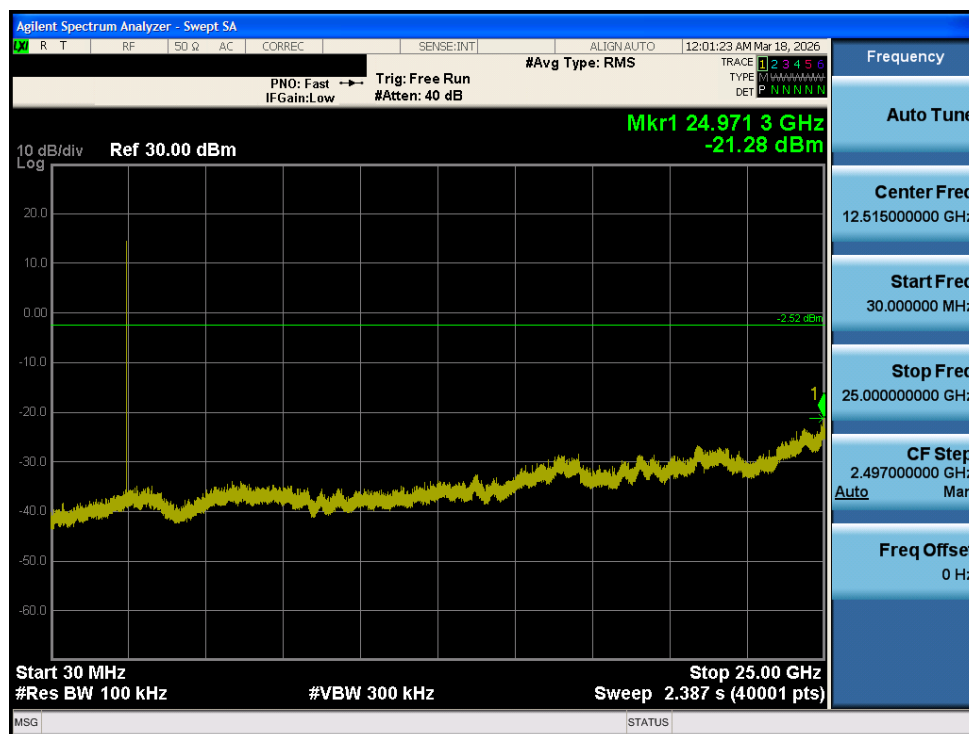
Plot 7-25. Conducted Spurious Antenna 1 Dedicated (802.15.4, ePA – Ch. 25)
