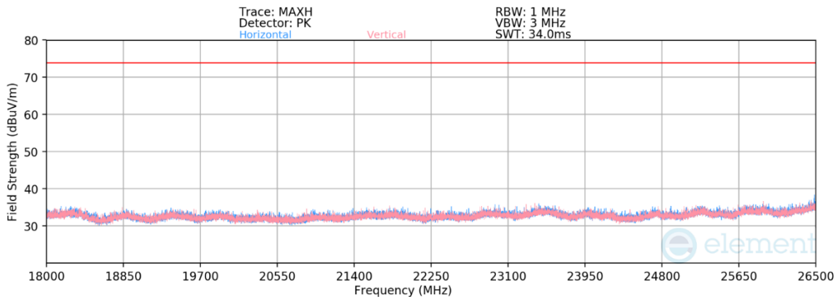
Plot 7-31. Radiated Spurious Emissions Above 18GHz Antenna 1 Dedicated (802.15.4 ePA – Ch. 18)
