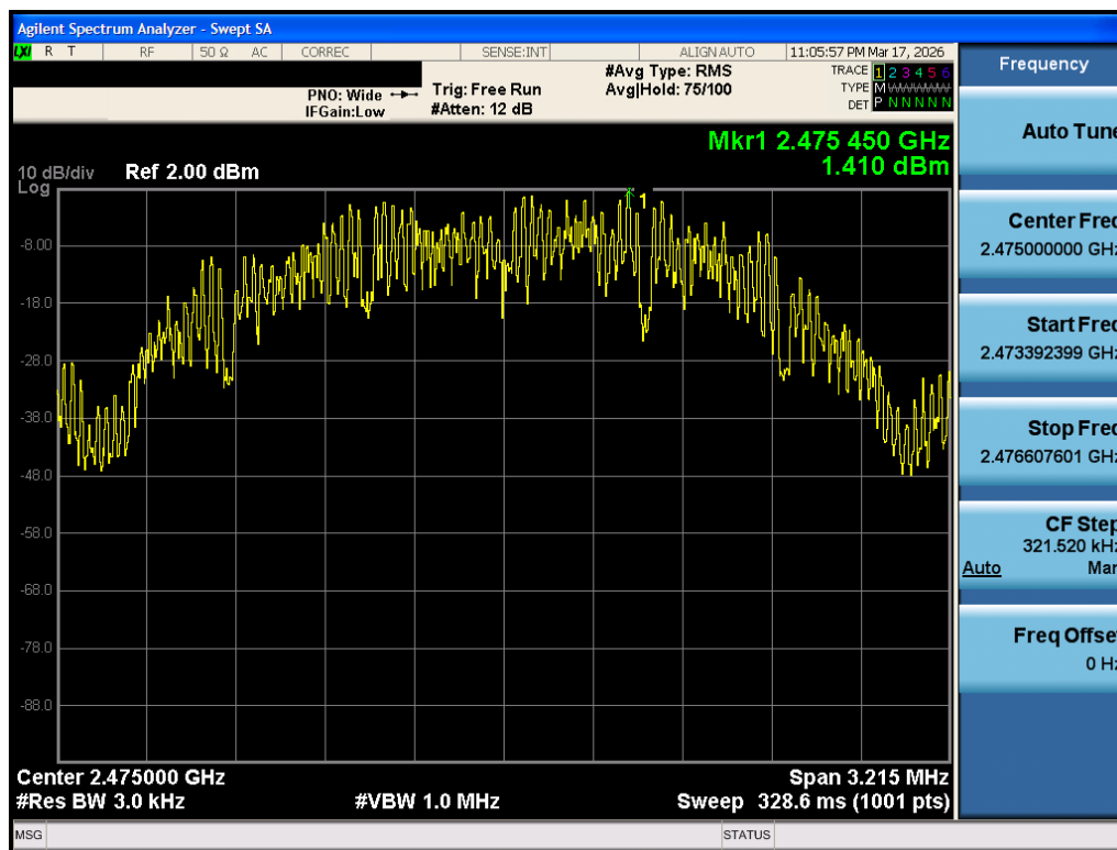
Plot 7-18. Power Spectral Density Antenna 1 Common (802.15.4, ePA – Ch. 25)
