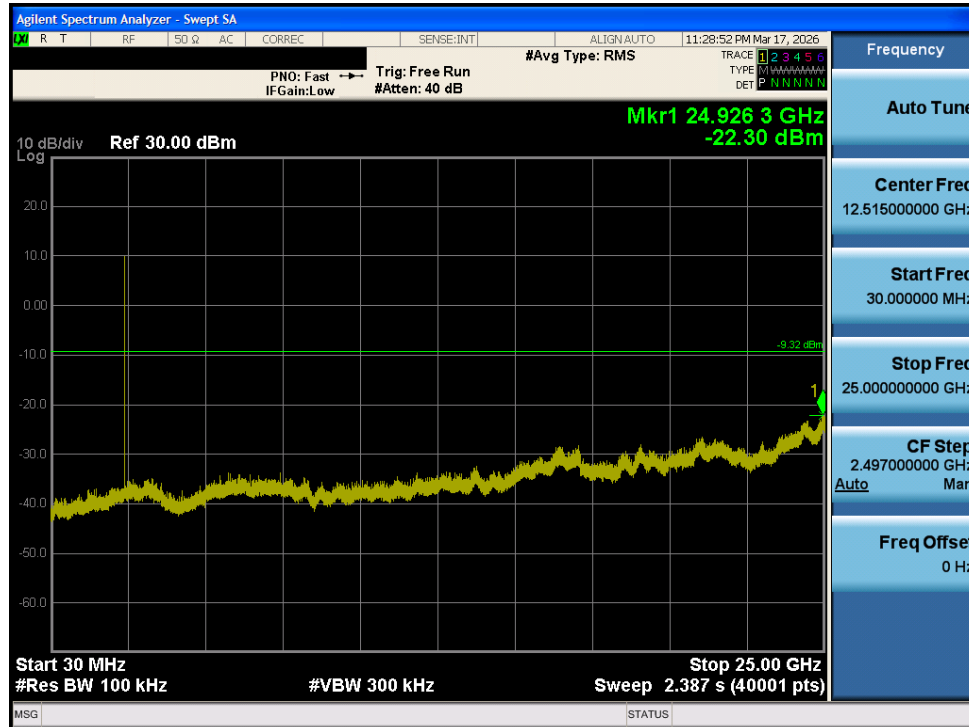
Plot 7-26. Conducted Spurious Antenna 1 Common (802.15.4, ePA – Ch. 11)
