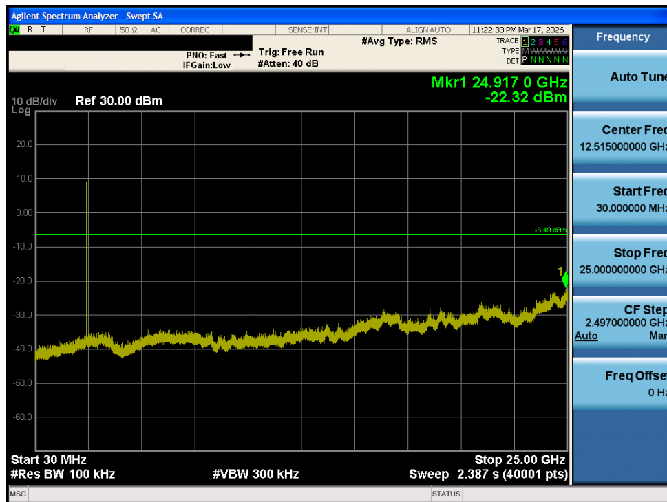
Plot 7-27. Conducted Spurious Antenna 1 Common (802.15.4, ePA – Ch. 18)
