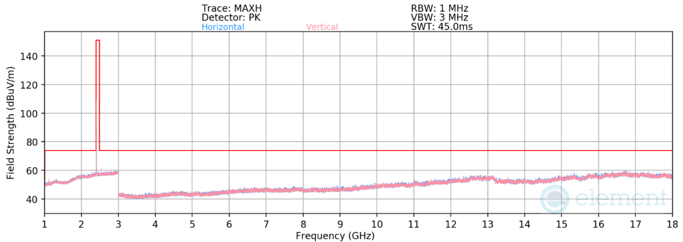
Plot 7-33. Radiated Spurious Emissions 1-18GHz Antenna 1 Common (802.15.4 ePA – Ch. 11)
