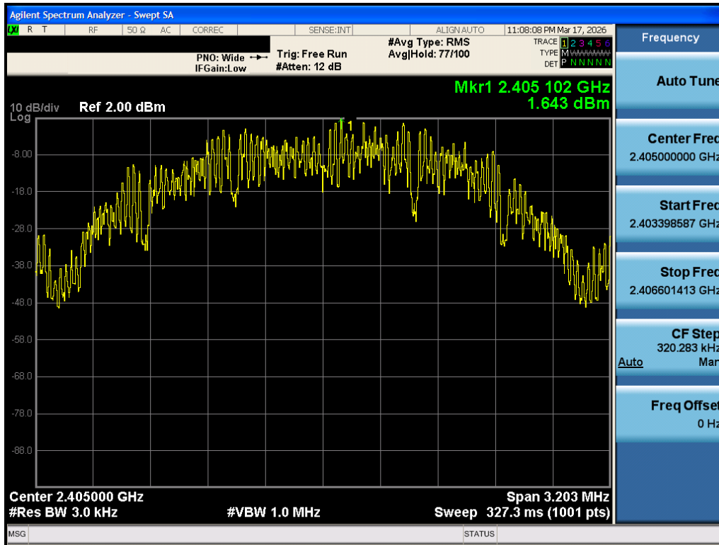
Plot 7-16. Power Spectral Density Antenna 1 Common (802.15.4, ePA – Ch. 11)
