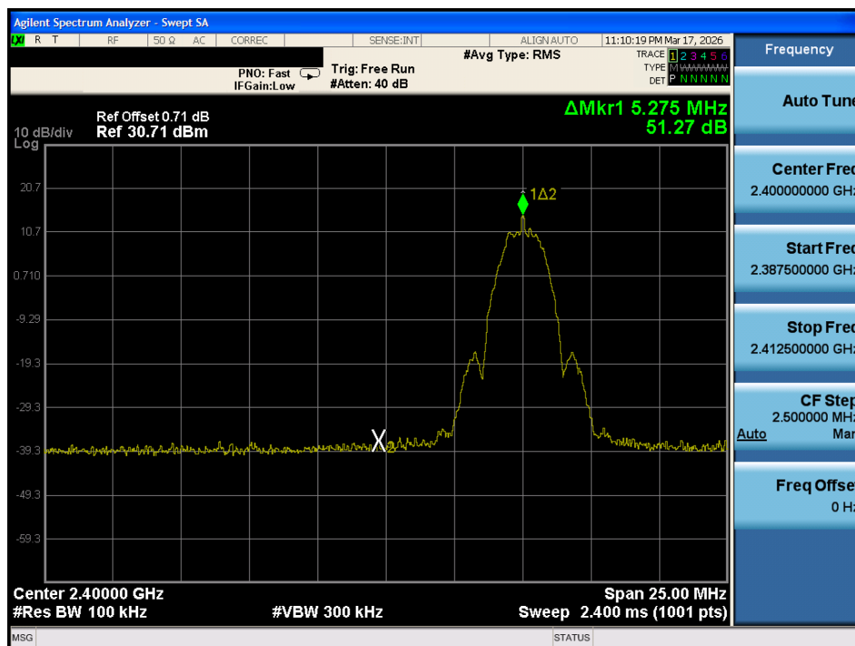
Plot 7-21. Band Edge Antenna 1 Common (802.15.4, ePA – Ch. 11)
