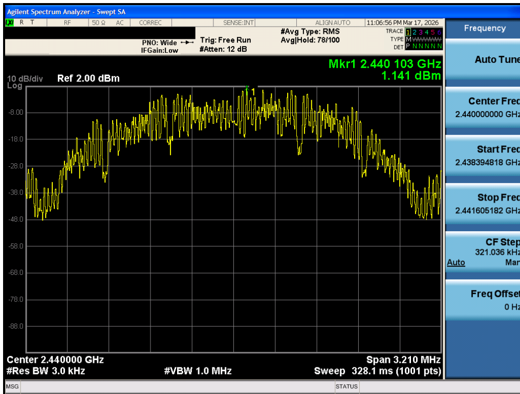
Plot 7-17. Power Spectral Density Antenna 1 Common (802.15.4, ePA – Ch. 18)
