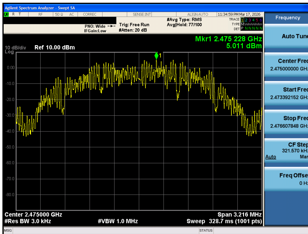
Plot 7-15. Power Spectral Density Antenna 1 Dedicated (802.15.4, ePA – Ch. 25)
