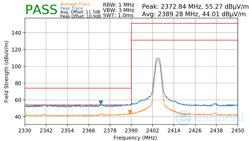
Plot 7-39. Radiated Restricted Lower Band Edge Measurement Antenna 1 Common
