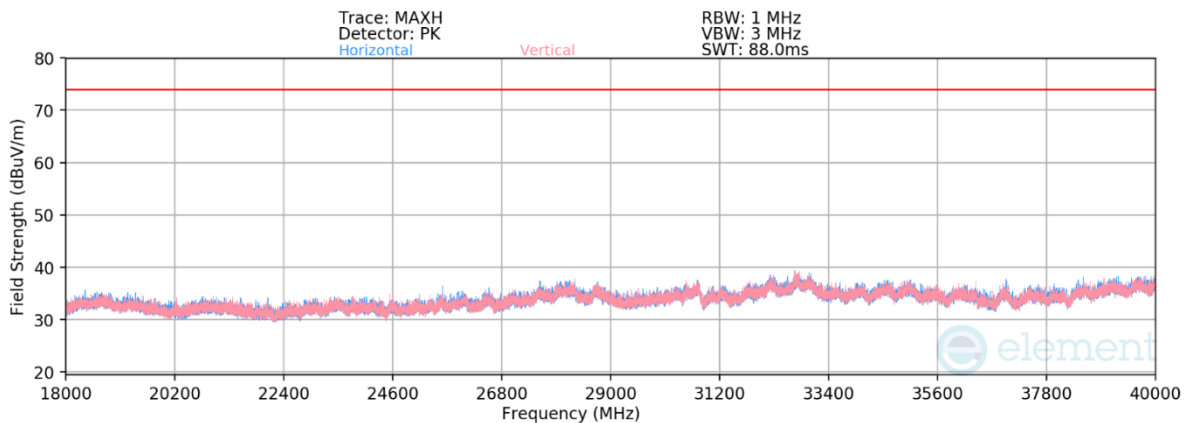
Plot 7-35. Radiated Spurious Emissions Above 18GHz Antenna 1 Common (802.15.4 ePA – Ch. 18)
