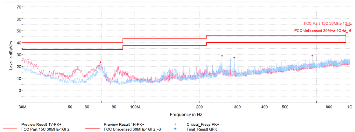
Plot 7-41. Radiated Spurious Emissions 30MHz-1GHz Antenna 1 Dedicated (ePA - Ch.18, with AC/DC Adapter)
