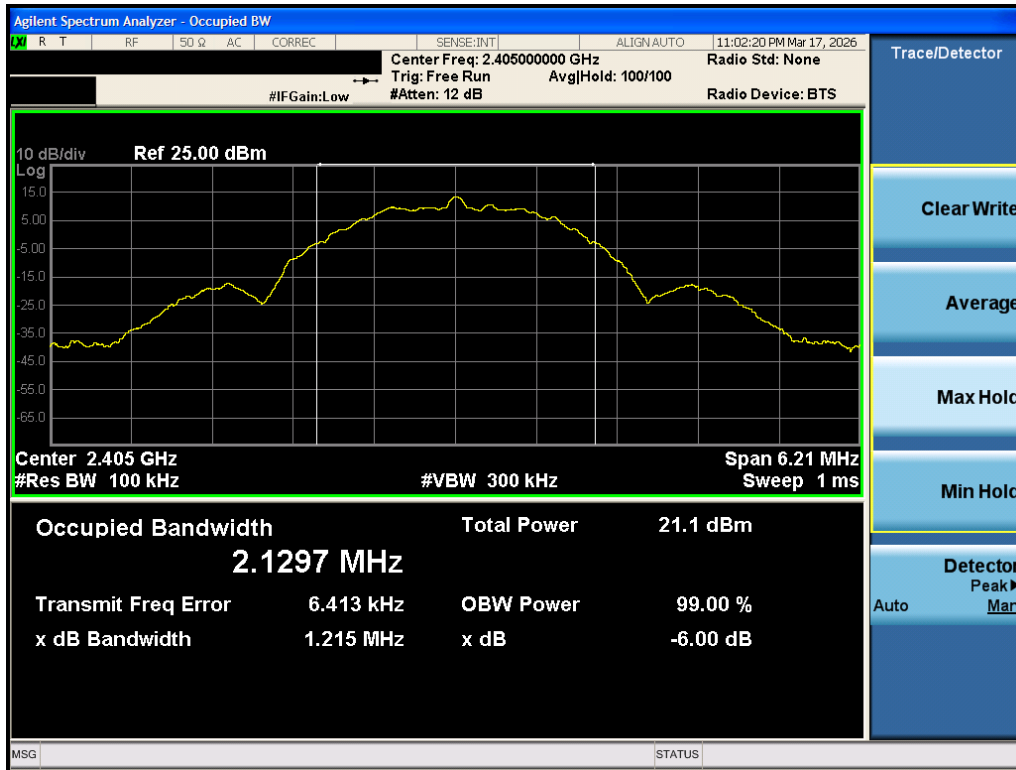
Plot 7-10. 6dB BW Antenna 1 Common (802.15.4, Ch. 11)
