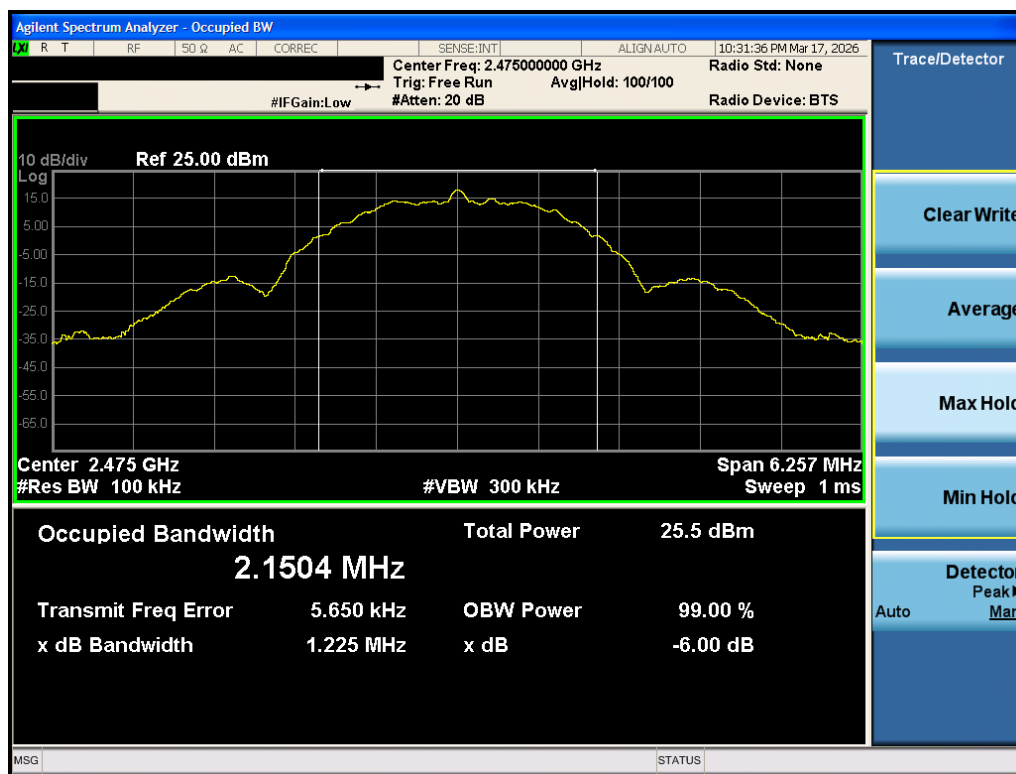
Plot 7-9. 6dB BW Antenna 1 Dedicated (802.15.4, Ch. 25)
