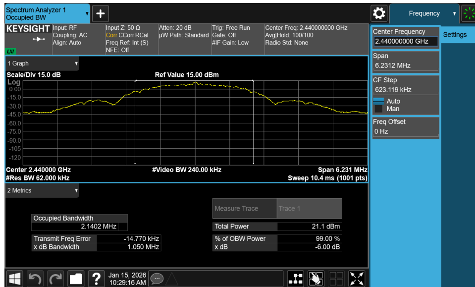
Plot 7-5. 99% OBW Antenna 1 Common (802.15.4, Ch. 18)
