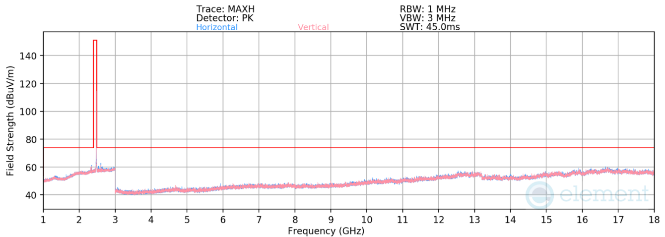
Plot 7-32. Radiated Spurious Emissions 1-18GHz Antenna 1 Dedicated (802.15.4 ePA – Ch. 25)
