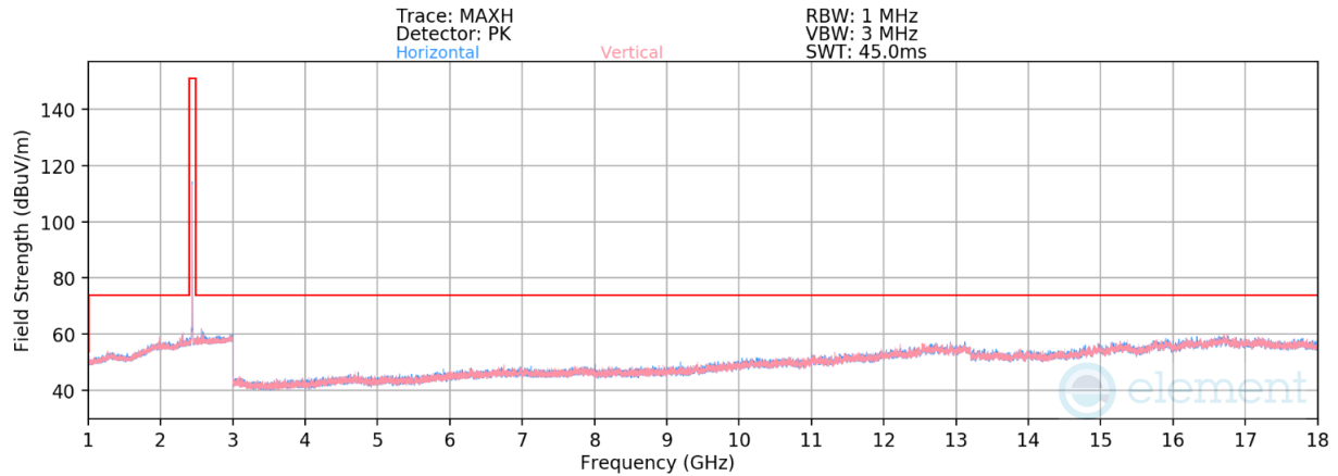
Plot 7-30. Radiated Spurious Emissions 1-18GHz Antenna 1 Dedicated (802.15.4 ePA – Ch. 18)
