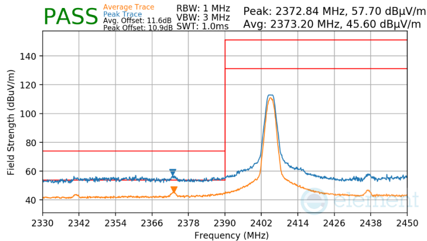
Plot 7-37. Radiated Restricted Lower Band Edge Measurement Antenna 1 Dedicated
