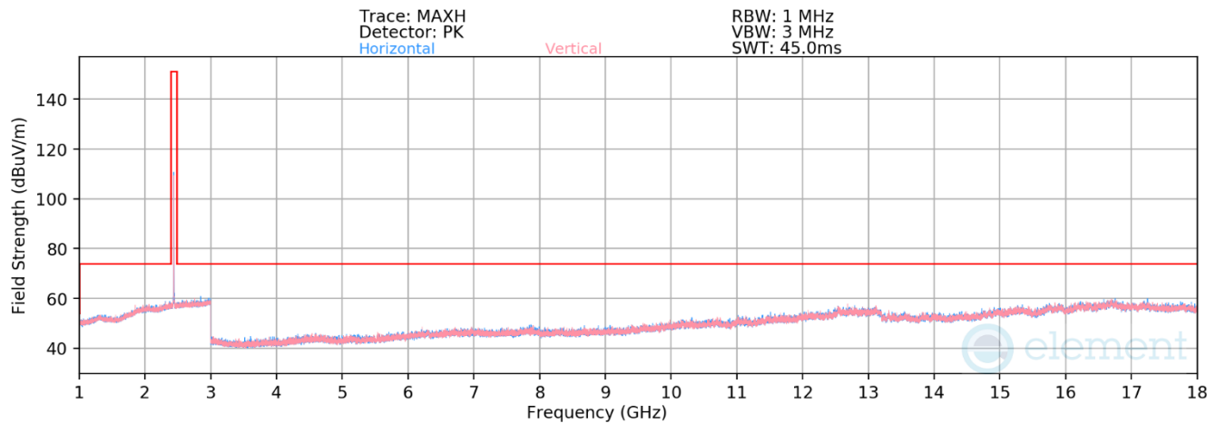
Plot 7-34. Radiated Spurious Emissions 1-18GHz Antenna 1 Common (802.15.4 ePA – Ch. 18)
