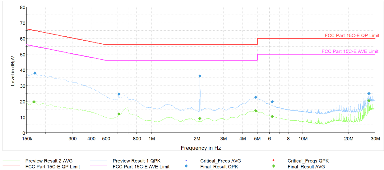
Plot 7-42. AC Line Conducted Emission with 802.15.4 Antenna 1 Dedicated (L1, Ch.18 - ePA, with AC/DC Adapter)
