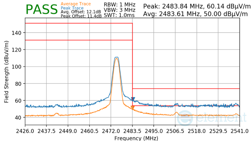
Plot 7-40. Radiated Restricted Upper Band Edge Measurement Antenna 1 Common
