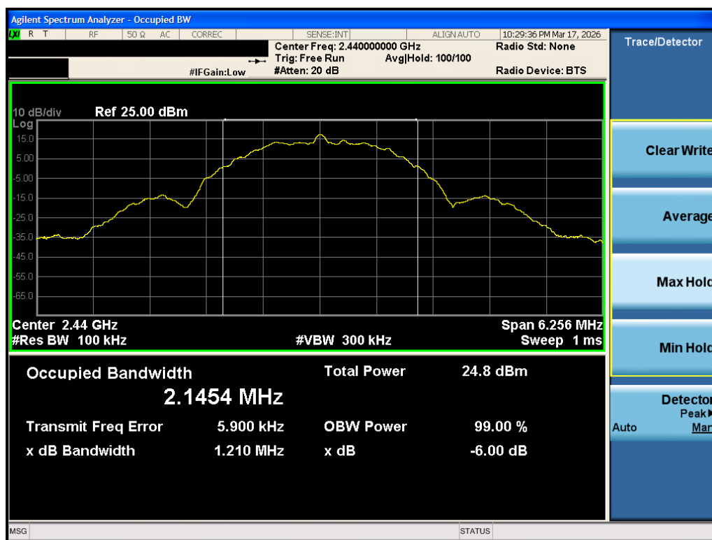
Plot 7-8. 6dB BW Antenna 1 Dedicated (802.15.4, Ch. 18)
