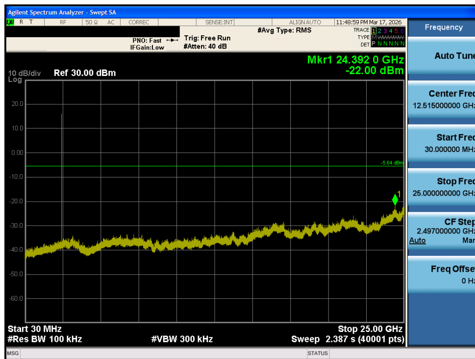
Plot 7-24. Conducted Spurious Antenna 1 Dedicated (802.15.4, ePA – Ch. 18)
