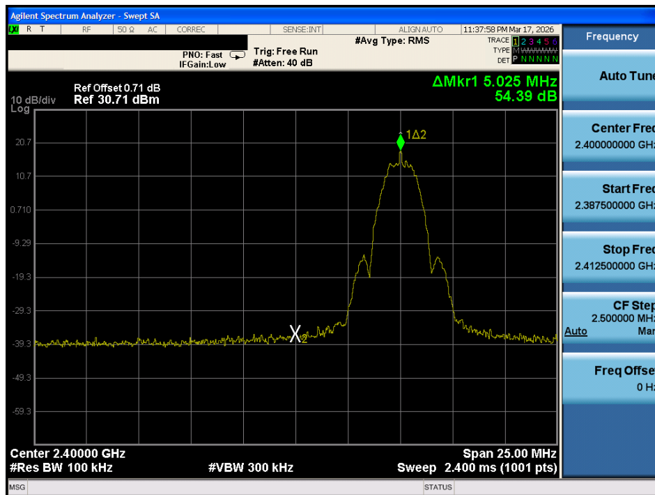
Plot 7-19. Band Edge Antenna 1 Dedicated (802.15.4, ePA – Ch. 11)
