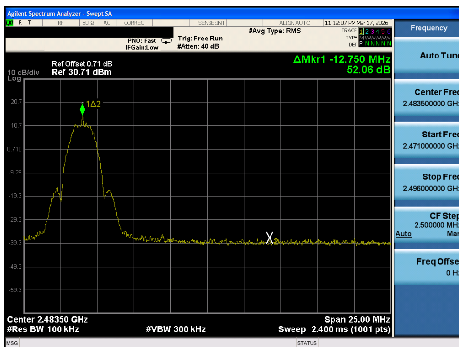
Plot 7-22. Band Edge Antenna 1 Common (802.15.4, ePA – Ch. 25)
