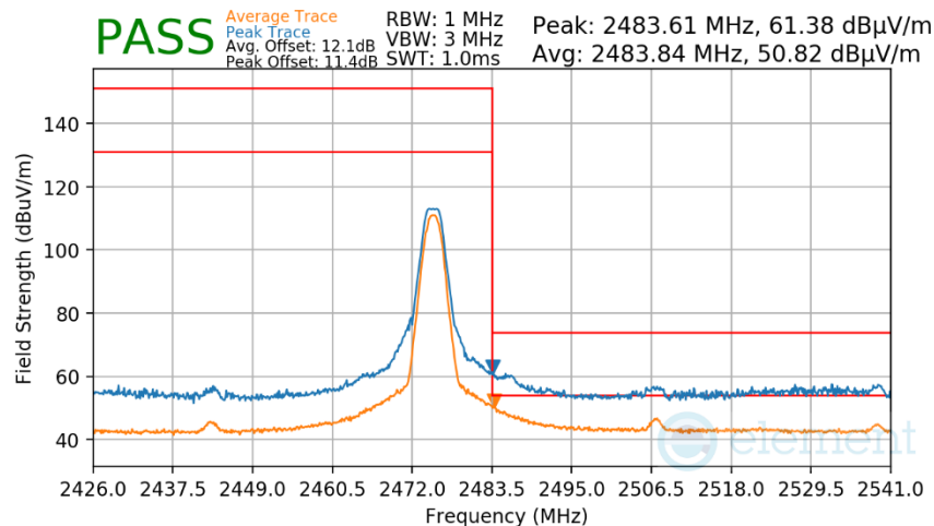
Plot 7-38. Radiated Restricted Upper Band Edge Measurement Antenna 1 Dedicated
