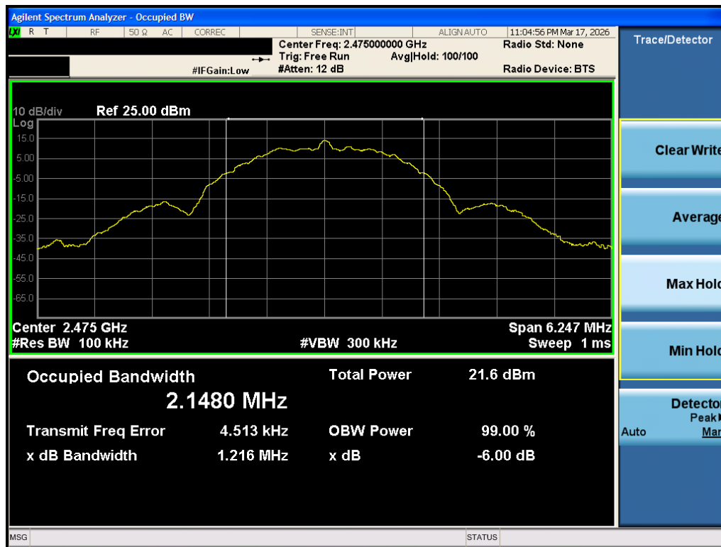
Plot 7-12. 6dB BW Antenna 1 Common(802.15.4, Ch. 25)
