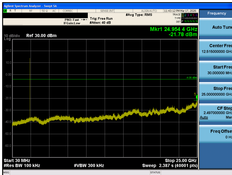
Plot 7-23. Conducted Spurious Antenna 1 Dedicated (802.15.4, ePA – Ch. 11)
