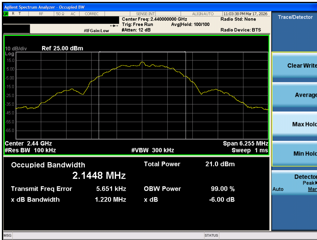
Plot 7-11. 6dB BW Antenna 1 Common (802.15.4, Ch. 18)
