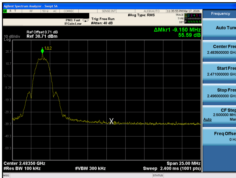
Plot 7-20. Band Edge Antenna 1 Dedicated (802.15.4, ePA – Ch. 25)
