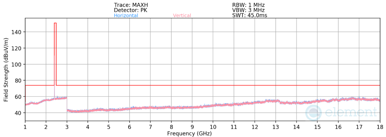
Plot 7-29. Radiated Spurious Emissions 1-18GHz Antenna 1 Dedicated (802.15.4 ePA – Ch. 11)
