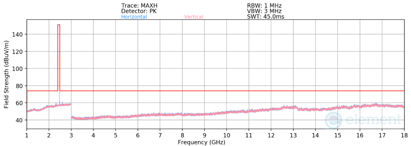
Plot 7-36. Radiated Spurious Emissions 1-18GHz Antenna 1 Common (802.15.4 ePA – Ch. 25)
