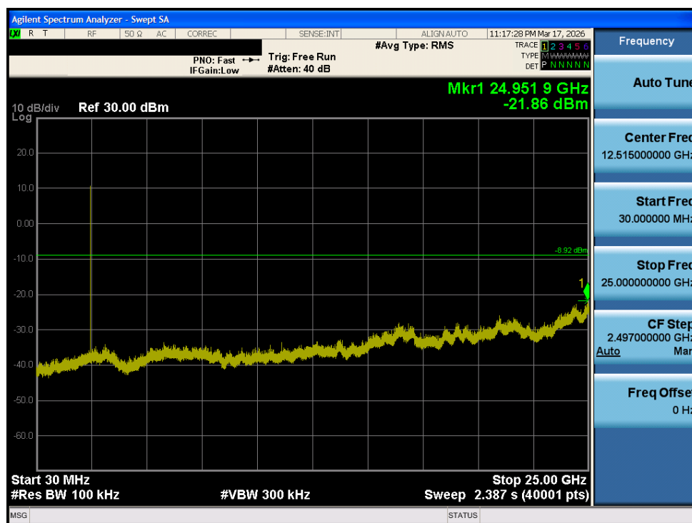
Plot 7-28. Conducted Spurious Antenna 1 Common (802.15.4, ePA – Ch. 25)
