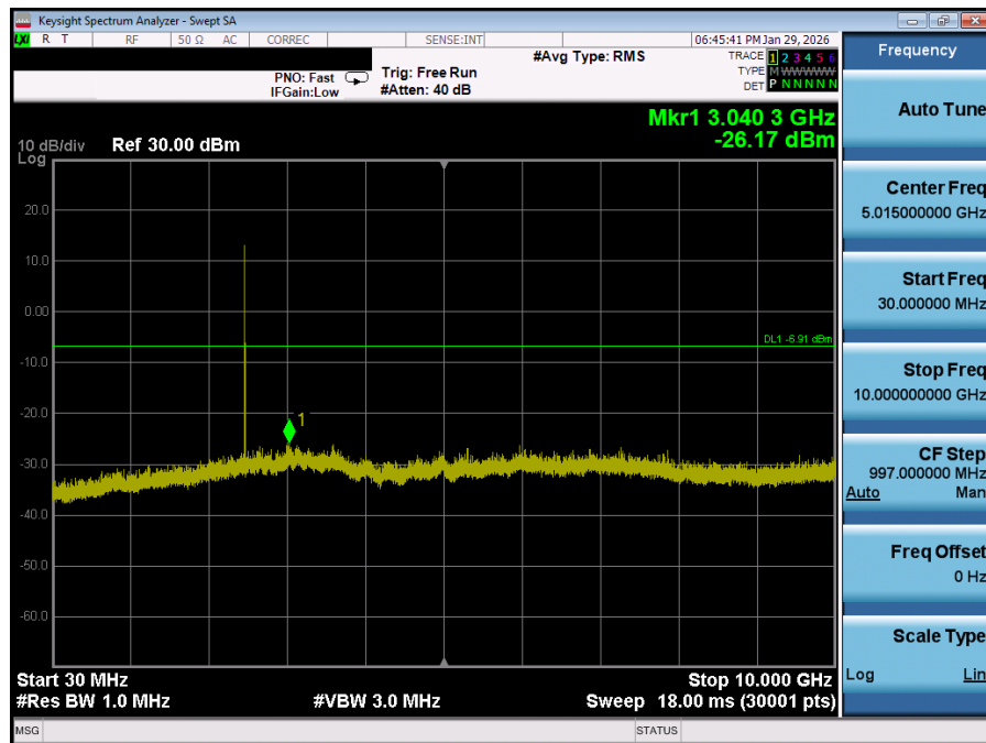
Plot 7-33. Conducted Spurious Plot Antenna 0 (Bluetooth (LE), 2Mbps, iPA – Ch. 36)
