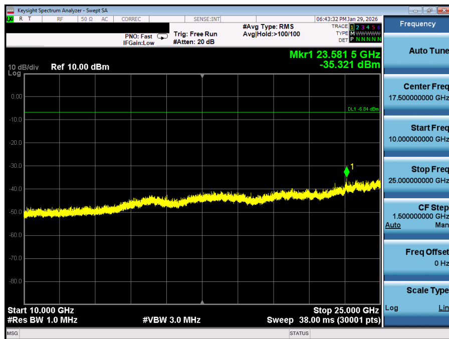
Plot 7-30. Conducted Spurious Plot Antenna 0 (Bluetooth (LE), 2Mbps, iPA – Ch. 0)
