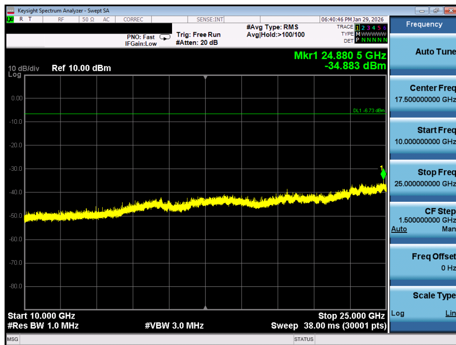
Plot 7-26. Conducted Spurious Plot Antenna 0 (Bluetooth (LE), 1Mbps, iPA – Ch. 17)
