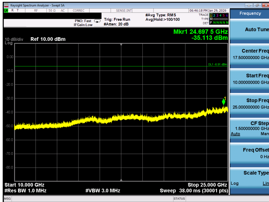
Plot 7-34. Conducted Spurious Plot Antenna 0 (Bluetooth (LE), 2Mbps, iPA – Ch. 36)
