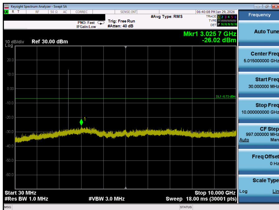
Plot 7-25. Conducted Spurious Plot Antenna 0 (Bluetooth (LE), 1Mbps, iPA – Ch. 17)
