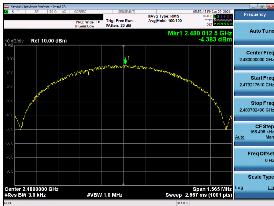
Plot 7-15. Power Spectral Density Plot Antenna 0 (Bluetooth (LE), 1Mbps, iPA – Ch. 39)
