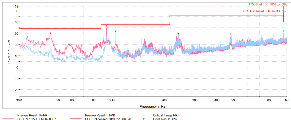
Plot 7-43. Radiated Spurious Emissions Below 1GHz Antenna 0 (1Mbps – Ch.39, iPA, Pol. H & V, with AC/DC Adapter)
