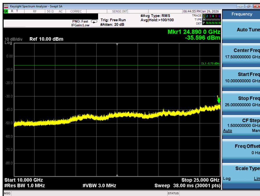
Plot 7-32. Conducted Spurious Plot Antenna 0 (Bluetooth (LE), 2Mbps, iPA – Ch. 17)
