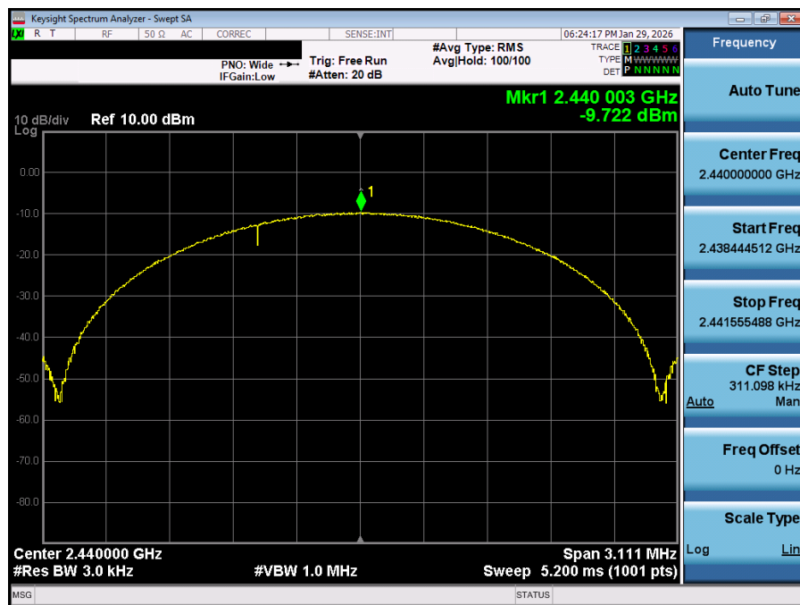
Plot 7-17. Power Spectral Density Plot Antenna 0 (Bluetooth (LE), 2Mbps, iPA – Ch. 17)
