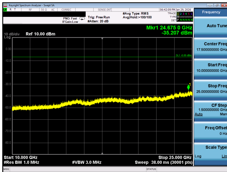
Plot 7-28. Conducted Spurious Plot Antenna 0 (Bluetooth (LE), 1Mbps, iPA – Ch. 39)
