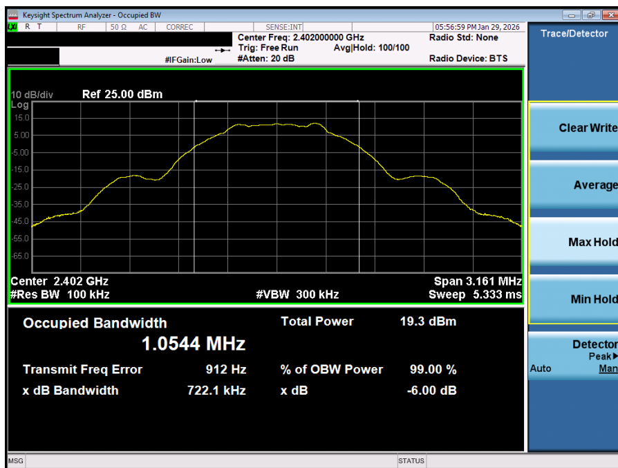
Plot 7-7. 6dB BW OBW Plot Antenna 0 (Bluetooth (LE), 1Mbps, iPA – Ch. 37)
