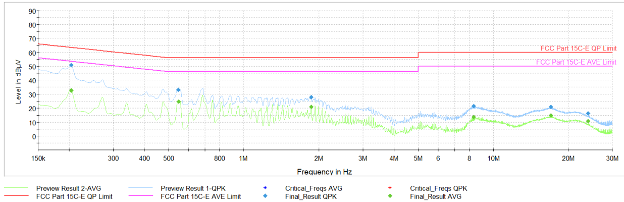
Plot 7-44. AC Line Conducted Plot with Bluetooth LE Antenna 0 (L1, 1Mbps iPA – Ch.39 with AC/DC Adapter)
