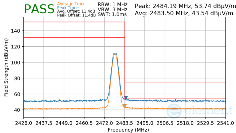
Plot 7-42. Radiated Restricted Upper Band Edge Measurement Antenna 0 (Average & Peak)
