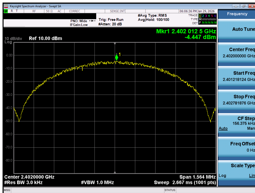
Plot 7-13. Power Spectral Density Plot Antenna 0 (Bluetooth (LE), 1Mbps, iPA – Ch. 37)
