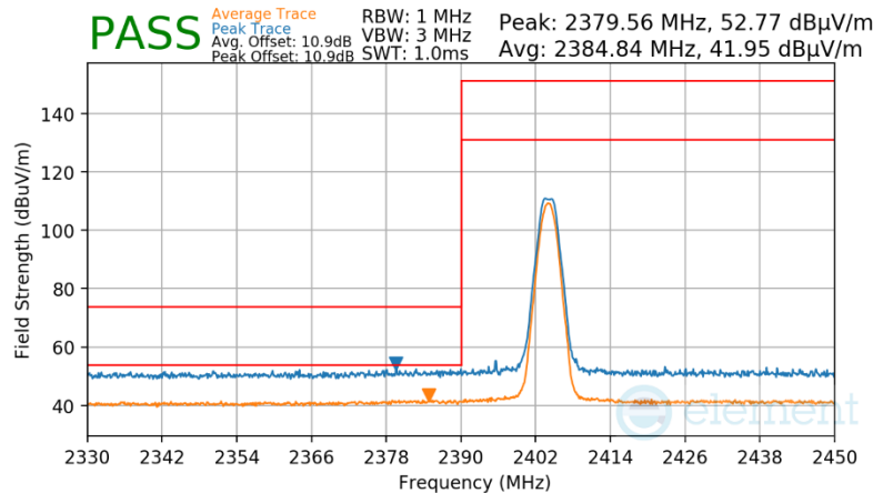
Plot 7-41. Radiated Restricted Lower Band Edge Measurement Antenna 0 (Average & Peak)
