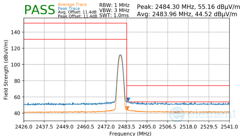
Plot 7-40. Radiated Restricted Upper Band Edge Measurement Antenna 0 (Average & Peak)
