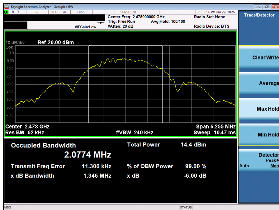
Plot 7-6. 99% OBW Plot Antenna 0 (Bluetooth (LE), 2Mbps, iPA – Ch. 36)
