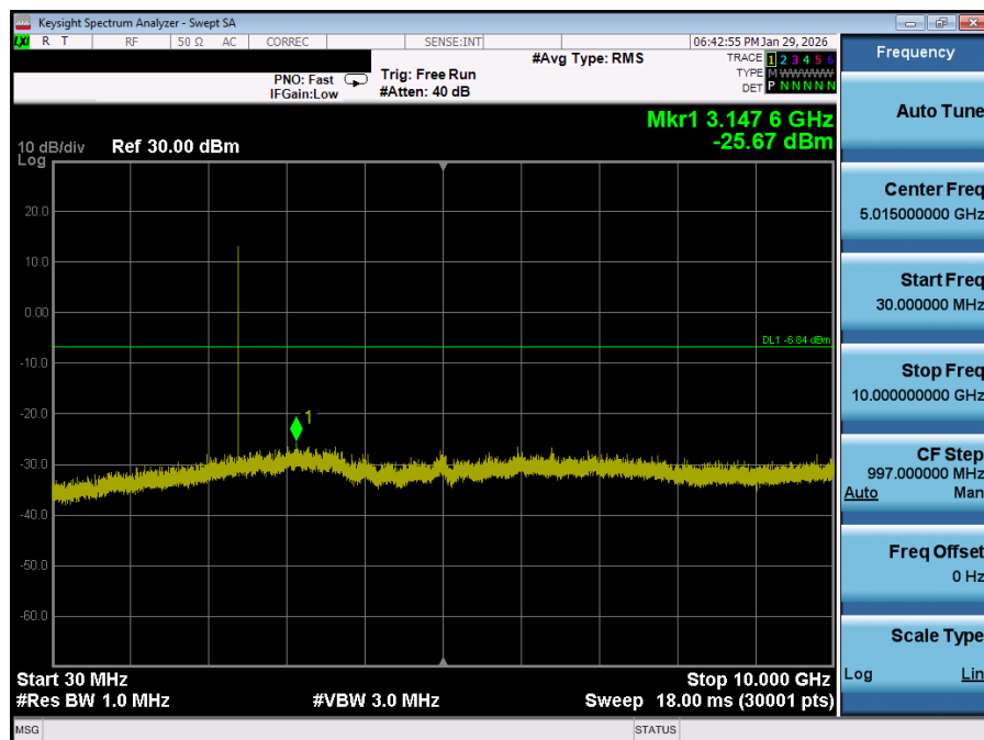
Plot 7-29. Conducted Spurious Plot Antenna 0 (Bluetooth (LE), 2Mbps, iPA – Ch. 0)
