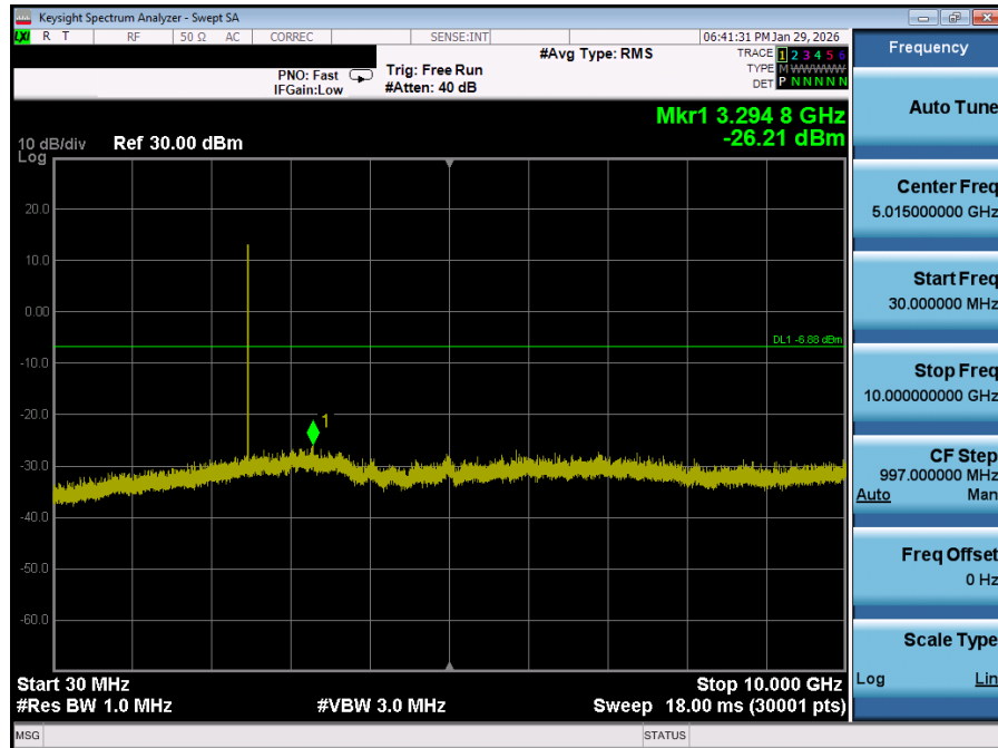
Plot 7-27. Conducted Spurious Plot Antenna 0 (Bluetooth (LE), 1Mbps, iPA – Ch. 39)
