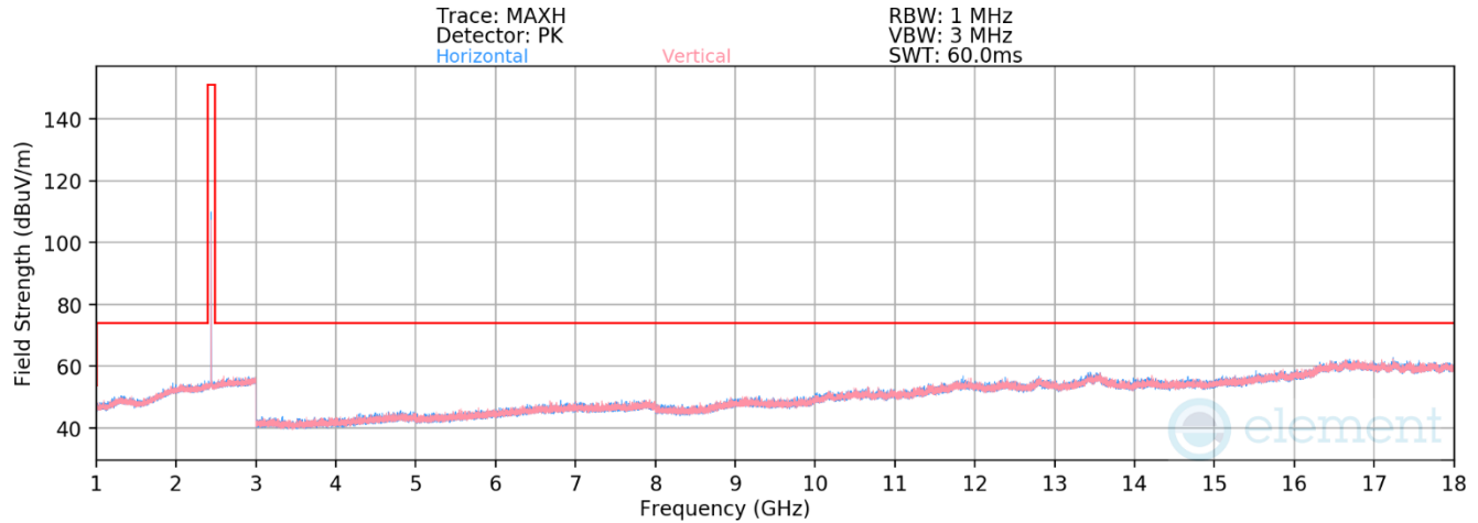
Plot 7-36. Radiated Spurious Emissions 1-18GHz Antenna 0 (1Mbps, iPA – Ch. 17)
