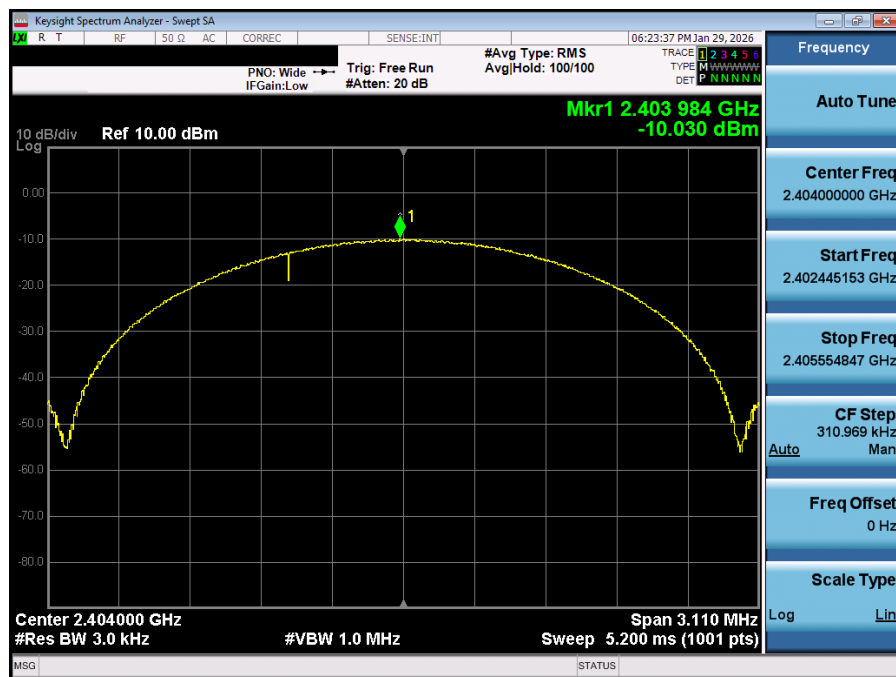
Plot 7-16. Power Spectral Density Plot Antenna 0 (Bluetooth (LE), 2Mbps, iPA – Ch. 0)
