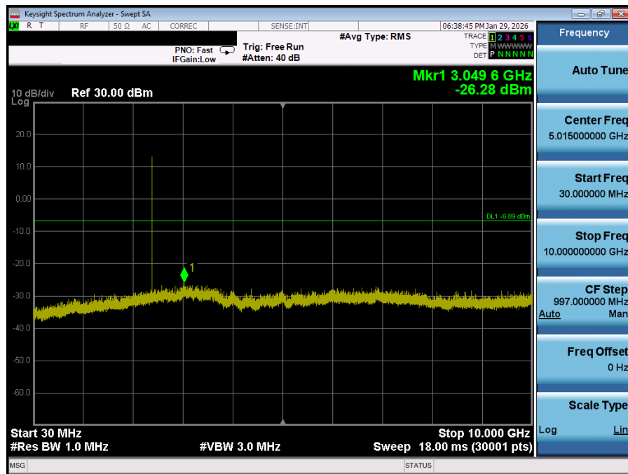
Plot 7-23. Conducted Spurious Plot Antenna 0 (Bluetooth (LE), 1Mbps, iPA – Ch. 37)
