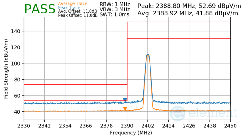
Plot 7-39. Radiated Restricted Lower Band Edge Measurement Antenna 0 (Average & Peak)
