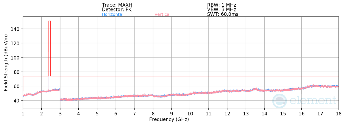
Plot 7-35. Radiated Spurious Emissions 1-18GHz Antenna 0 (1Mbps, iPA - Ch. 37)
