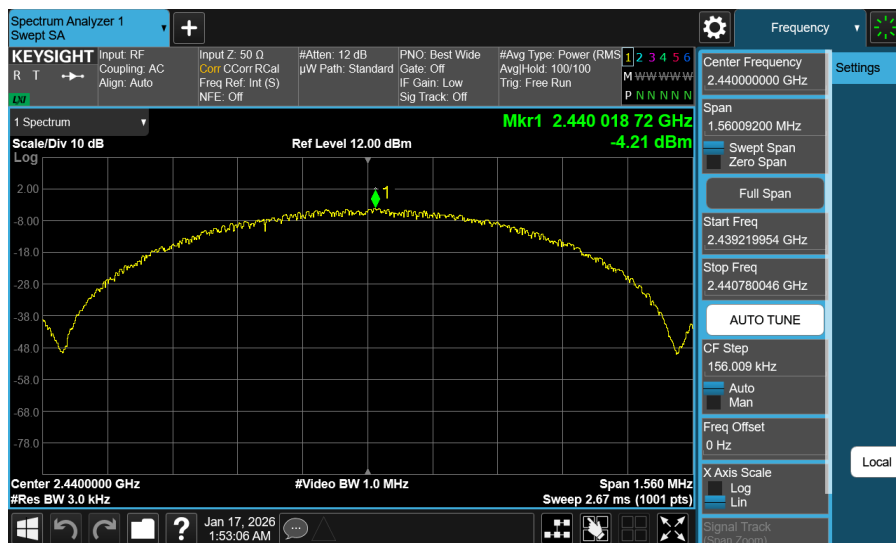
Plot 7-14. Power Spectral Density Plot Antenna 0 (Bluetooth (LE), 1Mbps, iPA – Ch. 17)
