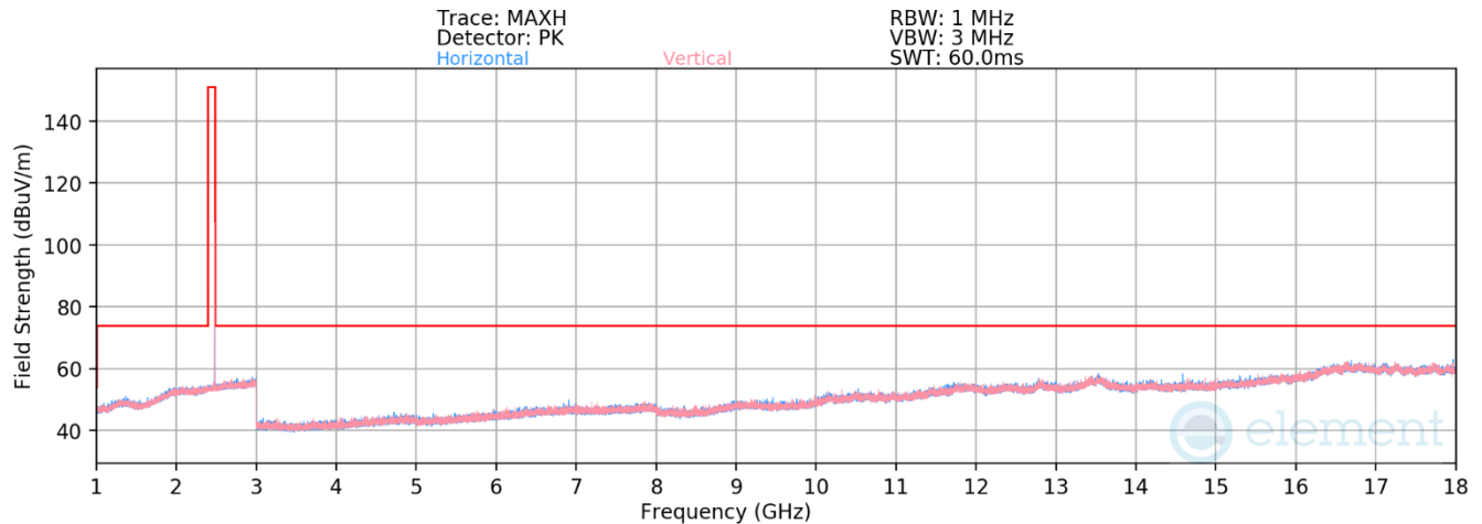
Plot 7-37. Radiated Spurious Emissions 1-18GHz Antenna 0 (1Mbps, iPA – Ch. 39)
