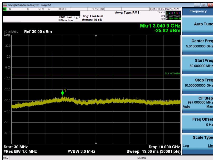
Plot 7-31. Conducted Spurious Plot Antenna 0 (Bluetooth (LE), 2Mbps, iPA – Ch. 17)
