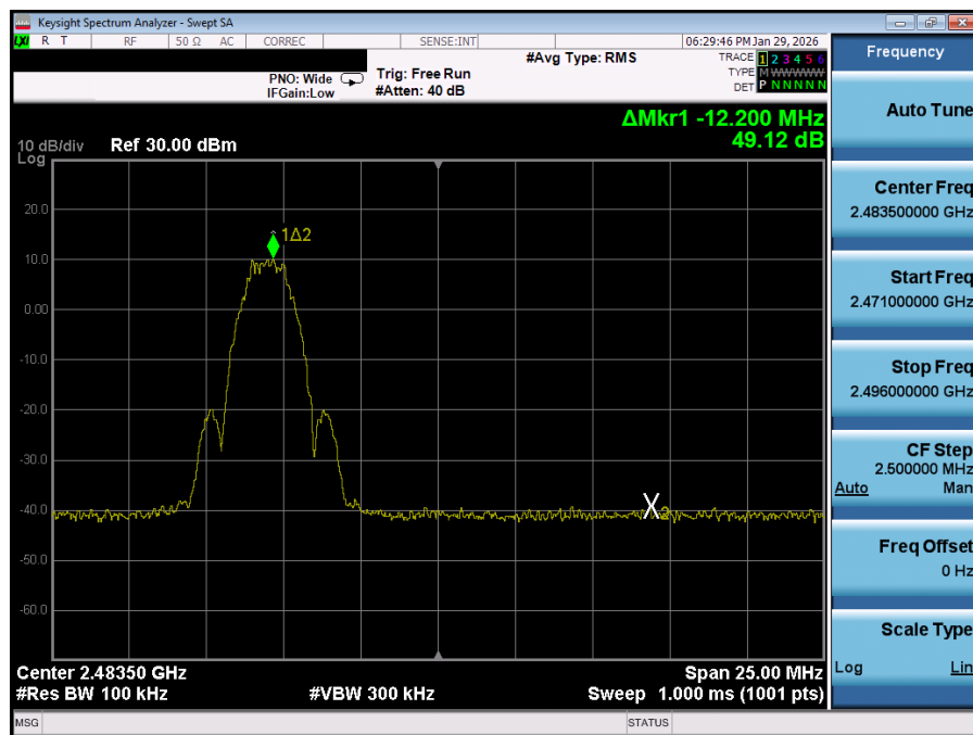
Plot 7-22. Band Edge Plot Antenna 0 (Bluetooth (LE), 2Mbps, iPA – Ch. 36)
