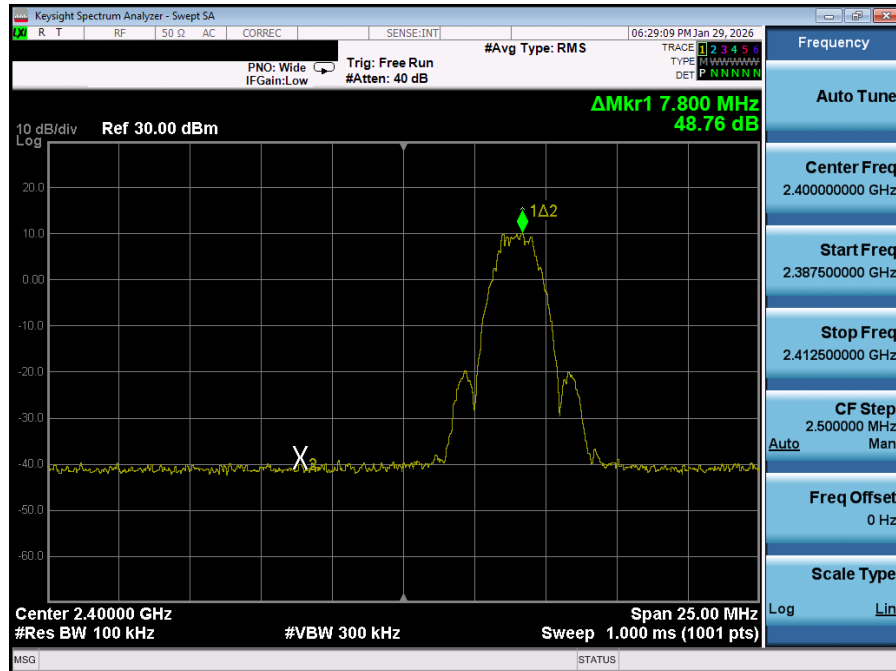
Plot 7-21. Band Edge Plot Antenna 0 (Bluetooth (LE), 2Mbps, iPA – Ch. 0)
