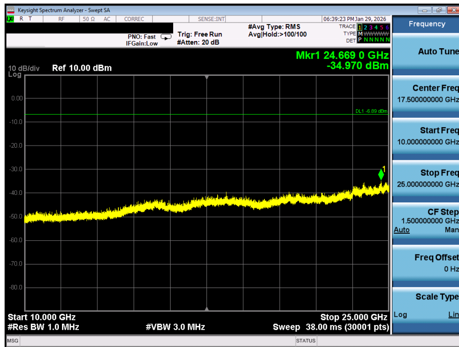
Plot 7-24. Conducted Spurious Plot Antenna 0 (Bluetooth (LE), 1Mbps, iPA – Ch. 37)
