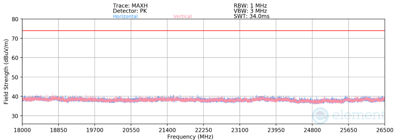
Plot 7-38. Radiated Spurious Emissions Above 18GHz Antenna 0 (1Mbps, iPA – Ch. 39)
