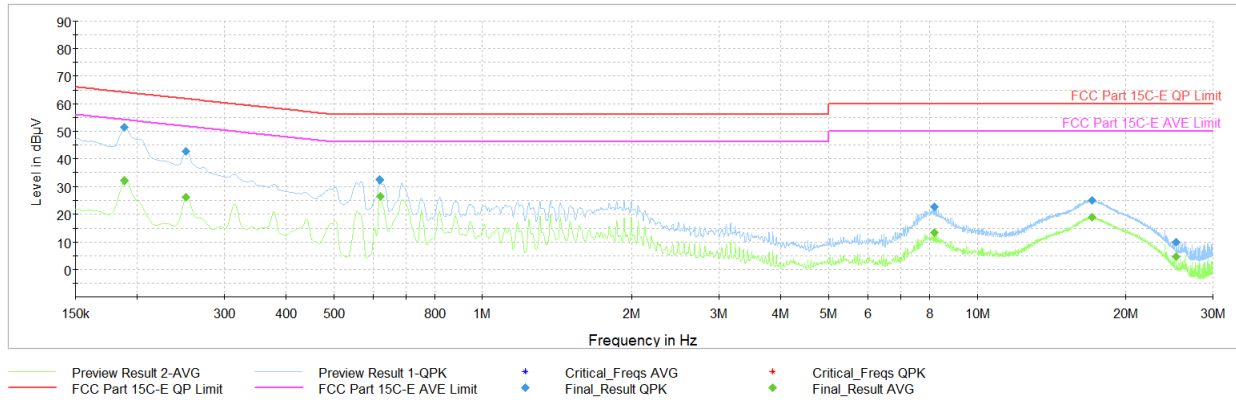
Plot 7-45. AC Line Conducted Plot with Bluetooth LE Antenna 0 (N, 1Mbps iPA – Ch.39, with AC/DC Adapter)
