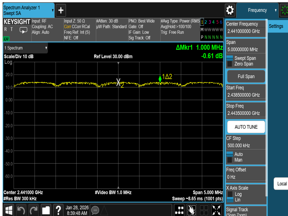
Plot 7-8. Channel Spacing Plot Antenna 0 (Bluetooth, 8DPSK, iPA)
