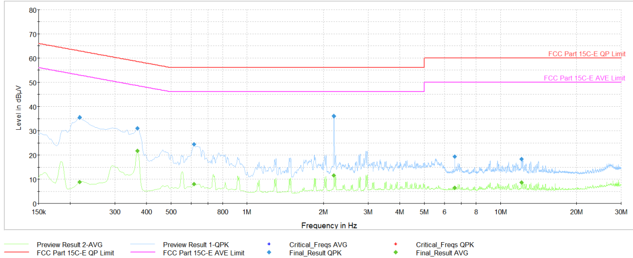
Plot 7-35. AC Line-Conducted Test Plot Antenna 0 (L1, GFSK iPA – Ch.39, with AC/DC adapter)
