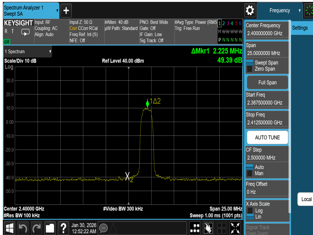
Plot 7-17. Band Edge Plot (Antenna 0) (Bluetooth with Hopping Disabled, 8DPSK, iPA – Ch. 0)
