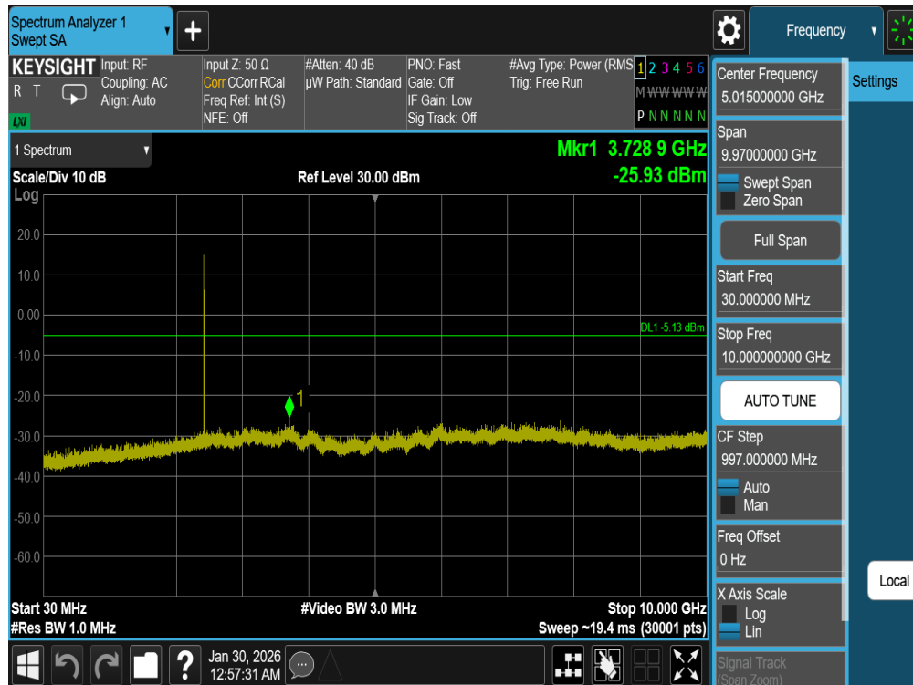
Plot 7-17. Conducted Spurious Plot Antenna 0 (Bluetooth, GFSK, iPA – Ch. 39)
