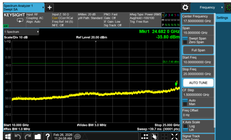
Plot 7-22. Conducted Spurious Plot – Simultaneous Transmission
