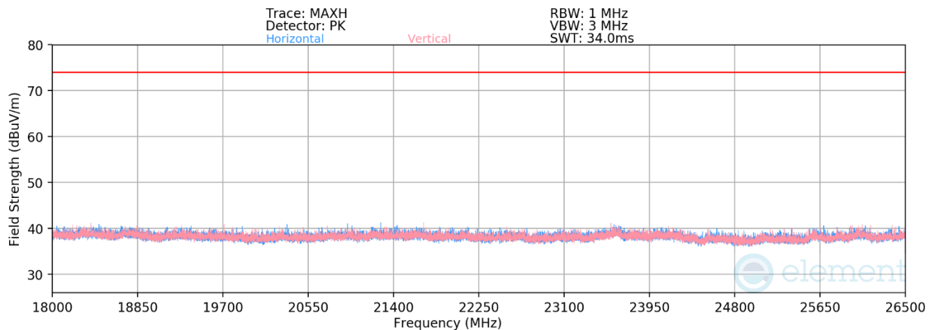
Plot 7-25. Radiated Spurious Emissions Above 18GHz (BT GFSK iPA – Ch. 39)
