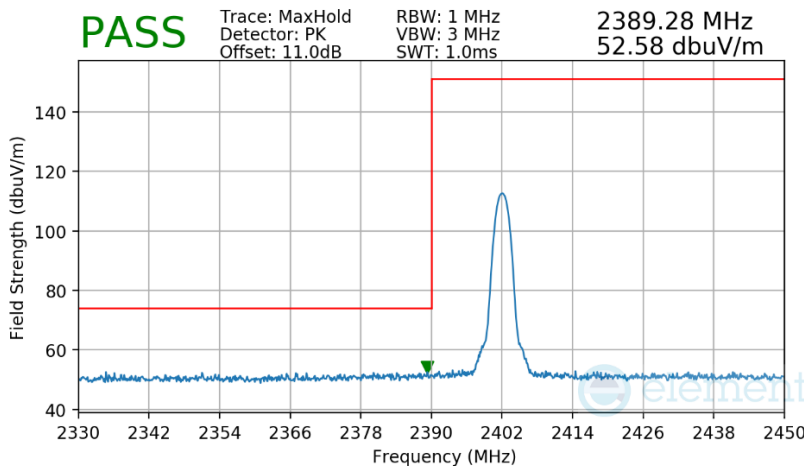
Plot 7-30. Radiated Restricted Lower Band Edge Measurement
