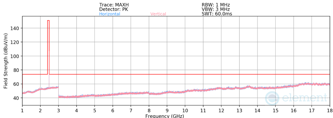
Plot 7-26. Radiated Spurious Emissions above 1GHz (BT GFSK iPA – Ch. 78)
