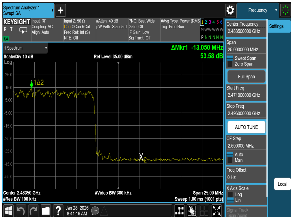
Plot 7-20. Band Edge Plot (Antenna 0) (Bluetooth with Hopping Enabled, 8DPSK, iPA – Ch. 78)
