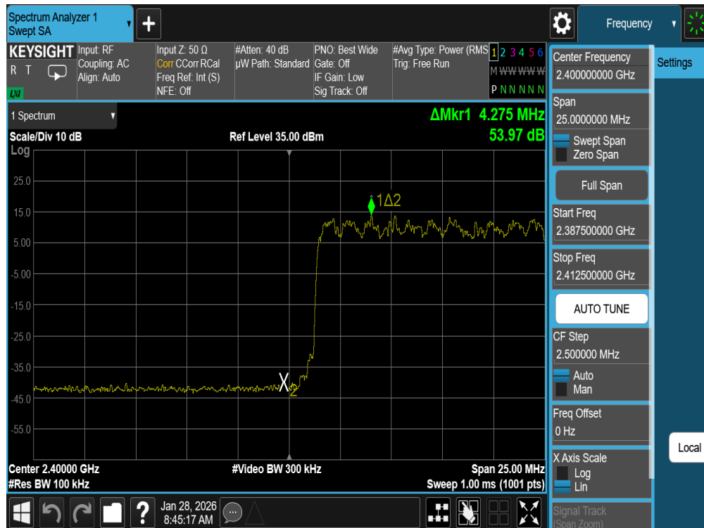
Plot 7-19. Band Edge Plot (Antenna 0) (Bluetooth with Hopping Enabled, 8DPSK, iPA – Ch. 0)
