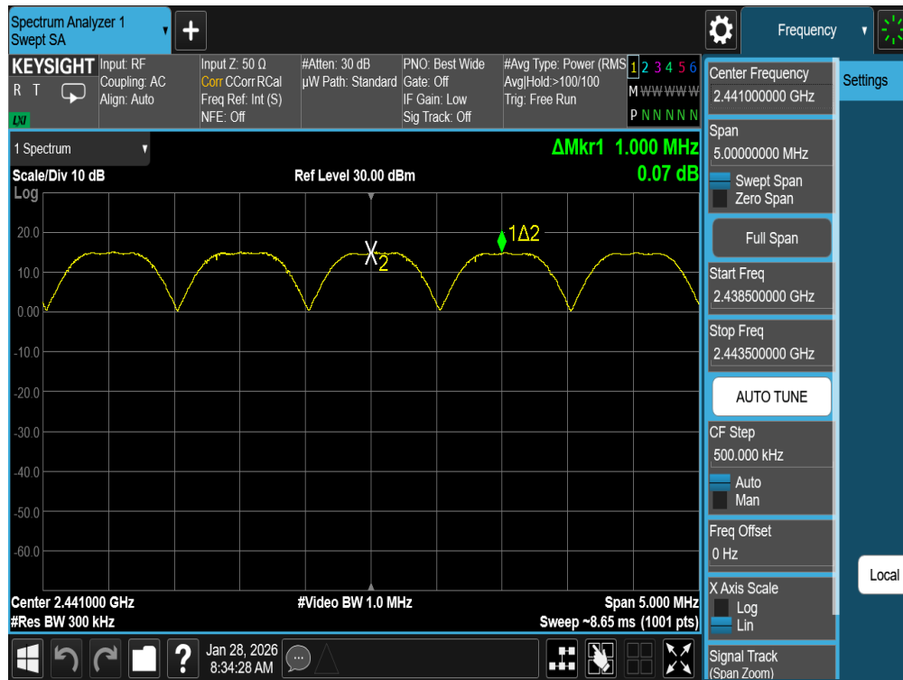
Plot 7-7. Channel Spacing Plot Antenna 0 (Bluetooth, GFSK, iPA)
