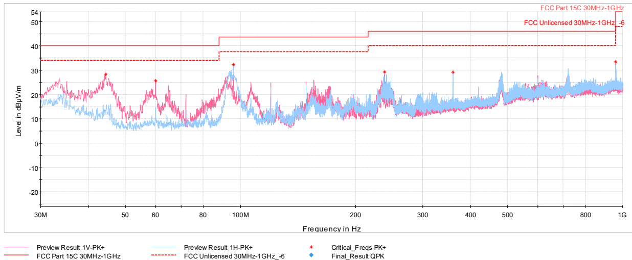
Plot 7-33. Radiated Spurious Emissions Below 1GHz Antenna 0 (GFSK iPA – Ch.0, with AC/DC Adapter)
