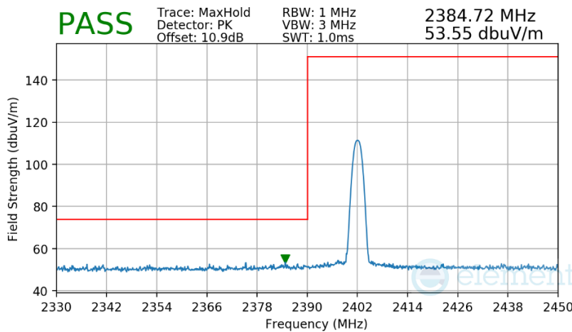
Plot 7-29. Radiated Restricted Lower Band Edge Measurement
