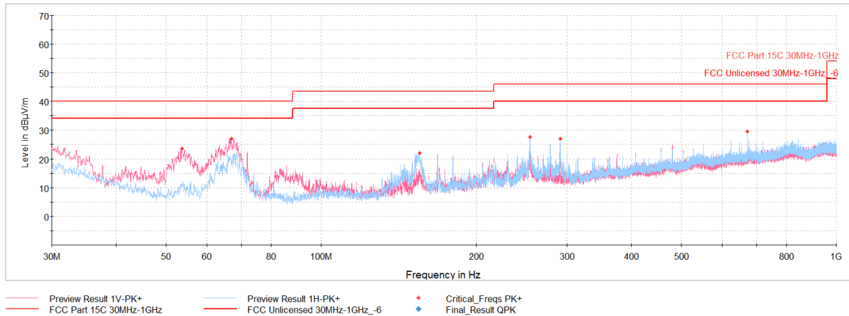
Plot 7-34. Radiated Spurious Emissions – Simultaneous Transmission 30MHz – 1GHz, with AC/DC Adapter)
