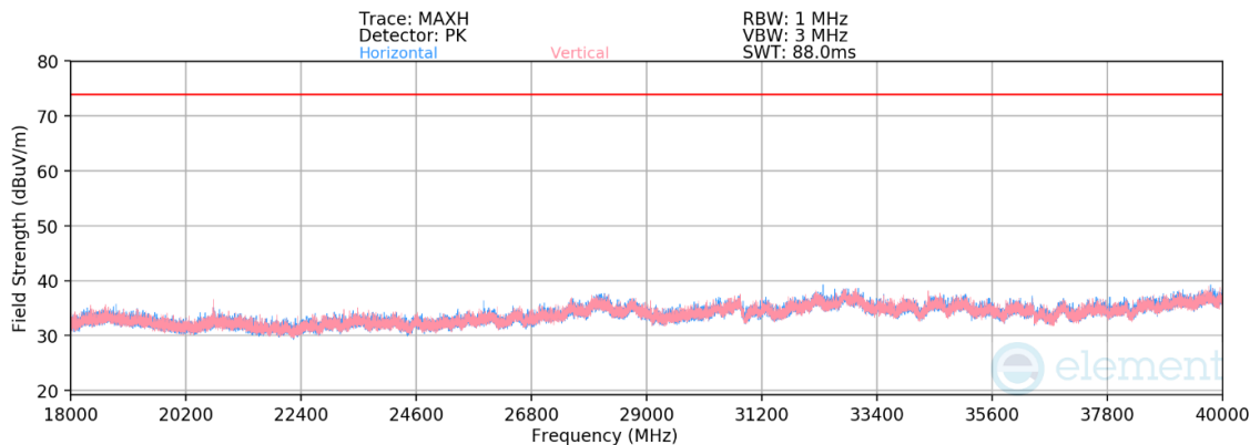
Plot 7-28. Radiated Spurious Emissions above 18GHz – Simultaneous Transmission
