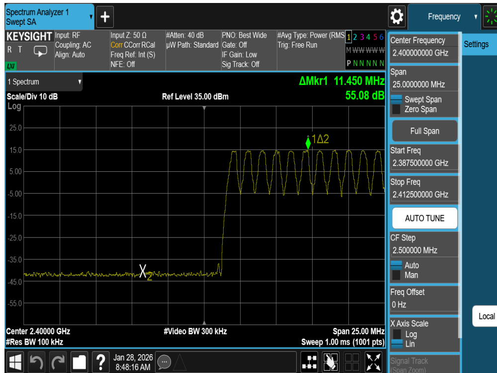
Plot 7-15. Band Edge Plot (Antenna 0) (Bluetooth with Hopping Enabled, GFSK, iPA – Ch.0)
