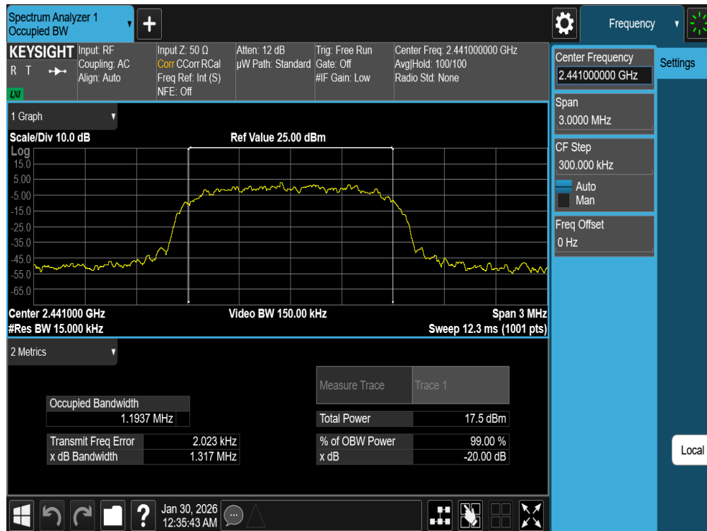
Plot 7-5. 20dB BW and 99% OBW Plot Antenna 0 (Bluetooth, 8DPSK, iPA – Ch. 39)
