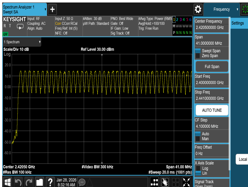
Plot 7-11. Low End Spectrum Channel Hopping Plot Antenna 0 (Bluetooth, GFSK, iPA)
