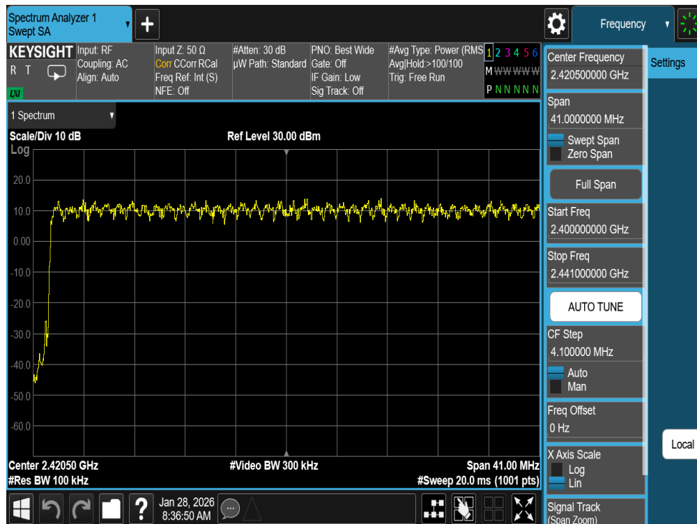
Plot 7-13. Low End Spectrum Channel Hopping Plot Antenna 0 (Bluetooth, 8DPSK, iPA)
