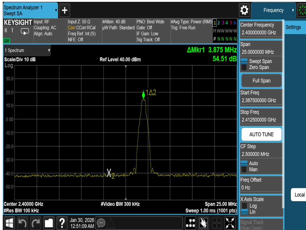
Plot 7-13. Band Edge Plot (Antenna 0) (Bluetooth with Hopping Disabled, GFSK, iPA – Ch.0)
