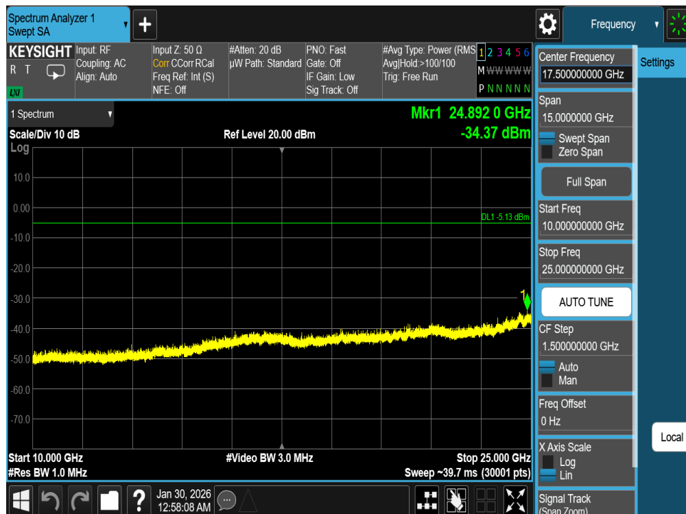
Plot 7-18. Conducted Spurious Plot Antenna 0 (Bluetooth, GFSK, iPA Ch. 39)
