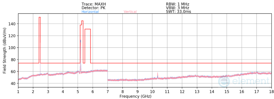
Plot 7-27. Radiated Spurious Emissions above 1GHz – Simultaneous Transmission
