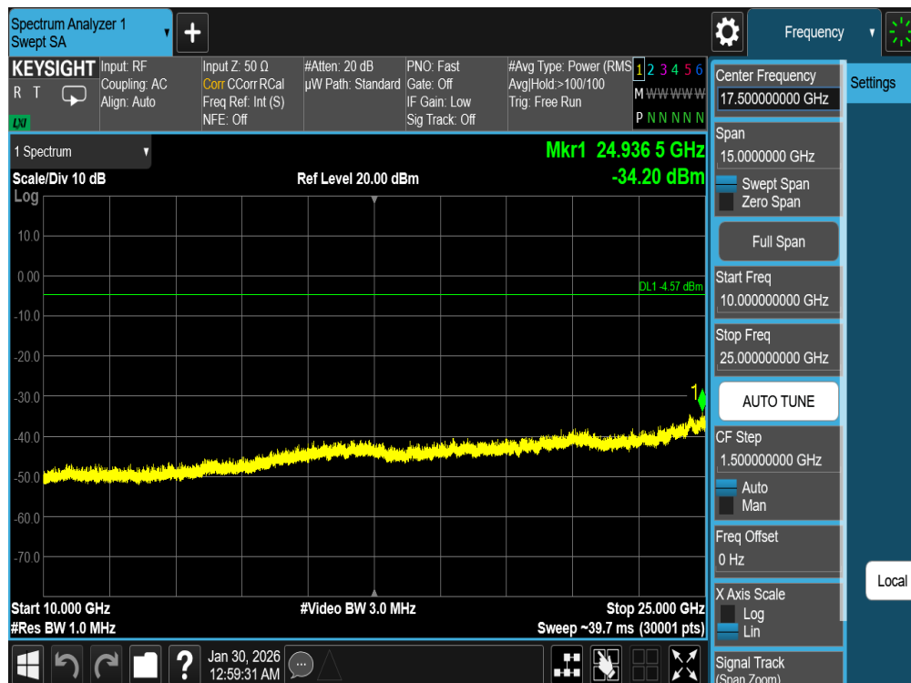
Plot 7-20. Conducted Spurious Plot Antenna 0 (Bluetooth, GFSK, iPA – Ch. 78)
