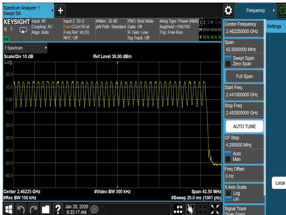
Plot 7-12. High End Spectrum Channel Hopping Plot Antenna 0 (Bluetooth, GFSK, iPA)
