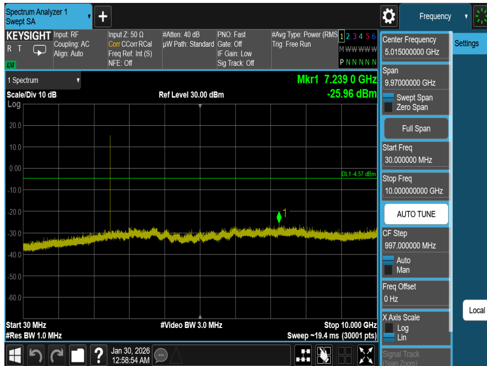
Plot 7-19. Conducted Spurious Plot Antenna 0 (Bluetooth, GFSK, iPA – Ch. 78)
