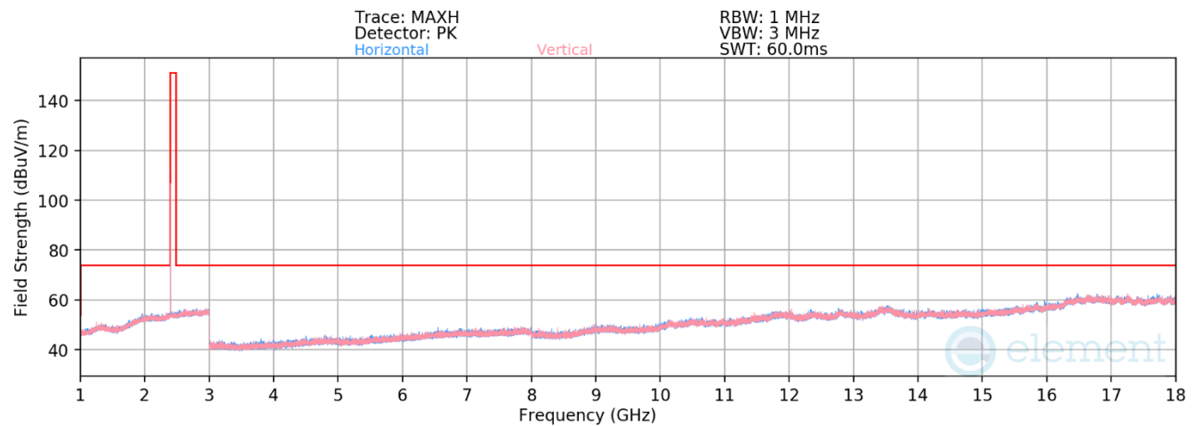
Plot 7-23. Radiated Spurious Emissions 1-18GHz (BT GFSK iPA – Ch. 0)
