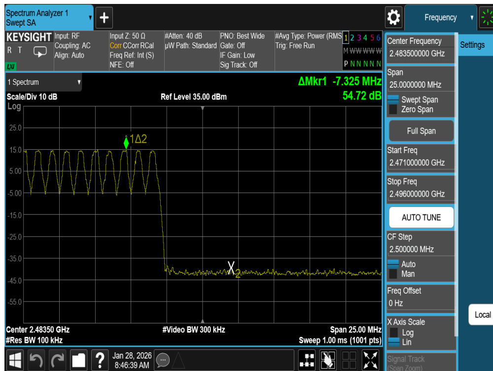
Plot 7-16. Band Edge Plot (Antenna 0) (Bluetooth with Hopping Enabled, GFSK, iPA – Ch.78)
