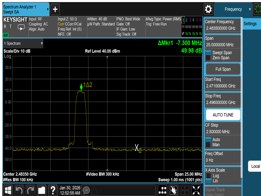
Plot 7-18. Band Edge Plot (Antenna 0) (Bluetooth with Hopping Disabled, 8DPSK, iPA – Ch. 78)
