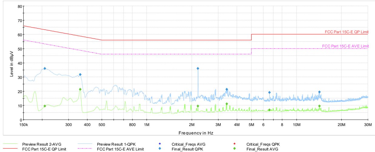
Plot 7-36. AC Line-Conducted Test Plot Antenna 0 (N, GFSK iPA – Ch.39, with AC/DC adapter)
