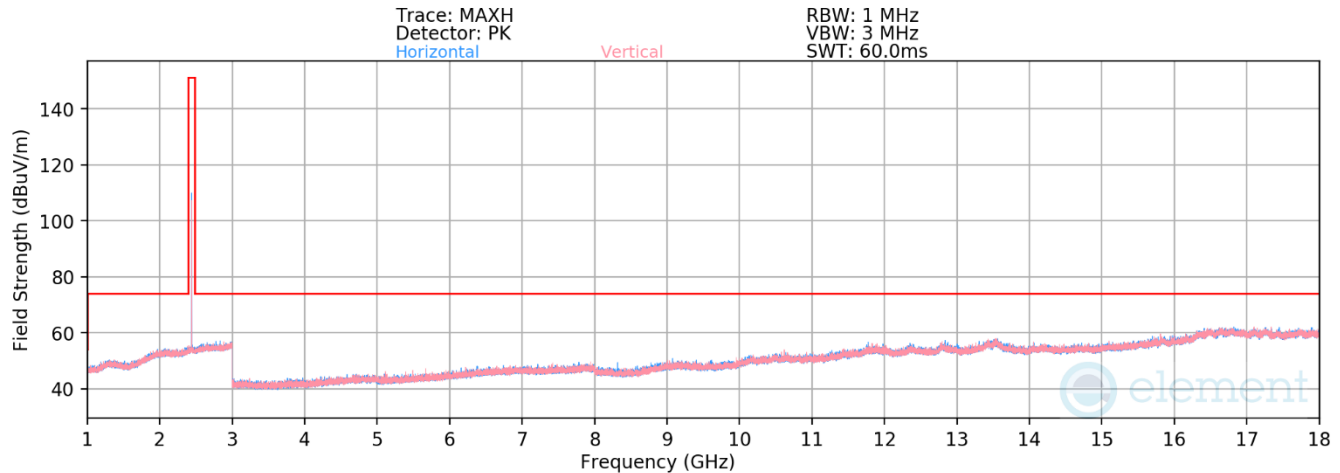
Plot 7-24. Radiated Spurious Emissions 1-18GHz (BT GFSK iPA – Ch. 39)
