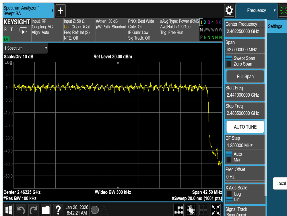
Plot 7-14. High End Spectrum Channel Hopping Plot Antenna 0 (Bluetooth, 8DPSK, iPA)
