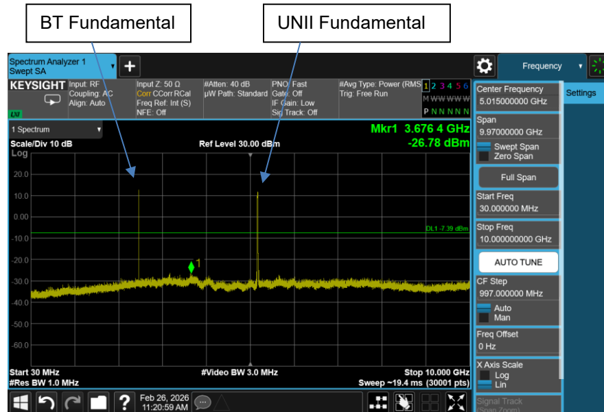
Plot 7-21. Conducted Spurious Plot – Simultaneous Transmission
