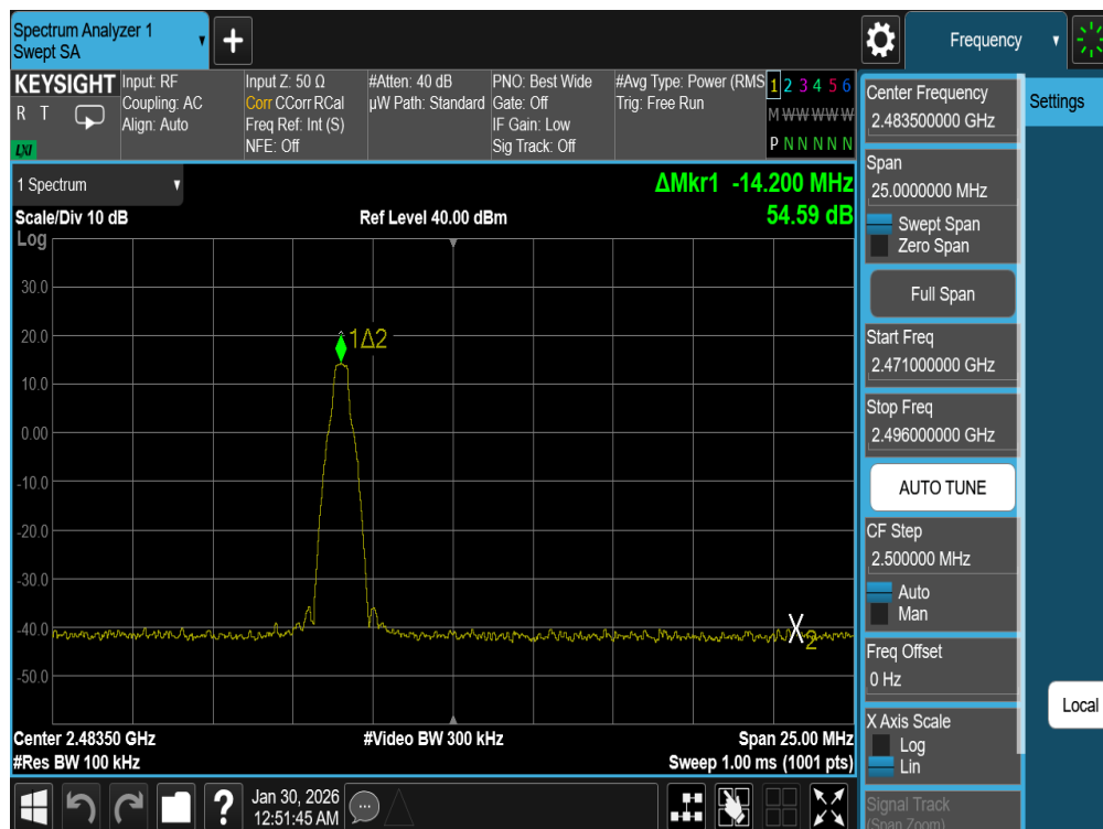
Plot 7-14. Band Edge Plot (Antenna 0) (Bluetooth with Hopping Disabled, GFSK, iPA – Ch.78)
